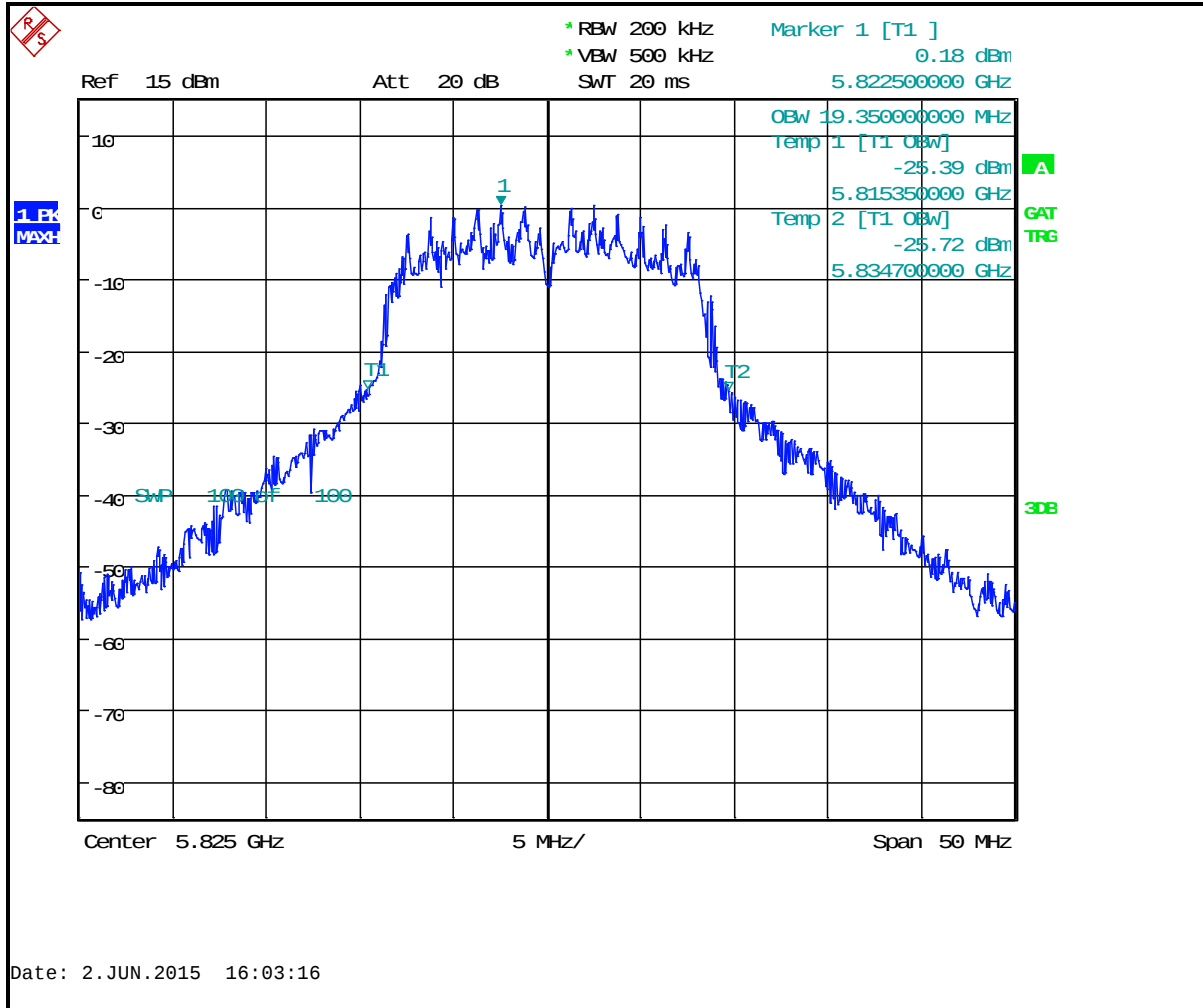
Plot 8-7: 26 dB Bandwidth Channel 165 (TX Frequency 5825 MHz) - 802.11a
