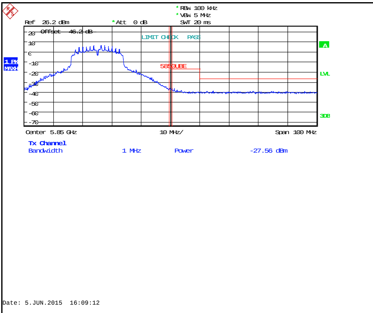
Plot 6-17: Upper Band Edge: Measurement Channel 165 (5825 MHz, 802.11a, Peak)
