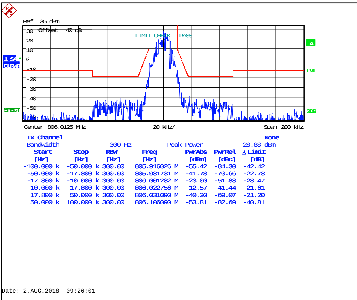
Plot 5-9: Occupied Bandwidth – HVD-TDMA NPSPAC; 806.0125 MHz; Mask G (ISED)
