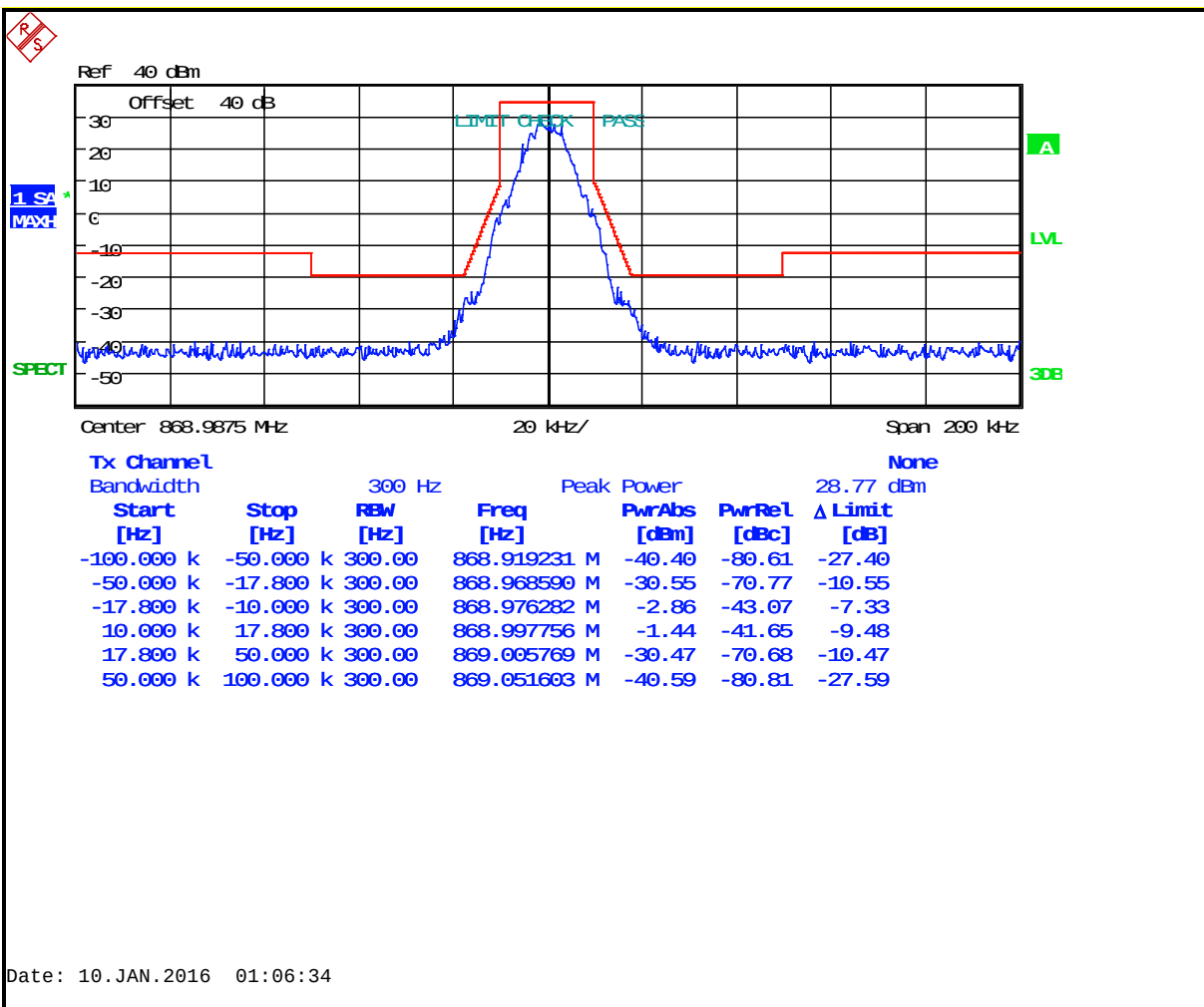
Plot 8-75: Occupied Bandwidth – 868.9875 MHz; OTP NPSPAC 4-level FSK (Mask G)
