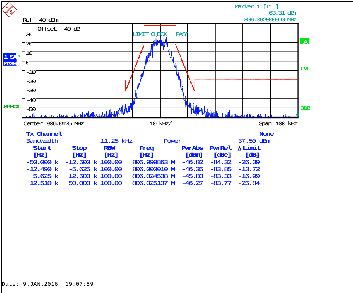
Plot 8-95: Occupied Bandwidth – 806.0125 MHz; C4FM Phase 2 (Mask D)
