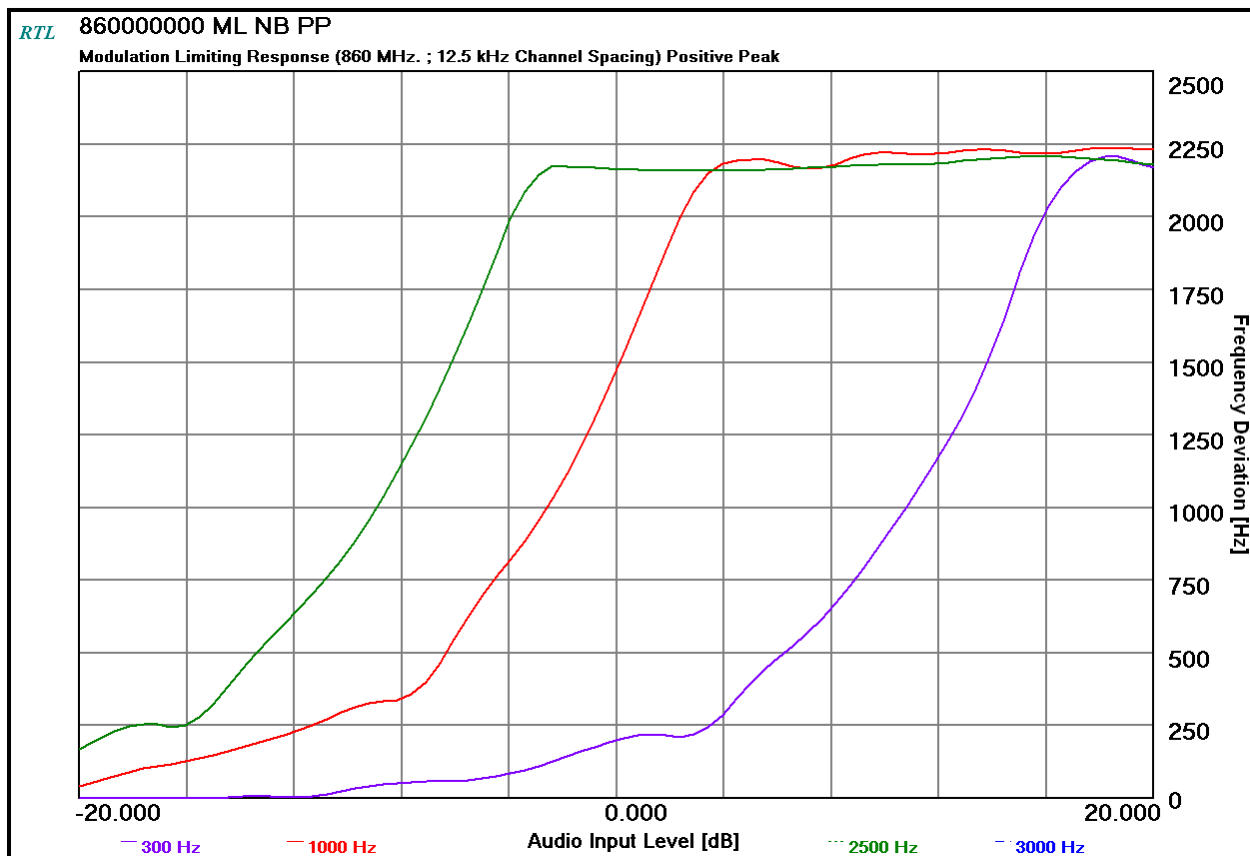
Plot 10-23: Modulation Characteristics – Modulation Limiting - 860 MHz; Positive Peak; NB
