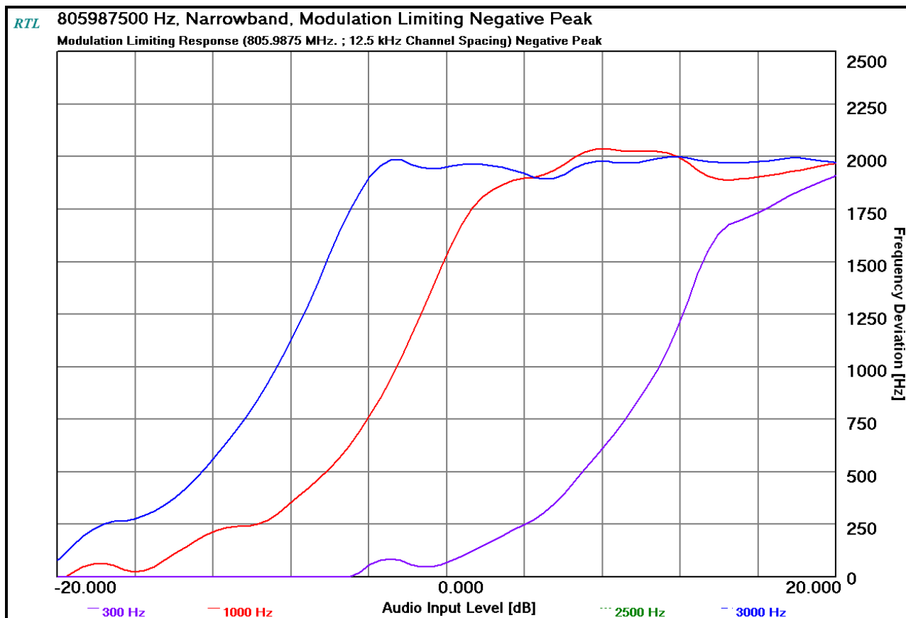
Plot 10-20: Modulation Characteristics – Modulation Limiting – 805.9875 MHz; Negative Peak; NB
