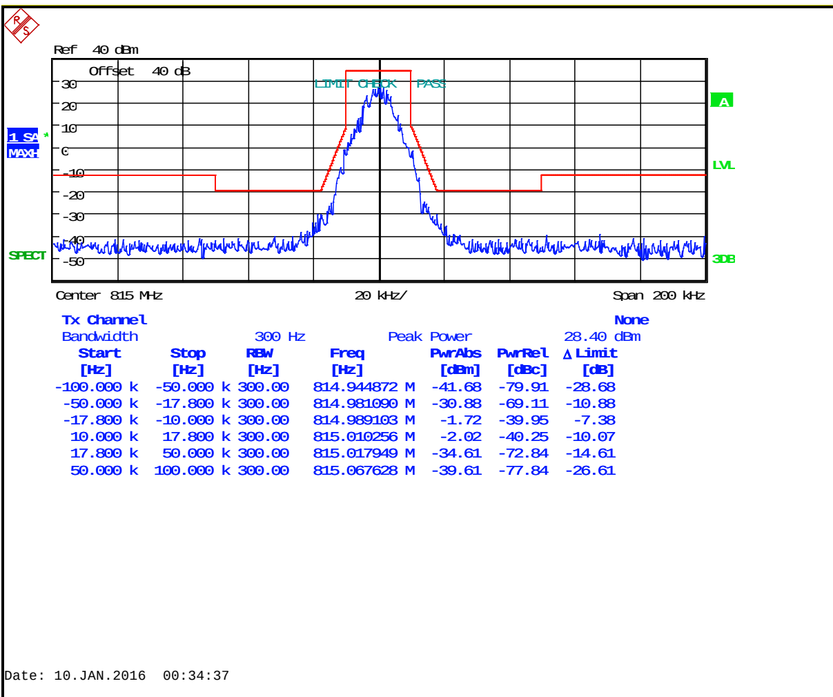
Plot 8-69: Occupied Bandwidth – 815.0000 MHz; OTP NPSPAC 4-level FSK (Mask G)
