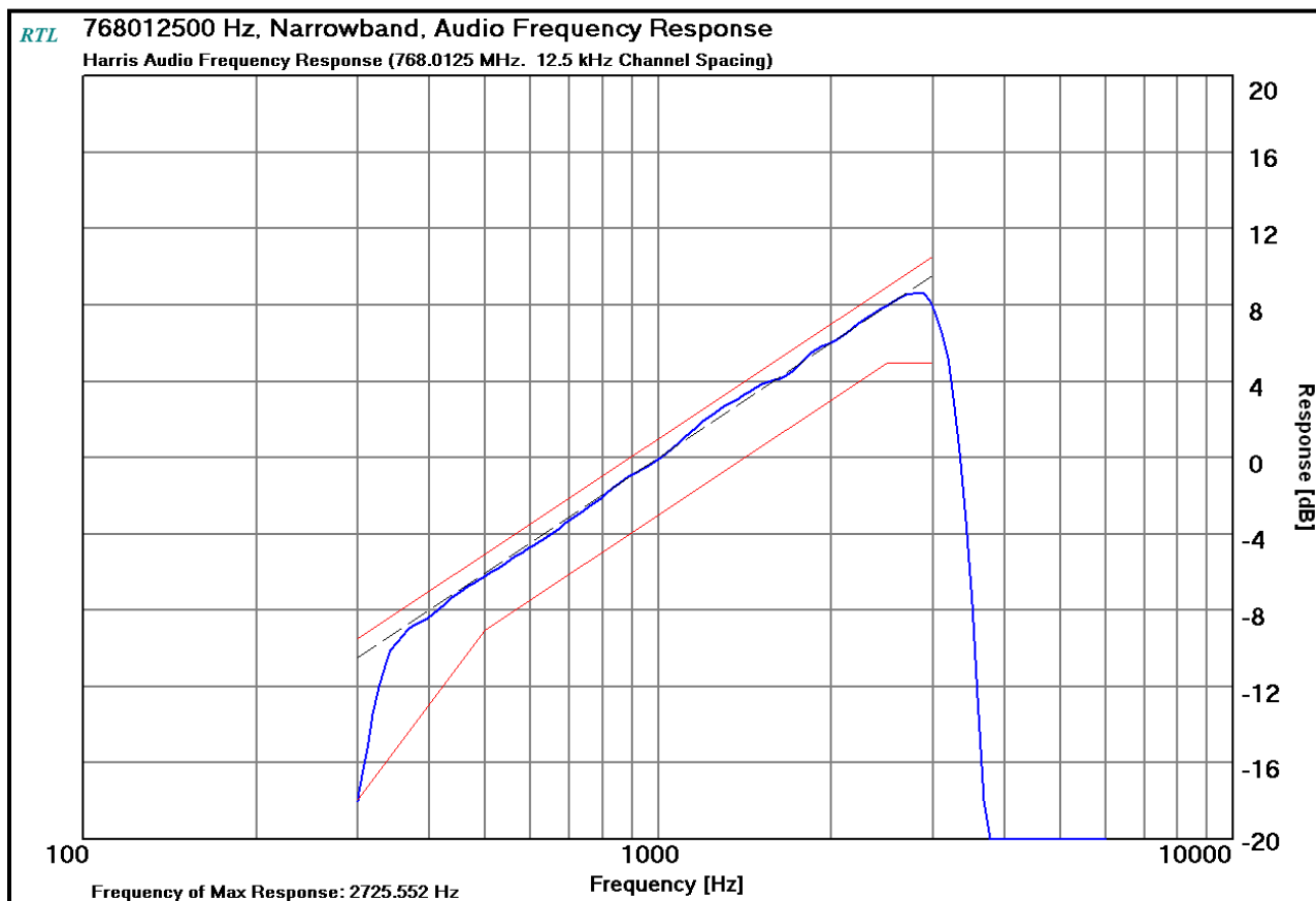
Plot 10-1: Modulation Characteristics - Audio Frequency Response – 768.0125 MHz
