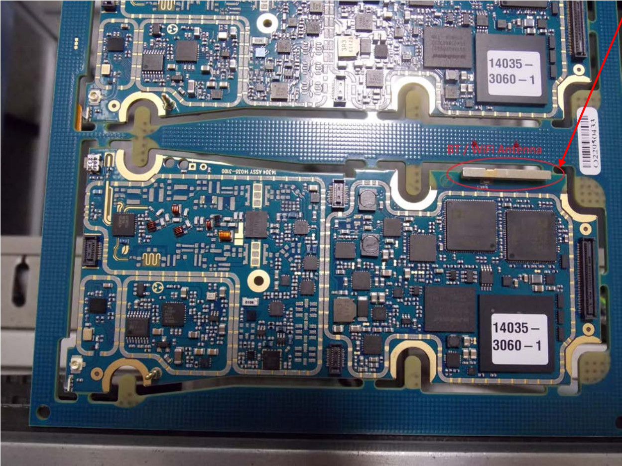
Main Board Top without Shields
