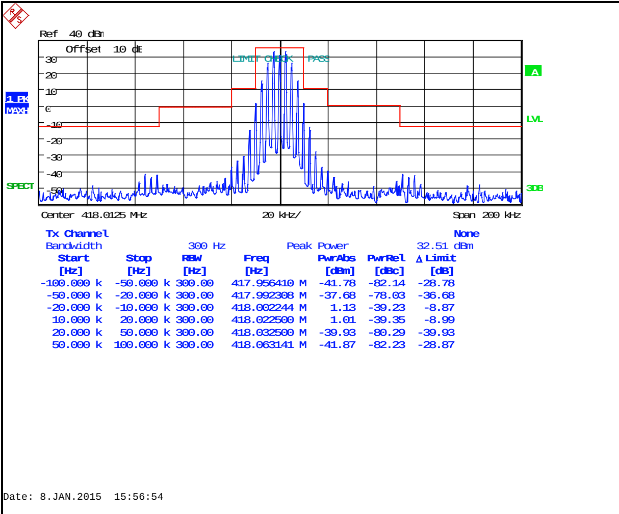
Plot 7-15: Occupied Bandwidth – 418.0125 MHz; Wideband Analog (Mask B)
