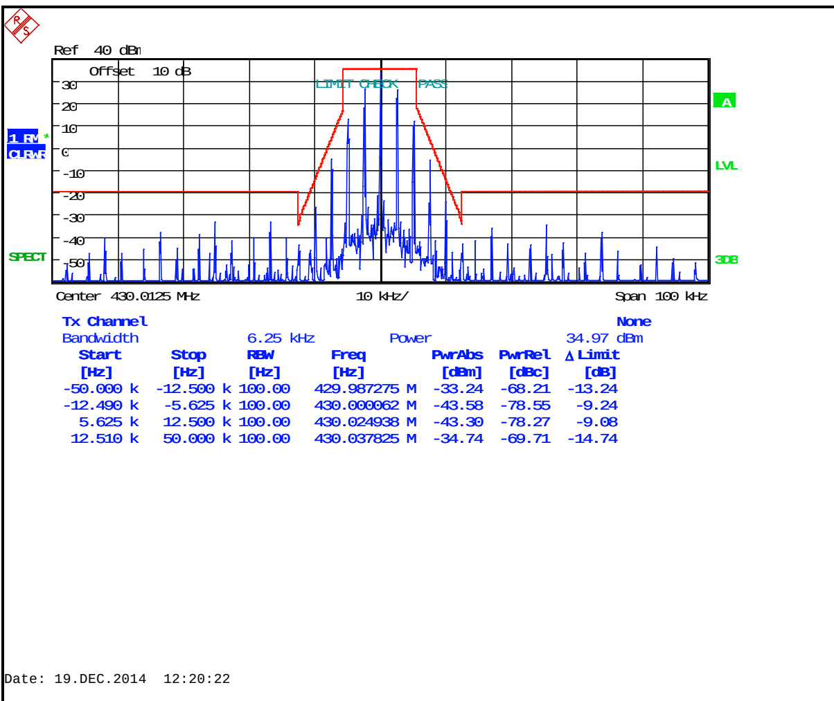
Plot 7-4: Occupied Bandwidth – 430.0125 MHz; Narrowband Analog (Mask D)
