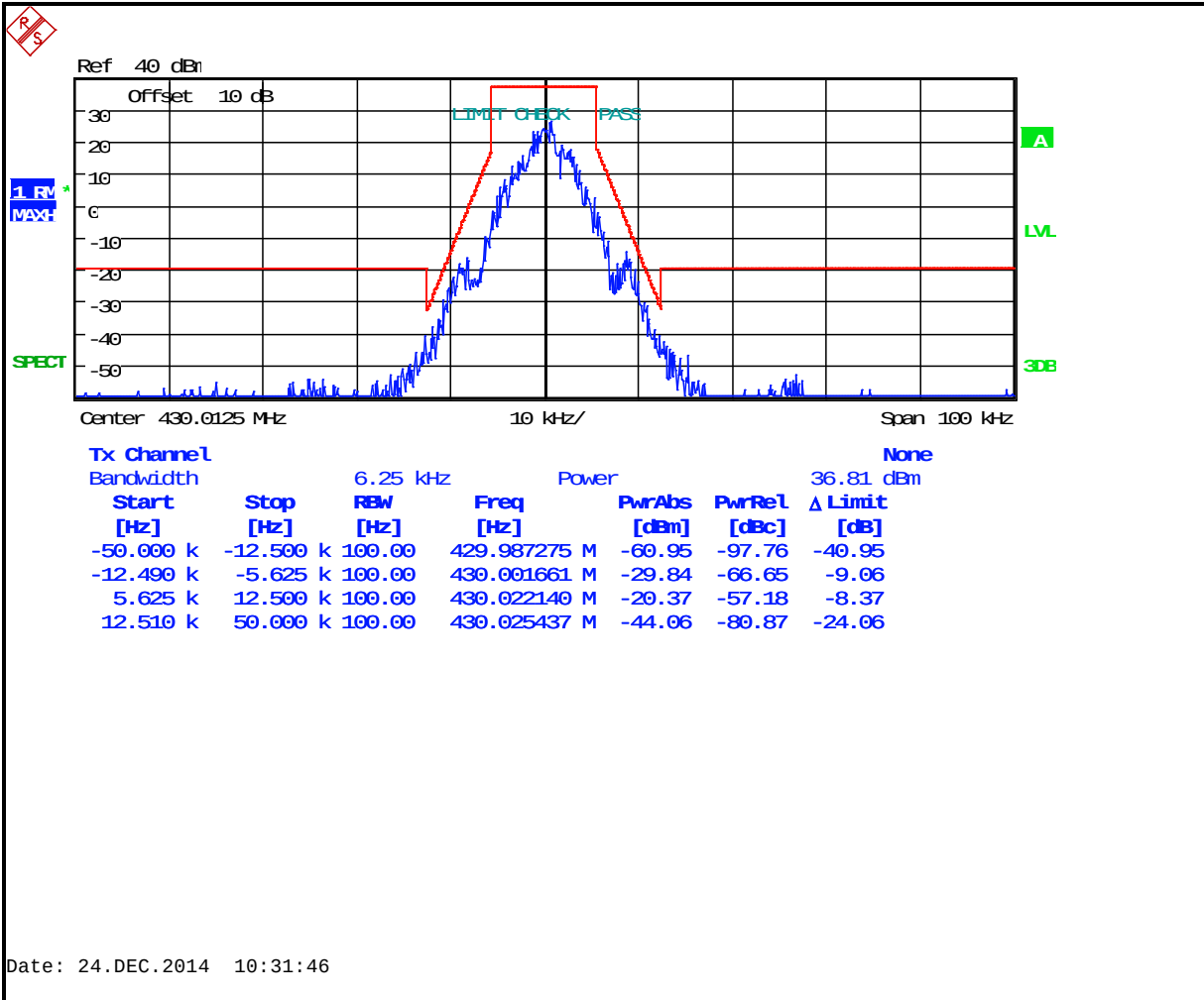
Plot 7-40: Occupied Bandwidth – 430.0125 MHz; EDACS Narrowband 2-level FSK 9600 (Mask D)
