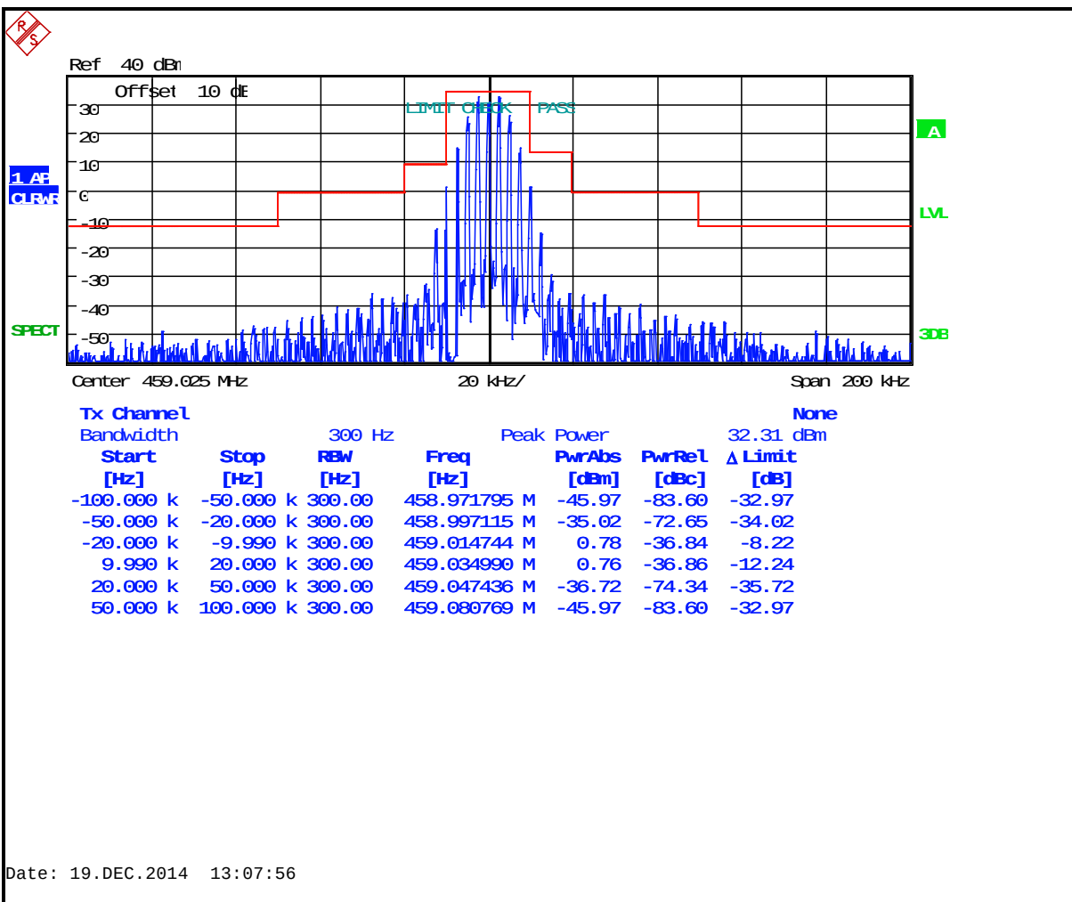
Plot 7-20: Occupied Bandwidth – 459.0250 MHz; Wideband Analog (Mask B)
