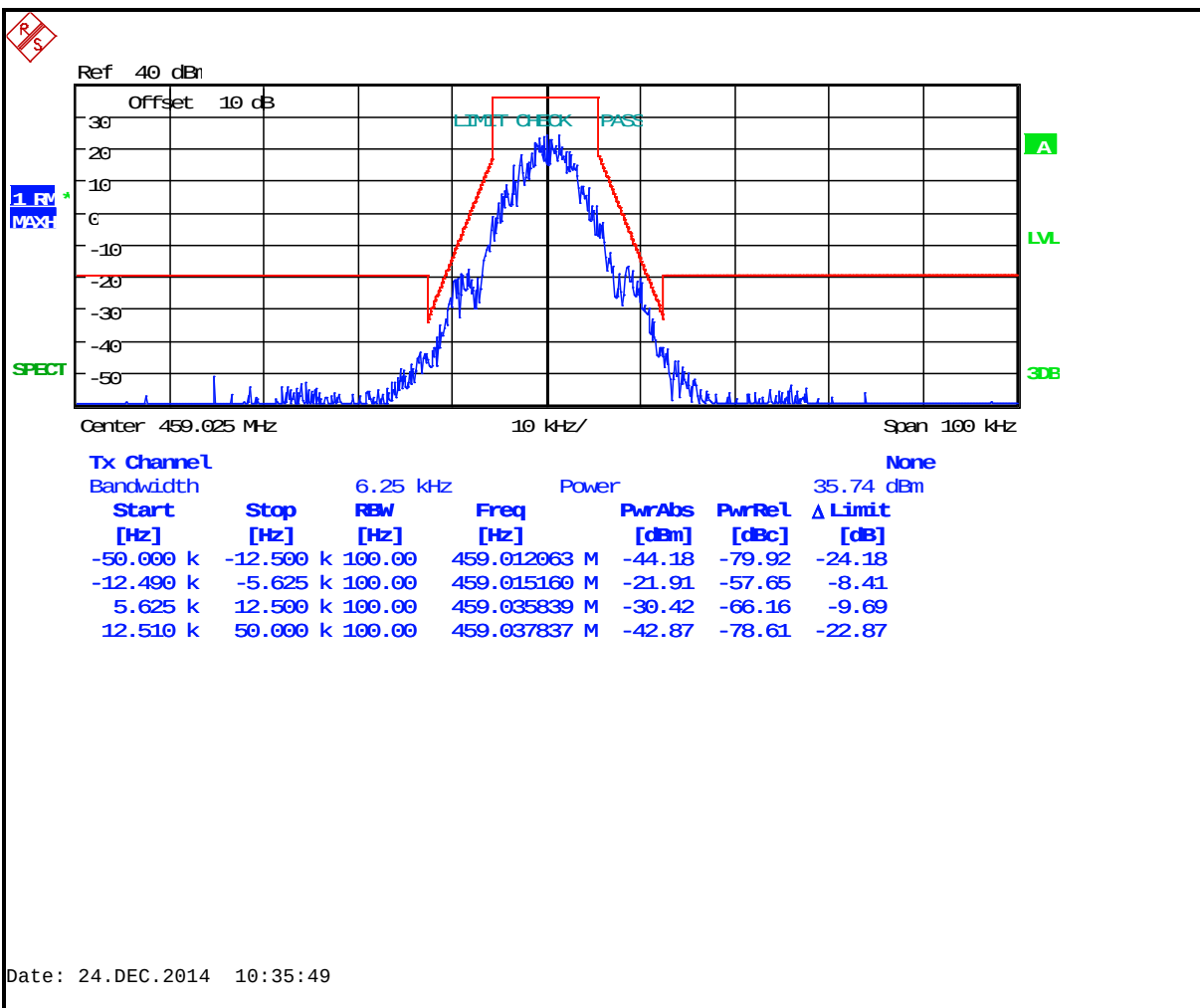
Plot 7-44: Occupied Bandwidth – 459.0250 MHz; EDACS Narrowband 2-level FSK 9600 (Mask D)
