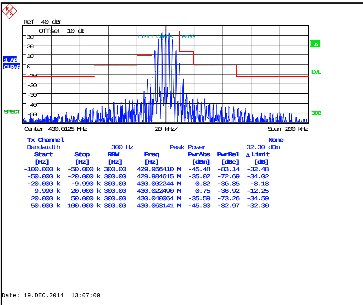
Plot 7-16: Occupied Bandwidth – 430.0125 MHz; Wideband Analog (Mask B)
