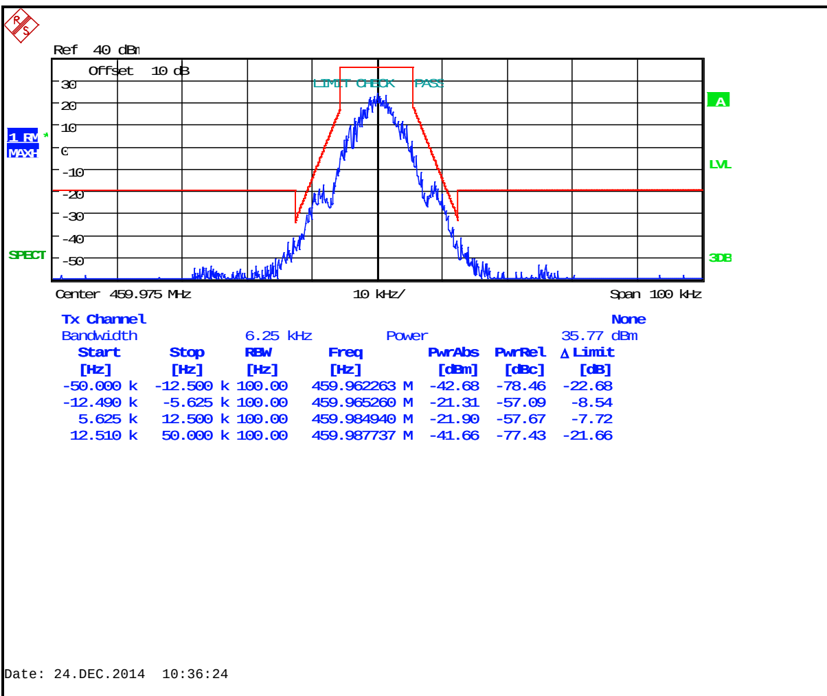
Plot 7-45: Occupied Bandwidth – 459.9750 MHz; EDACS Narrowband 2-level FSK 9600 (Mask D)
