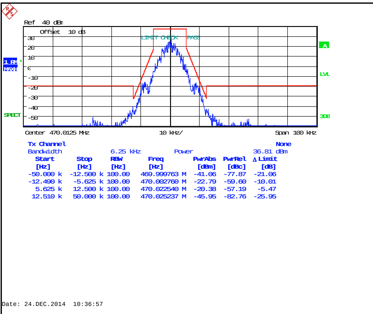
Plot 7-46: Occupied Bandwidth – 470.0125 MHz; EDACS Narrowband 2-level FSK 9600 (Mask D)
