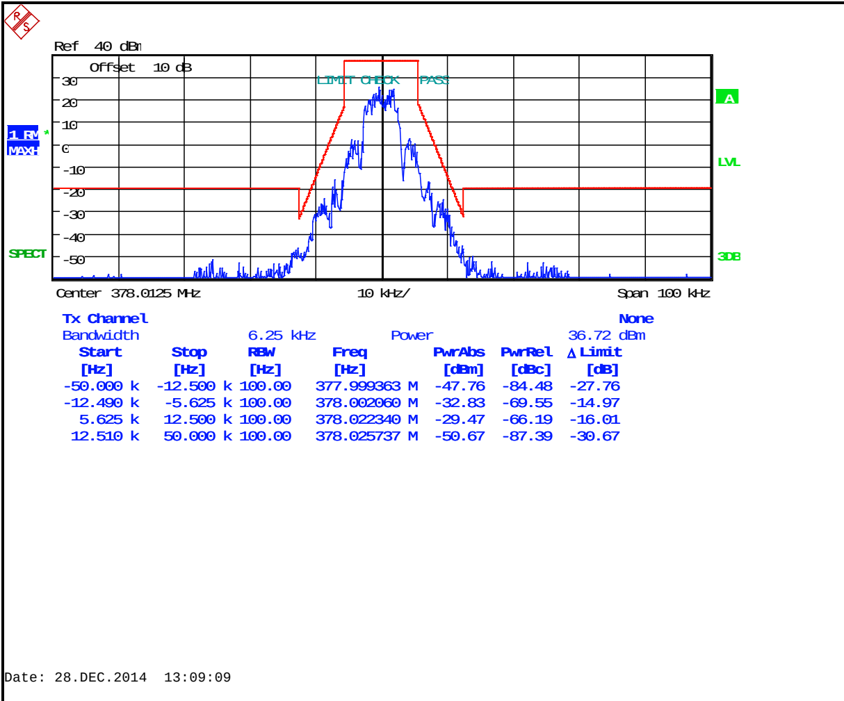
Plot 7-25: Occupied Bandwidth – 378.0125 MHz; EDACS Narrowband 2-level FSK 4800 (Mask D)
