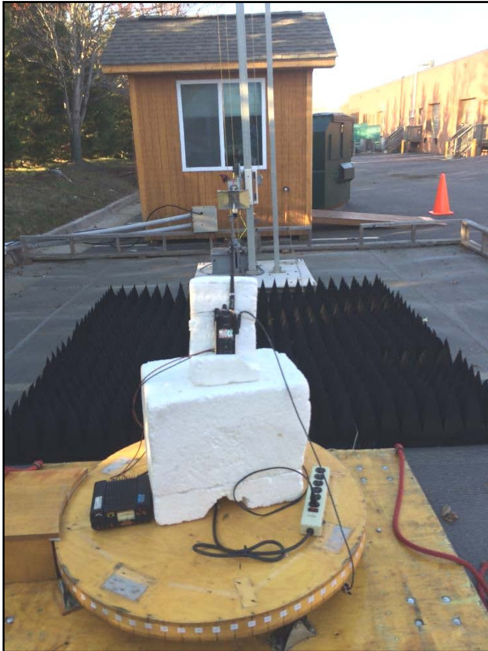
Photograph 1: Radiated Emissions – Front View
