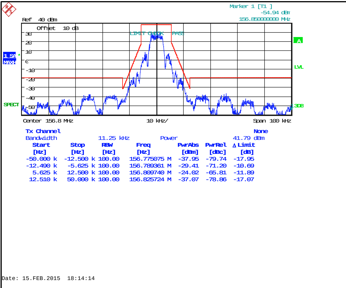
Plot 7-25: Occupied Bandwidth – 156.8000 MHz; EDACS Narrowband 2-level FSK 4800 (Mask D)
