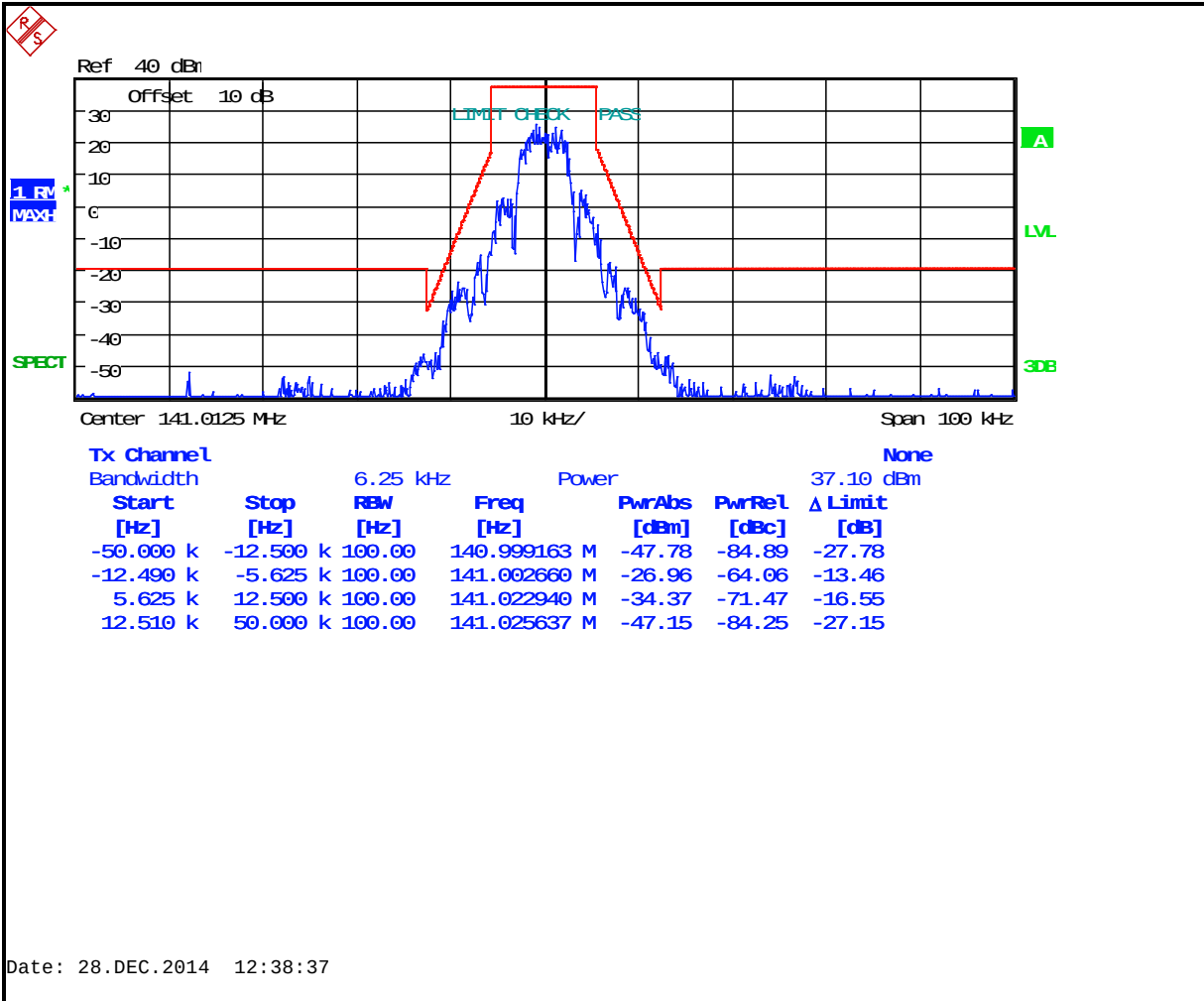
Plot 7-21: Occupied Bandwidth – 141.0125 MHz; EDACS Narrowband 2-level FSK 4800 (Mask D)
