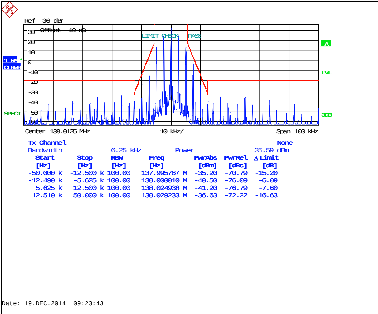
Plot 7-2: Occupied Bandwidth – 138.0125 MHz; Narrowband Analog (Mask D)
