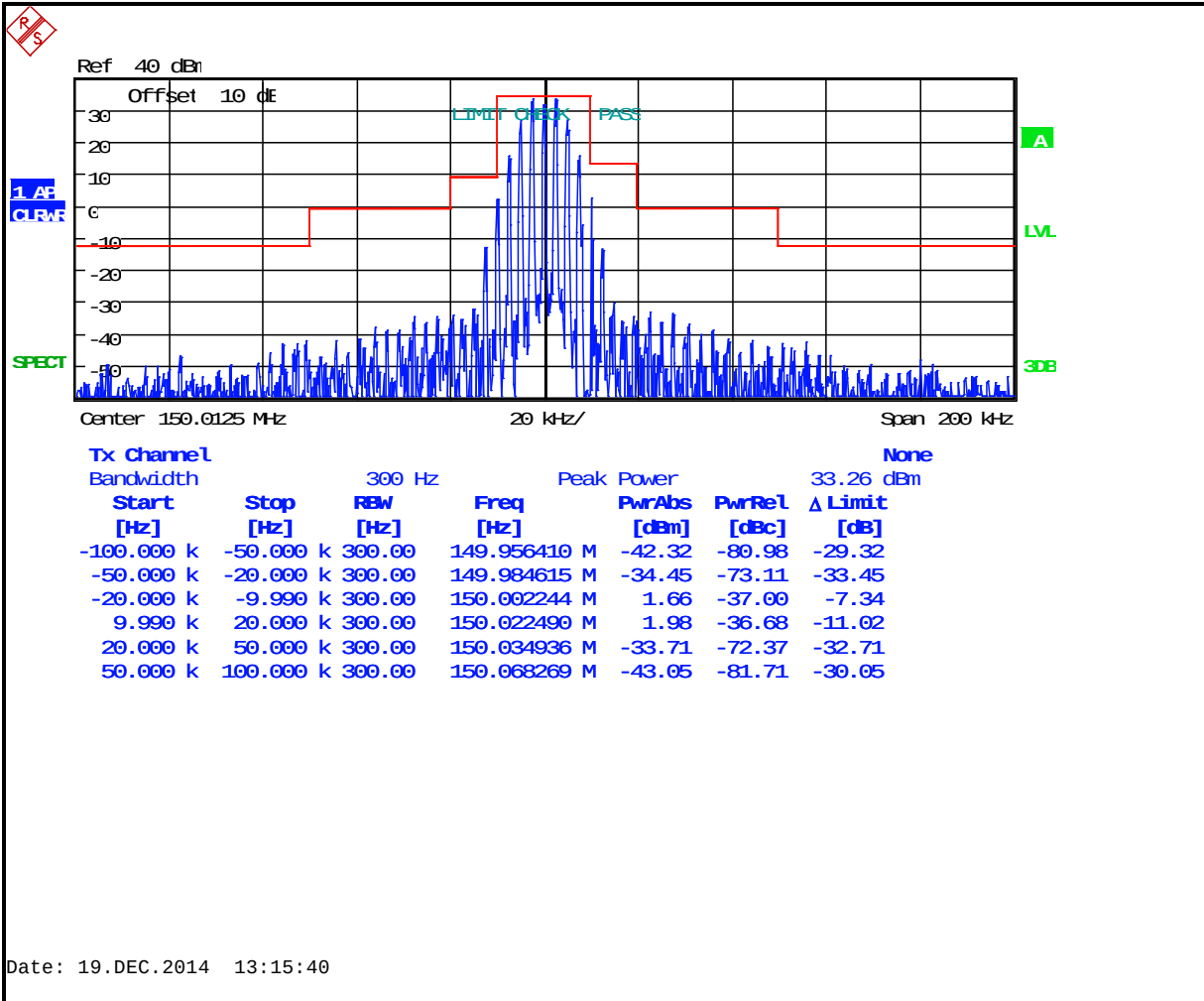
Plot 7-15: Occupied Bandwidth – 150.0125 MHz; Wideband Analog (Mask B)
