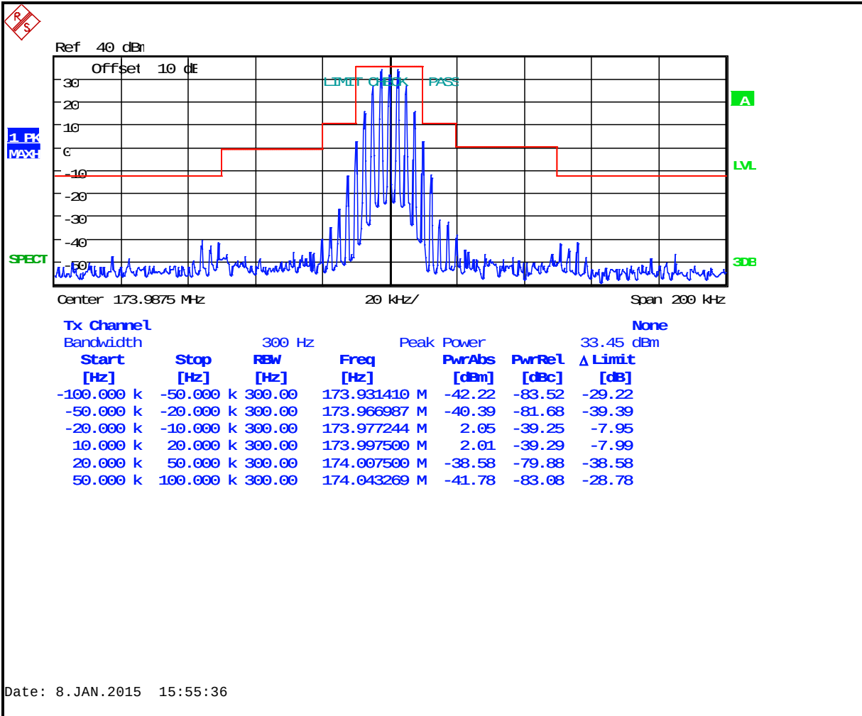
Plot 7-18: Occupied Bandwidth – 173.9875 MHz; Wideband Analog (Mask B)
