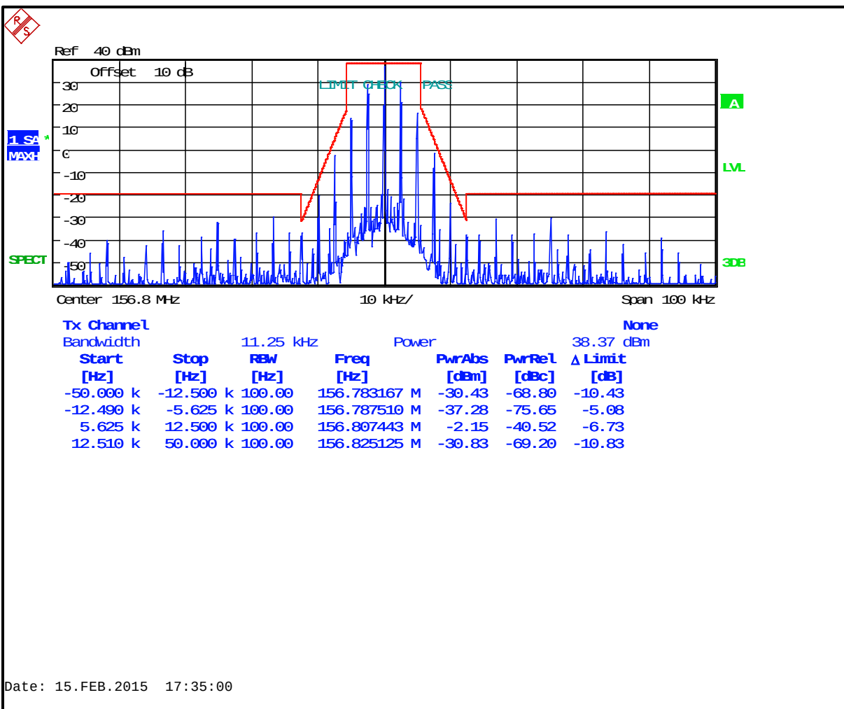
Plot 7-7: Occupied Bandwidth – 156.8000 MHz; Narrowband Analog (Mask D)
