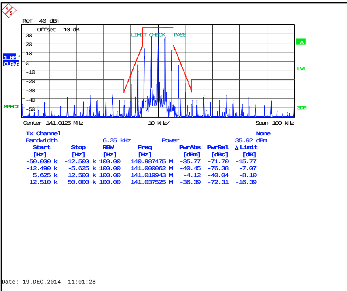
Plot 7-3: Occupied Bandwidth – 141.0125 MHz; Narrowband Analog (Mask D)
