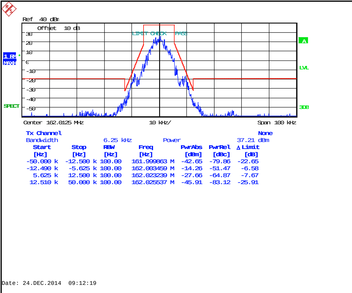
Plot 7-35: Occupied Bandwidth – 162.0125 MHz; EDACS Narrowband 2-level FSK 9600 (Mask D)
