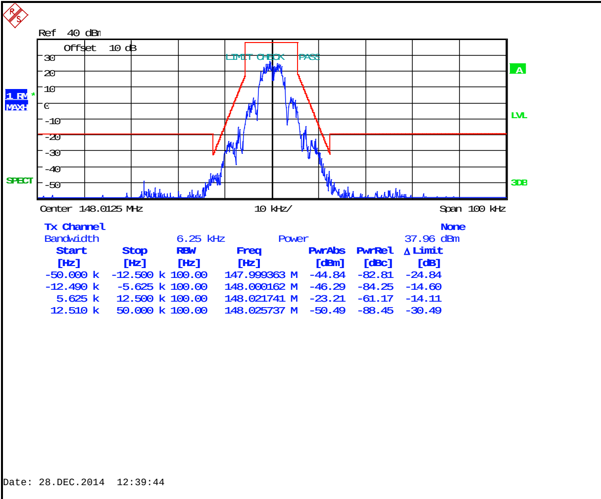
Plot 7-23: Occupied Bandwidth – 148.0125 MHz; EDACS Narrowband 2-level FSK 4800 (Mask D)
