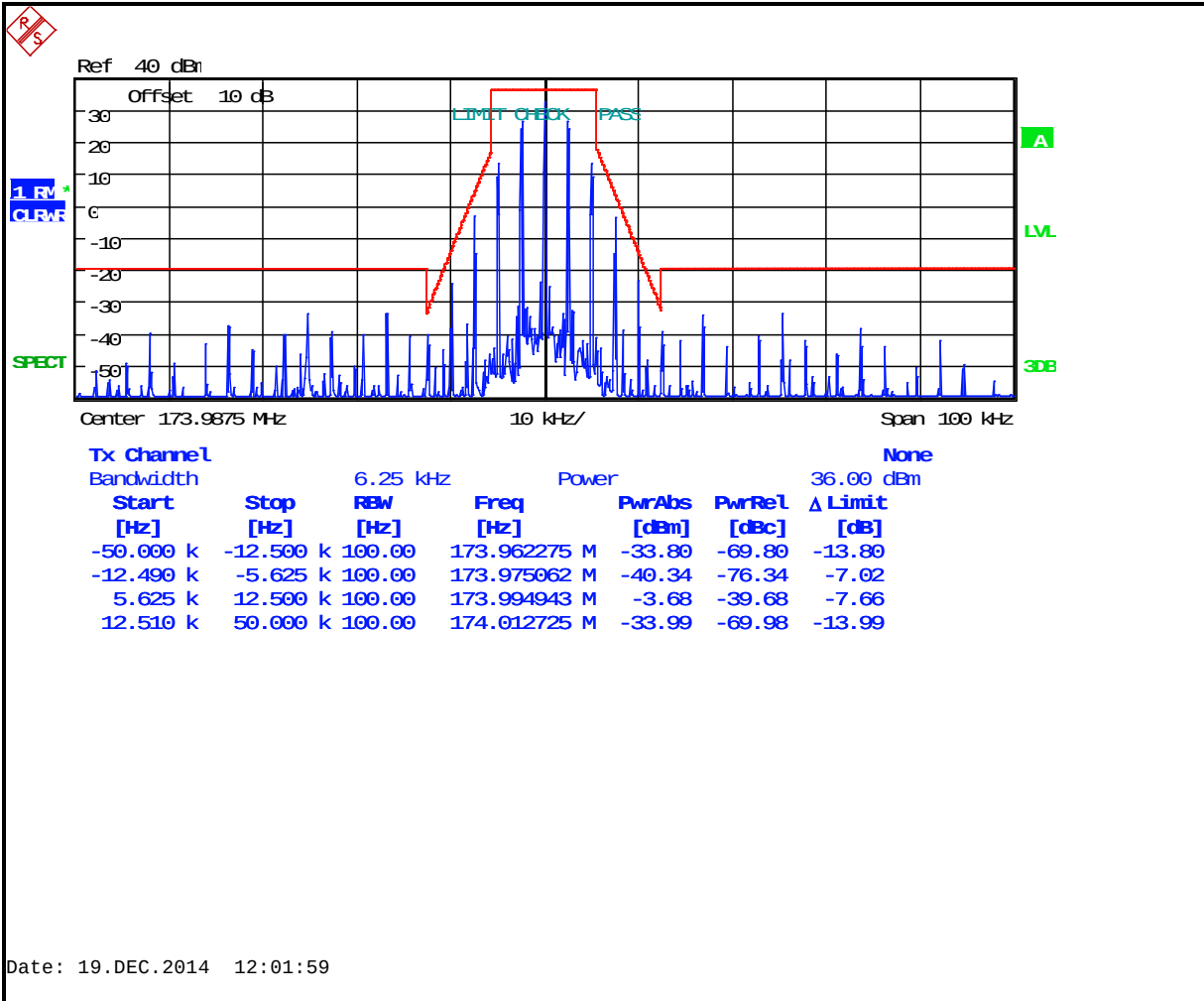
Plot 7-9: Occupied Bandwidth – 173.9875 MHz; Narrowband Analog (Mask D)
