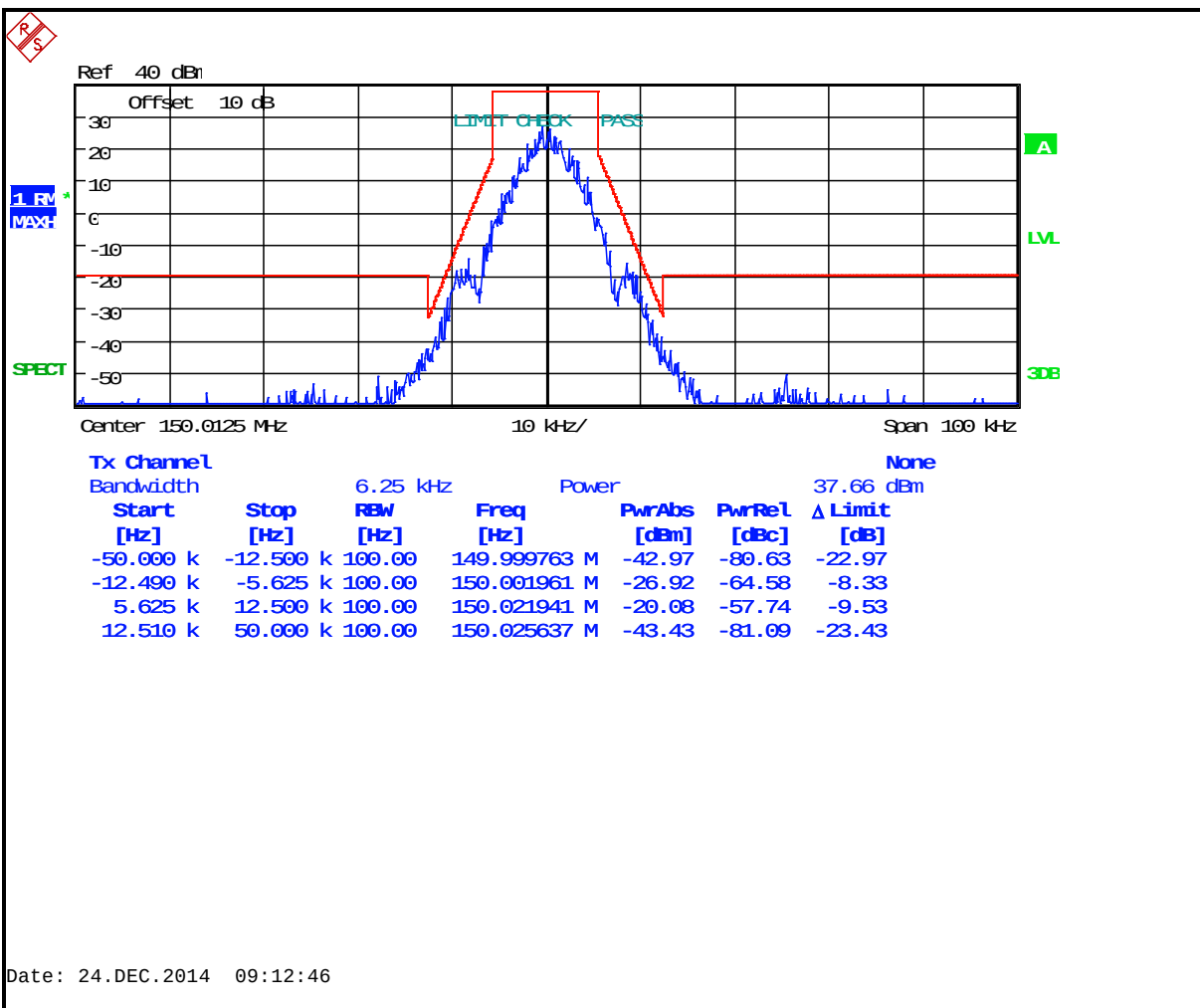
Plot 7-33: Occupied Bandwidth – 150.0125 MHz; EDACS Narrowband 2-level FSK 9600 (Mask D)
