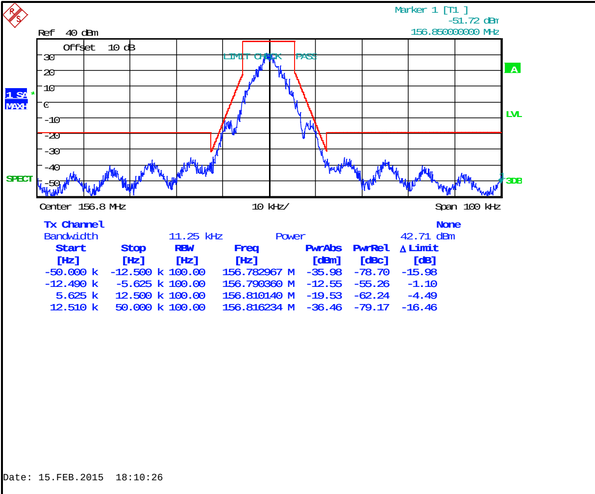
Plot 7-34: Occupied Bandwidth – 156.8000 MHz; EDACS Narrowband 2-level FSK 9600 (Mask D)
