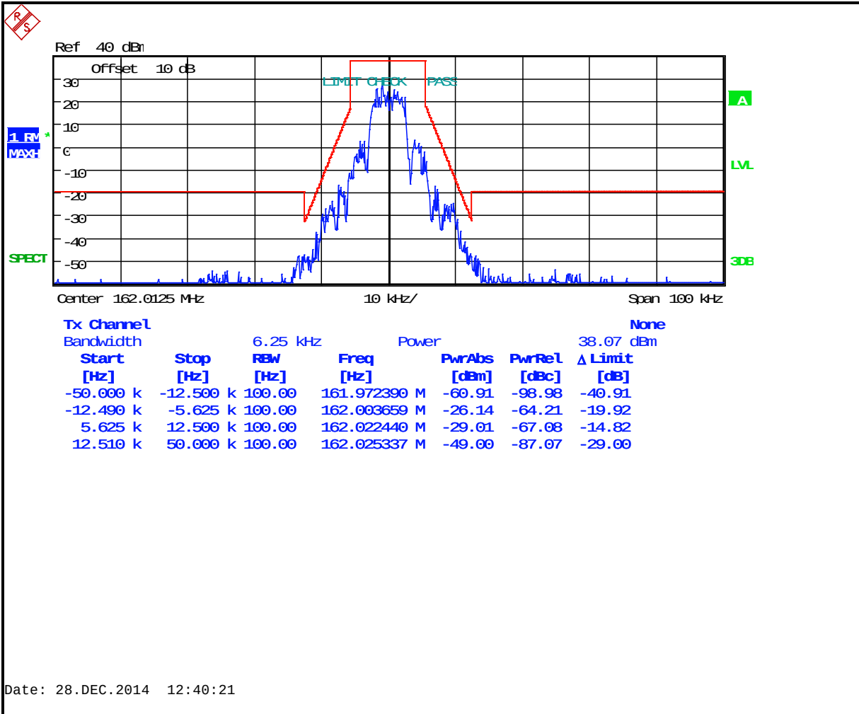
Plot 7-26: Occupied Bandwidth – 162.0125 MHz; EDACS Narrowband 2-level FSK 4800 (Mask D)
