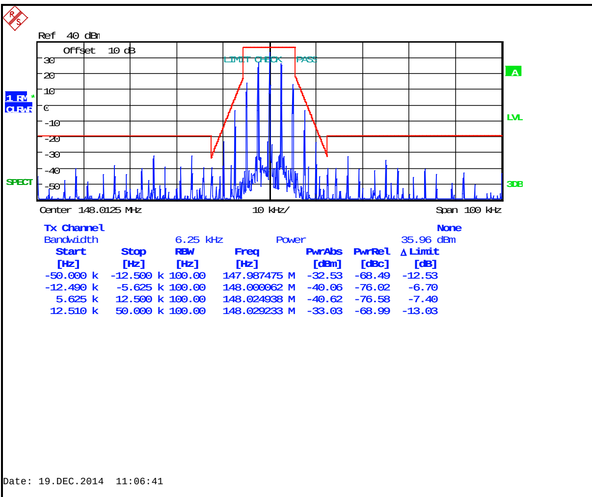
Plot 7-5: Occupied Bandwidth – 148.0125 MHz; Narrowband Analog (Mask D)
