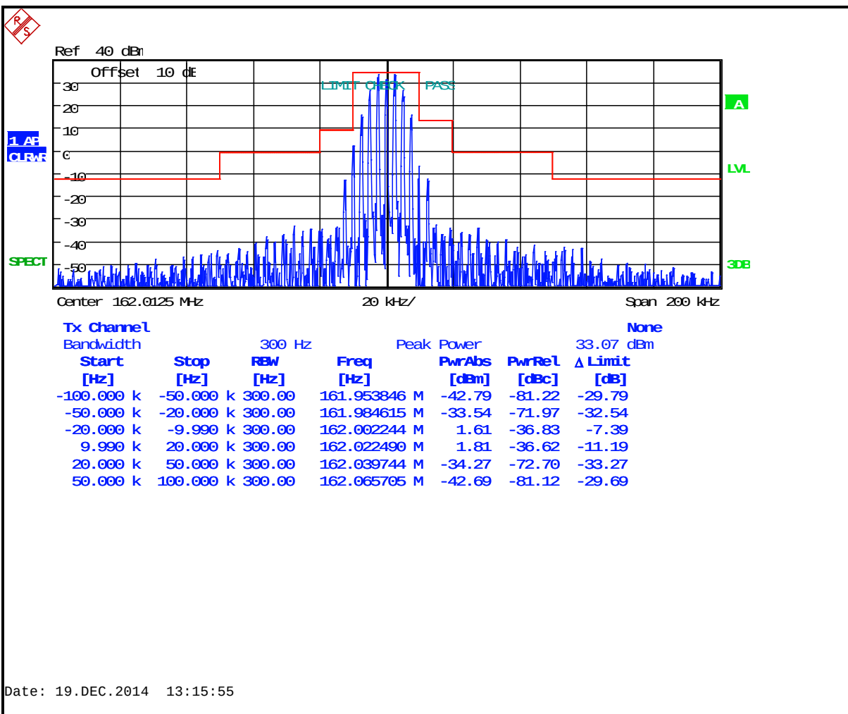
Plot 7-17: Occupied Bandwidth – 162.0125 MHz; Wideband Analog (Mask B)
