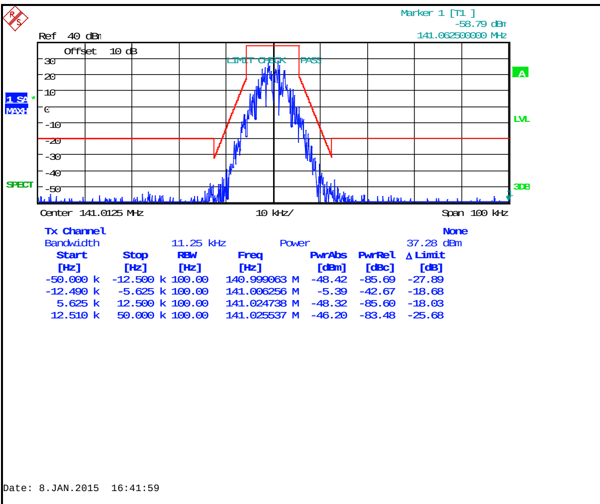
Plot 7-48: Occupied Bandwidth – 141.0125 MHz; C4FM (Mask D)
