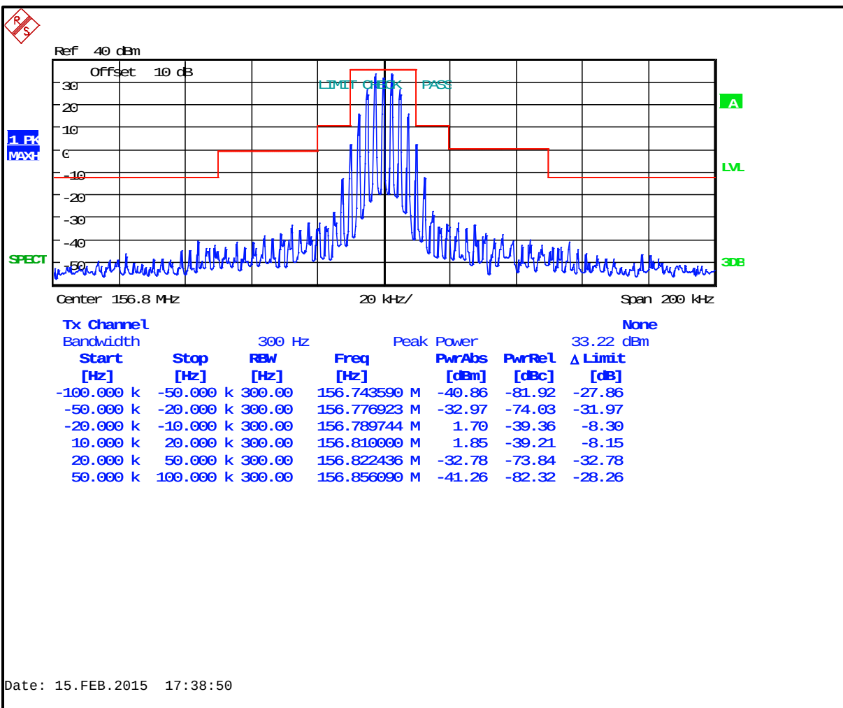
Plot 7-16: Occupied Bandwidth – 156.8000 MHz; Wideband Analog (Mask B)
