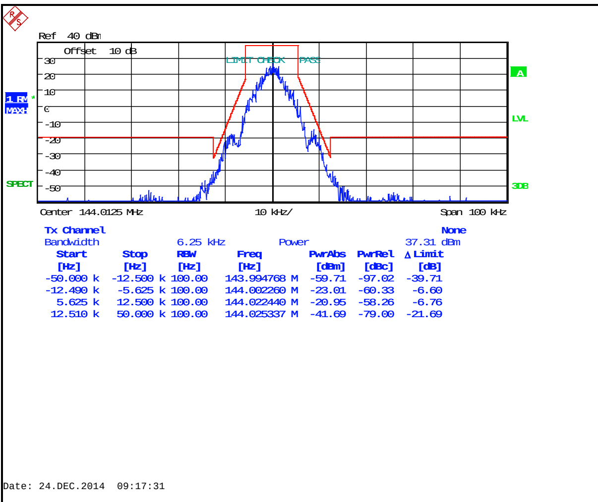
Plot 7-31: Occupied Bandwidth – 144.0125 MHz; EDACS Narrowband 2-level FSK 9600 (Mask D)
