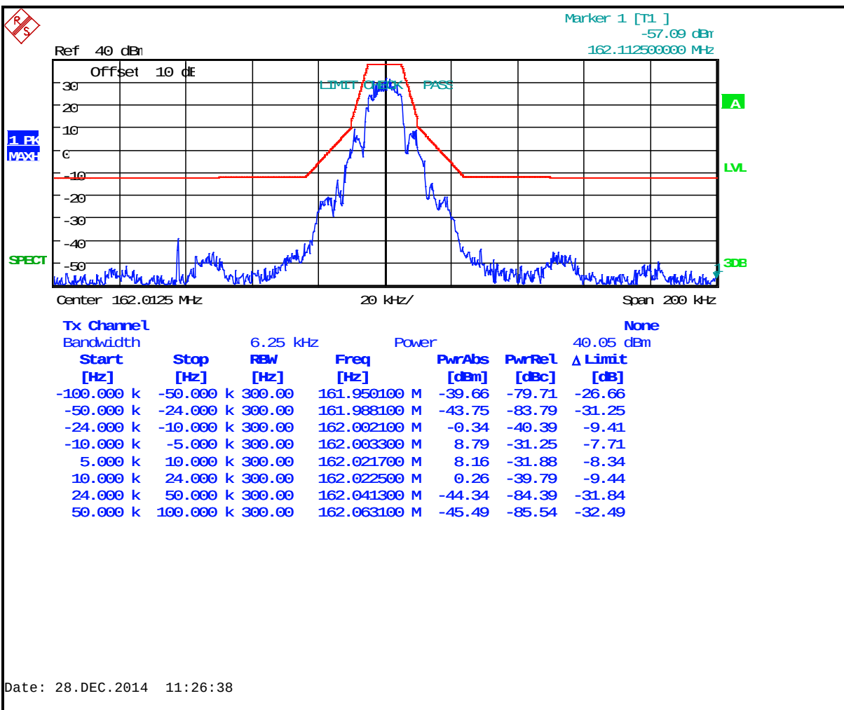
Plot 7-44: Occupied Bandwidth – 162.0125 MHz; EDACS Wideband 2-level FSK 9600 (Mask C)
