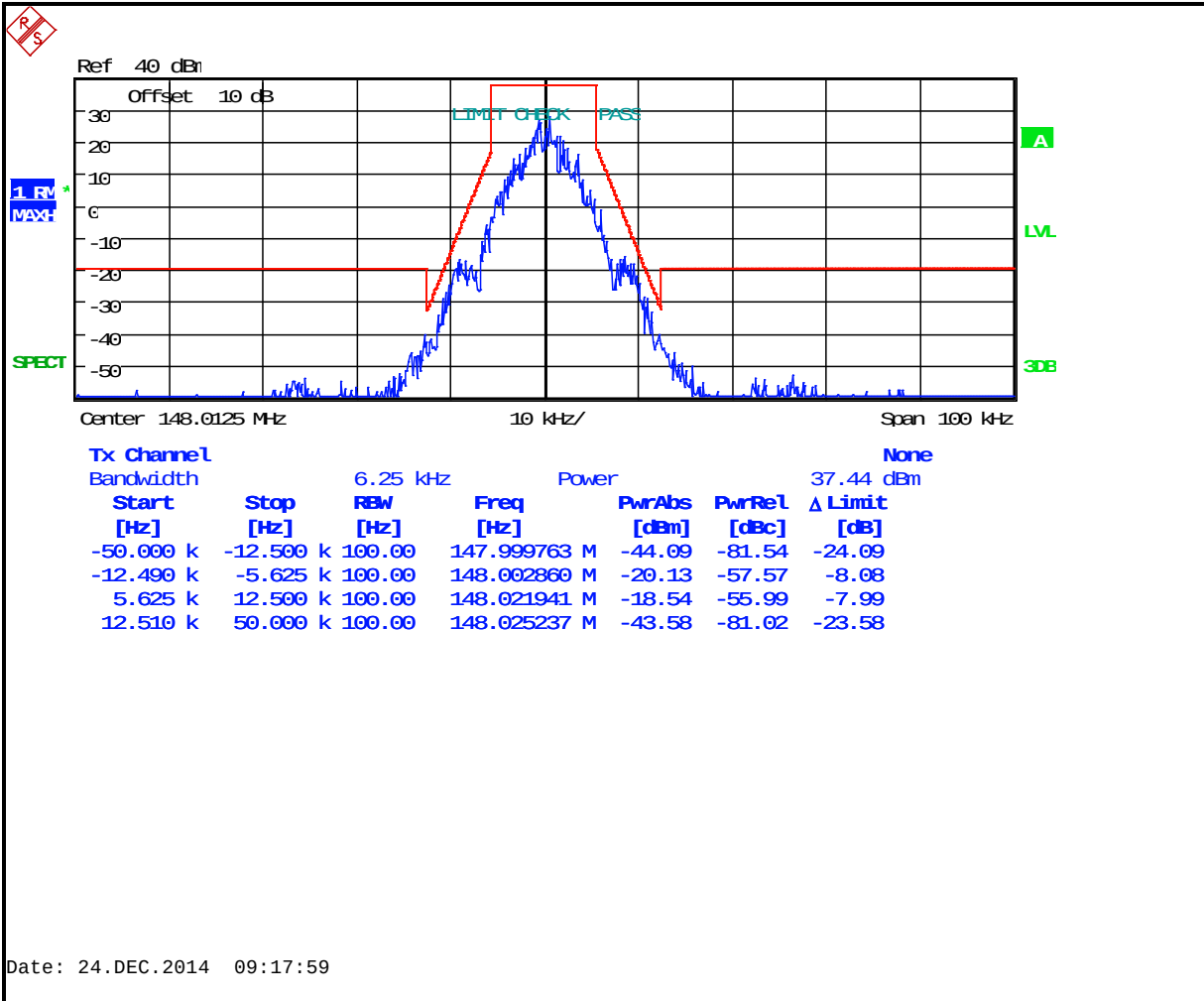
Plot 7-32: Occupied Bandwidth – 148.0125 MHz; EDACS Narrowband 2-level FSK 9600 (Mask D)
