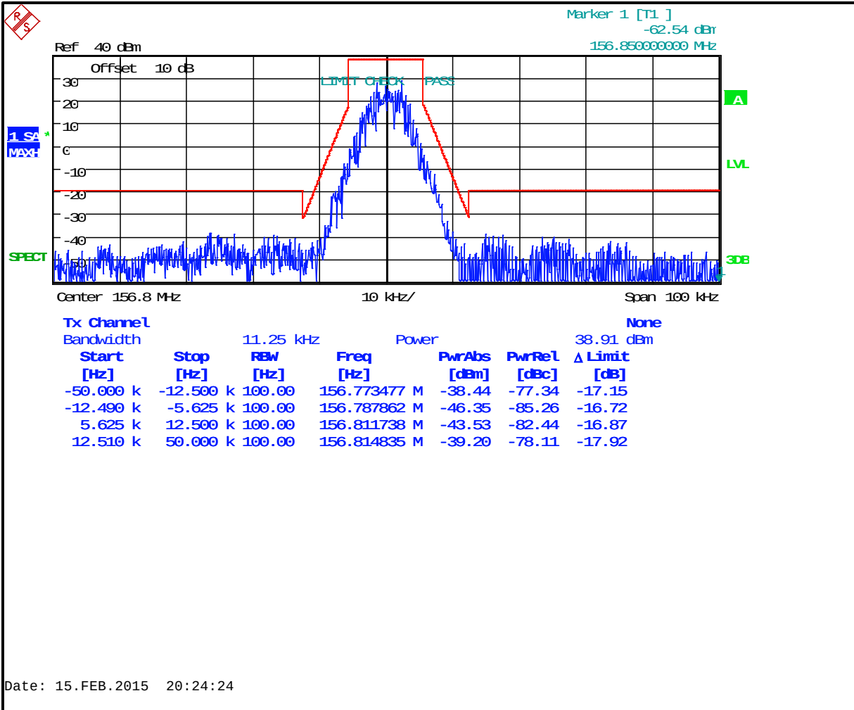
Plot 7-61: Occupied Bandwidth – 156.8000 MHz; C4FM Phase 2 (Mask D)
