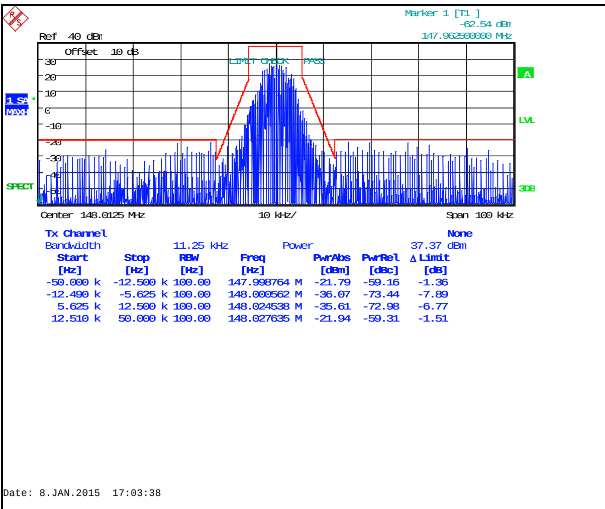
Plot 7-59: Occupied Bandwidth – 148.0125 MHz; C4FM Phase 2 (Mask D)
