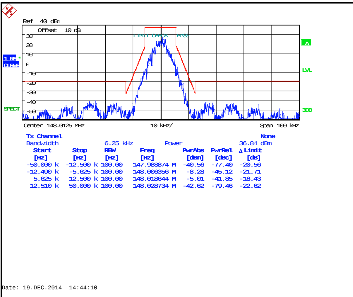
Plot 7-50: Occupied Bandwidth – 148.0125 MHz; C4FM (Mask D)
