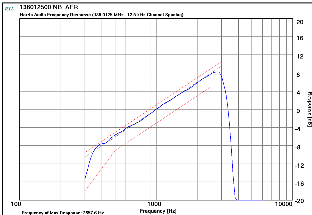
Plot 9-1: Modulation Characteristics - Audio Frequency Response – 136.0125 MHz
