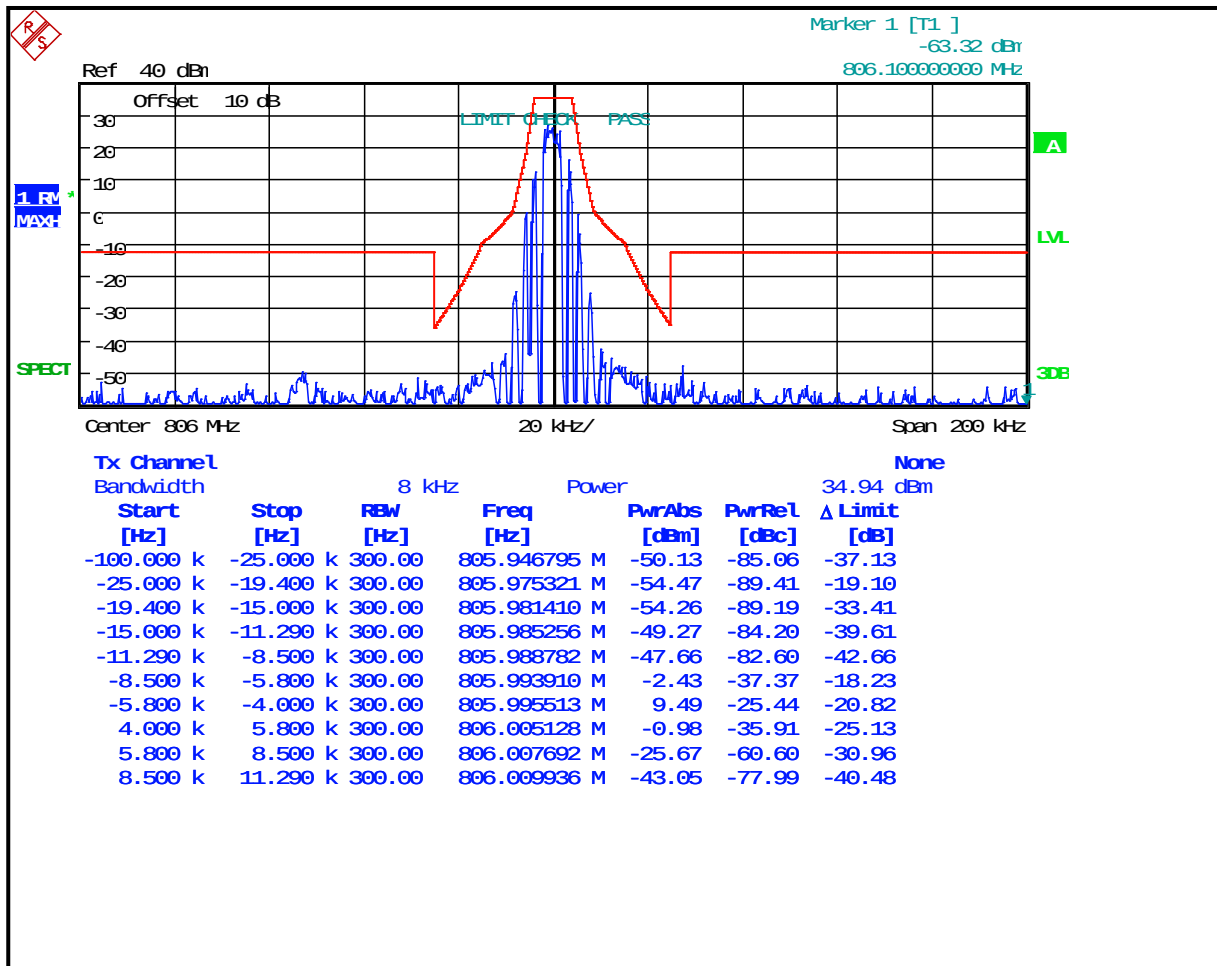
Plot 8-25: Occupied Bandwidth – 806 MHz; CPM TDMA; Mask H
