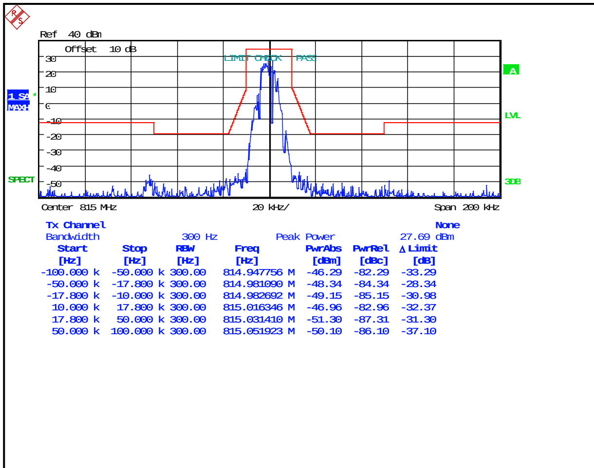
Plot 8-26: Occupied Bandwidth – 815 MHz; CPM TDMA; Mask G
