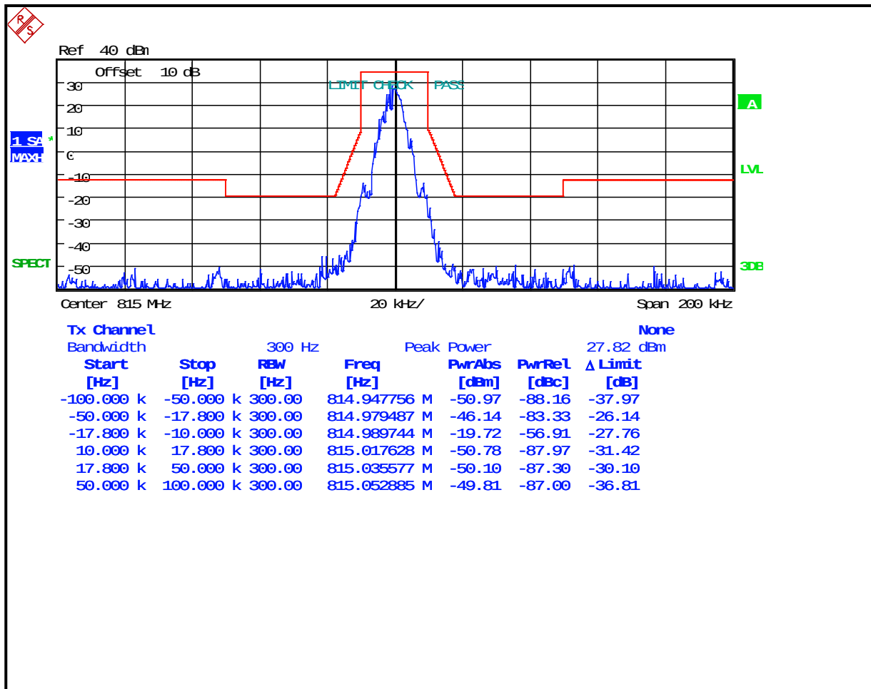
Plot 8-35: Occupied Bandwidth – 815 MHz; 2-level FSK 9600; NB EDACS; Mask G
