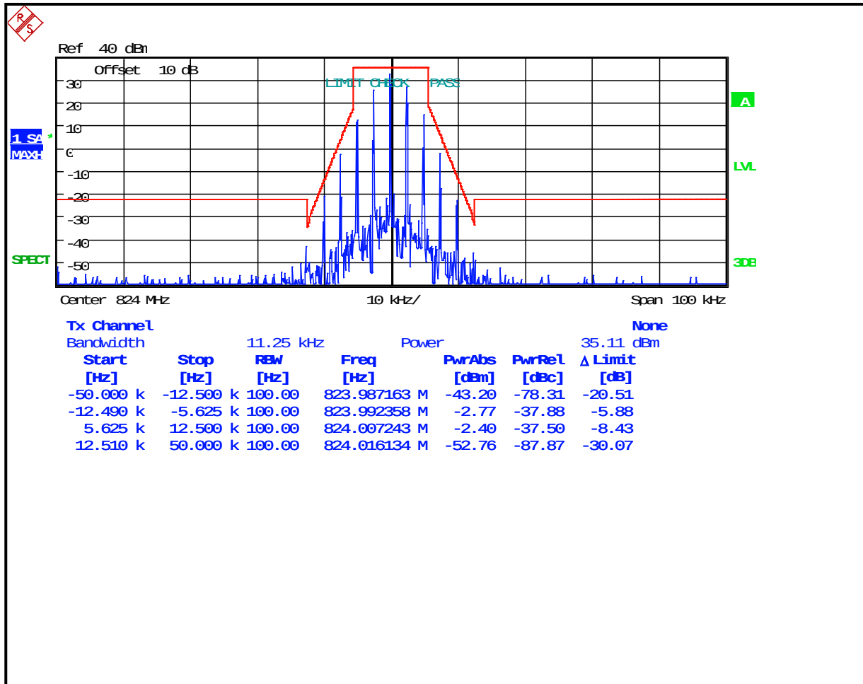
Plot 8-3: Occupied Bandwidth – 824 MHz; Narrowband Analog; Mask D
