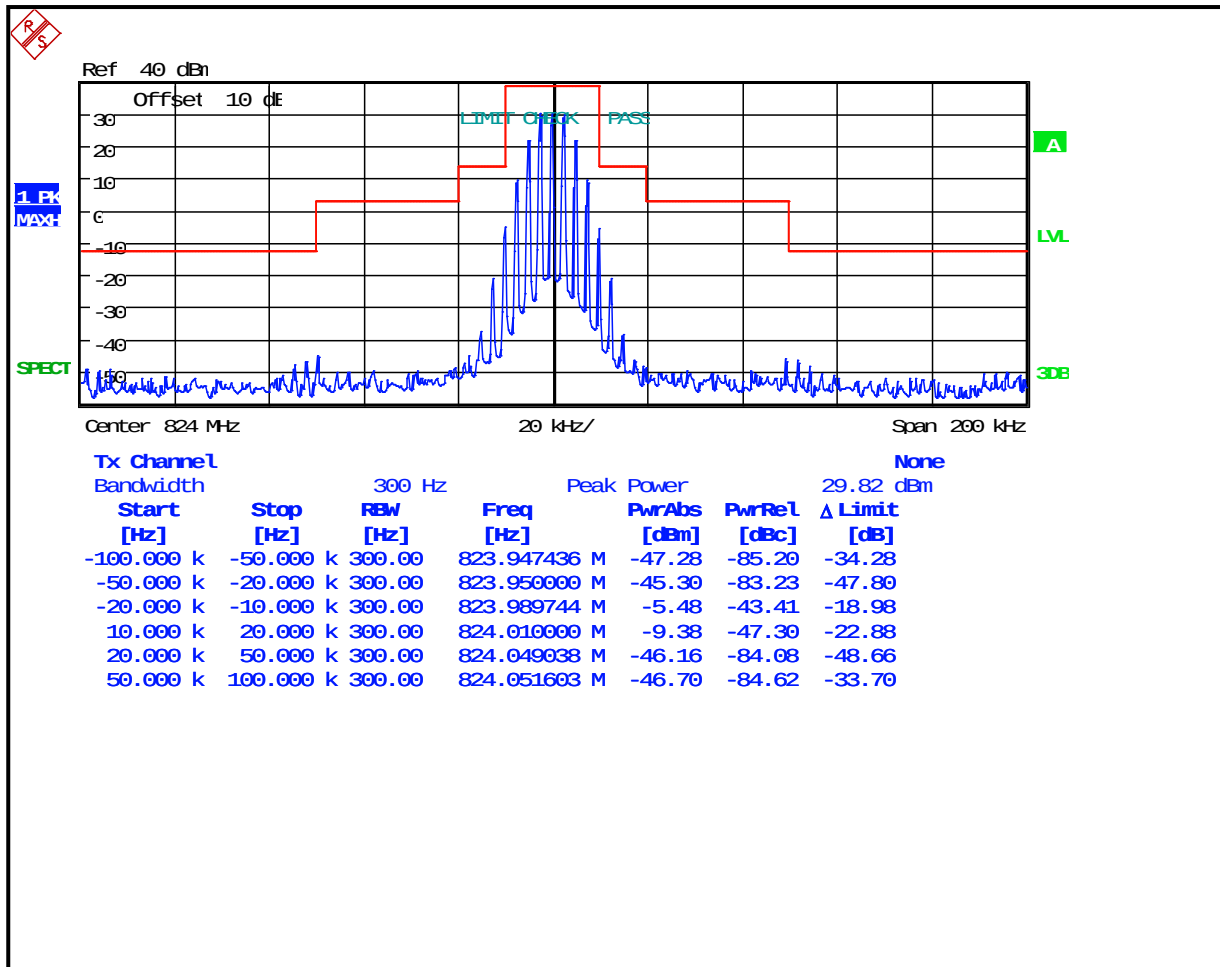
Plot 8-15: Occupied Bandwidth – 824 MHz; NPSPAC; Mask B
