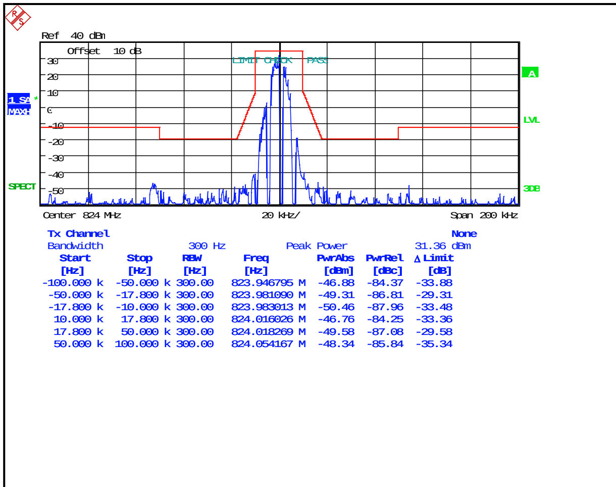
Plot 8-27: Occupied Bandwidth – 824 MHz; CPM TDMA; Mask G
