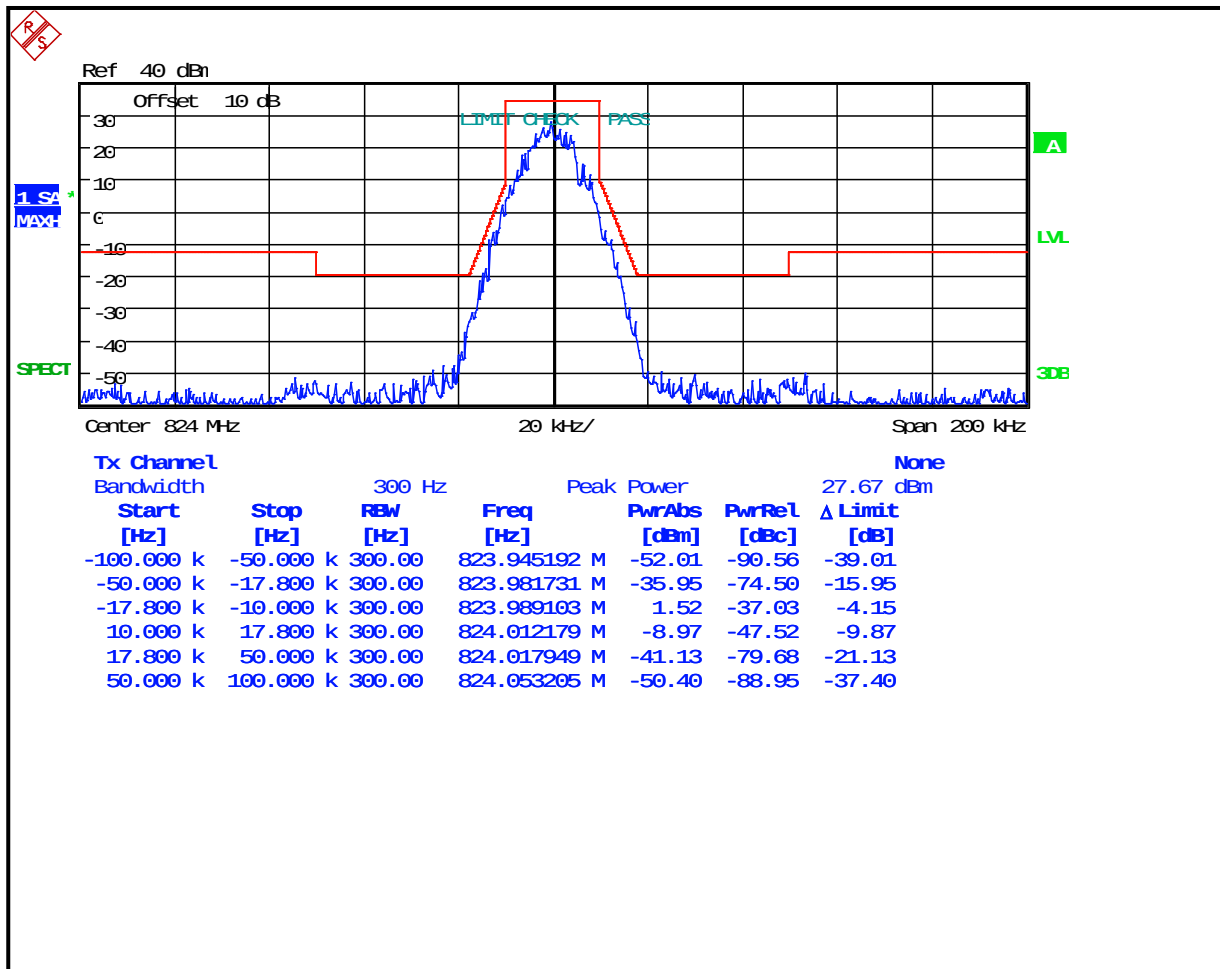
Plot 8-51: Occupied Bandwidth – 824 MHz; 4-level FSK Data/Voice; SMR OpenSky; Mask G
