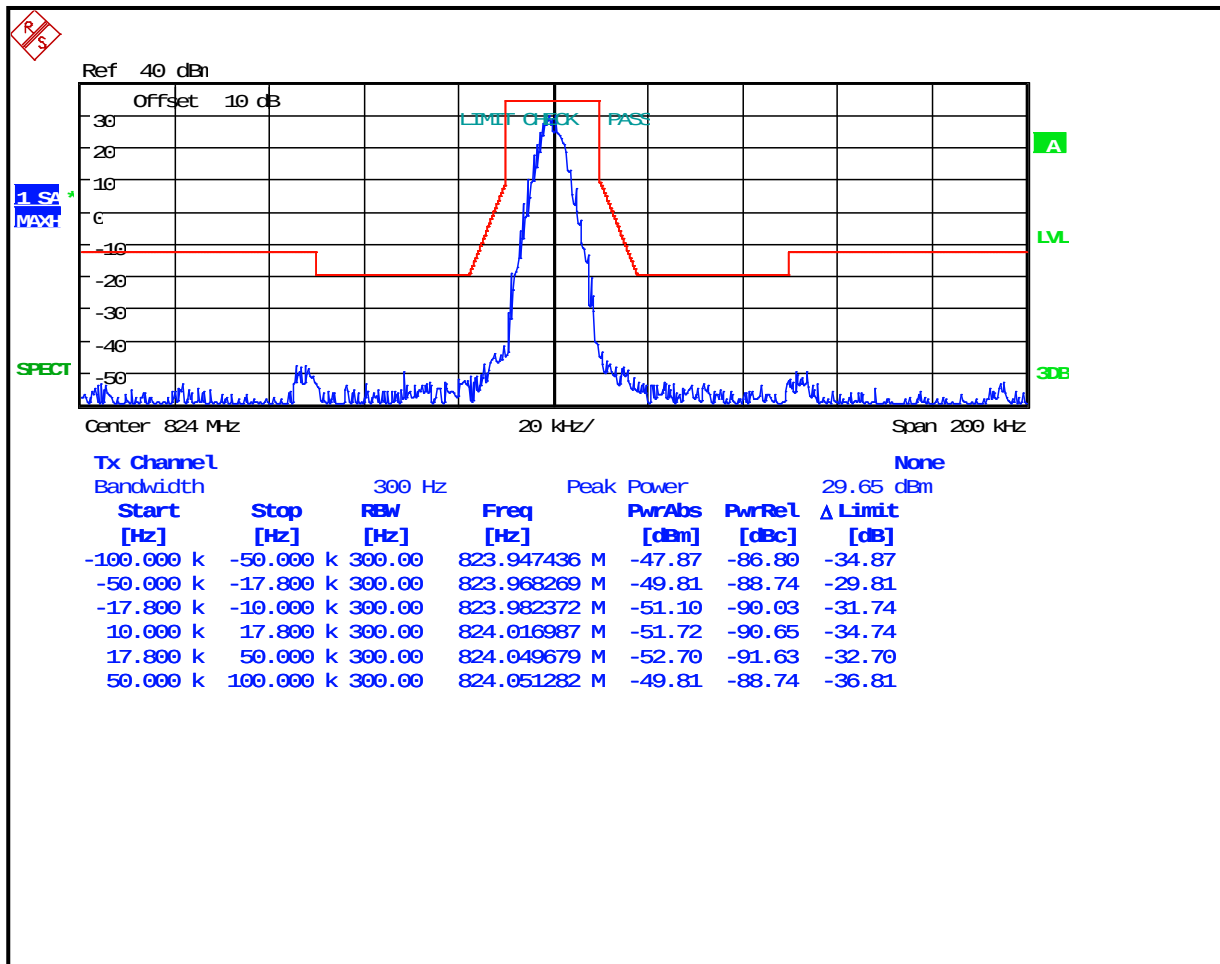
Plot 8-21: Occupied Bandwidth – 824 MHz; P25 RND; Mask G
