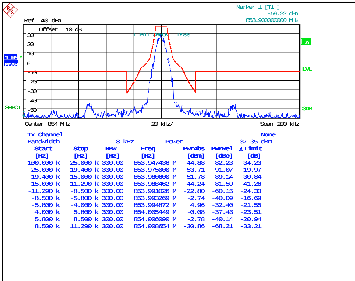
Plot 8-22: Occupied Bandwidth – 854 MHz; P25 RND; Mask H
