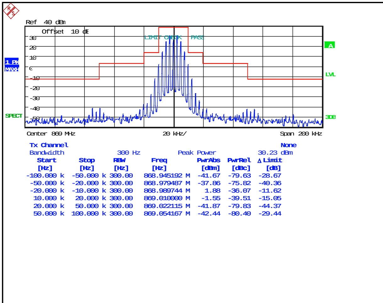
Plot 8-12: Occupied Bandwidth – 869 MHz; Wideband Analog; Mask B
