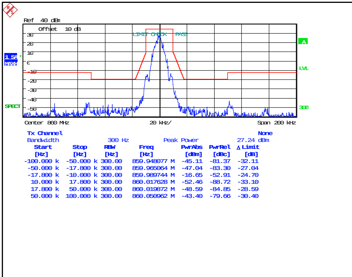
Plot 8-37: Occupied Bandwidth – 860 MHz; 2-level FSK 9600; NB EDACS; Mask G
