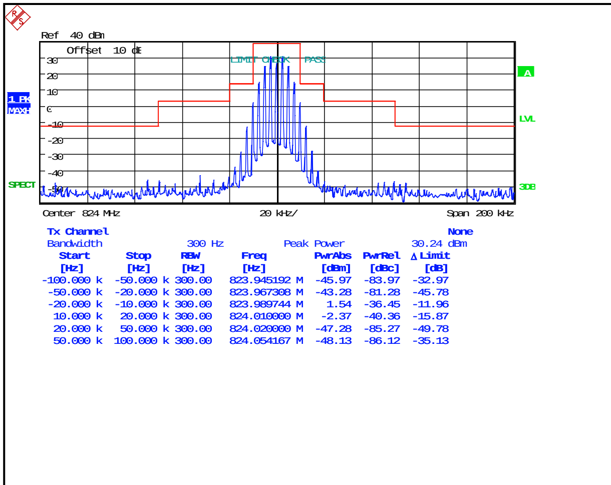
Plot 8-10: Occupied Bandwidth – 824 MHz; Wideband Analog; Mask B
