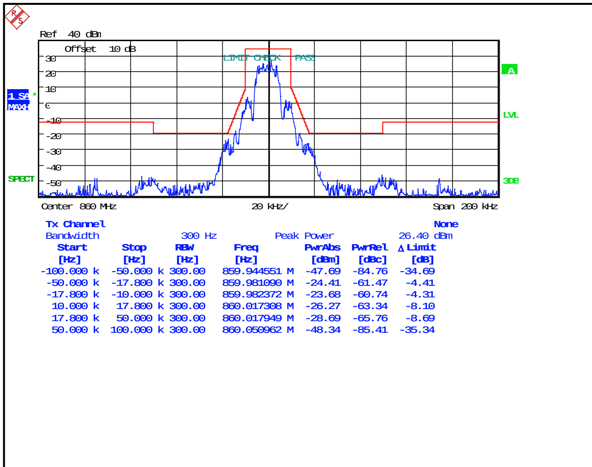
Plot 8-41: Occupied Bandwidth – 860 MHz; 2-level FSK 9600; WB EDACS; Mask G
