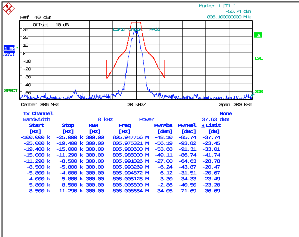
Plot 8-19: Occupied Bandwidth – 806 MHz; P25 RND; Mask H
