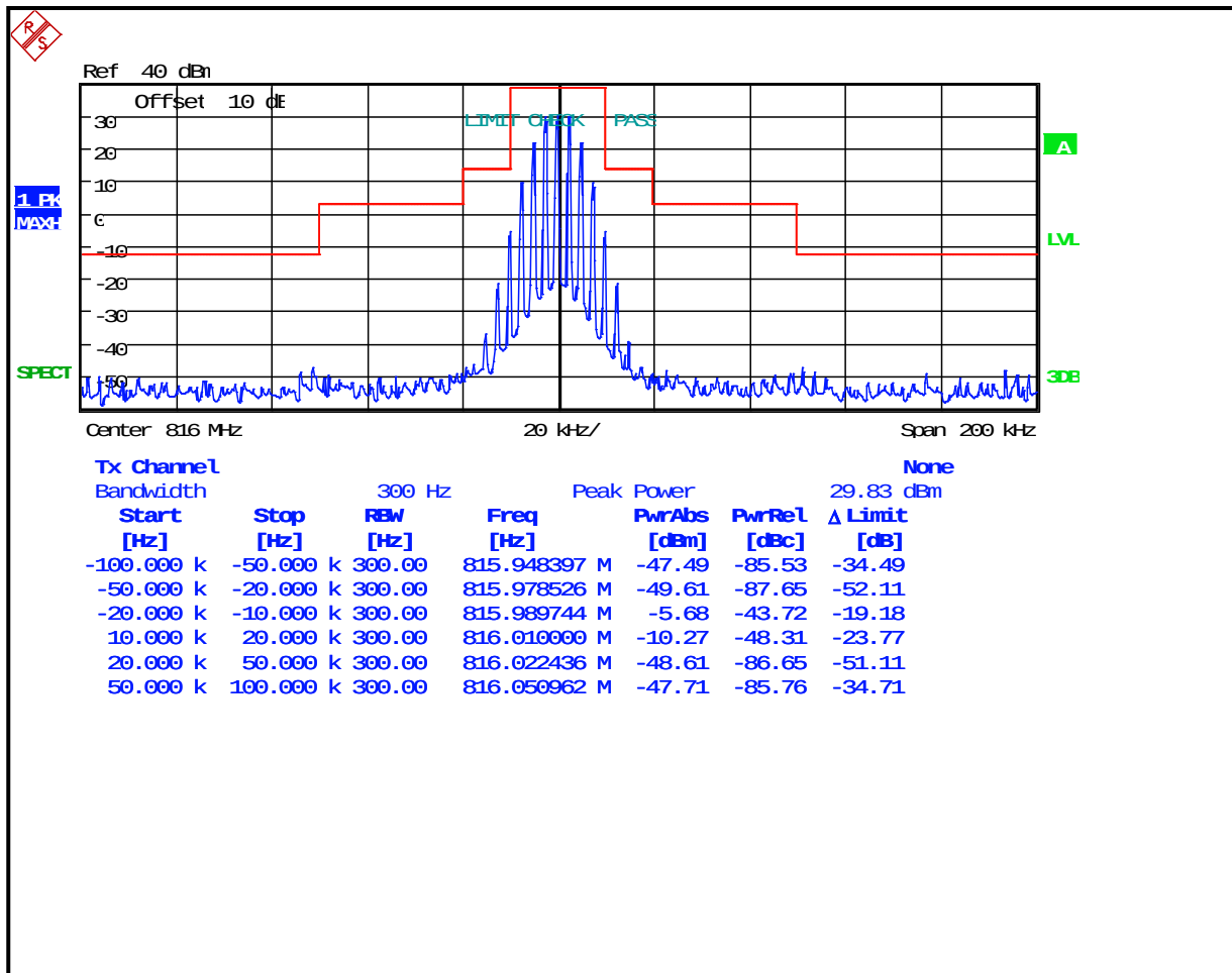
Plot 8-14: Occupied Bandwidth – 816 MHz; NPSPAC; Mask B
