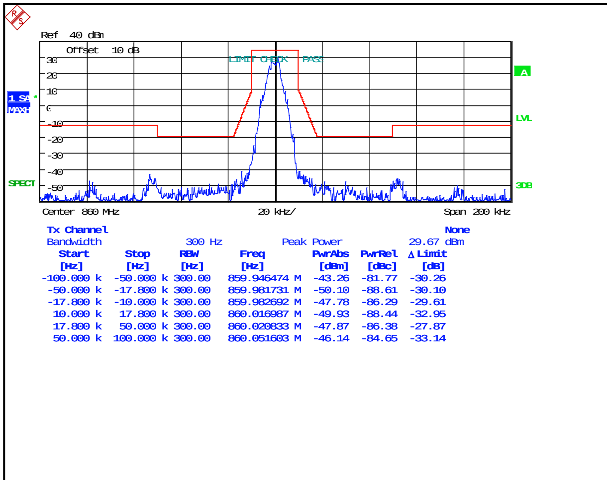
Plot 8-29: Occupied Bandwidth – 860 MHz; CPM TDMA; Mask G
