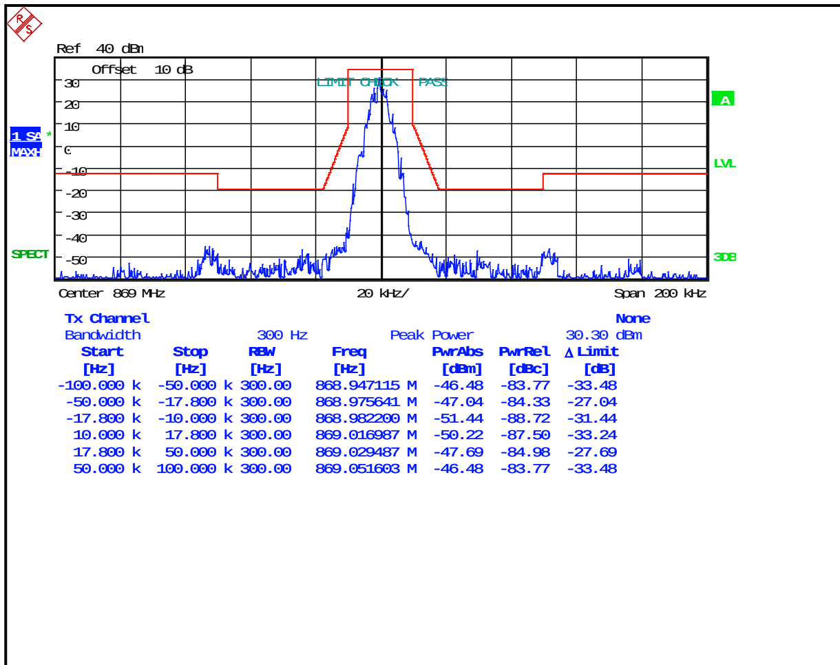
Plot 8-24: Occupied Bandwidth – 869 MHz; P25 RND; Mask G
