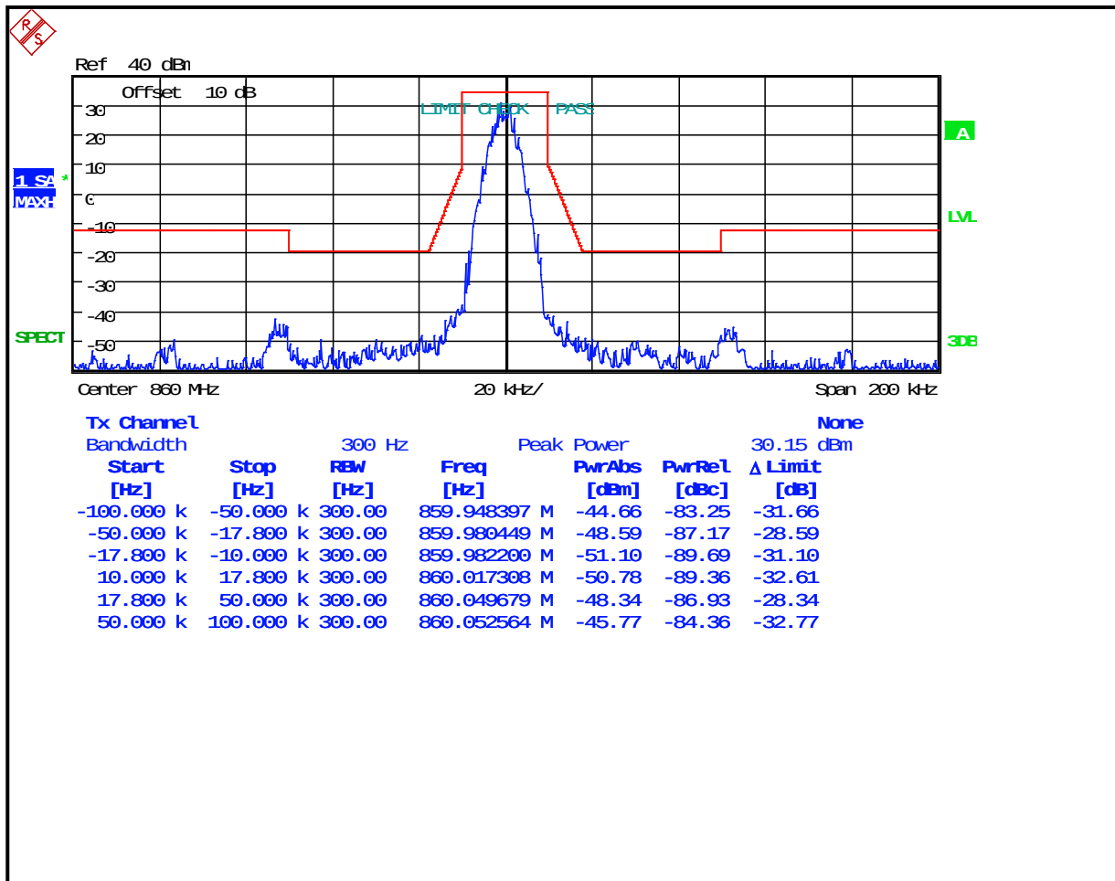
Plot 8-23: Occupied Bandwidth – 860 MHz; P25 RND; Mask G
