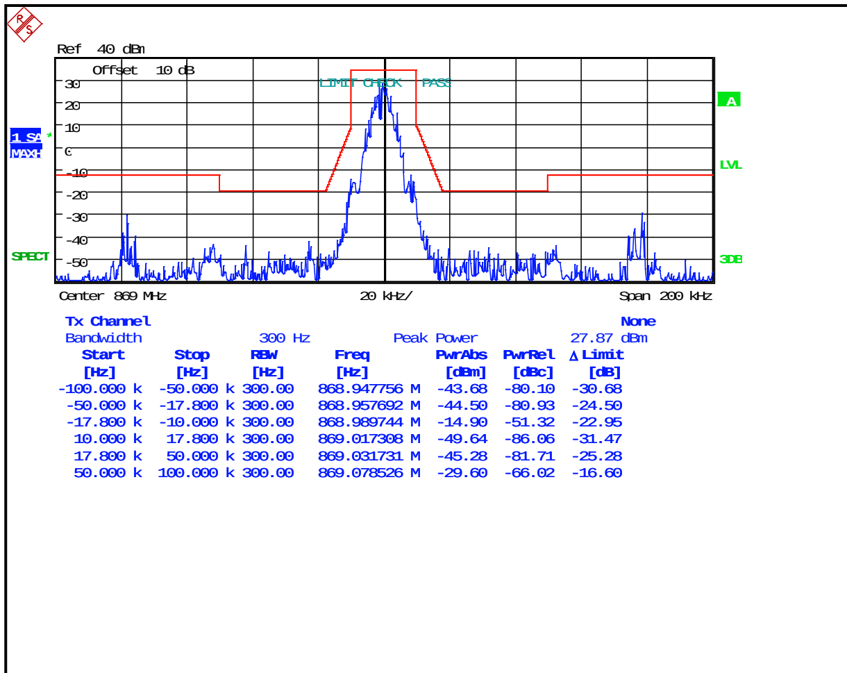
Plot 8-38: Occupied Bandwidth – 869 MHz; 2-level FSK 9600; NB EDACS; Mask G
