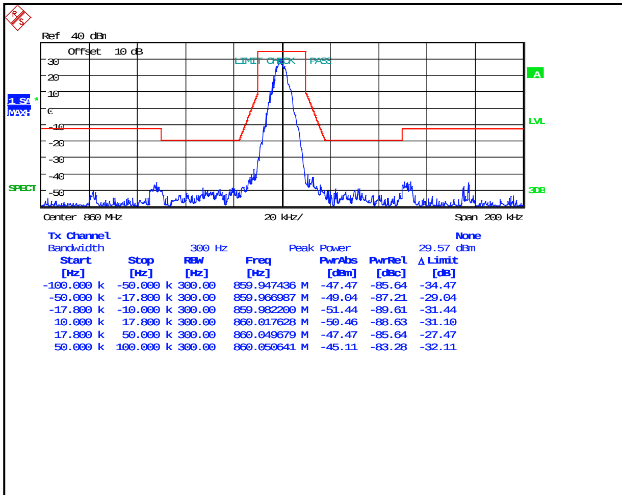
Plot 8-33: Occupied Bandwidth – 860 MHz; 4-level FSK Data/Voice; NB OpenSky; Mask G
