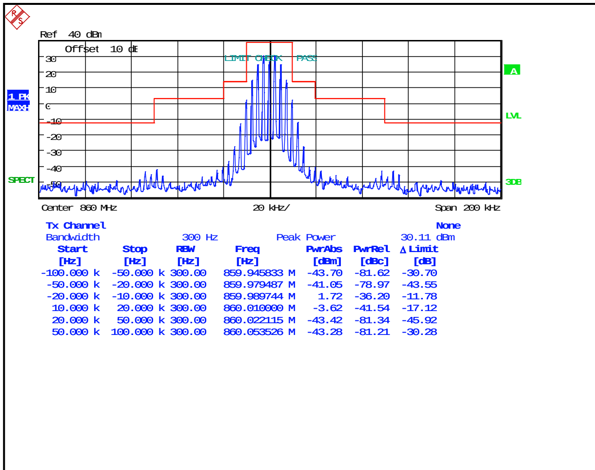
Plot 8-11: Occupied Bandwidth – 860 MHz; Wideband Analog; Mask B
