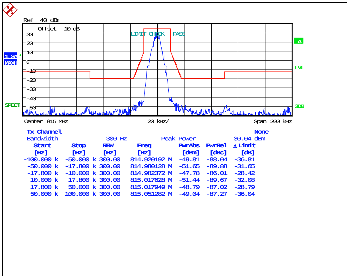
Plot 8-31: Occupied Bandwidth – 815 MHz; 4-level FSK Data/Voice; NB OpenSky; Mask G
