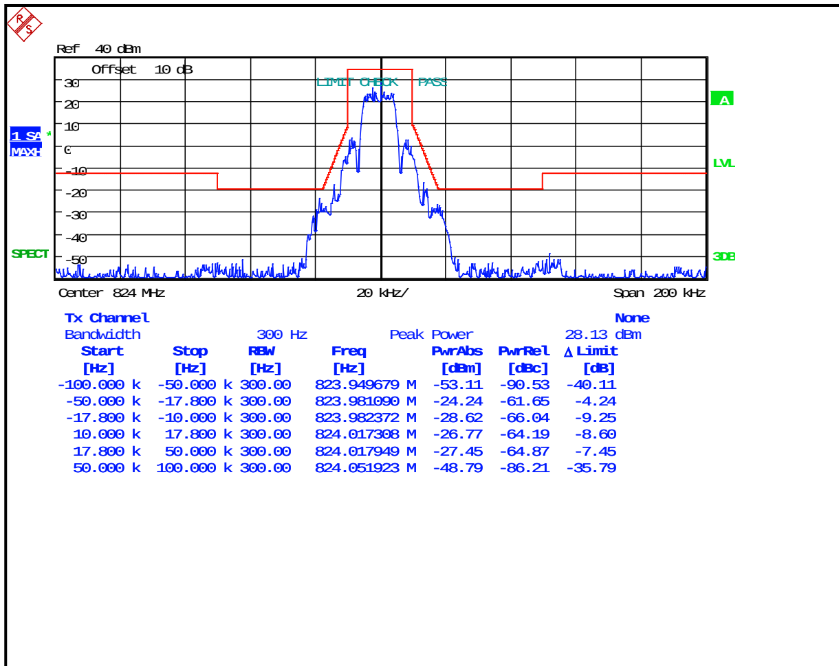
Plot 8-40: Occupied Bandwidth – 824 MHz; 2-level FSK 9600; WB EDACS; Mask G
