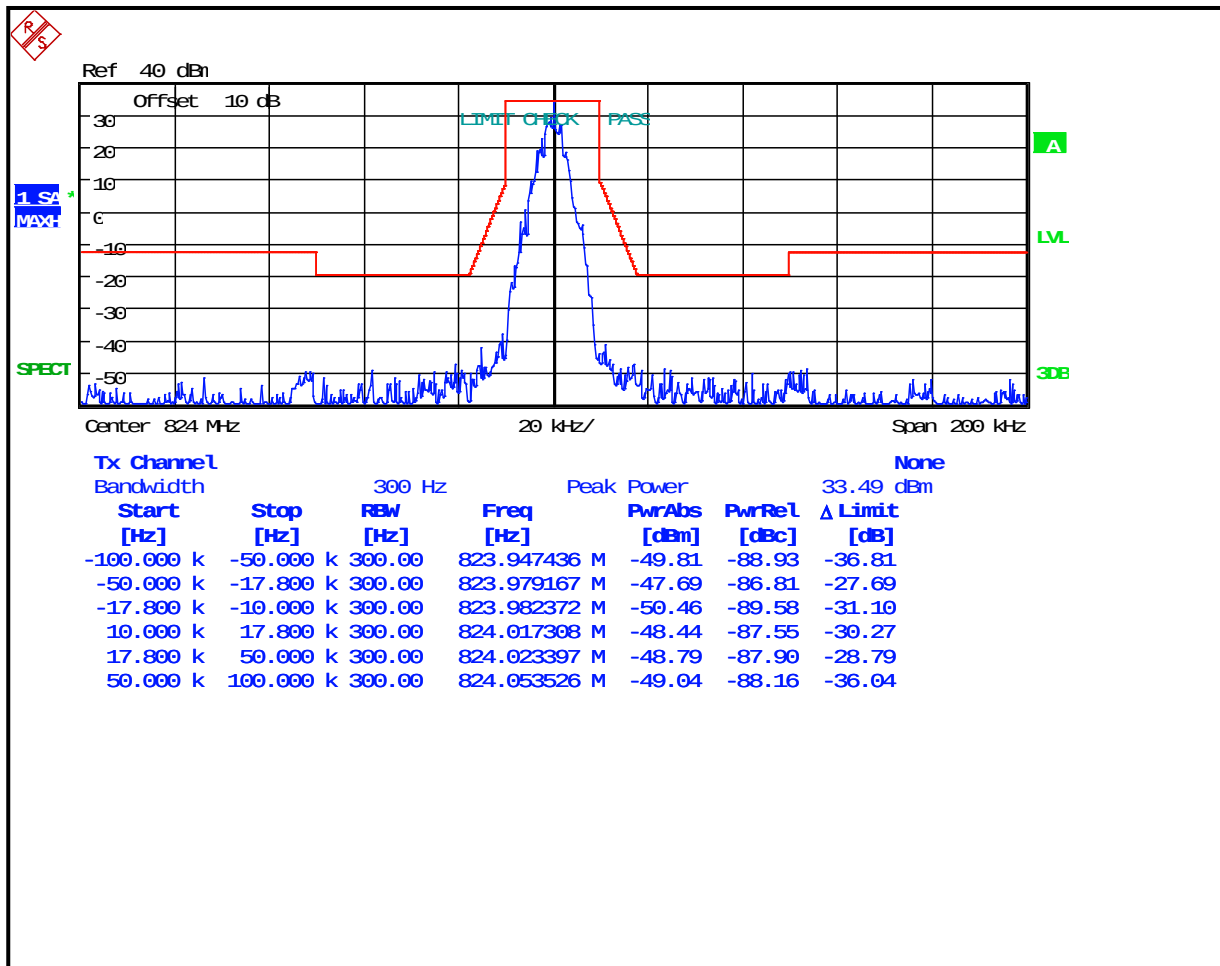
Plot 8-32: Occupied Bandwidth – 824 MHz; 4-level FSK Data/Voice; NB OpenSky; Mask G
