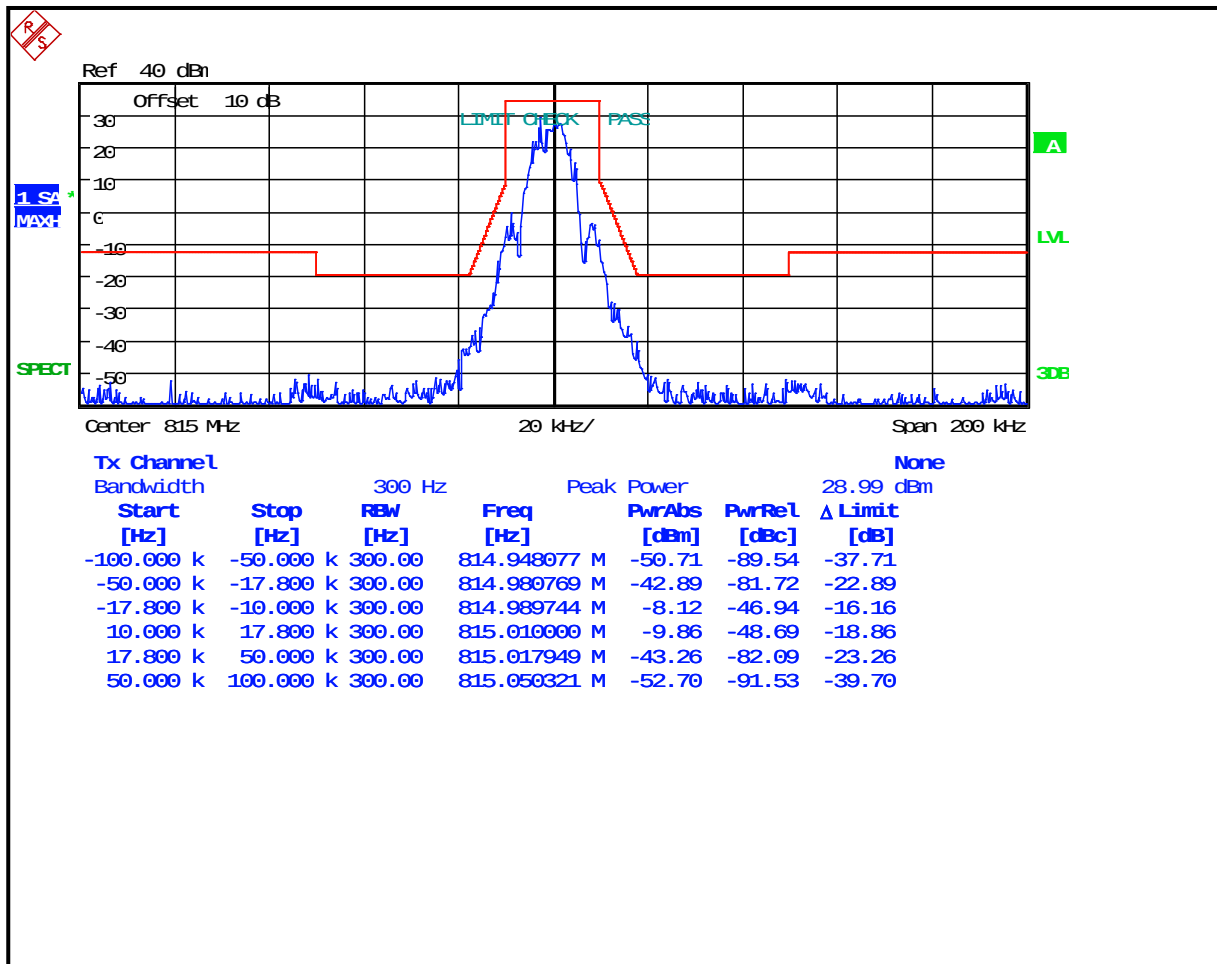
Plot 8-44: Occupied Bandwidth – 815 MHz; 4-level FSK Data/Voice; NB NPSPAC EDACS; Mask G
