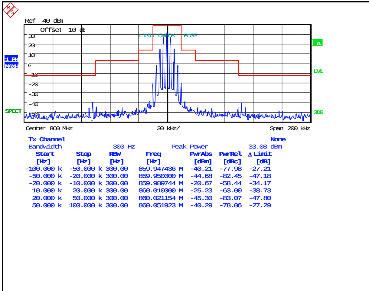
Plot 8-6: Occupied Bandwidth – 860 MHz; Narrowband Analog; Mask B
