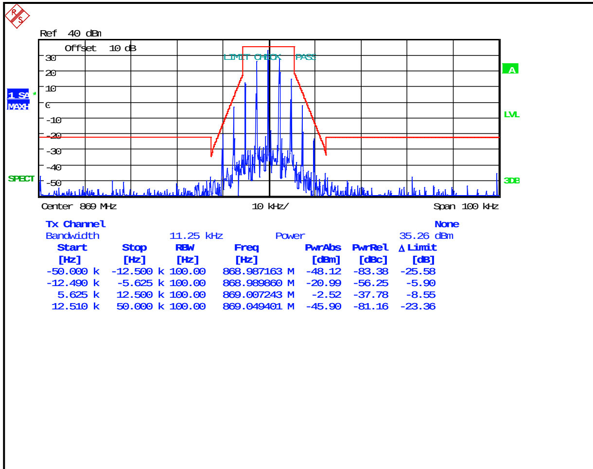
Plot 8-7: Occupied Bandwidth – 869 MHz; Narrowband Analog; Mask D
