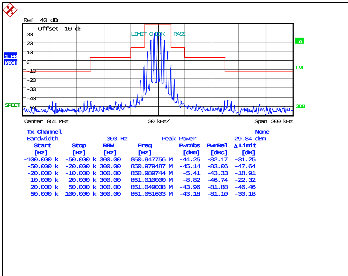
Plot 8-16: Occupied Bandwidth – 851 MHz; NPSPAC; Mask B
