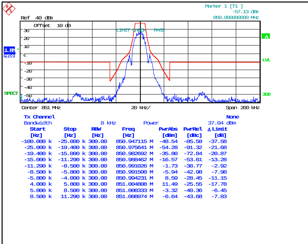
Plot 8-49: Occupied Bandwidth – 851 MHz; 4-level FSK Data/Voice; NPSPAC OpenSky; Mask H
