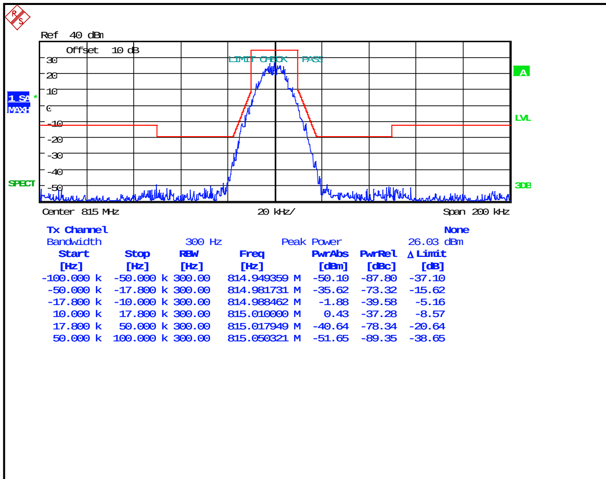
Plot 8-50: Occupied Bandwidth – 815 MHz; 4-level FSK Data/Voice; SMR OpenSky; Mask G
