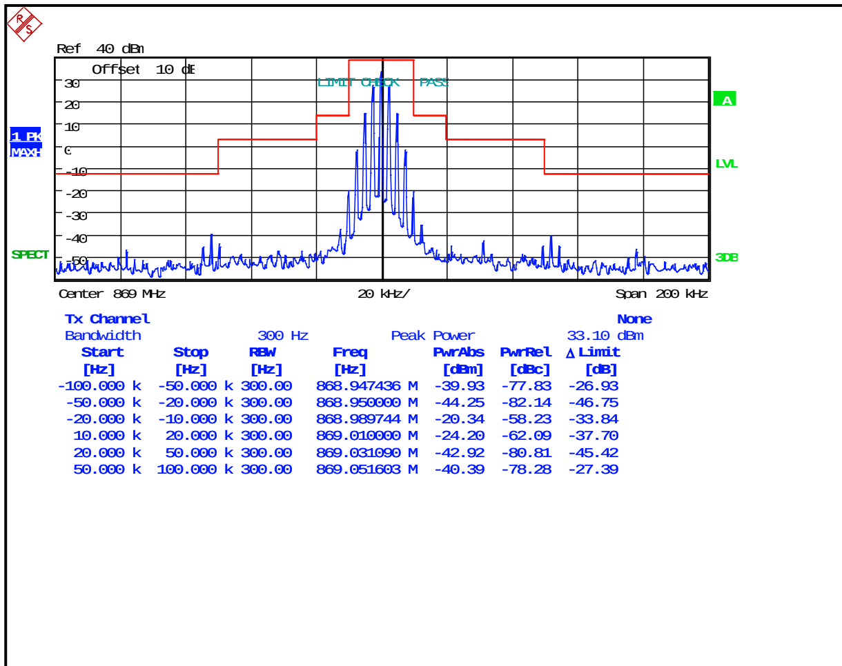
Plot 8-8: Occupied Bandwidth – 869 MHz; Narrowband Analog; Mask B
