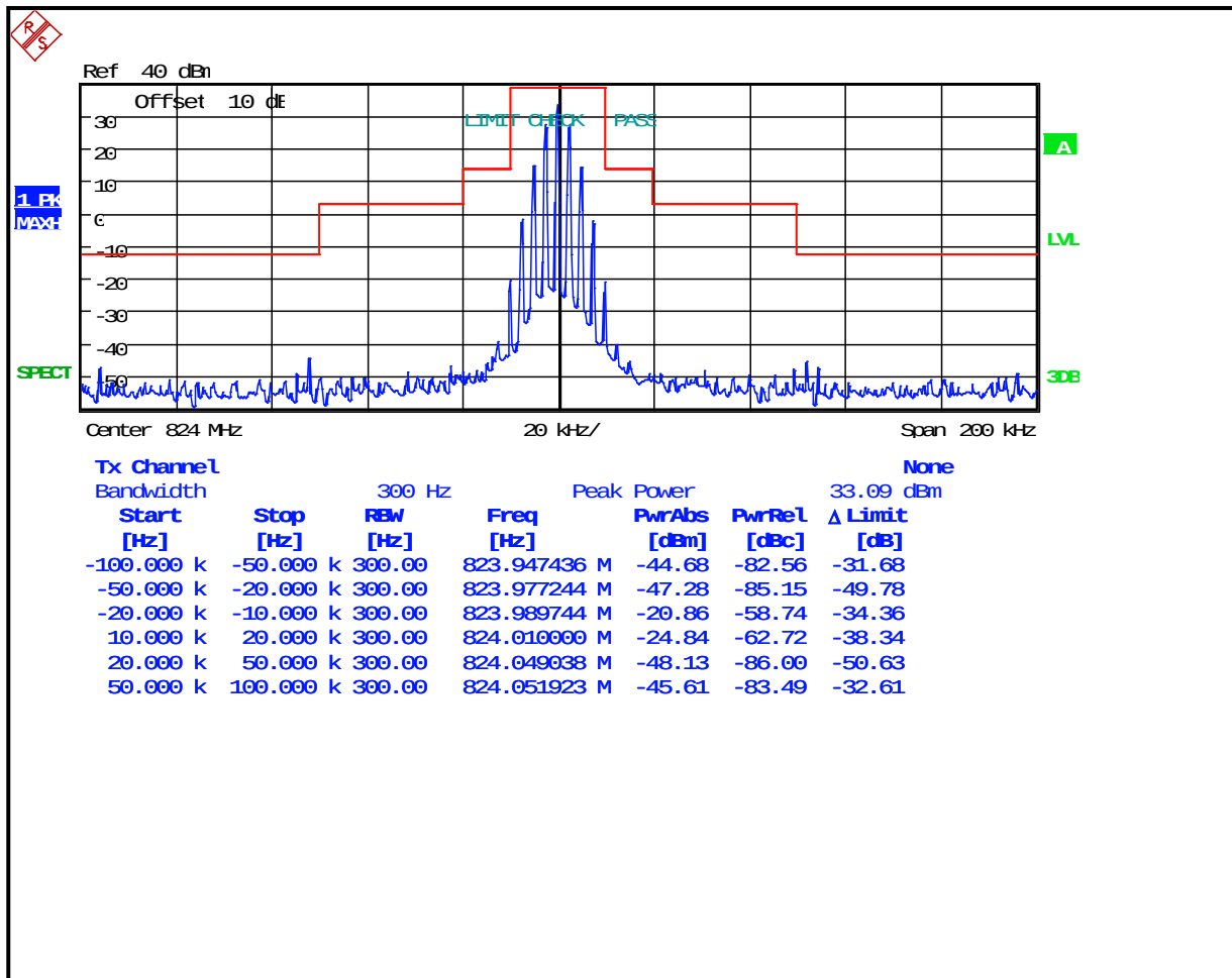
Plot 8-4: Occupied Bandwidth – 824 MHz; Narrowband Analog; Mask B
