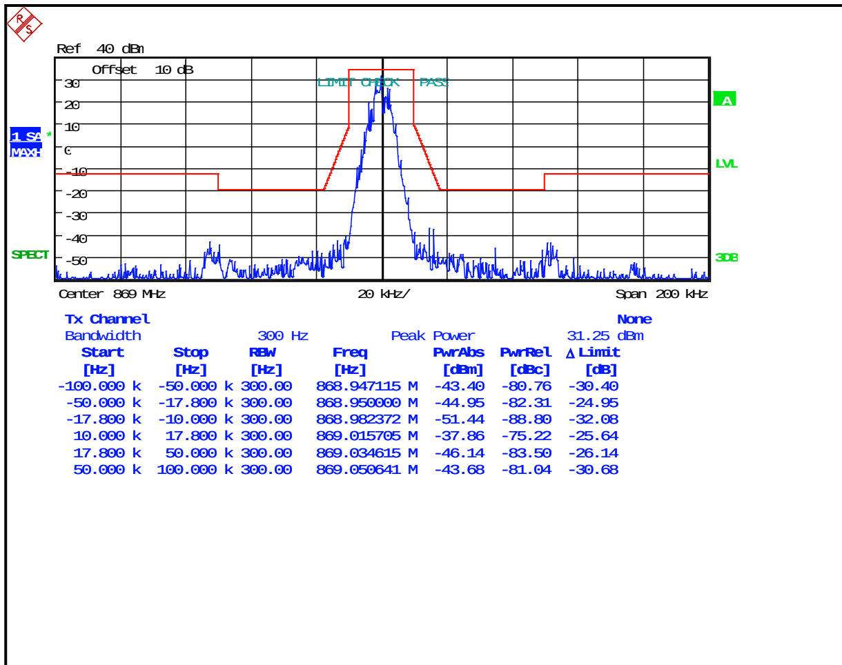
Plot 8-30: Occupied Bandwidth – 869 MHz; CPM TDMA; Mask G
