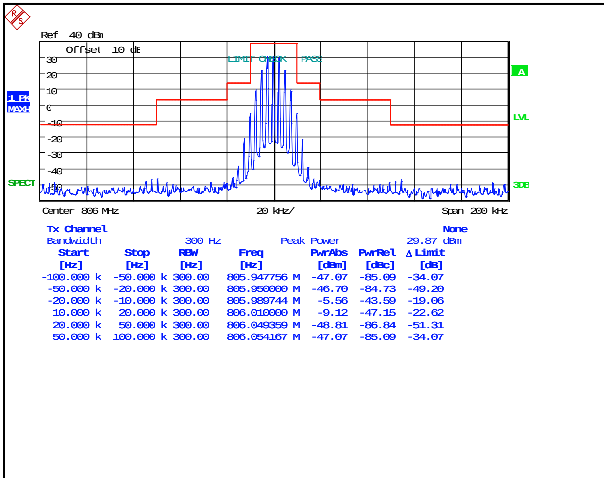
Plot 8-13: Occupied Bandwidth – 806 MHz; NPSPAC; Mask B
