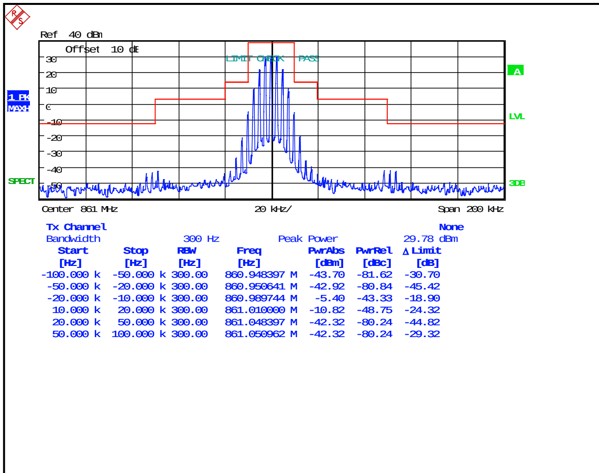
Plot 8-17: Occupied Bandwidth – 861 MHz; NPSPAC; Mask B
