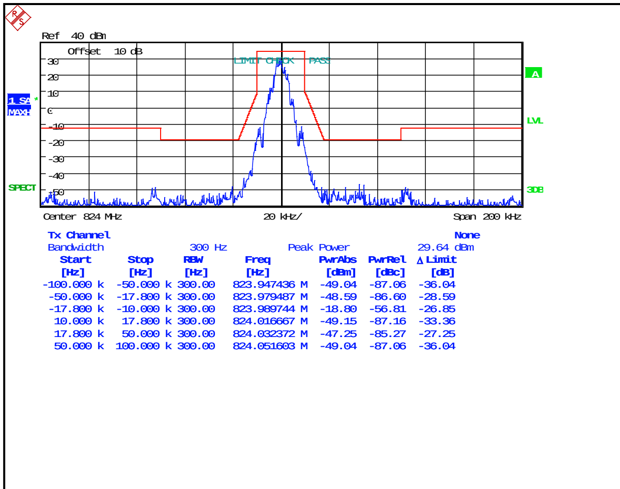
Plot 8-36: Occupied Bandwidth – 824 MHz; 2-level FSK 9600; NB EDACS; Mask G
