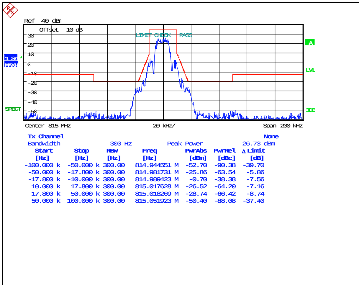
Plot 8-39: Occupied Bandwidth – 815 MHz; 2-level FSK 9600; WB EDACS; Mask G
