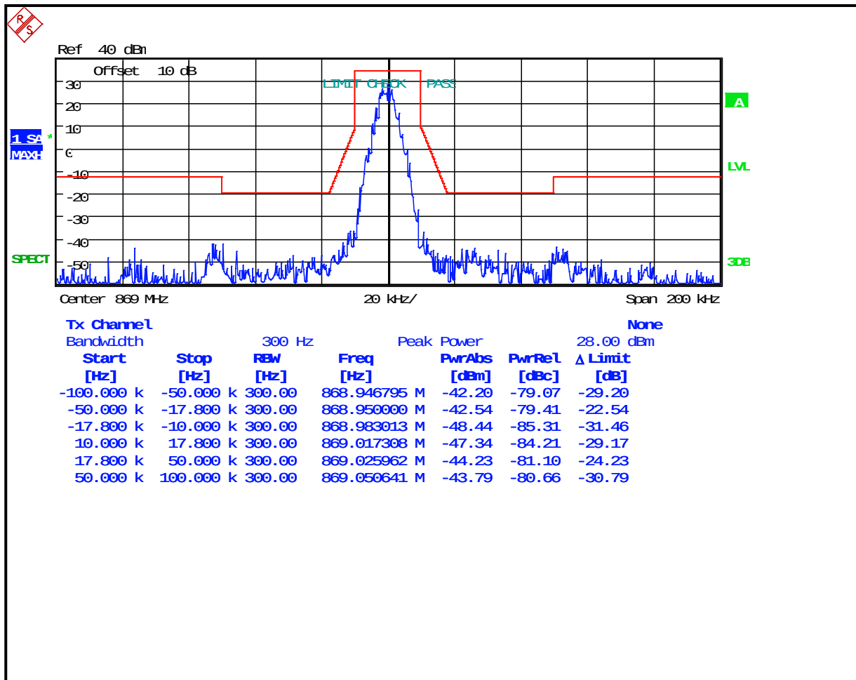
Plot 8-34: Occupied Bandwidth – 869 MHz; 4-level FSK Data/Voice; NB OpenSky; Mask G
