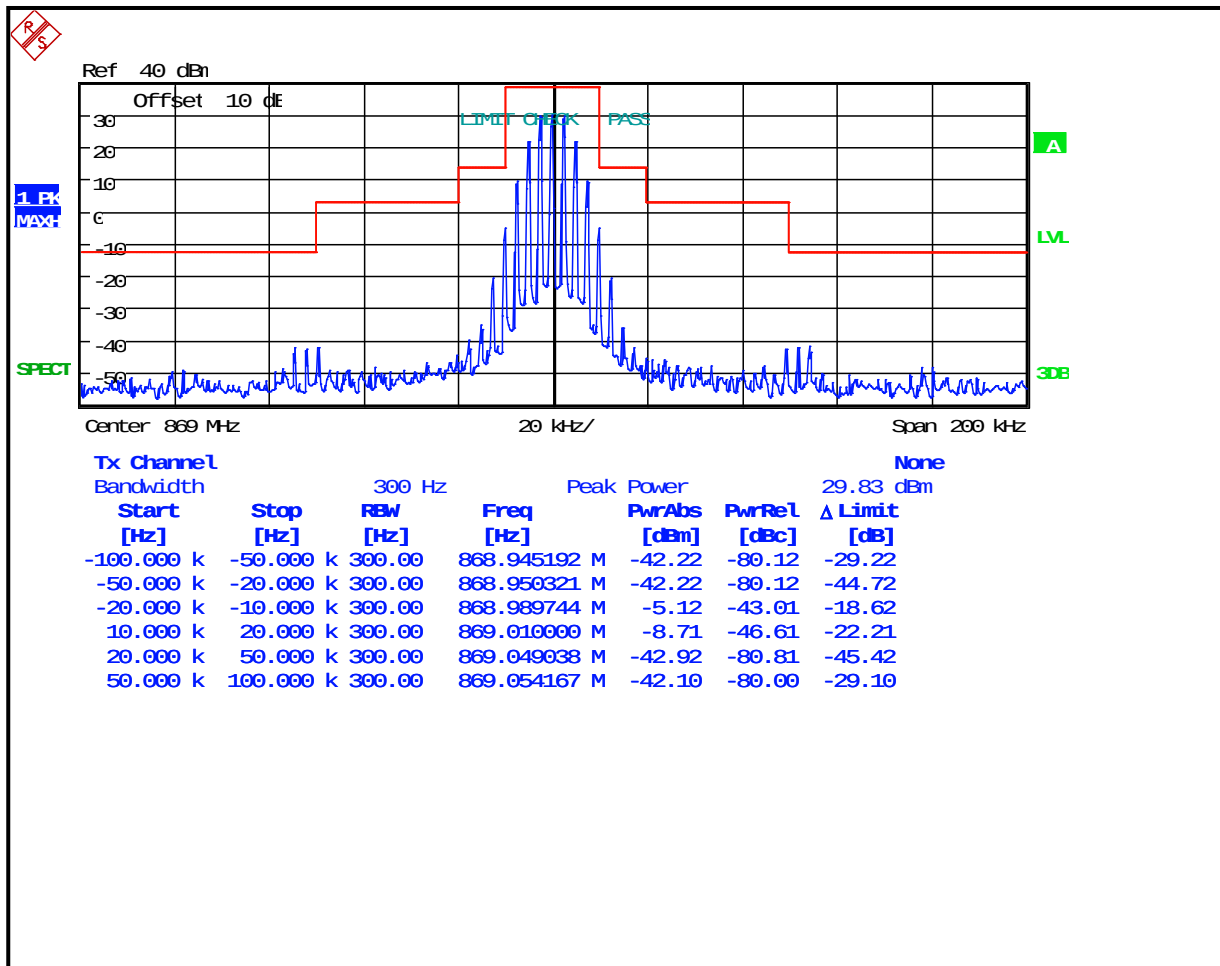
Plot 8-18: Occupied Bandwidth – 869 MHz; NPSPAC; Mask B
