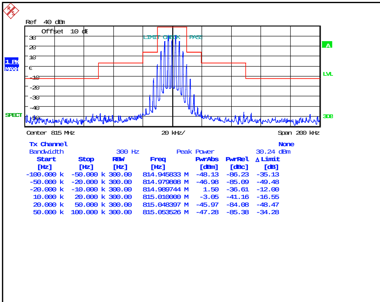
Plot 8-9: Occupied Bandwidth – 815 MHz; Wideband Analog; Mask B
