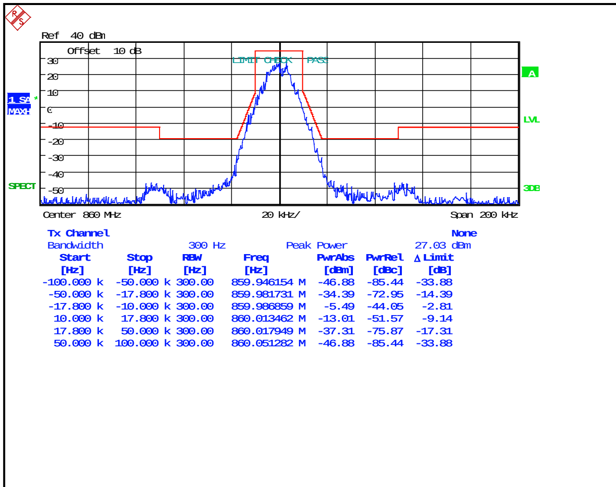
Plot 8-52: Occupied Bandwidth – 860 MHz; 4-level FSK Data/Voice; SMR OpenSky; Mask G
