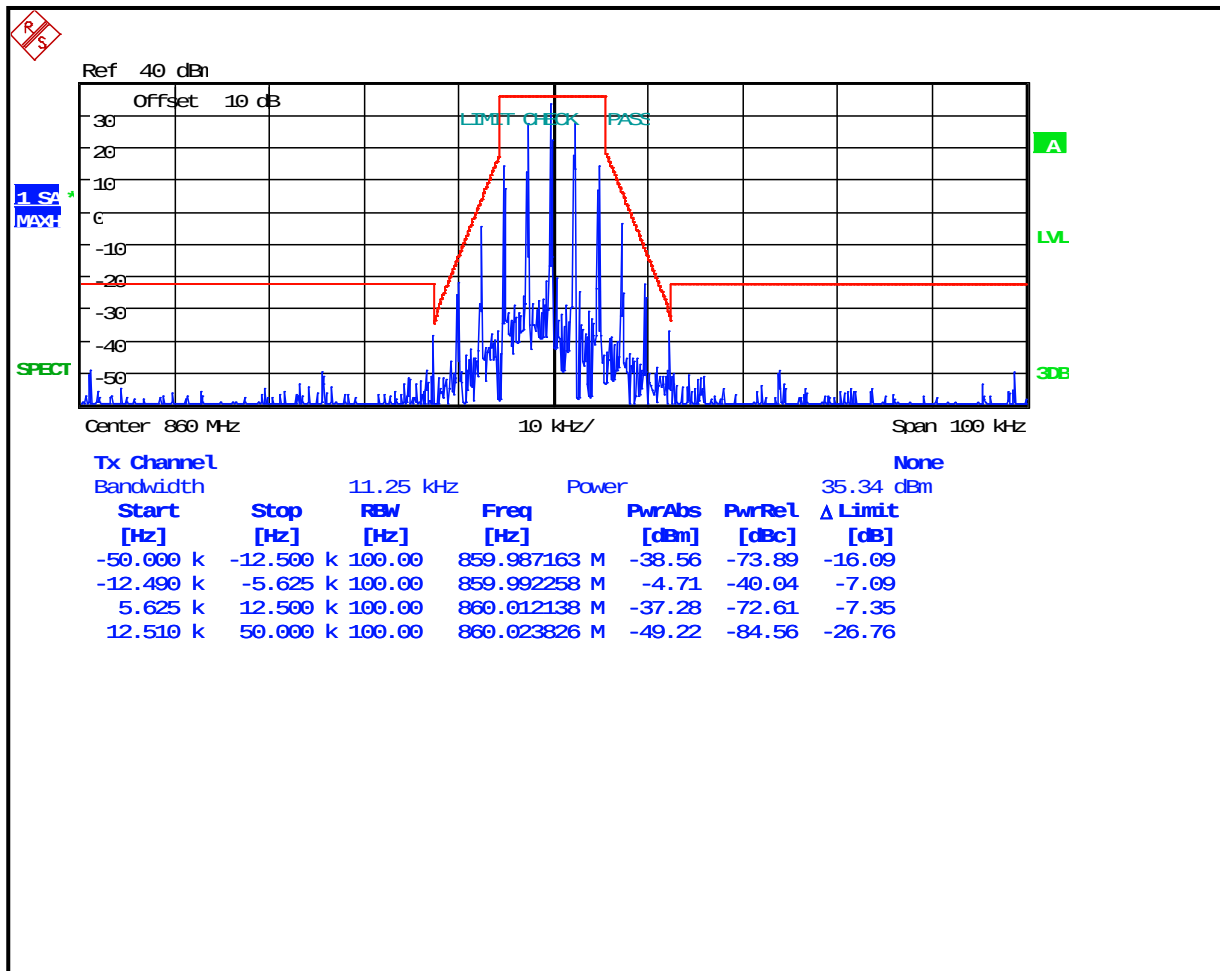
Plot 8-5: Occupied Bandwidth – 860 MHz; Narrowband Analog; Mask D
