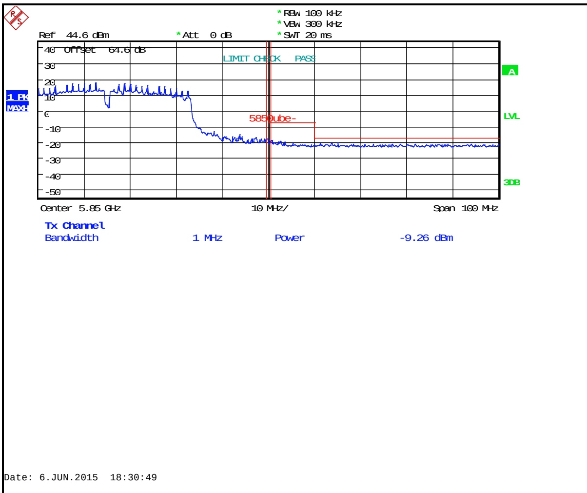
Plot 6-23: Upper Band Edge: Measurement Channel 165 (5825 MHz, 40 MHz BW, 802.11n, Peak)
