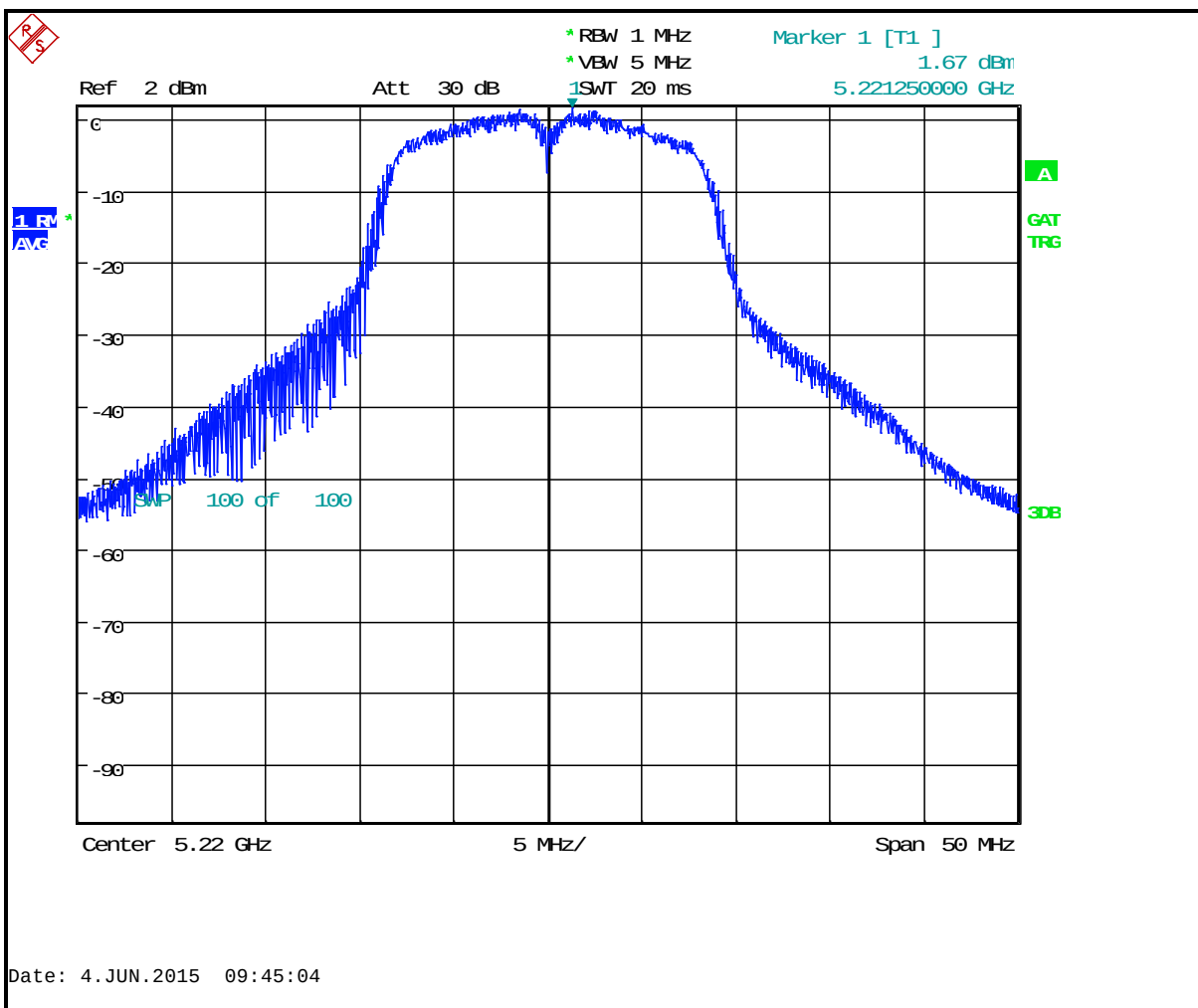
Plot 4-10: Peak Power Spectral Density: Channel 44 (5220 MHz) 802.11n 65 Mbps
