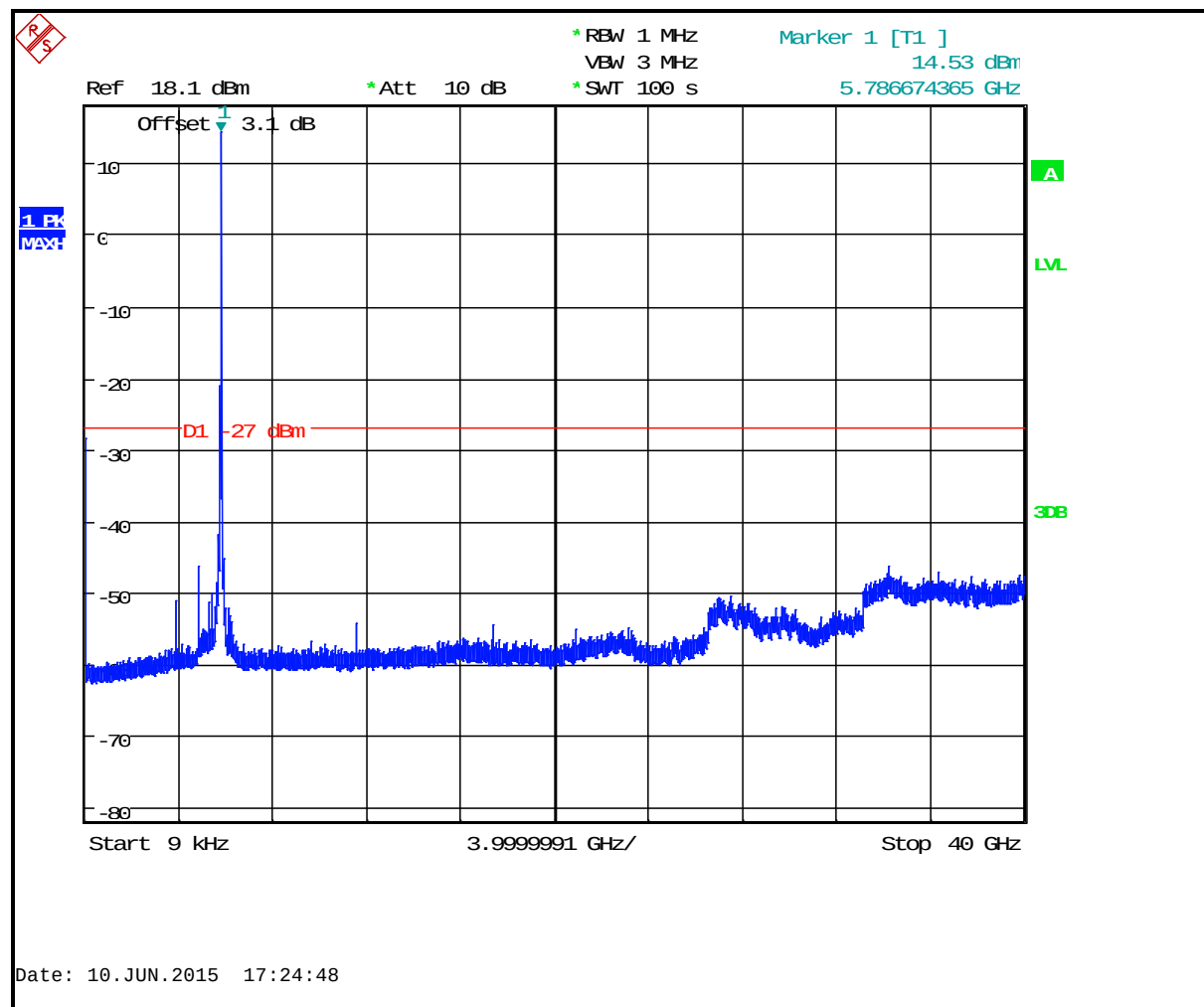
Plot 7-8: Undesirable Emissions Channel 157(5785 MHz)
