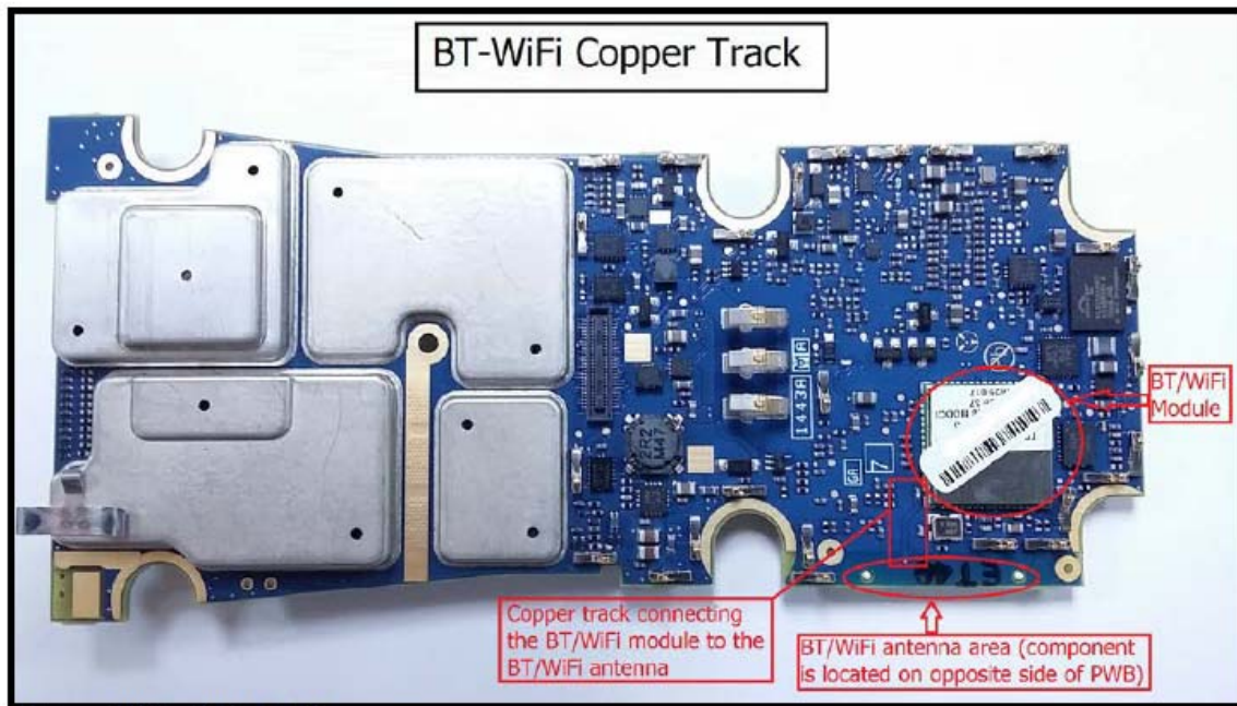
Bottom PWB with Shields
