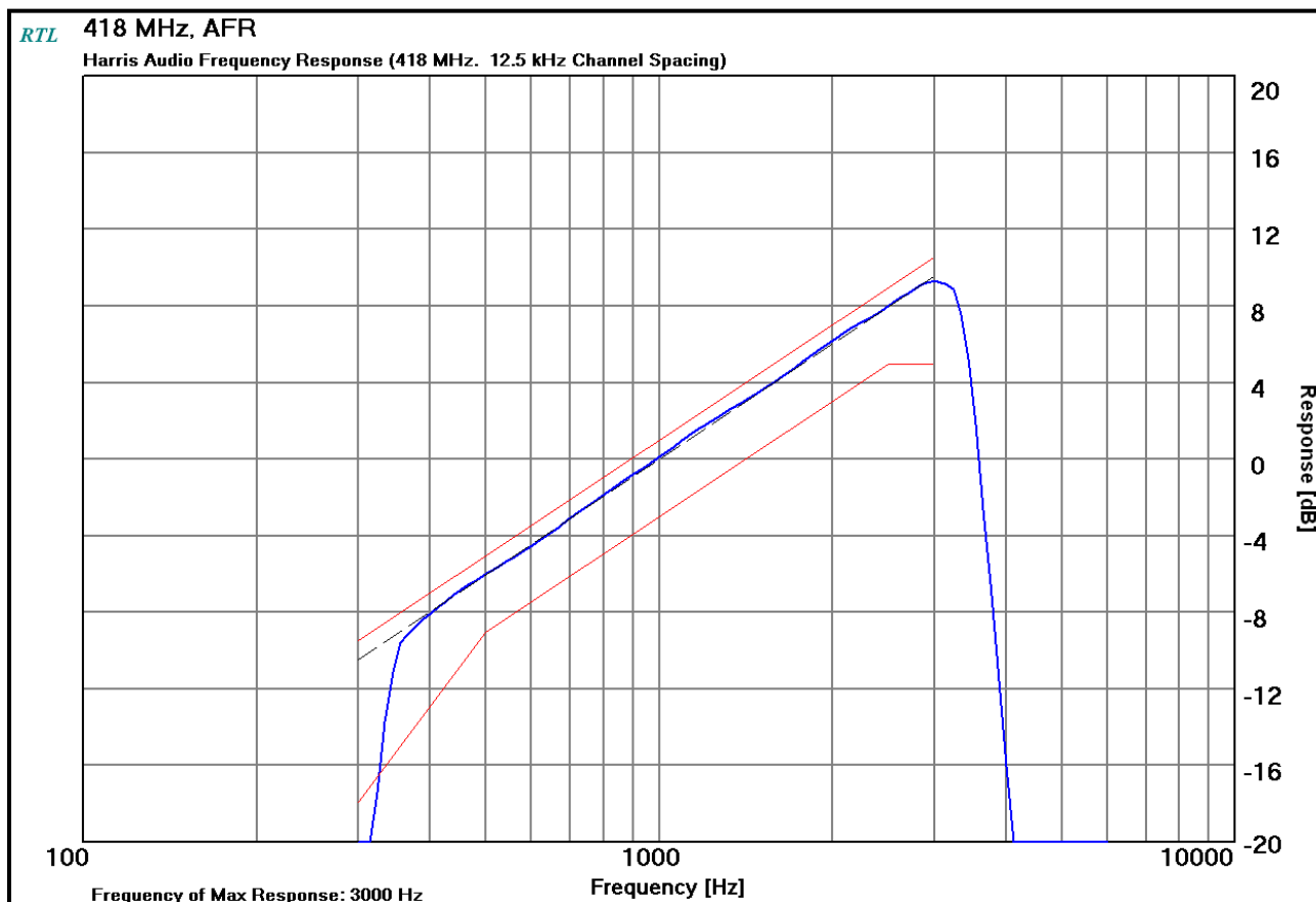
Plot 9-1: Modulation Characteristics - Audio Frequency Response - 418 MHz
