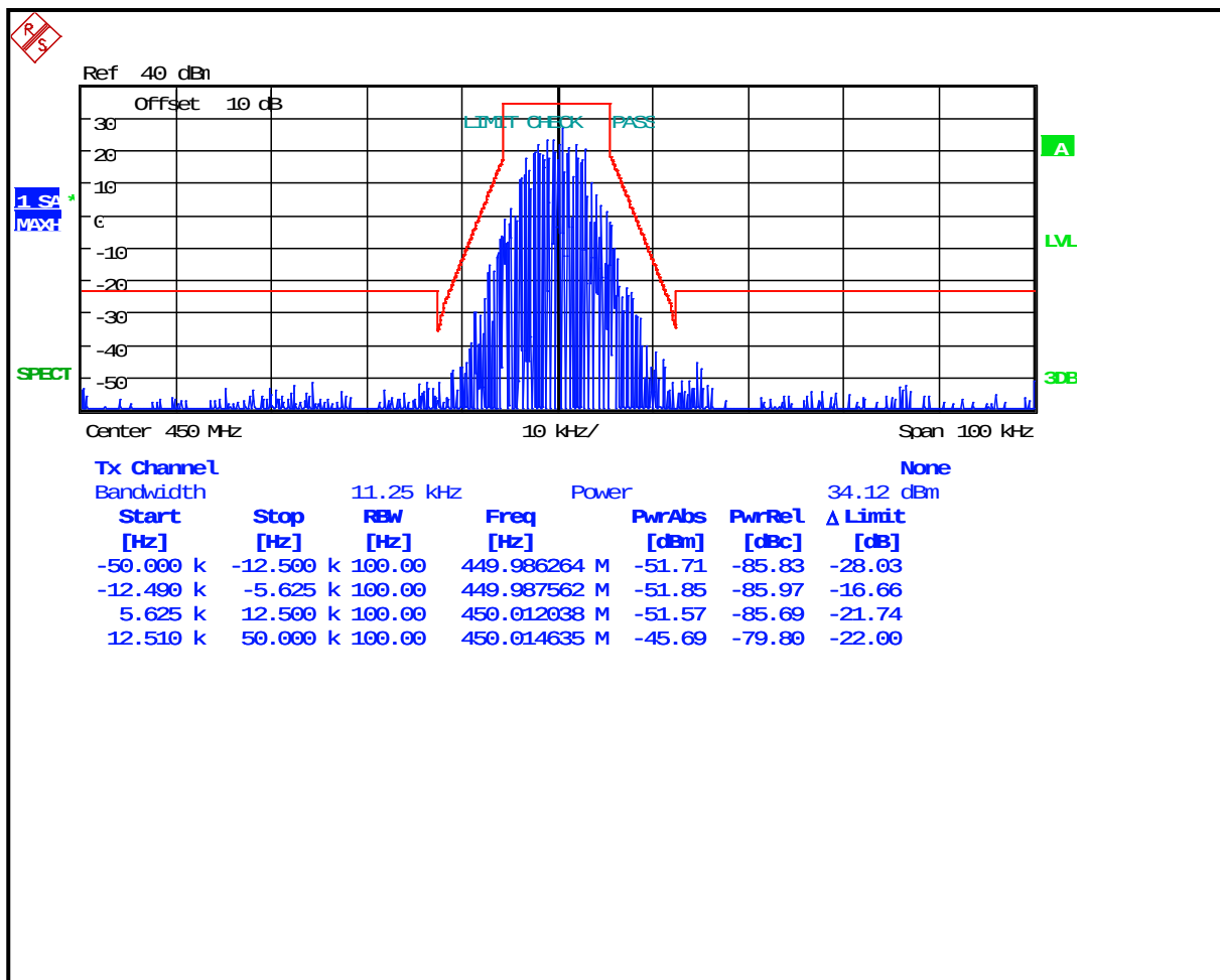
Plot 7-23: Occupied Bandwidth – 450 MHz; CPM TDMA; Mask D
