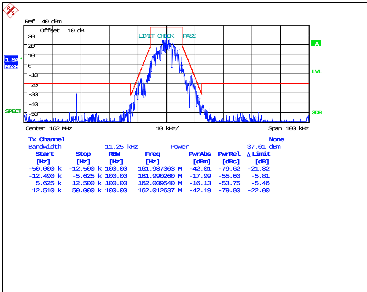
Plot 7-27: Occupied Bandwidth – 162 MHz; 2-Level FSK 49600; NB EDACS; (Mask D)
