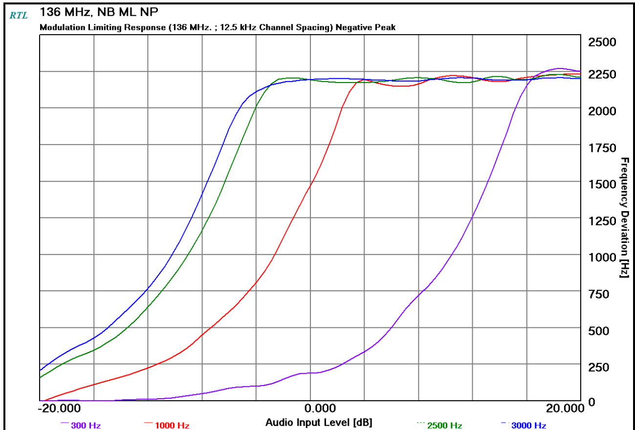
Plot 9-5: Modulation Characteristics – Modulation Limiting - 136 MHz; Negative Peak; NB
