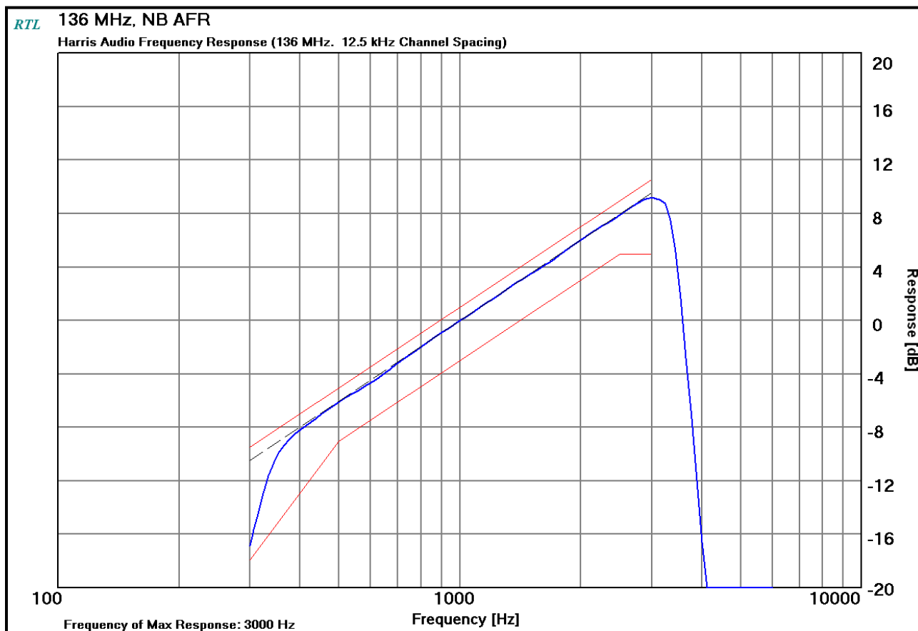
Plot 9-1: Modulation Characteristics - Audio Frequency Response - 136 MHz
