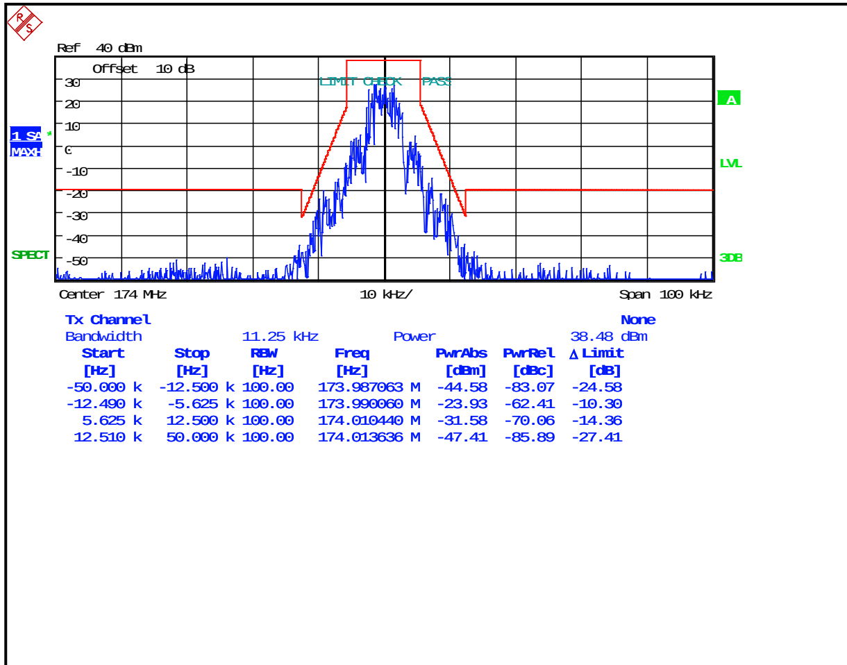
Plot 7-20: Occupied Bandwidth – 174 MHz; 2-Level FSK 4800; XNB EDACS; (Mask D)
