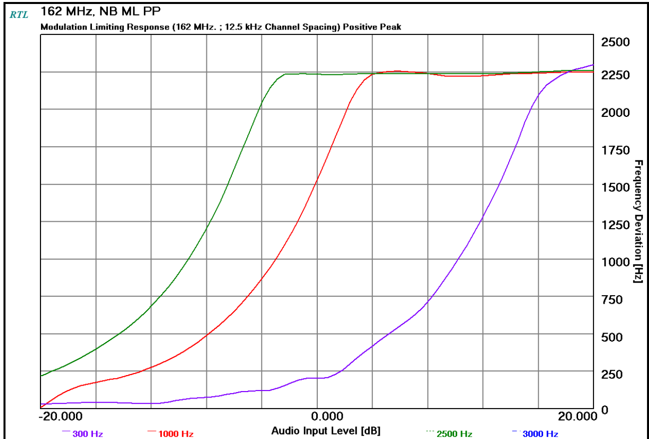
Plot 9-8: Modulation Characteristics – Modulation Limiting - 162 MHz; Positive Peak; NB
