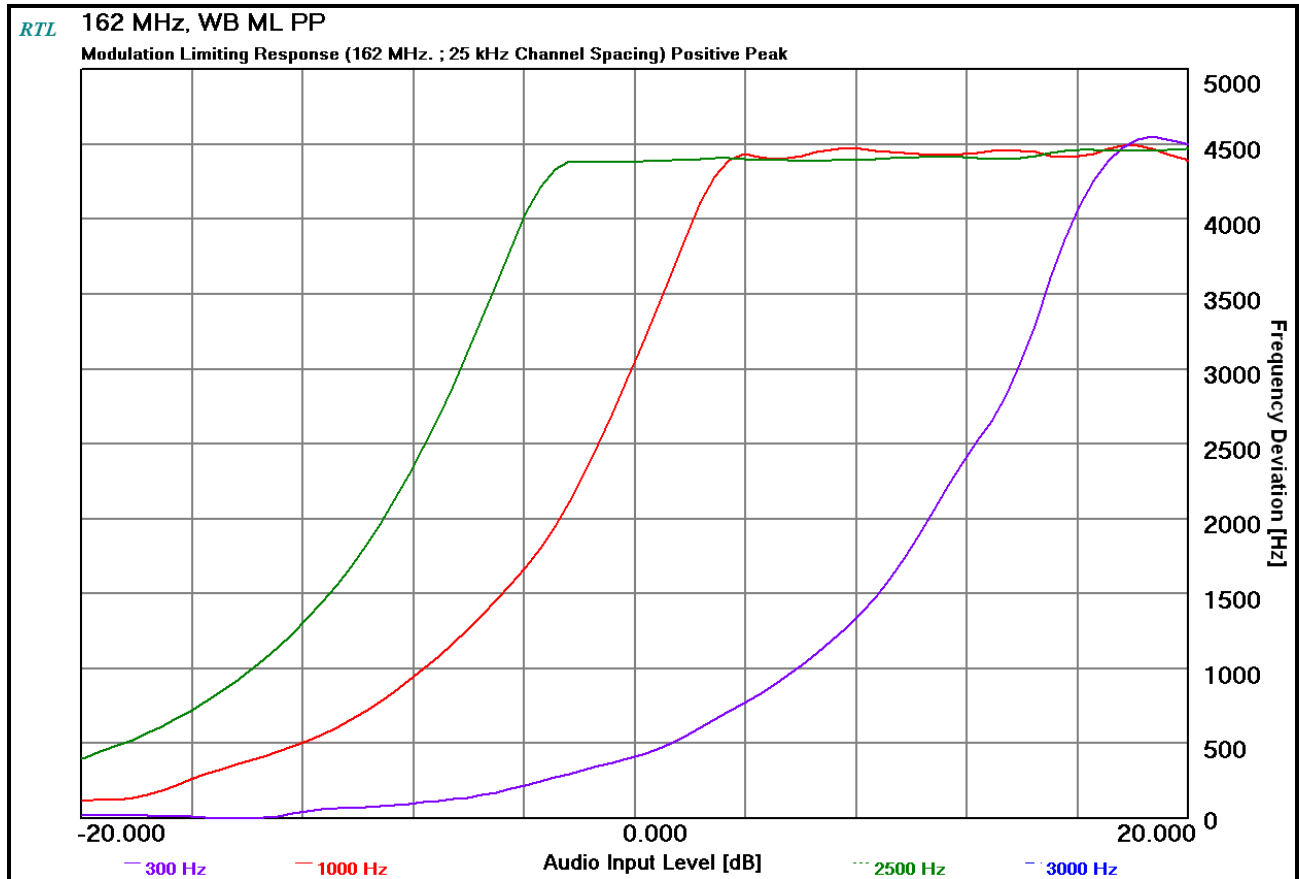
Plot 9-10: Modulation Characteristics – Modulation Limiting - 162 MHz; Positive Peak; WB
