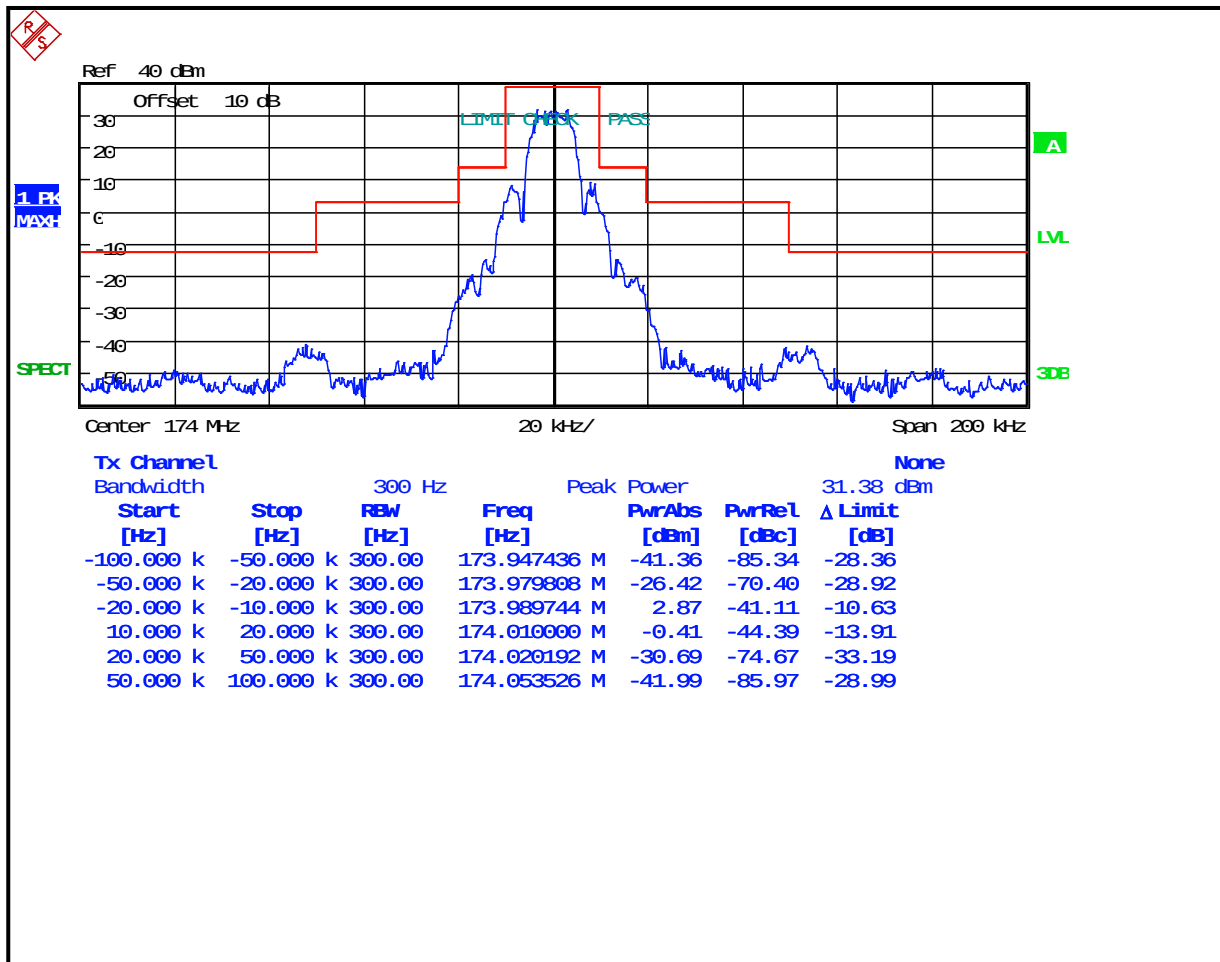
Plot 7-24: Occupied Bandwidth – 174 MHz; 2-Level FSK 9600; WB EDACS; (Mask B)
