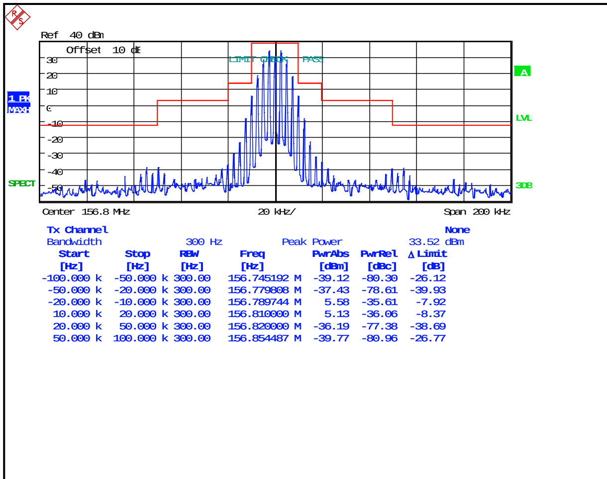
Plot 7-2: Occupied Bandwidth – 156.8 MHz; Analog WB (Mask B)
