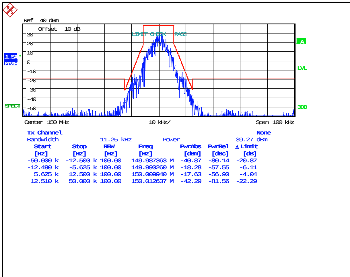
Plot 7-25: Occupied Bandwidth – 150 MHz; 2-Level FSK 9600; NB EDACS; (Mask D)
