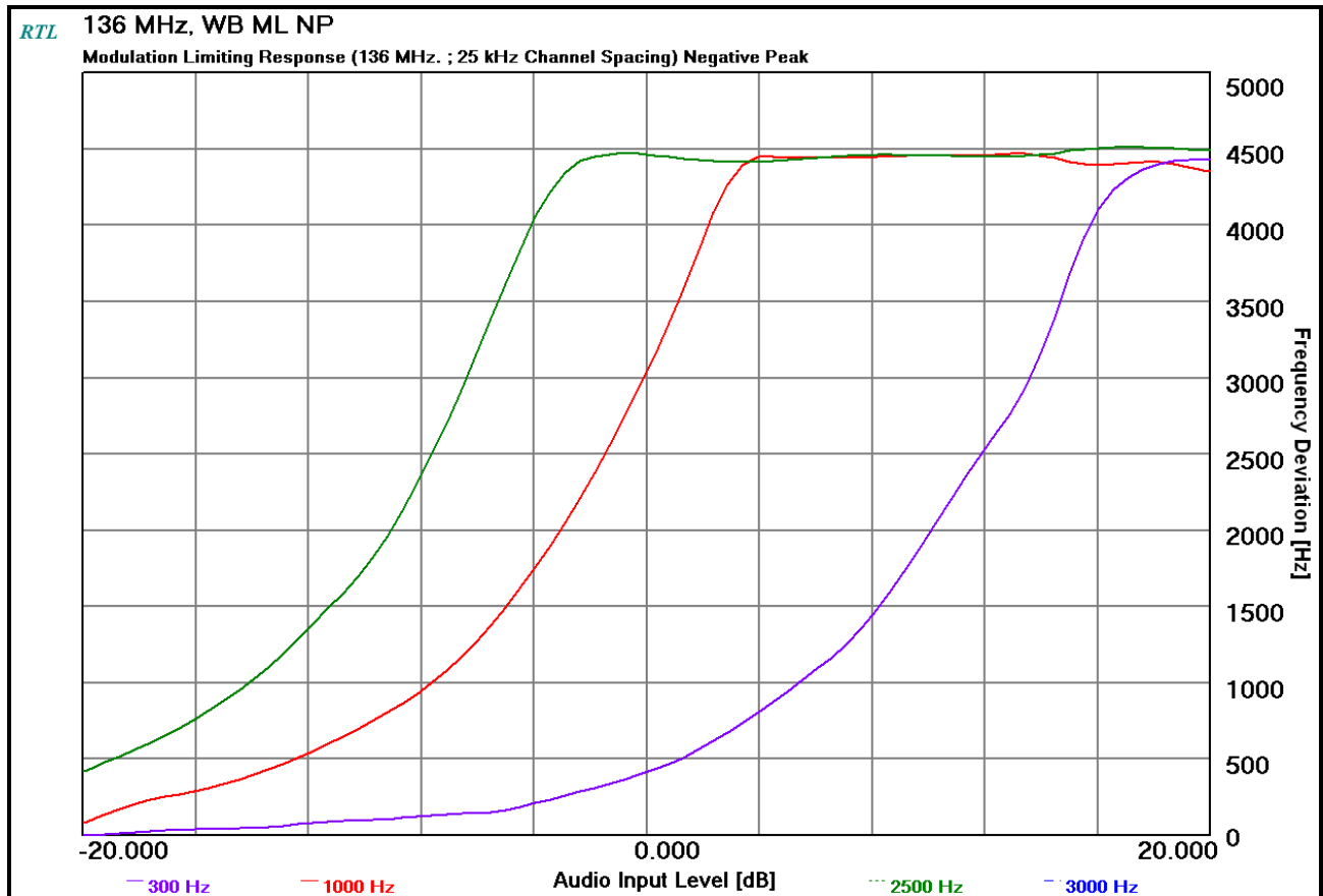
Plot 9-7: Modulation Characteristics – Modulation Limiting - 136 MHz; Negative Peak; WB
