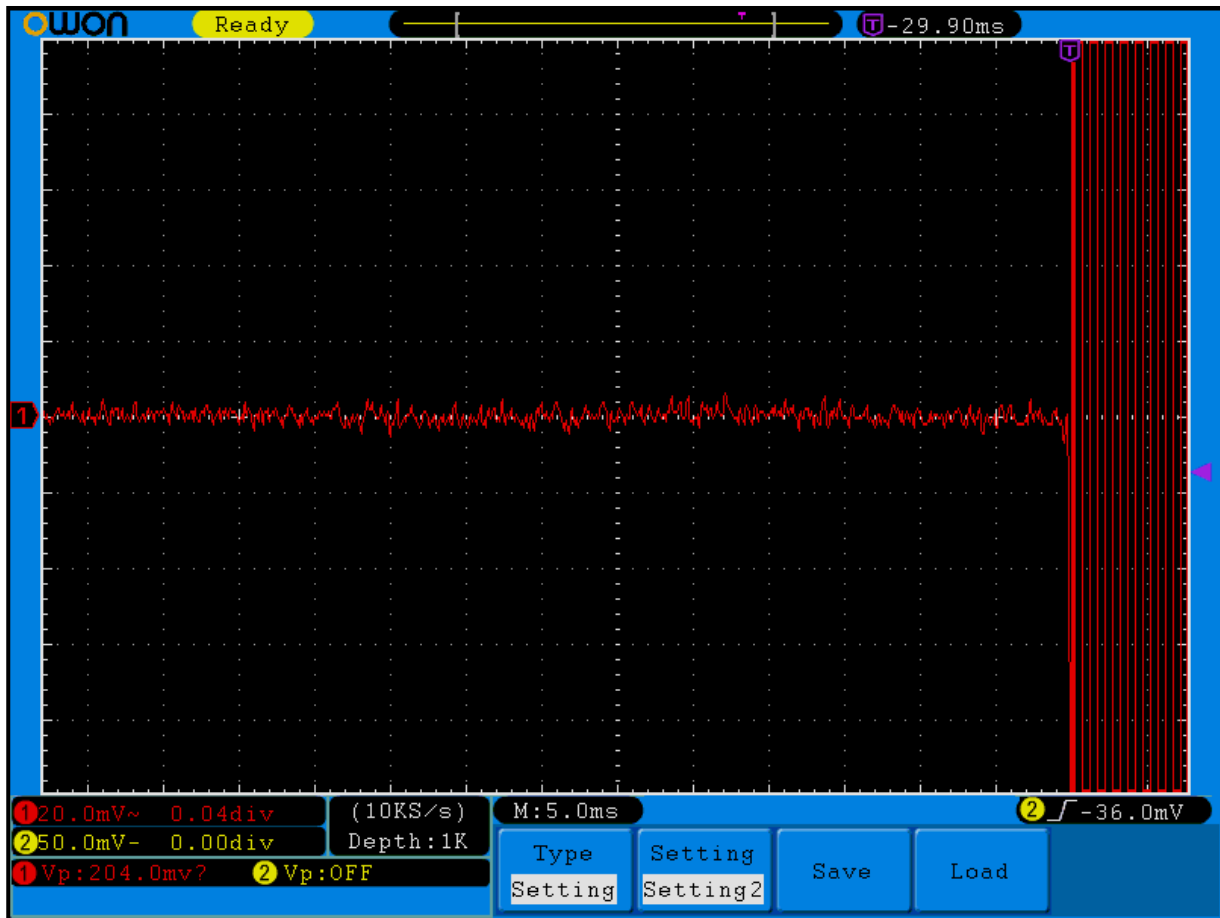
Plot 10-2: Transient Frequency Behavior – 162 MHz; High Power; Narrowband; Carrier OFF Time
