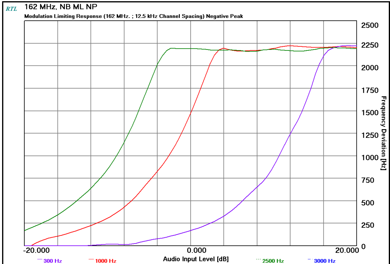
Plot 9-9: Modulation Characteristics – Modulation Limiting - 162 MHz; Negative Peak; NB
