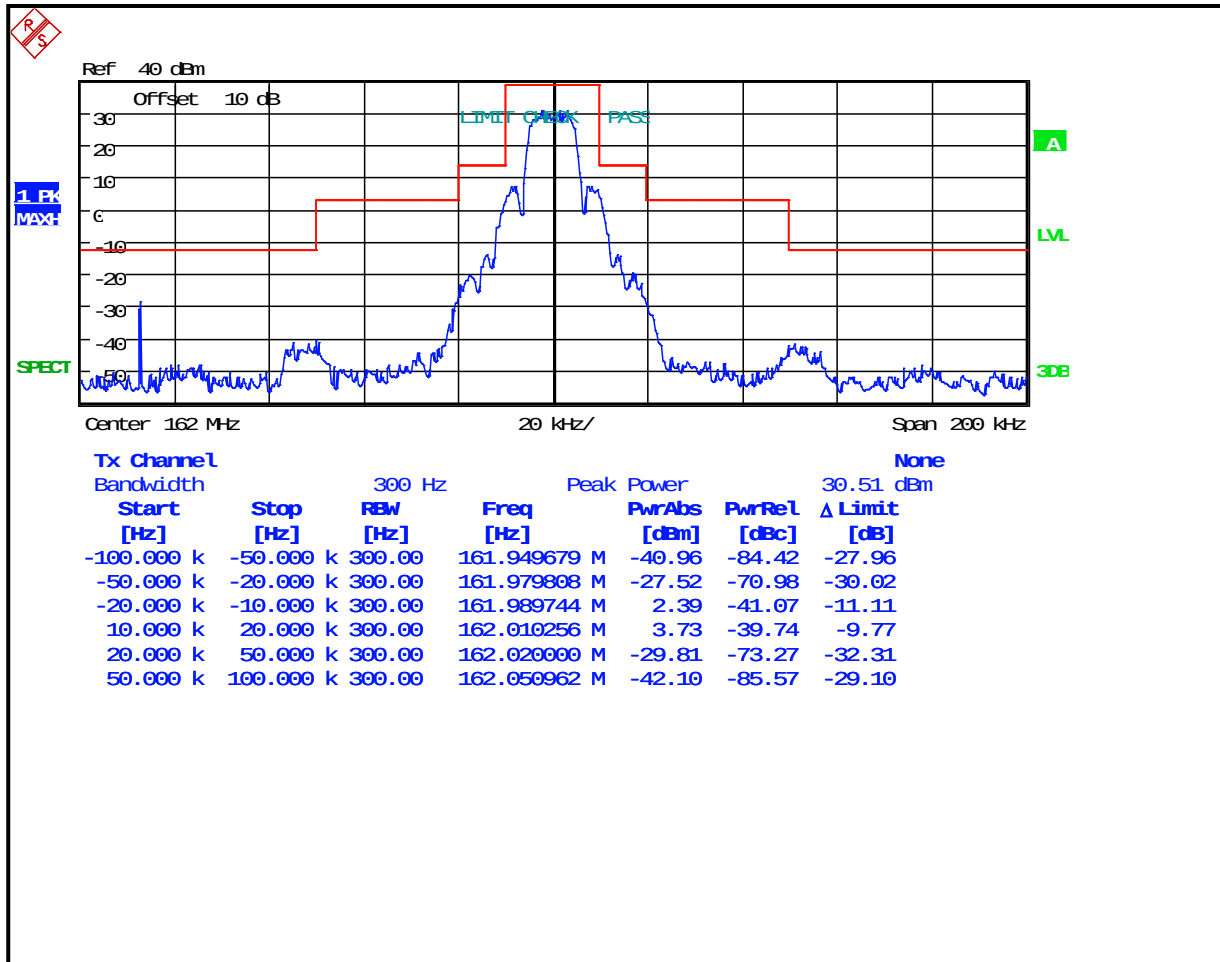
Plot 7-23: Occupied Bandwidth – 162 MHz; 2-Level FSK 9600; WB EDACS; (Mask B)
