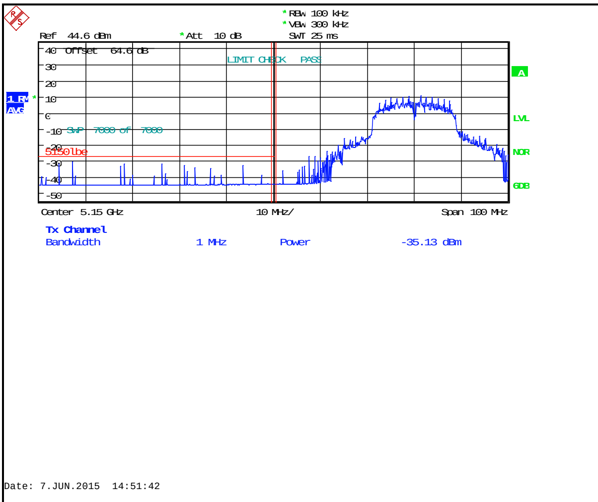
Plot 6-2: Lower Band Edge: Measurement Channel 36 (5180 MHz, 802.11a, Average)
