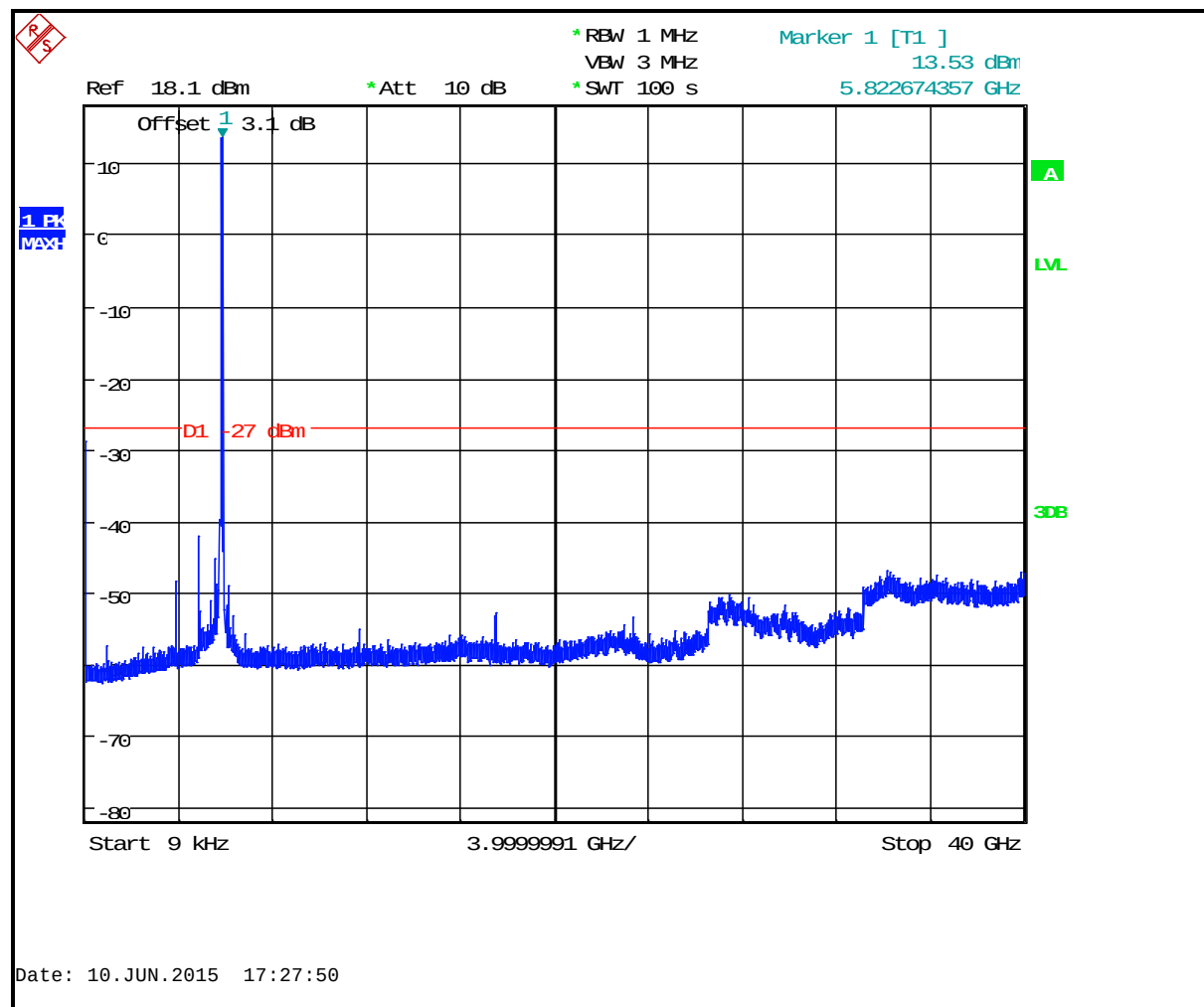
Plot 7-9: Undesirable Emissions Channel 165 (5825 MHz)
