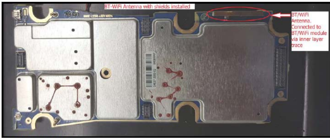
Top PWB with Shields
