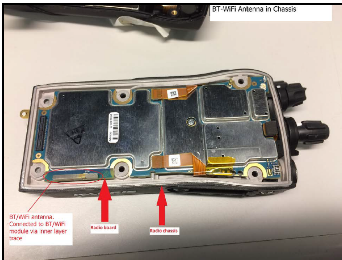
PWB in Chassis 2
