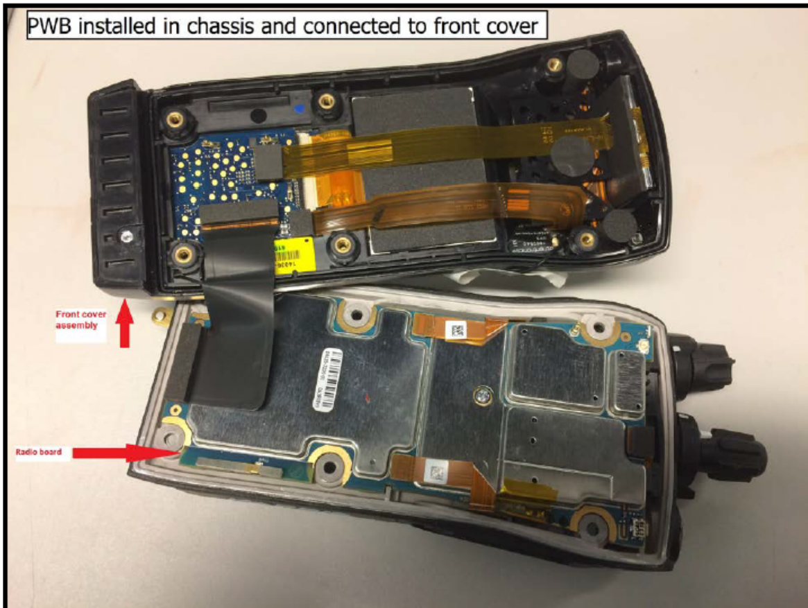
PWB in Chassis
