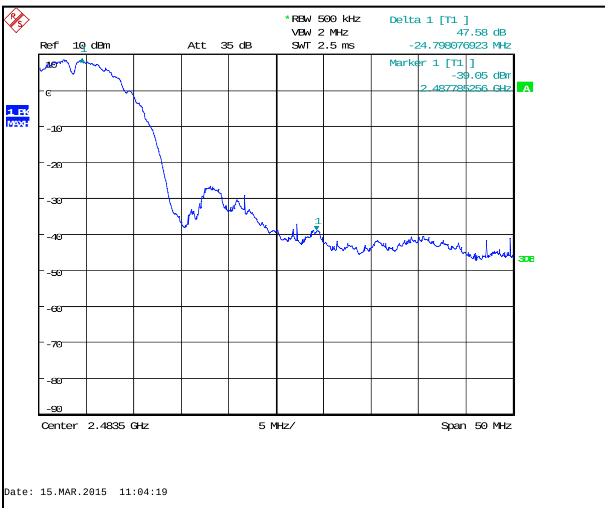
Plot 4-2: In Band Emissions - Channel 11 (2462 MHz); 802.11b (2 Mbps)
