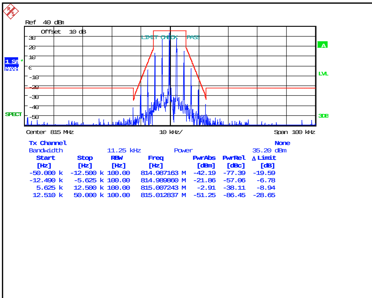
Plot 8-1: Occupied Bandwidth – 815 MHz; Narrowband Analog; Mask D
