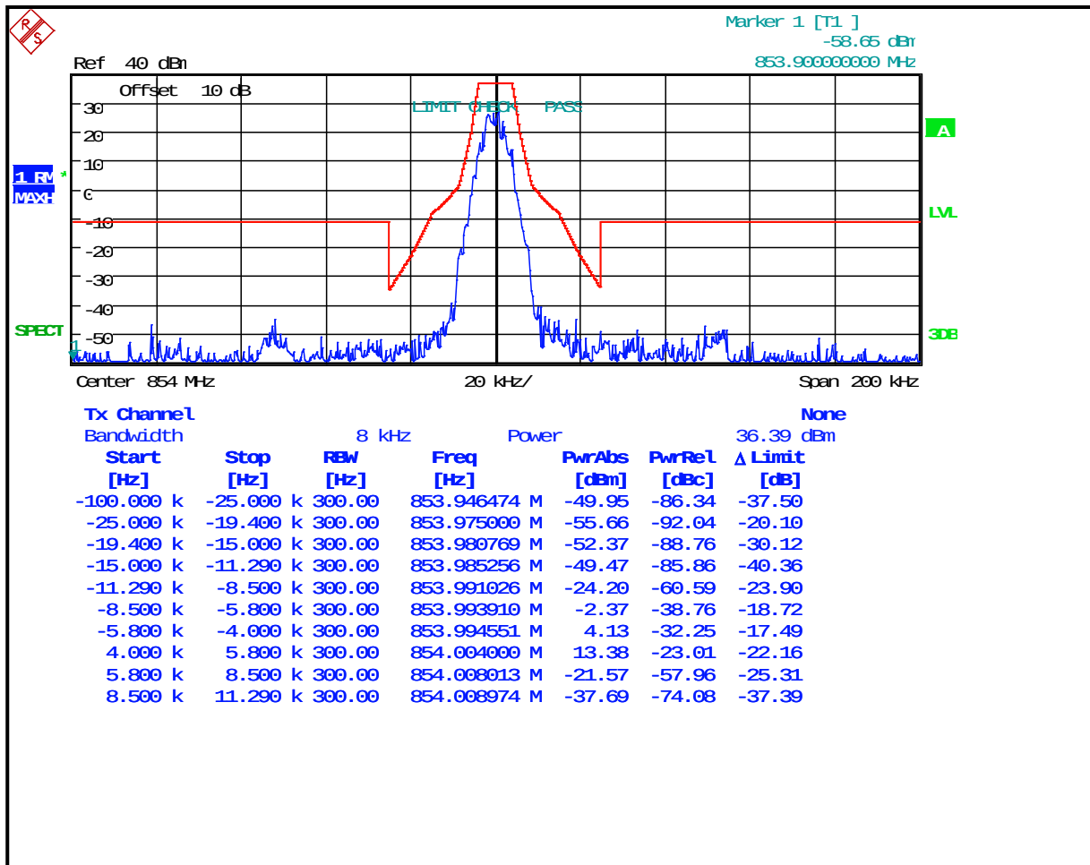
Plot 8-17: Occupied Bandwidth – 854 MHz; CPM TDMA; Mask H
