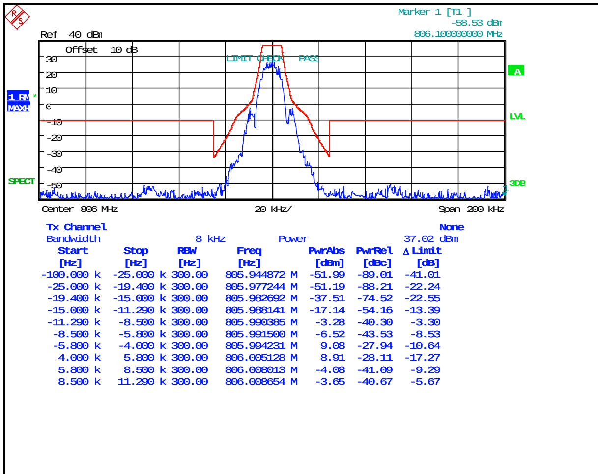
Plot 8-28: Occupied Bandwidth – 806 MHz; 4-level FSK Data/Voice; NPSPAC OpenSky; Mask H
