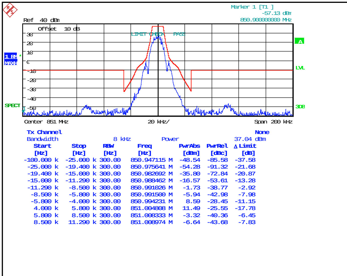
Plot 8-29: Occupied Bandwidth – 851 MHz; 4-level FSK Data/Voice; NPSPAC OpenSky; Mask H
