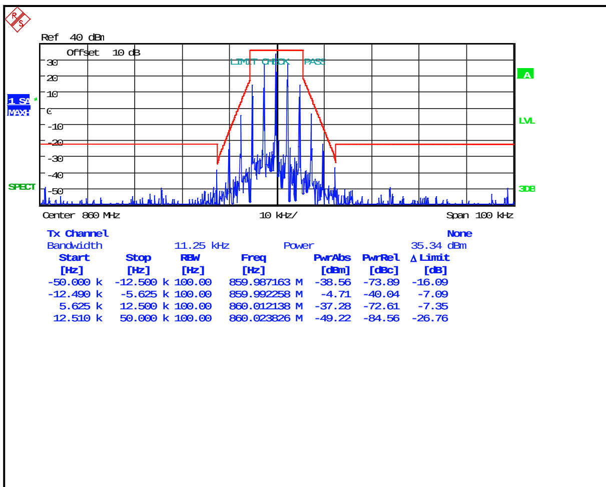
Plot 8-3: Occupied Bandwidth – 860 MHz; Narrowband Analog; Mask D
