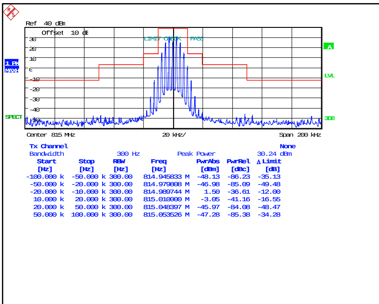
Plot 8-5: Occupied Bandwidth – 815 MHz; Wideband Analog; Mask B
