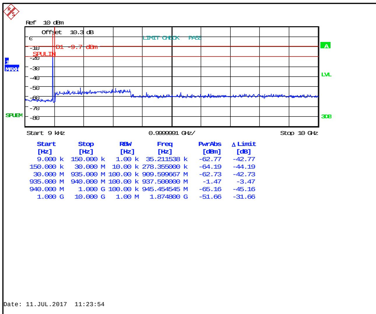
Plot 5-1: Conducted Antenna Spurious Emissions – 937.5 MHz; C4FM
