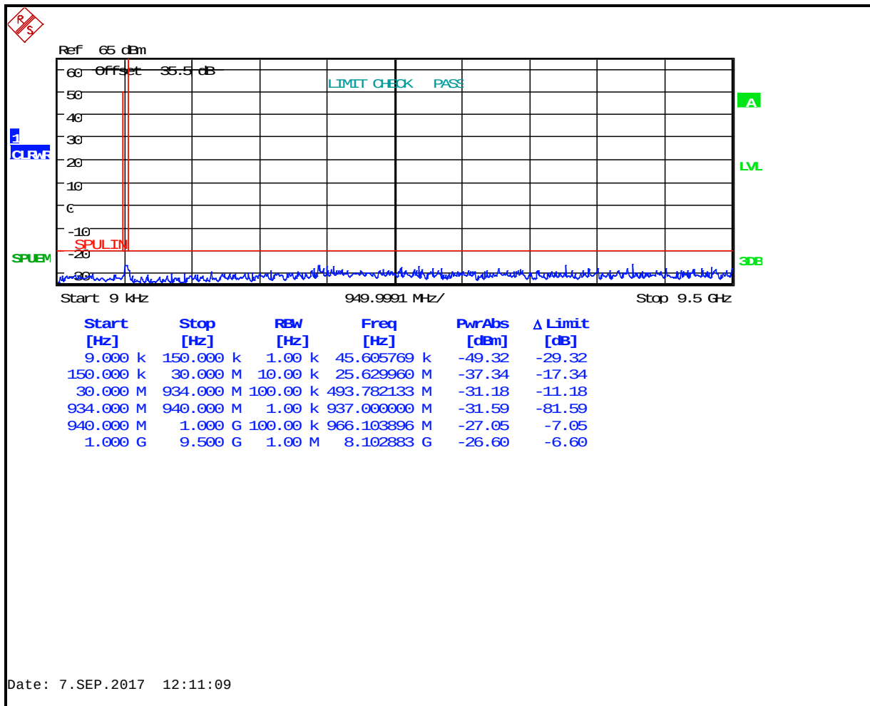
Plot 5-2: Conducted Antenna Spurious Emissions – 935.0125 MHz; WCQPSK
