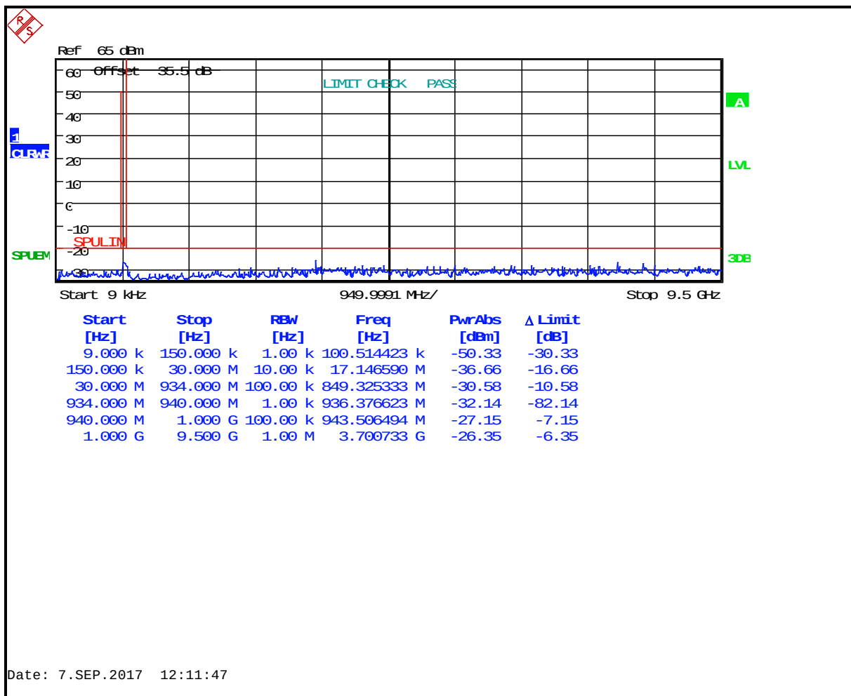
Plot 5-3: Conducted Antenna Spurious Emissions – 935.0125 MHz; HDQPSK
