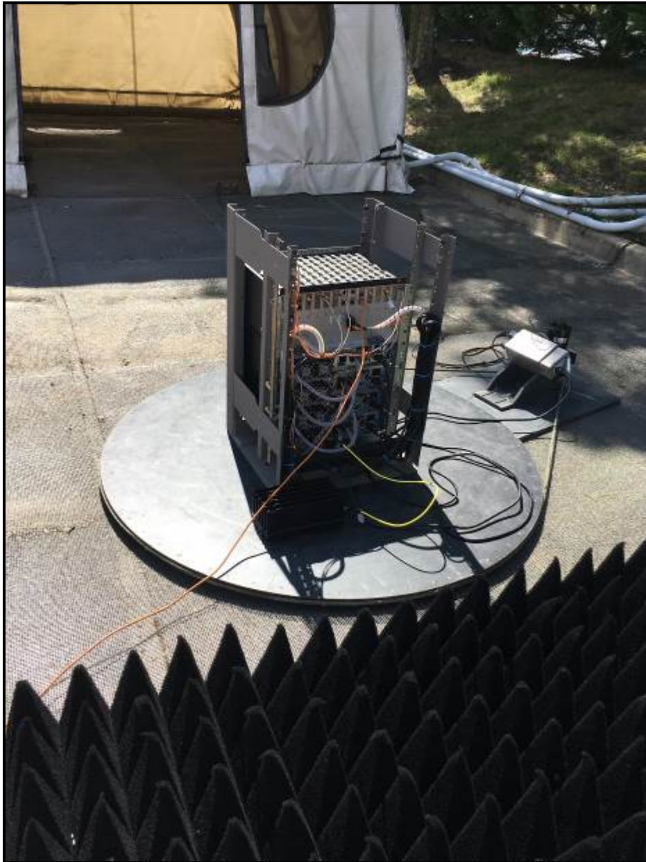
Photograph 2: Radiated Emissions (Spurious/Harmonics) – Back View (Above 1 GHz)
