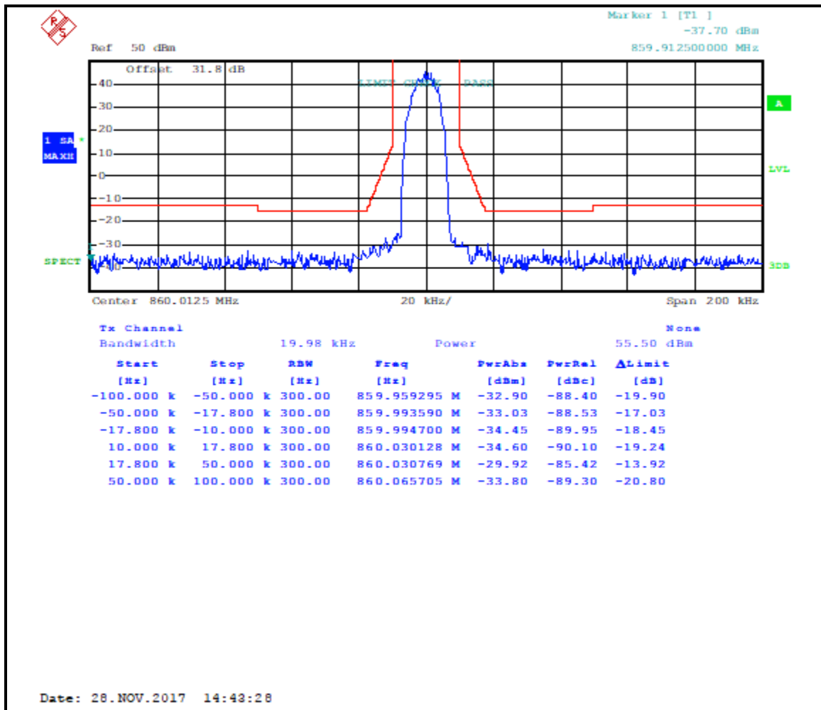
Plot 7-6: Occupied Bandwidth – 860.0125 MHz; WCQPSK; Mask G
