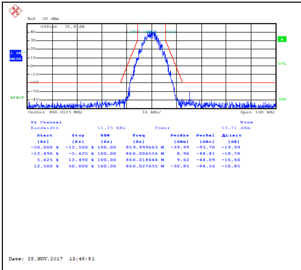
Plot 7-14: Occupied Bandwidth – 860.0125 MHz; C4FM; Mask D
