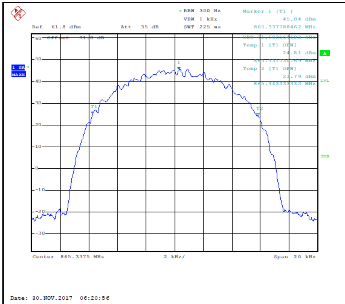
Plot 7-45: Occupied Bandwidth – 865.3375 MHz; HDQPSK; 20 dB BW
