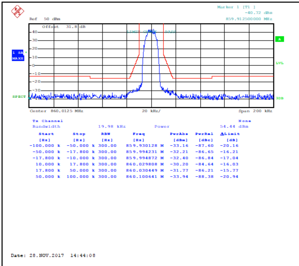
Plot 7-10: Occupied Bandwidth – 860.0125 MHz; HDQPSK; Mask G
