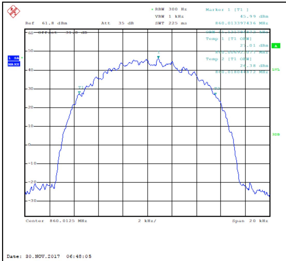
Plot 7-41: Occupied Bandwidth – 860. 0125 MHz; WCQPSK; 20 dB BW
