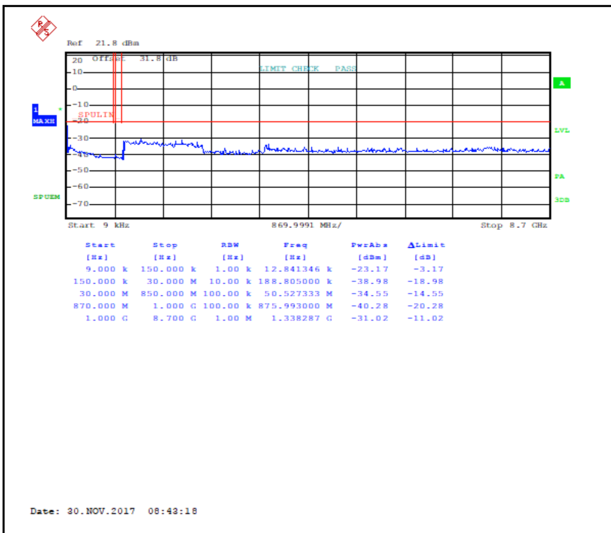
Plot 5-1: Conducted Antenna Spurious Emissions – 851.0125 MHz; C4FM
