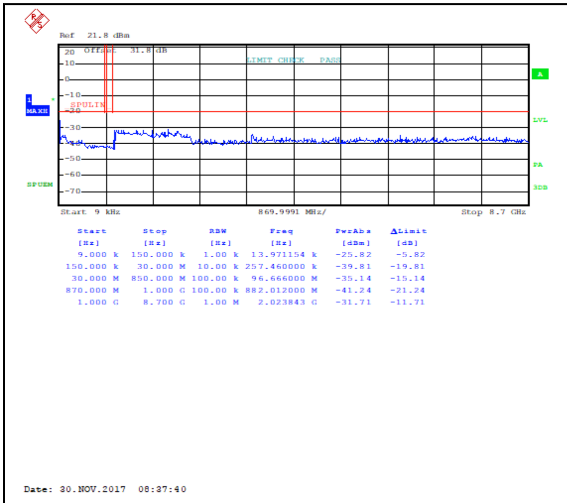
Plot 5-5: Conducted Antenna Spurious Emissions – 860.0125 MHz; WCQPSK
