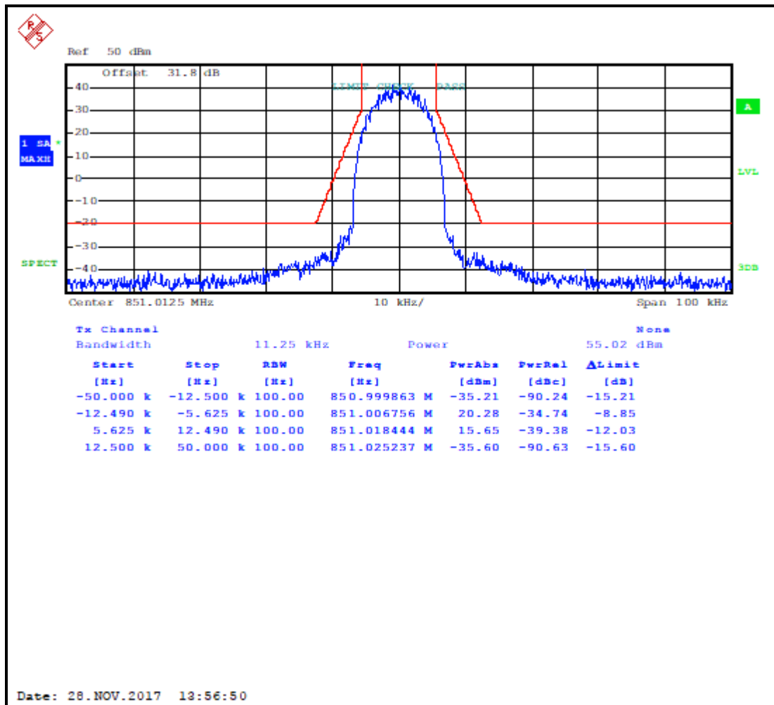
Plot 7-17: Occupied Bandwidth – 851.0125 MHz; WCQPSK; Mask D
