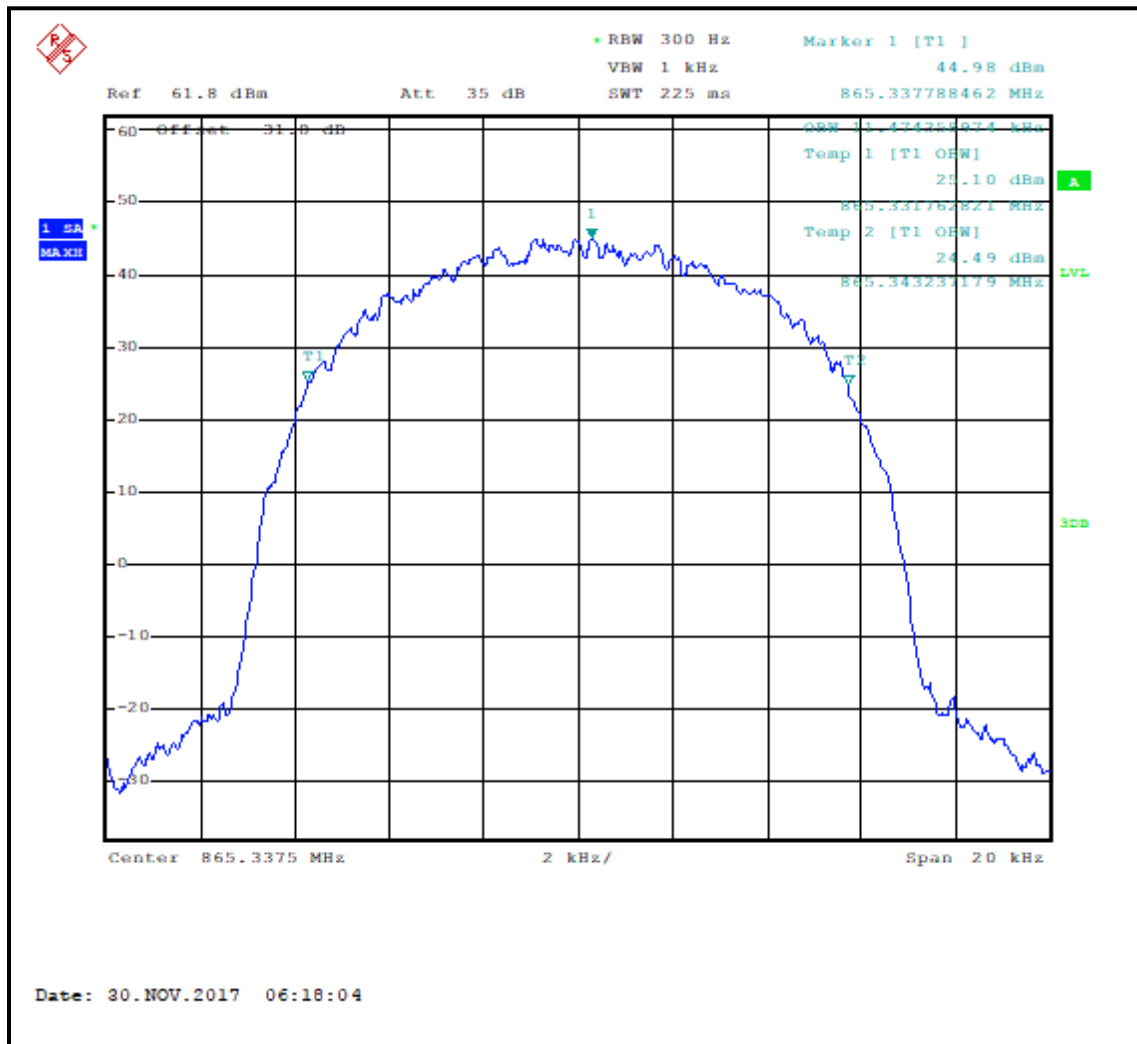
Plot 7-44: Occupied Bandwidth – 865.3375 MHz; WCQPSK; 20 dB BW
