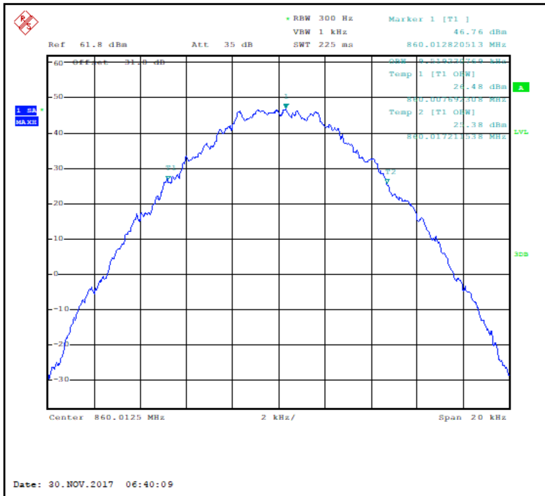
Plot 7-40: Occupied Bandwidth – 860.0125 MHz; C4FM; 20 dB BW
