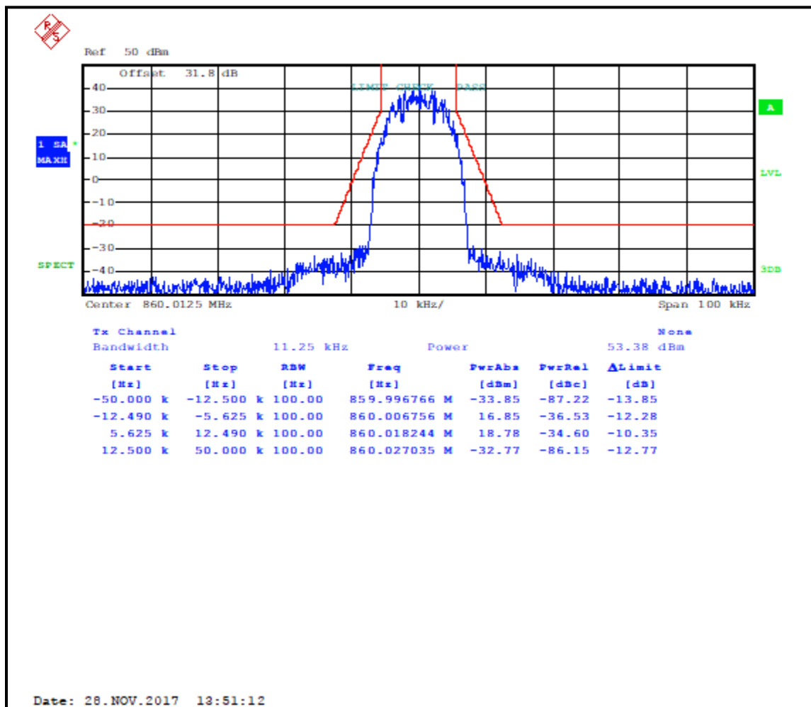
Plot 7-22: Occupied Bandwidth – 860.0125 MHz; HDQPSK; Mask D
