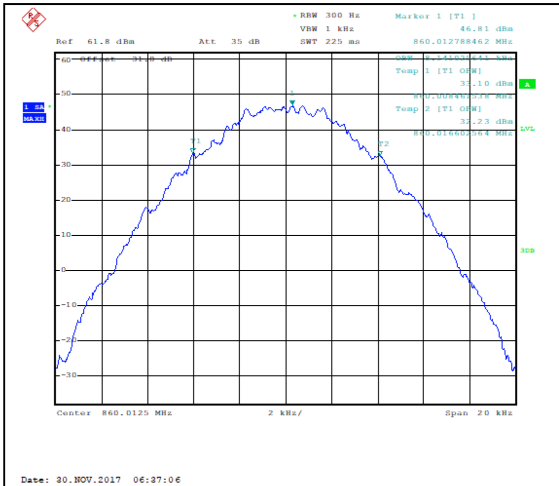
Plot 7-28: Occupied Bandwidth – 860.0125 MHz; C4FM; 99% BW
