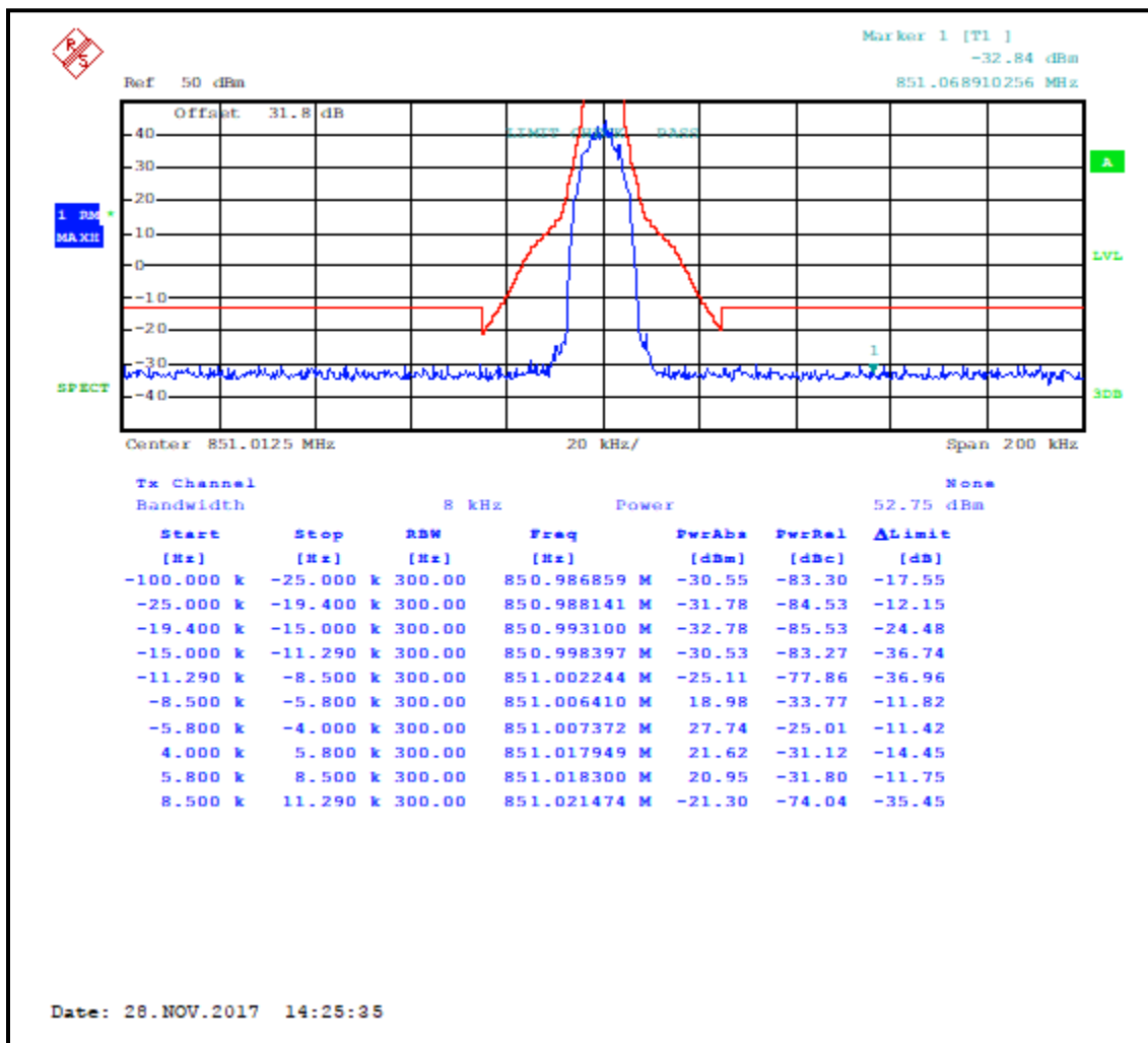
Plot 7-9: Occupied Bandwidth – 851.0125 MHz; HDQPSK; Mask H
