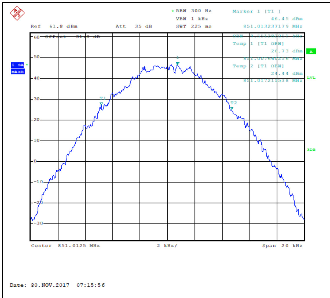
Plot 7-37: Occupied Bandwidth – 851.0125 MHz; C4FM; 20 dB BW
