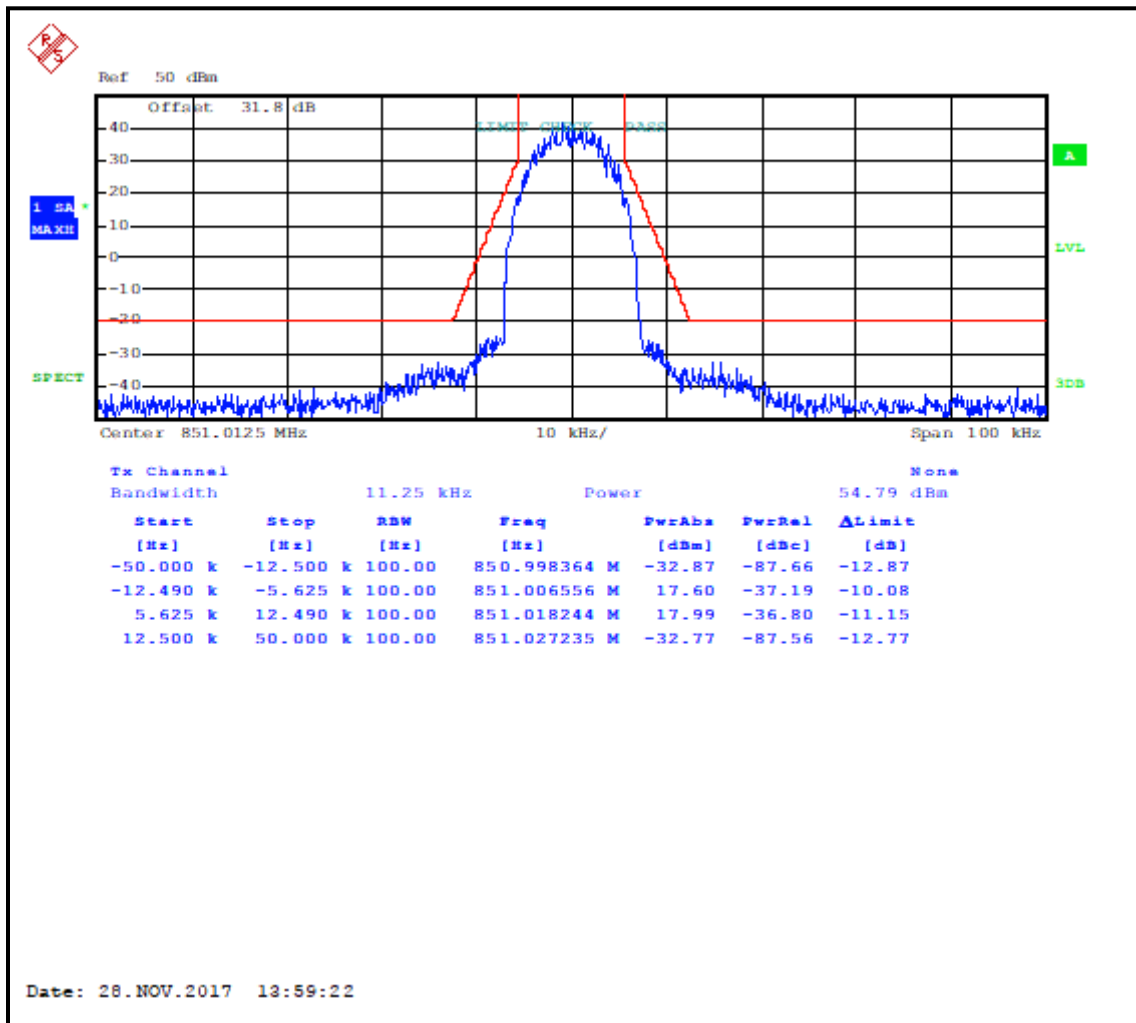
Plot 7-21: Occupied Bandwidth – 851.0125 MHz; HDQPSK; Mask D
