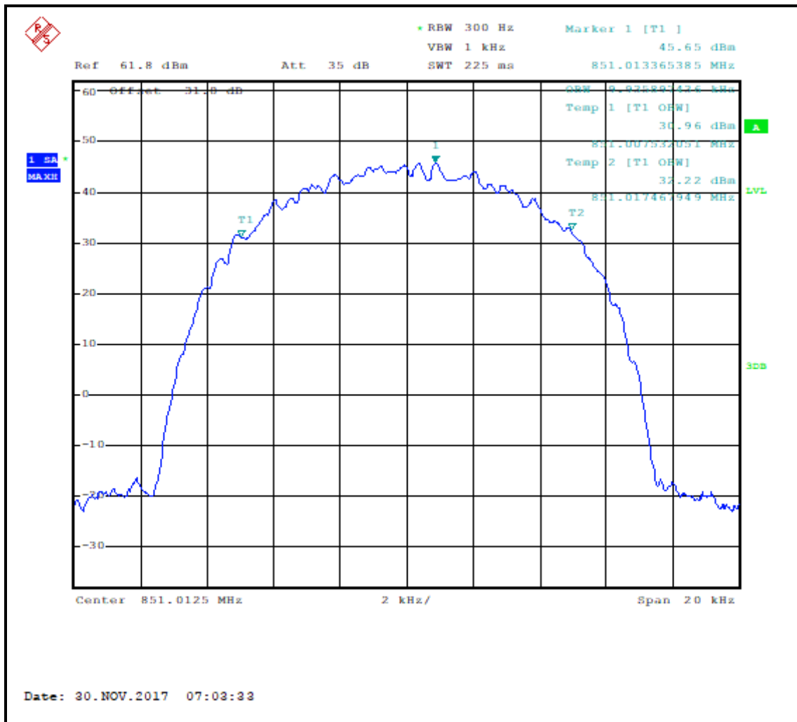
Plot 7-27: Occupied Bandwidth – 851.0125 MHz; HDQPSK; 99% BW
