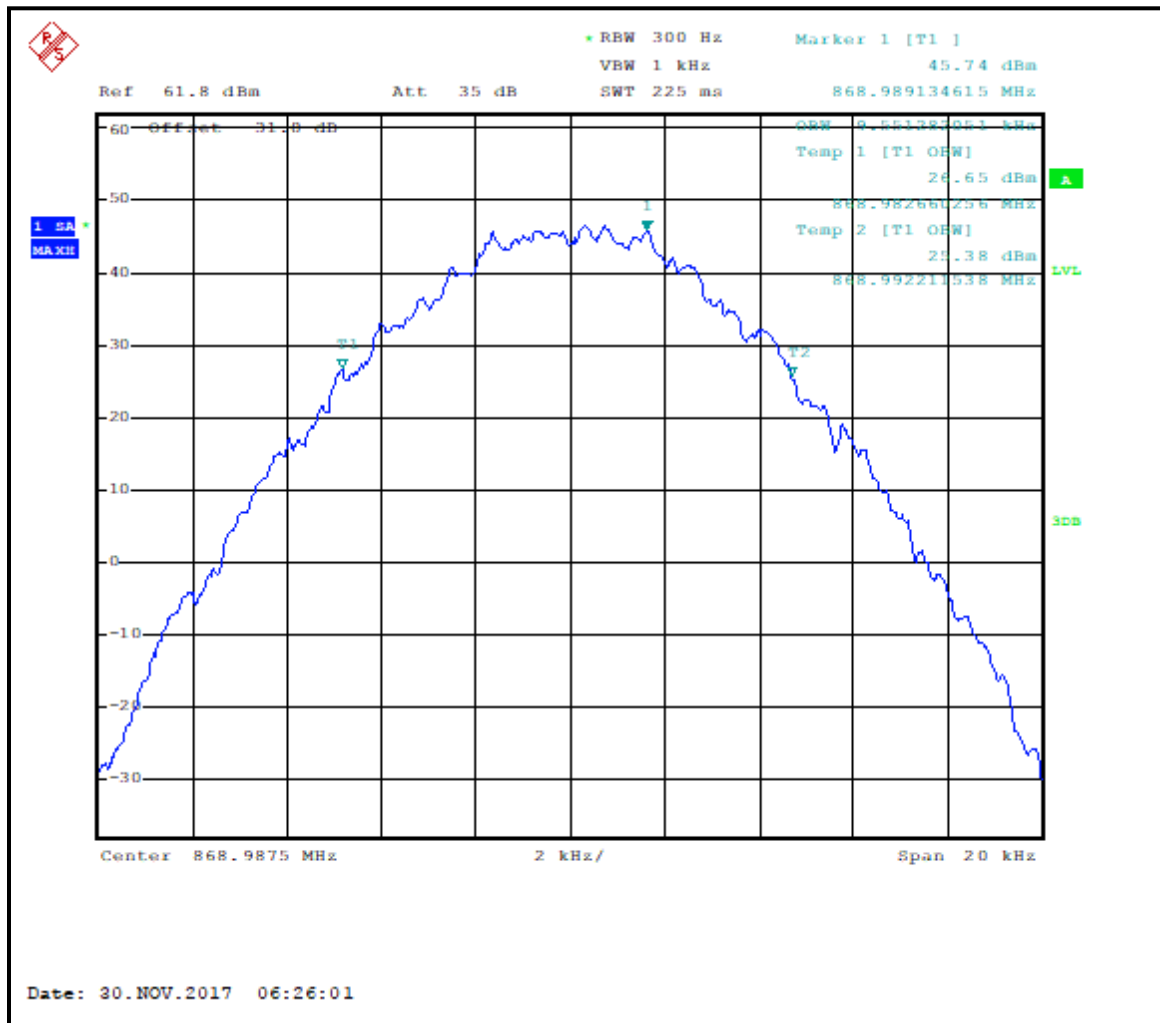
Plot 7-46: Occupied Bandwidth – 868.9875 MHz; C4FM; 20 dB BW
