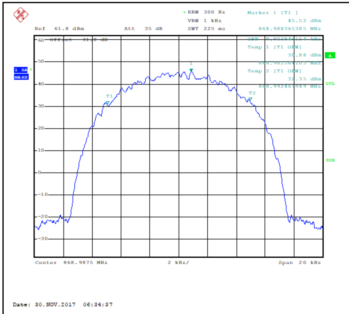
Plot 7-36: Occupied Bandwidth – 868.9875 MHz; HDQPSK; 99% BW
