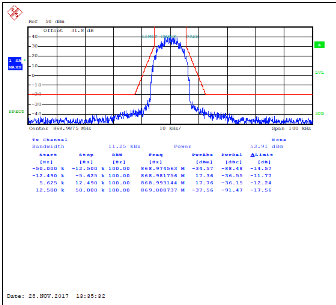
Plot 7-20: Occupied Bandwidth – 868.9875 MHz; WCQPSK; Mask D
