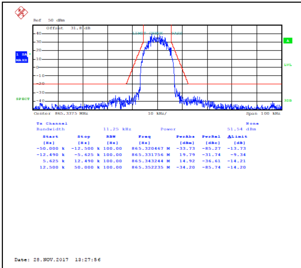
Plot 7-19: Occupied Bandwidth – 865.3375 MHz; WCQPSK; Mask D
