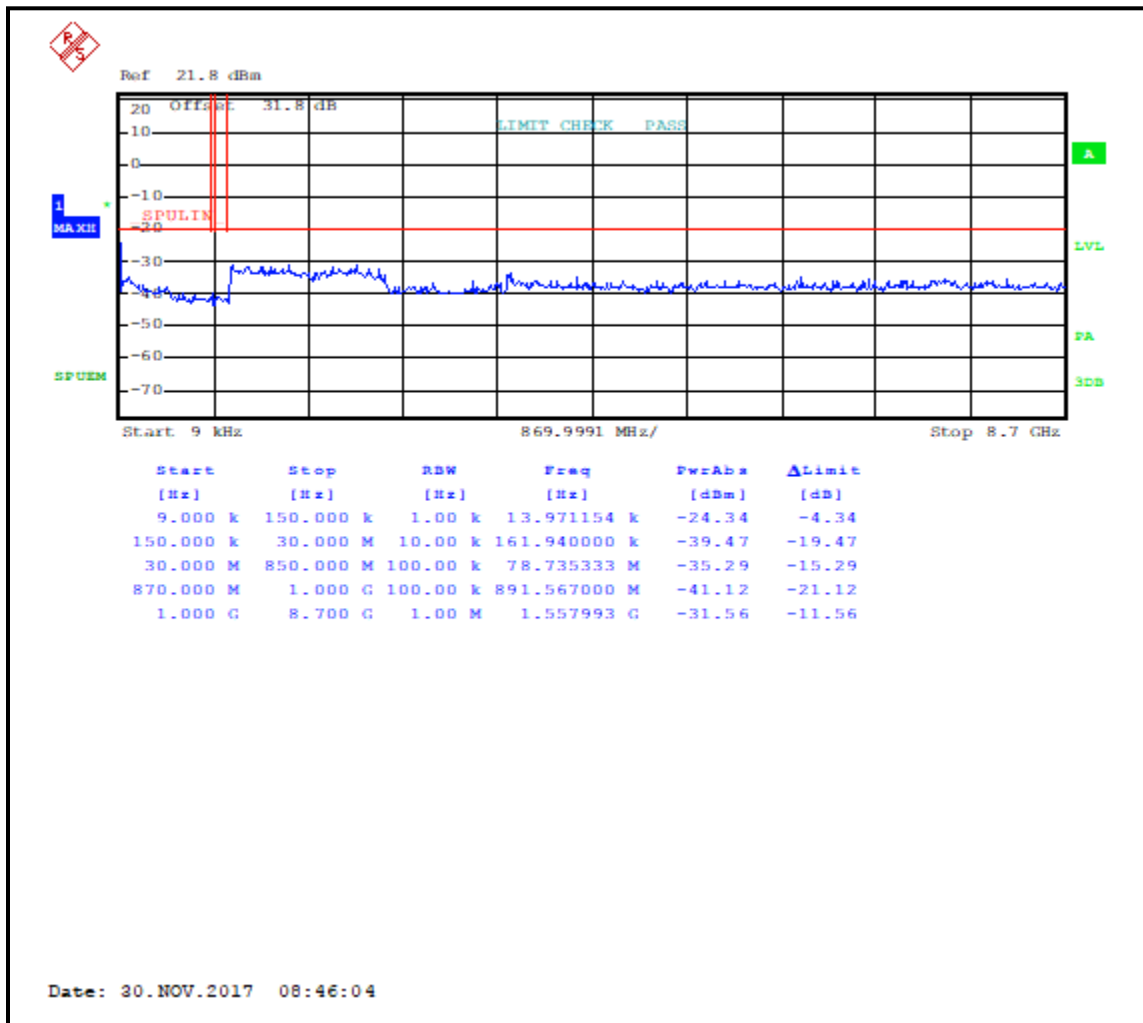
Plot 5-10: Conducted Antenna Spurious Emissions – 868.9875 MHz; C4FM
