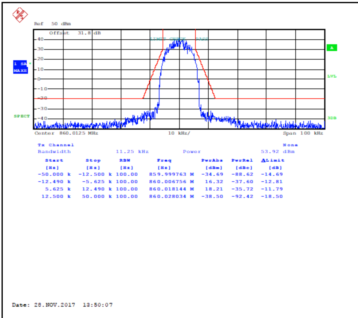
Plot 7-18: Occupied Bandwidth – 860.0125 MHz; WCQPSK; Mask D
