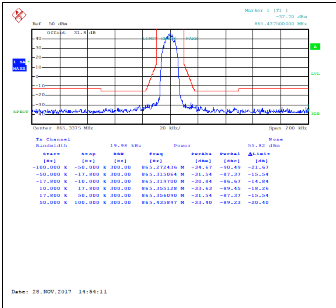
Plot 7-7: Occupied Bandwidth – 865.3375 MHz; WCQPSK; Mask G
