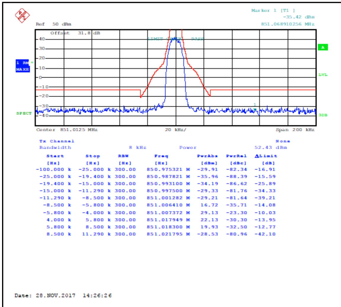
Plot 7-5: Occupied Bandwidth – 851.0125 MHz; WCQPSK; Mask H
