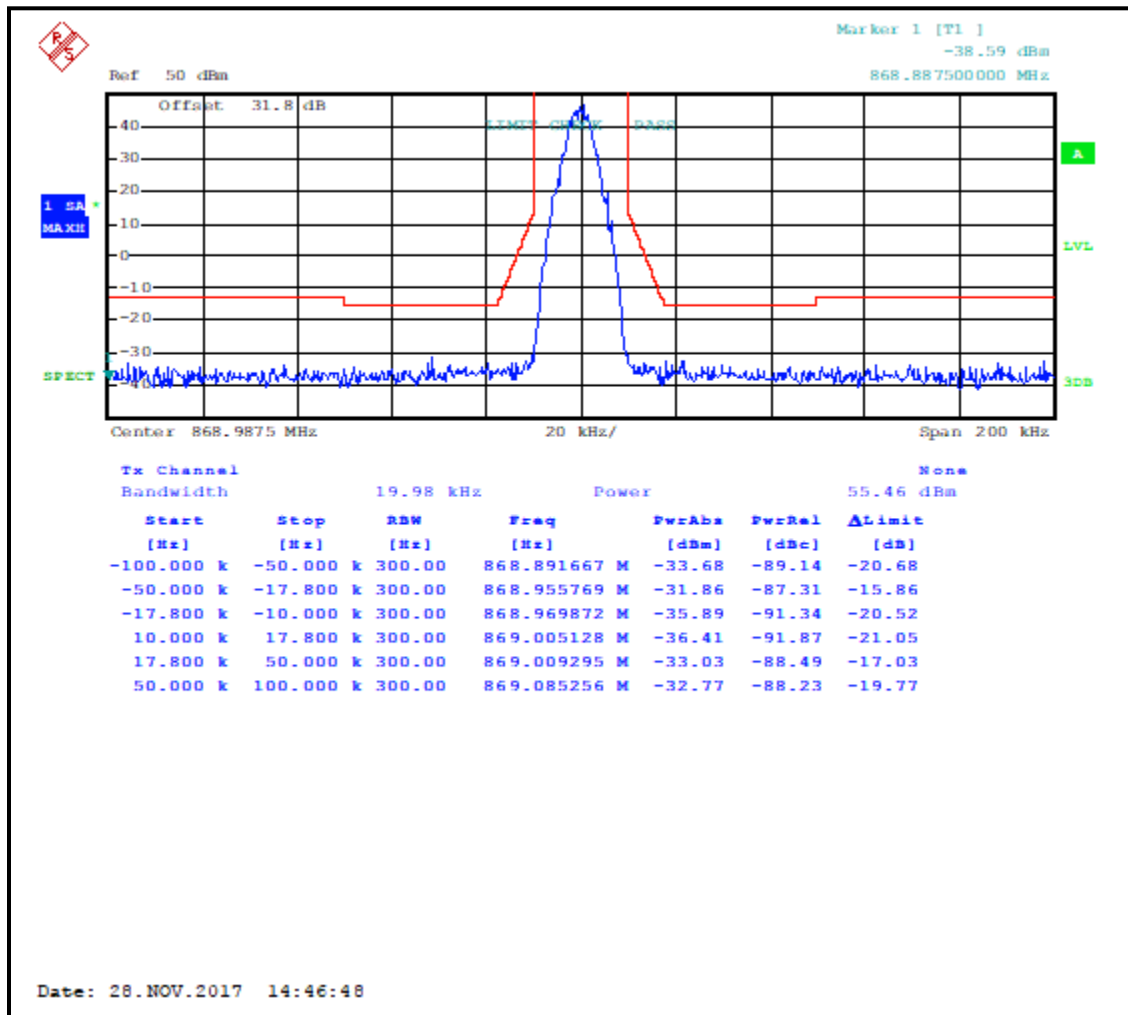
Plot 7-4: Occupied Bandwidth – 868.9875 MHz; C4FM; Mask G
