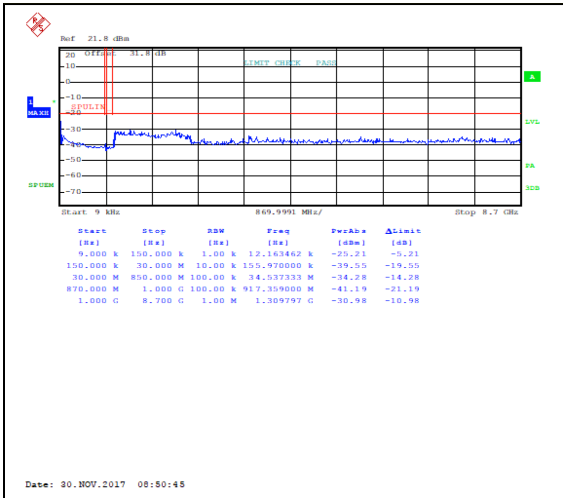
Plot 5-7: Conducted Antenna Spurious Emissions – 865.3375 MHz; C4FM
