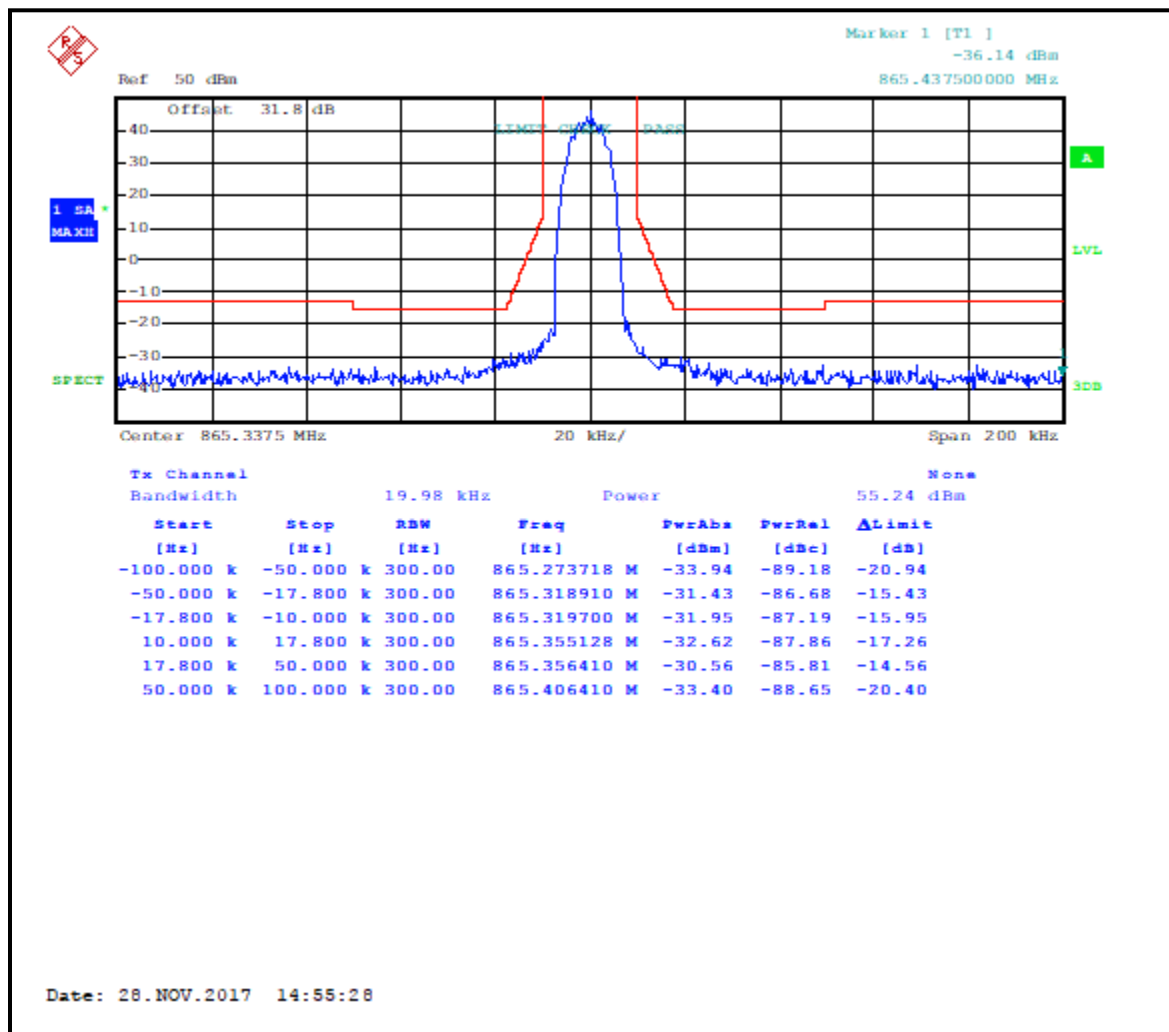
Plot 7-11: Occupied Bandwidth – 865.3375 MHz; HDQPSK; Mask G
