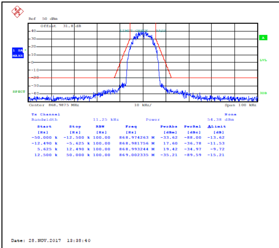
Plot 7-24: Occupied Bandwidth – 868.9875 MHz; HDQPSK; Mask D
