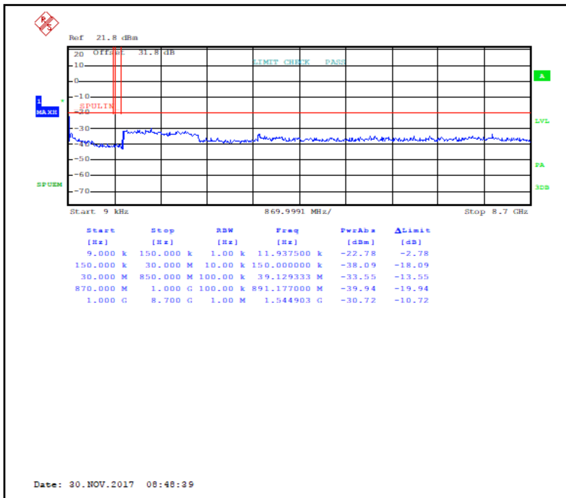
Plot 5-12: Conducted Antenna Spurious Emissions – 868.9875 MHz; HDQPSK
