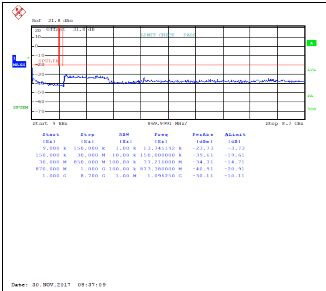
Plot 5-6: Conducted Antenna Spurious Emissions – 860.0125 MHz; HDQPSK
