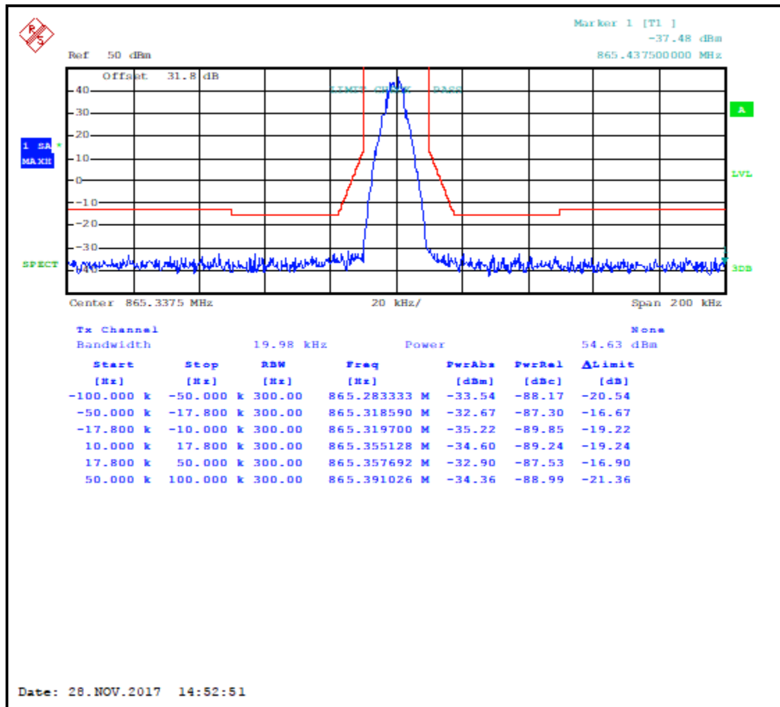
Plot 7-3: Occupied Bandwidth – 865.3375 MHz; C4FM; Mask G
