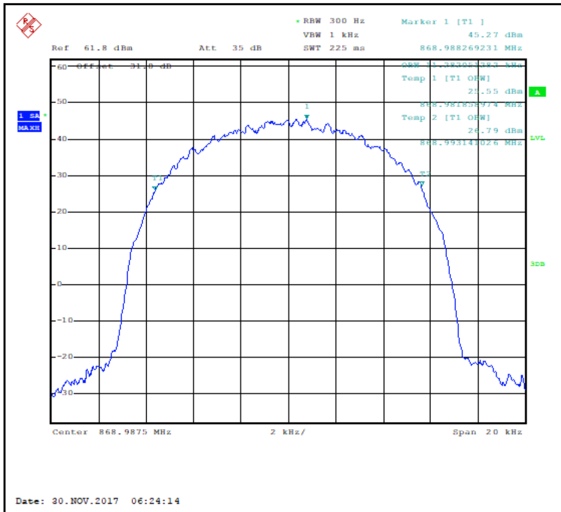
Plot 7-47: Occupied Bandwidth – 868.9875 MHz; WCQPSK; 20 dB BW
