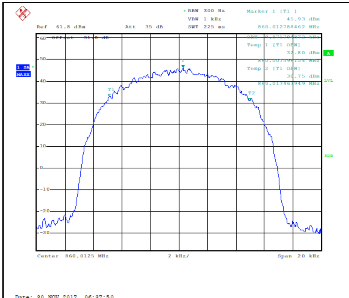
Plot 7-29: Occupied Bandwidth – 860.0125 MHz; WCQPSK; 99% BW
