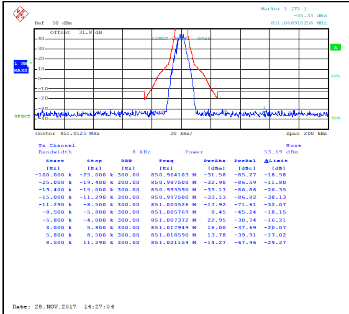
Plot 7-1: Occupied Bandwidth – 851.0125 MHz; C4FM; Mask H
