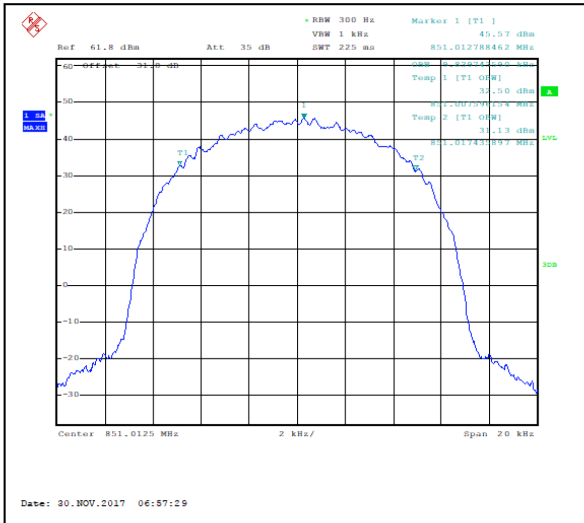
Plot 7-26: Occupied Bandwidth – 851.0125 MHz; WCQPSK; 99% BW
