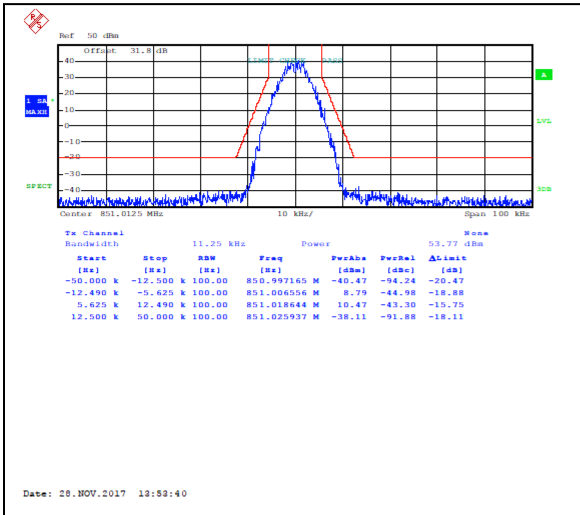
Plot 7-13: Occupied Bandwidth – 851.0125 MHz; C4FM; Mask D
