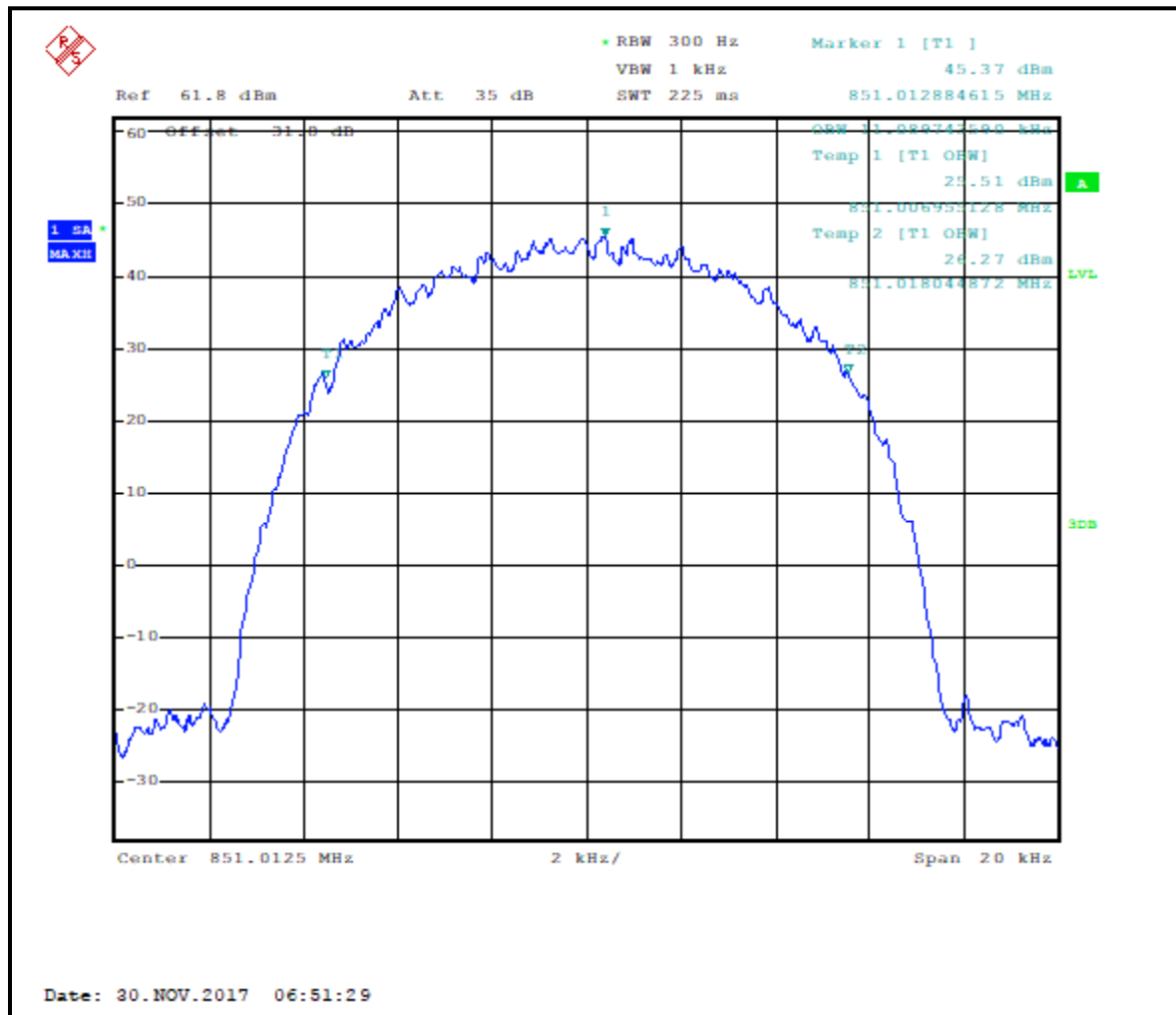
Plot 7-38: Occupied Bandwidth – 851.0125 MHz; WCQPSK; 20 dB BW
