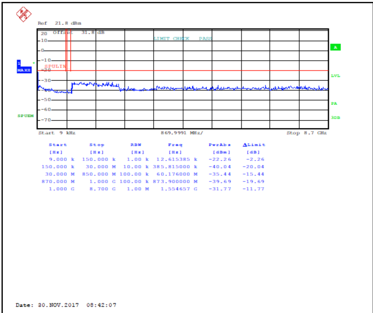
Plot 5-2: Conducted Antenna Spurious Emissions – 851.0125 MHz; WCQPSK
