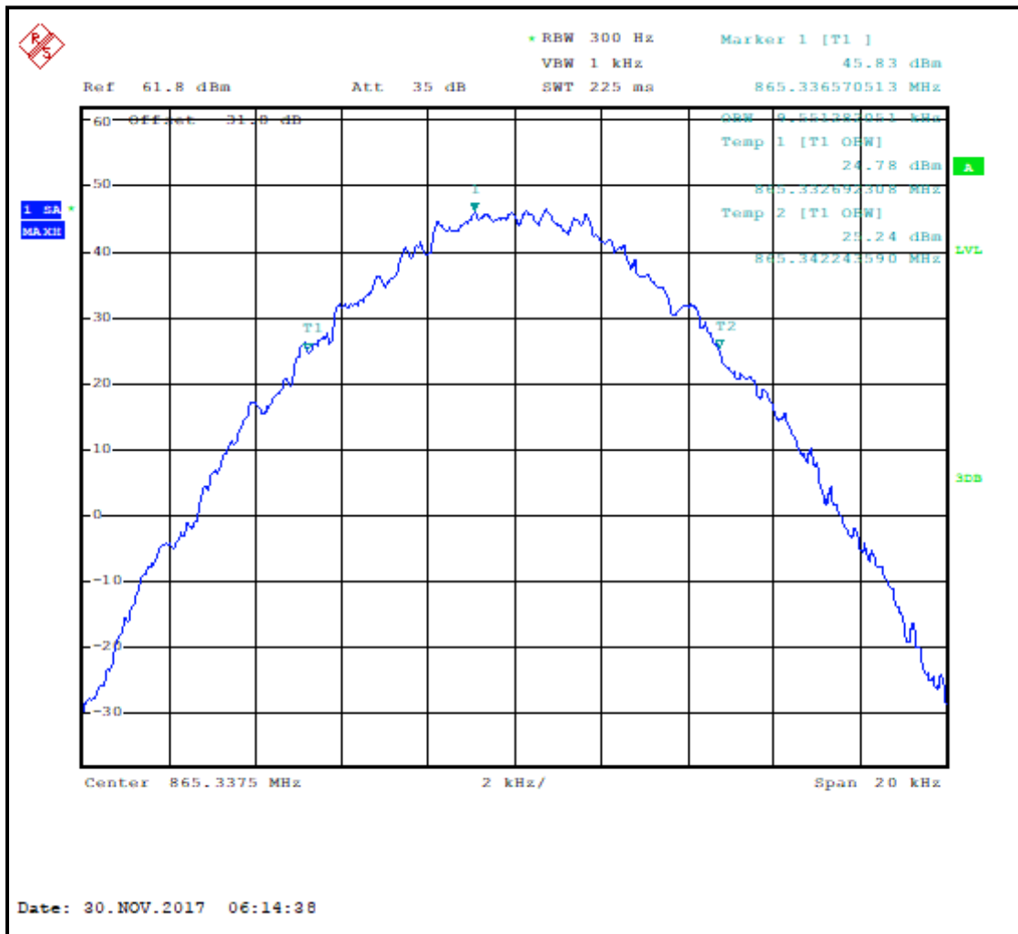
Plot 7-43: Occupied Bandwidth – 865.3375 MHz; C4FM; 20 dB BW
