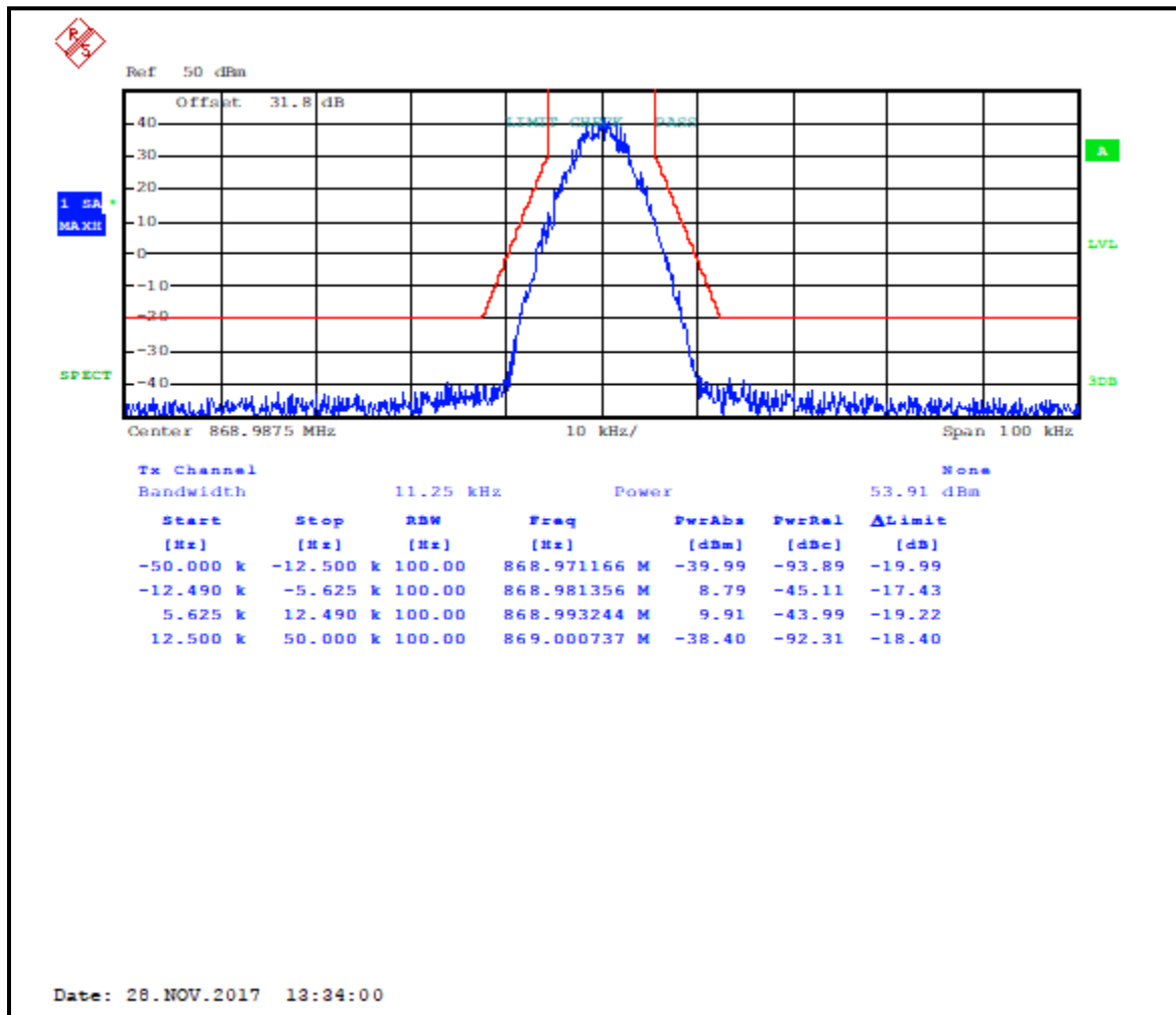
Plot 7-16: Occupied Bandwidth – 868.9875 MHz; C4FM; Mask D
