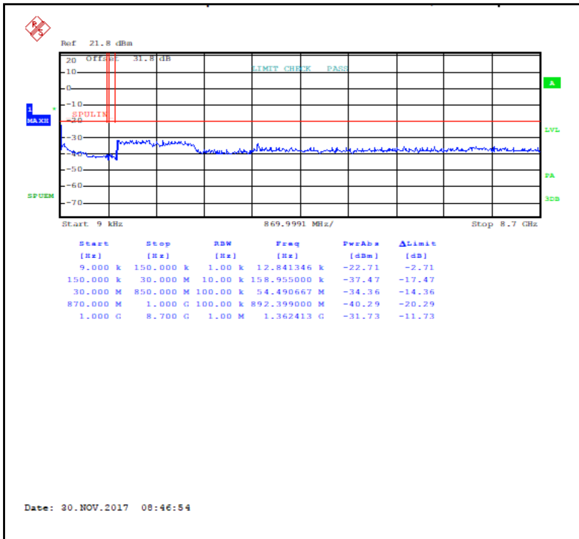
Plot 5-11: Conducted Antenna Spurious Emissions – 868.9875 MHz; WCQPSK
