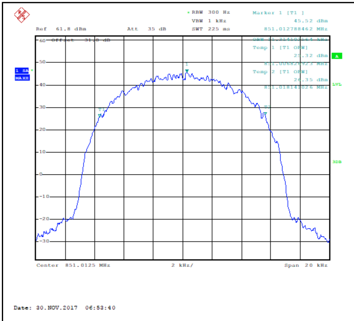
Plot 7-39: Occupied Bandwidth – 851.0125 MHz; HDQPSK; 20 dB BW
