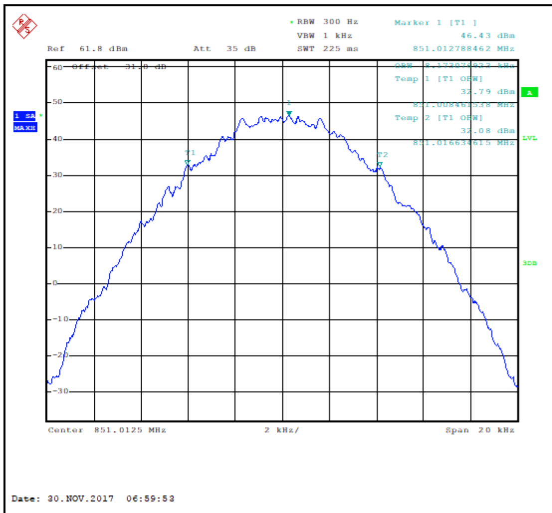
Plot 7-25: Occupied Bandwidth – 851.0125 MHz; C4FM; 99% BW
