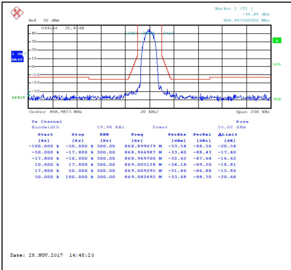
Plot 7-12: Occupied Bandwidth – 868.9875 MHz; HDQPSK; Mask G
