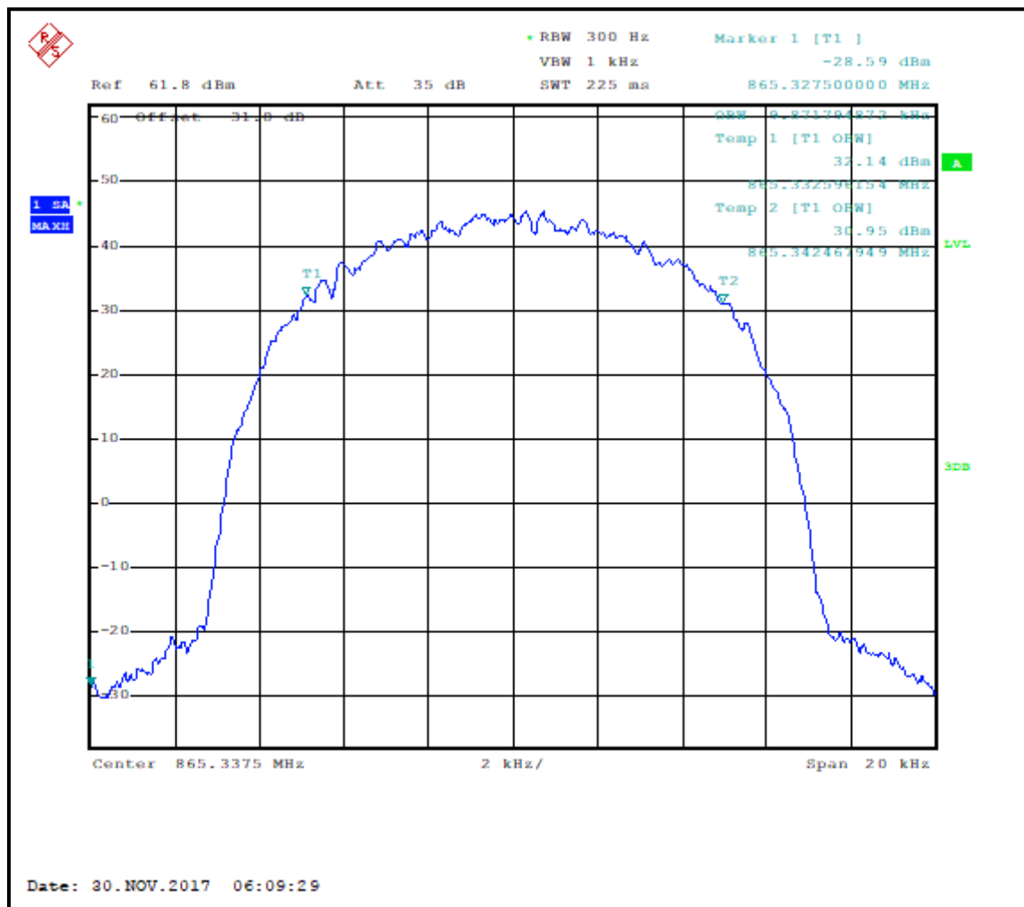
Plot 7-32: Occupied Bandwidth – 865.3375 MHz; WCQPSK; 99% BW
