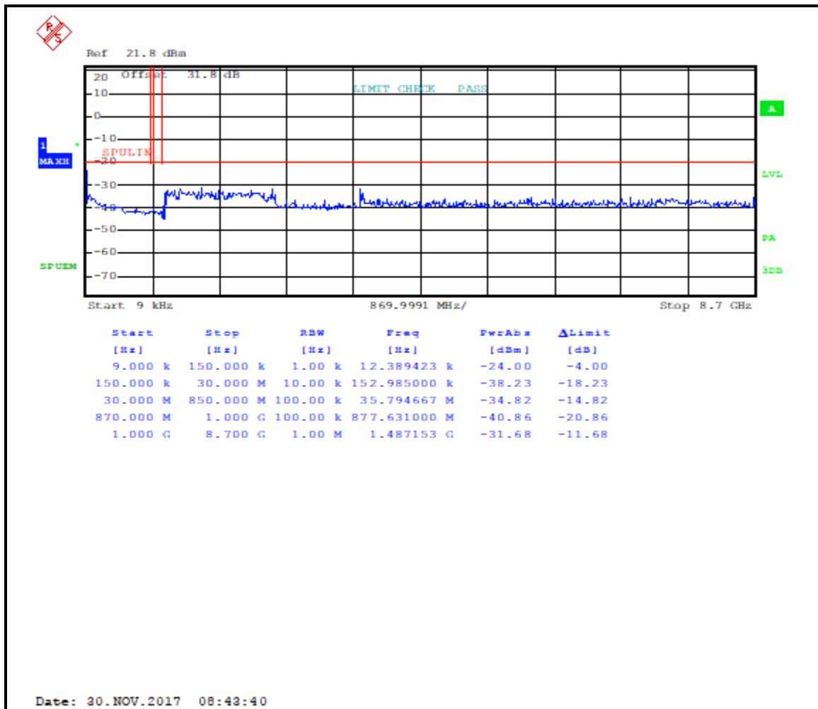
Plot 5-3: Conducted Antenna Spurious Emissions – 851.0125 MHz; HDQPSK
