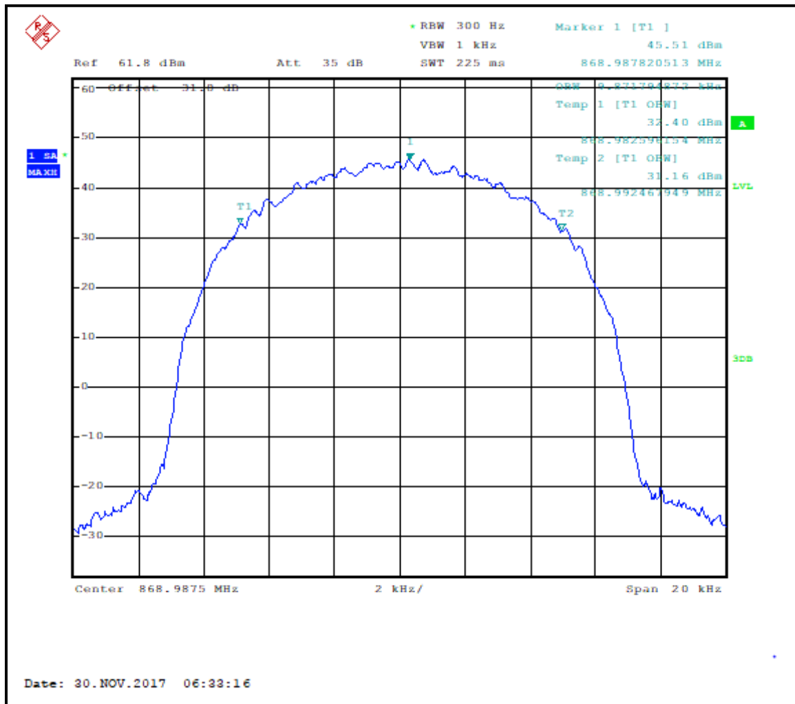
Plot 7-35: Occupied Bandwidth – 868.9875 MHz; WCQPSK; 99% BW
