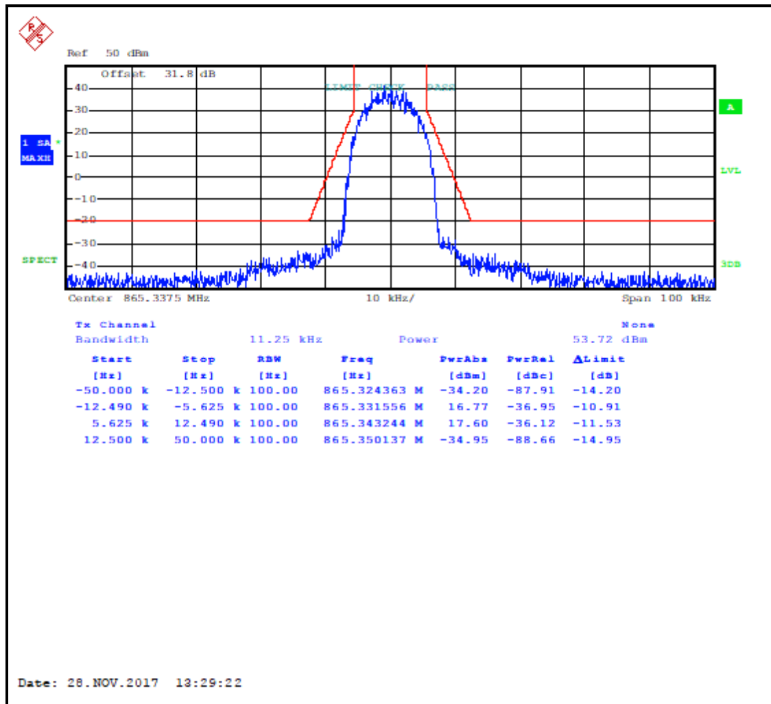
Plot 7-23: Occupied Bandwidth – 865.3375 MHz; HDQPSK; Mask D
