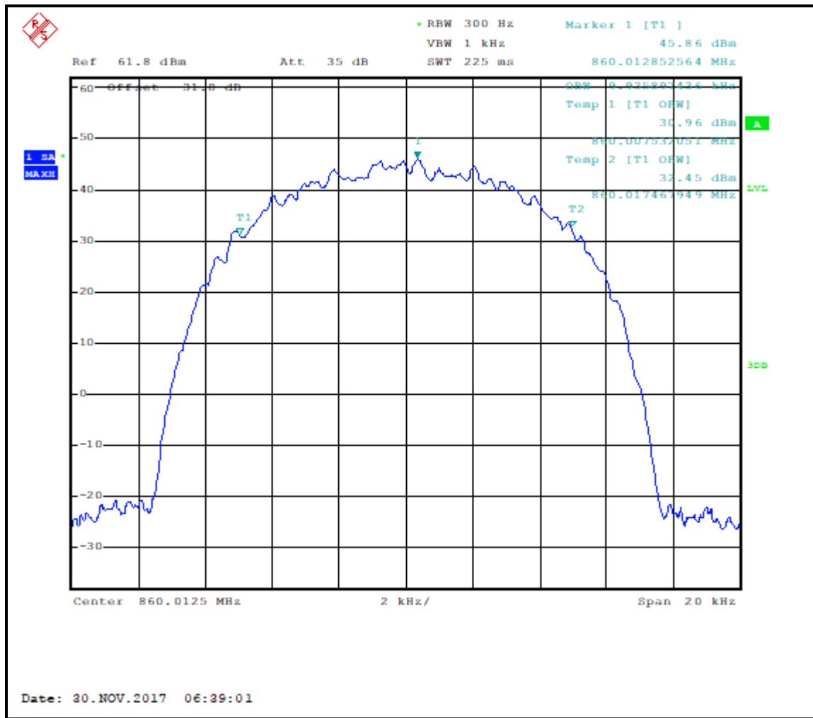
Plot 7-30: Occupied Bandwidth – 860.0125 MHz; HDQPSK; 99% BW
