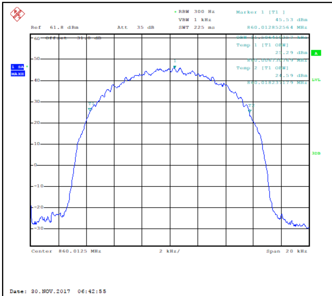
Plot 7-42: Occupied Bandwidth – 860. 0125 MHz; HDQPSK; 20 dB BW
