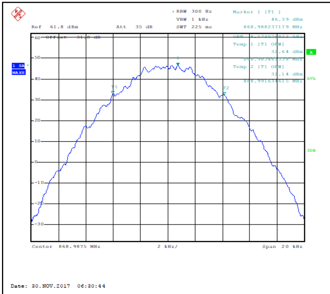
Plot 7-34: Occupied Bandwidth – 868.9875 MHz; C4FM; 99% BW
