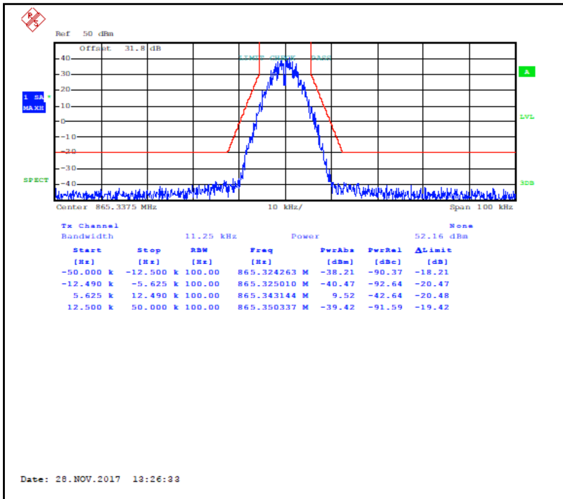
Plot 7-15: Occupied Bandwidth – 865.3375 MHz; C4FM; Mask D
