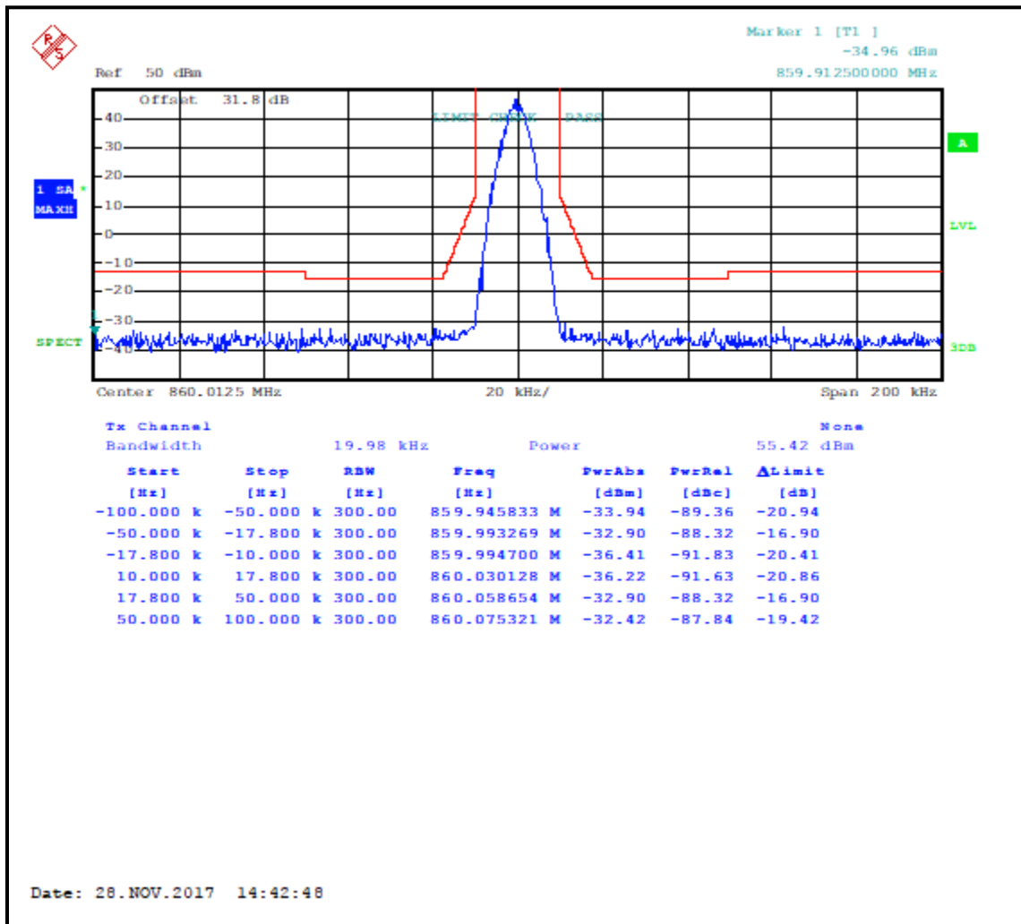
Plot 7-2: Occupied Bandwidth – 860.0125 MHz; C4FM; Mask G
