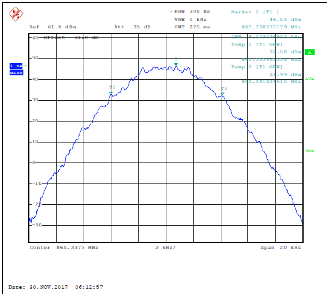
Plot 7-31: Occupied Bandwidth – 865.3375 MHz; C4FM; 99% BW
