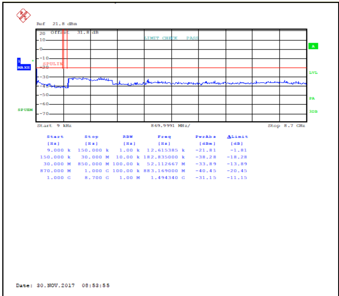
Plot 5-8: Conducted Antenna Spurious Emissions – 865.3375 MHz; WCQPSK
