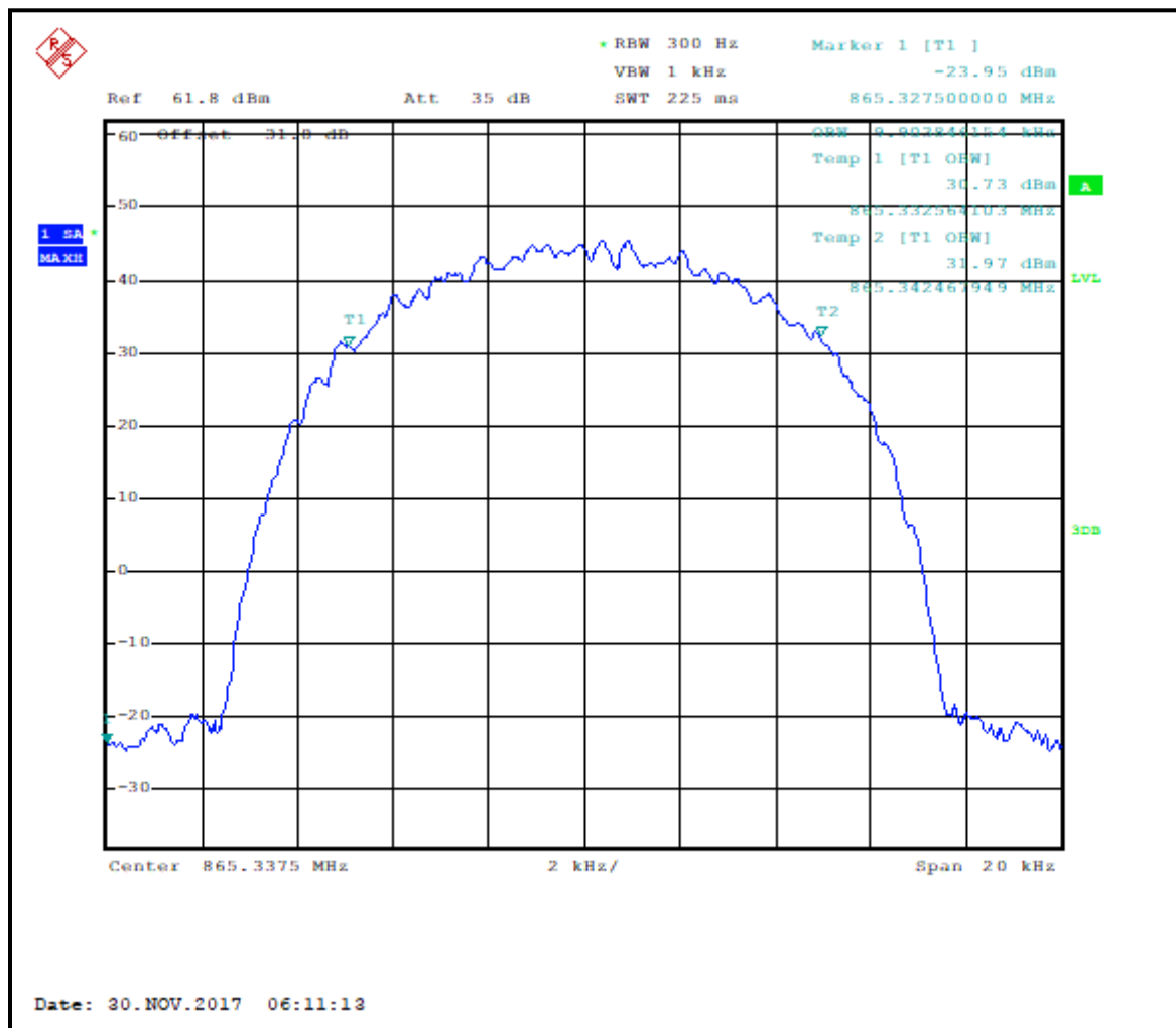
Plot 7-33: Occupied Bandwidth – 865.3375 MHz; HDQPSK; 99% BW
