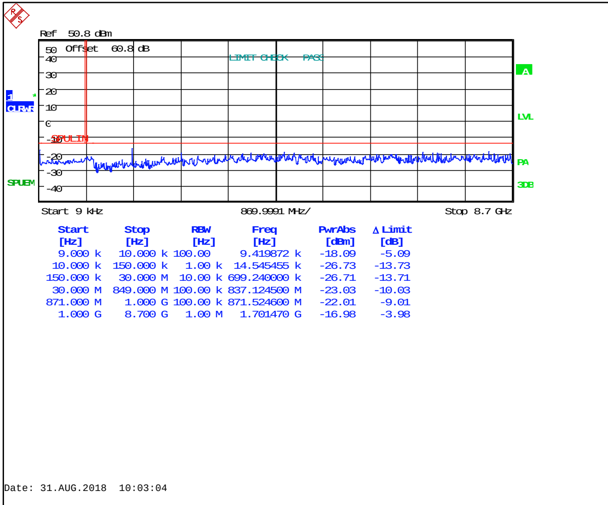
Plot 4-3: Conducted Antenna Spurious Emissions – 851.0125 MHz; HVD NPSPAC
