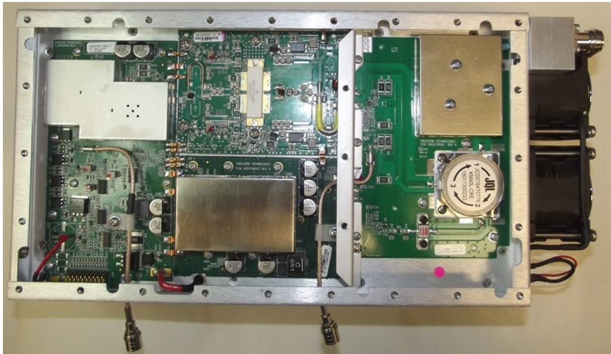
Power Amplifier Top View
