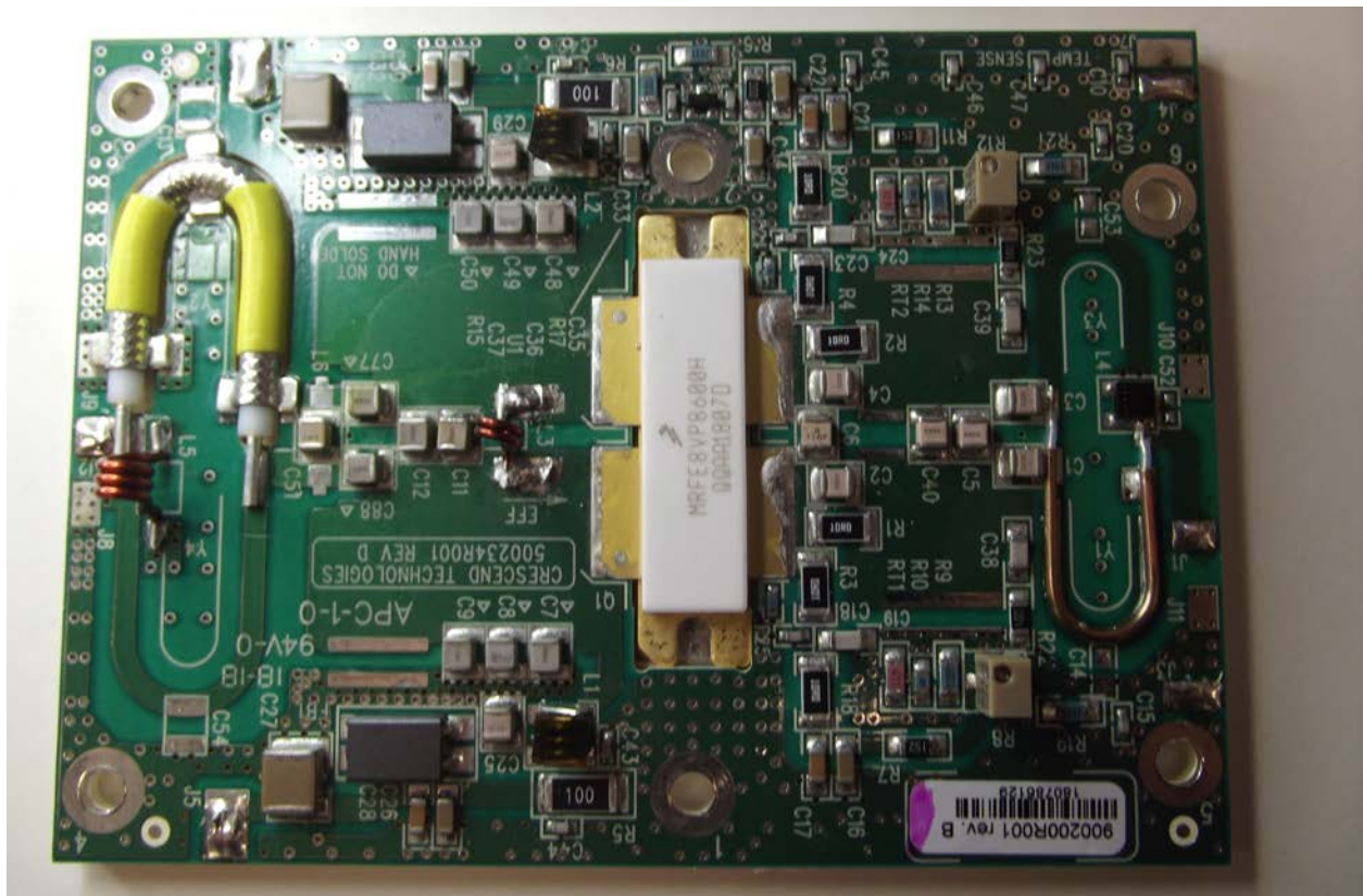
Power Amplifier Final Assembly Top View
