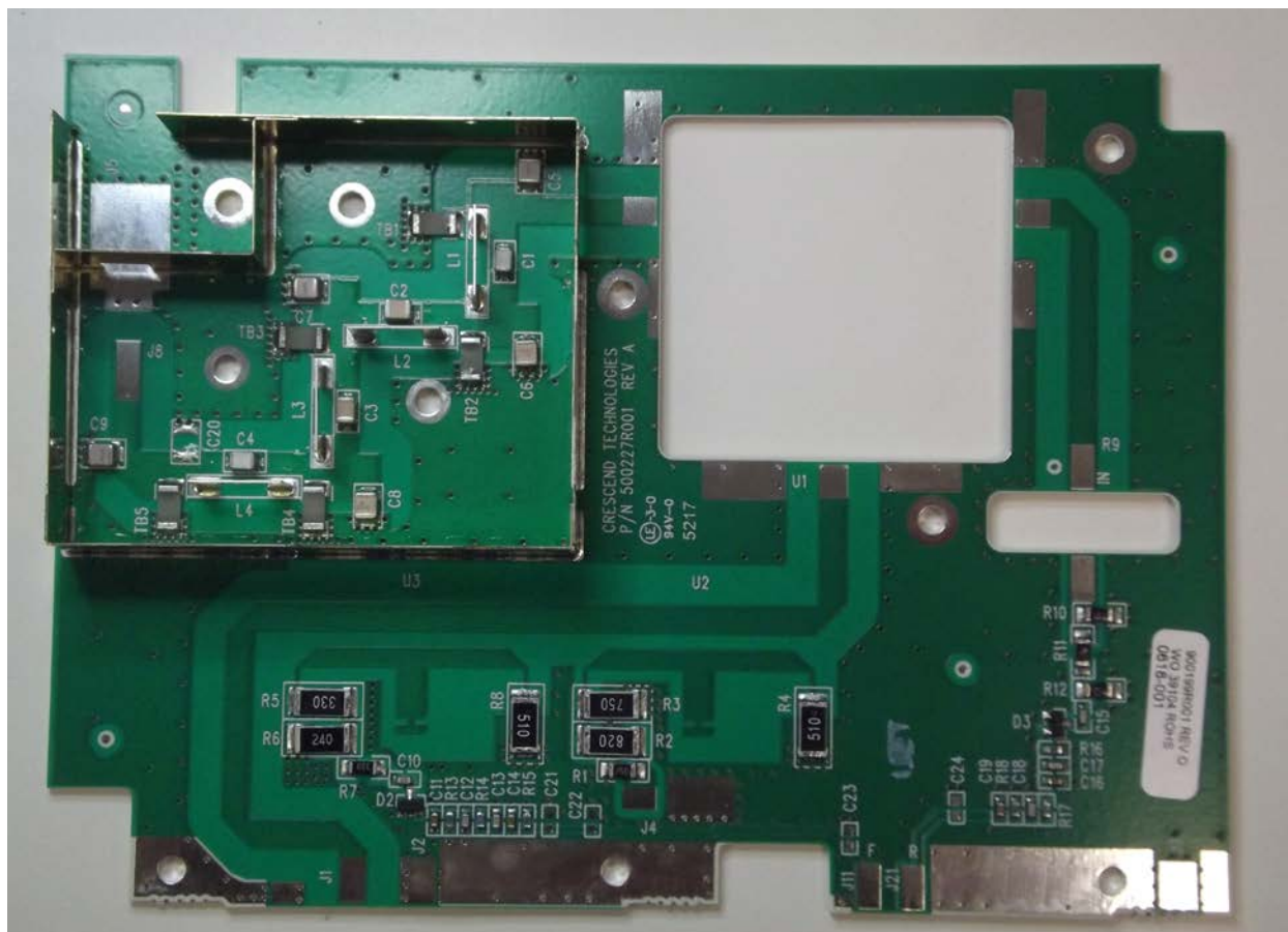
Power Amplifier Output Assembly Top View
