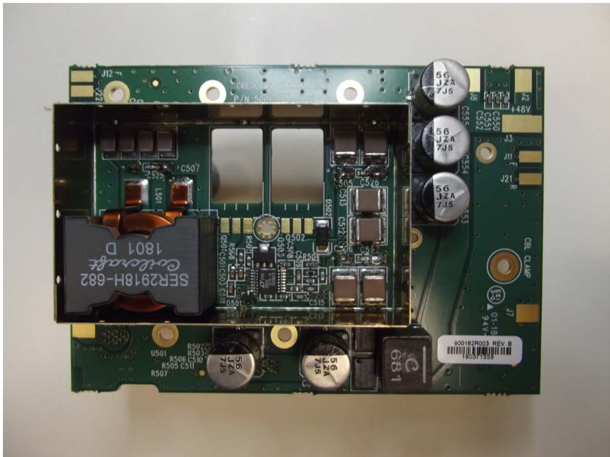
Power Amplifier Switcher Assembly Top View
