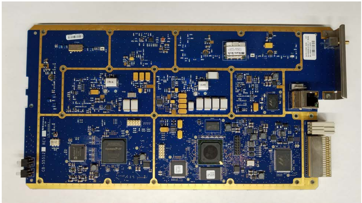
TX Module Top View
