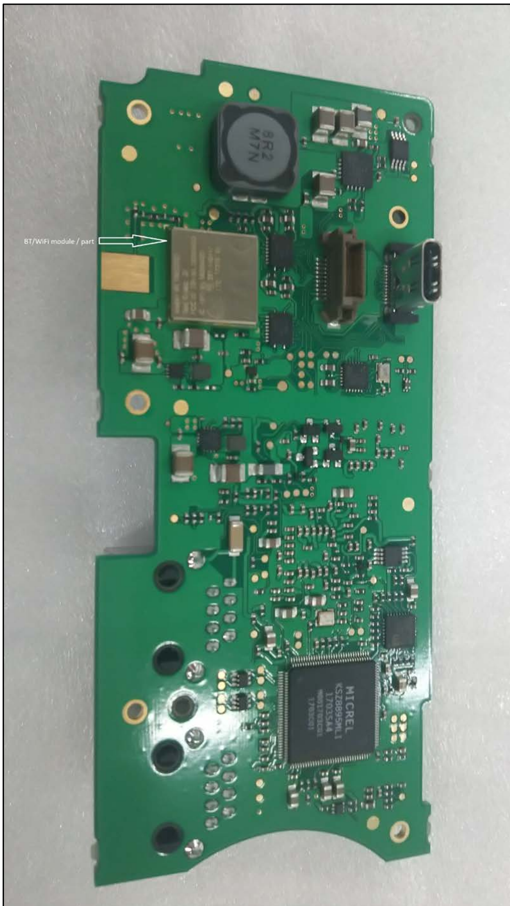
Main Board View 2 with BT/Wi-Fi Module Location Indicated
