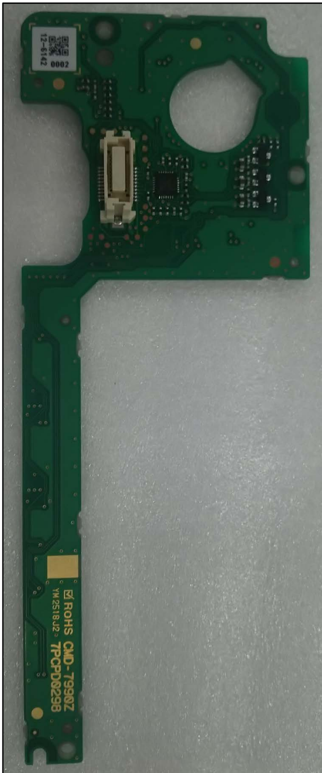
Keypad Board Front and Back Views
