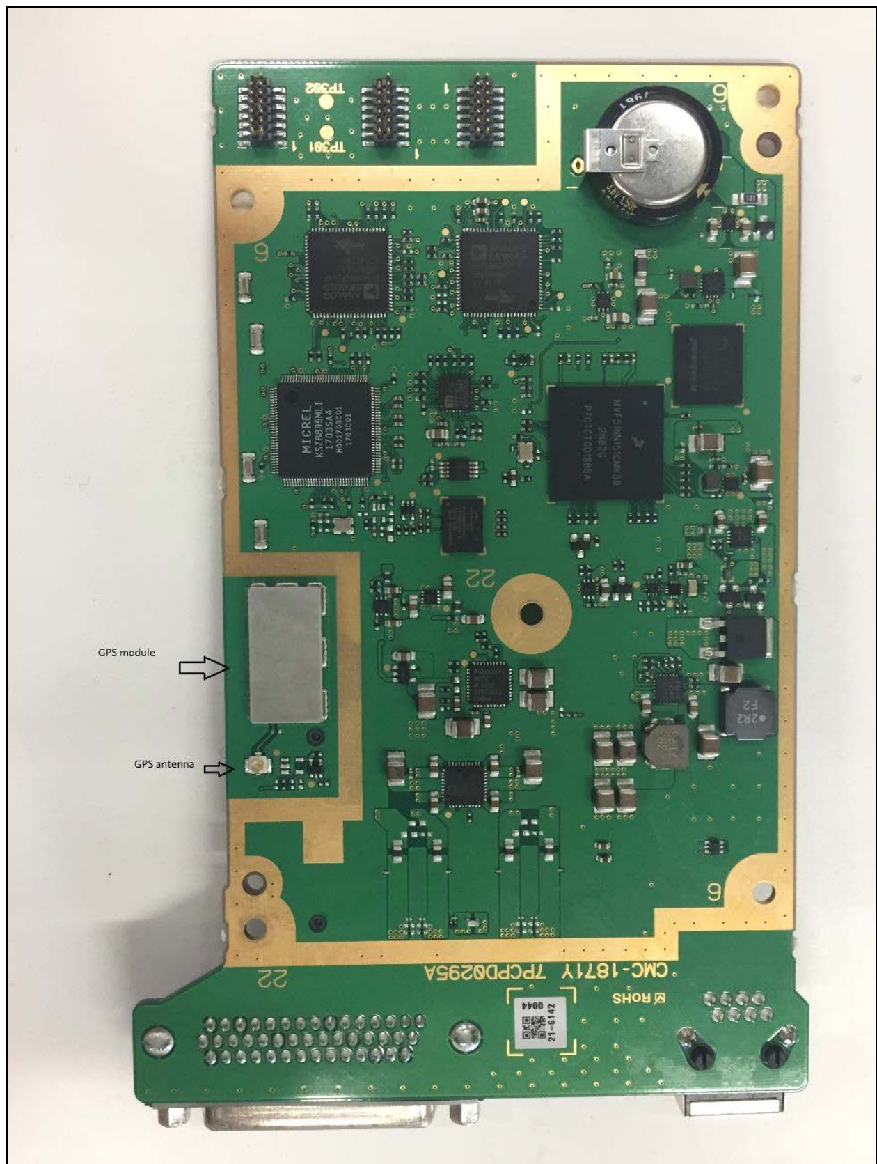
VCH Logic Board Component Side with Shields and GPS Module and Antenna Indicated
