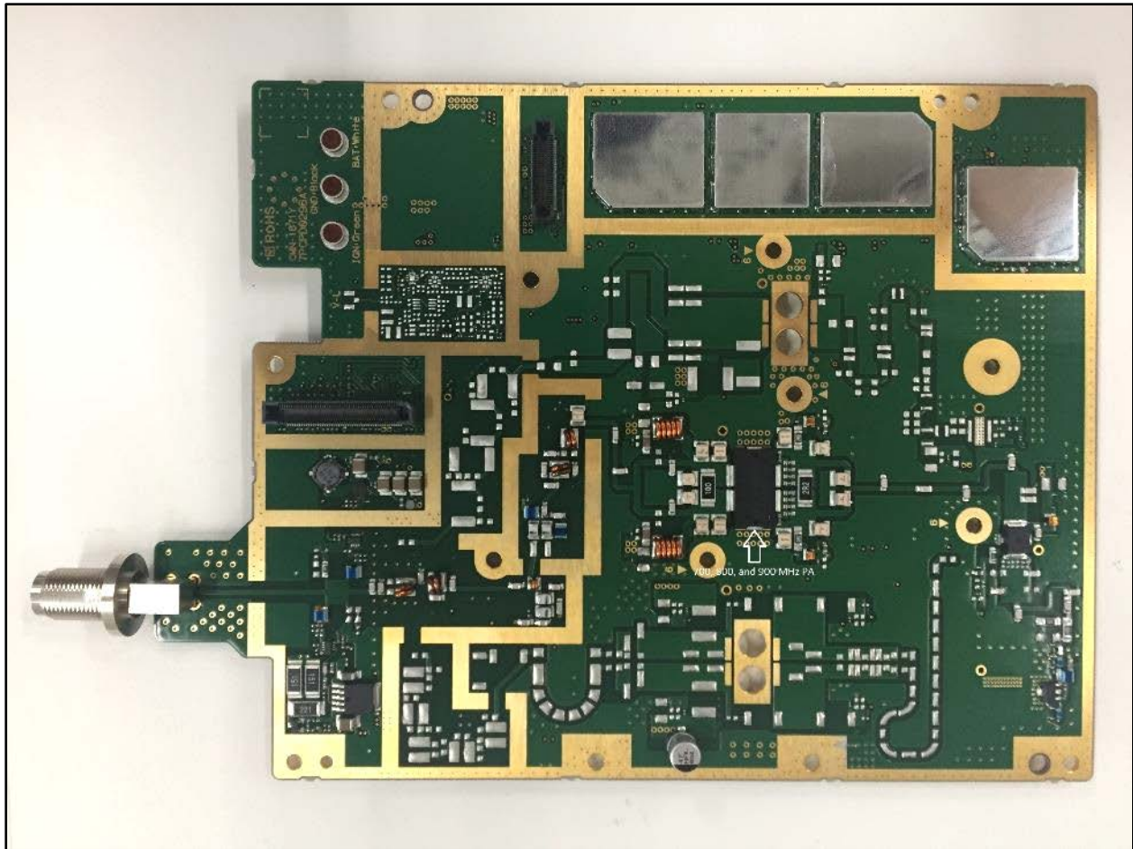
VCH RF Board Component Side with Shields and Transmitter Location Indicated
