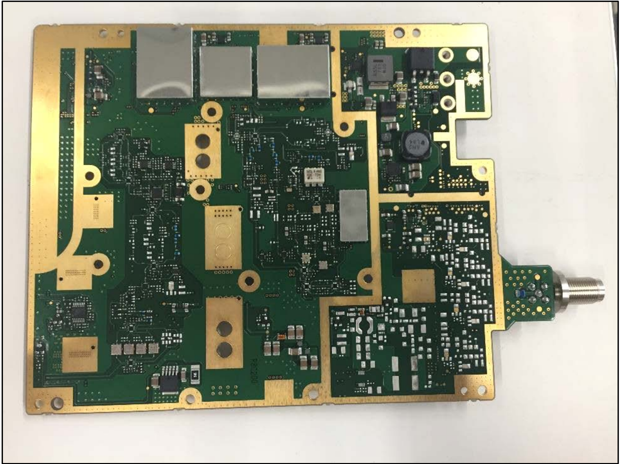
VCH RF Board Solder Side with Shields
