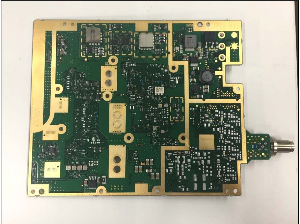
VCH RF Board Solder Side without Shields
