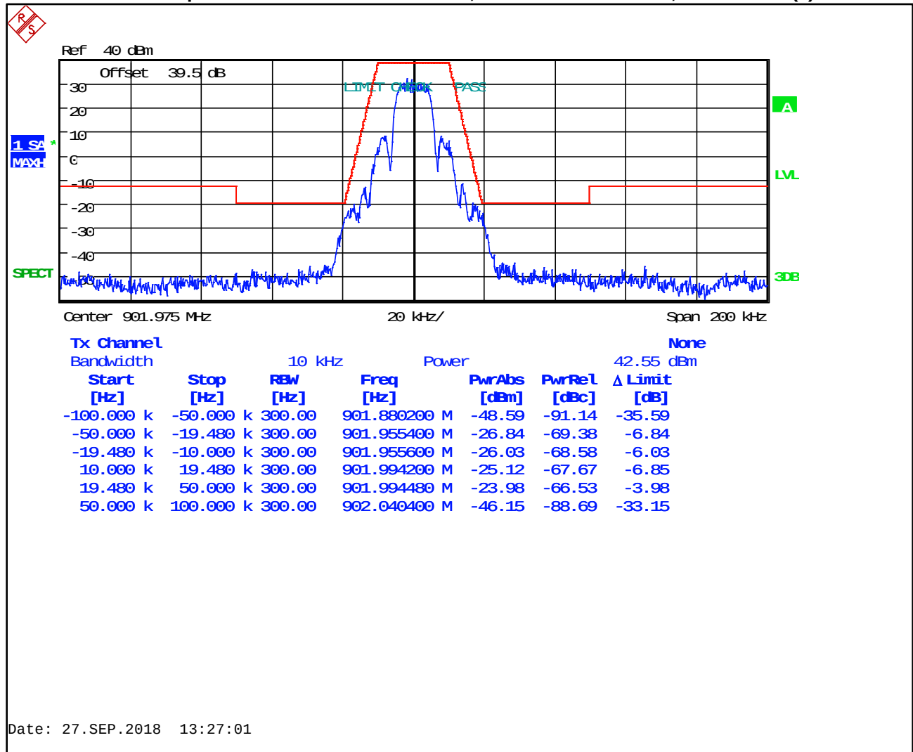
Plot 7-3: Occupied Bandwidth – 901.9750 MHz; 2-Level FSK 9600 WB; Mask 24.133(1)
