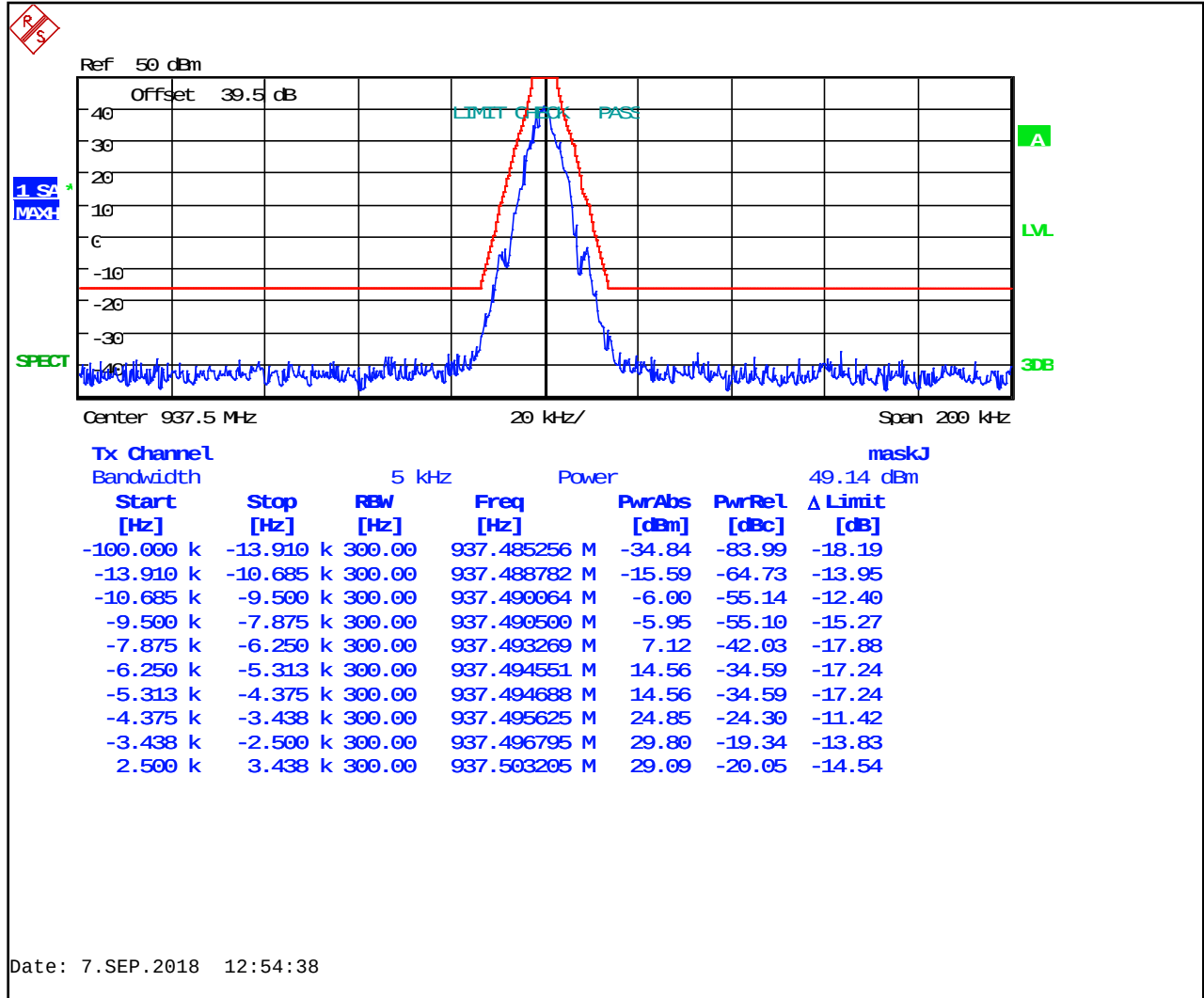
Plot 8-76: Occupied Bandwidth – 937.5000 MHz; P25; Mask J
