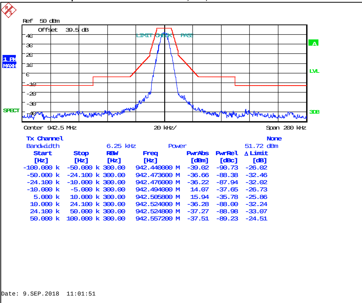
Plot 8-80: Occupied Bandwidth – 942.5000 MHz; P25; Mask C
