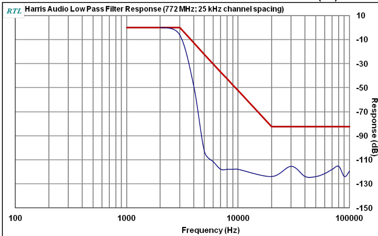
Plot 10-6: Modulation Characteristics – Audio Low Pass Filter – 772.0000 MHz (WB)
