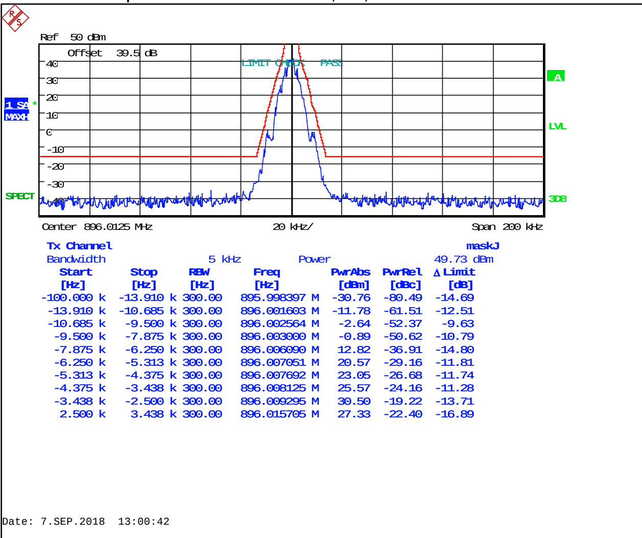
Plot 8-72: Occupied Bandwidth – 896.0125 MHz; P25; Mask J
