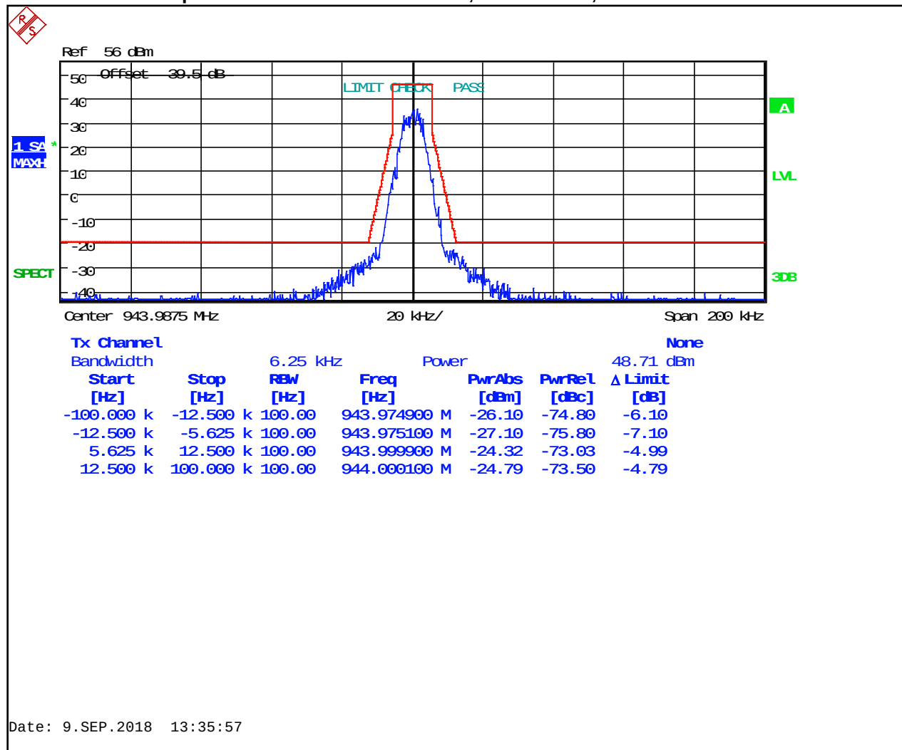
Plot 8-99: Occupied Bandwidth – 943.9875 MHz; P25 Phase 2; Mask D
