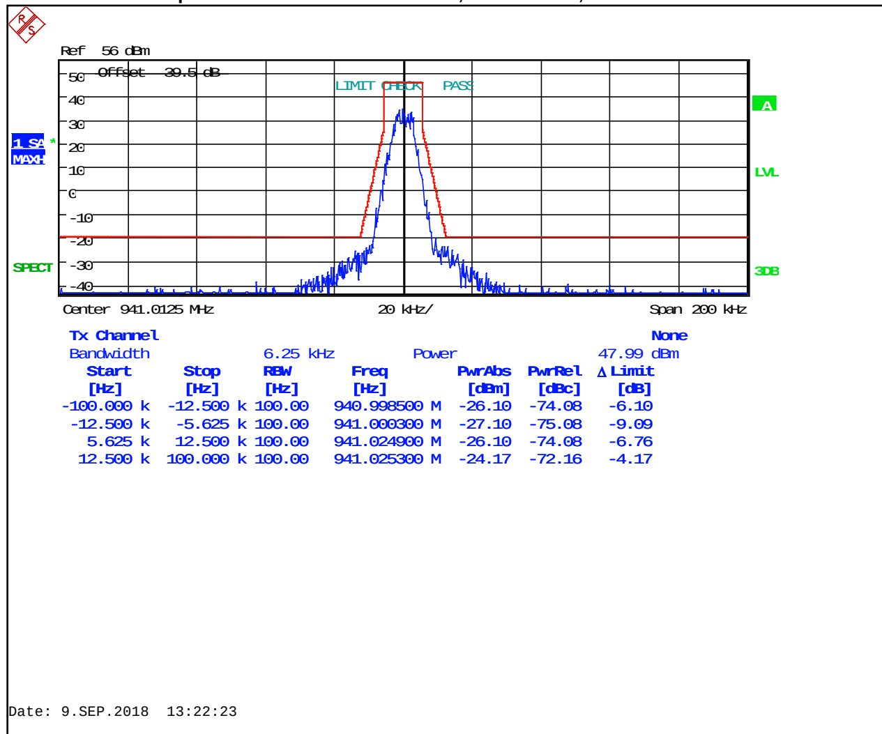
Plot 8-95: Occupied Bandwidth – 941.0125 MHz; P25 Phase 2; Mask D
