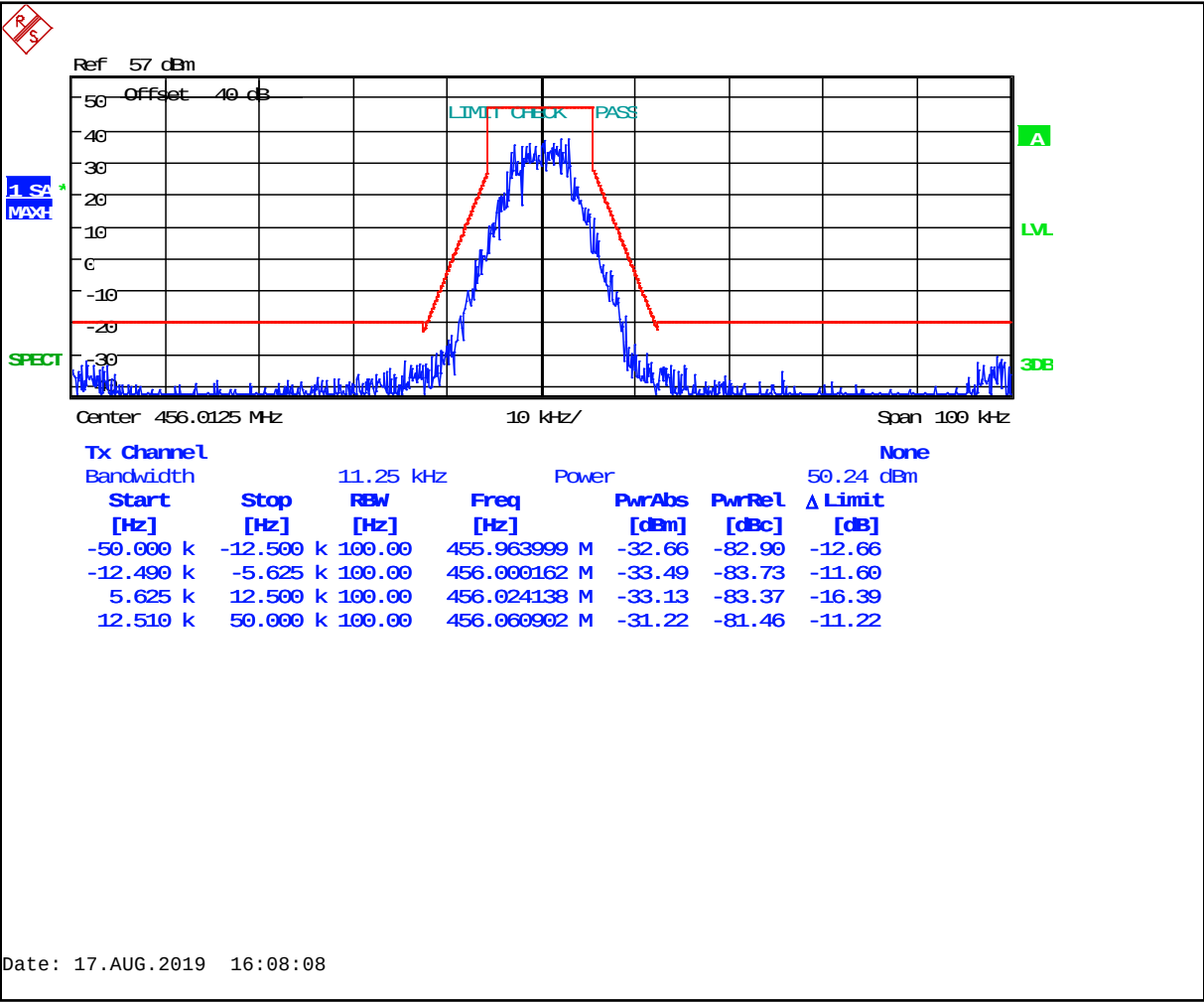
Plot 8-84: Occupied Bandwidth – 456.0125 MHz – CPM TDMA (Mask D)
