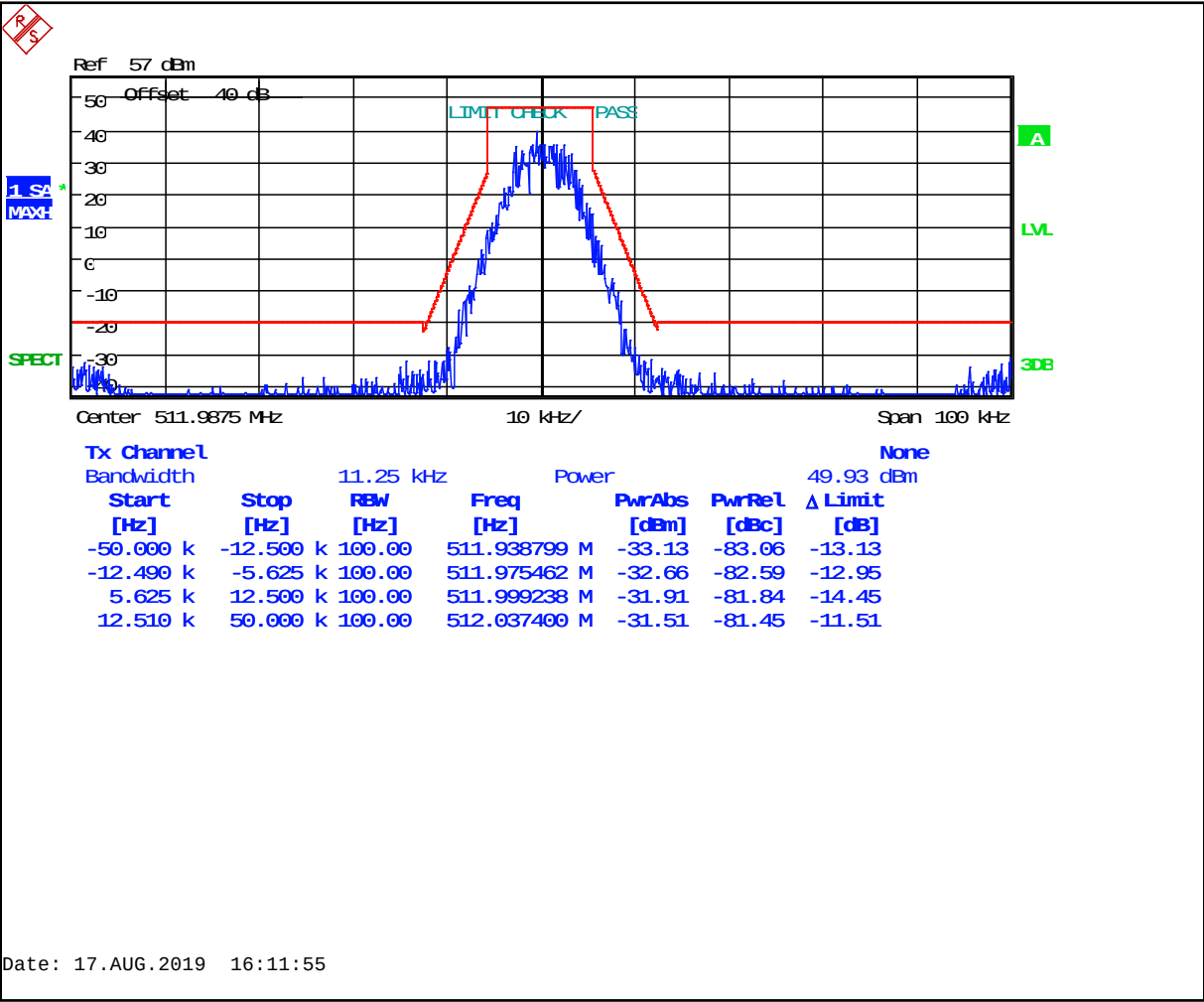
Plot 8-86: Occupied Bandwidth – 511.9875 MHz – CPM TDMA (Mask D)
