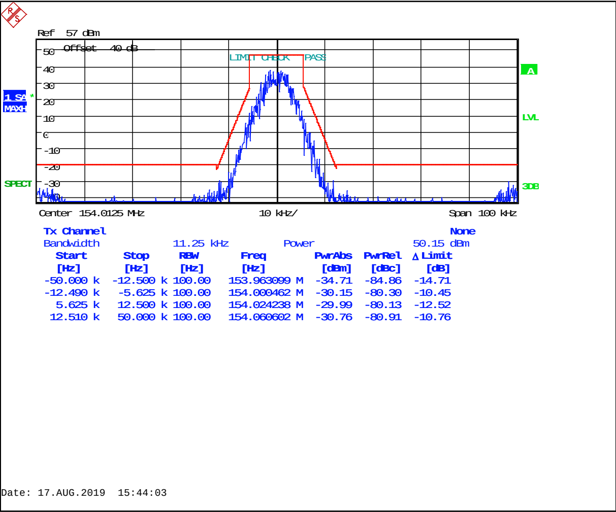
Plot 8-73: Occupied Bandwidth – 154.0125 MHz – CPM TDMA (Mask D)
