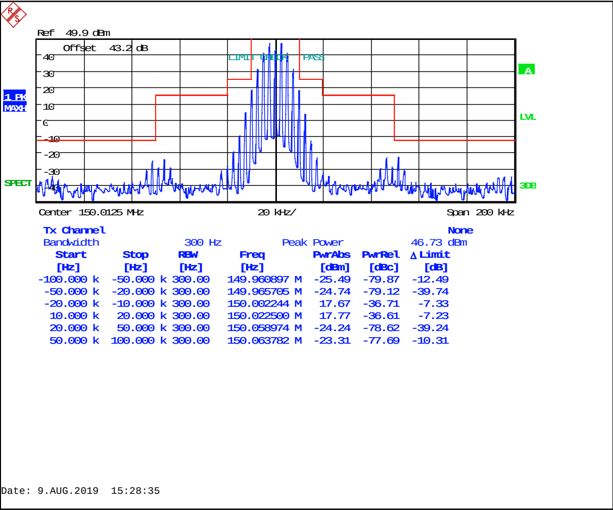
Plot 8-9: Occupied Bandwidth – 150.0125 MHz – Analog Wideband (Mask B)
