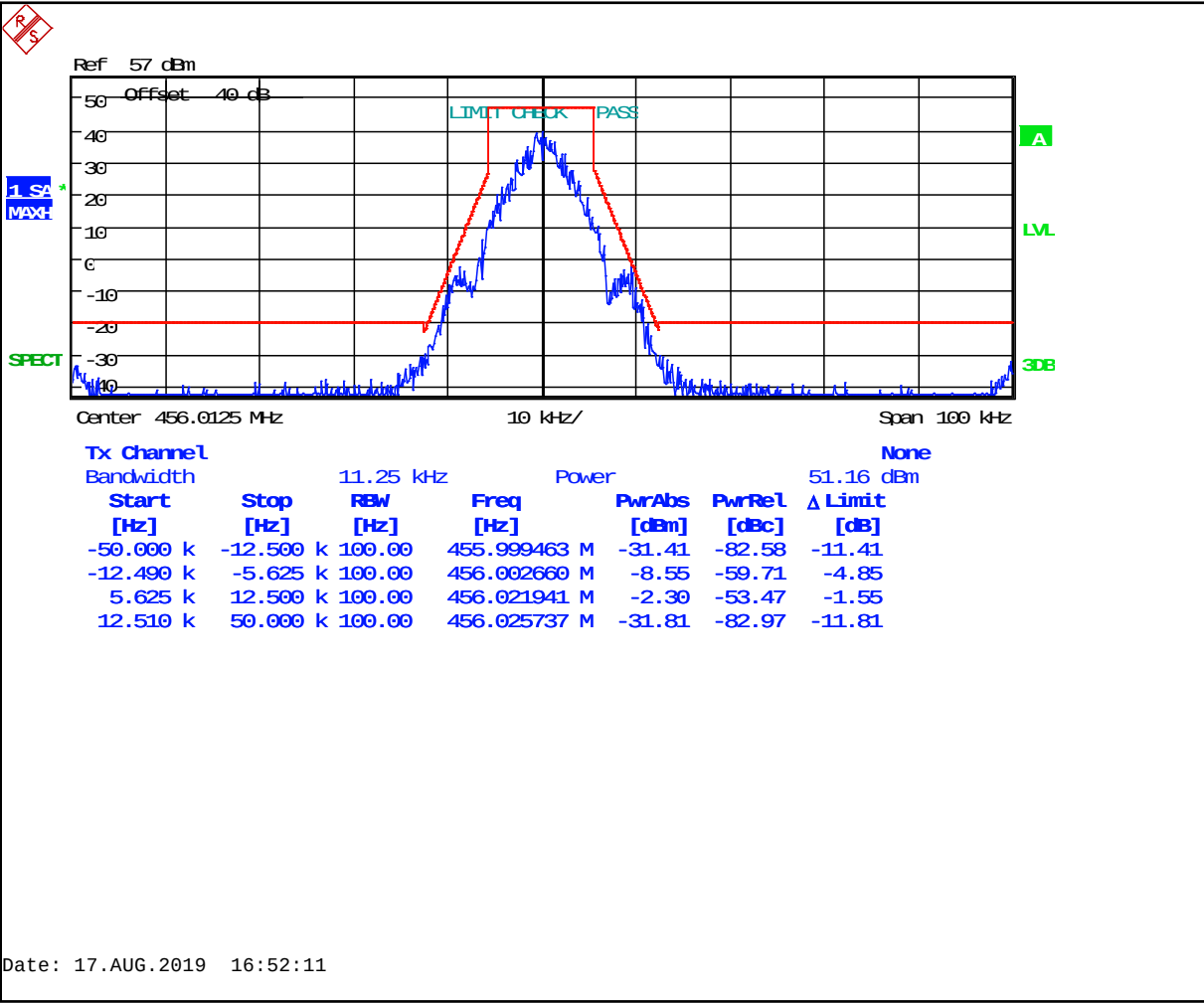
Plot 8-126: Occupied Bandwidth – 456.0125 MHz – 2-Level FSK 9600 NB (Mask D)
