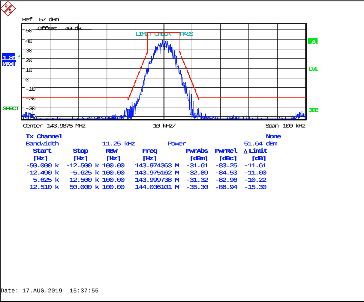
Plot 8-70: Occupied Bandwidth – 143.9875 MHz – CPM TDMA (Mask D)
