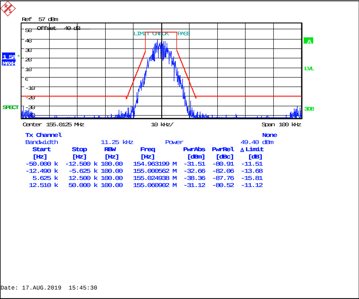
Plot 8-74: Occupied Bandwidth – 155.0125 MHz – CPM TDMA (Mask D)
