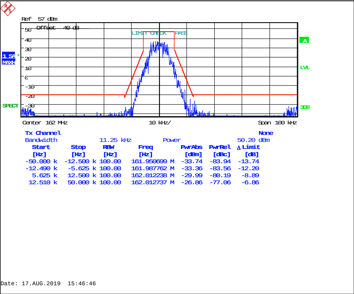
Plot 8-75: Occupied Bandwidth – 162.0000 MHz – CPM TDMA (Mask D)
