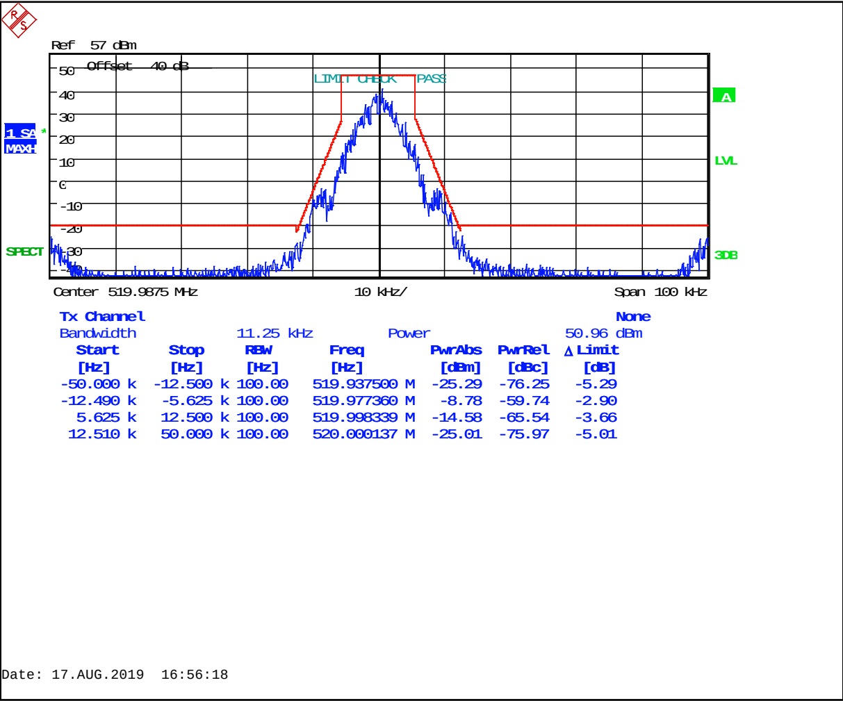
Plot 8-129: Occupied Bandwidth – 519.9875 MHz – 2-Level FSK 9600 NB (Mask D)
