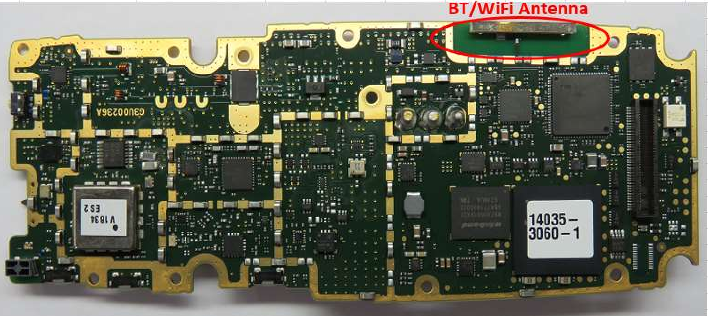
Main board showing BT/WiFi antenna locations
