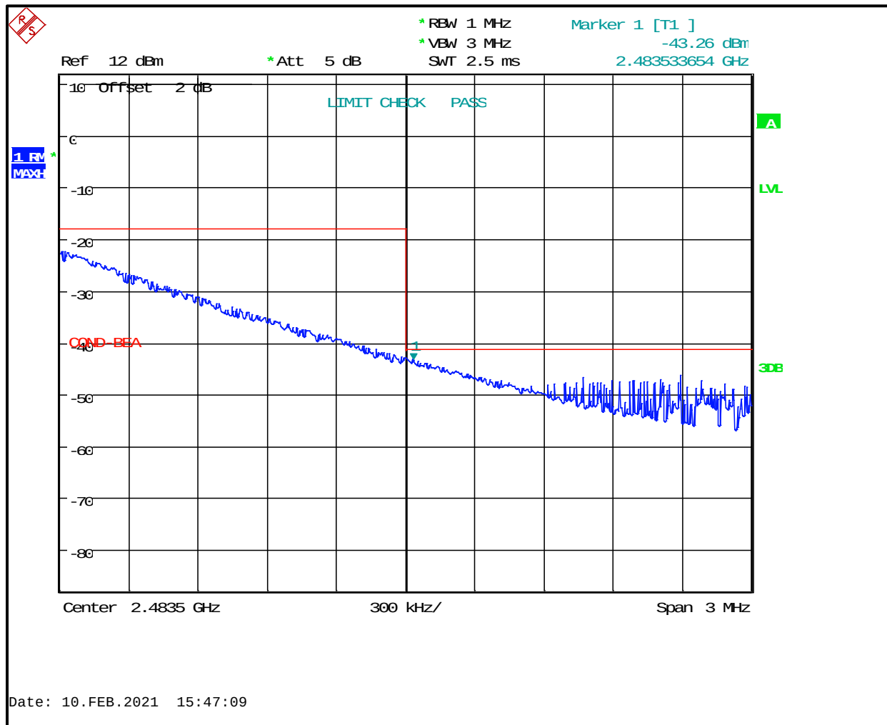
Plot 4-6: Upper Band Edge - Average Hopping
