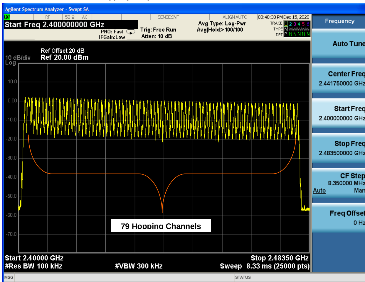
Plot 8-1: Number of Hopping Frequencies
