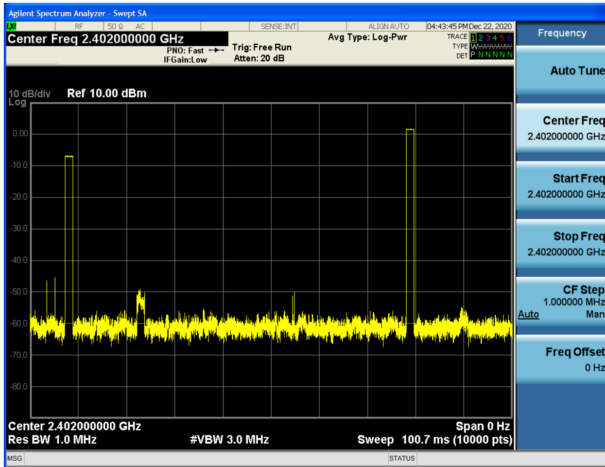
Plot 8-4: Duty Cycle in 100 ms
