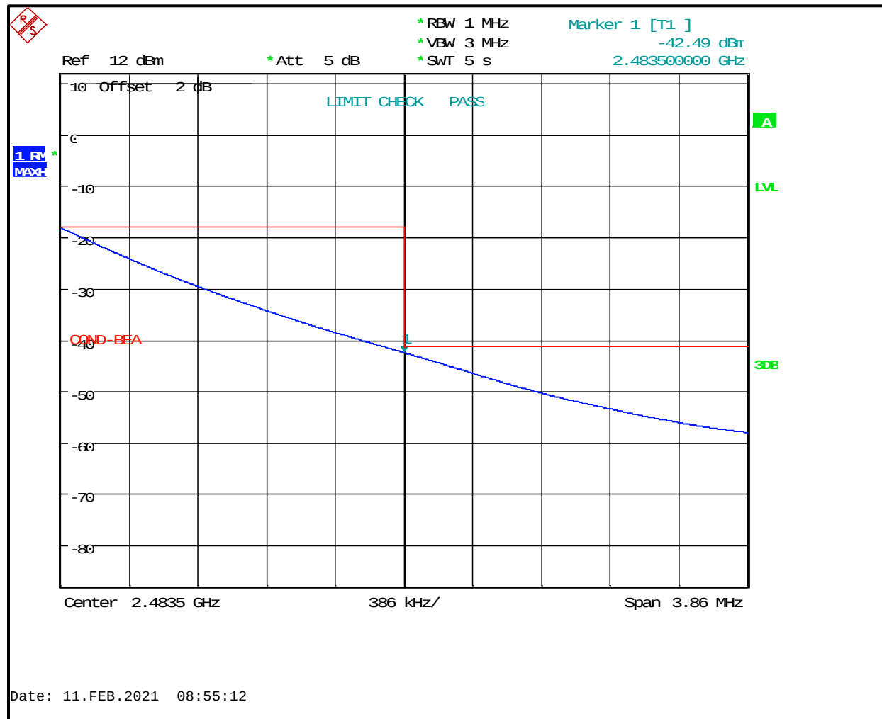
Plot 4-5: Upper Band Edge - Average
