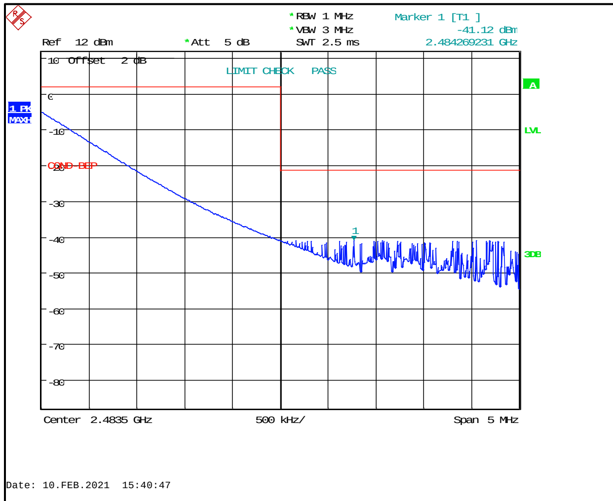
Plot 4-8: Upper Band Edge - Peak Hopping
