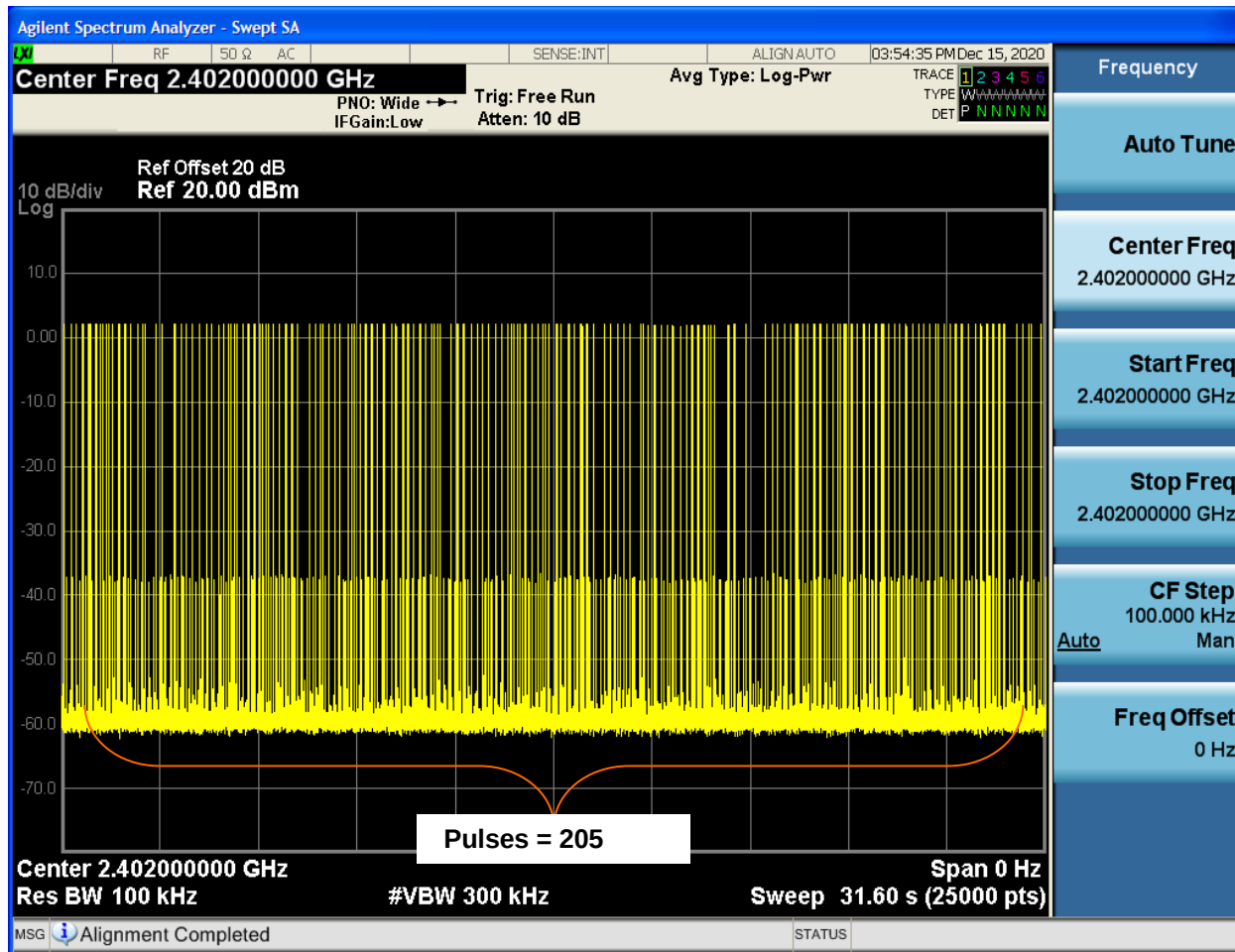
Plot 8-3: Time of Occupancy (Dwell Time 31.6 Second Sweep)
