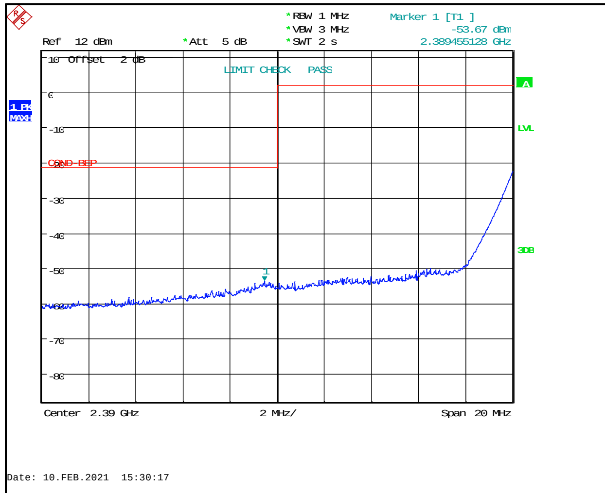
Plot 4-3: Lower Band Edge - Peak
