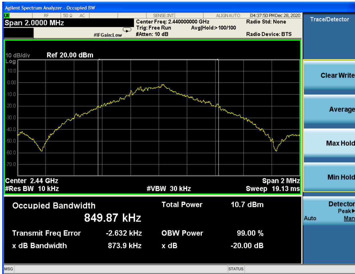
Plot 6-2: 20 dB and 99% Bandwidth – 2440 MHz – GFSK
