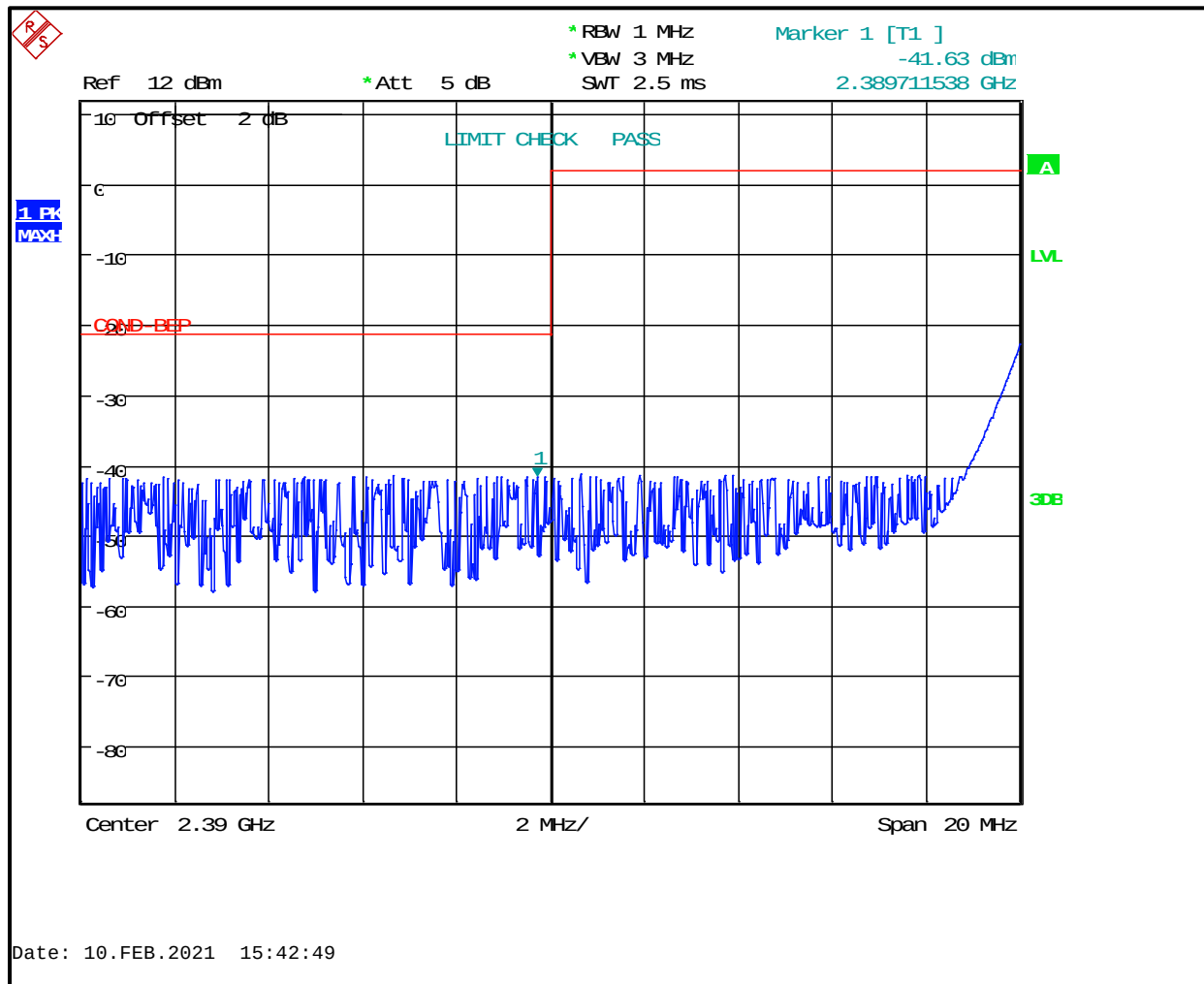
Plot 4-4: Lower Band Edge - Peak Hopping
