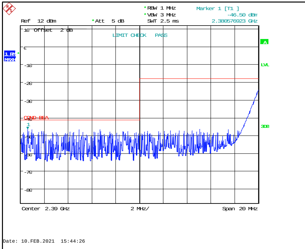
Plot 4-2: Lower Band Edge - Average Hopping
