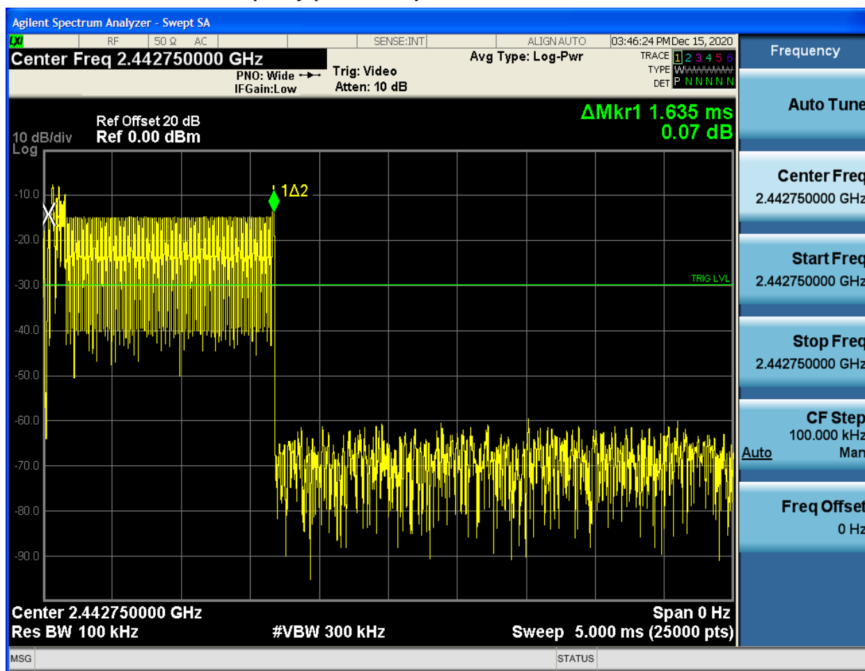
Plot 8-2: Time of Occupancy (Dwell Time)
