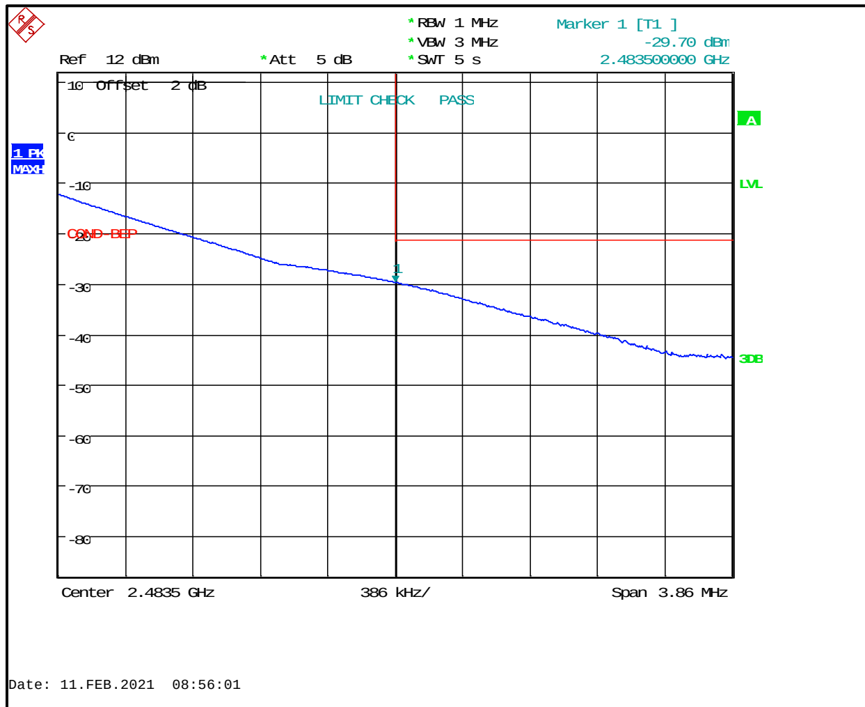
Plot 4-7: Upper Band Edge - Peak
