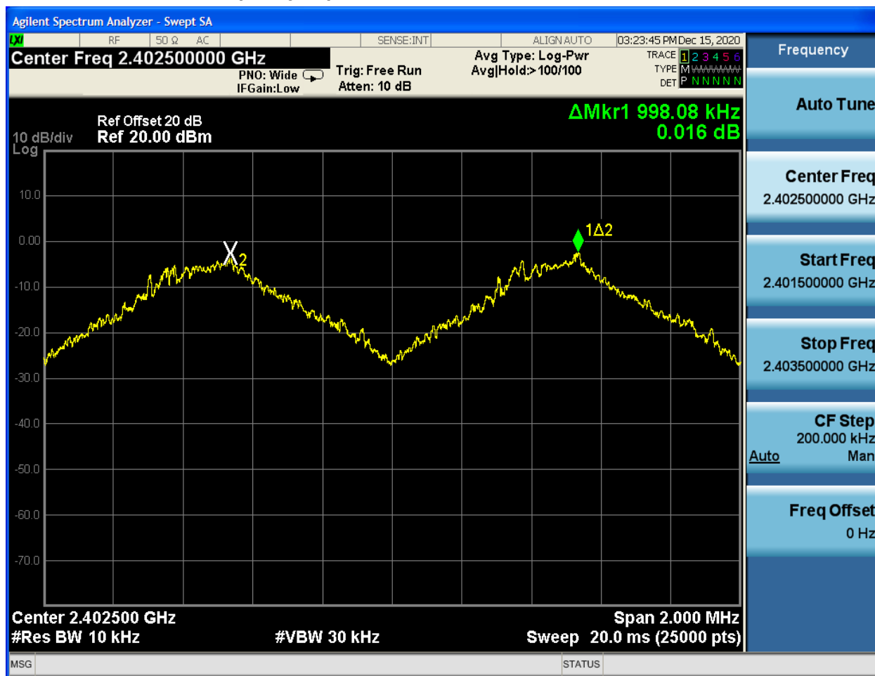
Plot 7-1: Carrier Frequency Separation
