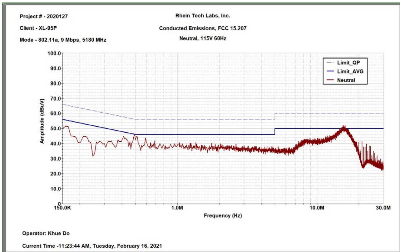
Plot 9-1: Conducted Emissions, AC, Neutral, U-NII1, 5180 MHz
