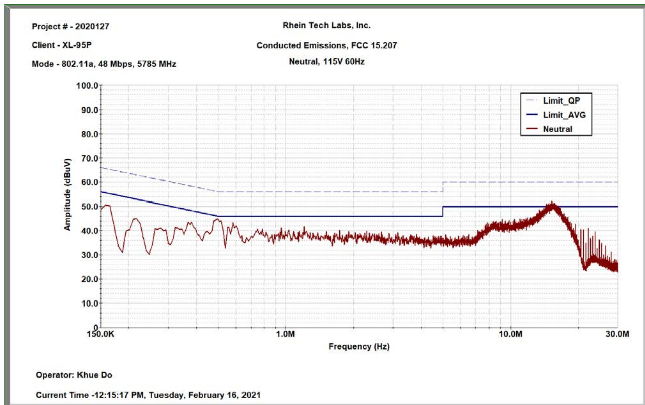
Plot 9-9: Conducted Emissions, AC, Neutral, U-NII3, 5785 MHz
