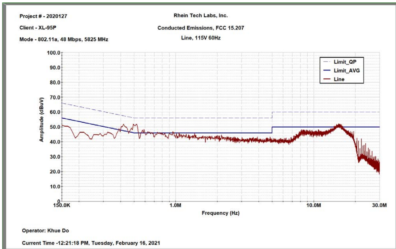
Plot 9-12: Conducted Emissions, AC, Line, U-NII3, 5825 MHz
