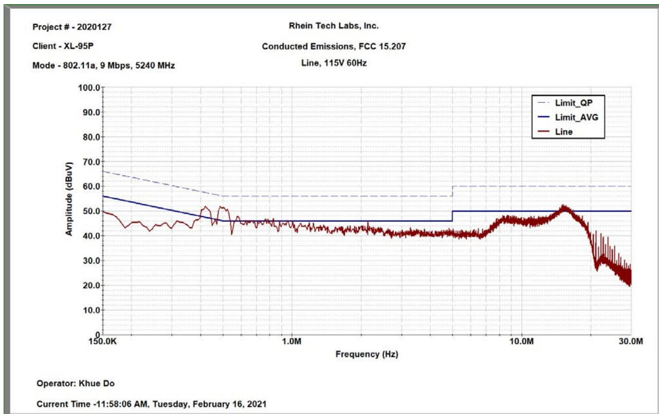
Plot 9-6: Conducted Emissions, AC, Line, U-NII1, 5240 MHz
