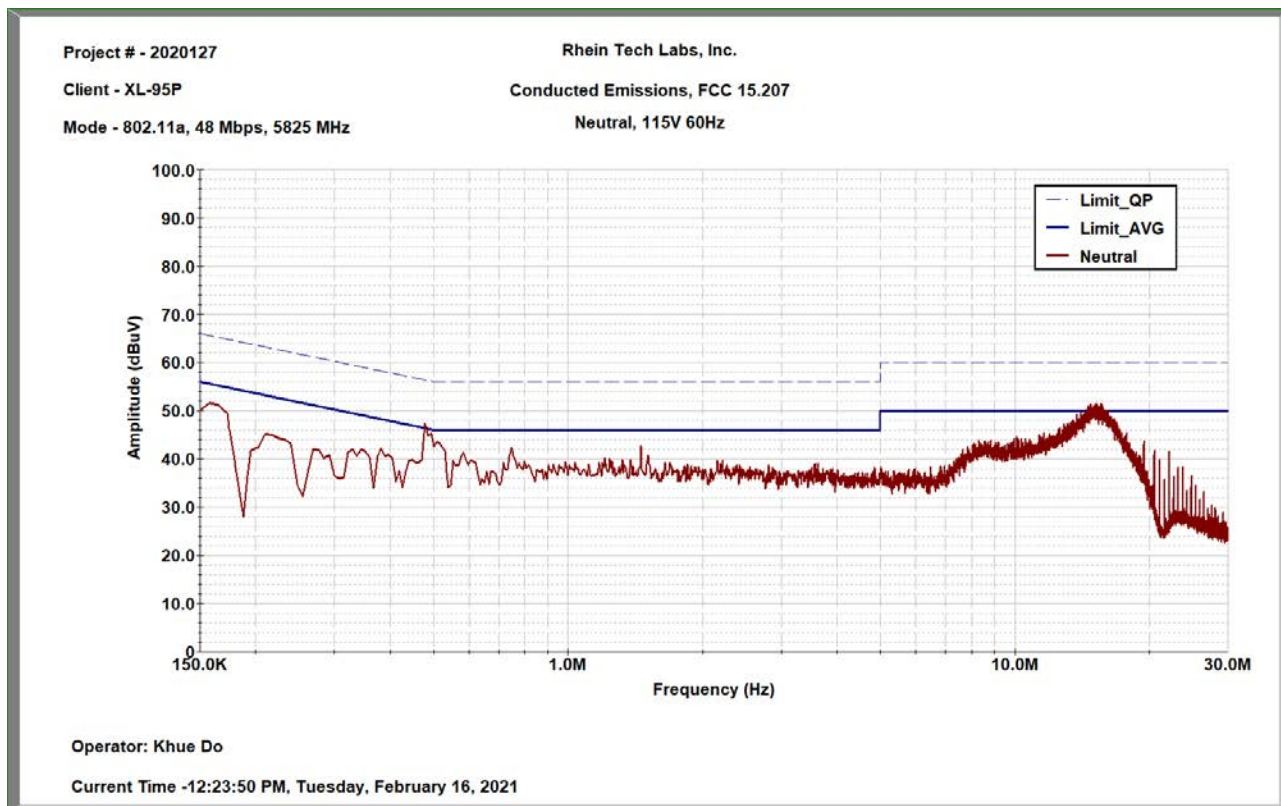
Plot 9-11: Conducted Emissions, AC, Neutral, U-NII3, 5825 MHz
