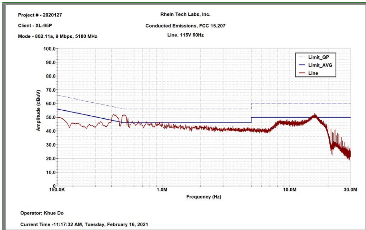
Plot 9-2: Conducted Emissions, AC, Line, U-NII1, 5180 MHz
