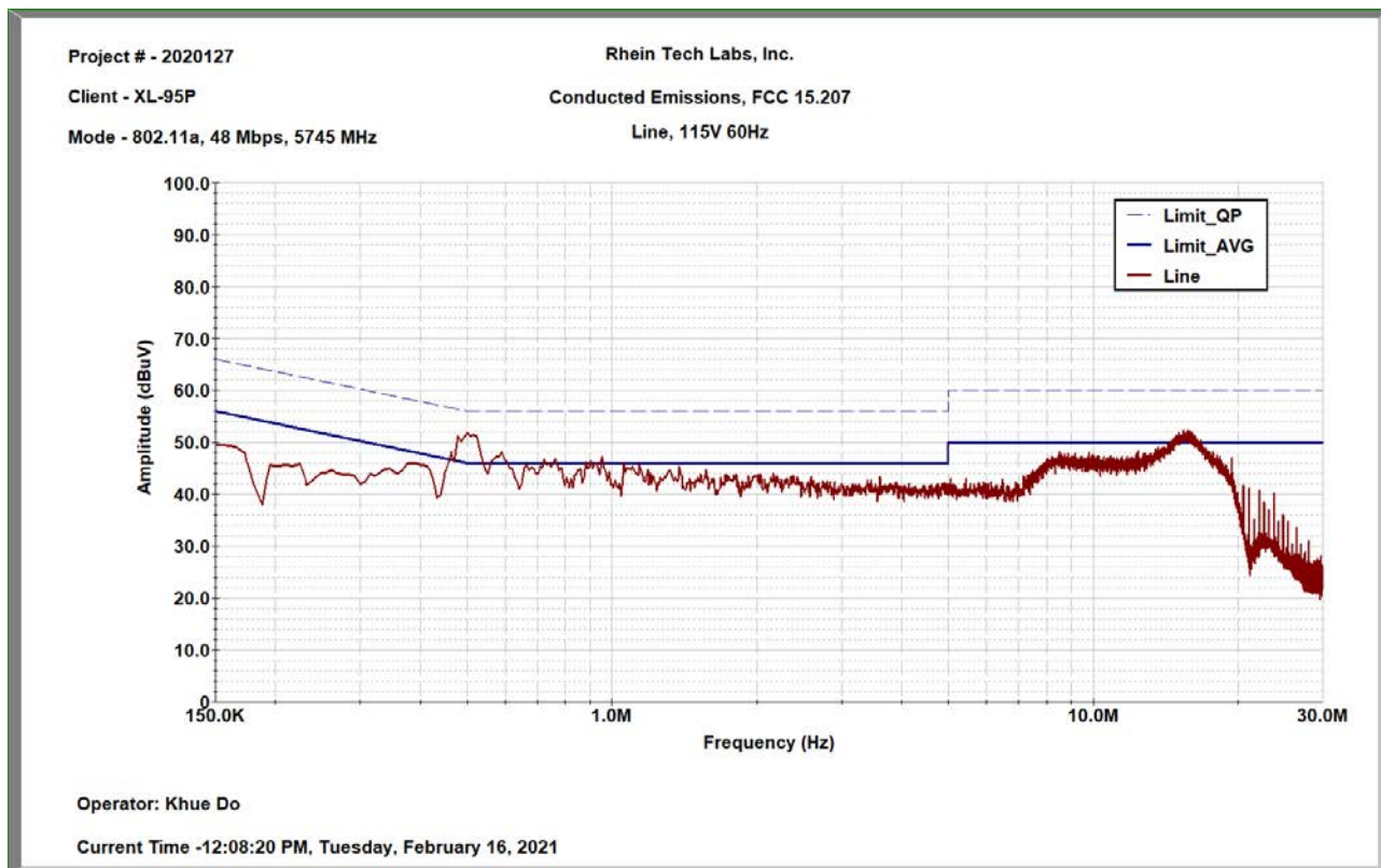
Plot 9-8: Conducted Emissions, AC, Line, U-NII3, 5745 MHz
