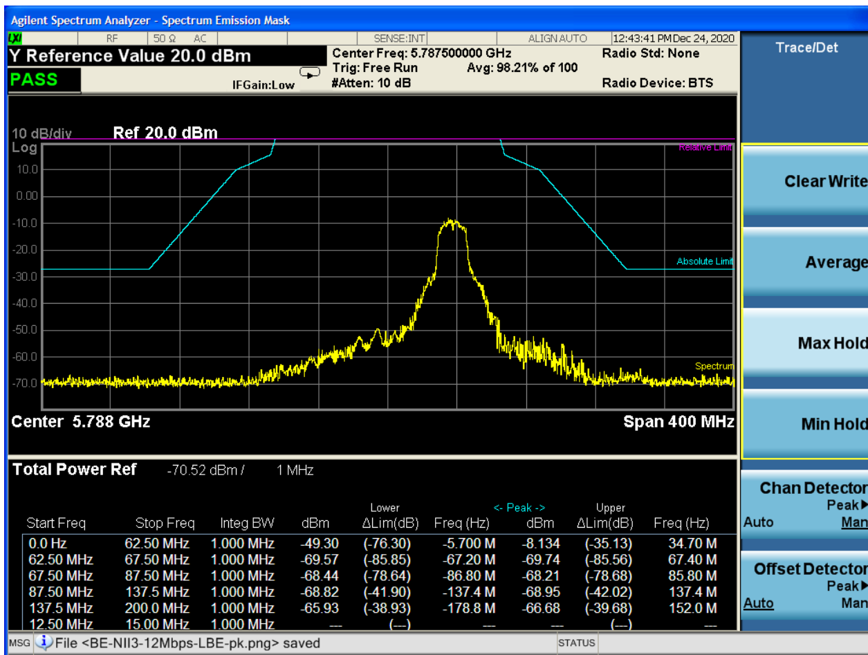
Plot 4-8: Upper Band Edge – Peak – U-NII3 – 802.11a (12.0 Mbps)
