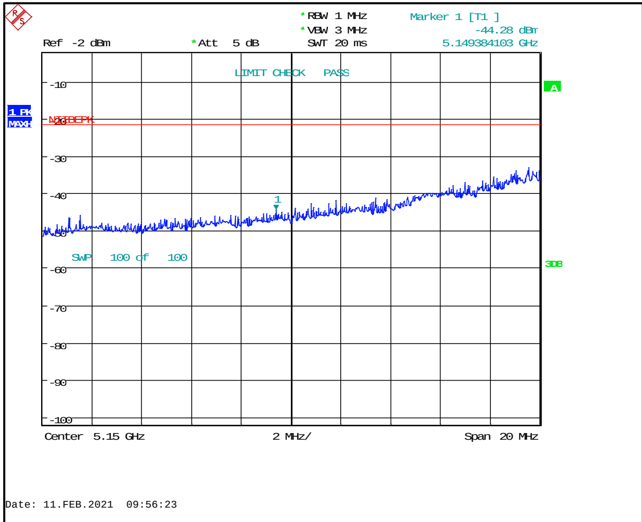
Plot 4-2: Lower Band Edge – U-NII1 – 802.11a (48.0 Mbps) – Peak
