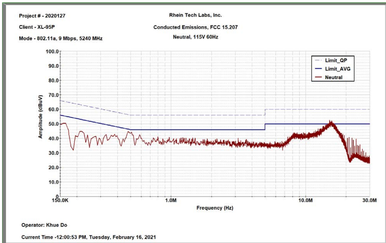
Plot 9-5: Conducted Emissions, AC, Neutral, U-NII1, 5240 MHz
