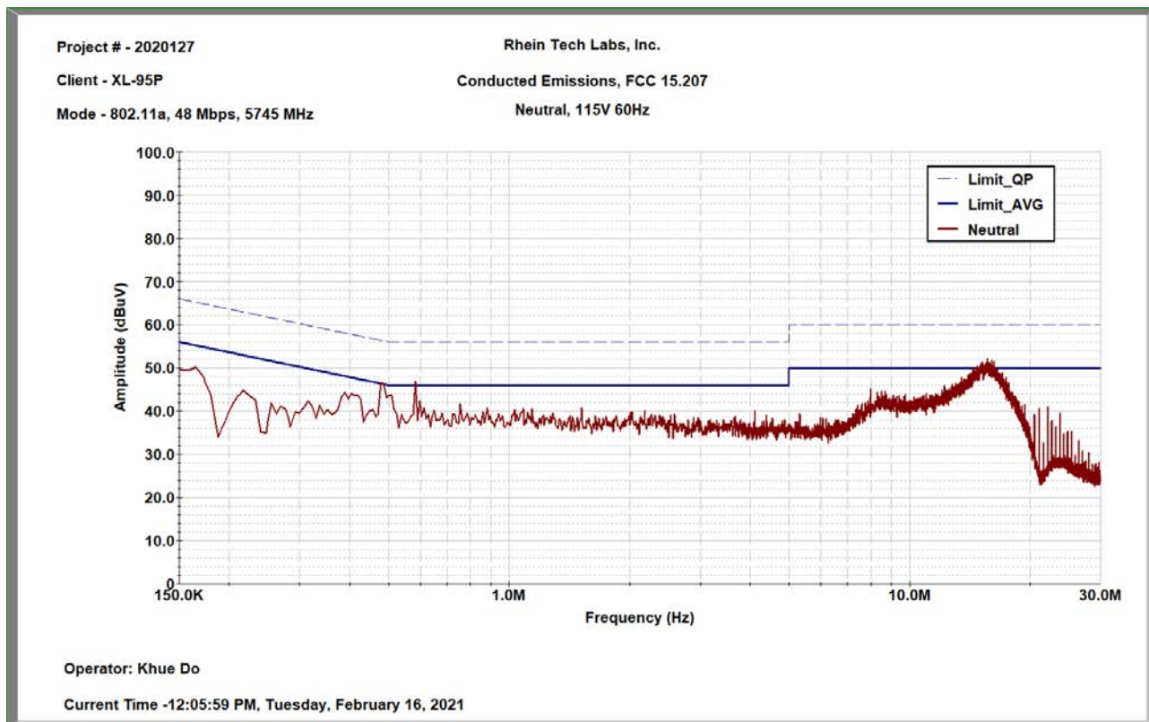
Plot 9-7: Conducted Emissions, AC, Neutral, U-NII3, 5745 MHz
