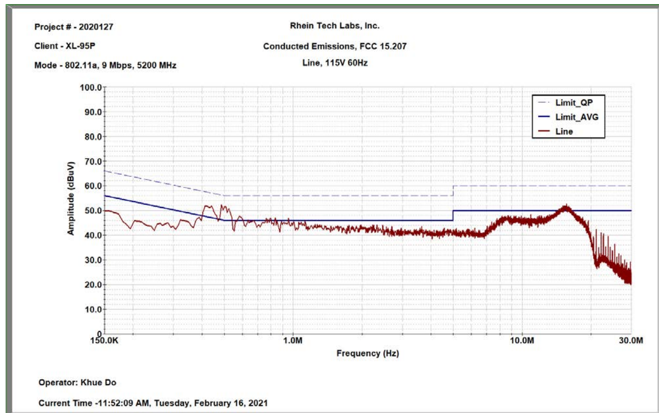
Plot 9-4: Conducted Emissions, AC, Line, U-NII1, 5200 MHz
