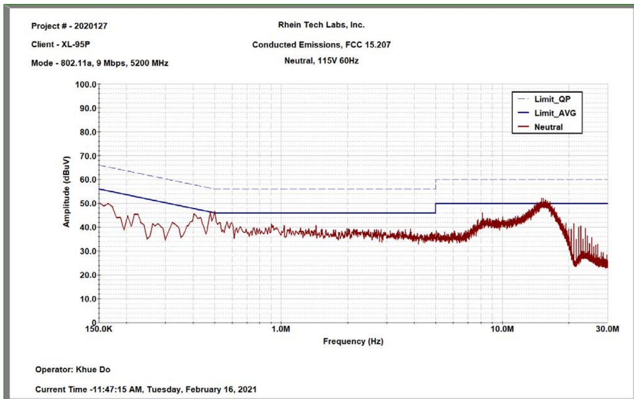
Plot 9-3: Conducted Emissions, AC, Neutral, U-NII1, 5200 MHz
