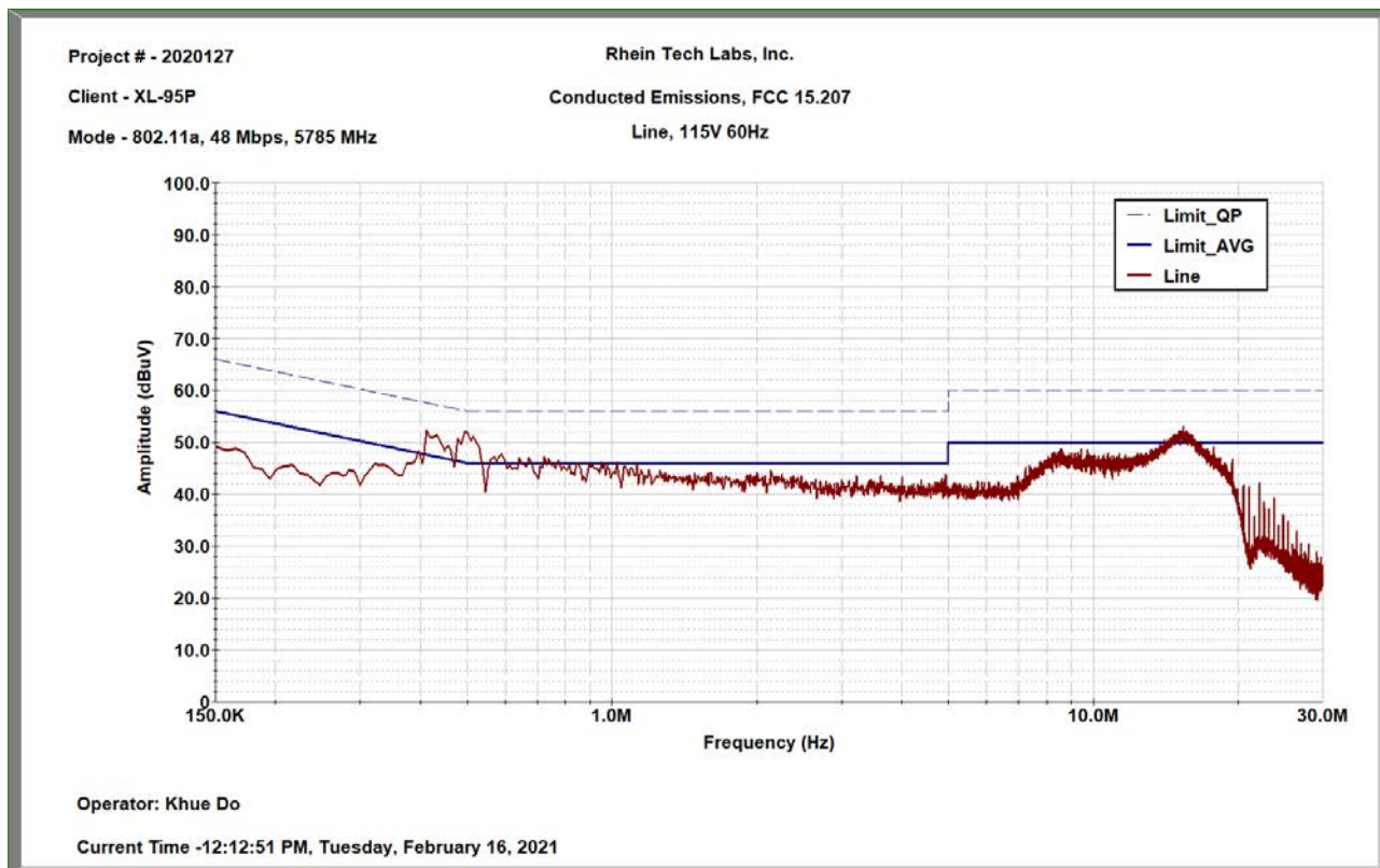
Plot 9-10: Conducted Emissions, AC, Line, U-NII3, 5785 MHz
