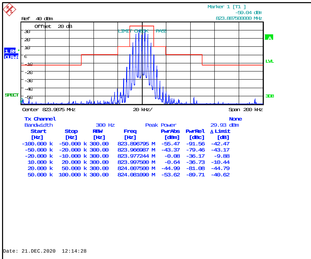
Plot 8-3: Occupied Bandwidth – 823.9875 MHz; WB Analog; Mask B
