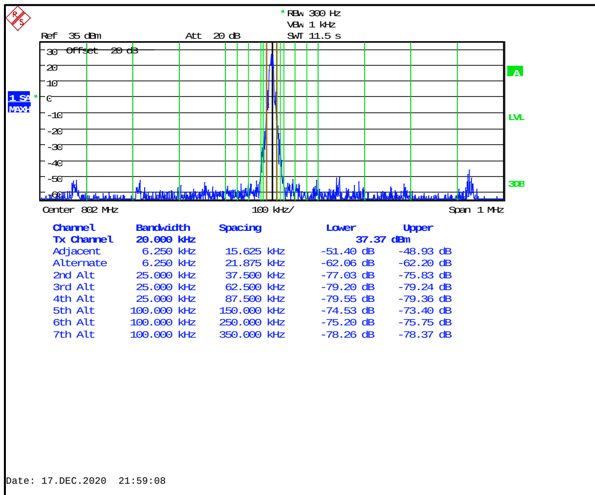
Plot 6-58: Adjacent Channel Power – 802.0000 MHz; WB 2-Lvl FSK 9600 Mode (9.375 kHz - 350 kHz)
