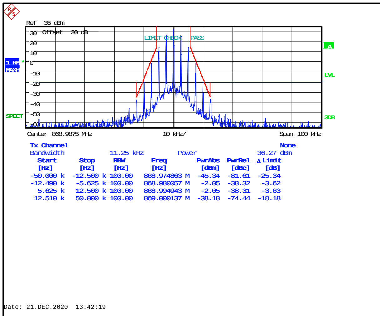
Plot 8-23: Occupied Bandwidth – 868.9875 MHz; NB Analog; Mask D (ISED)
