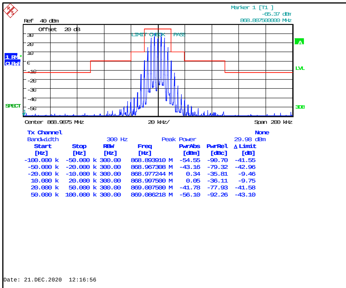
Plot 8-7: Occupied Bandwidth – 868.9875 MHz; WB Analog; Mask B
