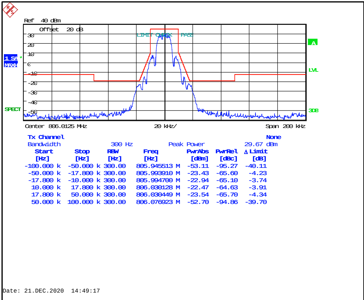
Plot 8-25: Occupied Bandwidth – 806.0125 MHz; WB 2-level FSK 9600; Mask G (ISED)
