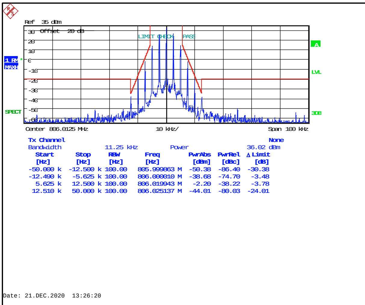
Plot 8-12: Occupied Bandwidth – 806.0125 MHz; NB Analog; Mask D (ISED)
