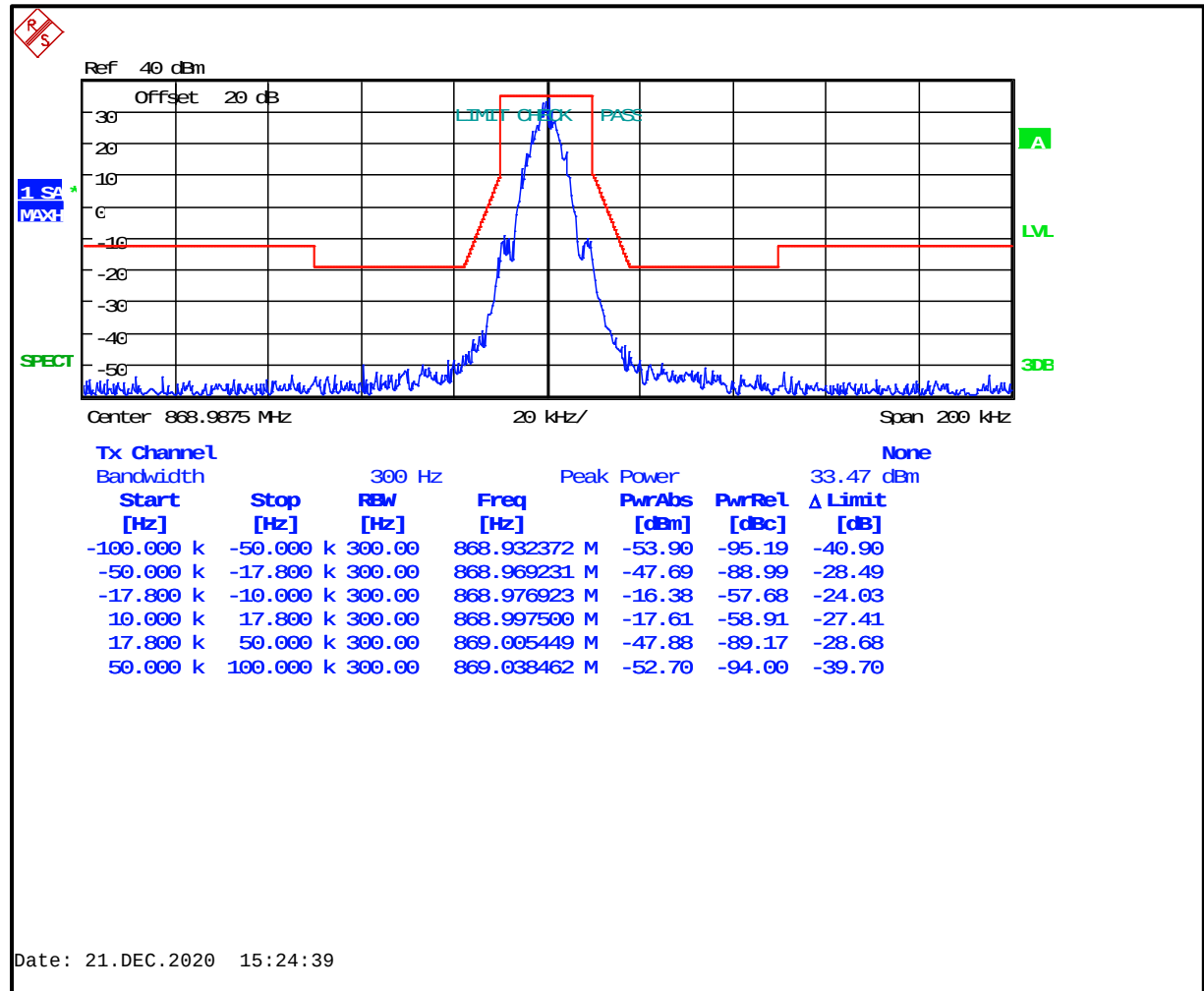
Plot 8-50: Occupied Bandwidth – 868.9875 MHz; NB 2-Level FSK 9600; Mask G
