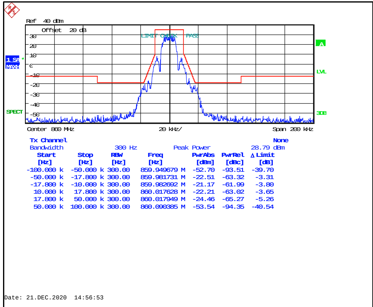
Plot 8-32: Occupied Bandwidth – 860.0000 MHz; WB 2-level FSK 9600; Mask G
