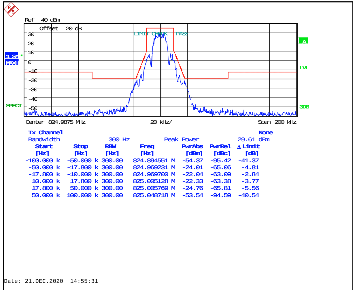
Plot 8-29: Occupied Bandwidth – 824.9875 MHz 9 (EF); WB 2-level FSK 9600; Mask G
