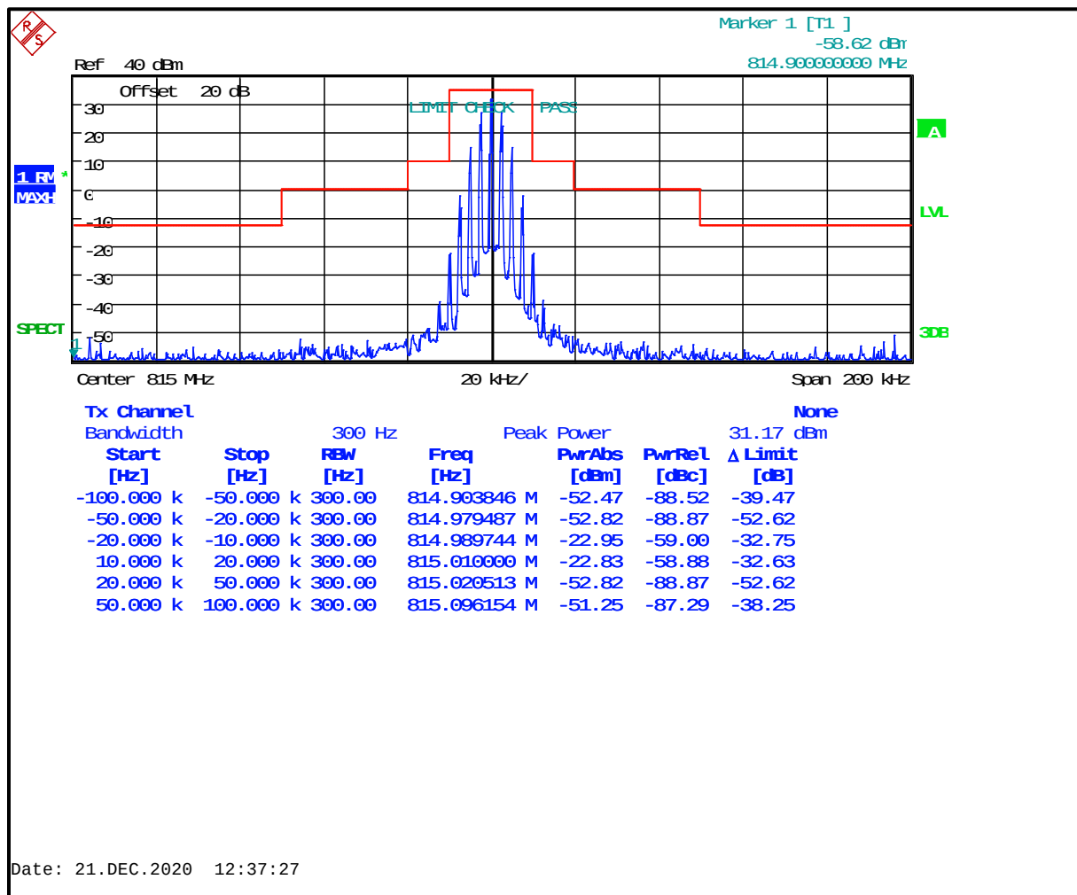
Plot 8-13: Occupied Bandwidth – 815.0000 MHz; NB Analog; Mask B
