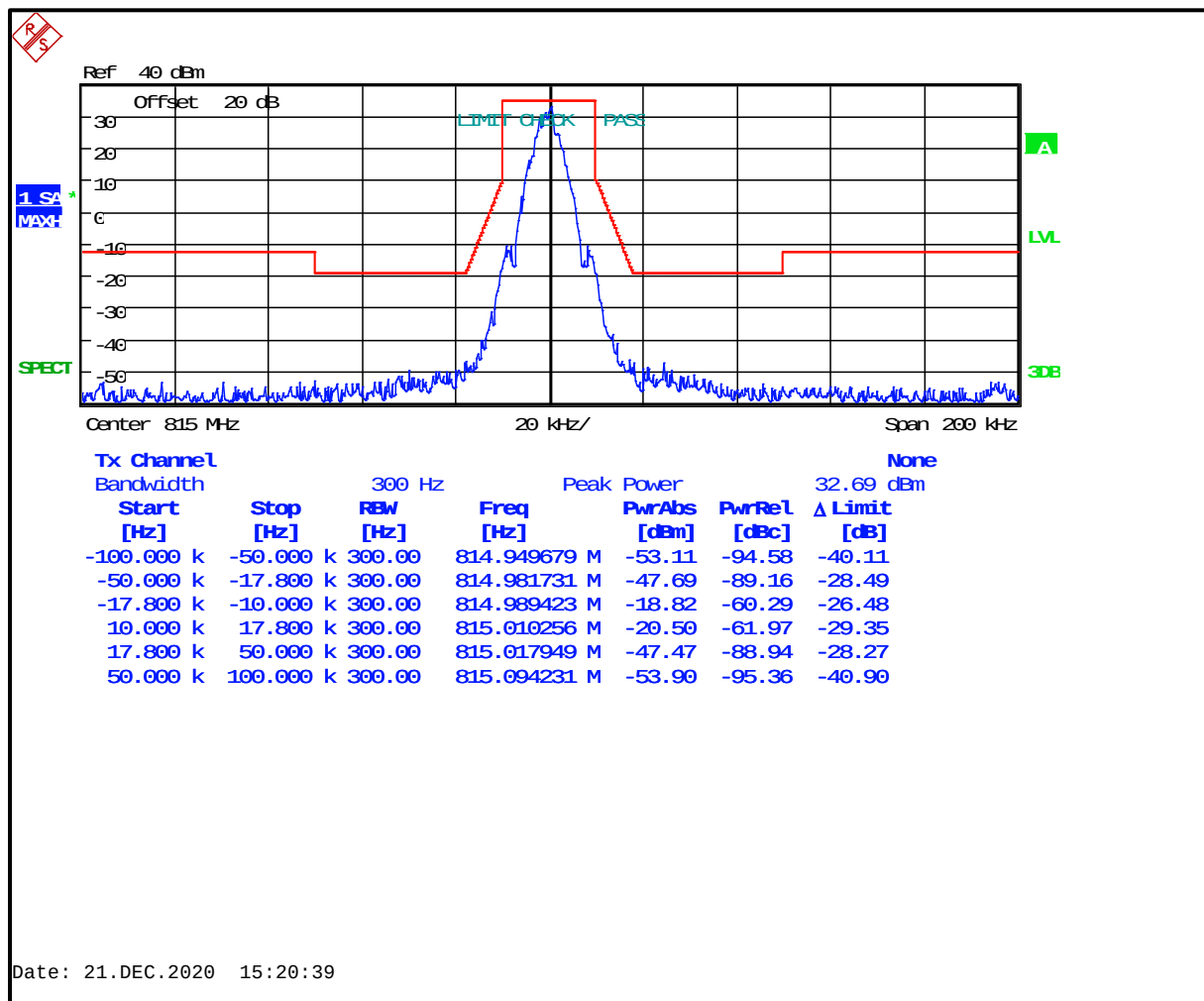
Plot 8-41: Occupied Bandwidth – 815.0000 MHz; NB 2-Level FSK 9600; Mask G
