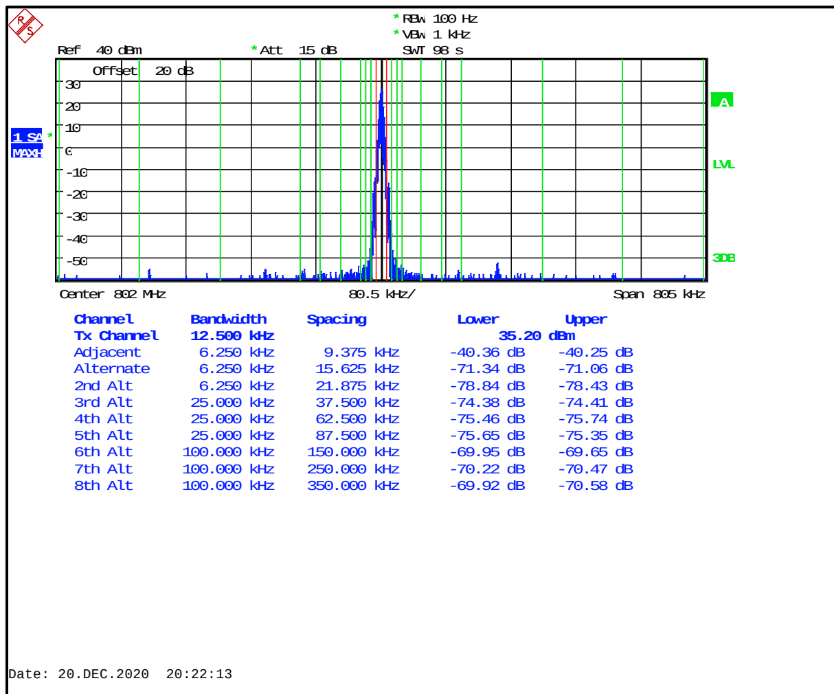
Plot 6-28: Adjacent Channel Power – 802.0000 MHz; NB 2-Level FSK 9600 (9.375 kHz - 350 kHz)
