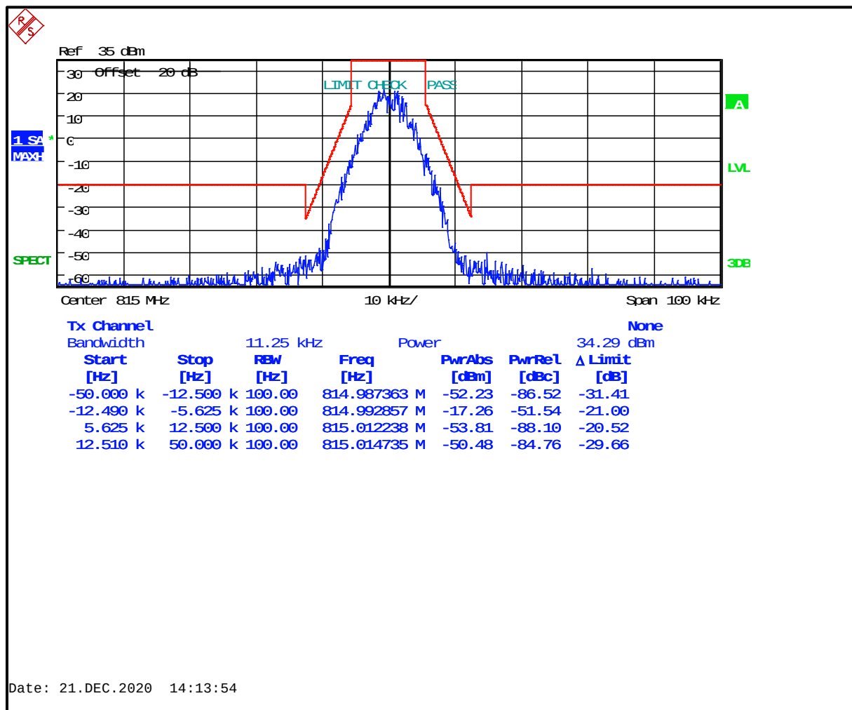
Plot 8-56: Occupied Bandwidth – 815.0000 MHz; C4FM; Mask D (ISED)
