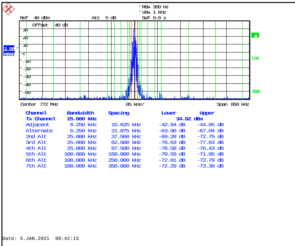
Plot 6-63: Adjacent Channel Power – 772.0000 MHz; HVD-SMR Mode (9.375 kHz - 350 kHz)
