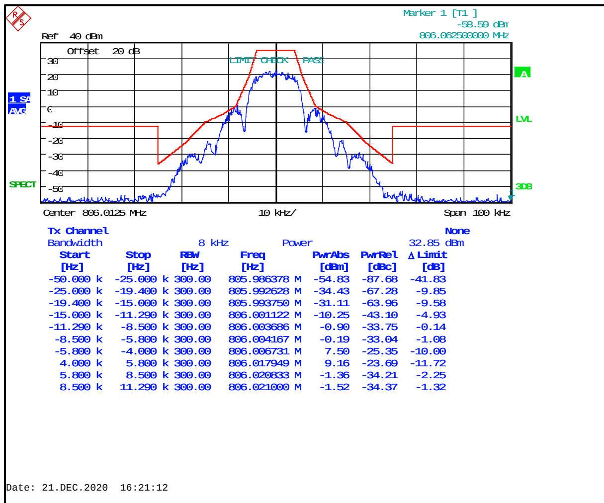
Plot 8-26: Occupied Bandwidth – 806.0125 MHz; WB 2-level FSK 9600; Mask H
