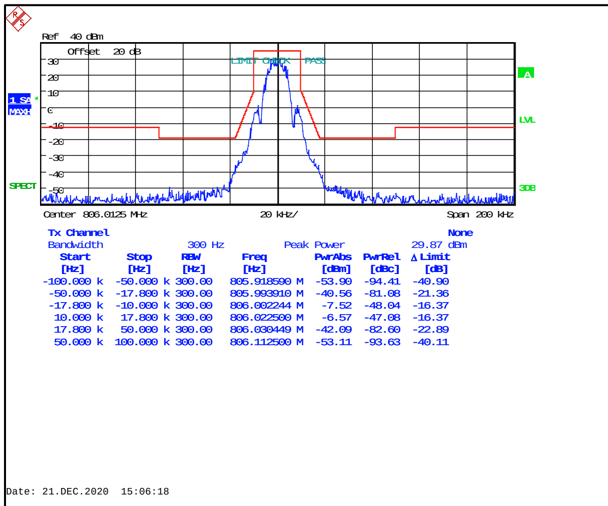
Plot 8-35: Occupied Bandwidth – 806.0125 MHz; NPSPAC 2-level FSK 9600; Mask G (ISED)
