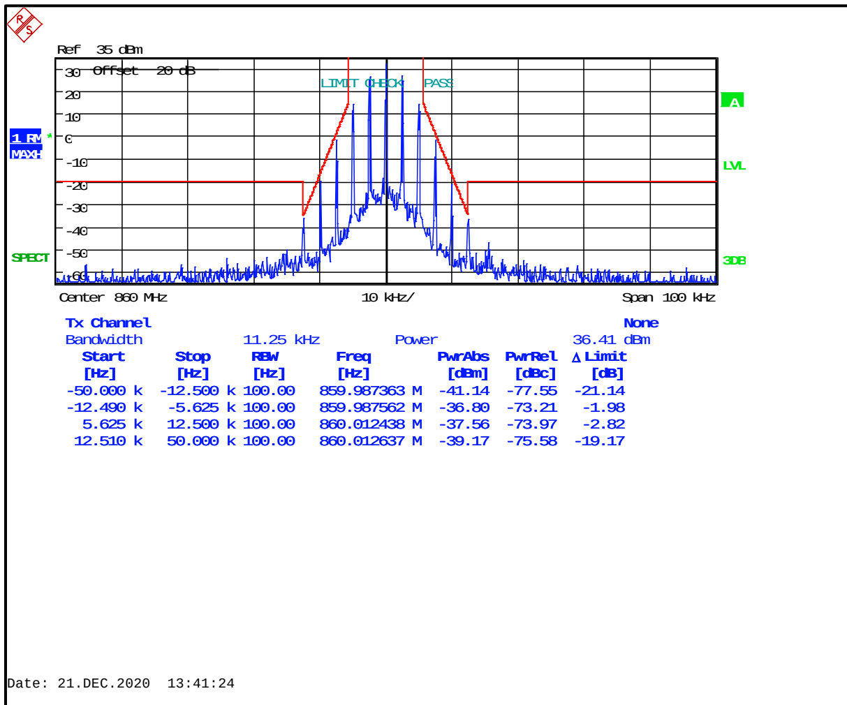
Plot 8-21: Occupied Bandwidth – 860.0000 MHz; NB Analog; Mask D (ISED)
