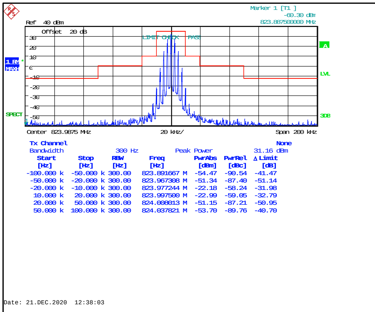
Plot 8-15: Occupied Bandwidth – 823.9875 MHz; NB Analog; Mask B
