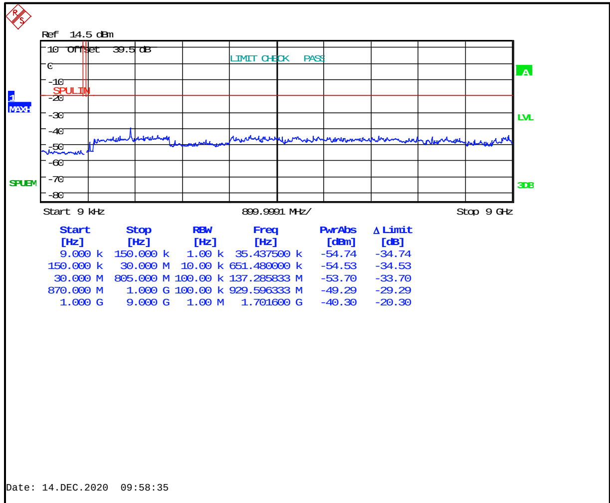
Plot 5-17: Antenna Spurious Emissions - 851.0125 MHz; NB Analog Mode
