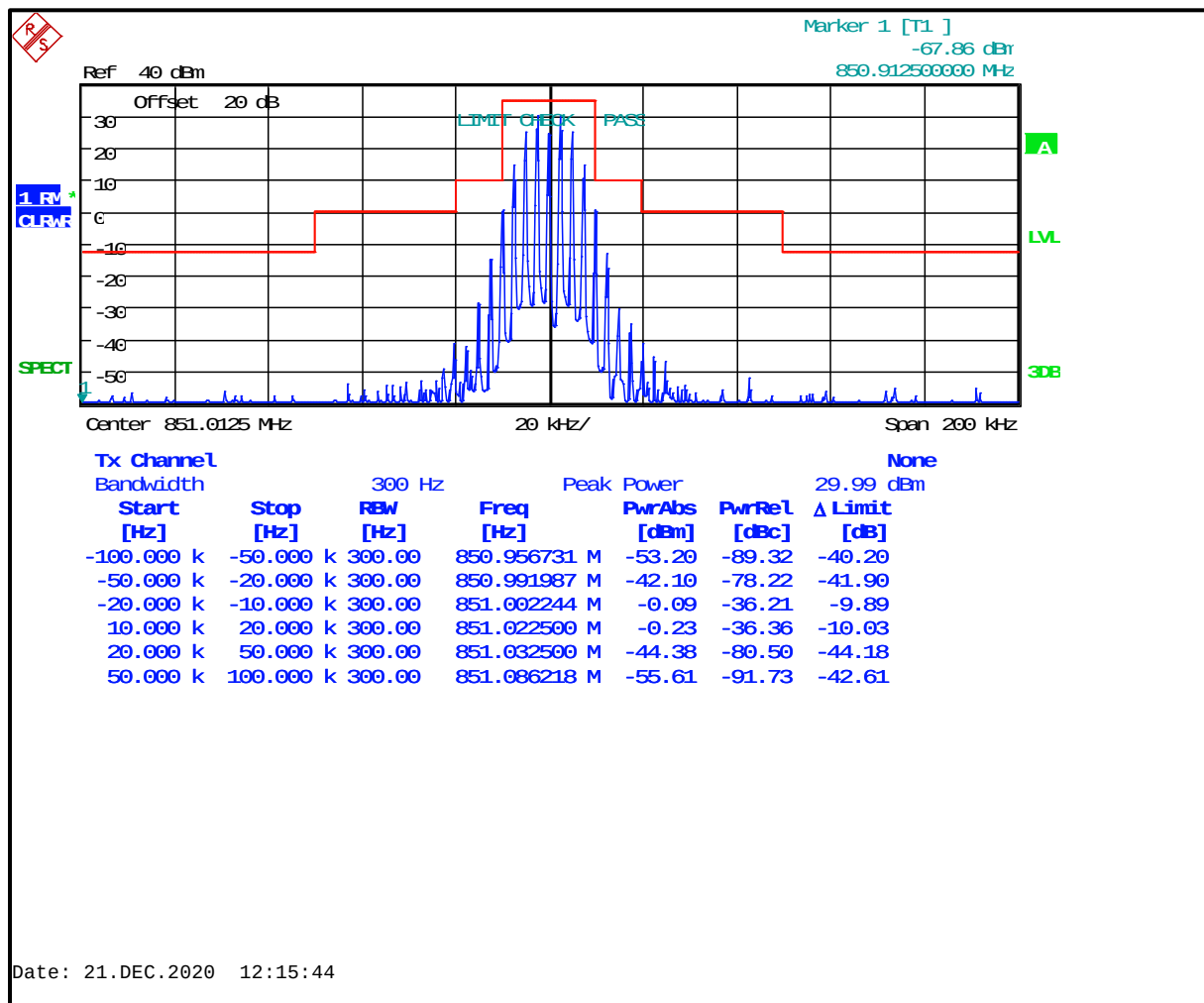
Plot 8-5: Occupied Bandwidth – 851.0125 MHz; WB Analog; Mask B
