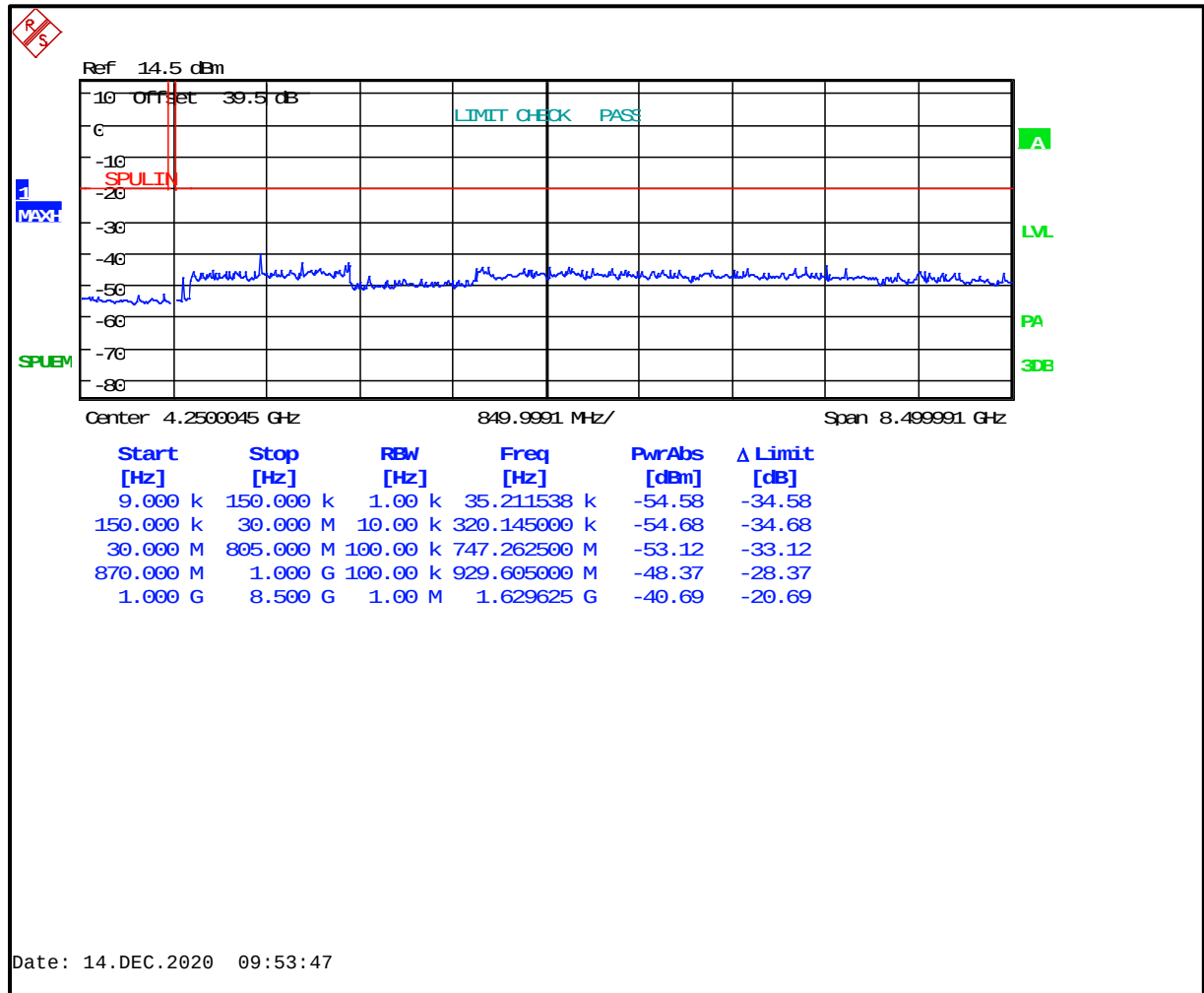
Plot 5-14: Antenna Spurious Emissions - 815.0000 MHz; NB Analog Mode
