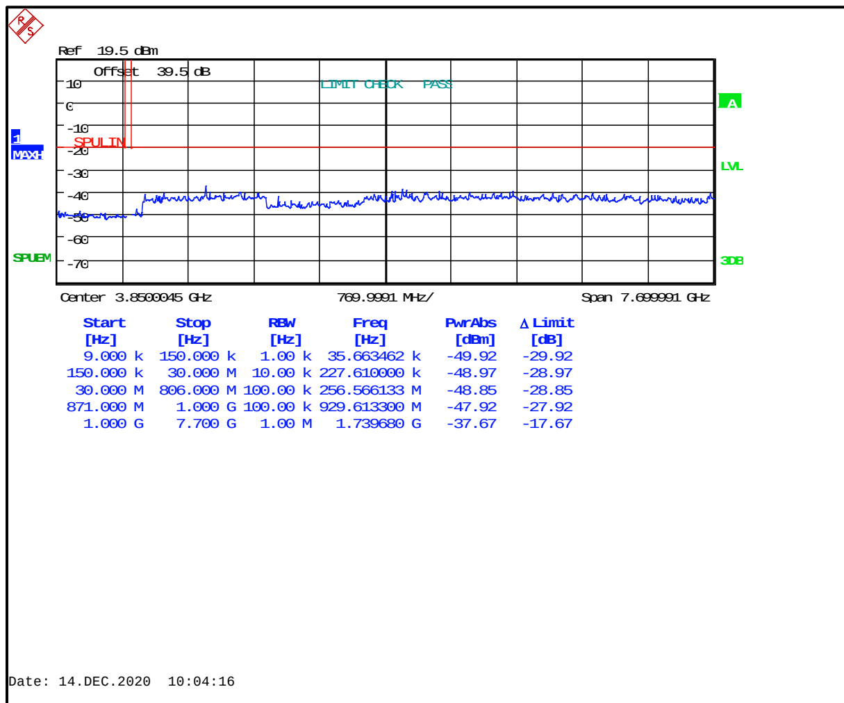
Plot 5-20: Antenna Spurious Emissions - 869.9875 MHz; NB Analog Mode
