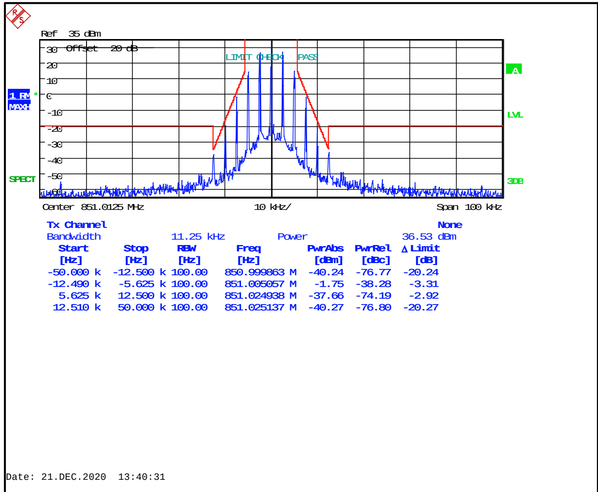
Plot 8-19: Occupied Bandwidth – 851.0125 MHz; NB Analog; Mask D (ISED)
