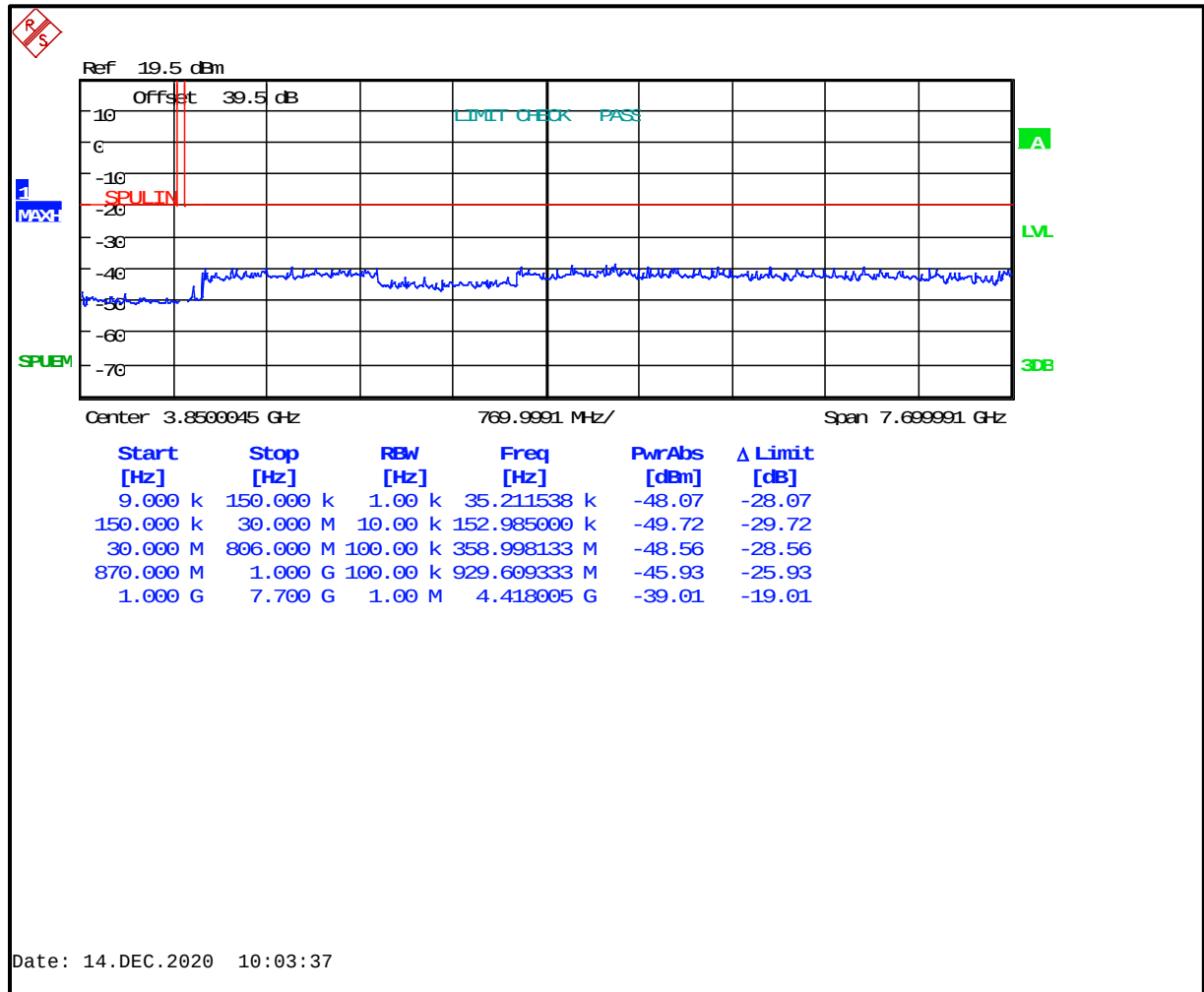
Plot 5-19: Antenna Spurious Emissions - 868.9875 MHz; NB Analog Mode
