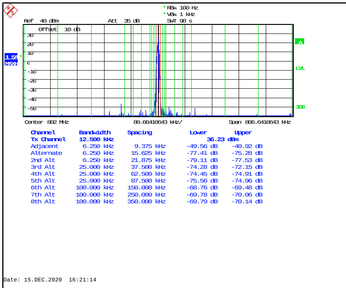
Plot 6-48: Adjacent Channel Power – 802.0000 MHz; H-CPM (TDMA) Mode; (9.375 kHz - 350 kHz)
