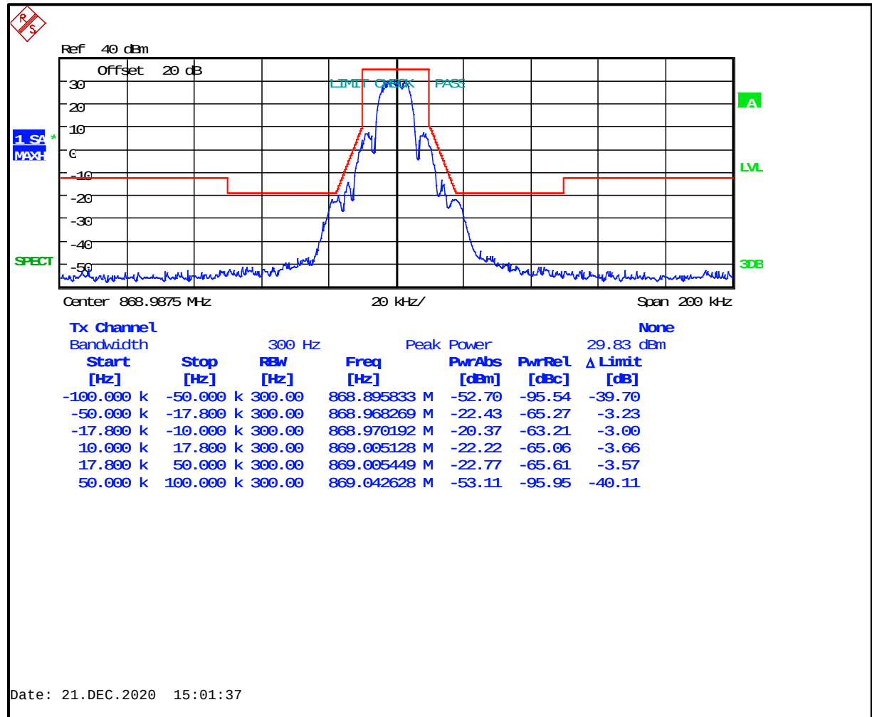
Plot 8-33: Occupied Bandwidth – 868.9875 MHz; WB 2-level FSK 9600; Mask G
