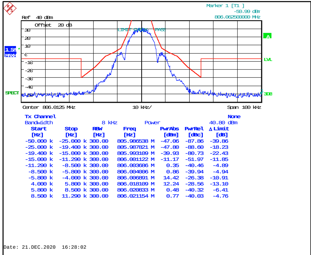
Plot 8-36: Occupied Bandwidth – 806.0125 MHz; NPSPAC 2-level FSK 9600; Mask H
