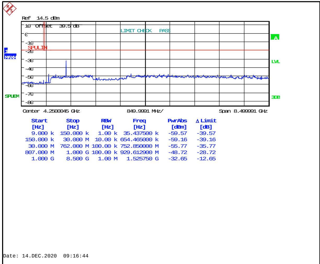
Plot 5-1: Antenna Spurious Emissions - 763.0125 MHz; NB Analog Mode
