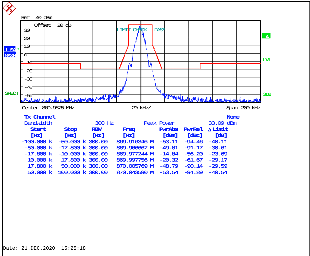
Plot 8-52: Occupied Bandwidth – 869.9875 MHz (EF); NB 2-Level FSK 9600; Mask G
