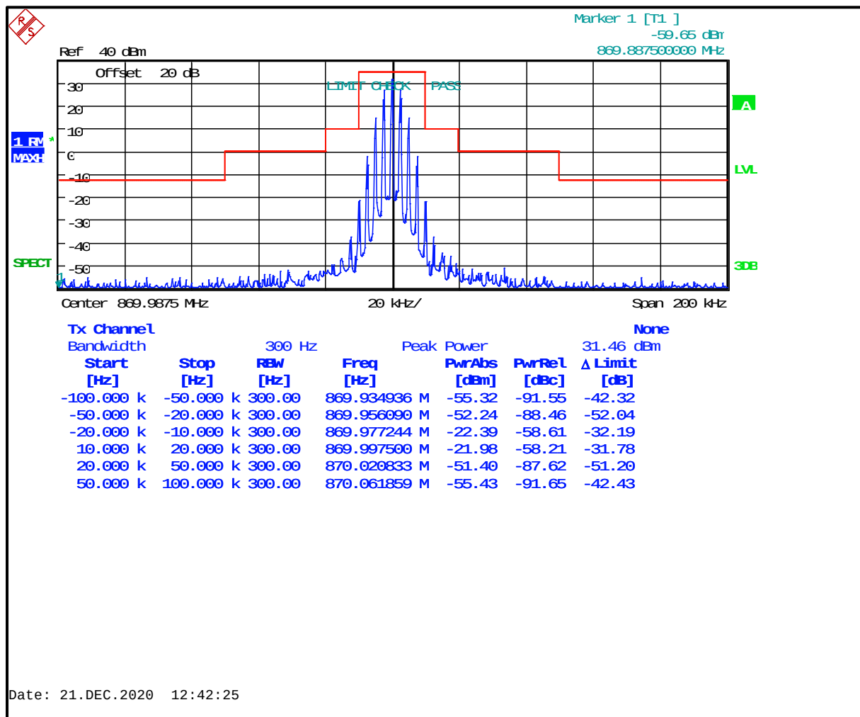
Plot 8-24: Occupied Bandwidth – 869.9875 MHz (EF); NB Analog; Mask B
