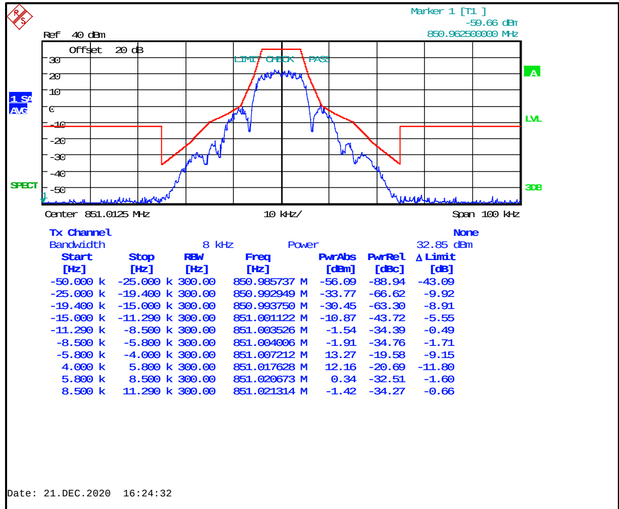
Plot 8-31: Occupied Bandwidth – 851.0125 MHz; WB 2-level FSK 9600; Mask H
