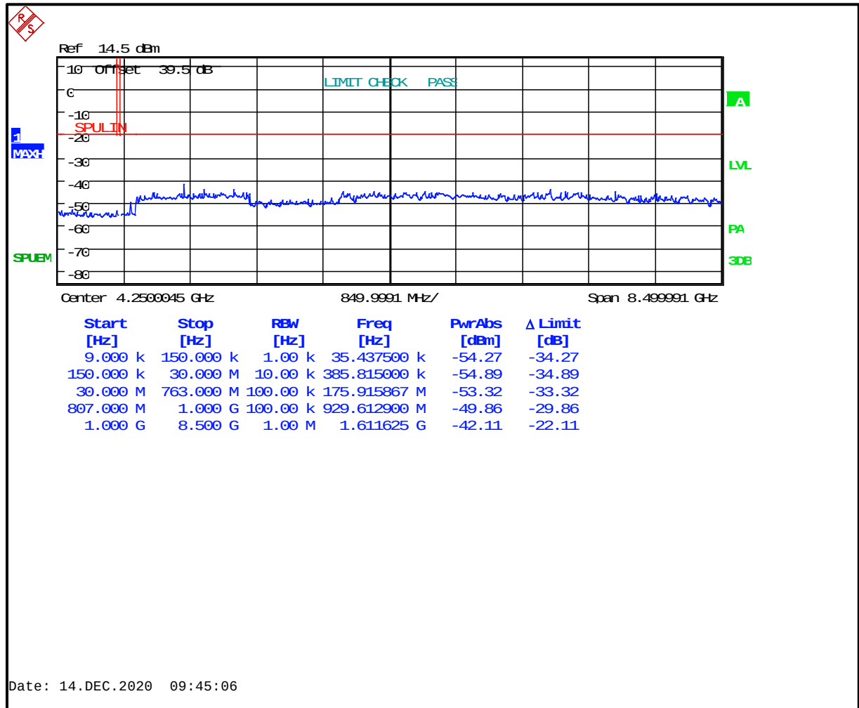
Plot 5-12: Antenna Spurious Emissions - 805.9875 MHz; NB Analog Mode
