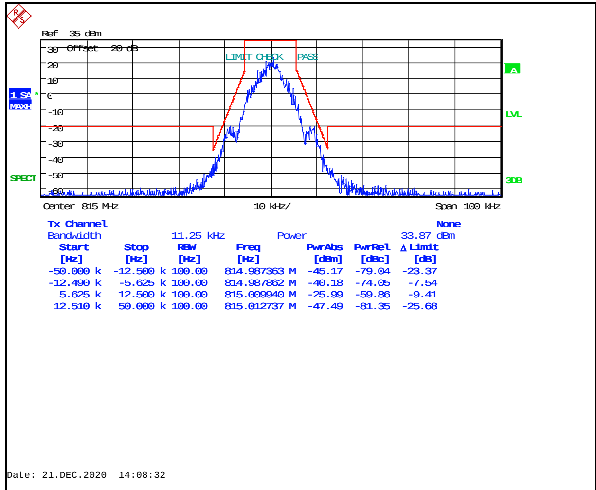
Plot 8-42: Occupied Bandwidth – 815.0000 MHz; NB 2-Level FSK 9600; Mask D (ISED)
