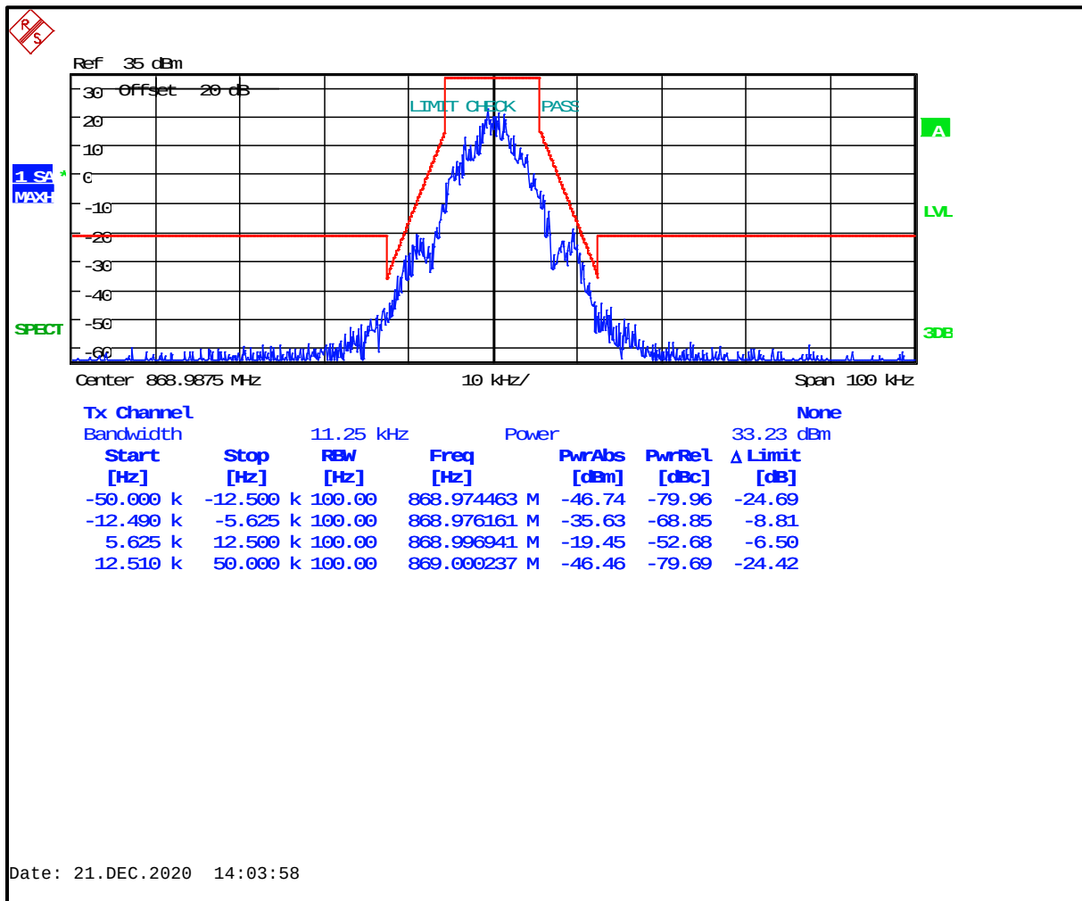
Plot 8-51: Occupied Bandwidth – 868.9875 MHz; NB 2-Level FSK 9600; Mask D (ISED)
