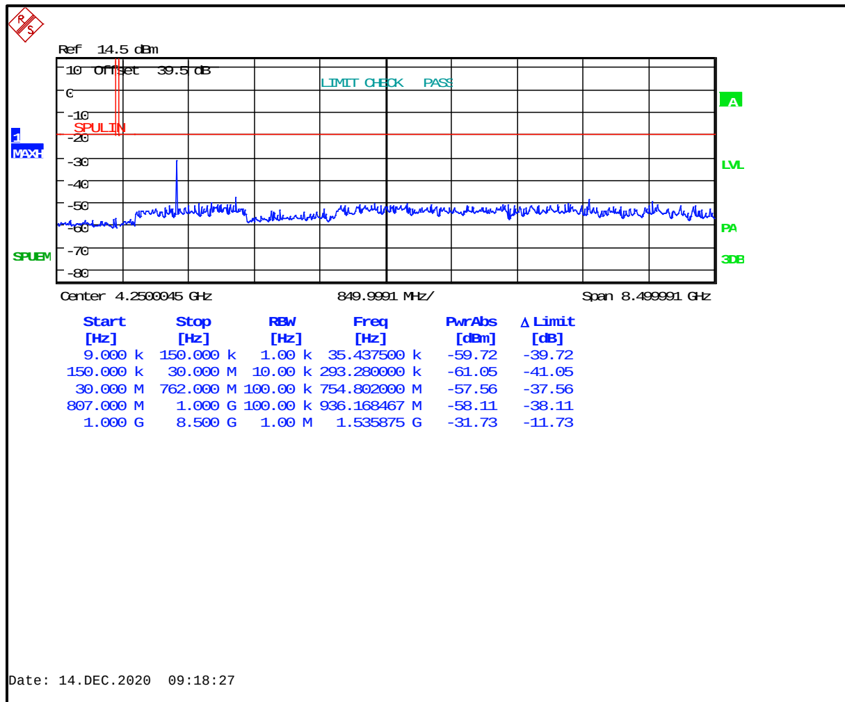
Plot 5-2: Antenna Spurious Emissions - 768.0125 MHz; NB Analog
