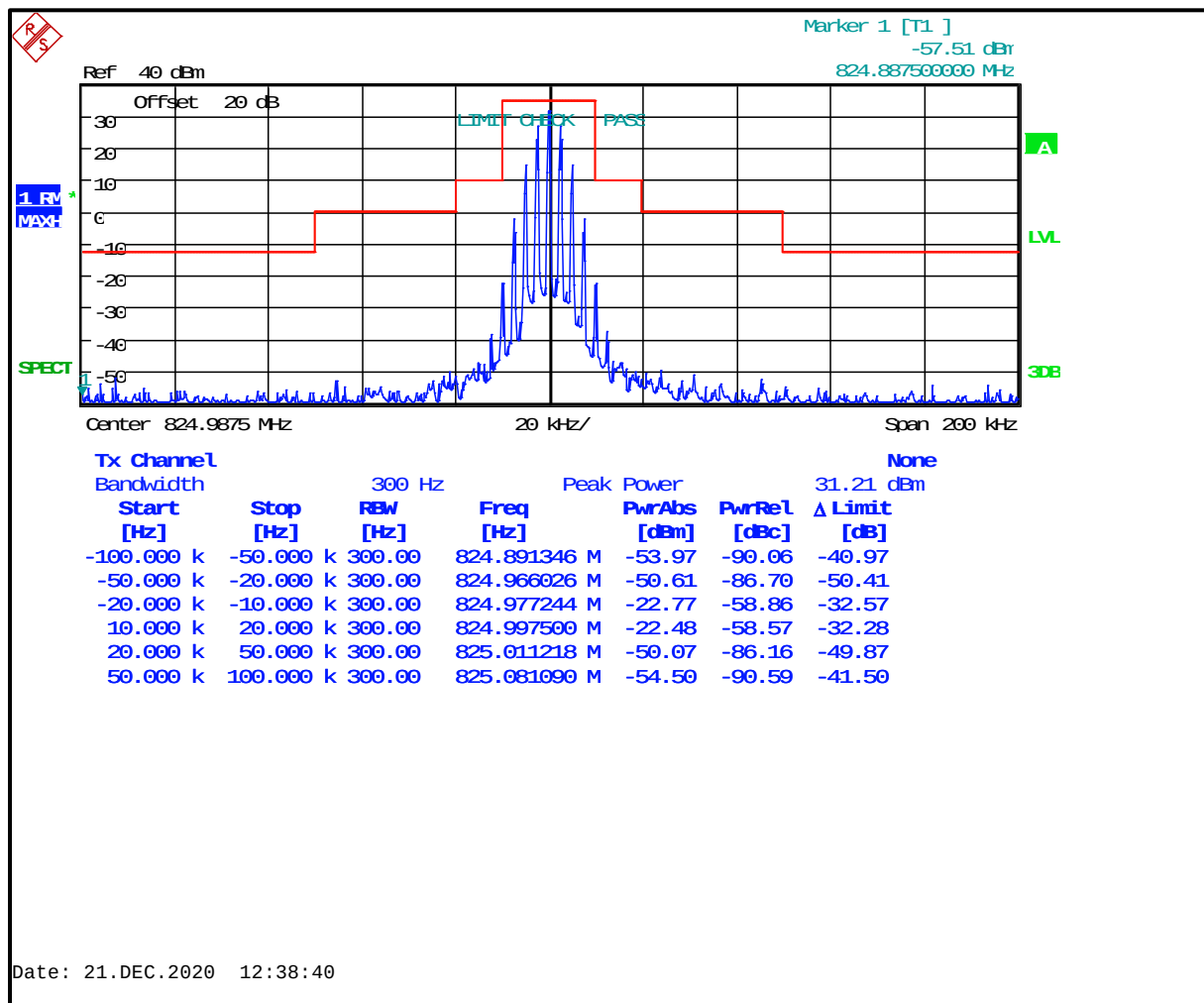
Plot 8-17: Occupied Bandwidth – 824.9875 MHz (EF); NB Analog; Mask B
