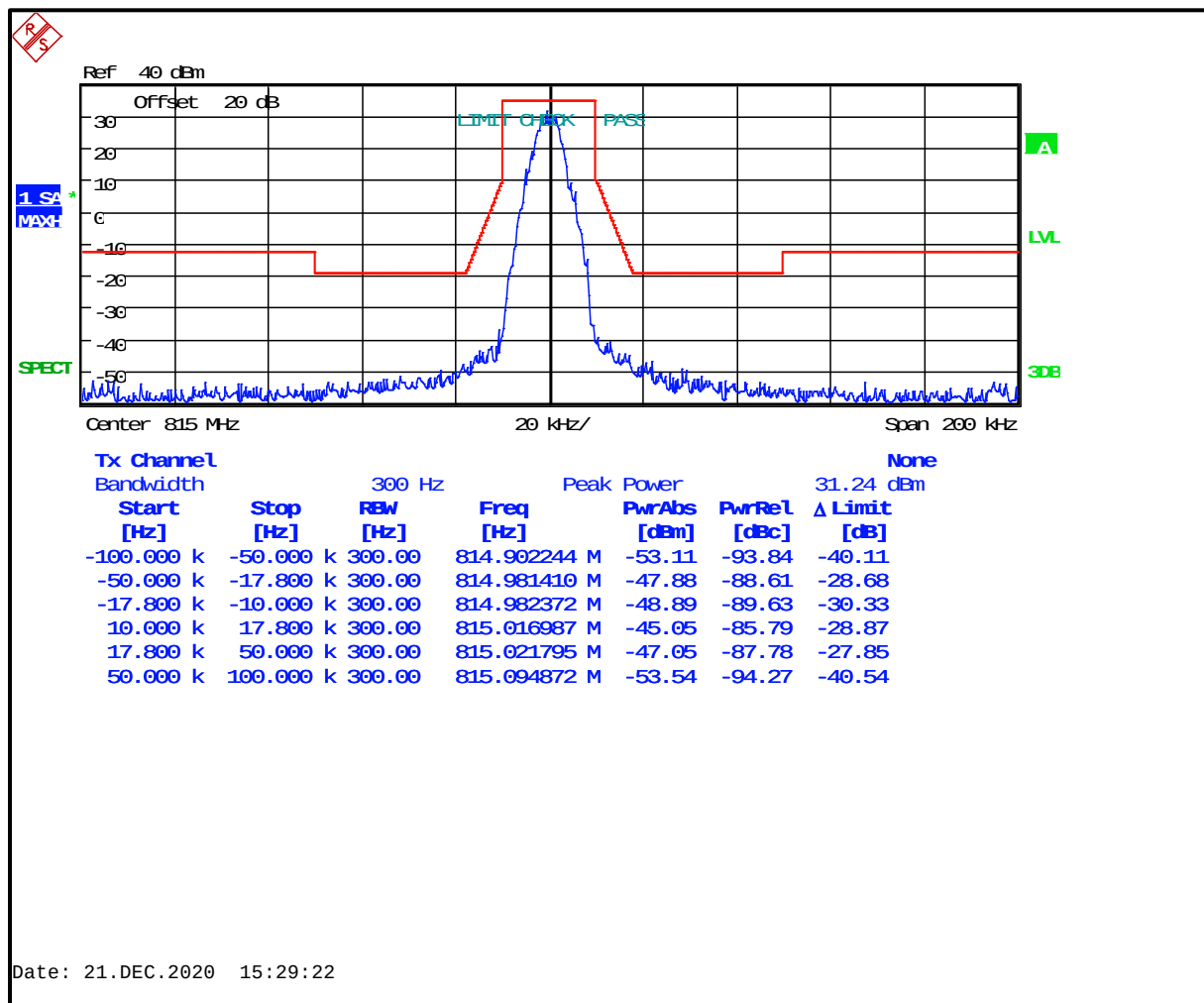
Plot 8-55: Occupied Bandwidth – 815.0000 MHz; C4FM; Mask G
