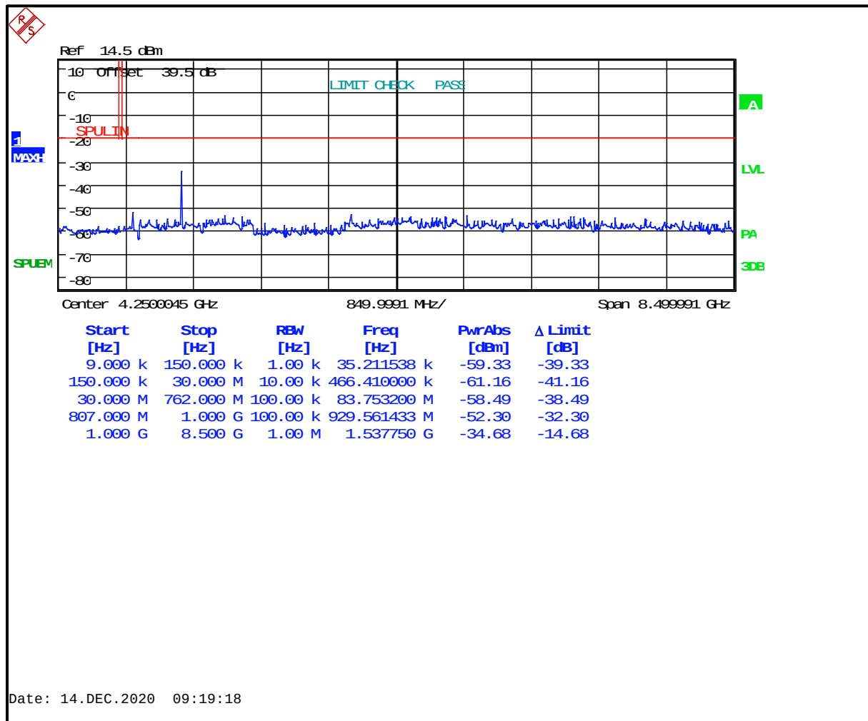
Plot 5-3: Antenna Spurious Emissions - 769.0125 MHz; NB Analog Mode
