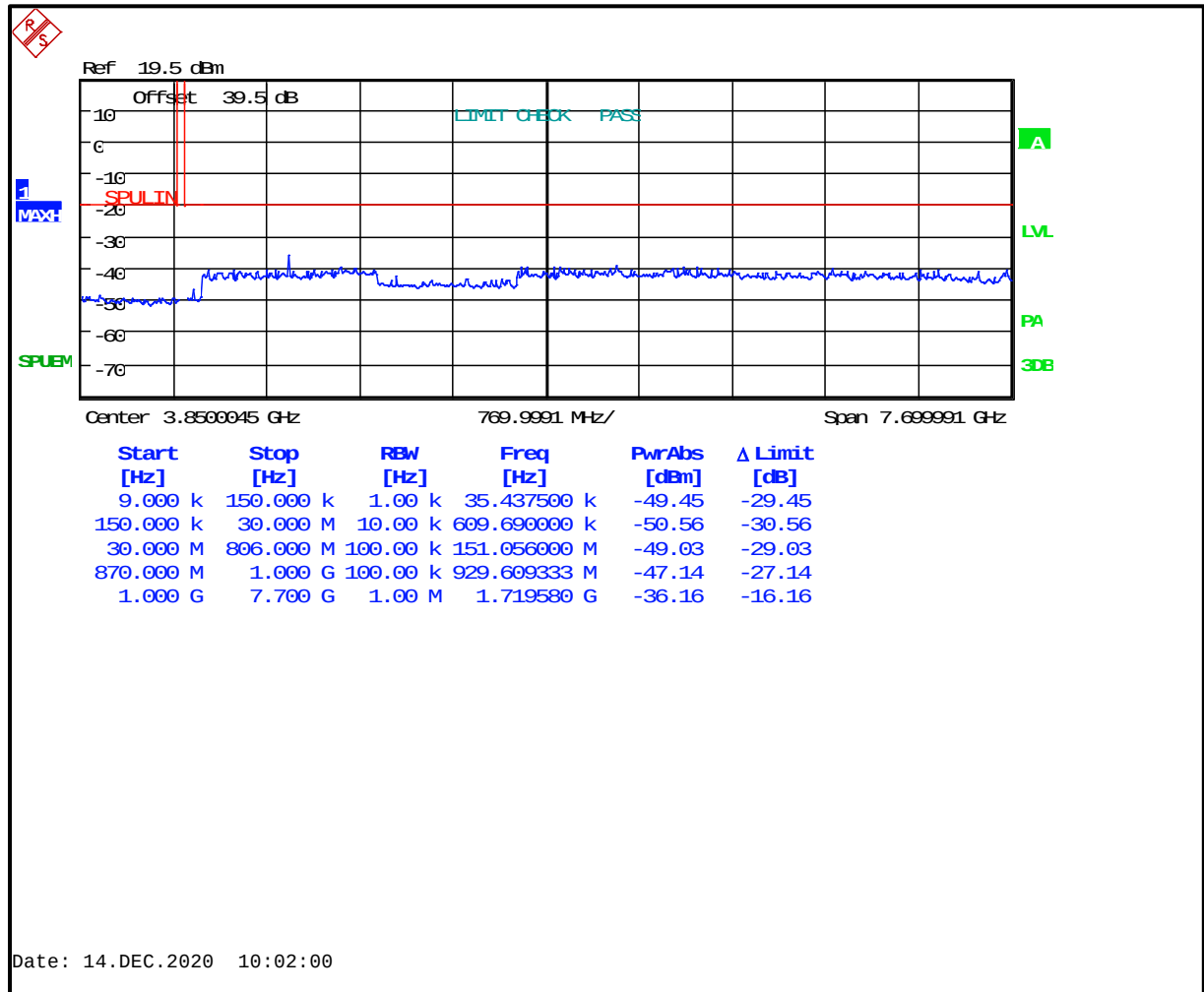
Plot 5-18: Antenna Spurious Emissions - 860.0000 MHz; NB Analog Mode
