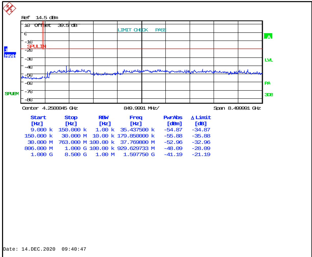
Plot 5-9: Antenna Spurious Emissions - 799.0125 MHz; NB Analog Mode
