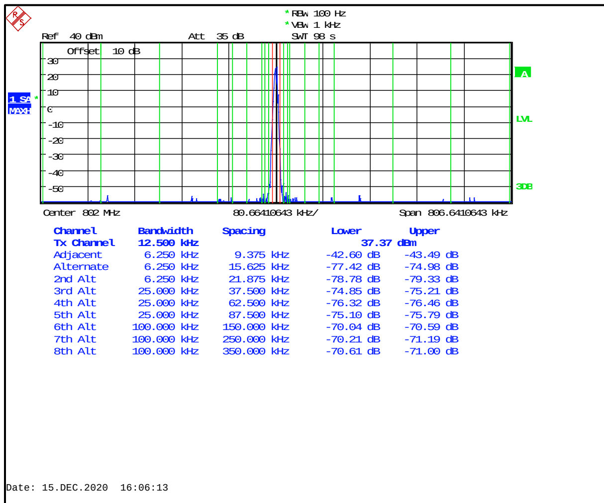
Plot 6-38: Adjacent Channel Power – 802.0000 MHz; C4FM Mode (9.375 kHz - 350 kHz)
