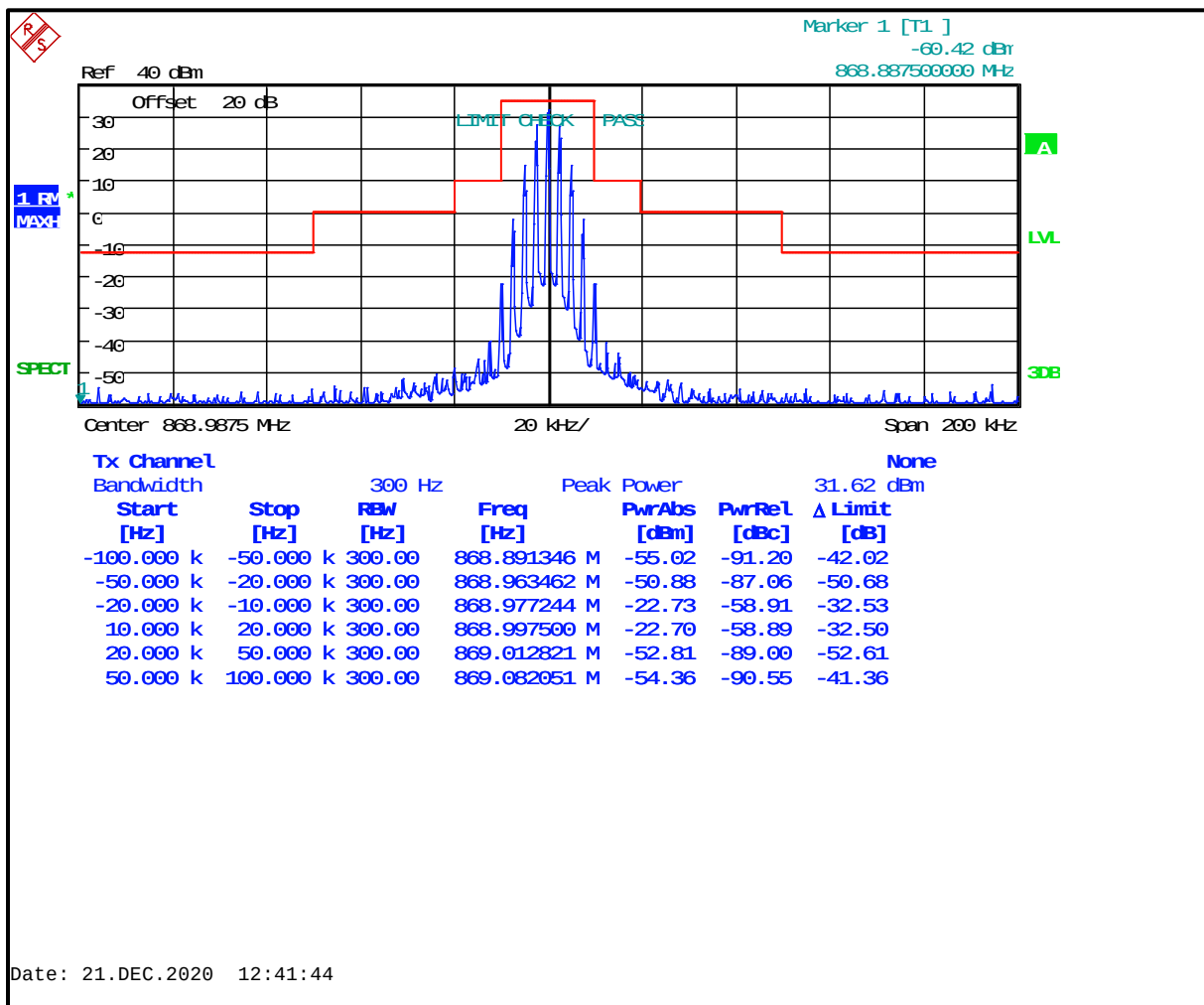
Plot 8-22: Occupied Bandwidth – 868.9875 MHz; NB Analog; Mask B
