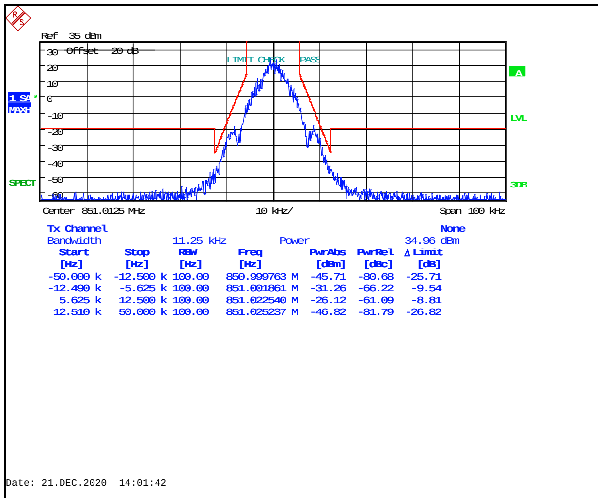
Plot 8-47: Occupied Bandwidth – 851.0125 MHz; NB 2-Level FSK 9600; Mask D (ISED)
