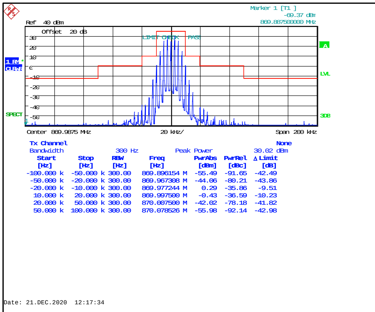
Plot 8-8: Occupied Bandwidth – 869.9875 MHz (EF); WB Analog; Mask B
