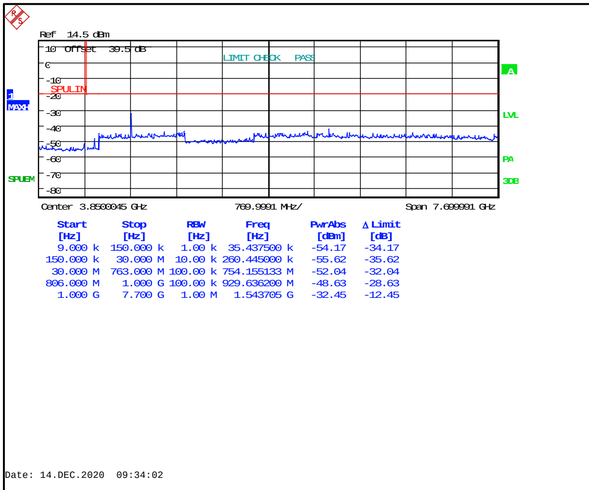
Plot 5-4: Antenna Spurious Emissions - 772.0000 MHz; NB Analog Mode
