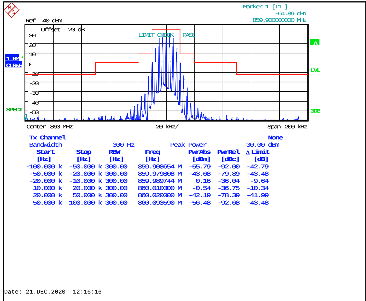
Plot 8-6: Occupied Bandwidth – 860.0000 MHz; WB Analog; Mask B
