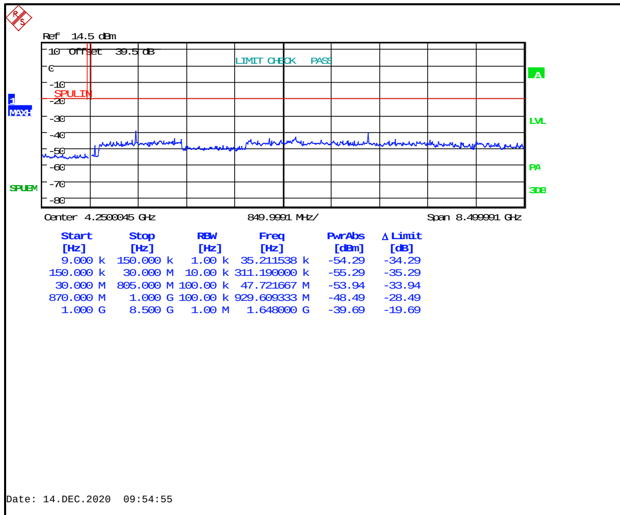
Plot 5-15: Antenna Spurious Emissions - 823.9875 MHz; NB Analog
