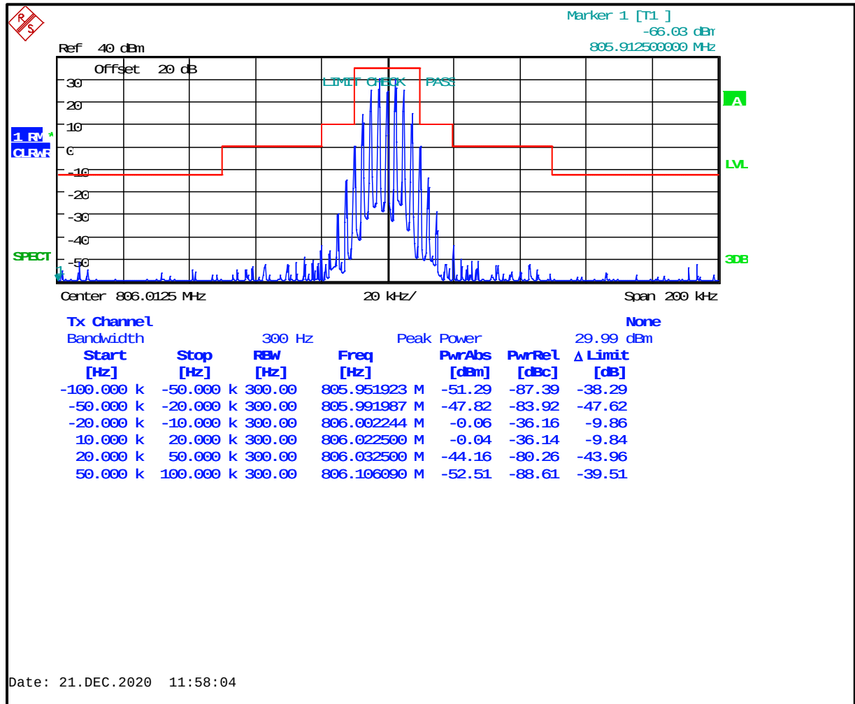
Plot 8-9: Occupied Bandwidth – 806.0125 MHz; NPSPAC Analog; Mask B
