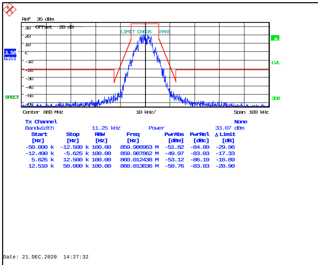
Plot 8-63: Occupied Bandwidth – 860.0000 MHz; C4FM; Mask D (ISED)
