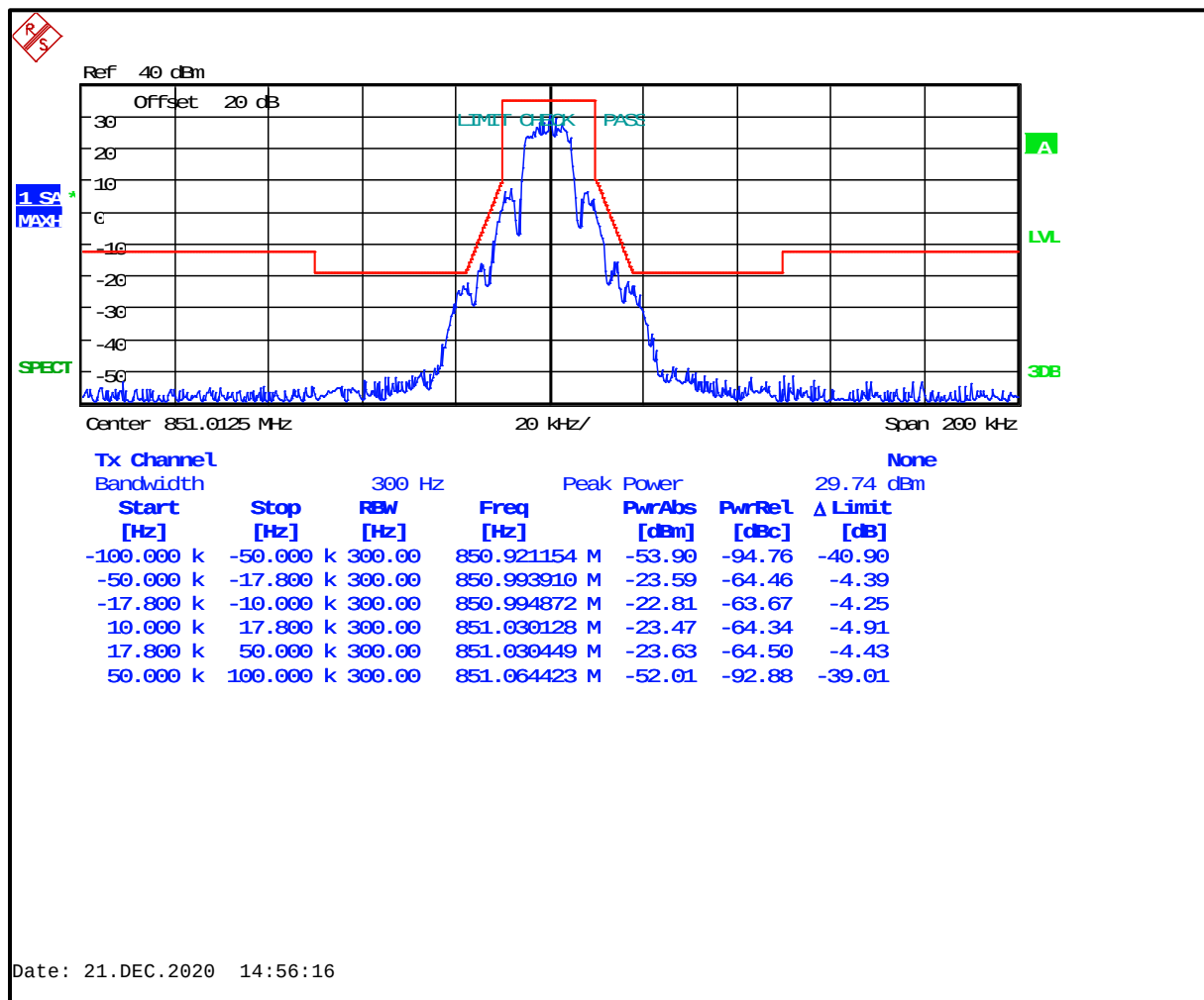
Plot 8-30: Occupied Bandwidth – 851.0125 MHz; WB 2-level FSK 9600; Mask G (ISED)
