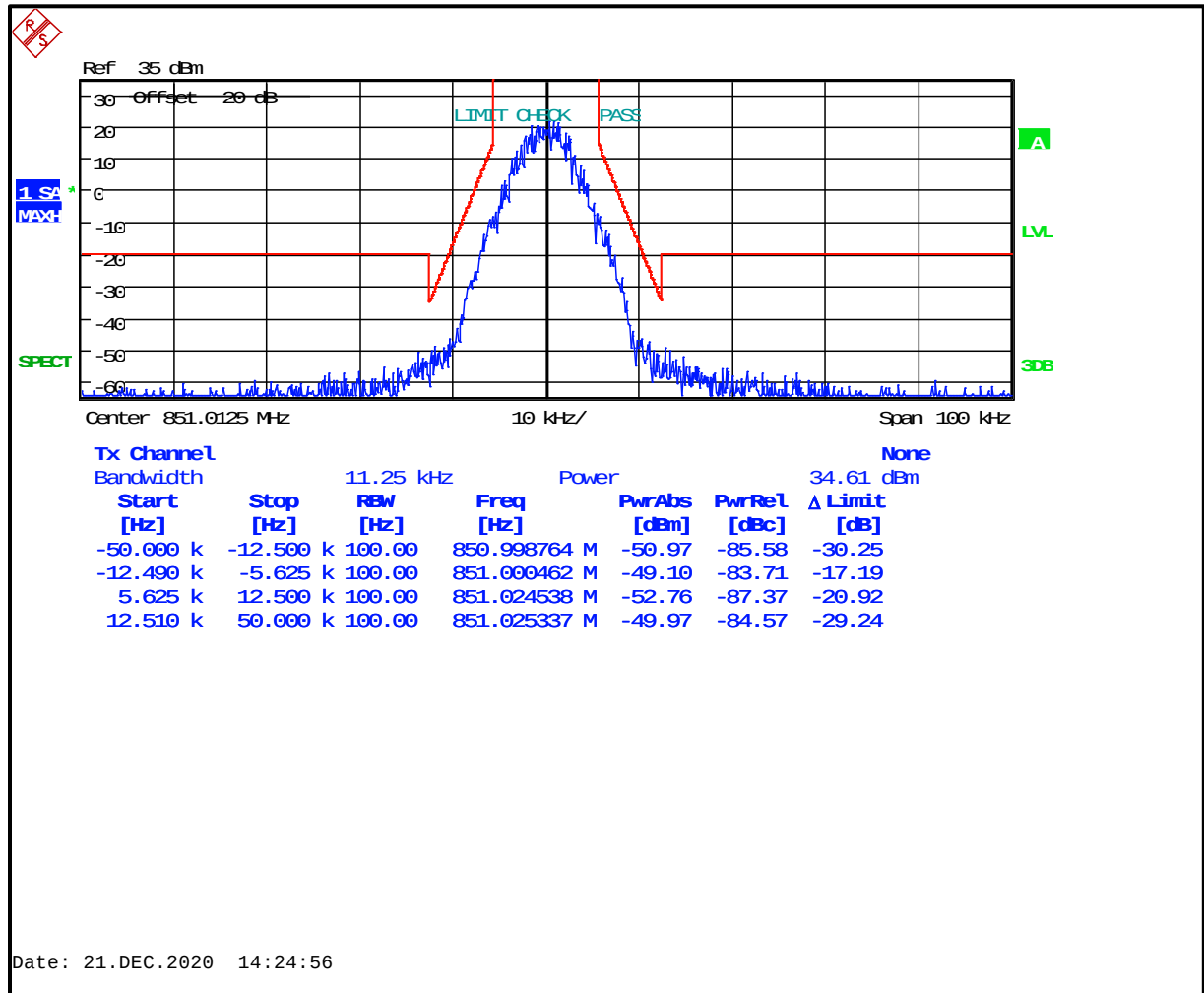
Plot 8-61: Occupied Bandwidth – 851.0125 MHz; C4FM; Mask D (ISED)
