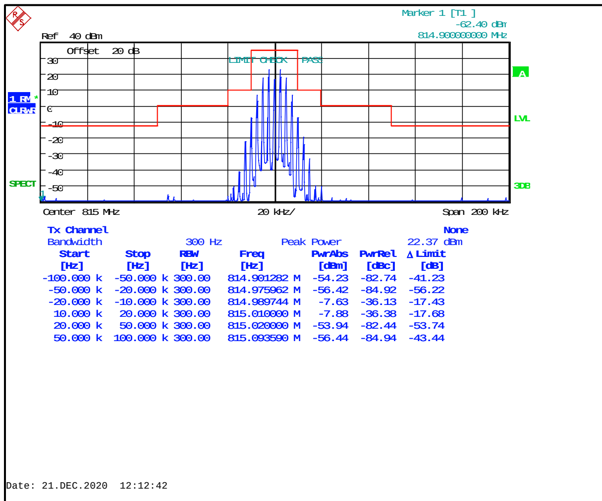
Plot 8-2: Occupied Bandwidth – 815.0000 MHz; WB Analog; Mask B
