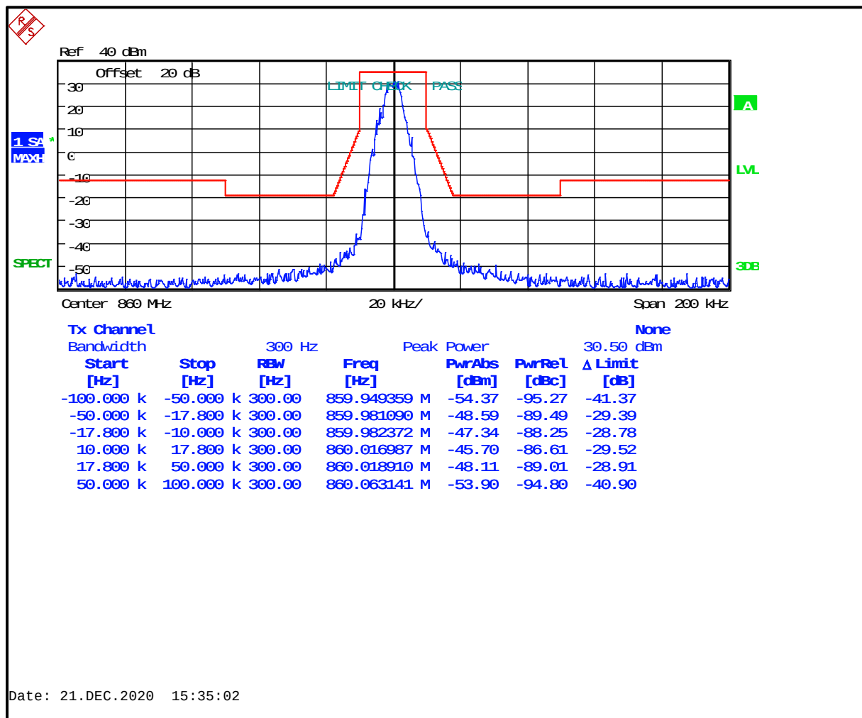
Plot 8-62: Occupied Bandwidth – 860.0000 MHz; C4FM; Mask G
