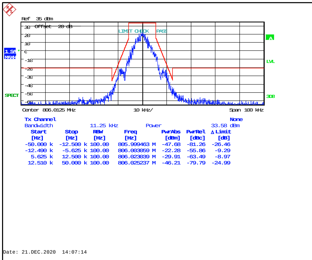
Plot 8-40: Occupied Bandwidth – 806.0125 MHz; NB 2-Level FSK 9600; Mask D (ISED)
