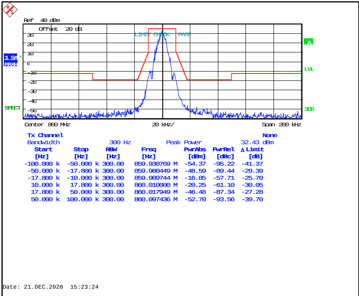
Plot 8-48: Occupied Bandwidth – 860.0000 MHz; NB 2-Level FSK 9600; Mask G
