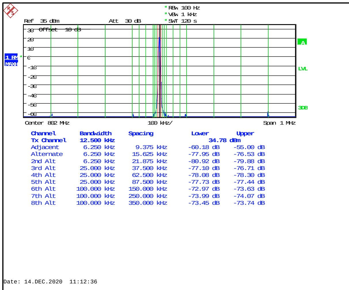
Plot 6-8: Adjacent Channel Power – 802.0000 MHz; NB Analog Mode; (9.375 kHz - 350 kHz)
