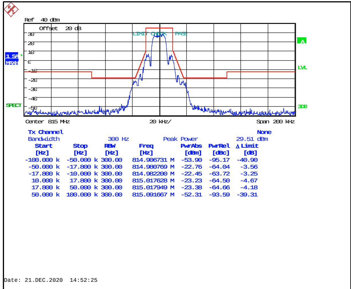
Plot 8-27: Occupied Bandwidth – 815.0000 MHz; WB 2-level FSK 9600; Mask G
