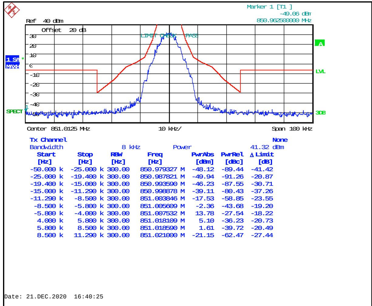
Plot 8-60: Occupied Bandwidth – 851.0125 MHz; C4FM; Mask H
