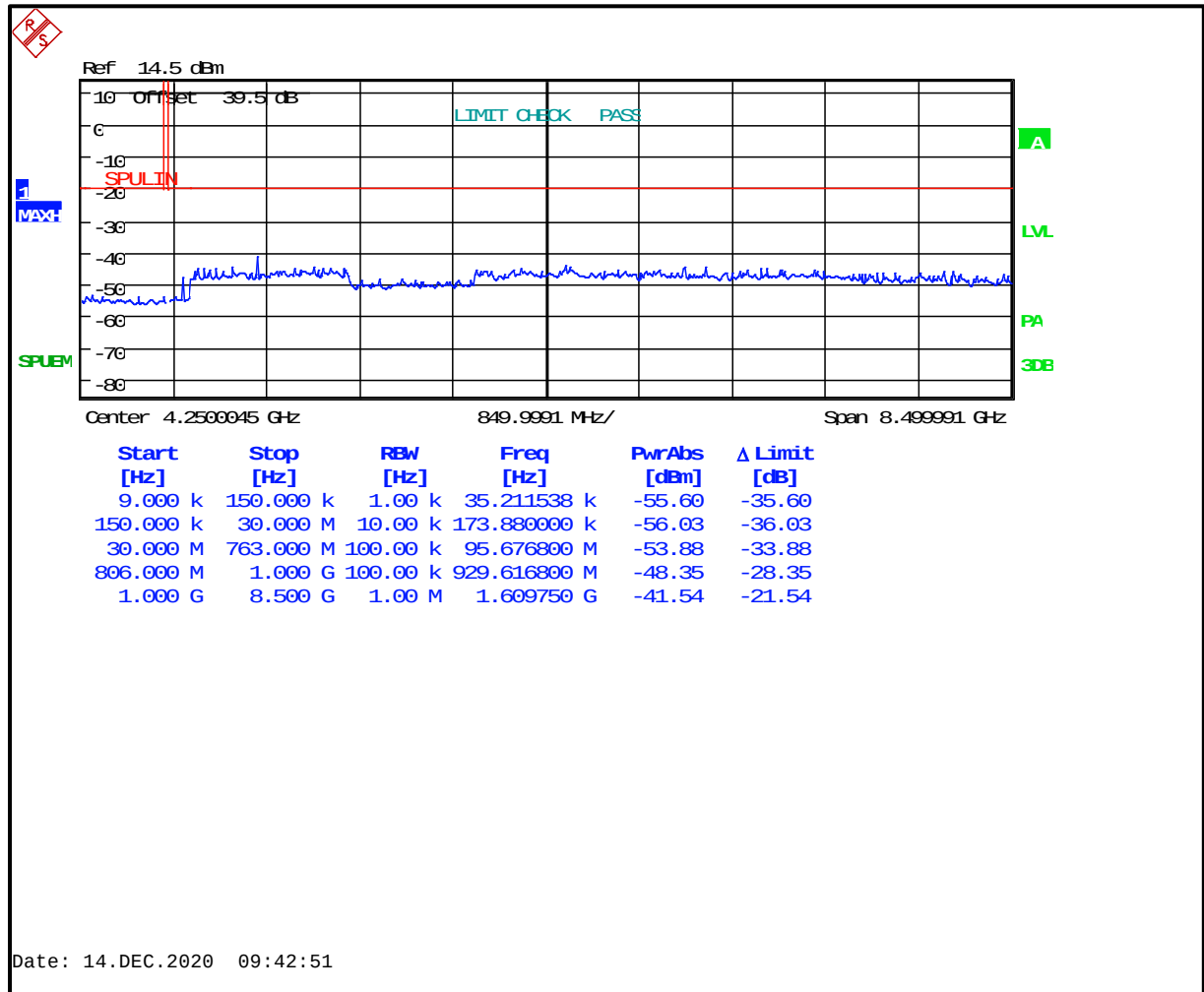
Plot 5-11: Antenna Spurious Emissions - 804.9875 MHz; NB Analog Mode
