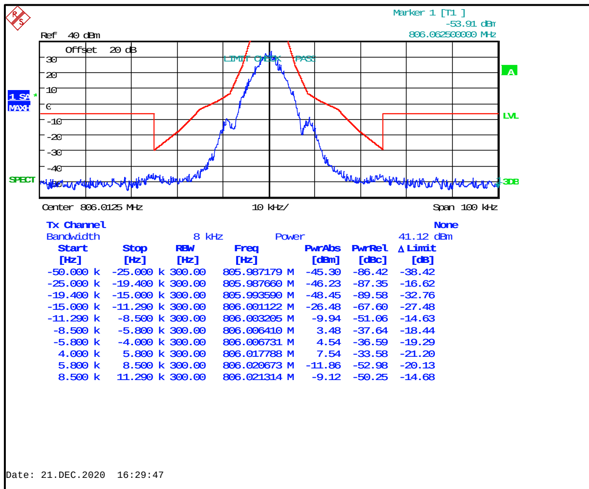
Plot 8-39: Occupied Bandwidth – 806.0125 MHz; NB 2-Level FSK 9600; Mask H
