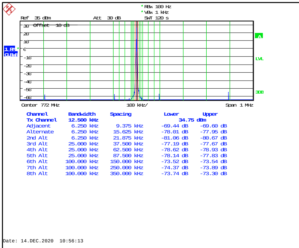
Plot 6-3: Adjacent Channel Power – 772.0000 MHz; NB Analog Mode (9.375 kHz - 350 kHz)
