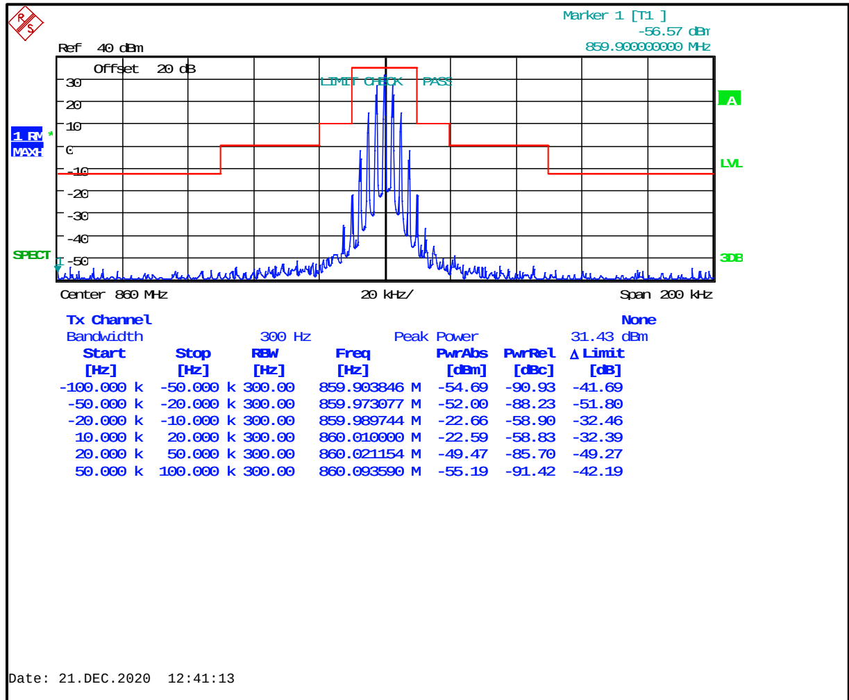
Plot 8-20: Occupied Bandwidth – 860.0000 MHz; NB Analog; Mask B
