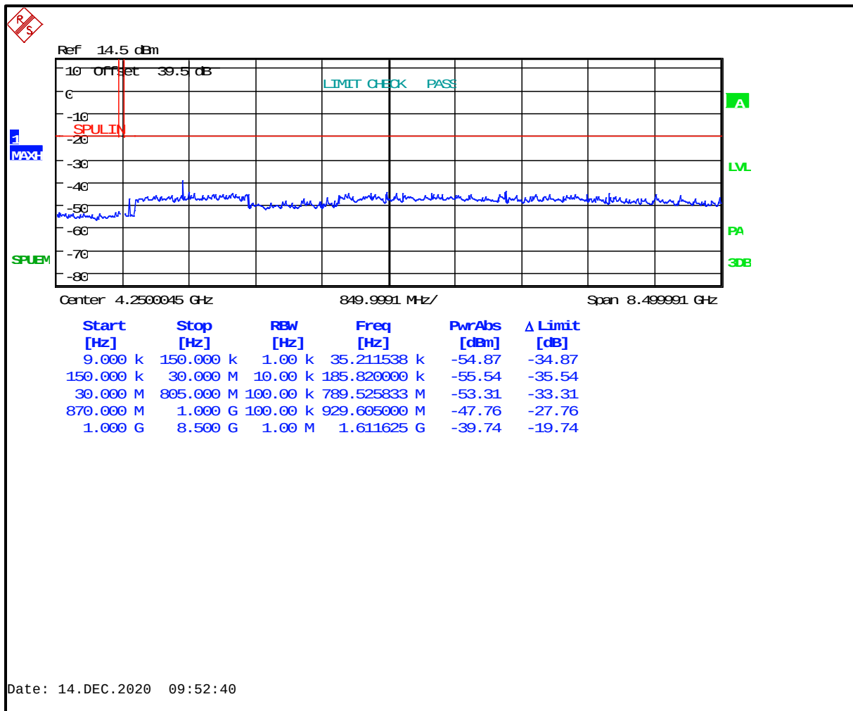
Plot 5-13: Antenna Spurious Emissions - 806.0125 MHz; NB Analog Mode
