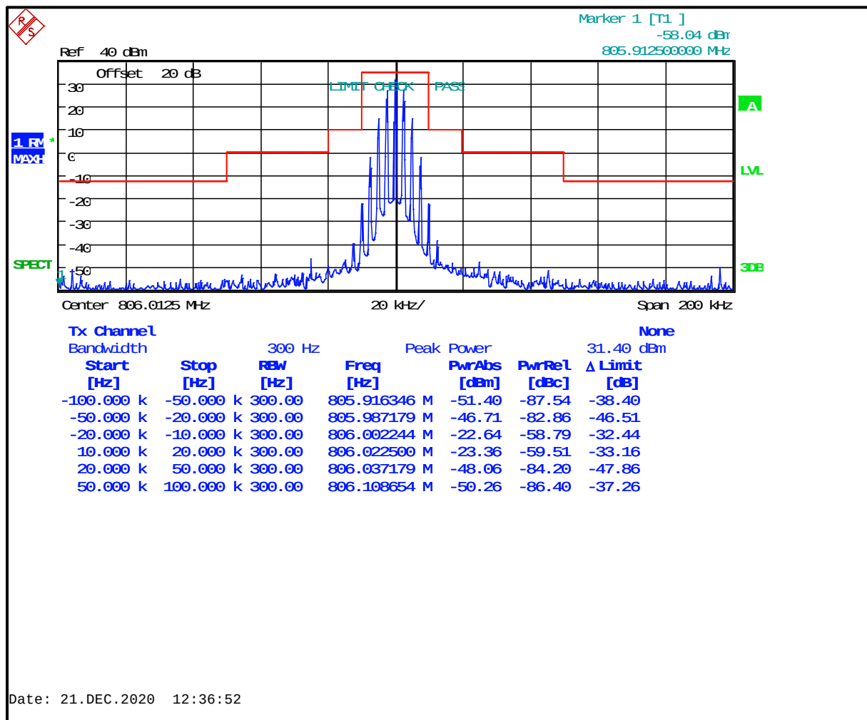
Plot 8-11: Occupied Bandwidth – 806.0125 MHz; NB Analog; Mask B
