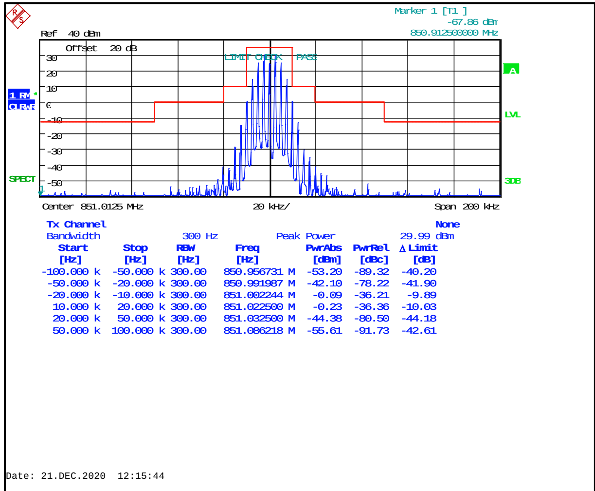
Plot 8-10: Occupied Bandwidth – 851.0125 MHz; NPSPAC Analog; Mask B
