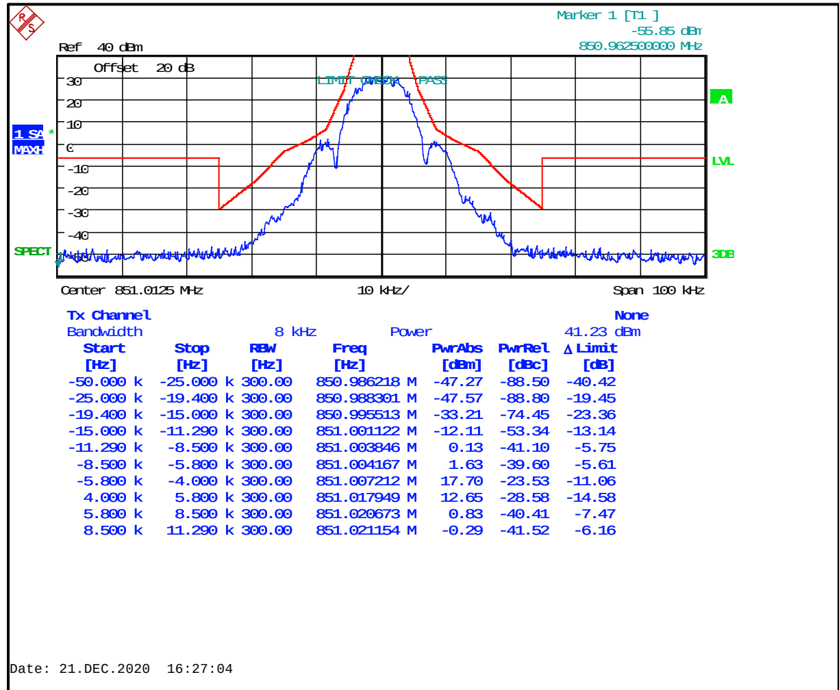
Plot 8-38: Occupied Bandwidth – 851.0125 MHz; NPSPAC 2-level FSK 9600; Mask H
