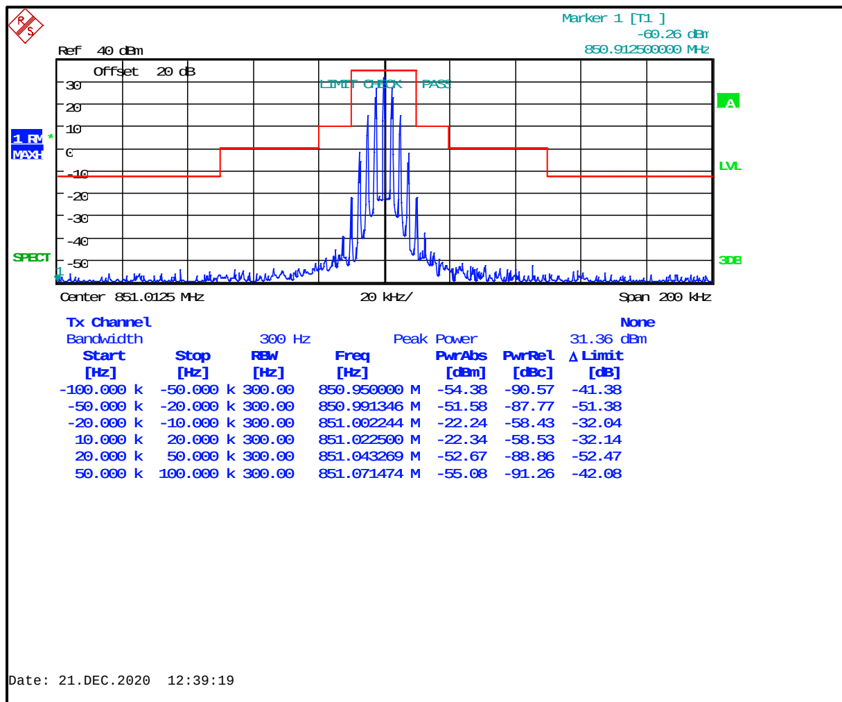
Plot 8-18: Occupied Bandwidth – 851.0125 MHz; NB Analog; Mask B
