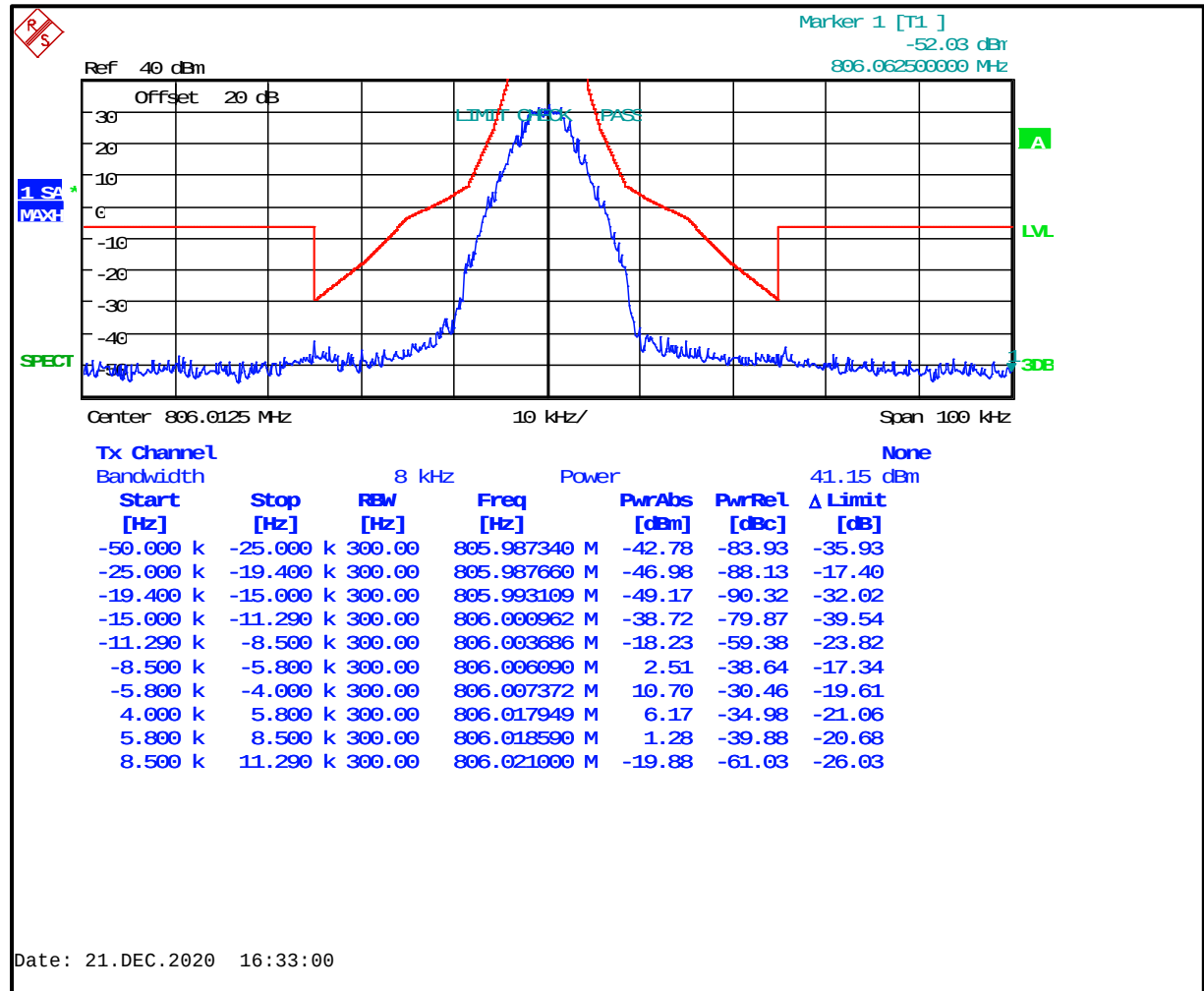
Plot 8-53: Occupied Bandwidth – 806.0125 MHz; C4FM; Mask H
