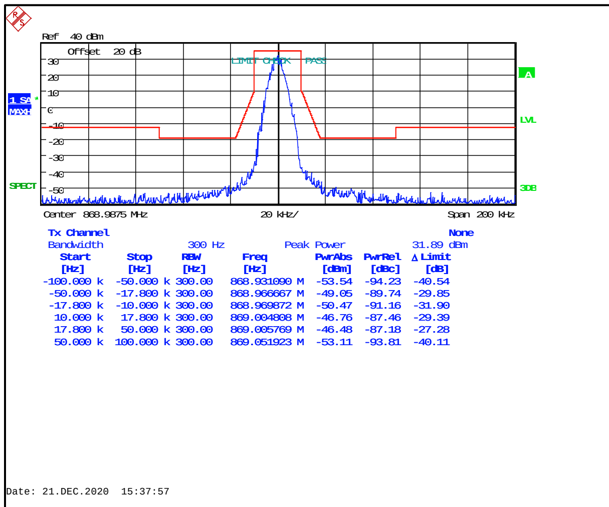
Plot 8-64: Occupied Bandwidth – 868.9875 MHz; C4FM; Mask G
