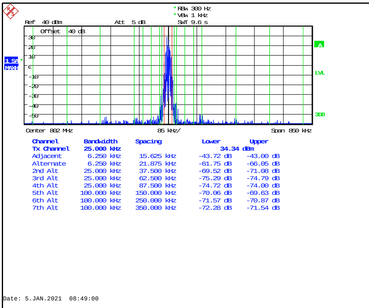
Plot 6-68: Adjacent Channel Power – 802.0000 MHz; HVD-SMR Mode; (9.375 kHz - 350 kHz)
