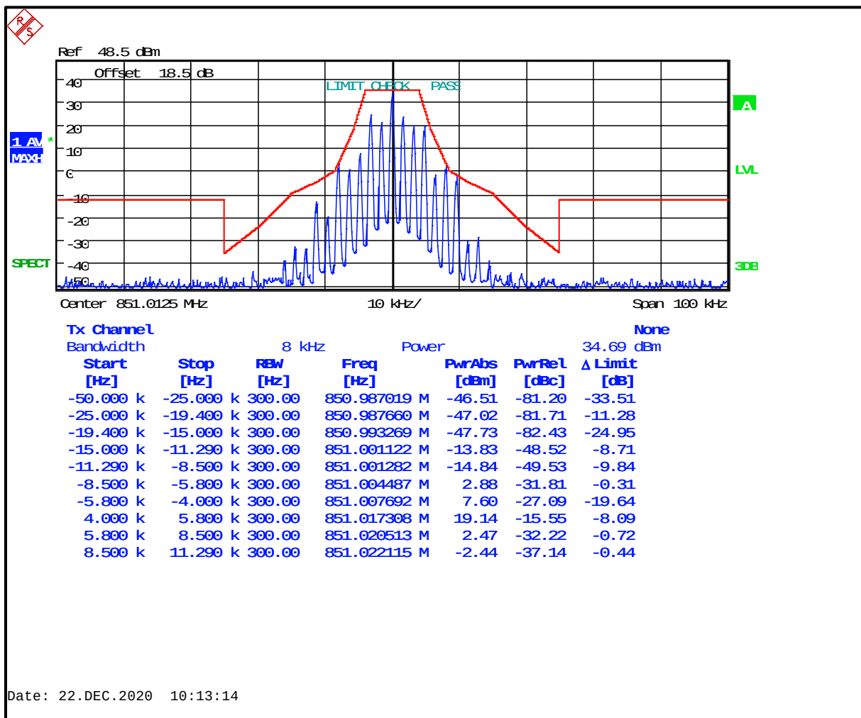
Plot 8-91: Occupied Bandwidth – 851.0125 MHz; HVD NPSPAC; Mask H
