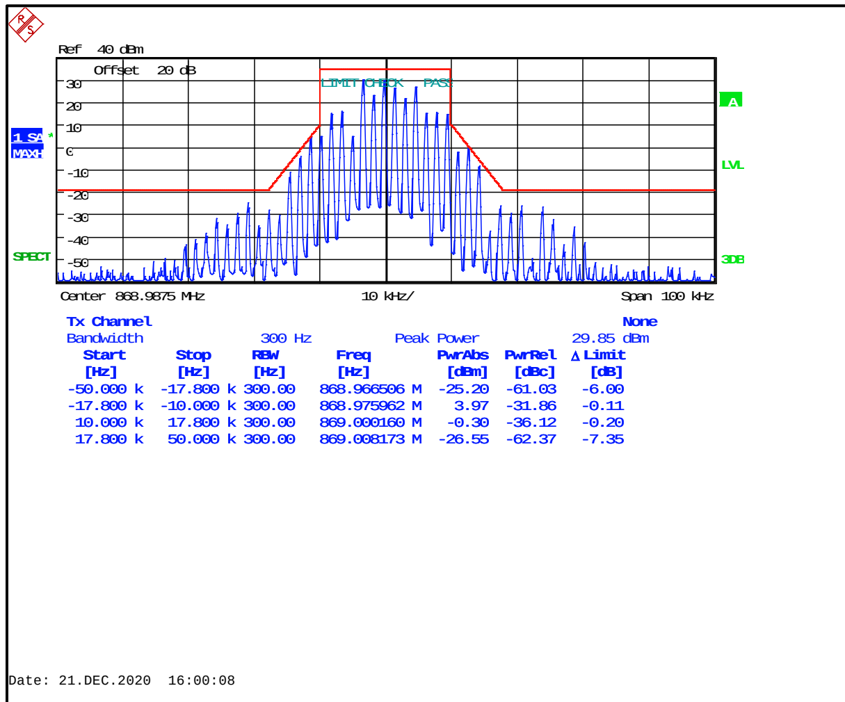
Plot 8-87: Occupied Bandwidth – 868.9875 MHz; HVD SMR; Mask G
