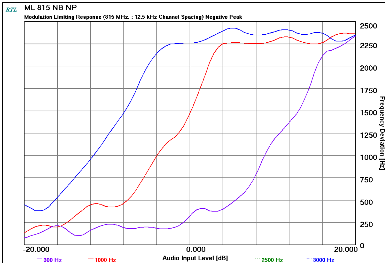
Plot 10-12: Modulation Characteristics – Modulation Limiting – 815.0000 MHz; (NB); Negative Peak
