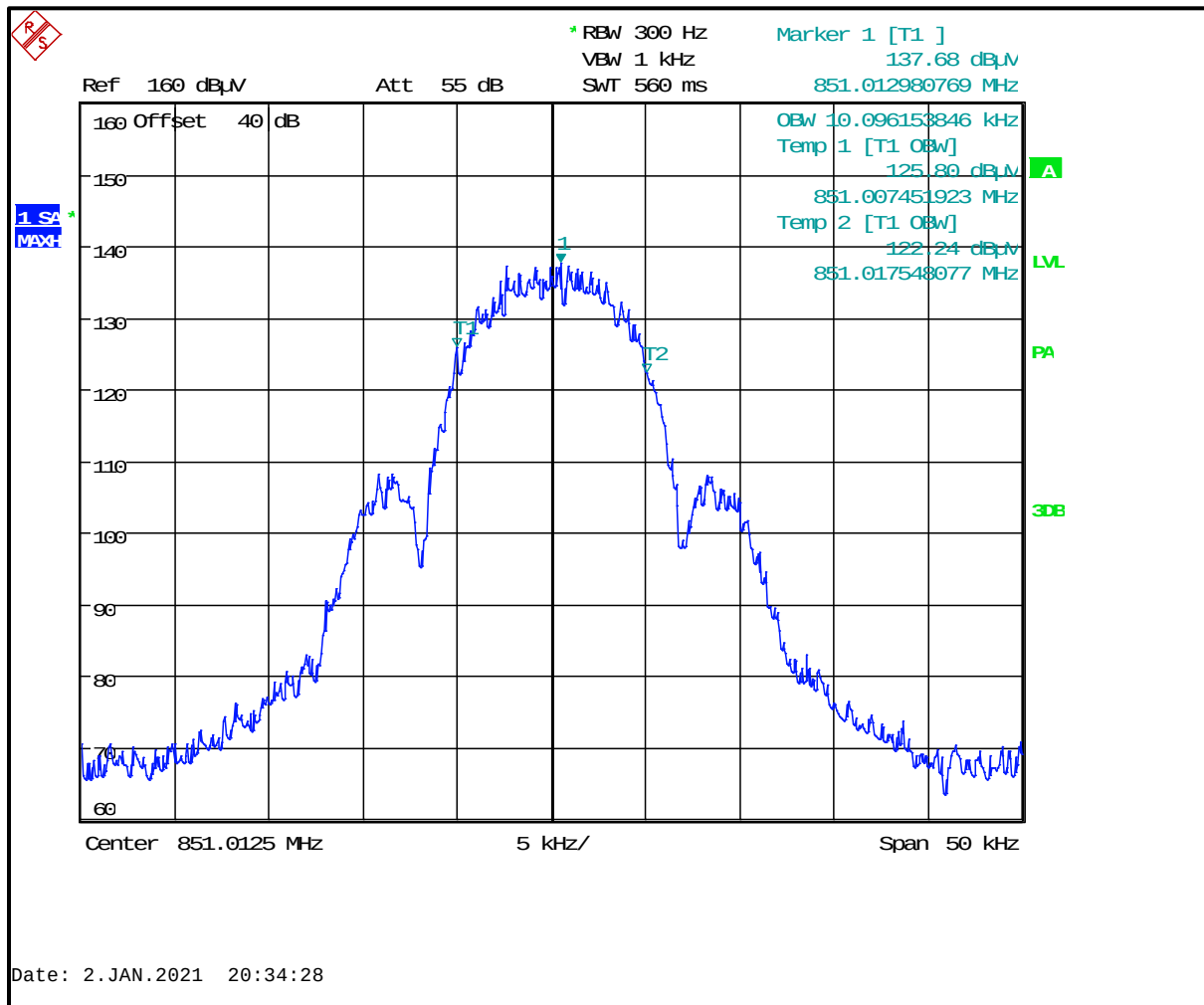
Plot 8-216: 99% Occupied Bandwidth – 851.0125 MHz; NPSPAC 2-LVL FSK 9600
