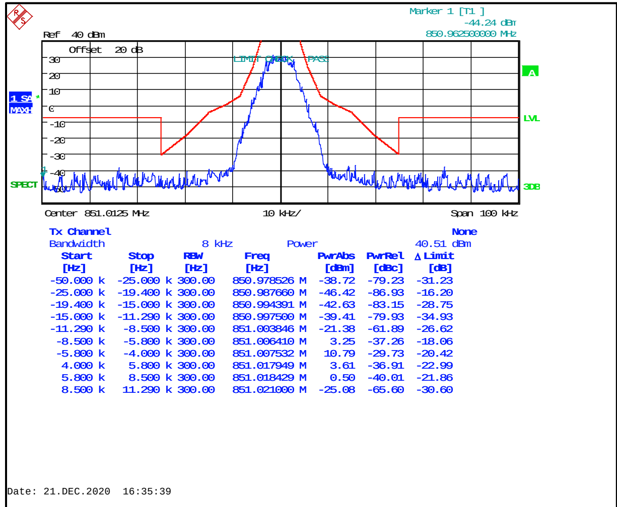
Plot 8-74: Occupied Bandwidth – 851.0125 MHz; H-CPM (TDMA); Mask H
