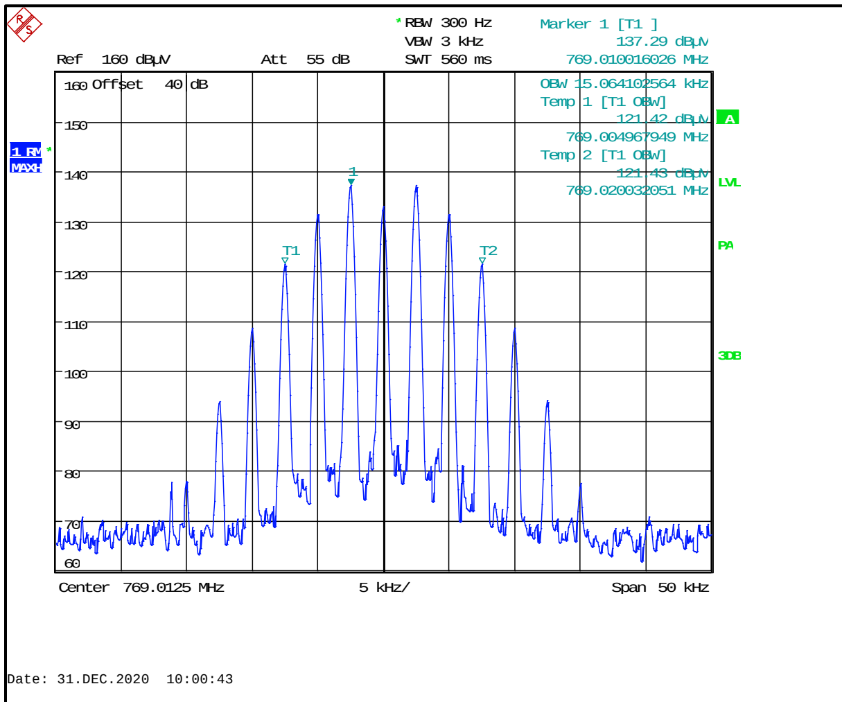
Plot 8-95: 99% Occupied Bandwidth – 769.0125 MHz; WB Analog
