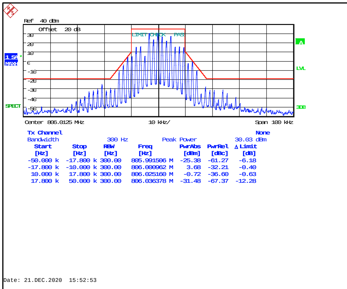
Plot 8-81: Occupied Bandwidth – 806.0125 MHz; HVD SMR; Mask G (ISED)
