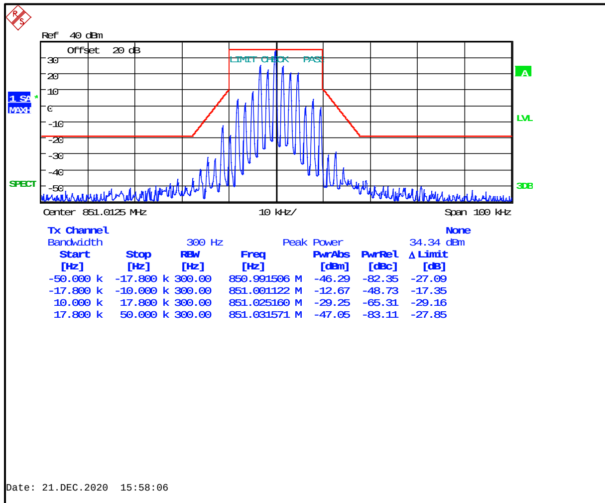
Plot 8-92: Occupied Bandwidth – 851.0125 MHz; HVD NPSPAC; Mask G (ISED)
