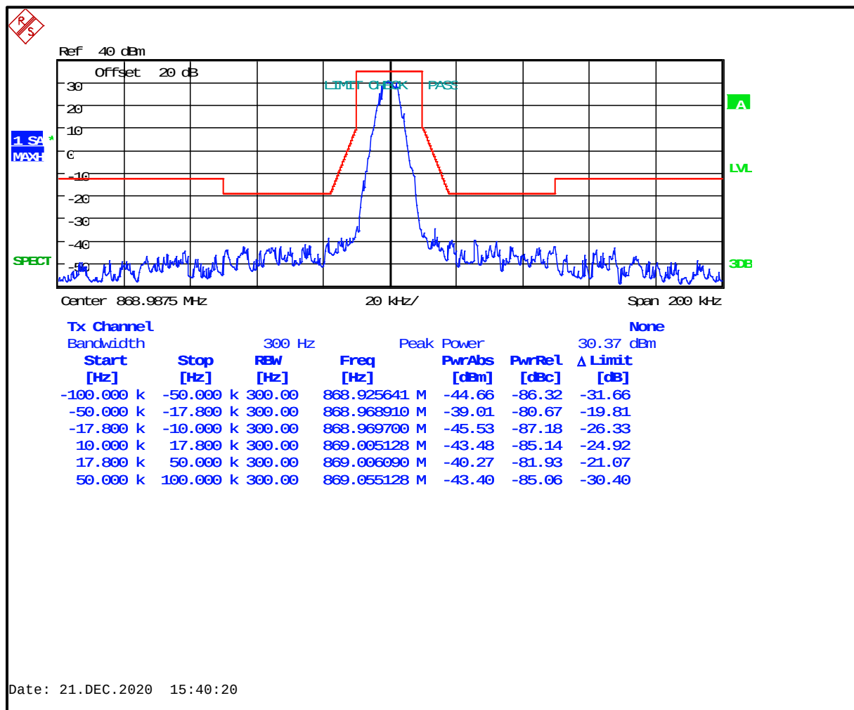
Plot 8-78: Occupied Bandwidth – 868.9875 MHz; H-CPM (TDMA); Mask G
