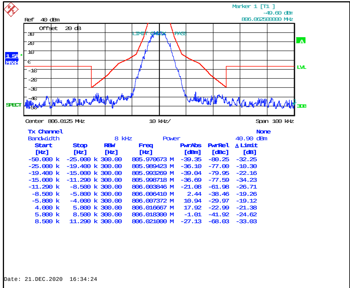
Plot 8-67: Occupied Bandwidth – 806.0125 MHz; H-CPM (TDMA); Mask H
