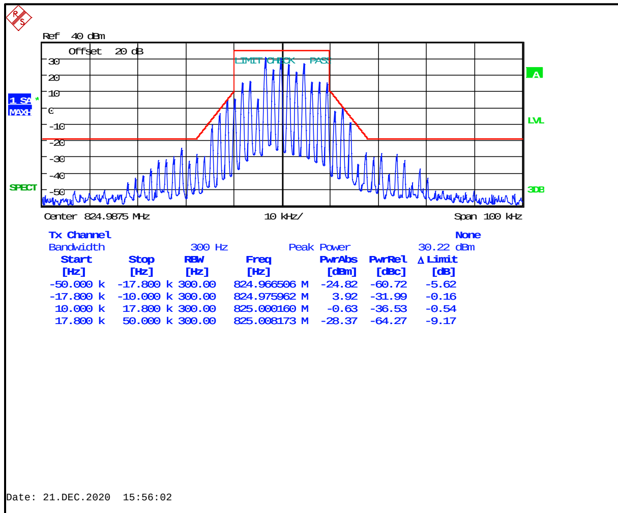
Plot 8-84: Occupied Bandwidth – 824.9875 MHz 9 (EF); HVD SMR; Mask G
