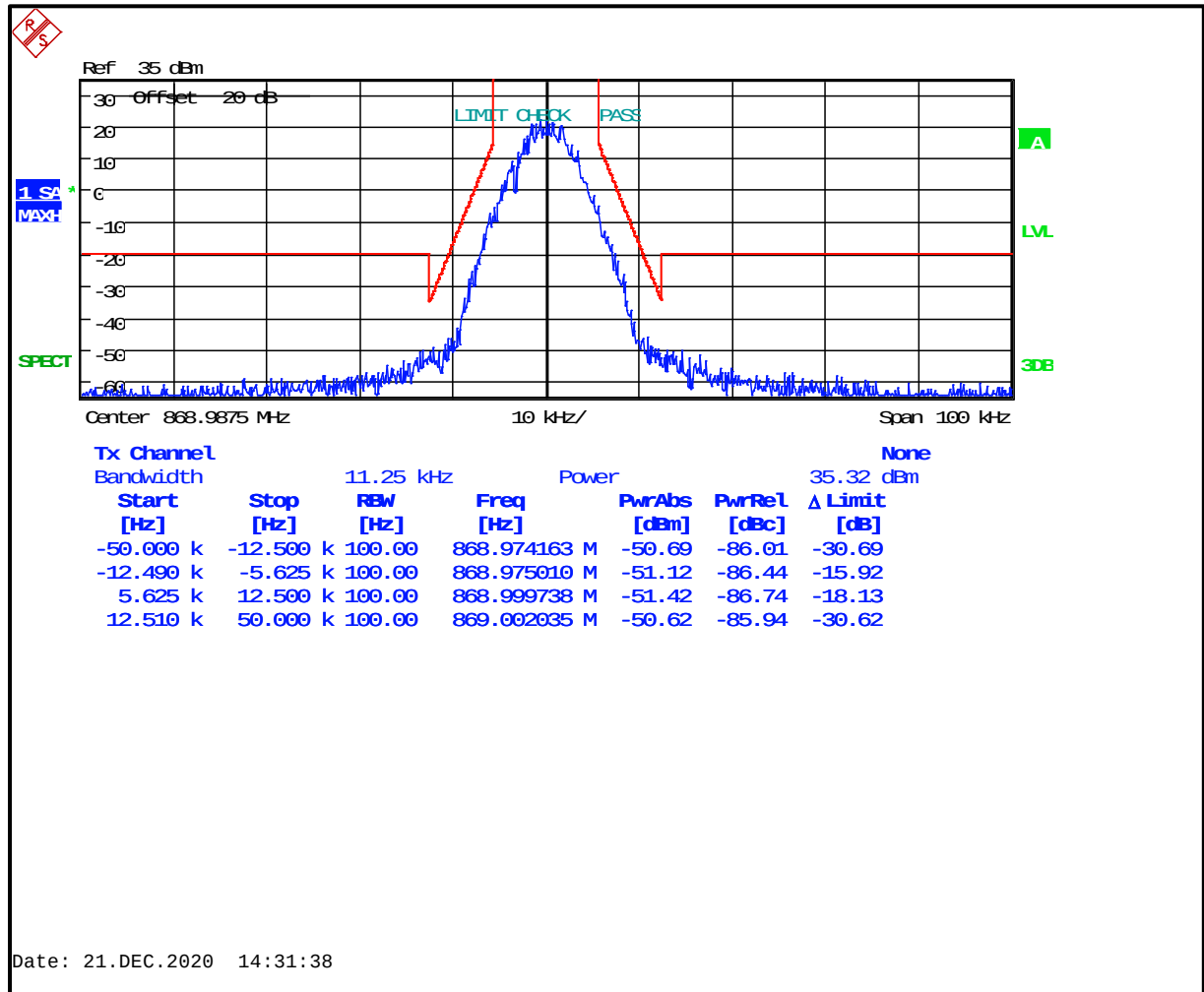
Plot 8-65: Occupied Bandwidth – 868.9875 MHz; C4FM; Mask D (ISED)
