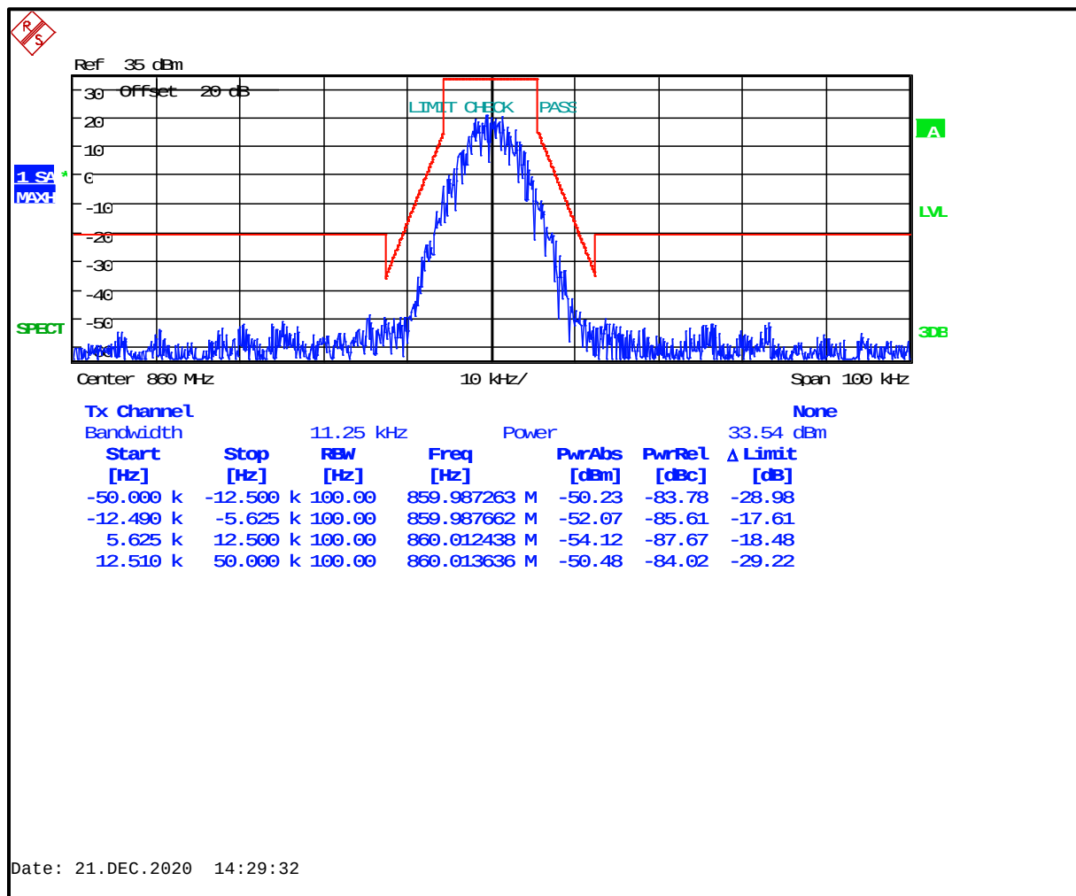
Plot 8-77: Occupied Bandwidth – 860.0000 MHz; H-CPM (TDMA); Mask D (ISED)
