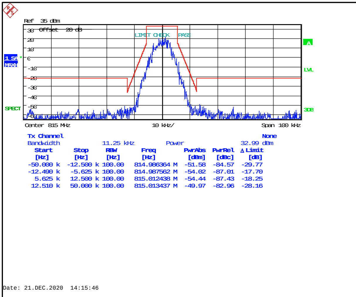
Plot 8-70: Occupied Bandwidth – 815.0000 MHz; H-CPM (TDMA); Mask D (ISED)
