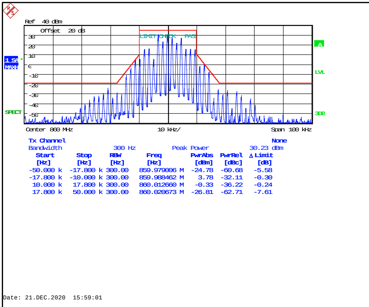
Plot 8-86: Occupied Bandwidth – 860.0000 MHz; HVD SMR; Mask G
