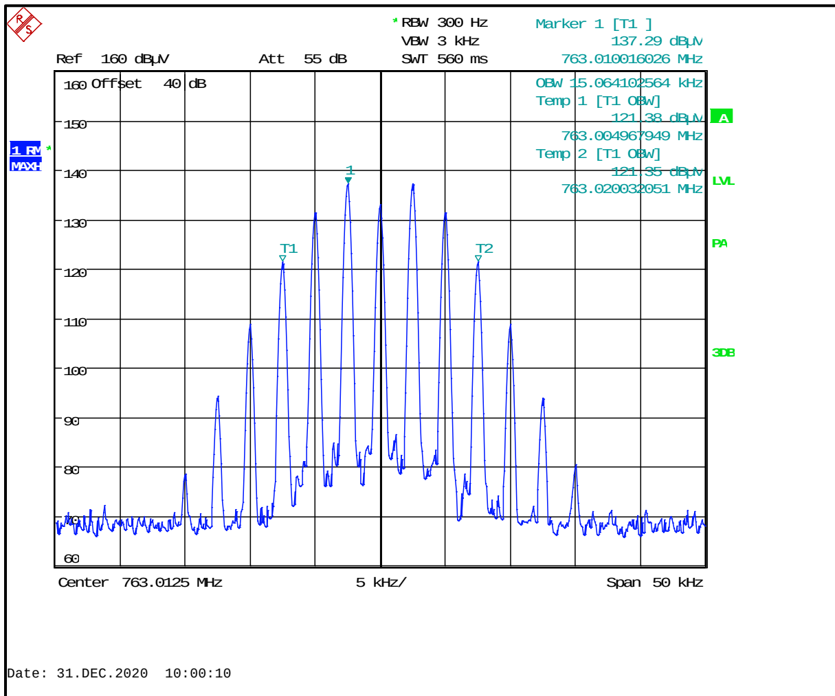
Plot 8-93: 99% Occupied Bandwidth – 763.0125 MHz; WB Analog
