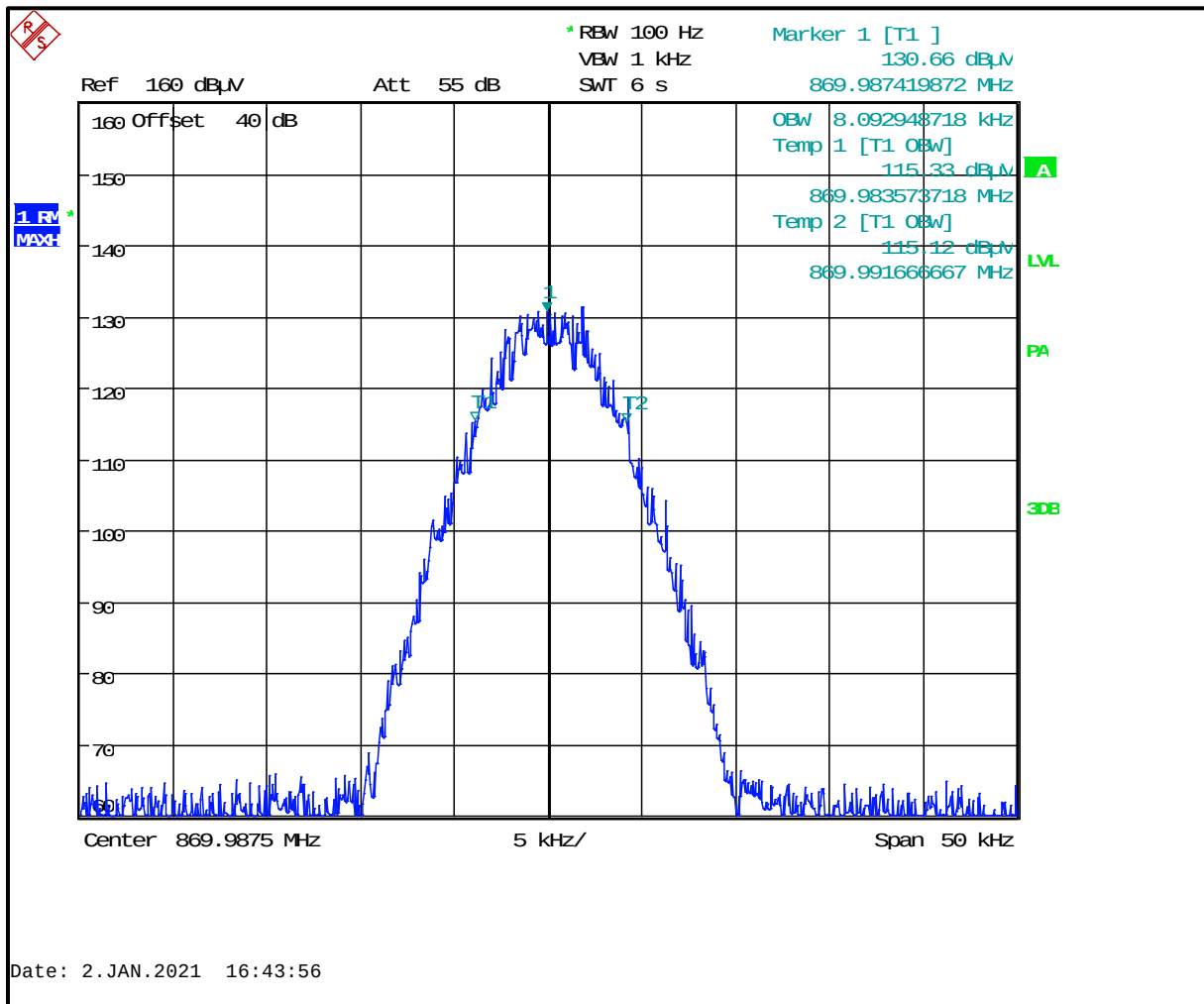
Plot 8-154: 99% Occupied Bandwidth – 869.9875 MHz; C4FM
