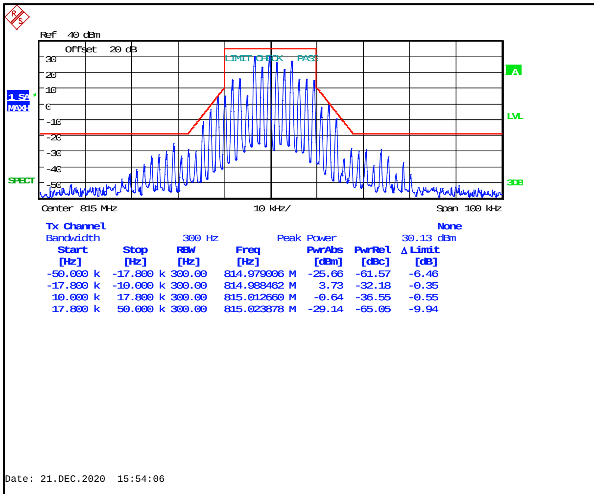
Plot 8-82: Occupied Bandwidth – 815.0000 MHz; HVD SMR; Mask G
