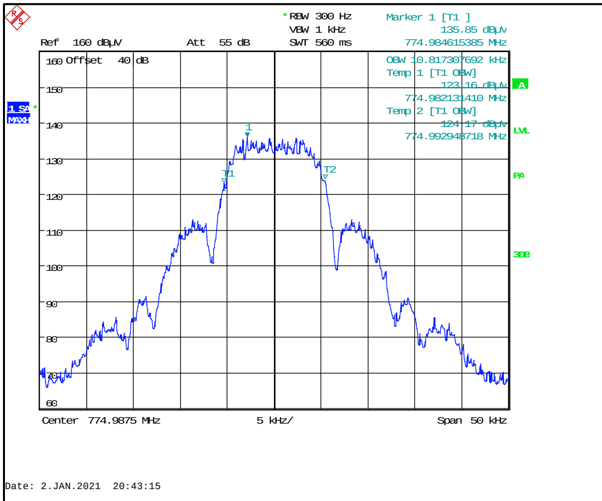
Plot 8-199: 99% Occupied Bandwidth – 774.9875 MHz; WB 2-LVL FSK 9600
