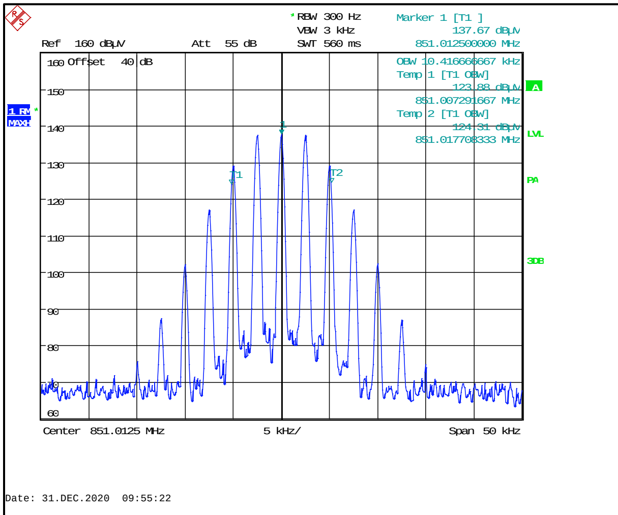
Plot 8-134: 99% Occupied Bandwidth – 851.0125 MHz; NPSPAC Analog
