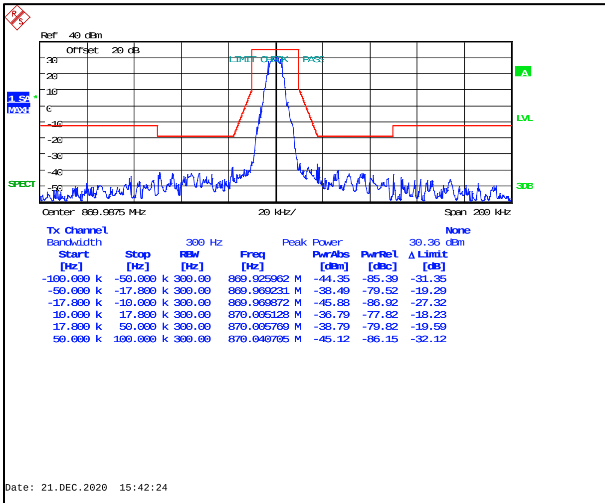
Plot 8-80: Occupied Bandwidth – 869.9875 MHz (EF); H-CPM (TDMA); Mask G
