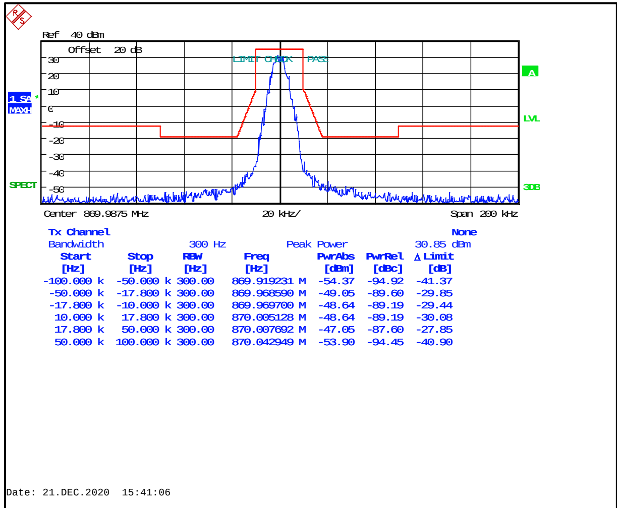
Plot 8-66: Occupied Bandwidth – 869.9875 MHz (EF); C4FM; Mask G
