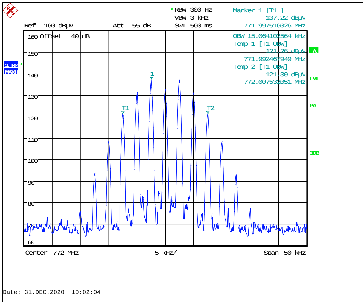
Plot 8-96: 99% Occupied Bandwidth – 772.0000 MHz; WB Analog
