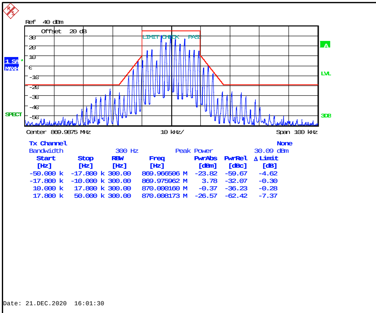
Plot 8-88: Occupied Bandwidth – 869.9875 MHz (EF); HVD SMR; Mask G
