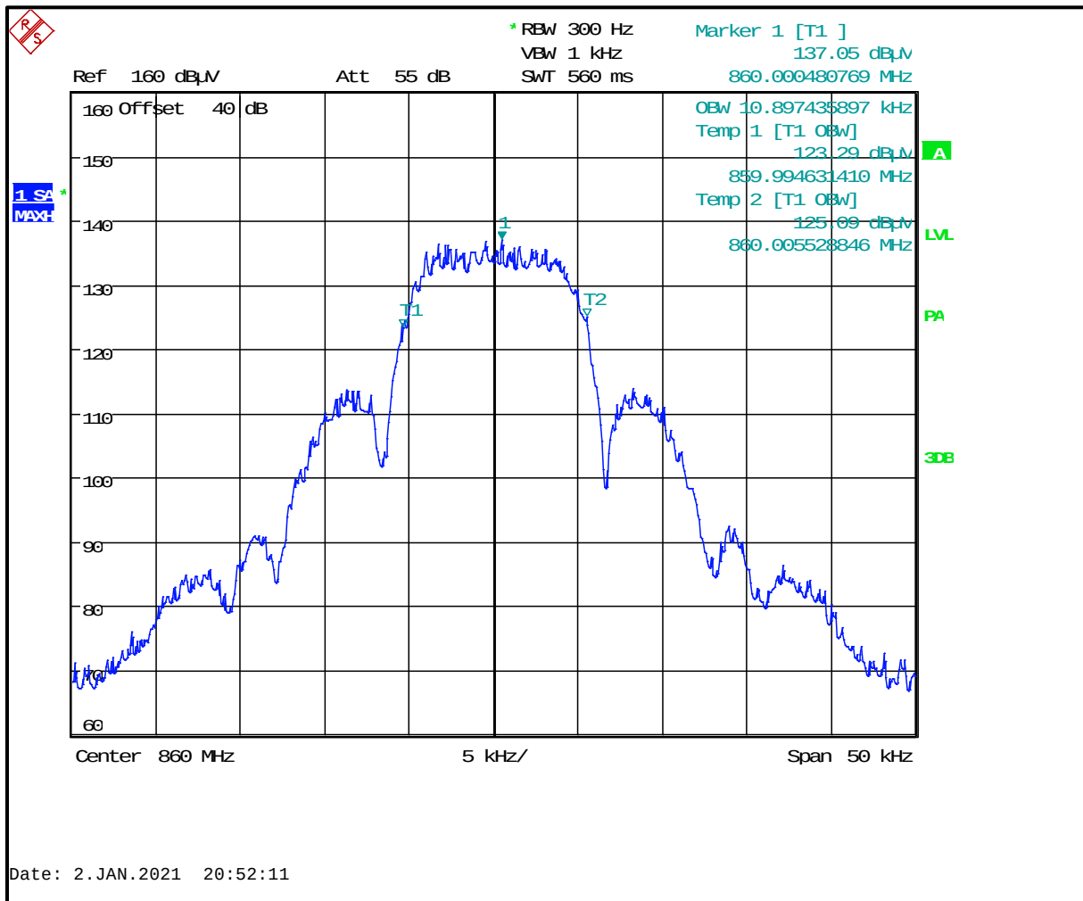
Plot 8-212: 99% Occupied Bandwidth – 860.0000 MHz; WB 2-LVL FSK 9600
