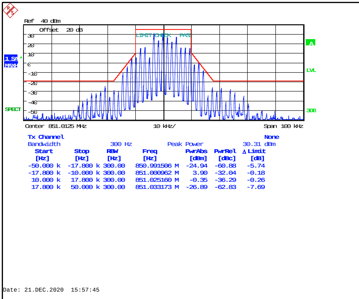
Plot 8-85: Occupied Bandwidth – 851.0125 MHz; HVD SMR; Mask G (ISED)
