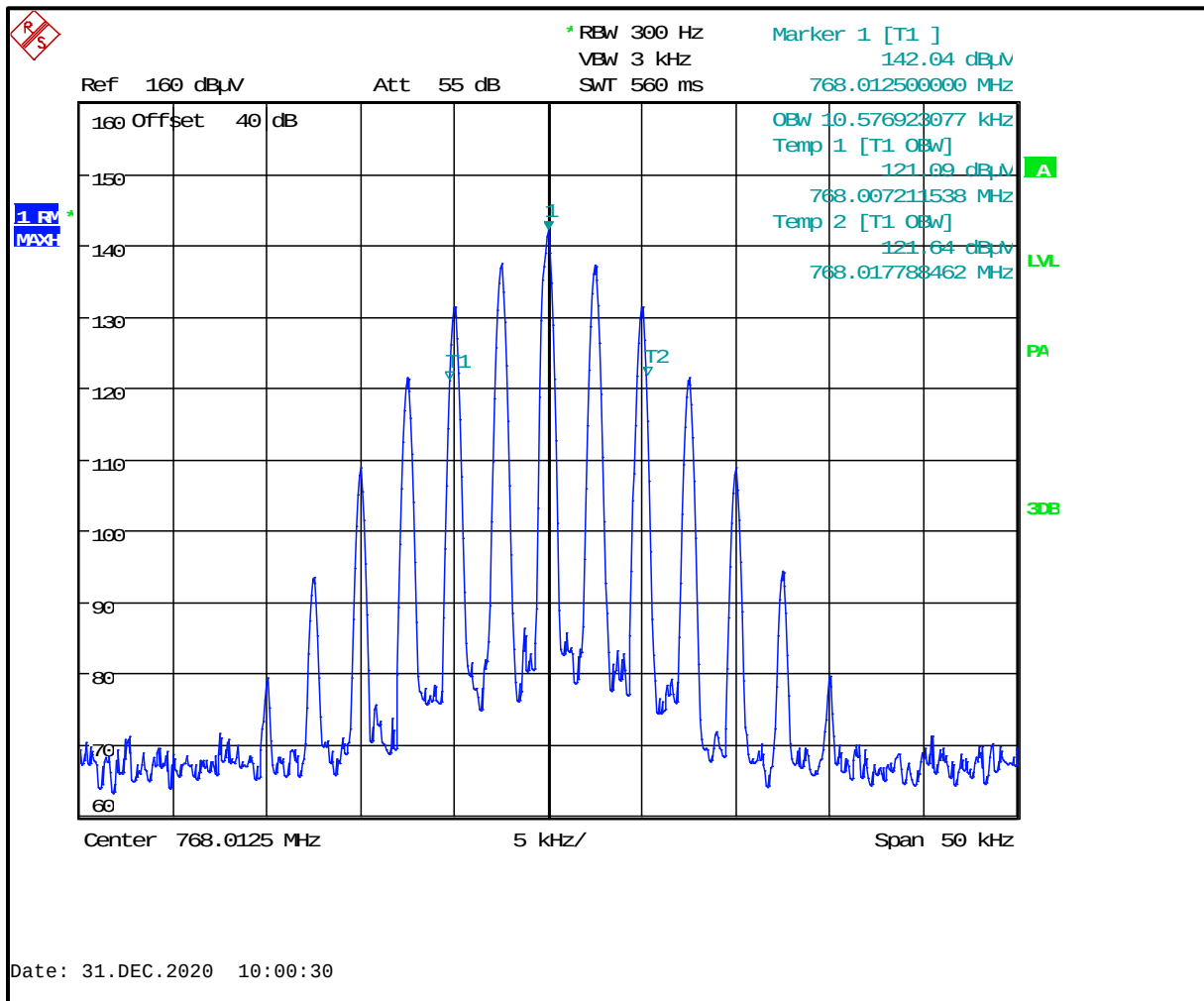
Plot 8-94: 99% Occupied Bandwidth – 768.0125 MHz; WB Analog
