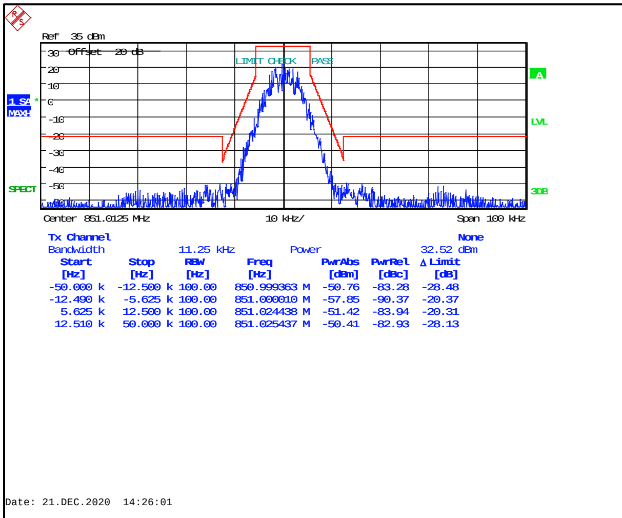
Plot 8-75: Occupied Bandwidth – 851.0125 MHz; H-CPM (TDMA); Mask D (ISED)
