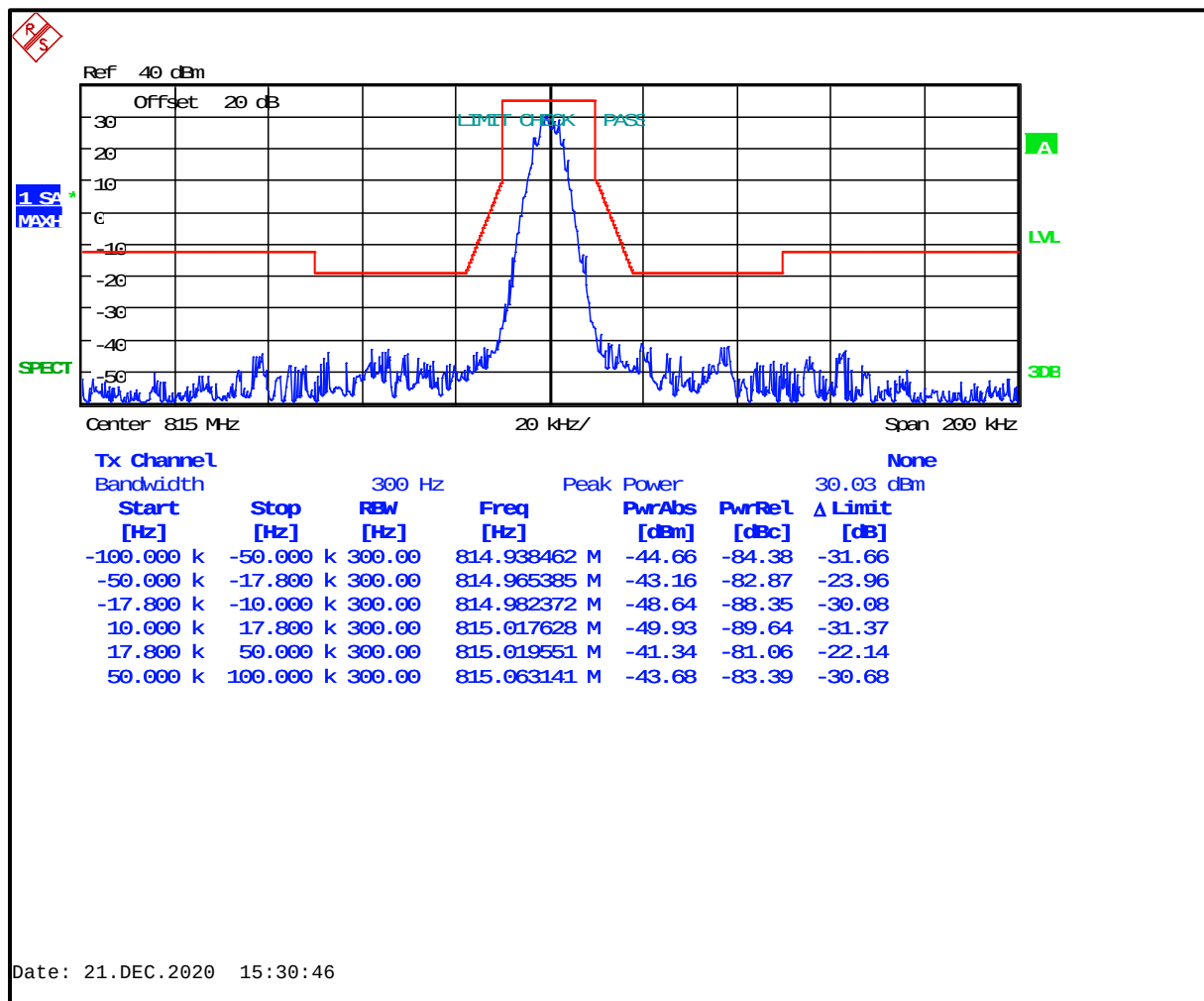
Plot 8-69: Occupied Bandwidth – 815.0000 MHz; H-CPM (TDMA);; Mask G
