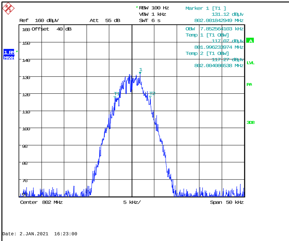
Plot 8-144: 99% Occupied Bandwidth – 802.0000 MHz; C4FM
