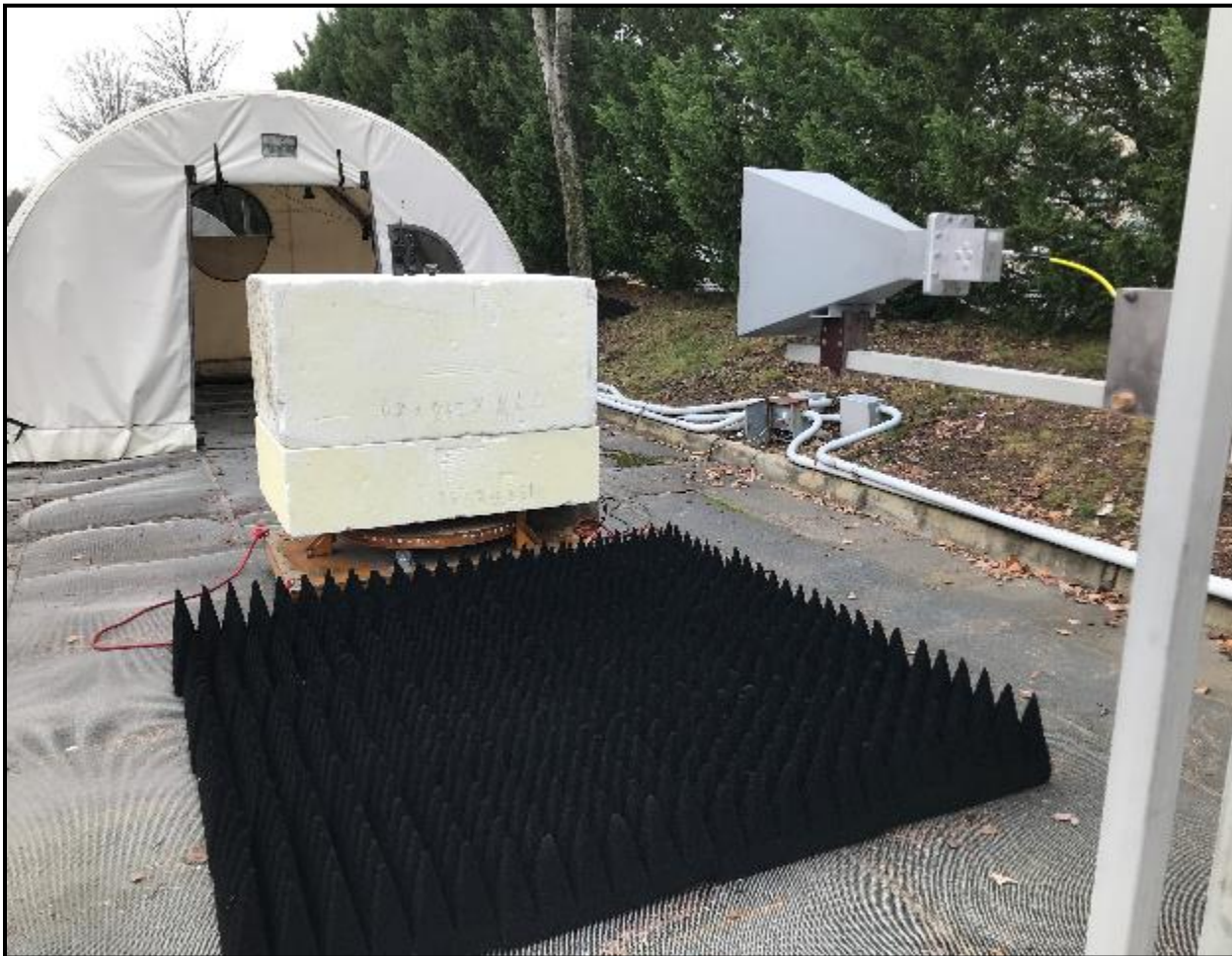
Photograph 1: Radiated Emissions Testing – Front View (Above 1 GHz)
