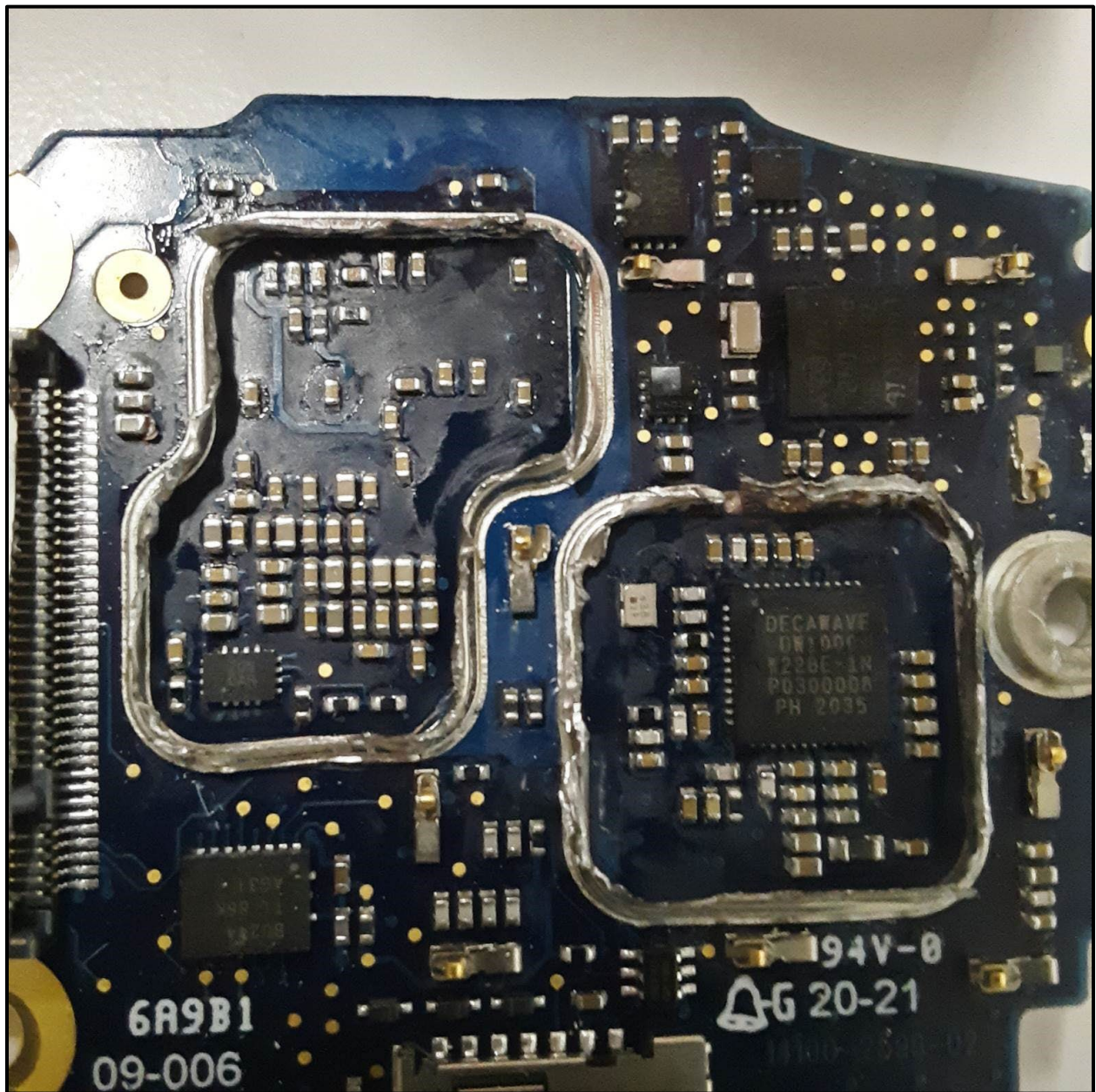
CCM Top View without Shields
