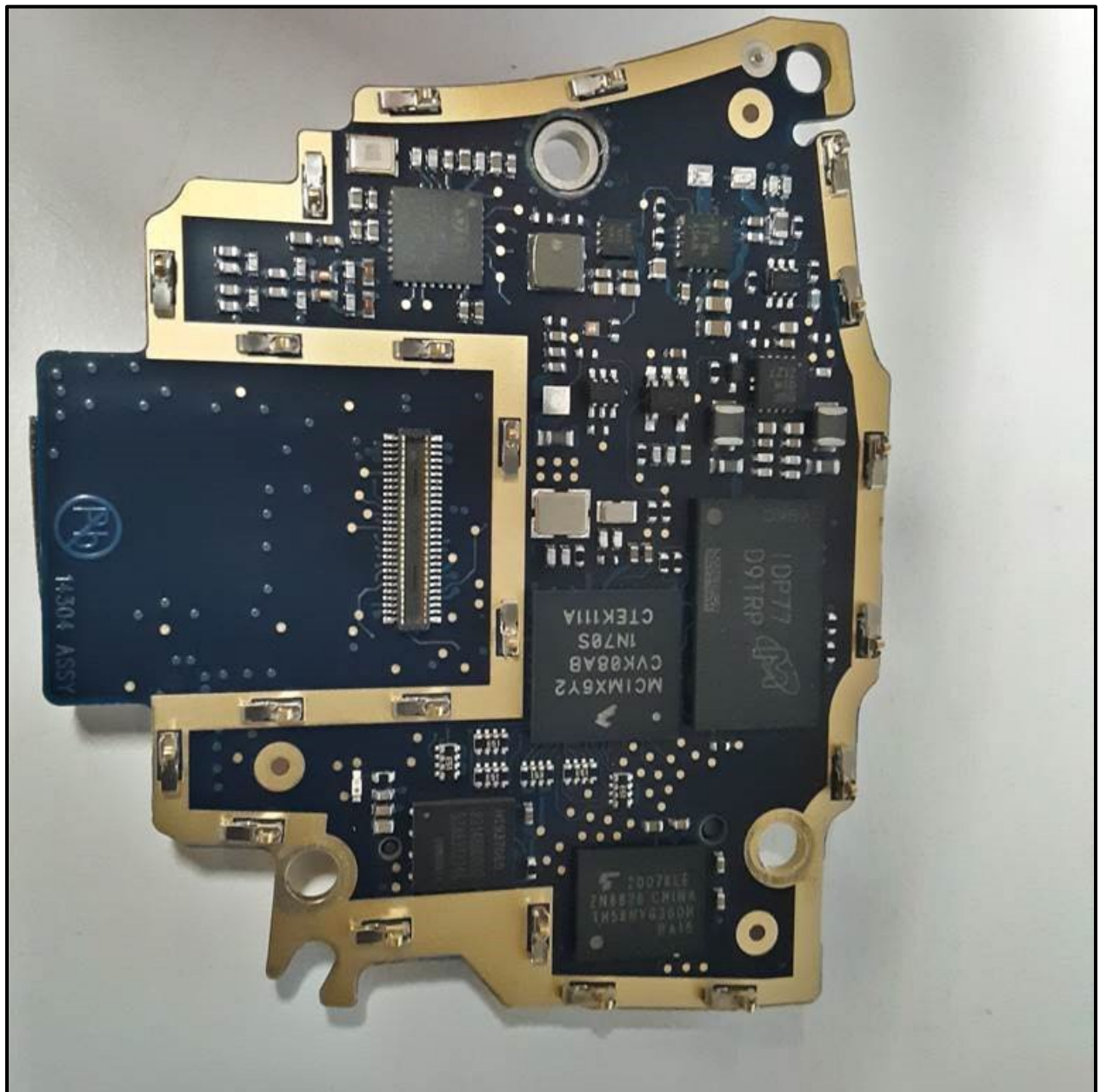
CCM Bottom View
