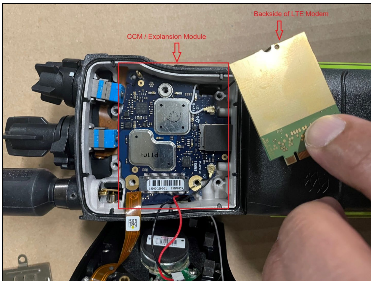
CCM Board
