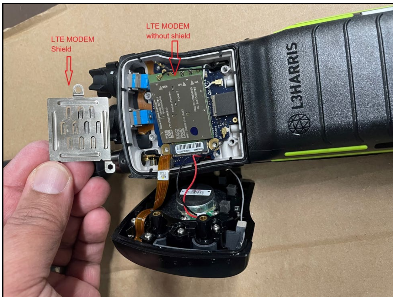
LTE Modem Shield Removed
