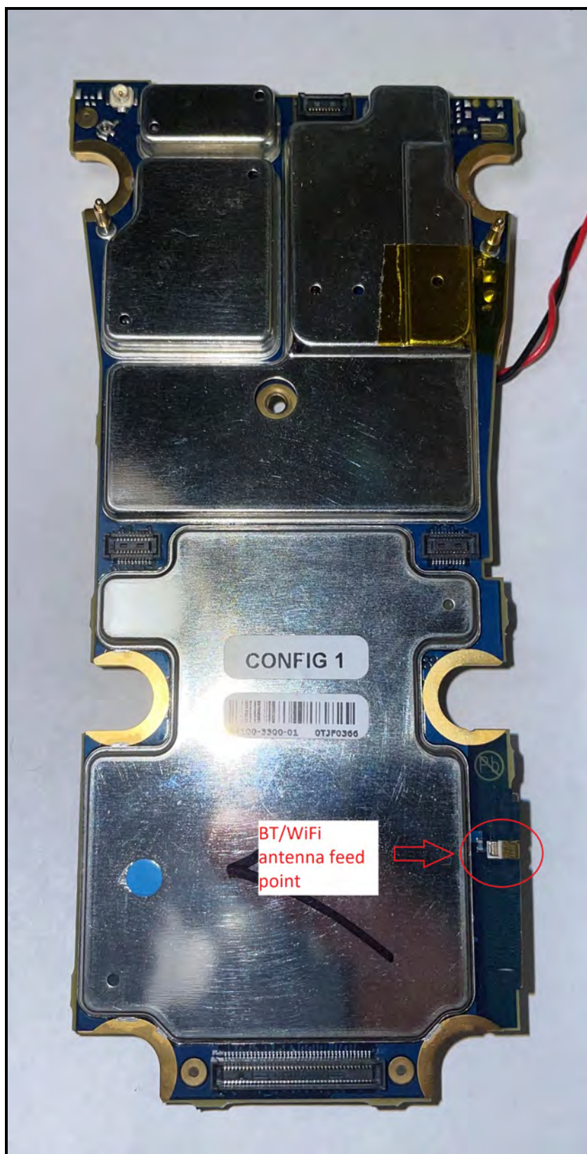
BT/Wi-Fi Antenna Feed Point
