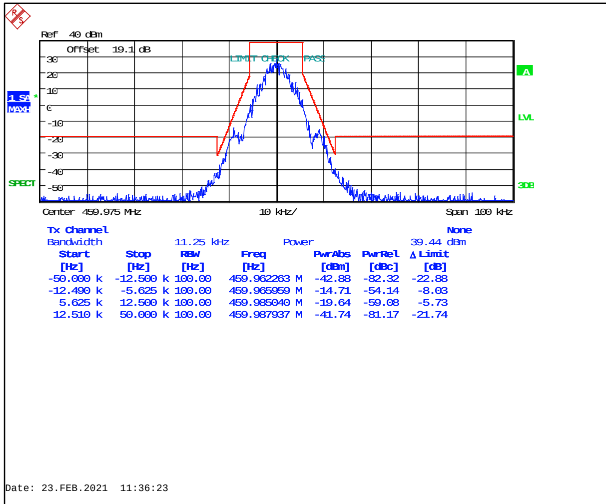
Plot 8-127: Occupied Bandwidth – 459.9750 MHz; Narrowband 2-level FSK 9600; Mask D
