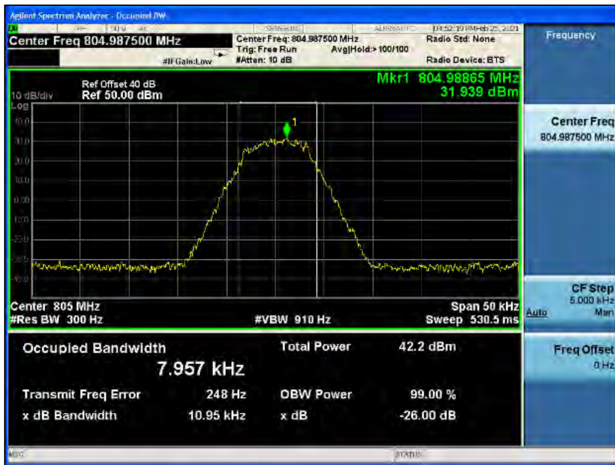
Plot 8-537: OBW 99%, 804.9875 MHz, H-CPM TDMA
