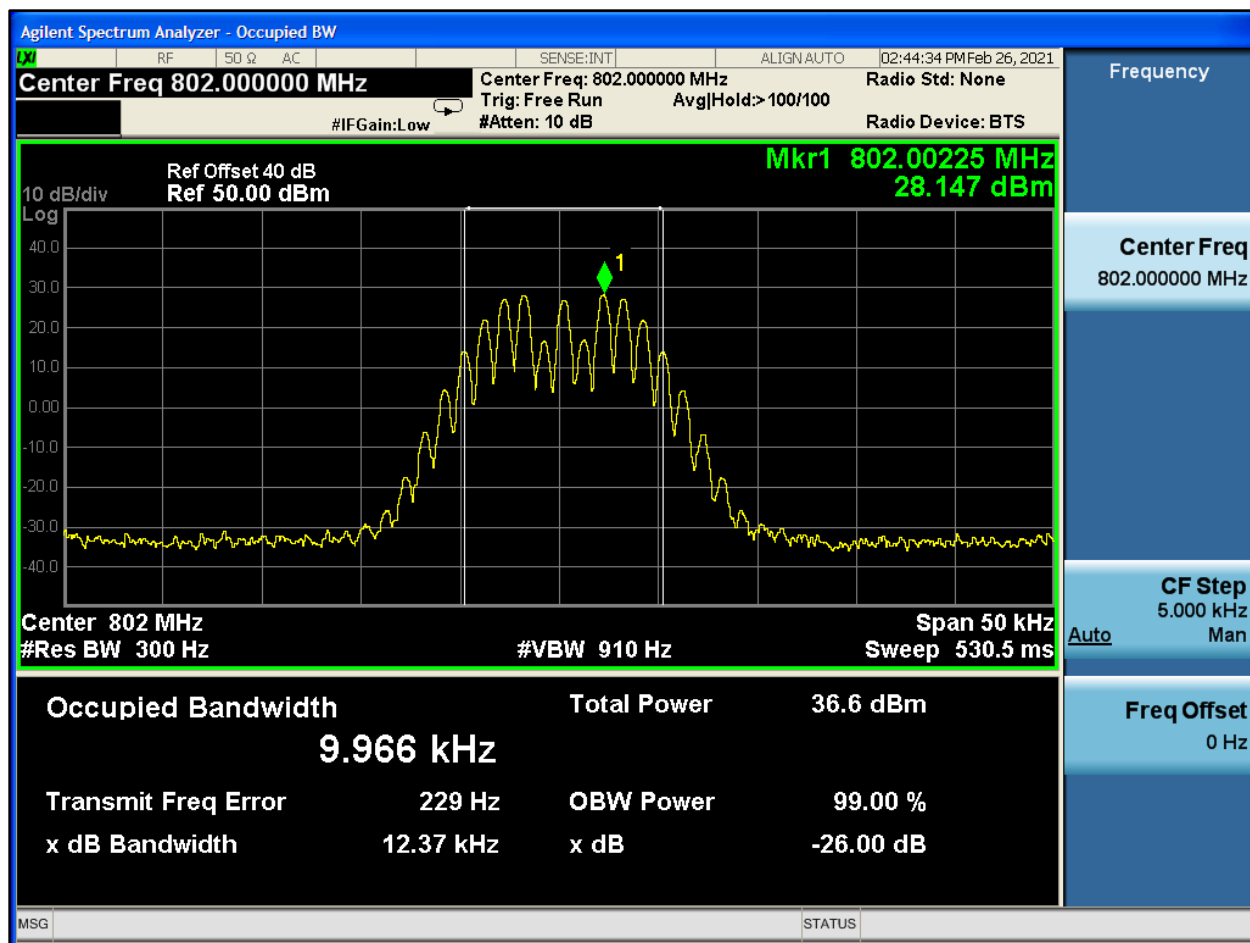
Plot 8-524: OBW 99%, 802.0000 MHz, NPSPAC
