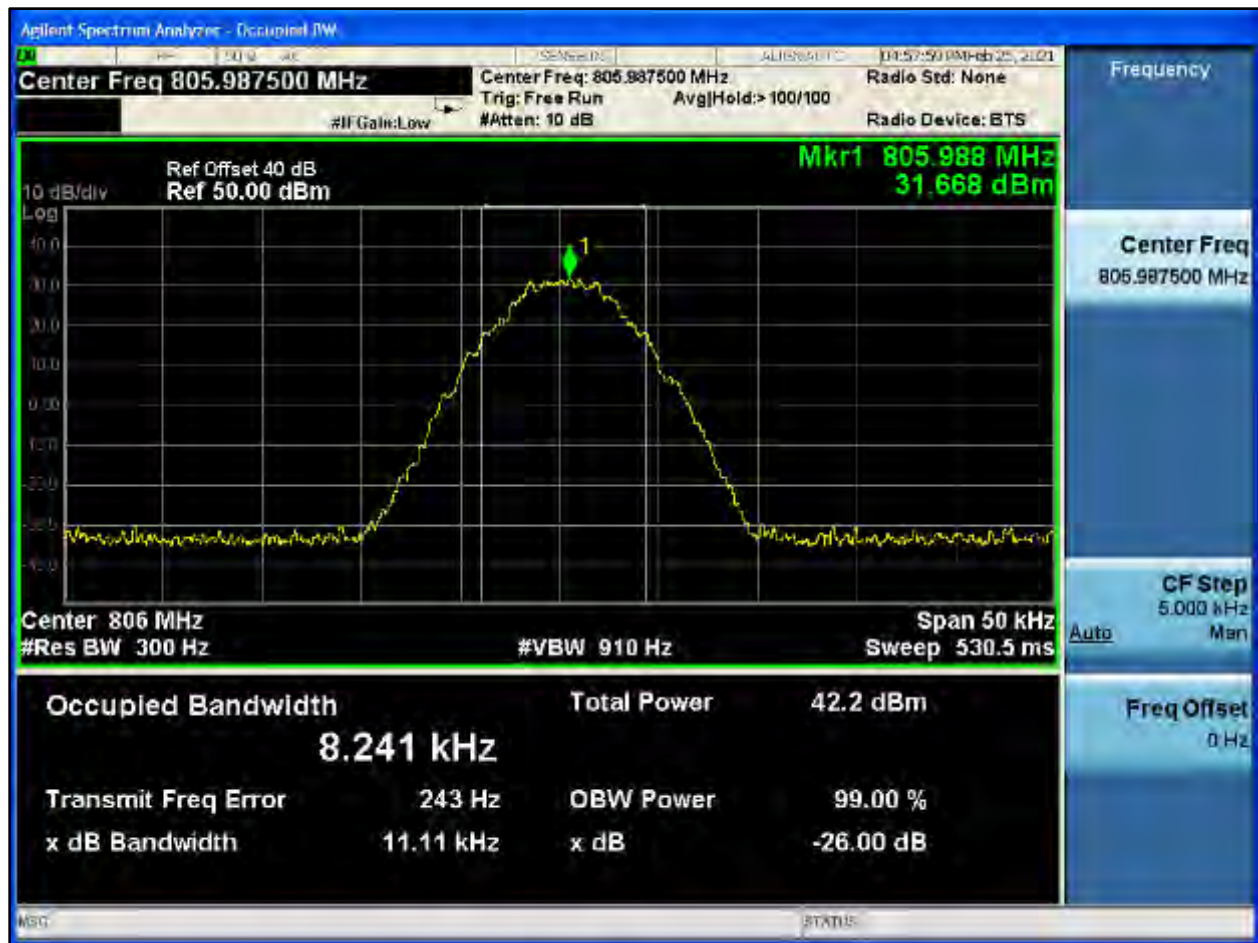
Plot 8-546: OBW 99%, 805.9875 MHz, C4FM
