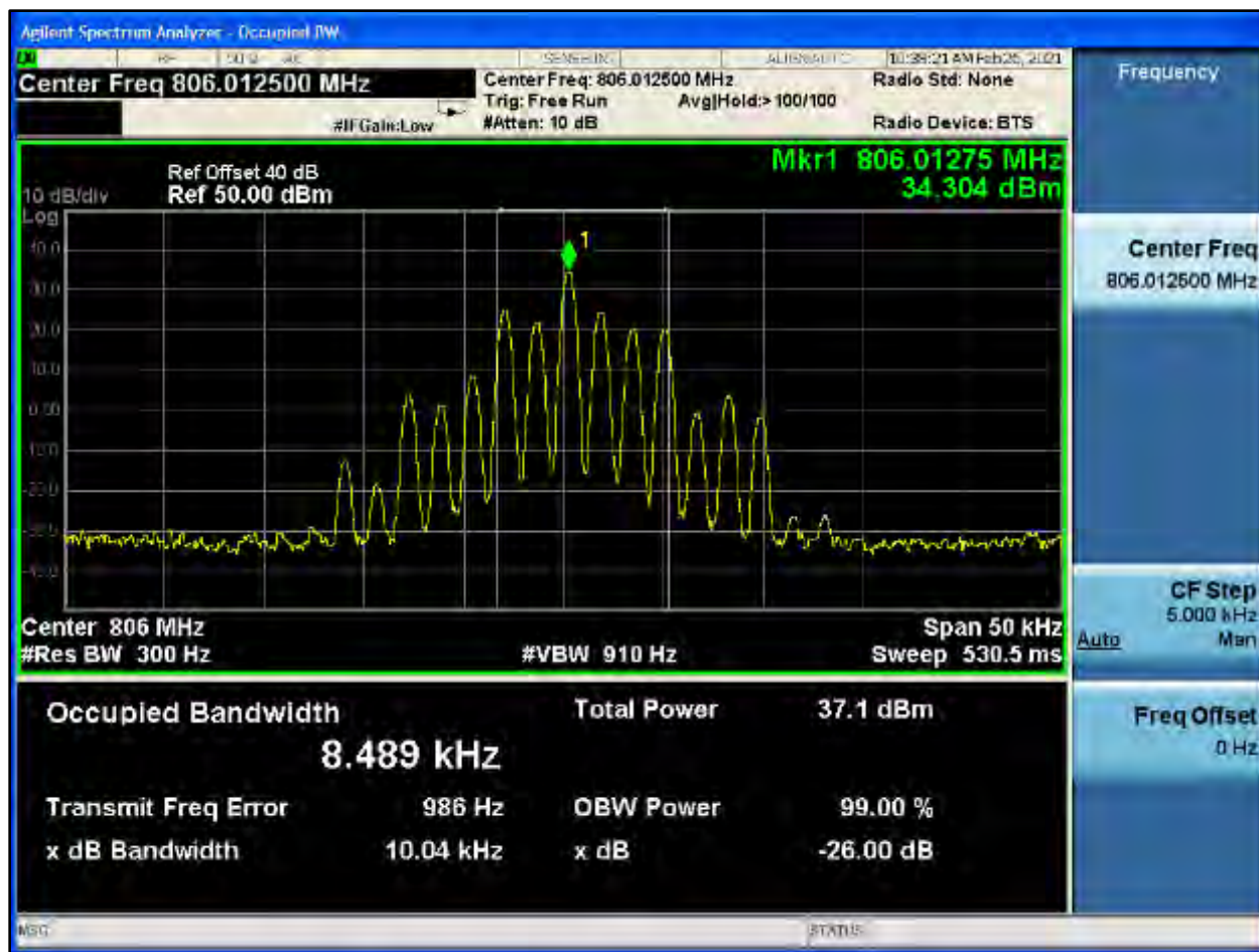
Plot 8-562: OBW 99%, 806.0125 MHz, HVD NPSPAC
