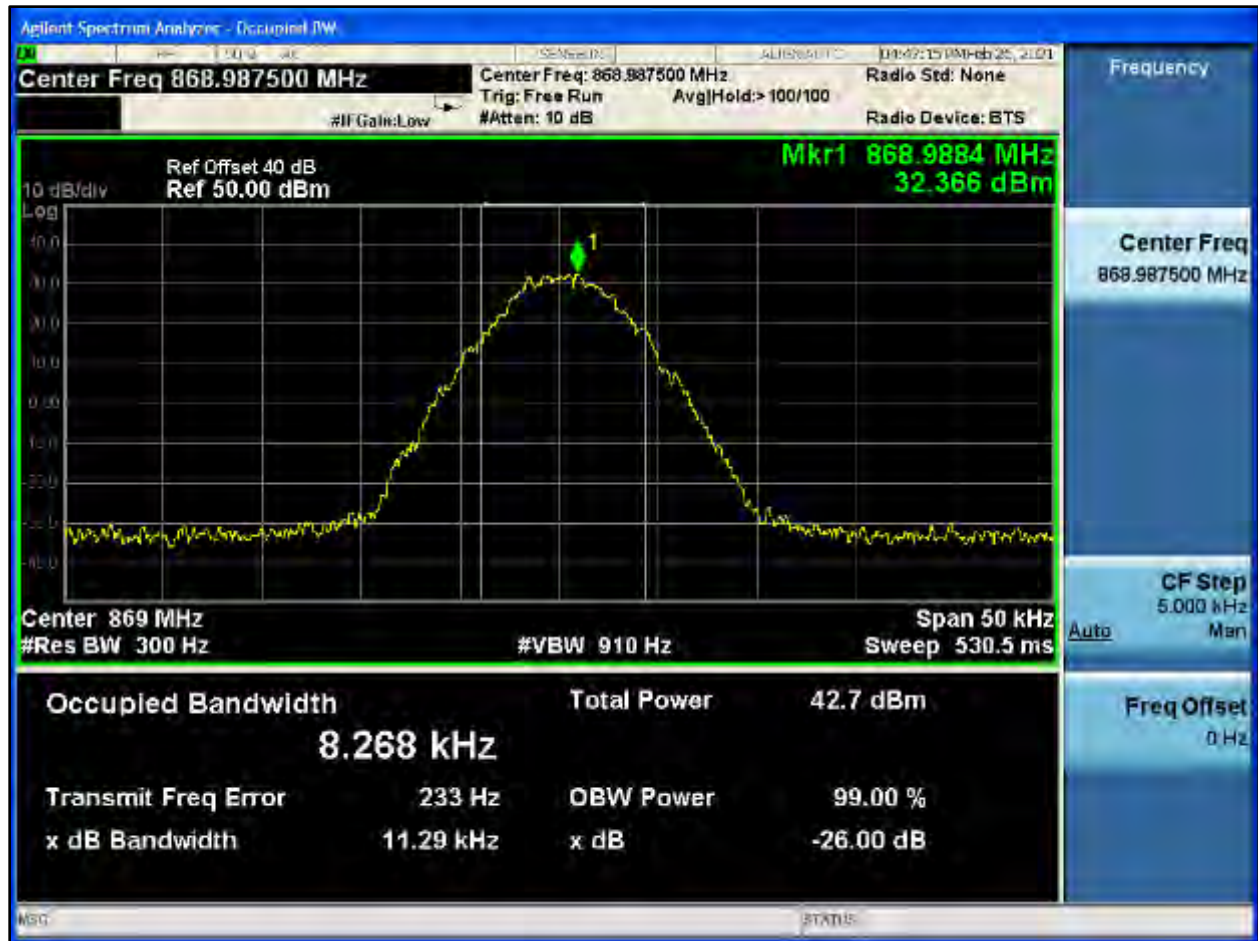
Plot 8-616: OBW 99%, 868.9875 MHz, C4FM
