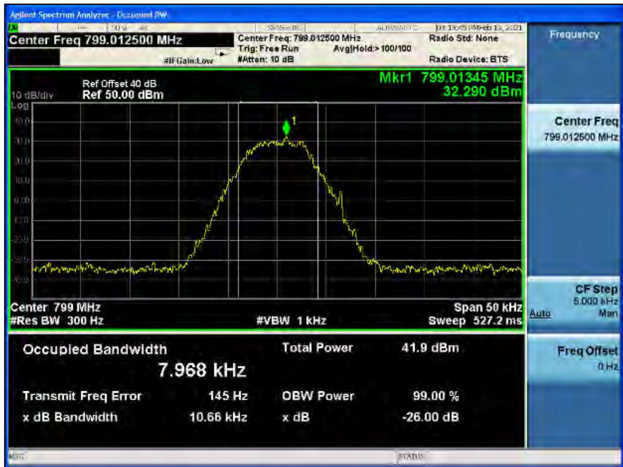
Plot 8-517: OBW 99%, 799.0125 MHz, H-CPM TDMA
