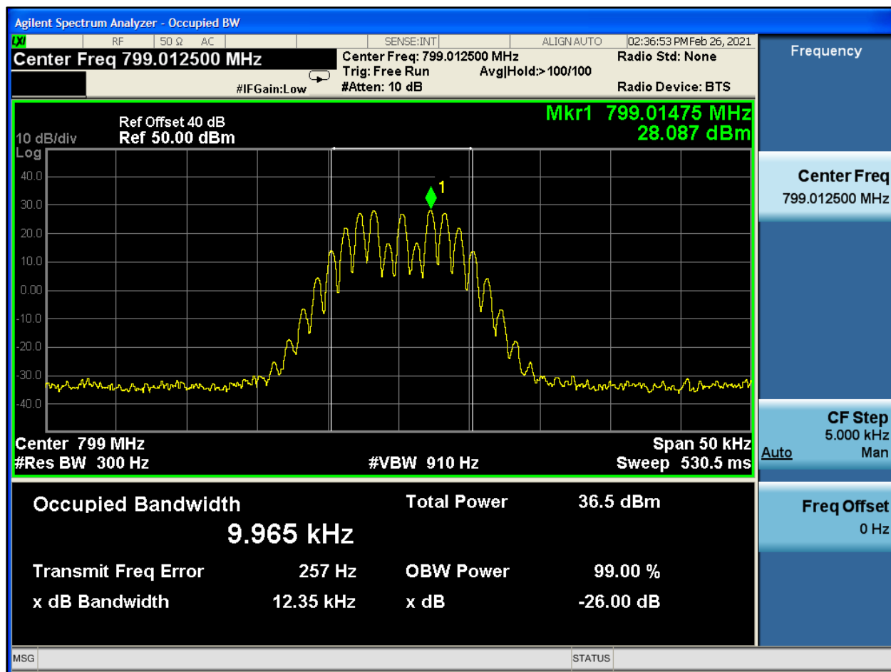
Plot 8-514: OBW 99%, 799.0125 MHz, NPSPAC
