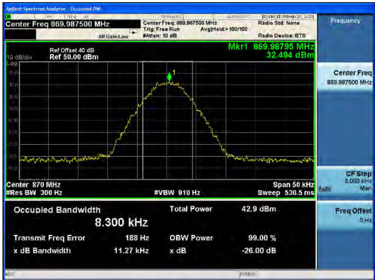
Plot 8-626: OBW 99%, 869.9875 MHz, C4FM
