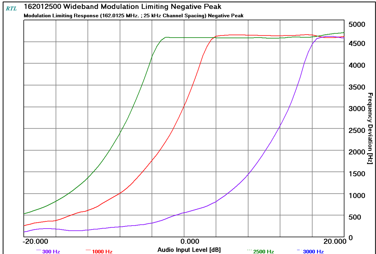
Plot 10-6: Modulation Characteristics – Modulation Limiting - 162.0125 MHz; (WB) Negative Peak
