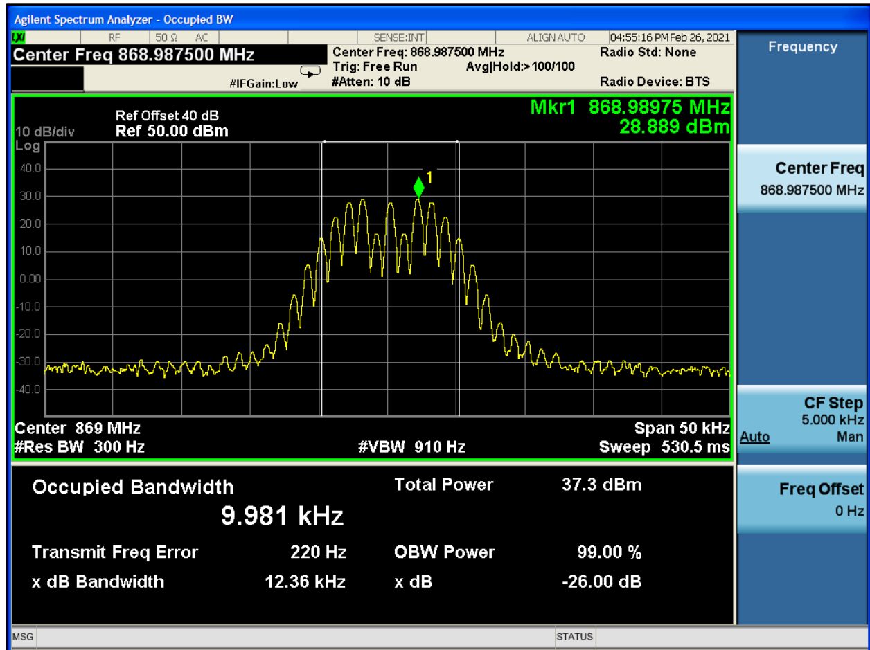
Plot 8-614: OBW 99%, 868.9875 MHz, NPSPAC
