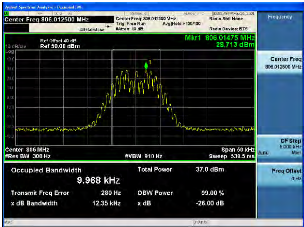
Plot 8-554: OBW 99%, 806.0125 MHz, NPSPAC
