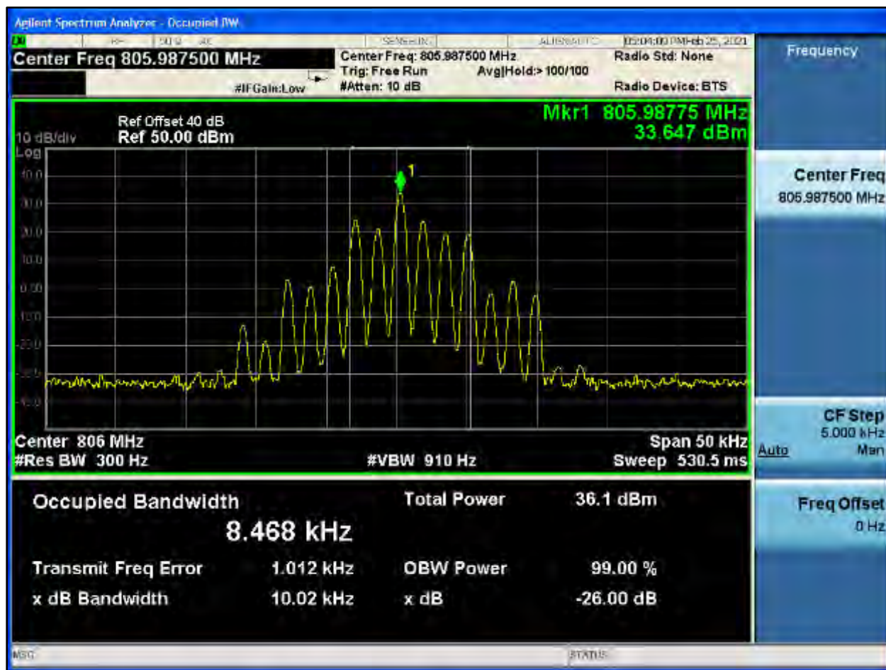
Plot 8-552: OBW 99%, 805.9875 MHz, HVD NPSPAC
