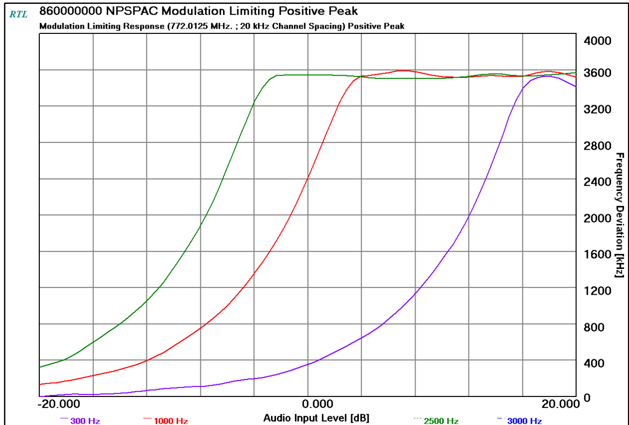
Plot 10-11: Modulation Characteristics – Modulation Limiting – 860.0000 MHz; (NPSPAC); Positive Peak
