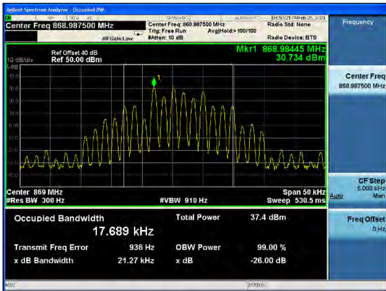
Plot 8-621: OBW 99%, 868.9875 MHz, HVD SMR
