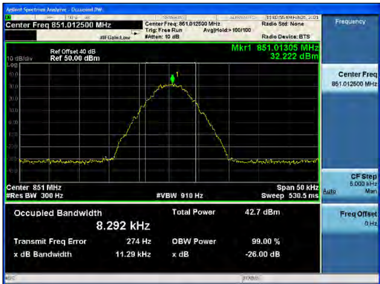
Plot 8-596: OBW 99%, 851.0125 MHz, C4FM
