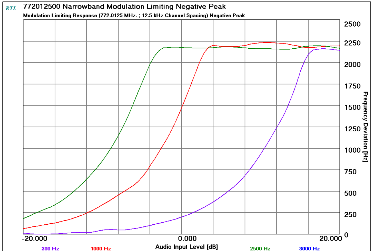
Plot 10-10: Modulation Characteristics – Modulation Limiting – 772.0125 MHz; (NB); Negative Peak
