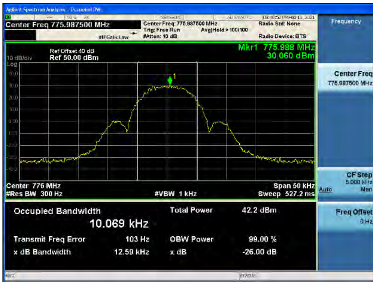
Plot 8-489: OBW 99%, 775.9875 MHz, NPSPAC 2 FSK
