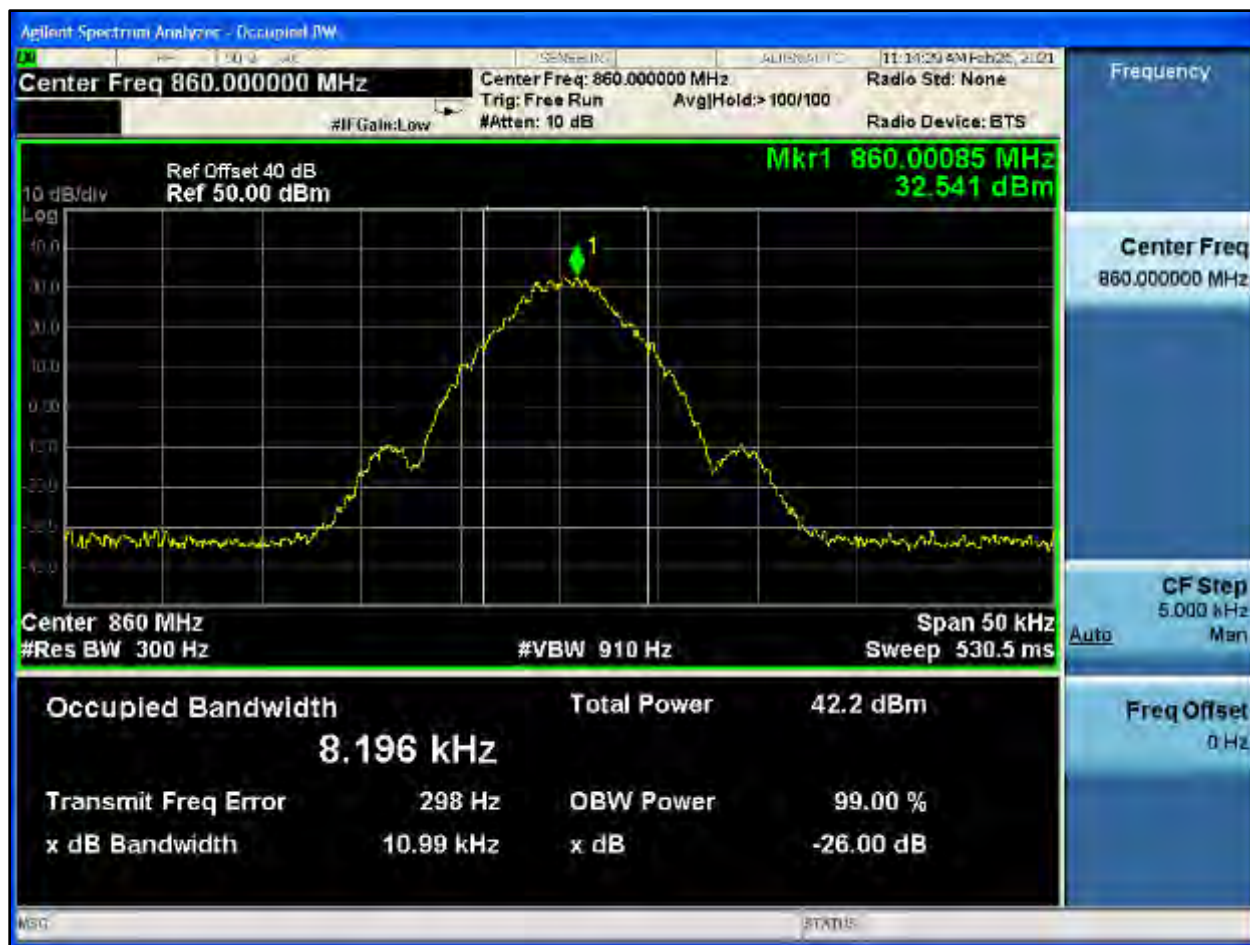
Plot 8-608: OBW 99%, 860.0000 MHz, NB 2 FSK
