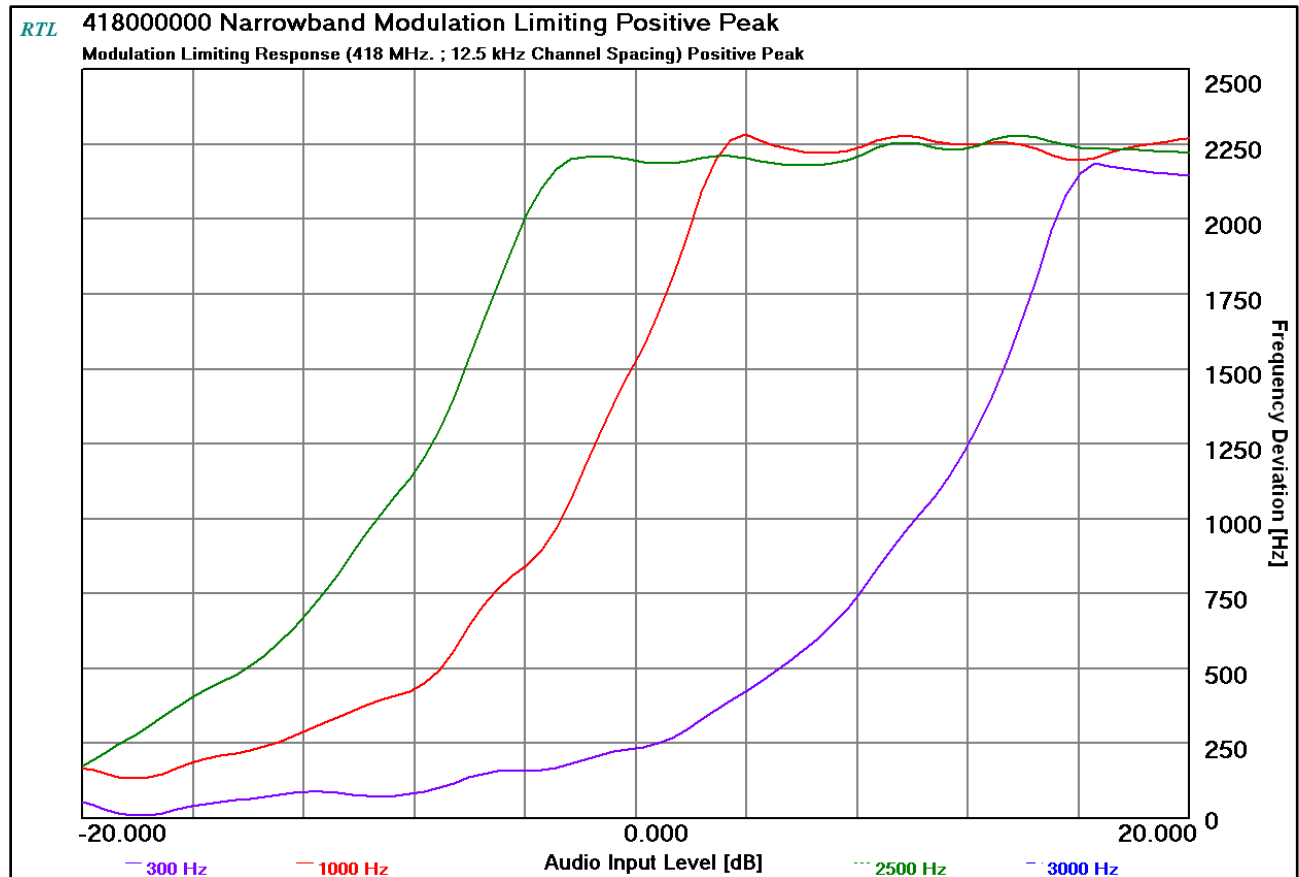
Plot 10-7: Modulation Characteristics – Modulation Limiting – 418.0 MHz; (NB); Positive Peak
