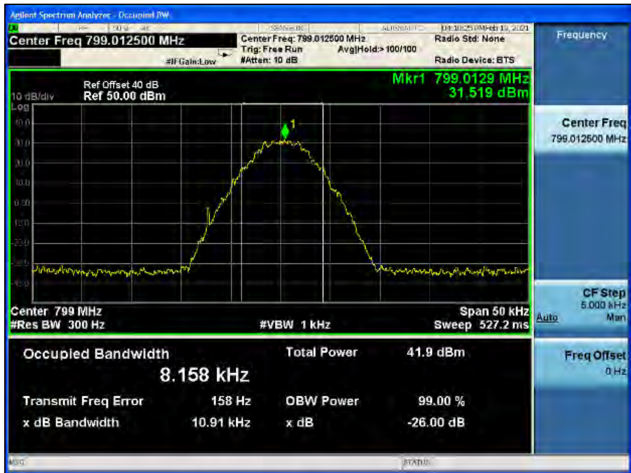
Plot 8-516: OBW 99%, 799.0125 MHz, C4FM
