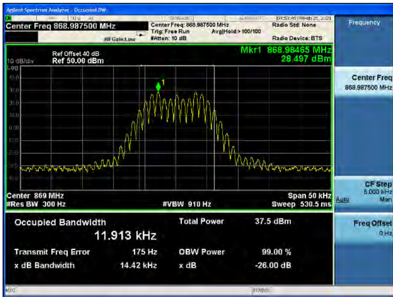
Plot 8-615: OBW 99%, 868.9875 MHz, WB
