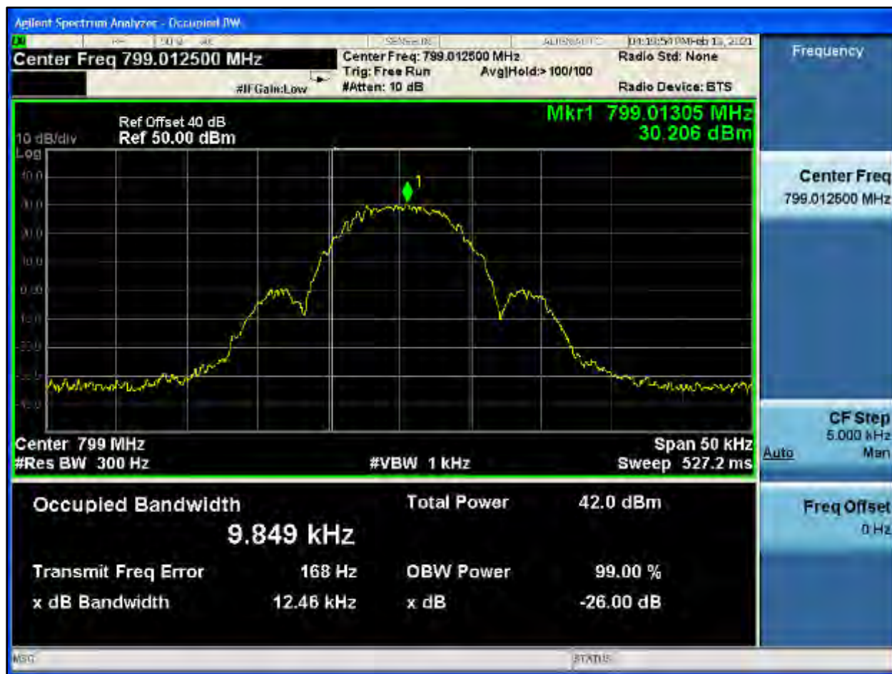
Plot 8-519: OBW 99%, 799.0125 MHz, NPSPAC 2 FSK
