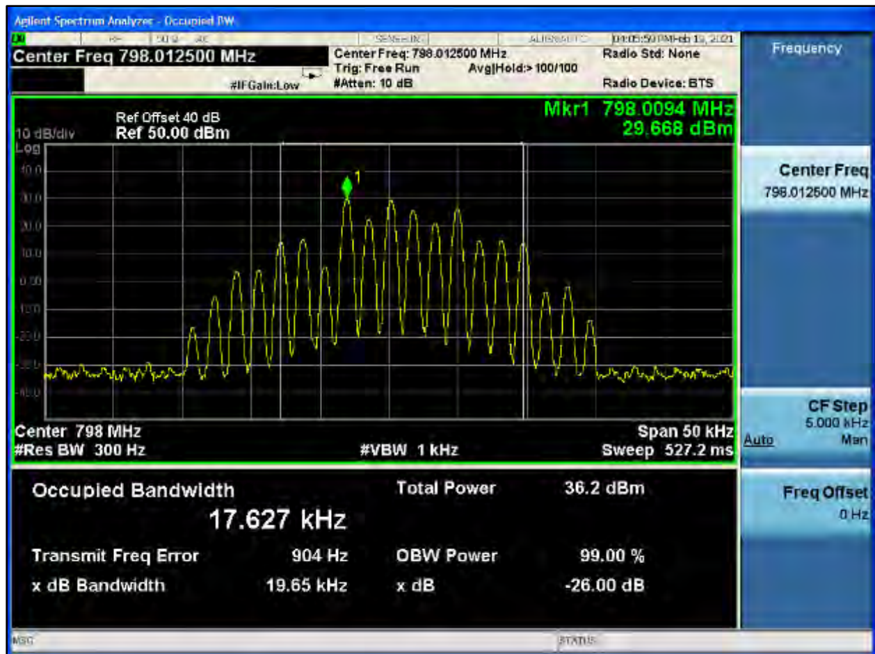
Plot 8-511: OBW 99%, 798.0125 MHz, HVD SMR
