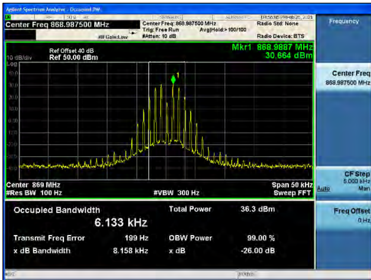
Plot 8-613: OBW 99%, 868.9875 MHz, NB
