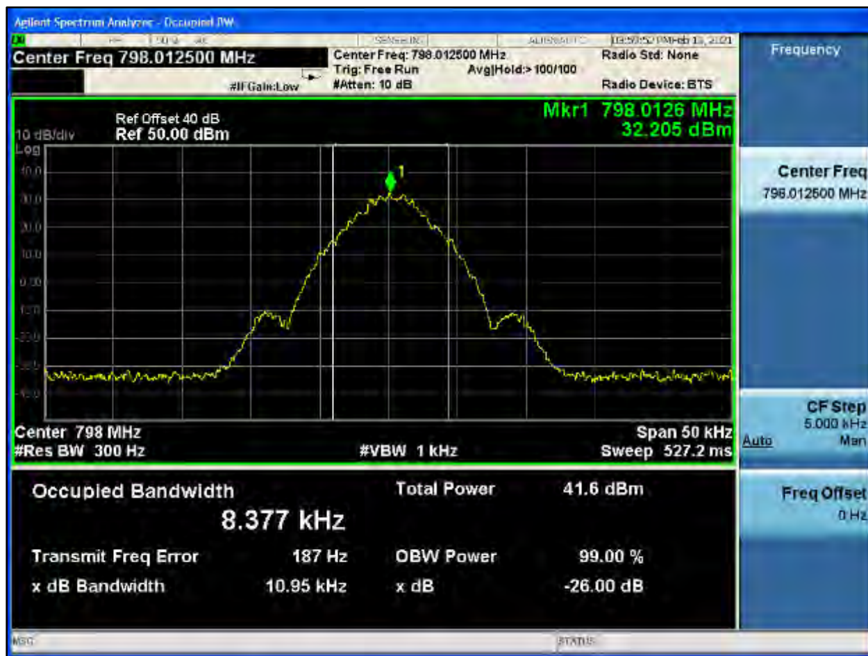
Plot 8-508: OBW 99%, 798.0125 MHz, NB 2 FSK
