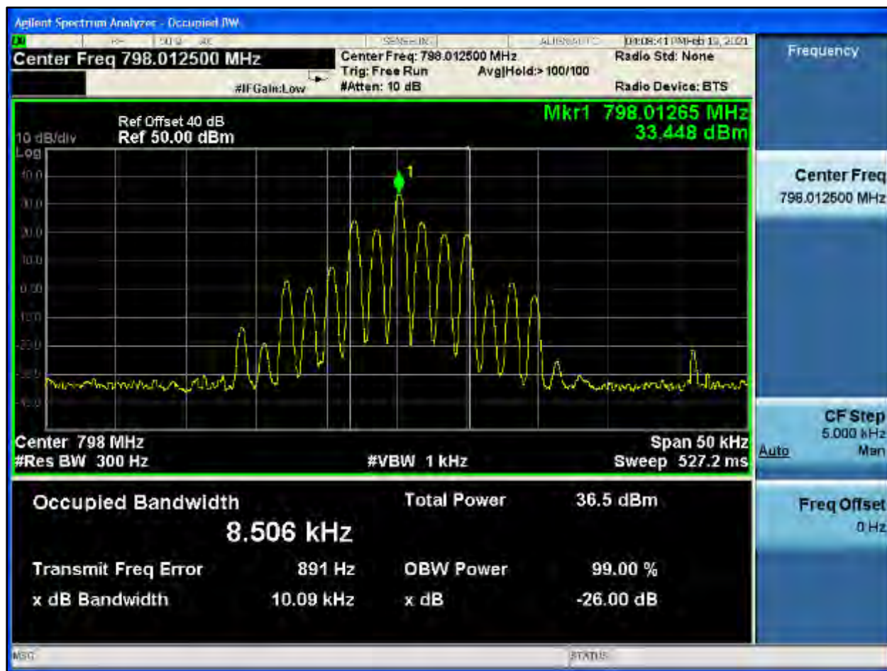
Plot 8-512: OBW 99%, 798.0125 MHz, HVD NPSPAC
