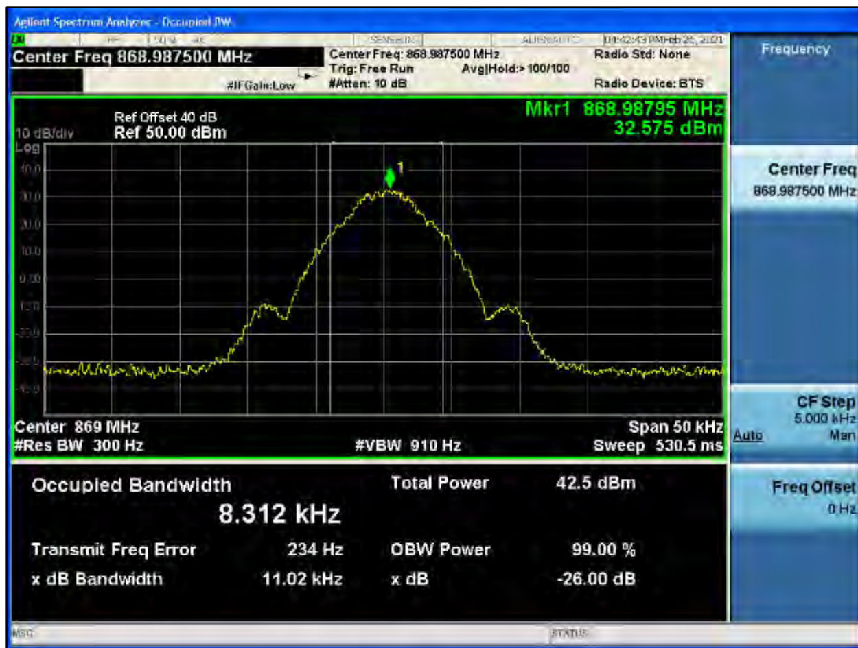
Plot 8-618: OBW 99%, 868.9875 MHz, NB 2 FSK
