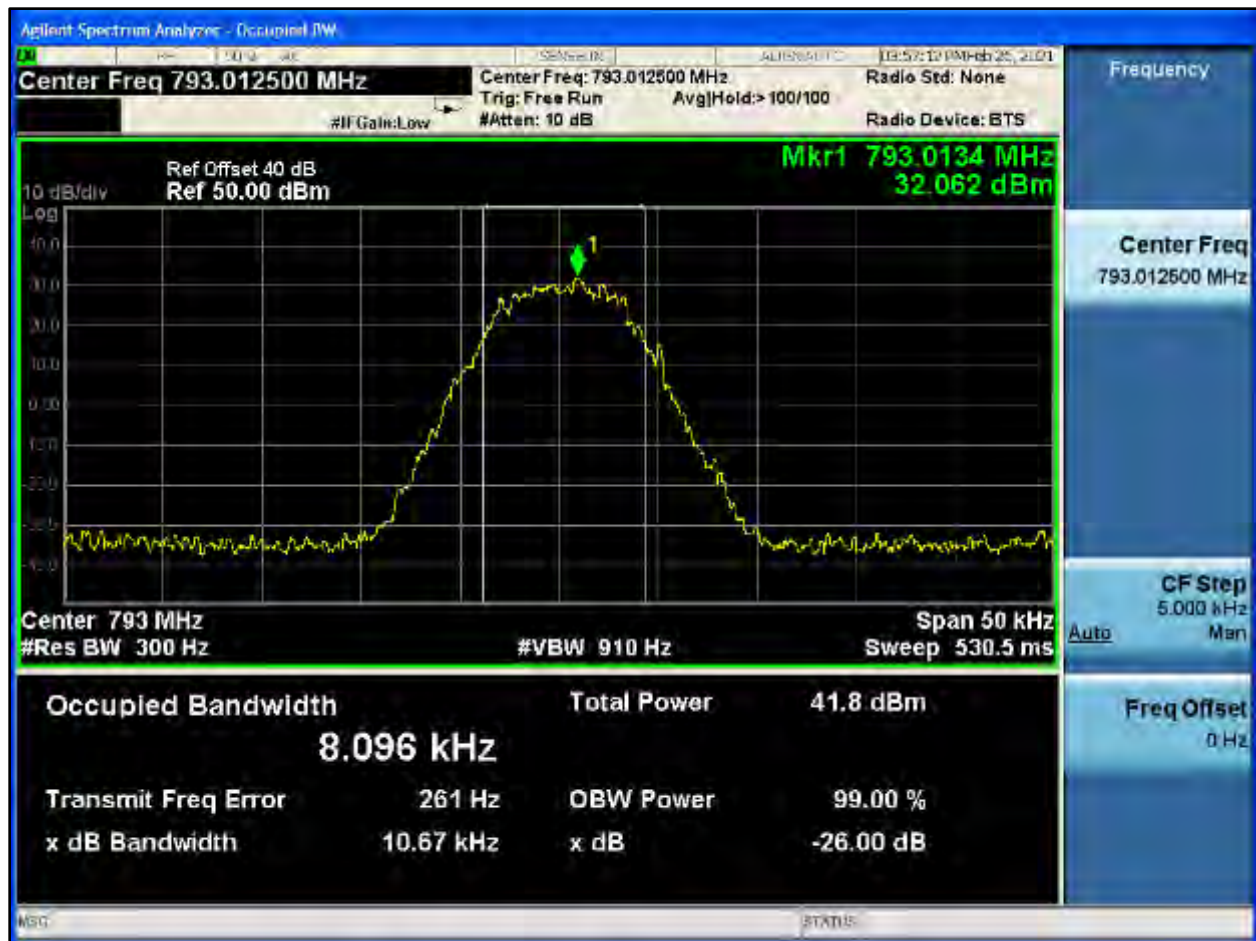
Plot 8-497: OBW 99%, 793.0125 MHz, H-CPM TDMA
