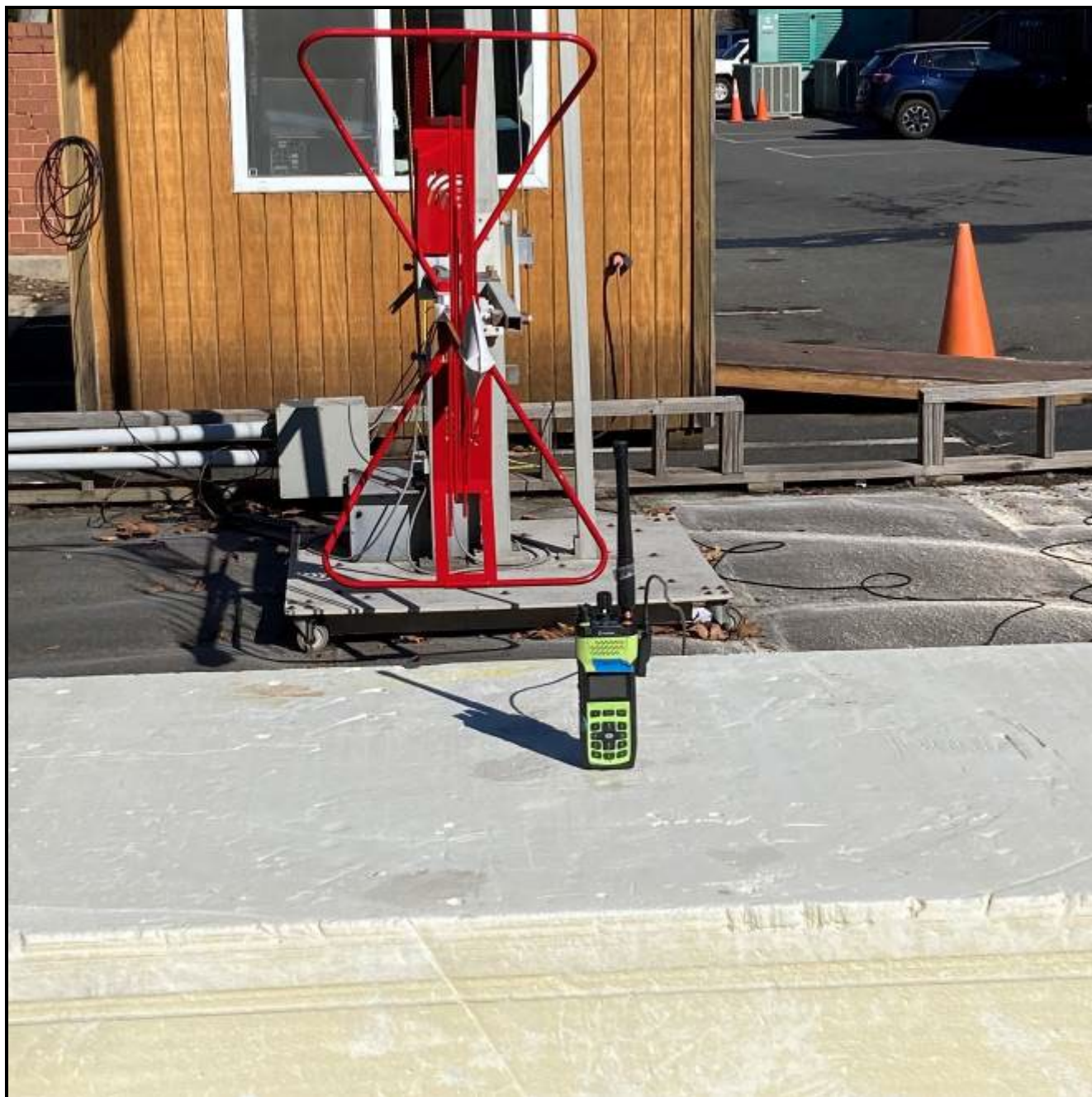
Photograph 3: Radiated Emissions (Spurious/Harmonics) Under 1 GHz, Front View
