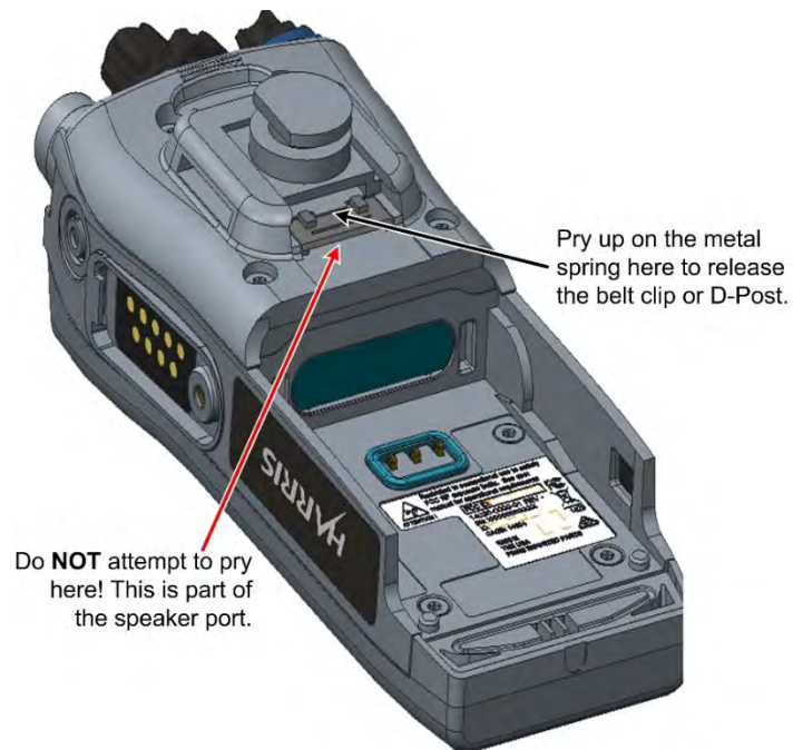
Figure 4-3: Remove Belt Clip
