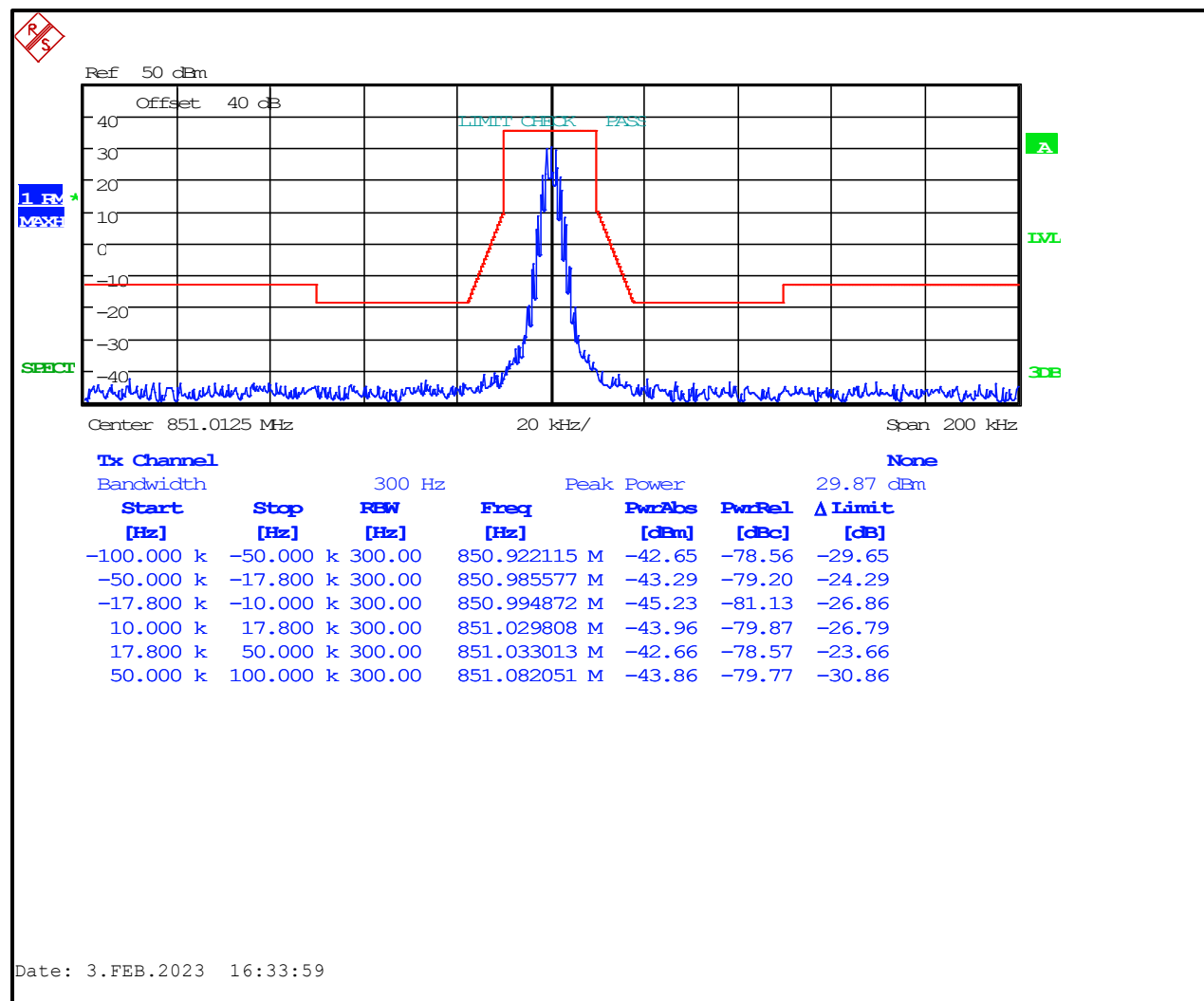
Plot 4-7: Occupied Bandwidth – HVD-NSPPAC; 851.0125 MHz; Mask G (ISED)
