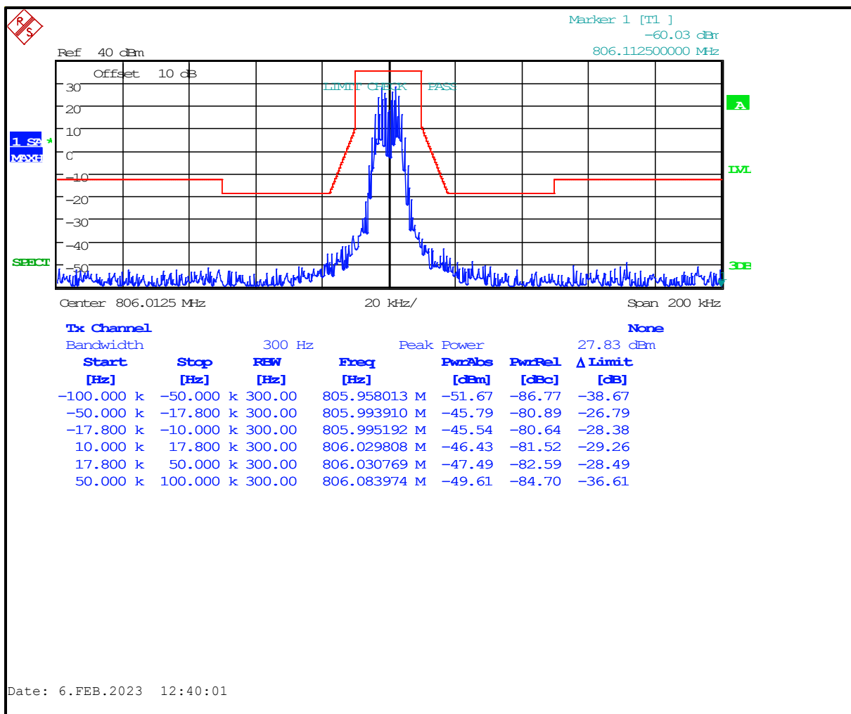
Plot 4-3: Occupied Bandwidth – HVD-SMR; 806.0125 MHz; Mask G (ISED)
