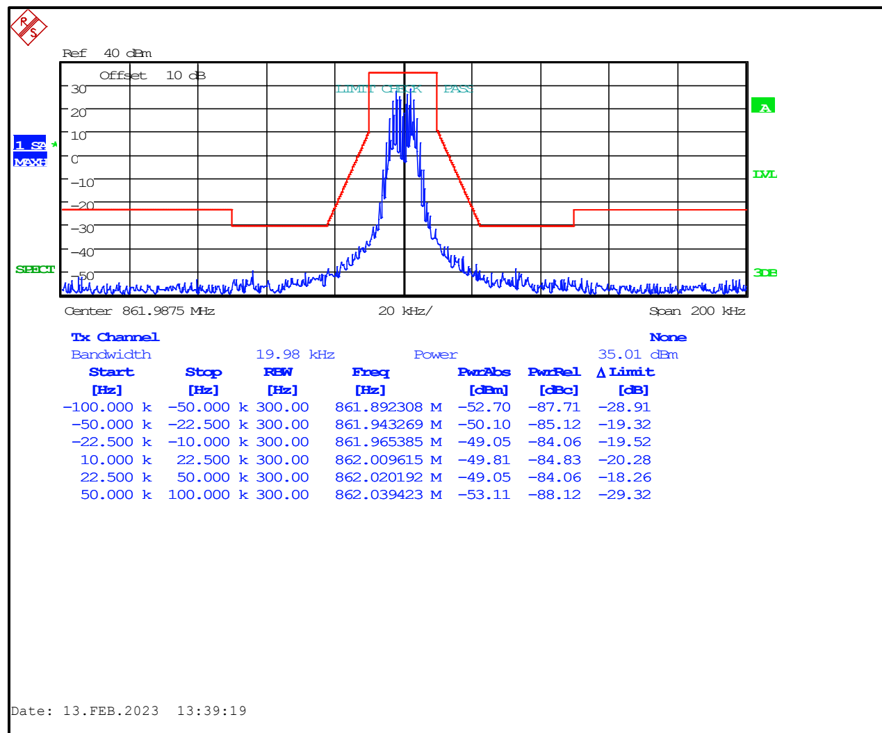
Plot 4-10: Occupied Bandwidth – HVD-SMR; 861.9875 MHz; Mask G (FCC/ISED)
