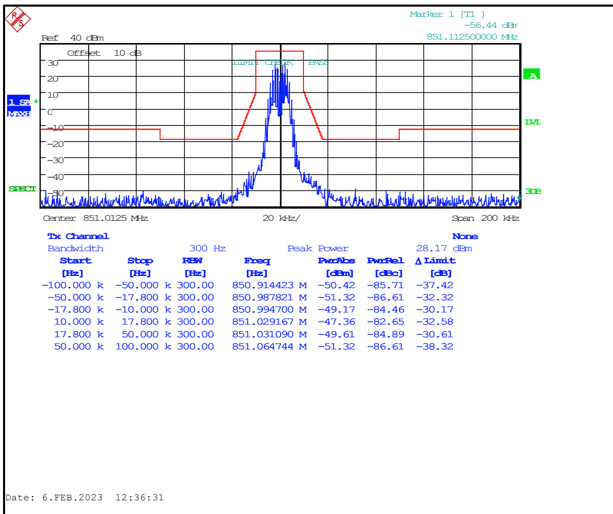
Plot 4-8: Occupied Bandwidth – HVD-SMR; 851.0125 MHz; Mask G (ISED)
