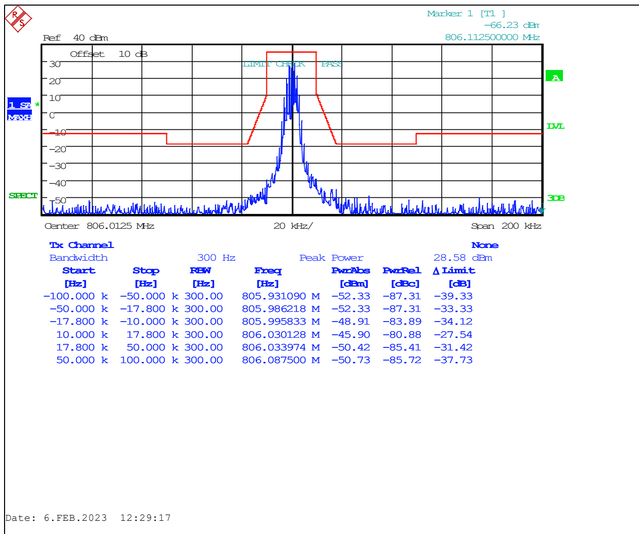
Plot 4-2: Occupied Bandwidth – HVD-NPSPAC; 806.0125 MHz; Mask G (ISED)
