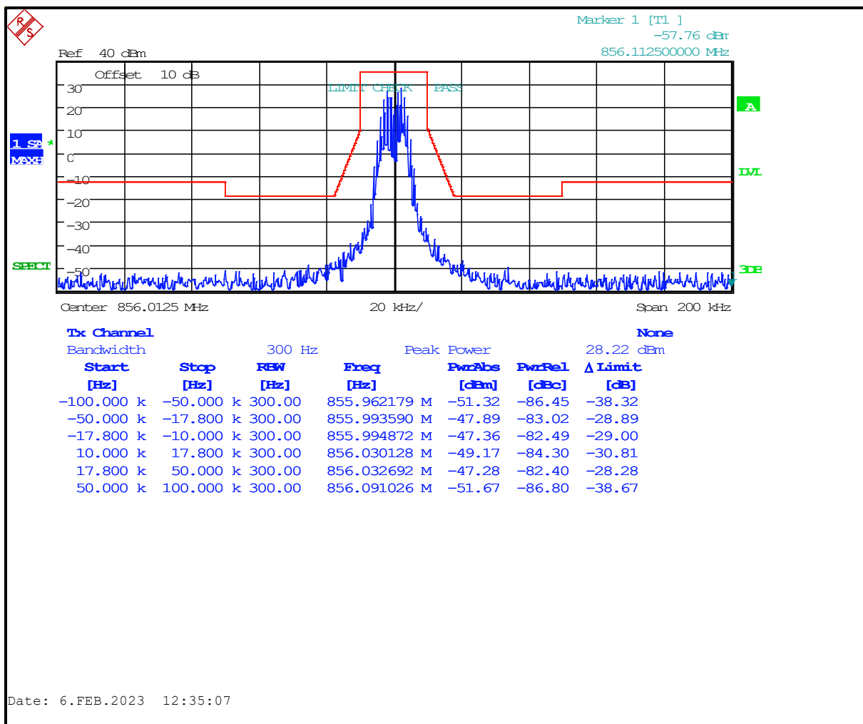
Plot 4-9: Occupied Bandwidth – HVD-SMR; 856.0125 MHz; Mask G (FCC/ISED)
