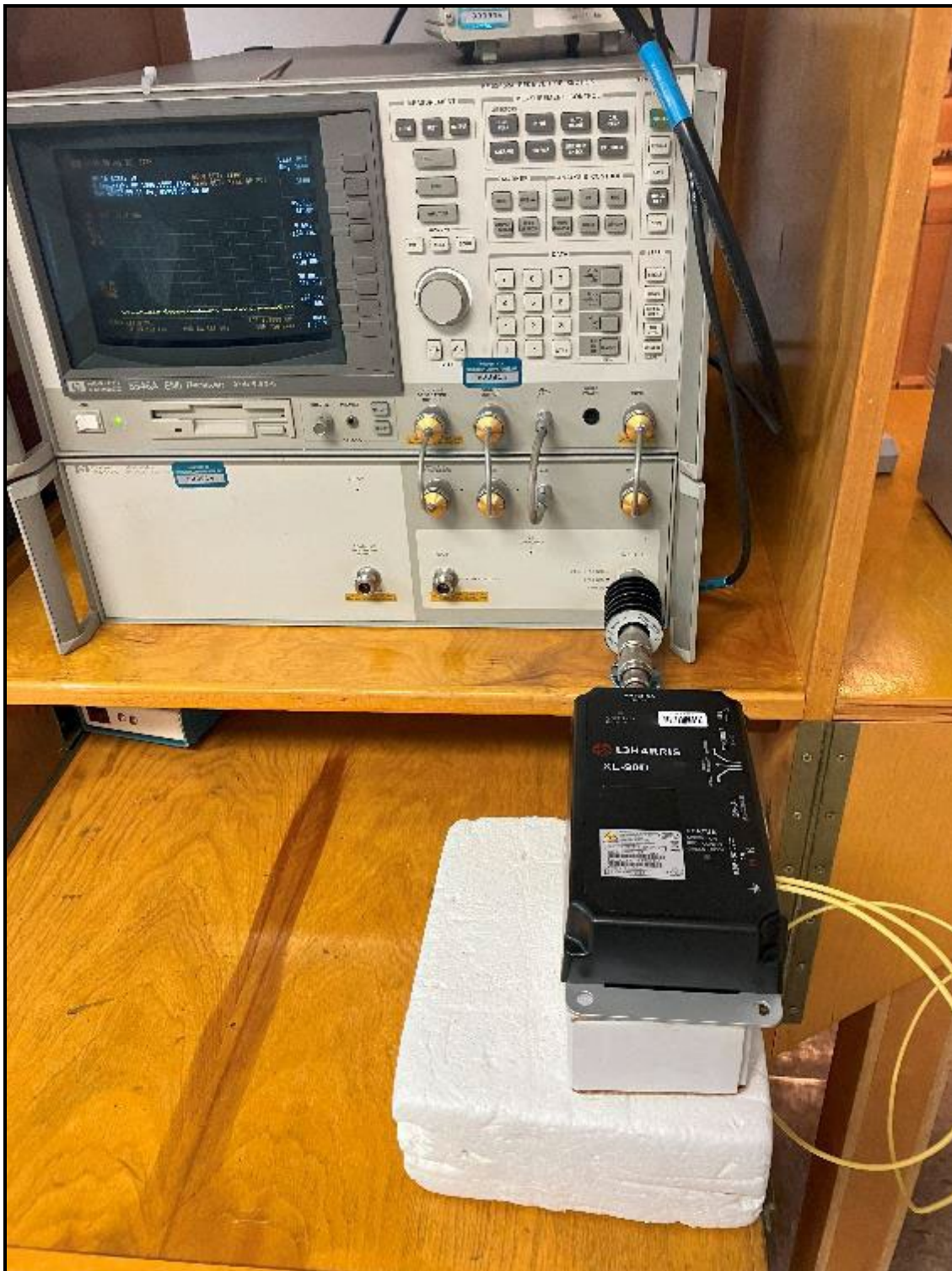
Photograph 5: Conducted Antenna Port Emissions
