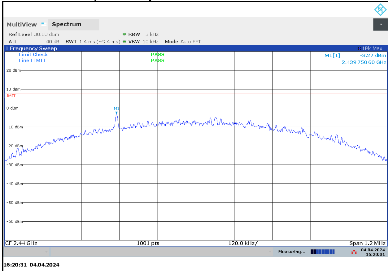
Plot 7-2: Power Spectral Density – 2440 MHz
