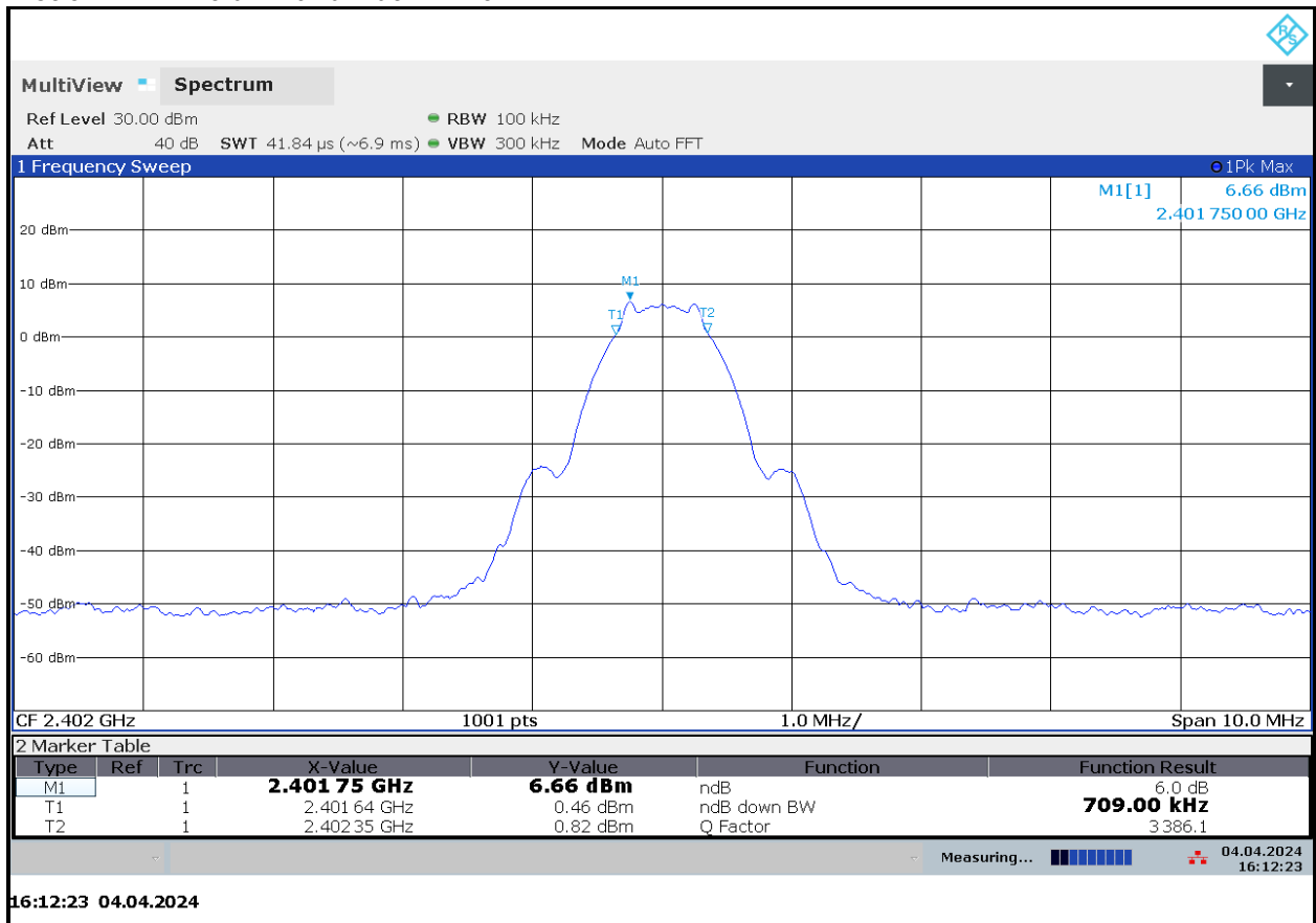
Plot 6-1: 6 dB Bandwidth – 2402 MHz
