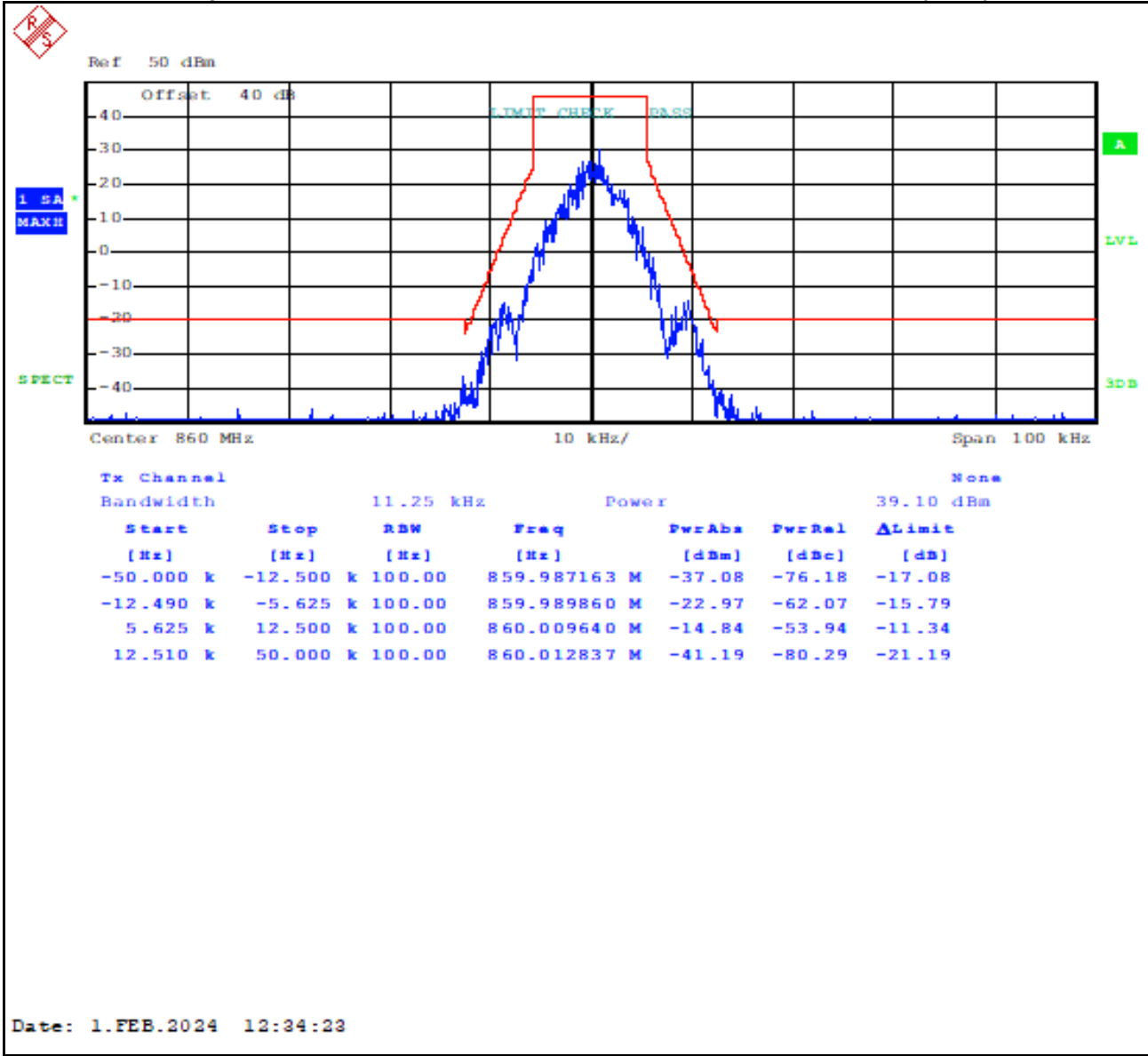
Plot 8-51: Occupied Bandwidth – 860.0000 MHz; 2-Level FSK 9600 NB; Mask D (ISED)
