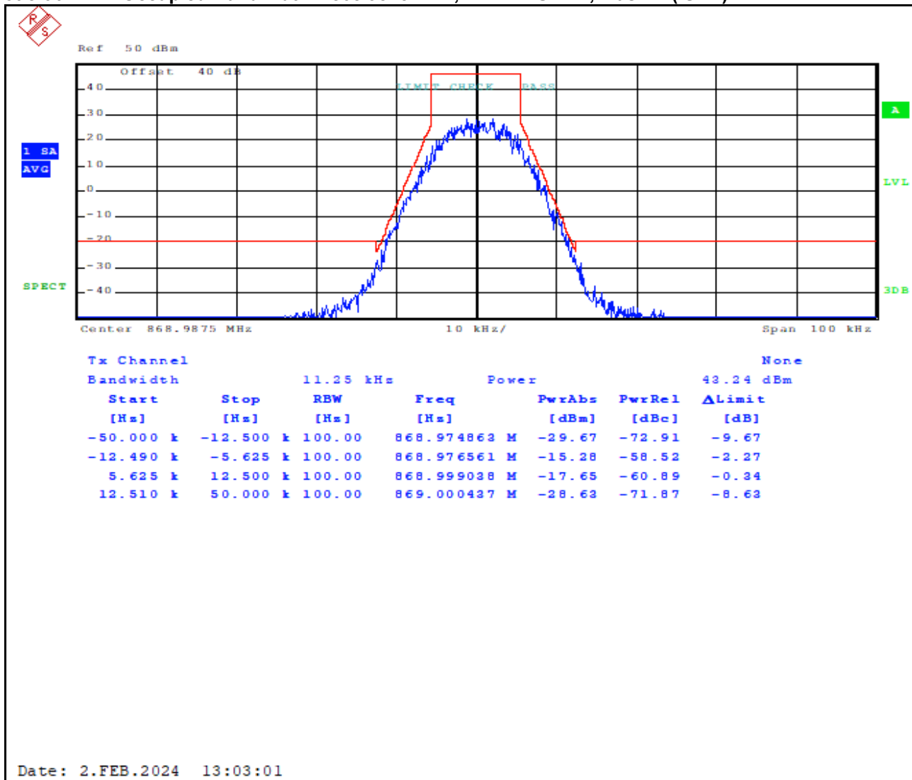
Plot 8-96: Occupied Bandwidth – 868.9875 MHz; HVD NPSPAC; Mask D (ISED)
