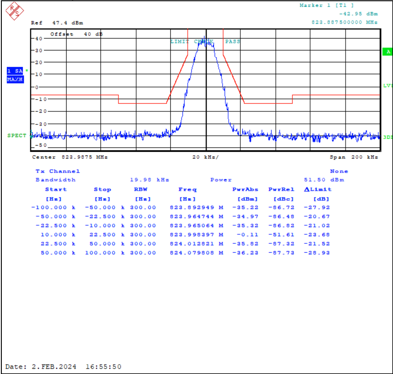
Plot 8-86: Occupied Bandwidth – 823.9875 MHz; HVD NPSPAC; Mask G
