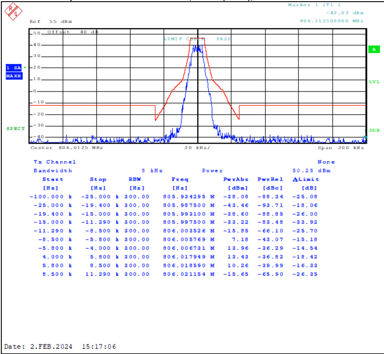
Plot 8-65: Occupied Bandwidth – 806.0125 MHz; H-CPM (TDMA); Mask H
