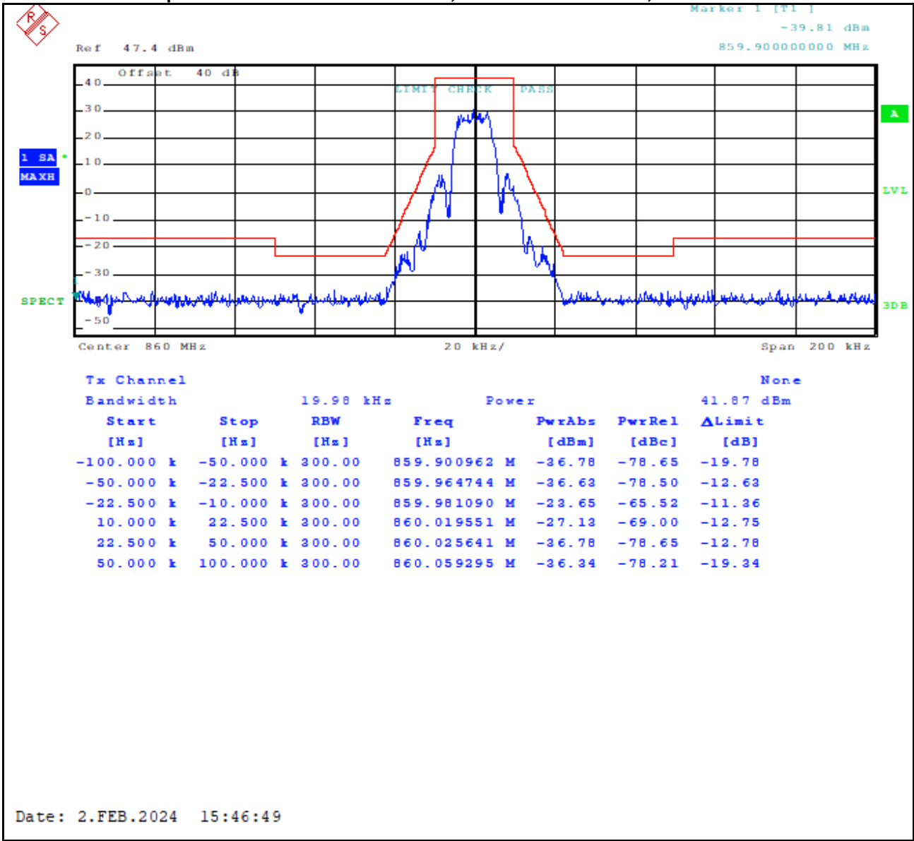
Plot 8-13: Occupied Bandwidth – 860.0000 MHz; WB 2-level FSK 9600; Mask G
