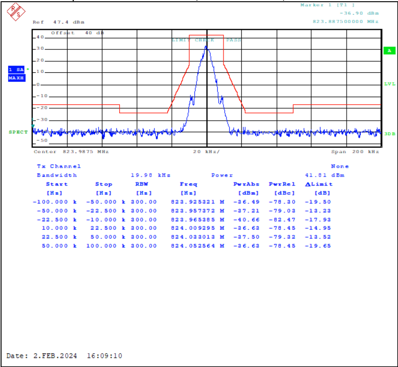
Plot 8-43: Occupied Bandwidth – 823.9875 MHz; 2-Level FSK 9600 NB; Mask G
