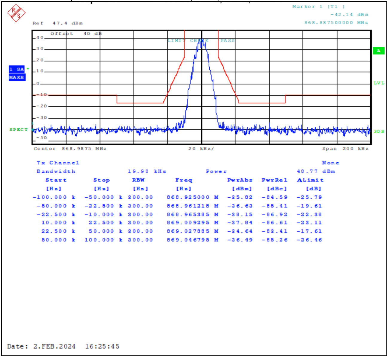
Plot 8-58: Occupied Bandwidth – 868.9875 MHz; C4FM; Mask G
