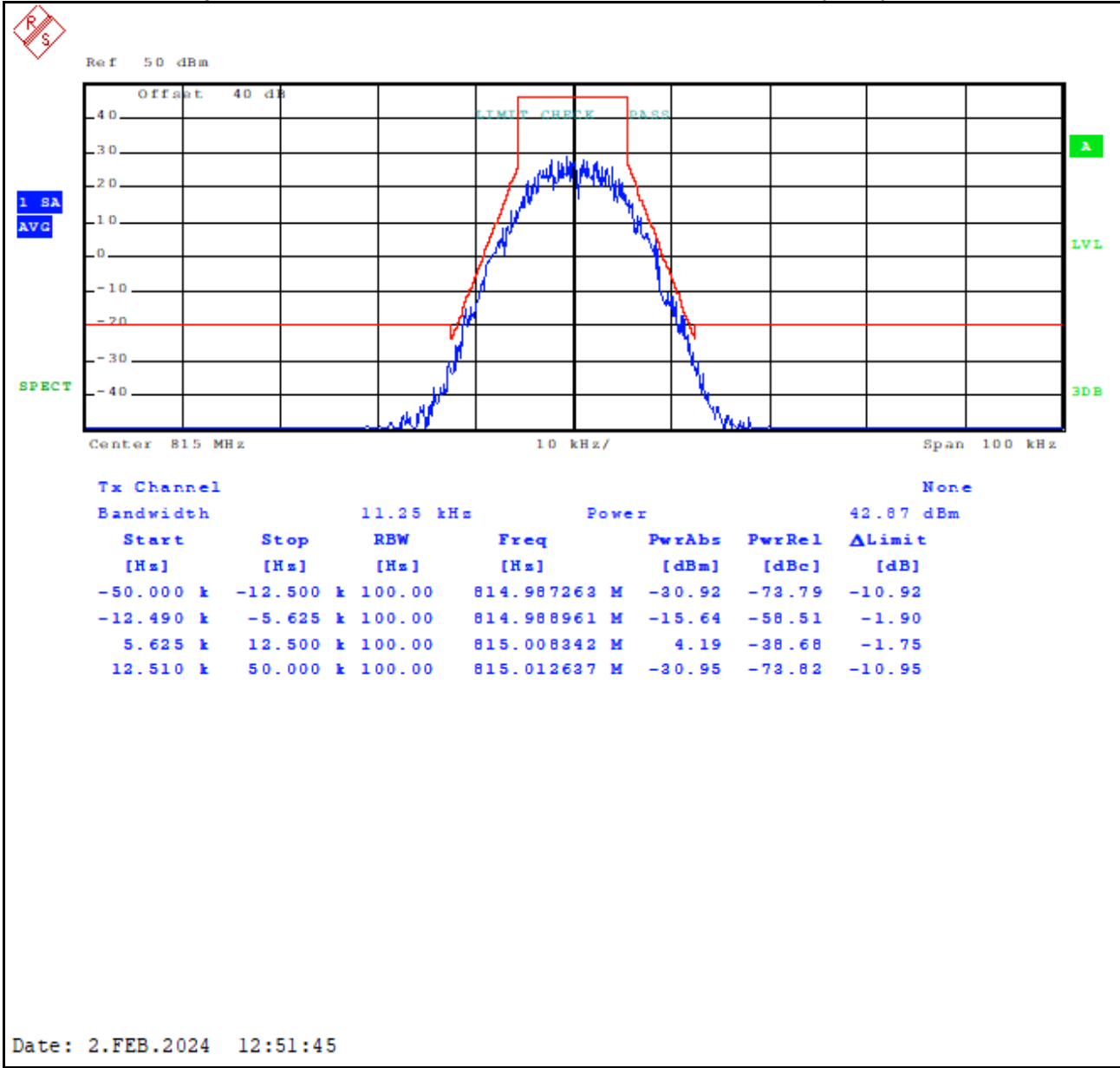
Plot 8-92: Occupied Bandwidth – 815.0000 MHz; HVD NPSPAC; Mask D (ISED)
