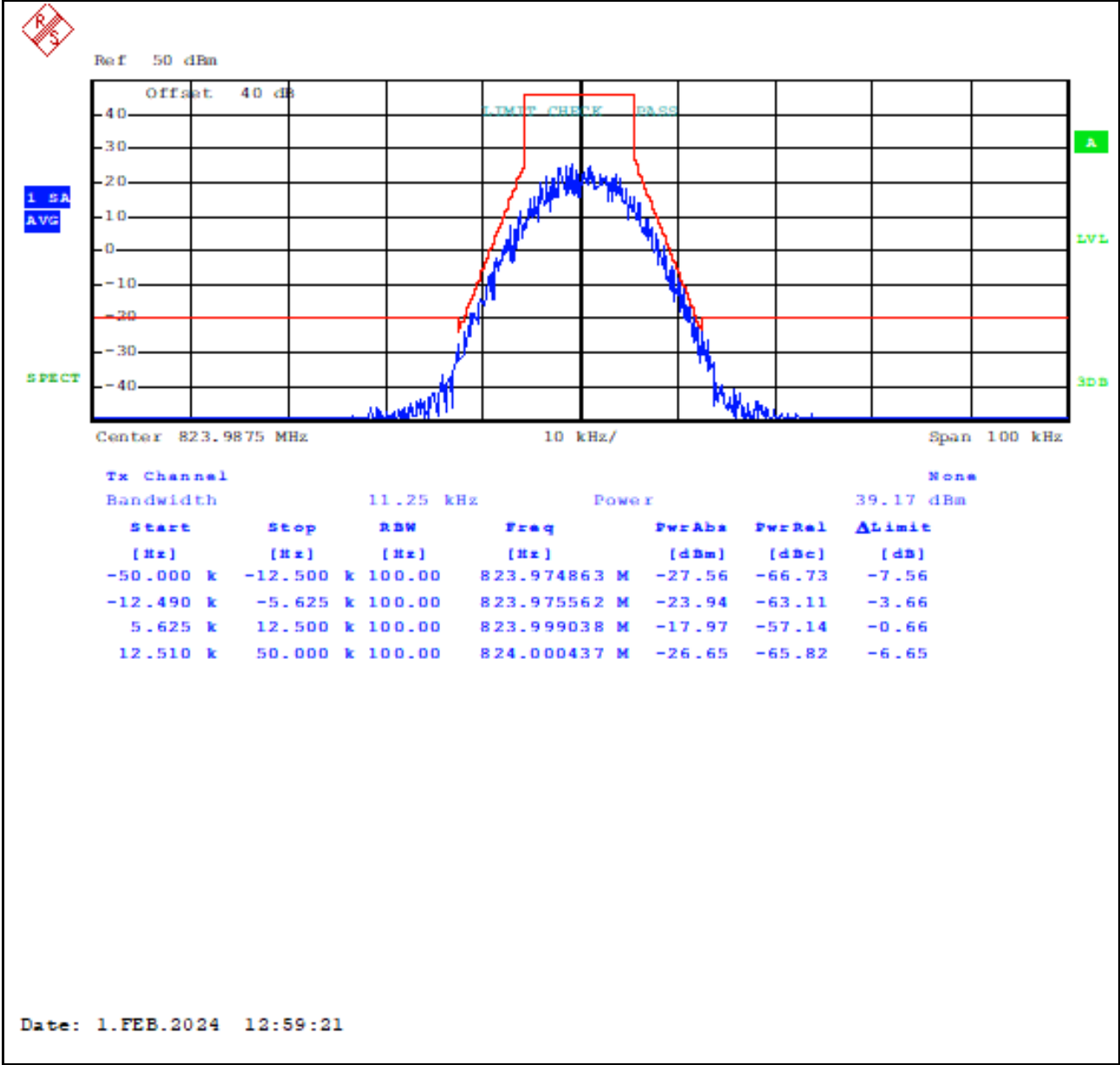
Plot 8-93: Occupied Bandwidth – 823.9875 MHz; HVD NPSPAC; Mask D (ISED)
