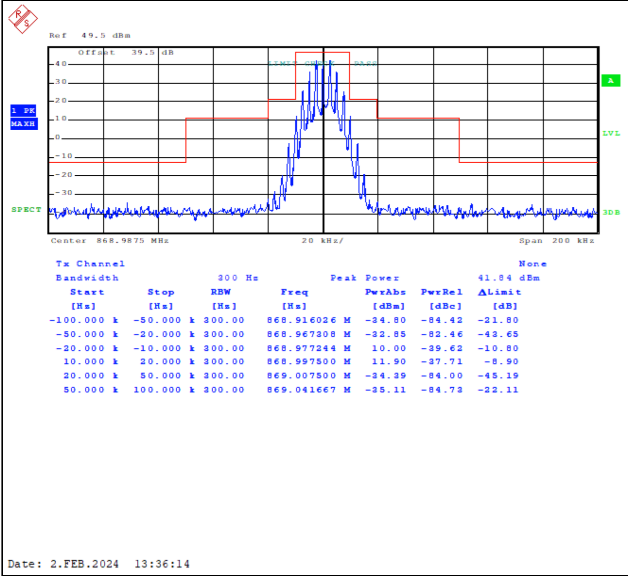
Plot 8-6: Occupied Bandwidth – 868.9875 MHz; WB Analog; Mask B
