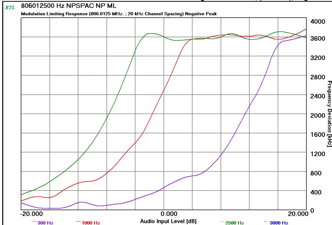
Plot 10-8: Modulation Characteristics – Modulation Limiting – 806.0125 MHz; (NPSPAC); Negative Peak
