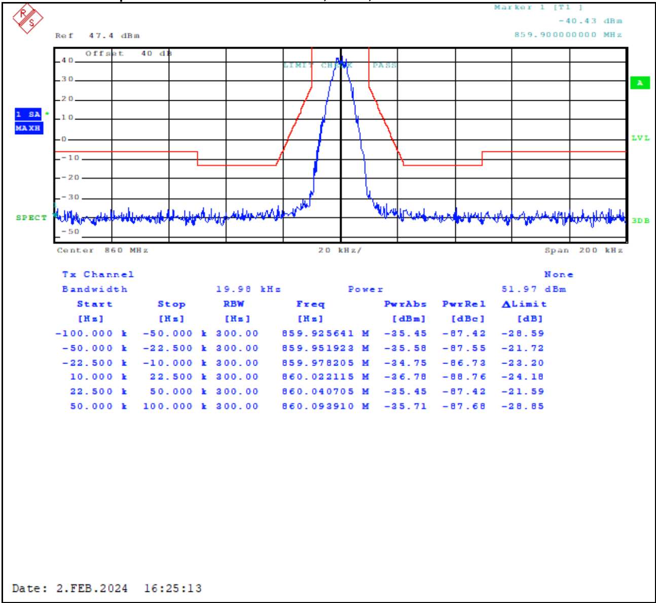
Plot 8-57: Occupied Bandwidth – 860.0000 MHz; C4FM; Mask G
