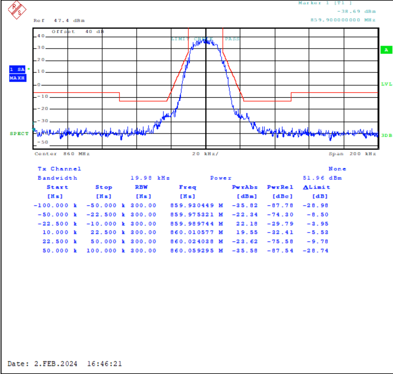
Plot 8-81: Occupied Bandwidth – 860.0000 MHz; HVD SMR; Mask G
