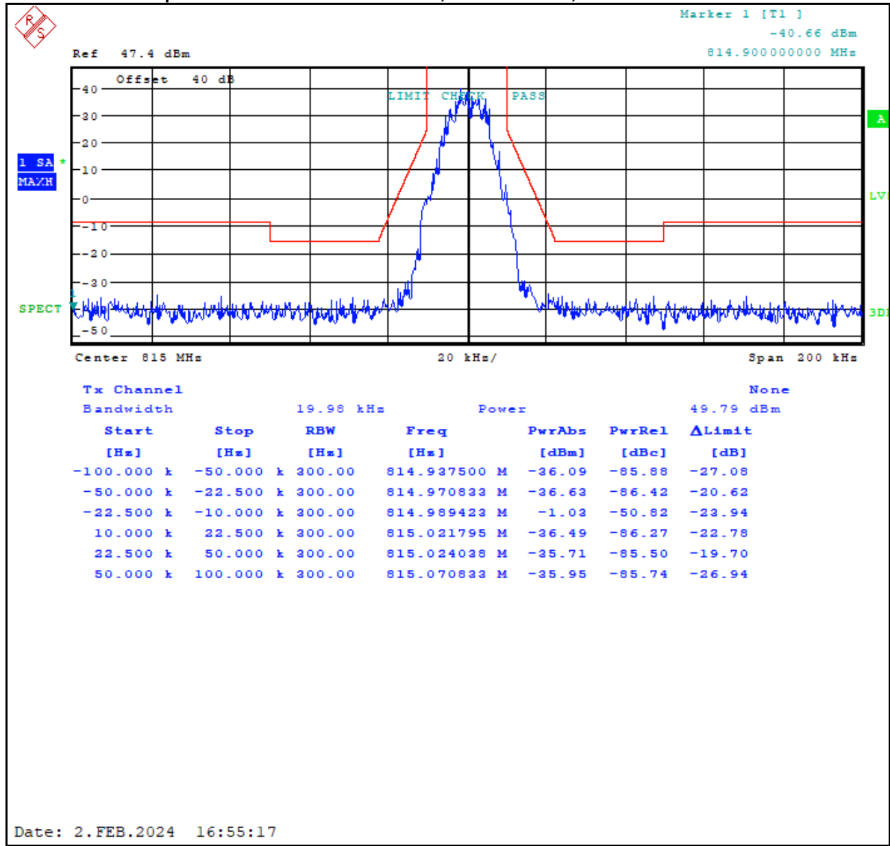
Plot 8-85: Occupied Bandwidth – 815.0000 MHz; HVD NPSPAC; Mask G
