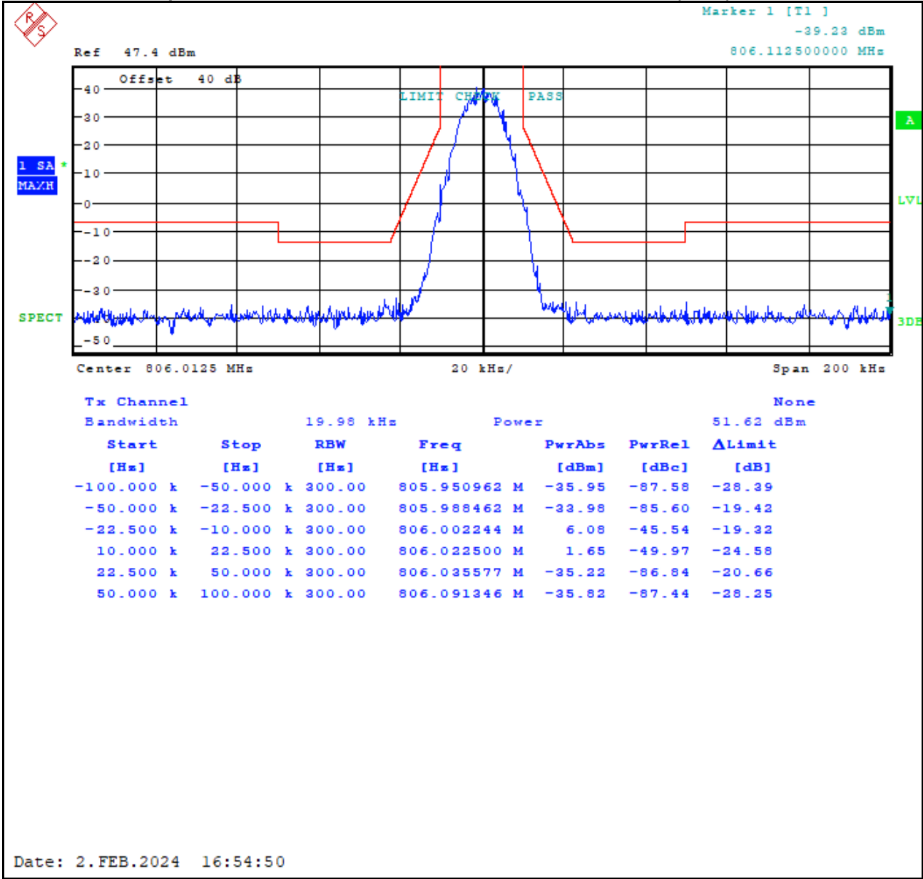
Plot 8-84: Occupied Bandwidth – 806.0125 MHz; HVD NPSPAC; Mask G (ISED)
