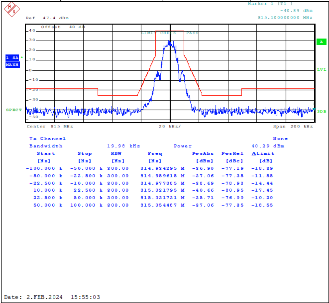
Plot 8-23: Occupied Bandwidth – 815.0000 MHz; 2-level FSK 9600 NPSPAC; Mask G
