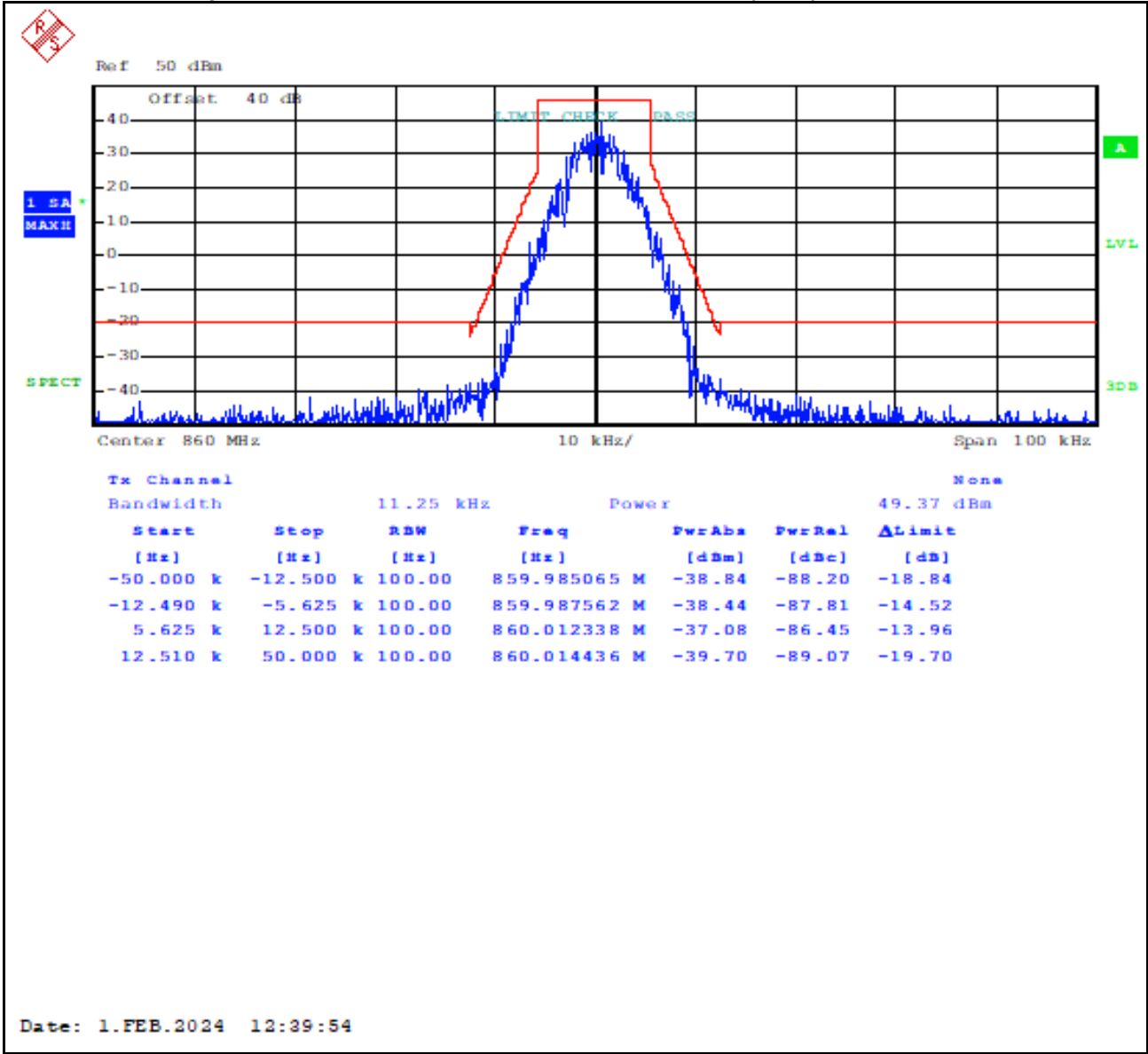
Plot 8-63: Occupied Bandwidth – 860.0000 MHz; C4FM; Mask D (ISED)
