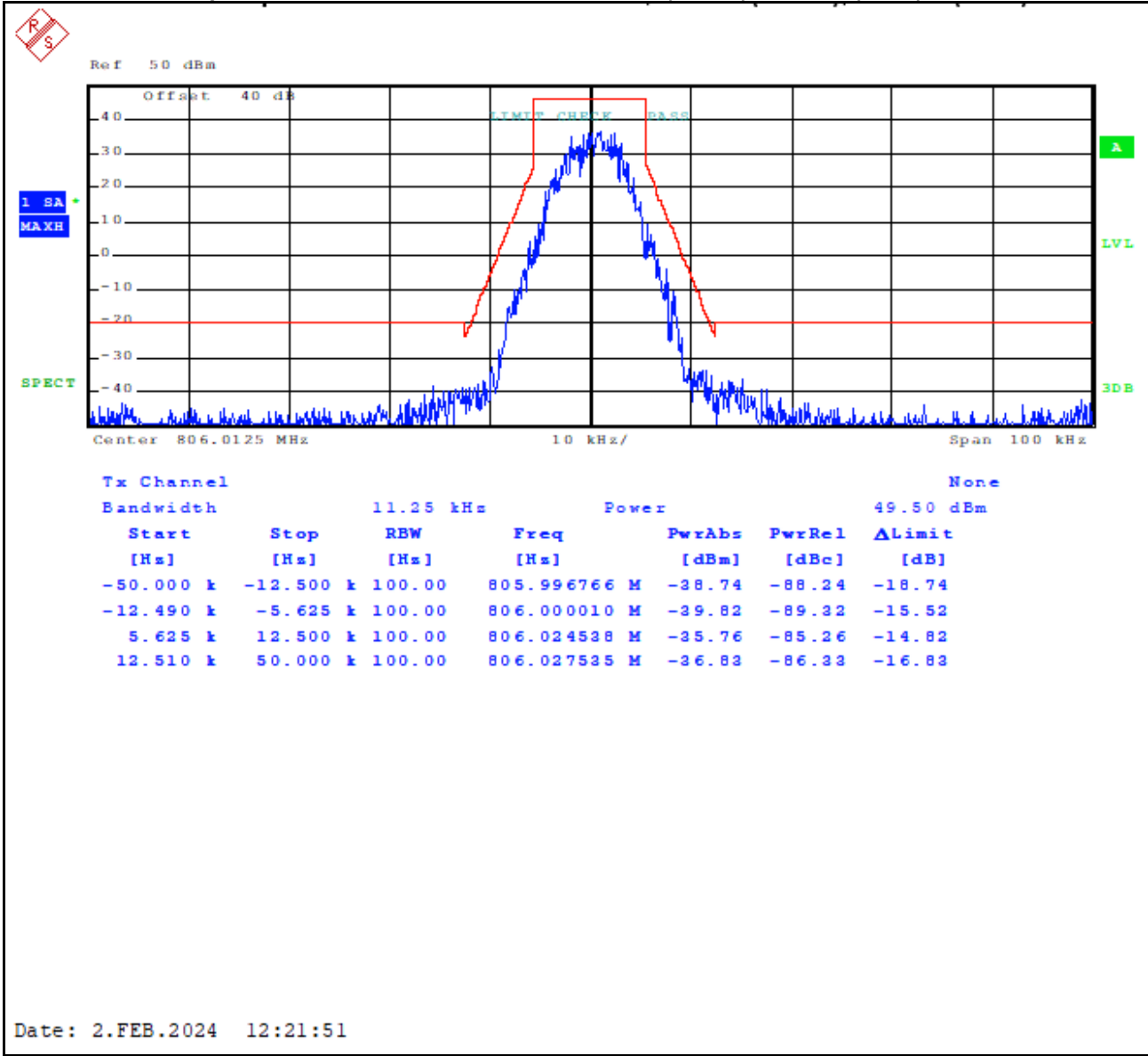
Plot 8-71: Occupied Bandwidth – 806.0125 MHz; H-CPM (TDMA); Mask D (ISED)
