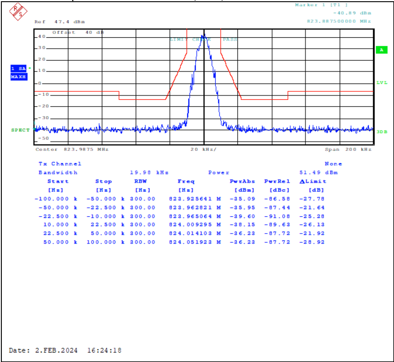
Plot 8-55: Occupied Bandwidth – 823.9875 MHz; C4FM; Mask G
