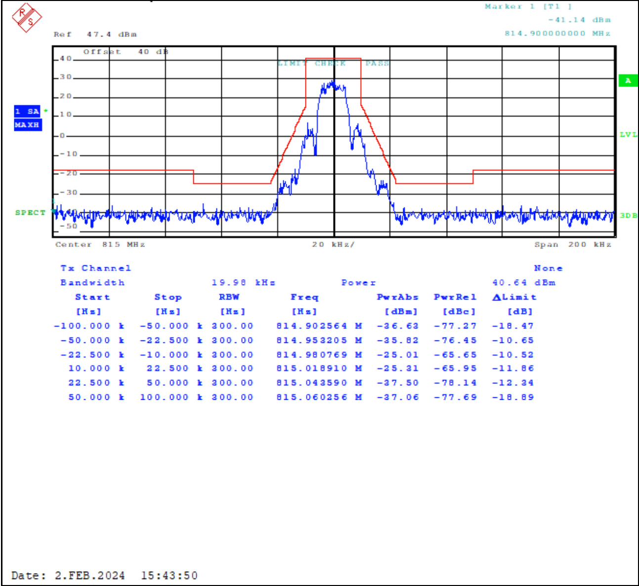
Plot 8-9: Occupied Bandwidth – 815.0000 MHz; WB 2-level FSK 9600; Mask G
