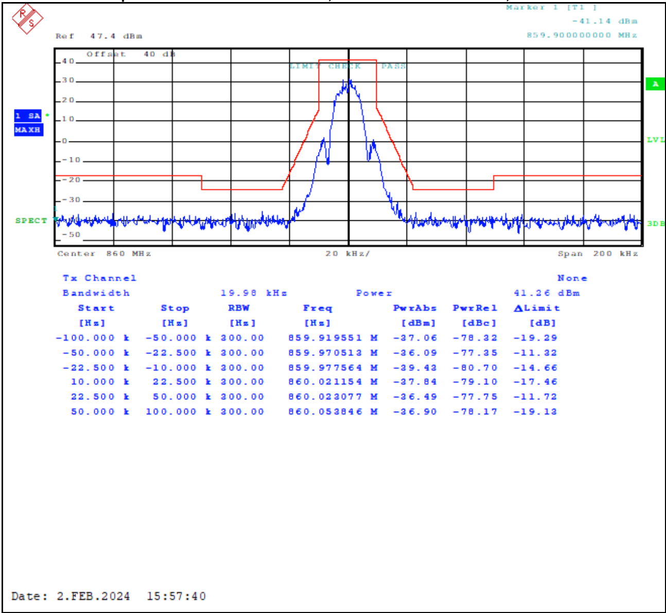
Plot 8-27: Occupied Bandwidth – 860.0000 MHz; 2-level FSK 9600 NPSPAC; Mask G
