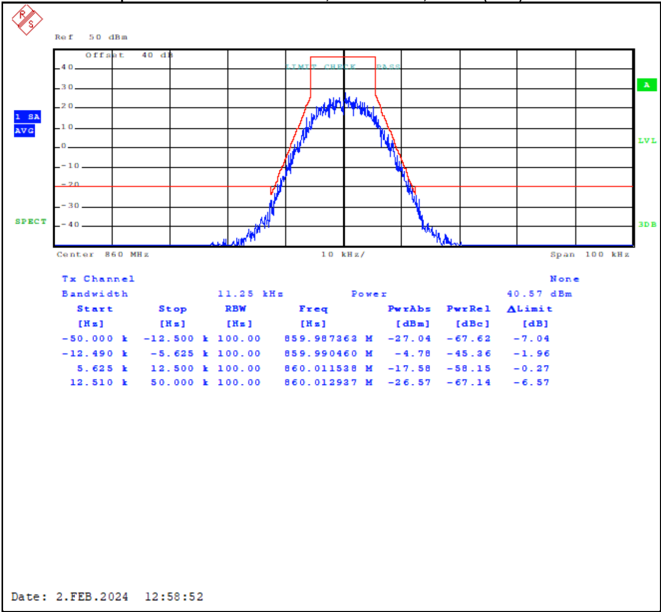
Plot 8-95: Occupied Bandwidth – 860.0000 MHz; HVD NPSPAC; Mask D (ISED)
