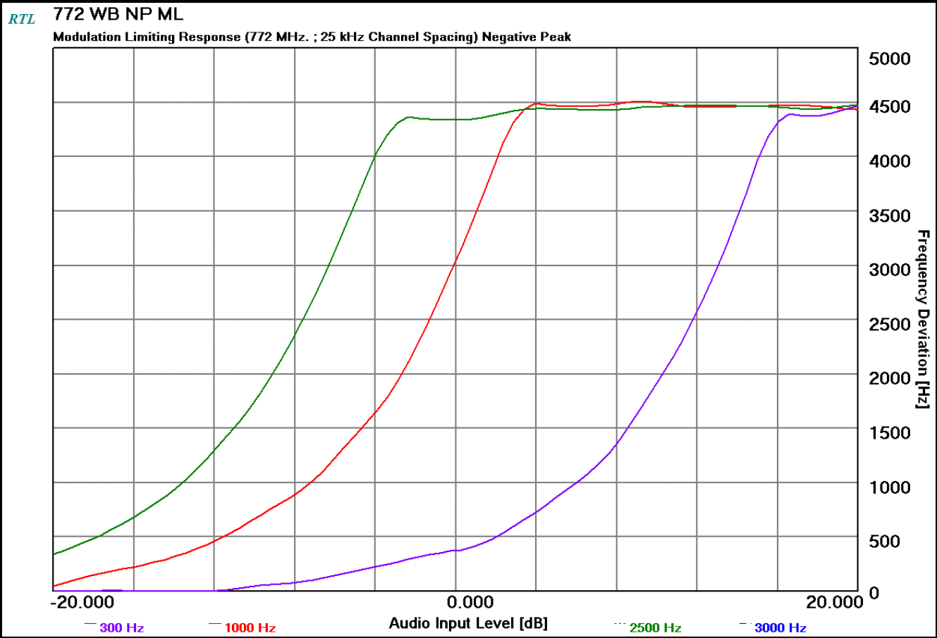
Plot 10-6: Modulation Characteristics – Modulation Limiting - 772.0000 MHz; (WB) Negative Peak
