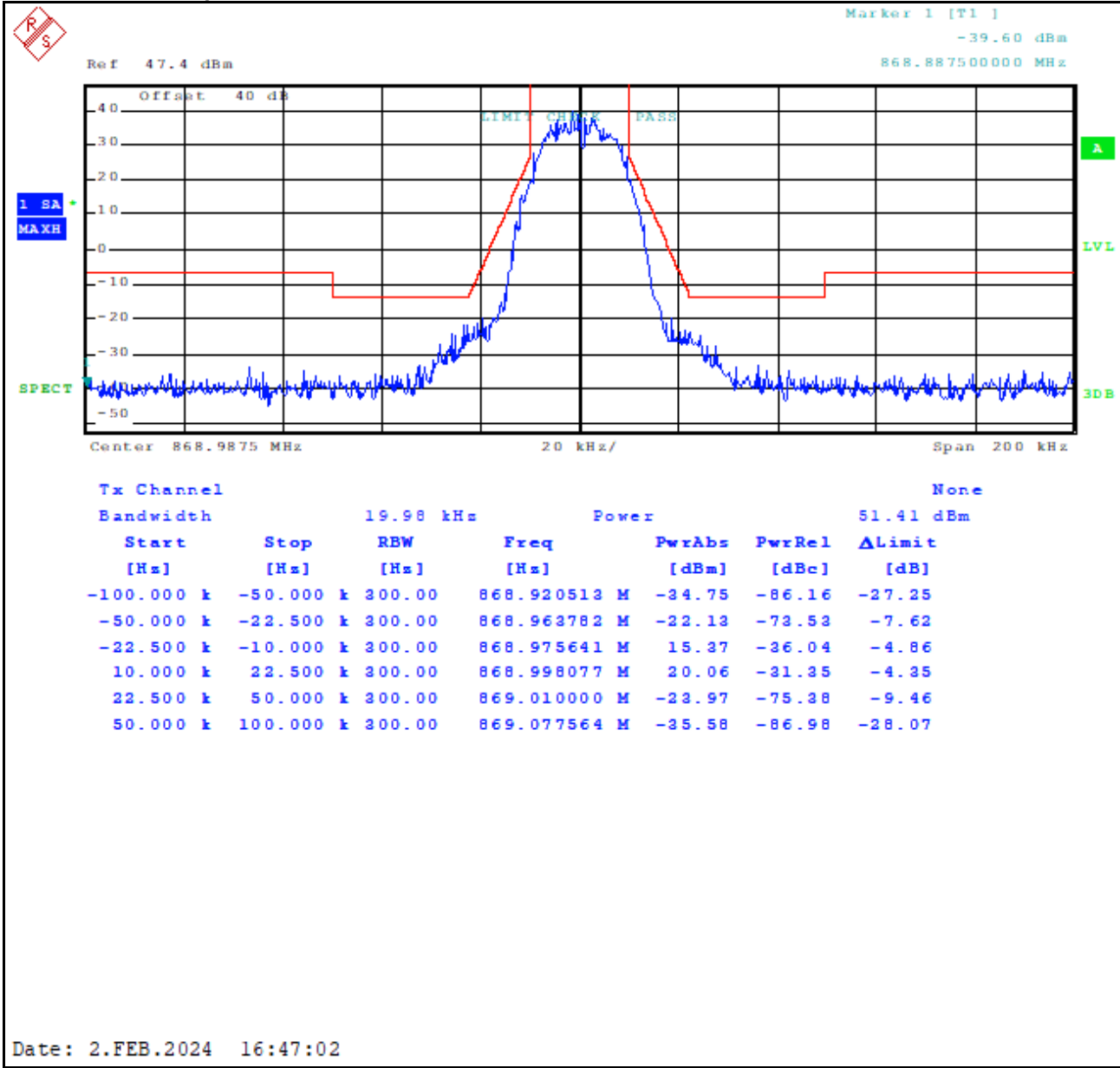
Plot 8-82: Occupied Bandwidth – 868.9875 MHz; HVD SMR; Mask G
