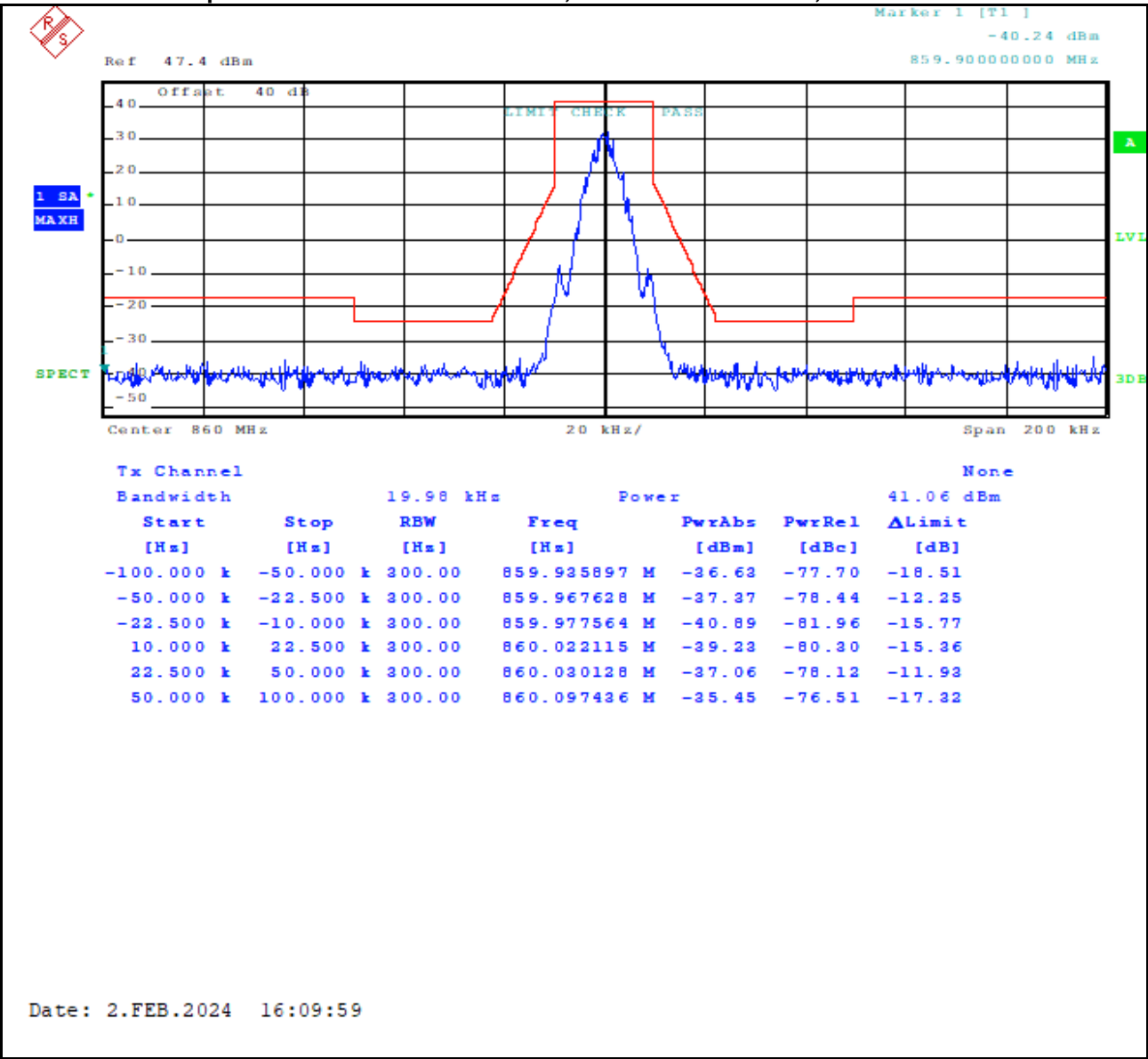
Plot 8-45: Occupied Bandwidth – 860.0000 MHz; 2-Level FSK 9600 NB; Mask G
