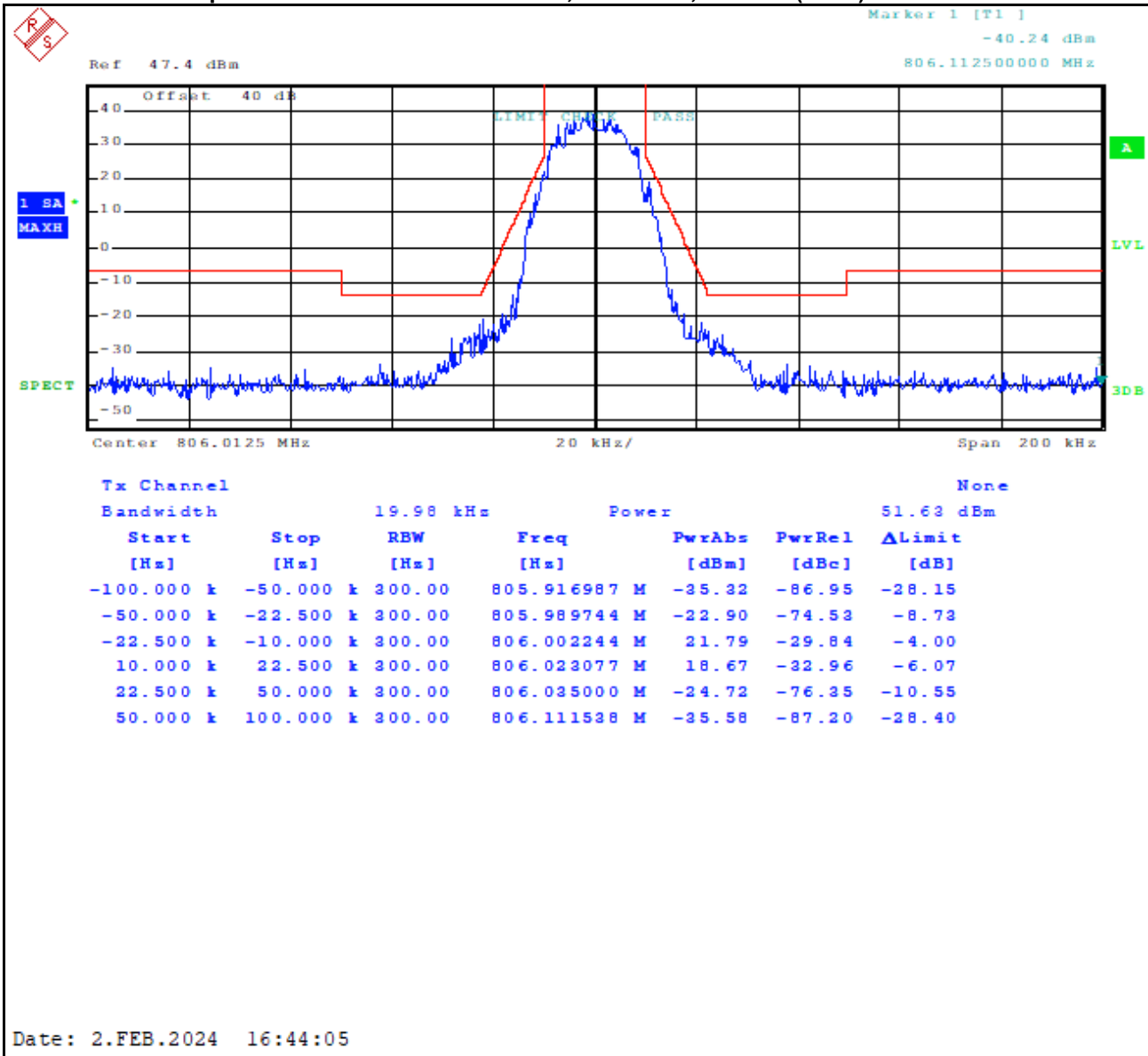
Plot 8-77: Occupied Bandwidth – 806.0125 MHz; HVD SMR; Mask G (ISED)
