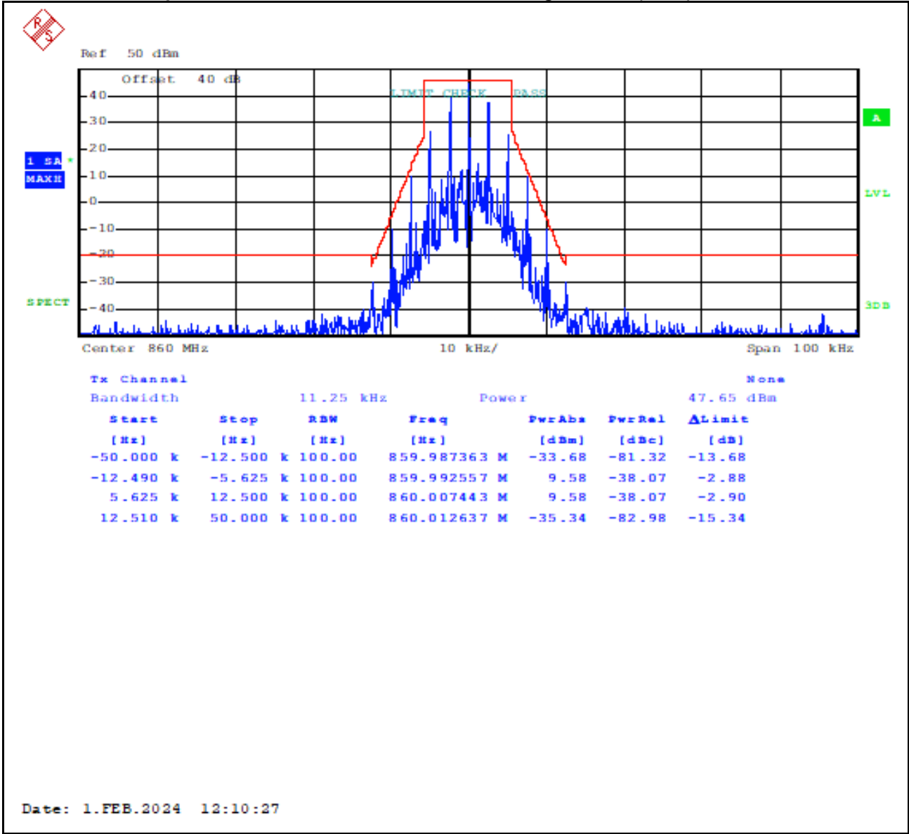
Plot 8-39: Occupied Bandwidth – 860.0000 MHz; NB Analog; Mask D (ISED)
