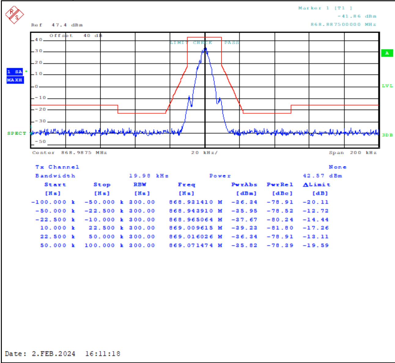
Plot 8-46: Occupied Bandwidth – 868.9875 MHz; 2-Level FSK 9600 NB; Mask G
