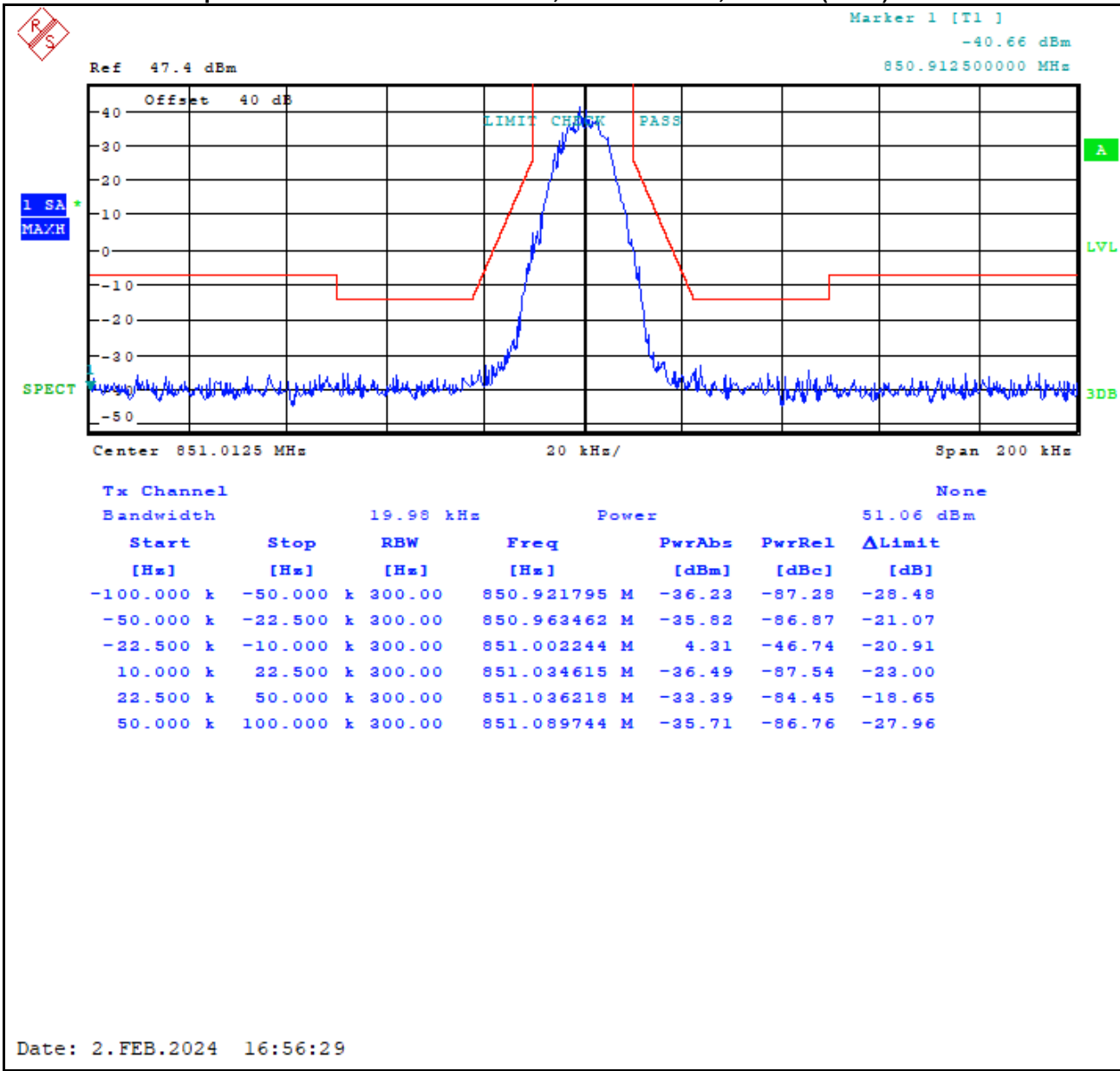
Plot 8-88: Occupied Bandwidth – 851.0125 MHz; HVD NPSPAC; Mask G (ISED)
