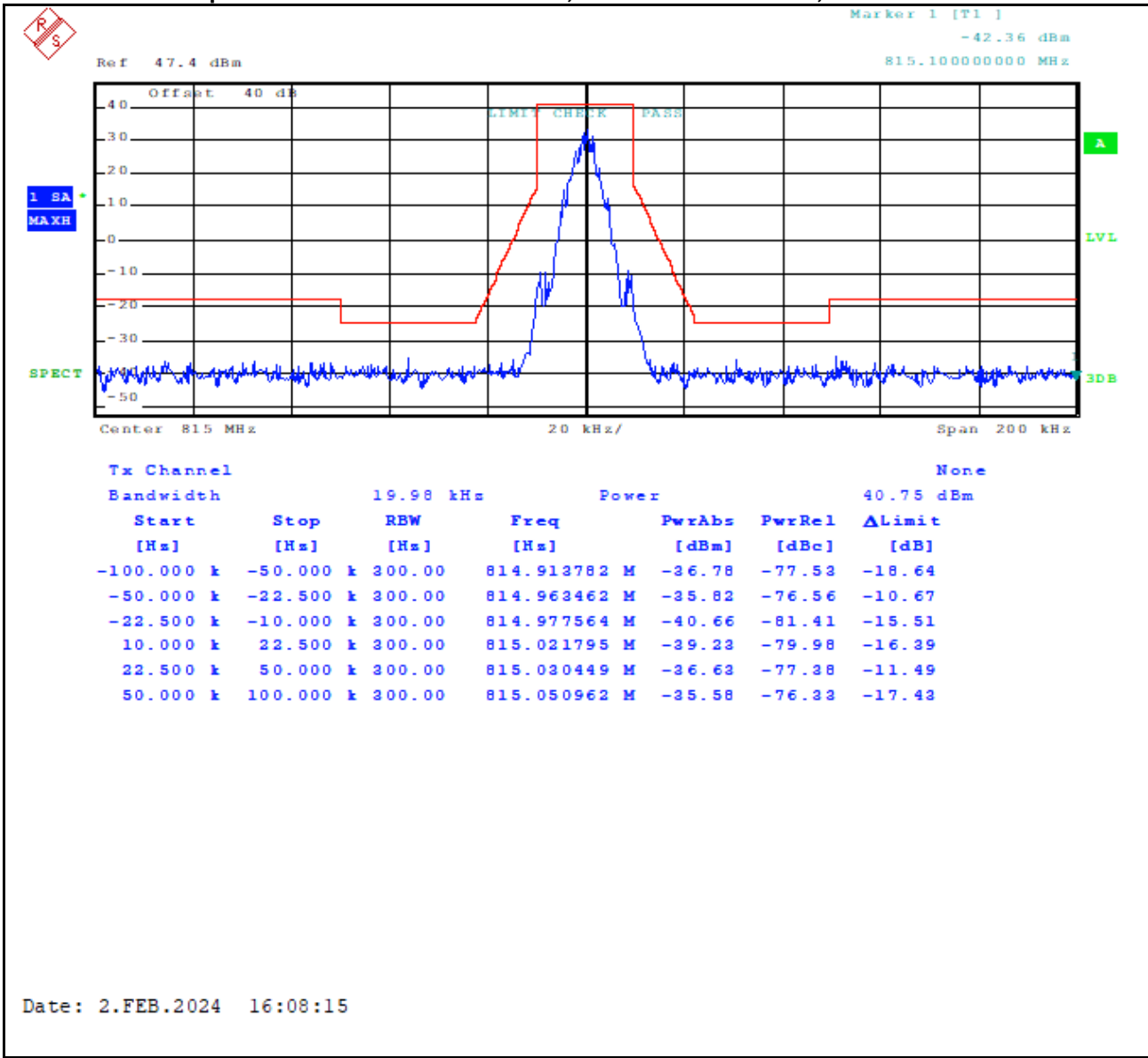
Plot 8-42: Occupied Bandwidth – 815.0000 MHz; 2-Level FSK 9600 NB; Mask G
