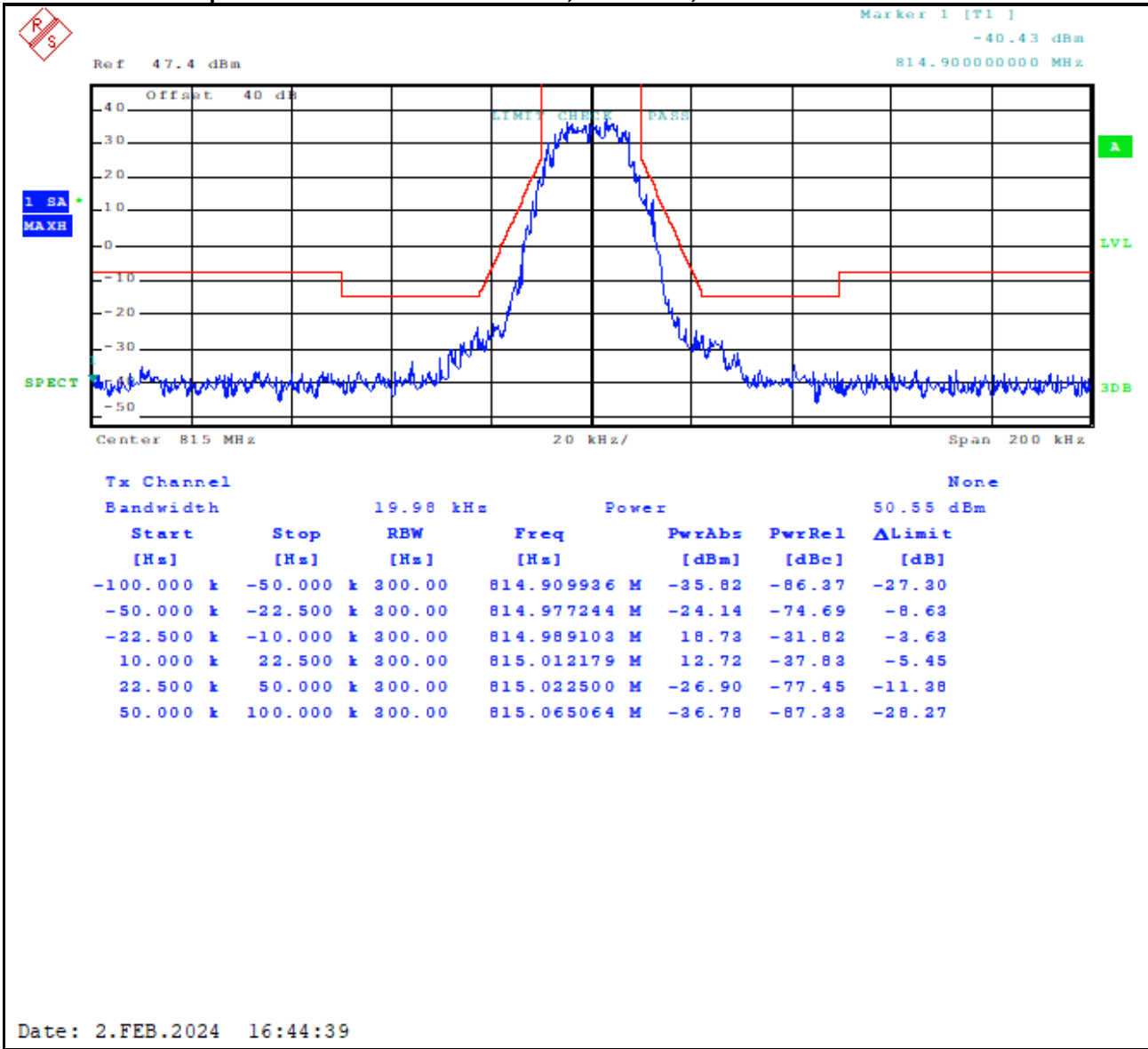
Plot 8-78: Occupied Bandwidth – 815.0000 MHz; HVD SMR; Mask G
