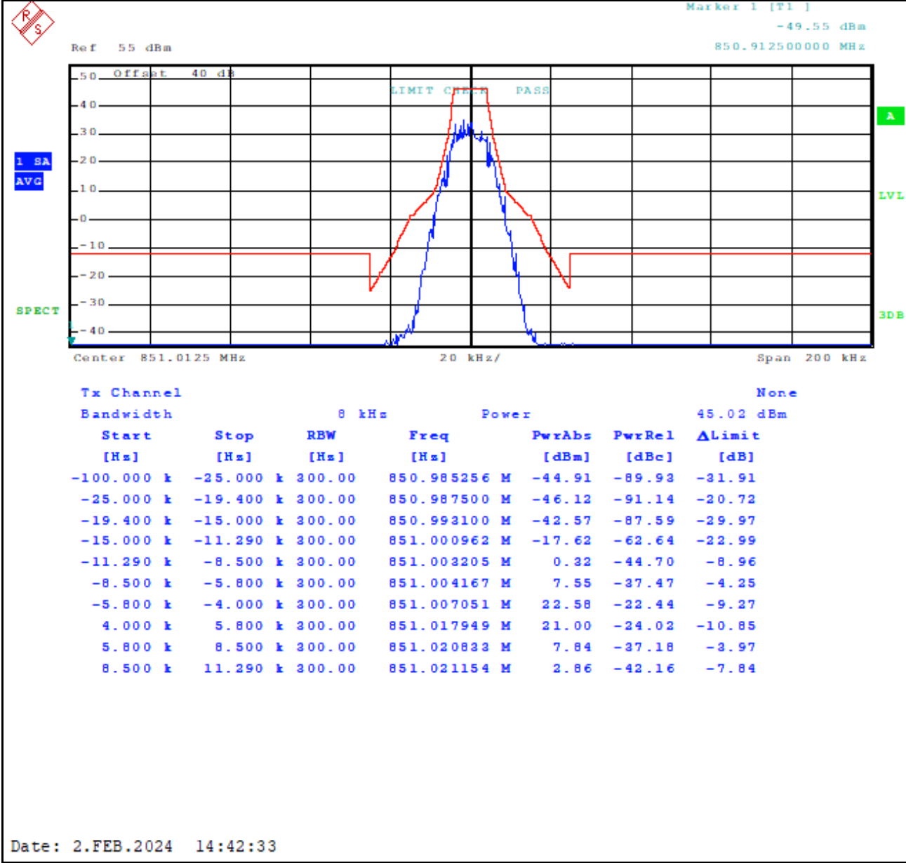
Plot 8-87: Occupied Bandwidth – 851.0125 MHz; HVD NPSPAC; Mask H
