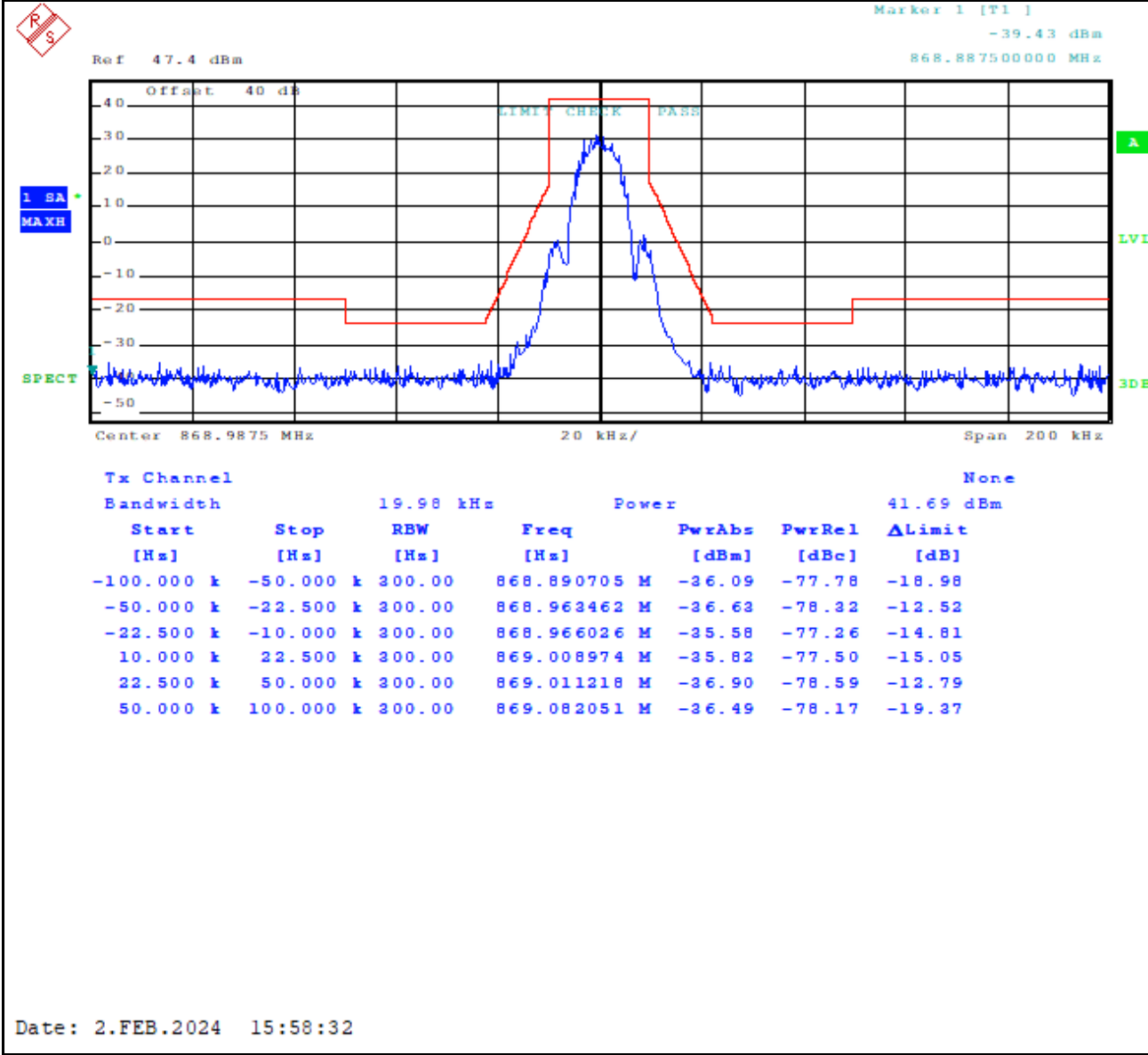
Plot 8-28: Occupied Bandwidth – 868.9875 MHz; 2-level FSK 9600 NPSPAC; Mask G
