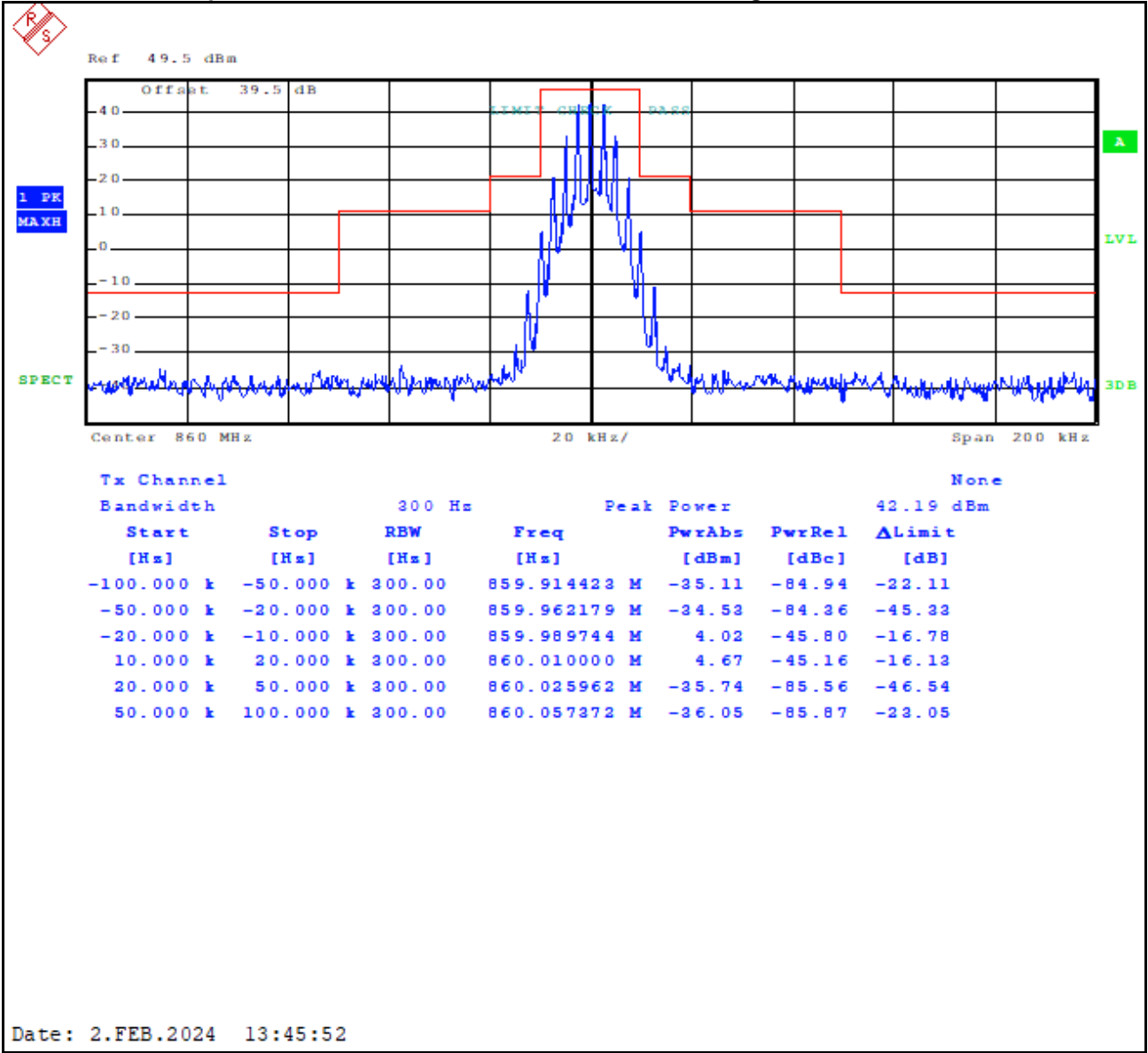
Plot 8-19: Occupied Bandwidth – 860.0000 MHz; NPSPAC Analog; Mask B
