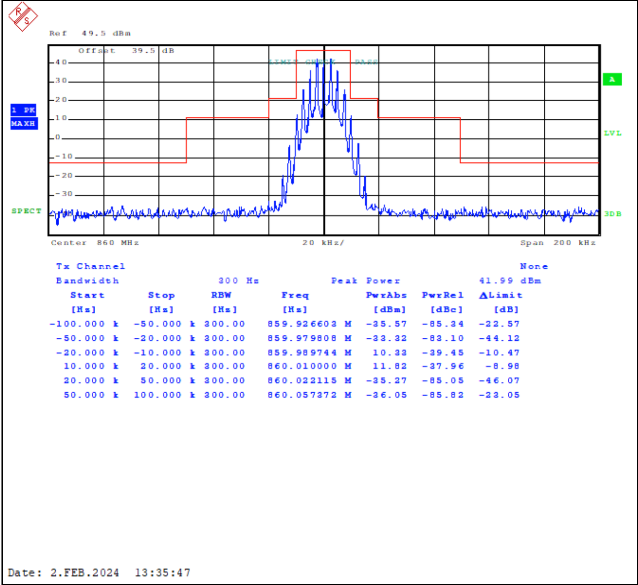
Plot 8-5: Occupied Bandwidth – 860.0000 MHz; WB Analog; Mask B
