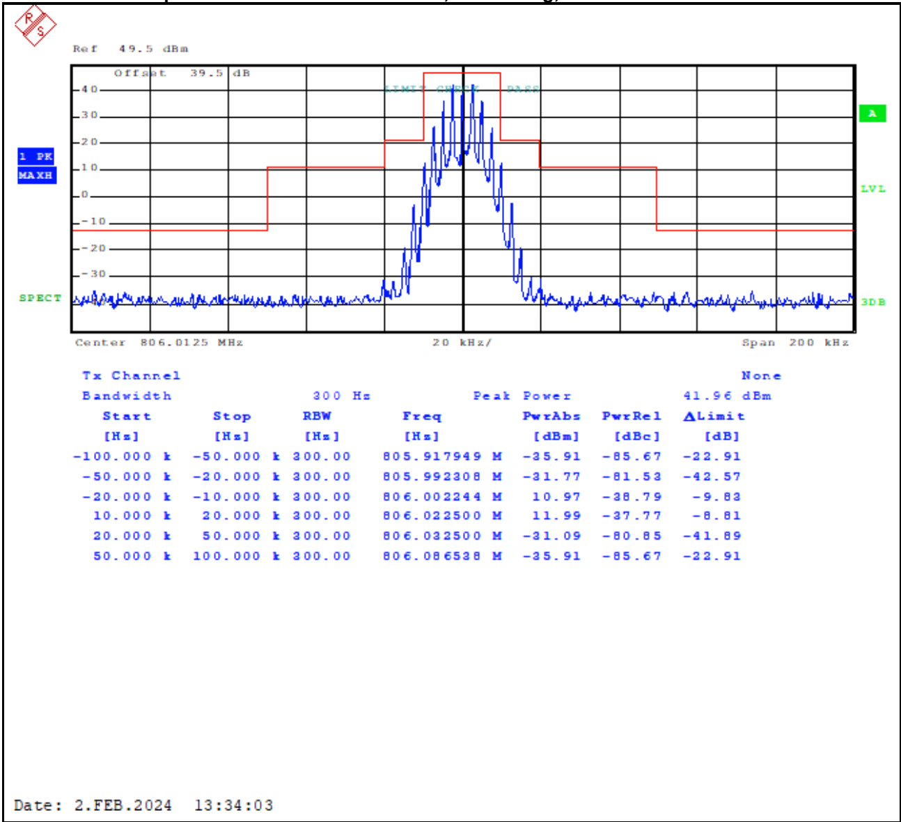
Plot 8-1: Occupied Bandwidth – 806.0125 MHz; WB Analog; Mask B
