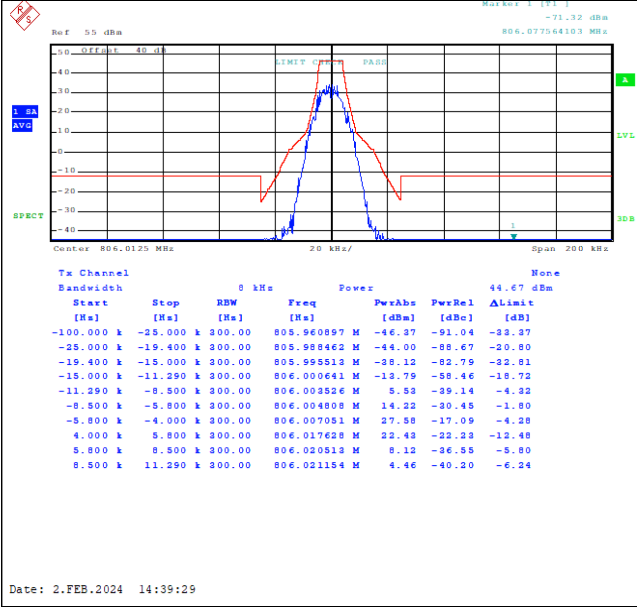
Plot 8-83: Occupied Bandwidth – 806.0125 MHz; HVD NPSPAC; Mask H
