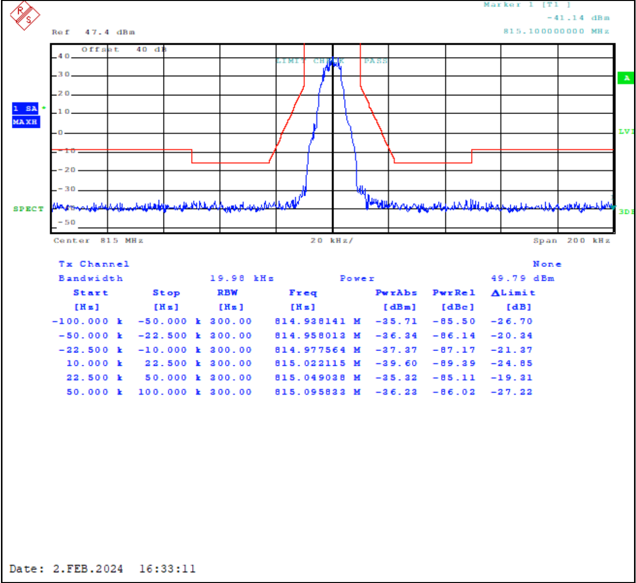
Plot 8-66: Occupied Bandwidth – 815.0000 MHz; H-CPM (TDMA); Mask G
