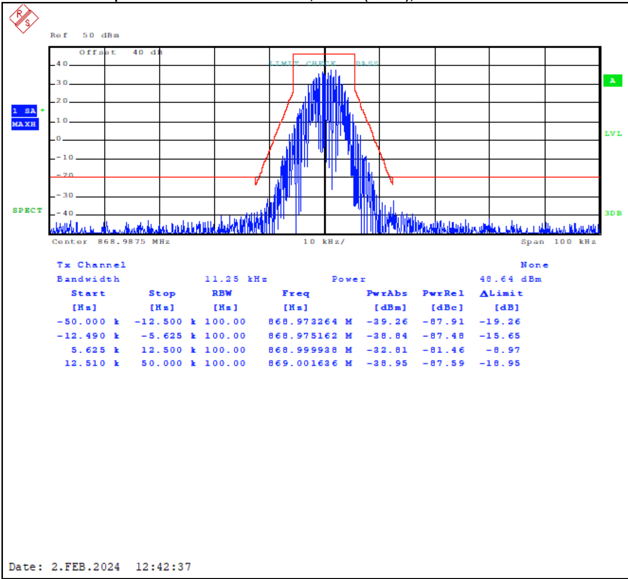
Plot 8-76: Occupied Bandwidth – 868.9875 MHz; H-CPM (TDMA); Mask D
