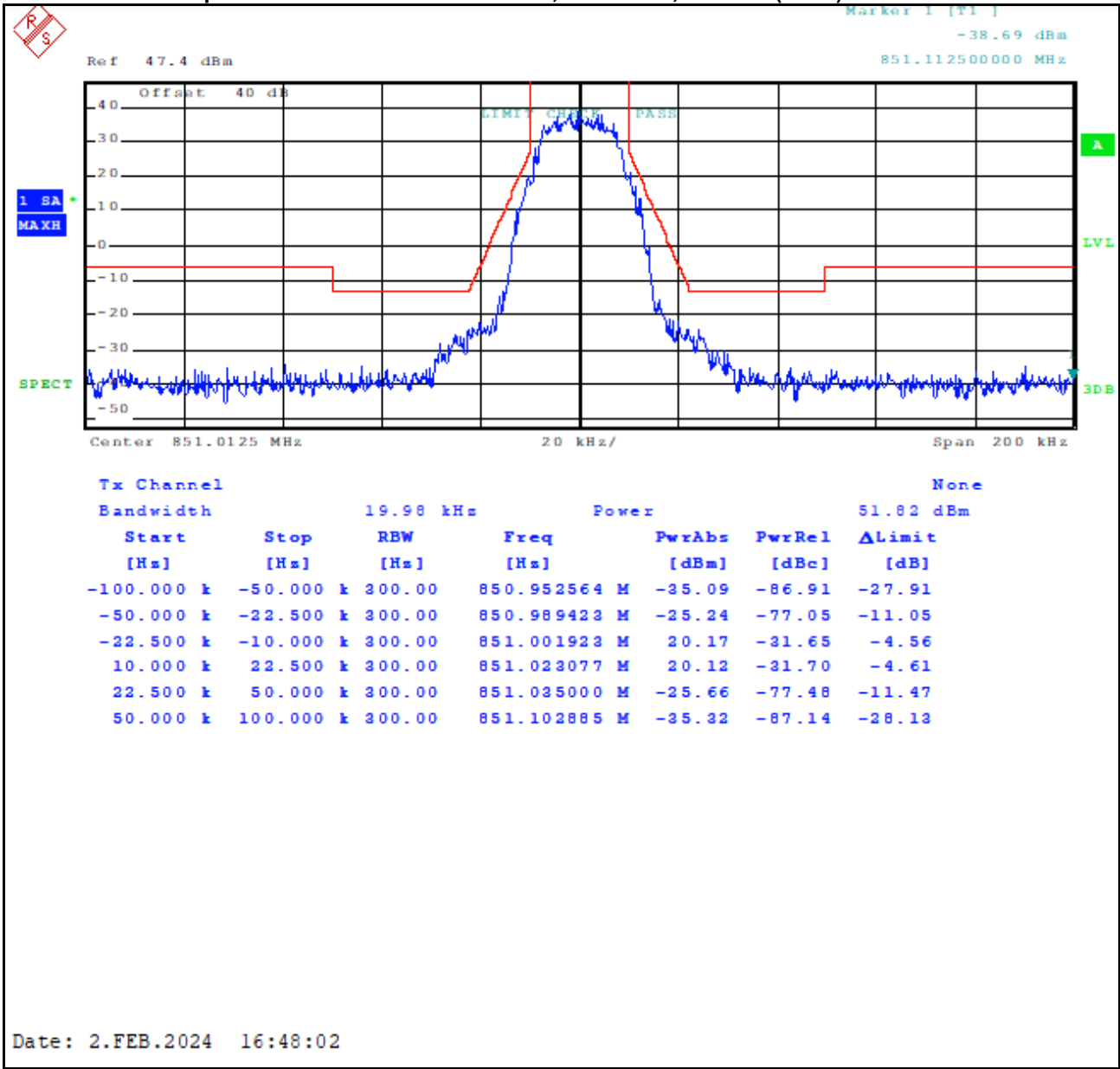
Plot 8-80: Occupied Bandwidth – 851.0125 MHz; HVD SMR; Mask G (ISED)
