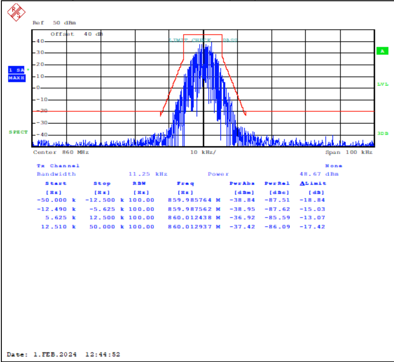
Plot 8-75: Occupied Bandwidth – 860.0000 MHz; H-CPM (TDMA); Mask D
