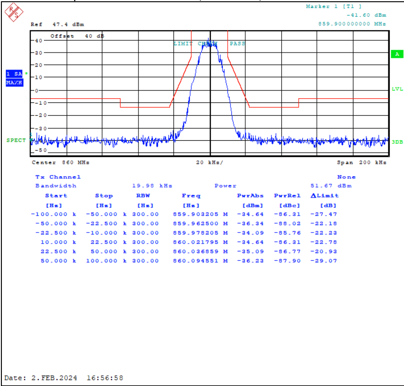
Plot 8-89: Occupied Bandwidth – 860.0000 MHz; HVD NPSPAC; Mask G
