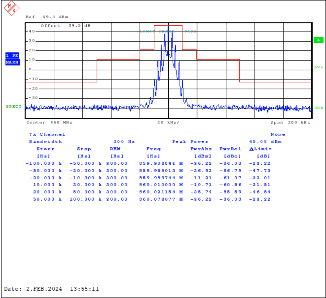
Plot 8-33: Occupied Bandwidth – 860.0000 MHz; NB Analog; Mask B
