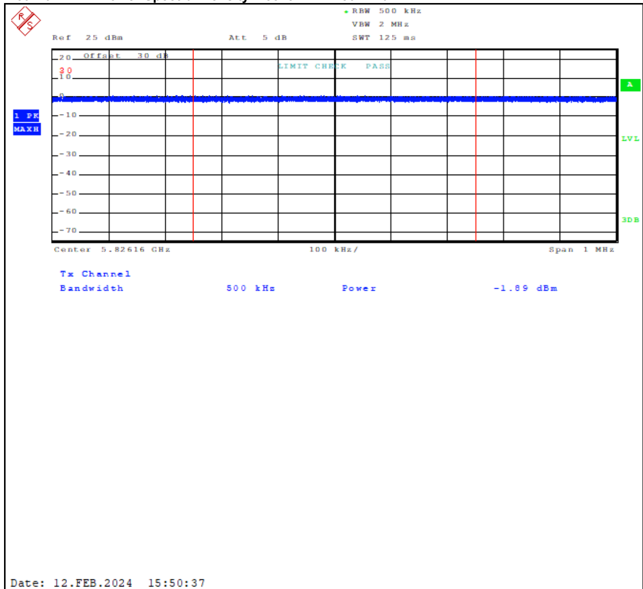
Plot 7-6: Power Spectral Density – 5825 MHz – 802.11a
