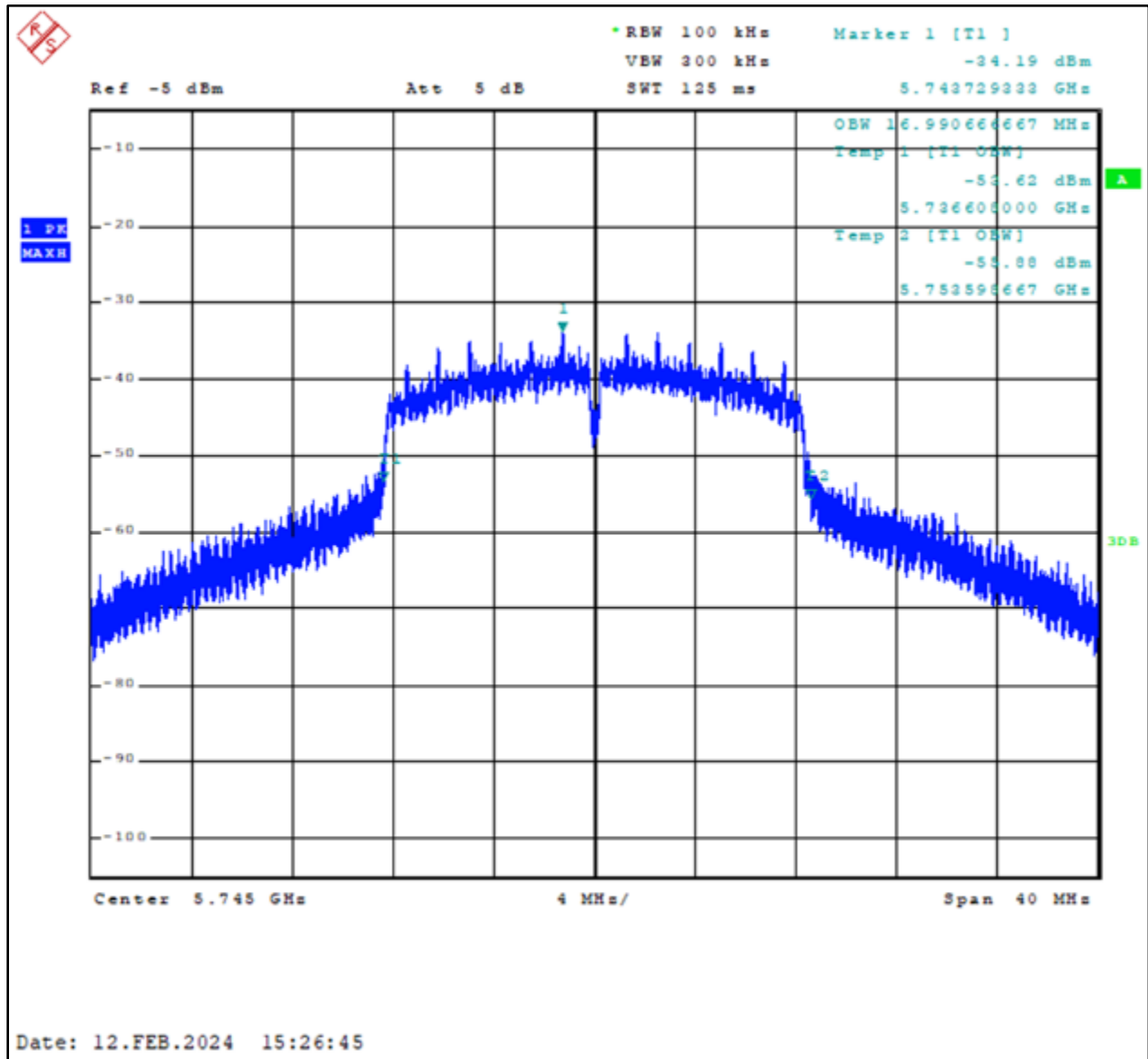
Plot 6-7: 99% dB Bandwidth – 5745 MHz – 802.11a
