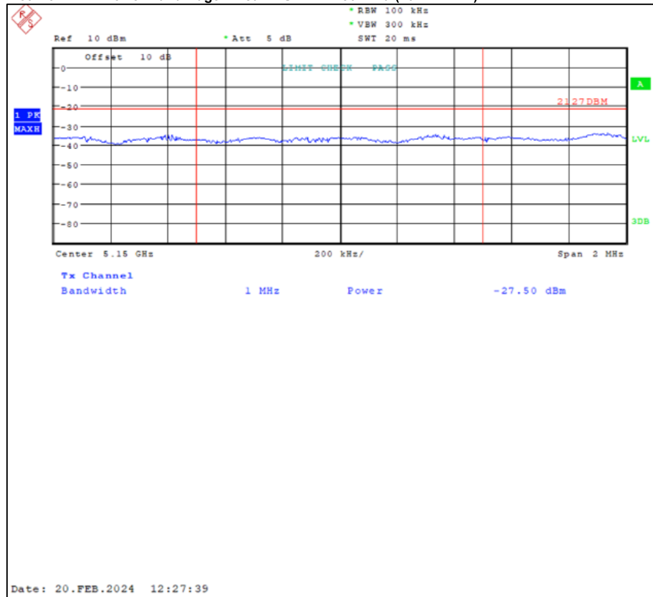
Plot 4-6: Lower Band Edge – Peak – U-NII 1 – 802.11a (40 MHz BW)
