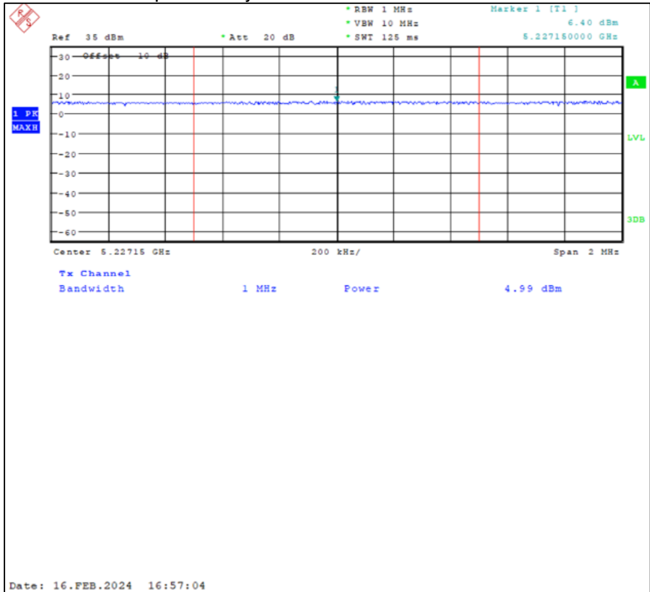
Plot 7-8: Power Spectral Density – 5230 MHz – 802.11a
