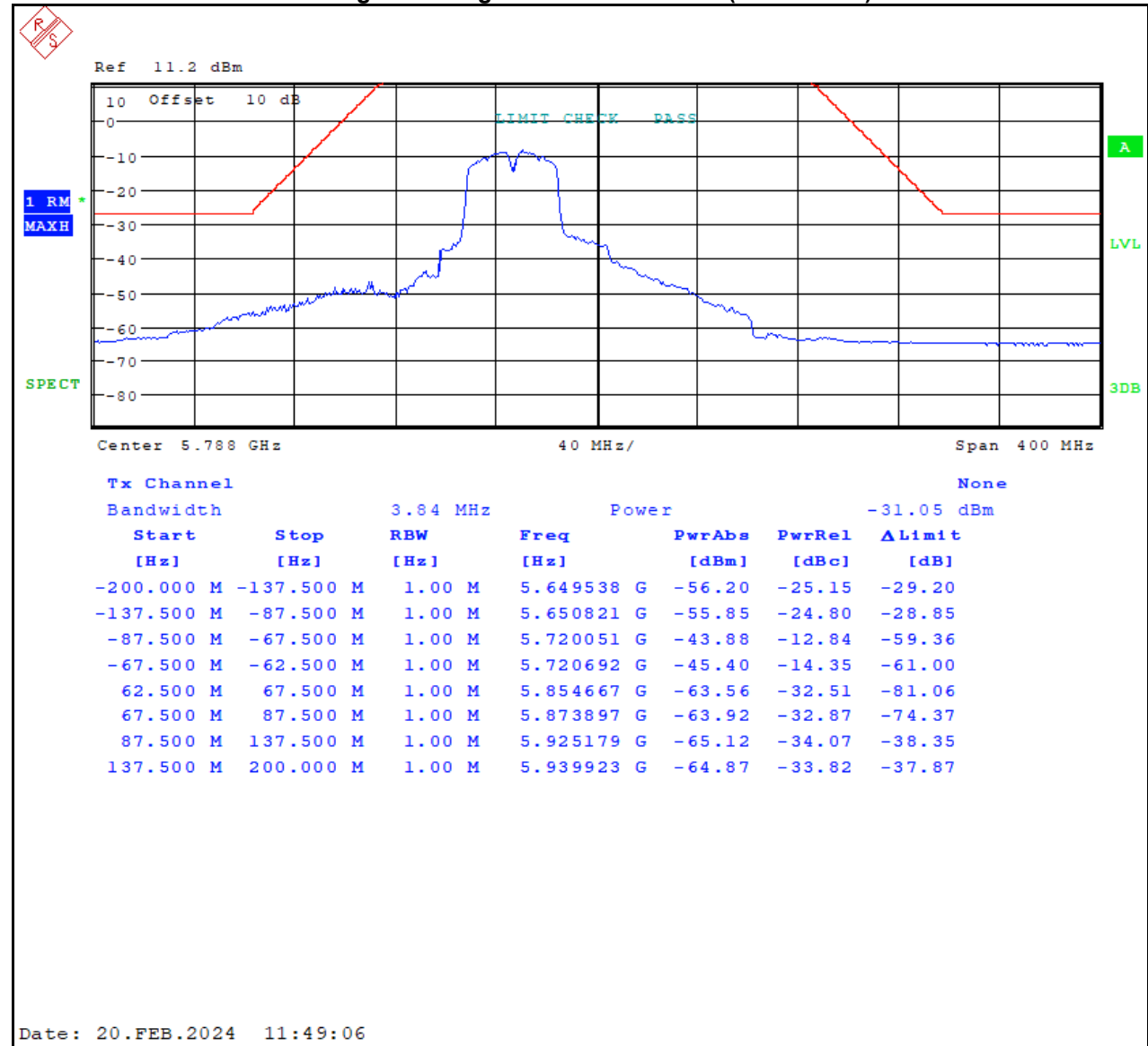
Plot 4-13: Lower Band Edge – Average – U-NII 3 – 802.11a (40 MHz BW)
