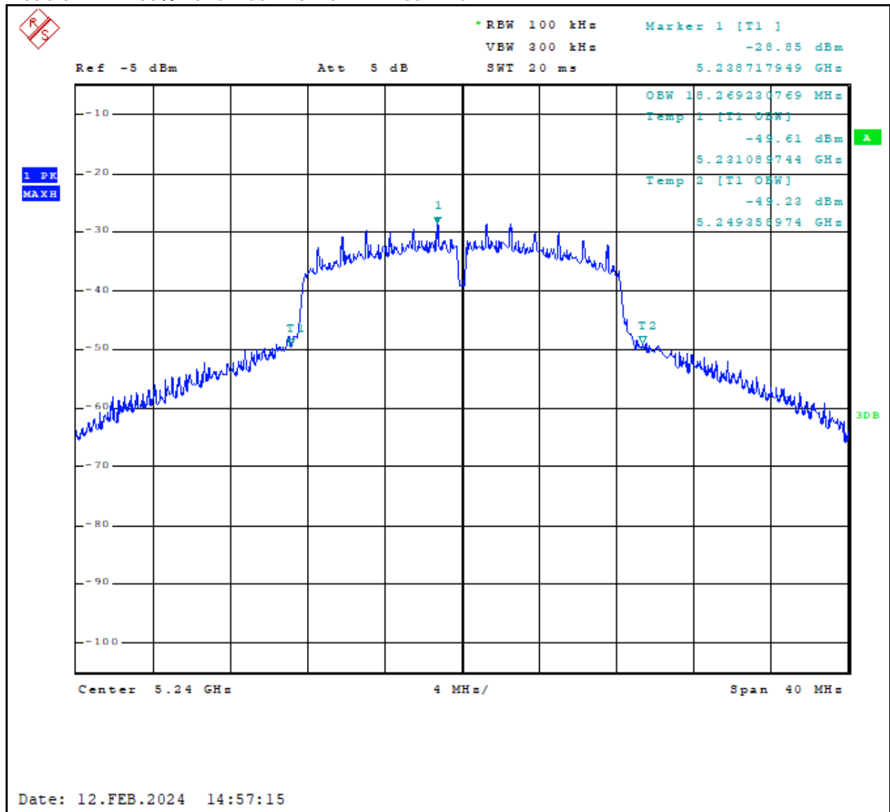
Plot 6-3: 99% Bandwidth – 5240 MHz – 802.11a
