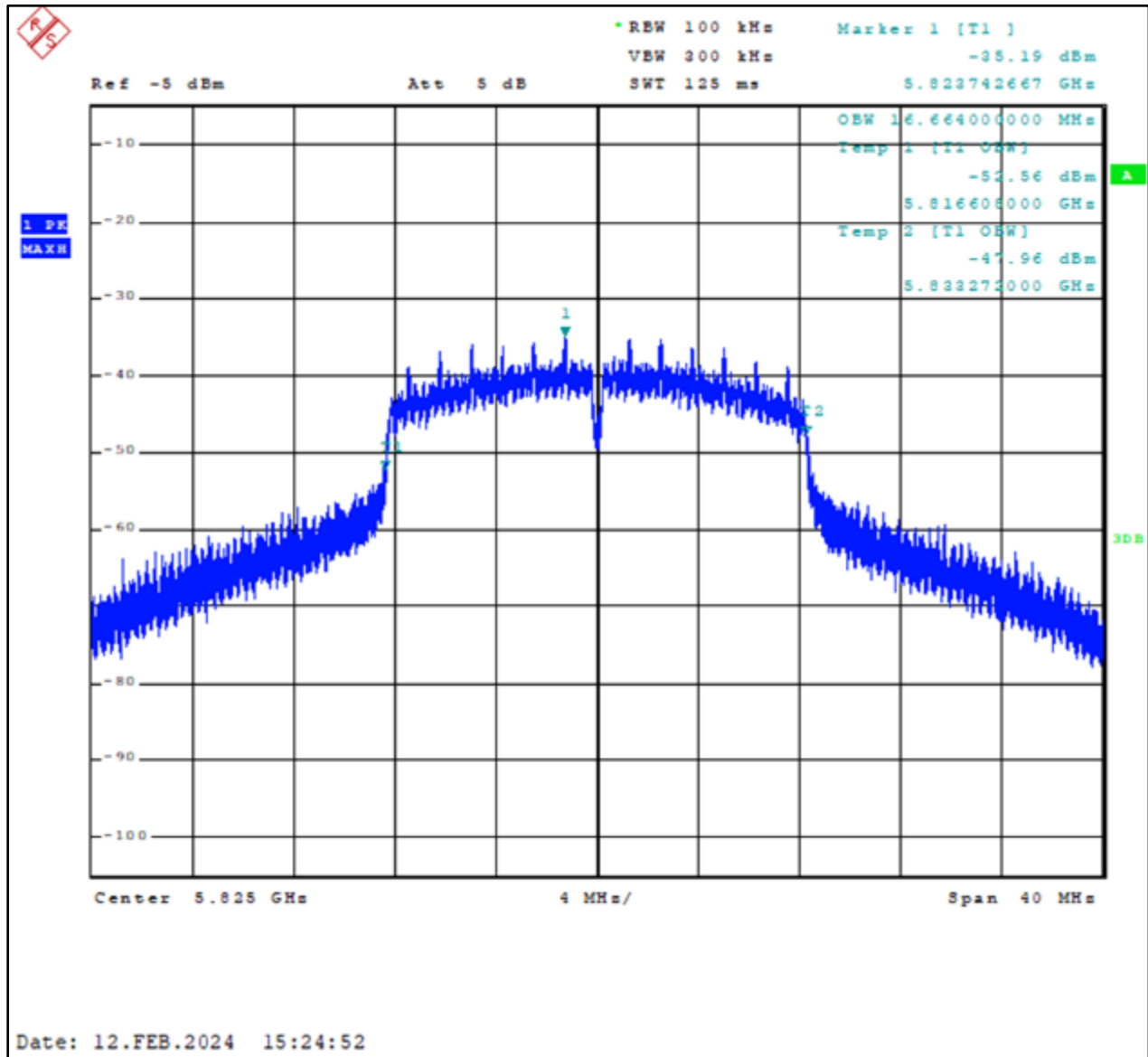
Plot 6-9: 99% dB Bandwidth – 5825 MHz – 802.11a
