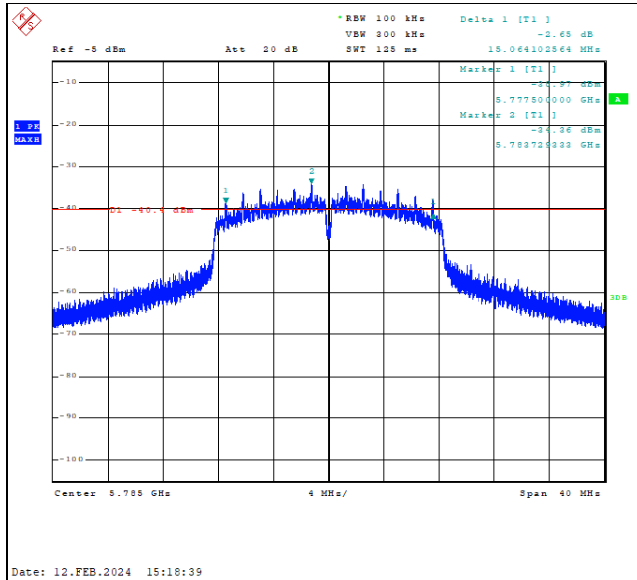
Plot 6-5: 6 dB Bandwidth – 5785 MHz – 802.11a
