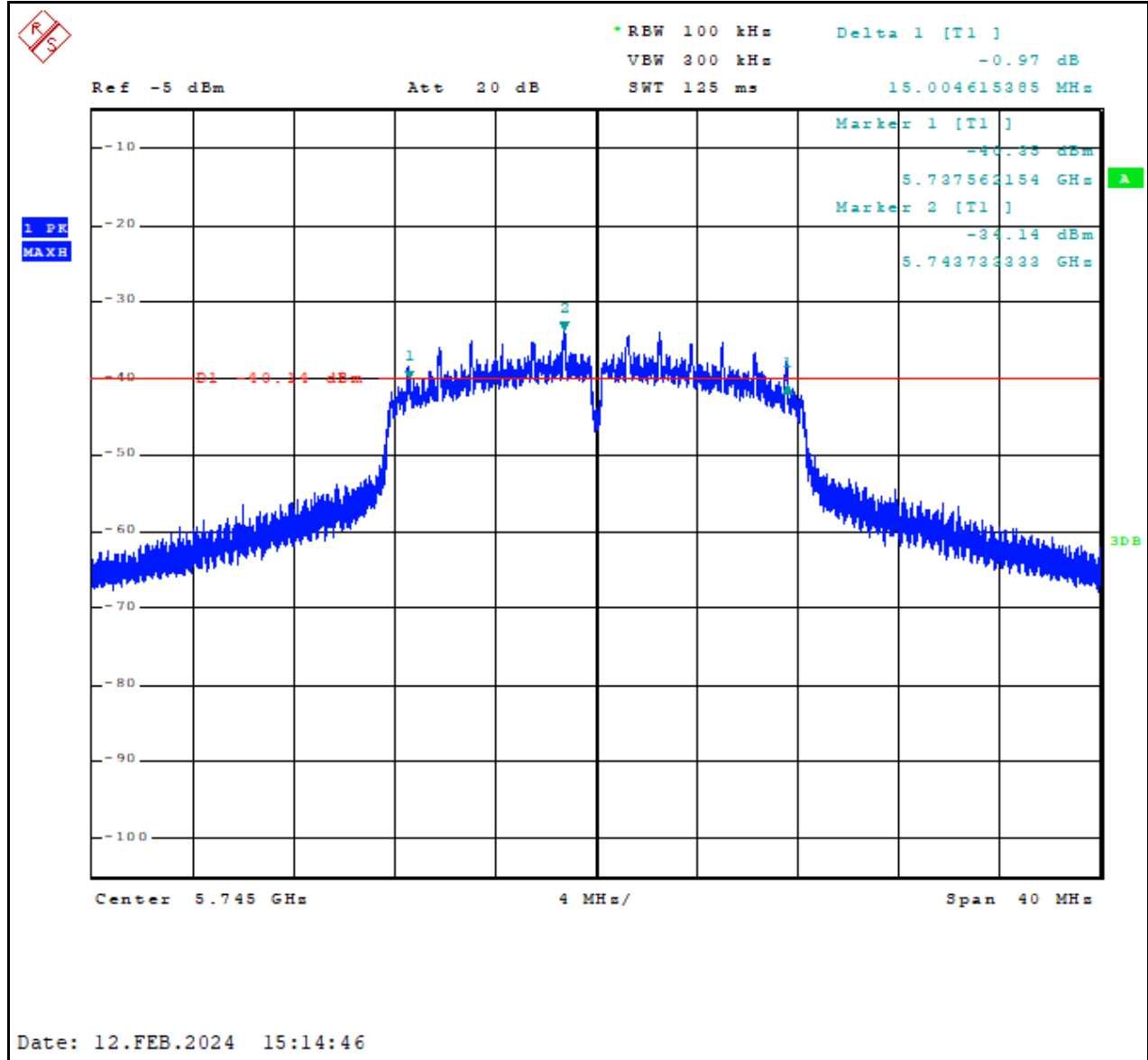
Plot 6-4: 6 dB Bandwidth – 5745 MHz – 802.11a
