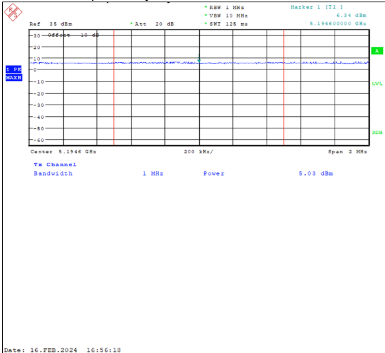
Plot 7-7: Power Spectral Density – 5190 MHz – 802.11a
