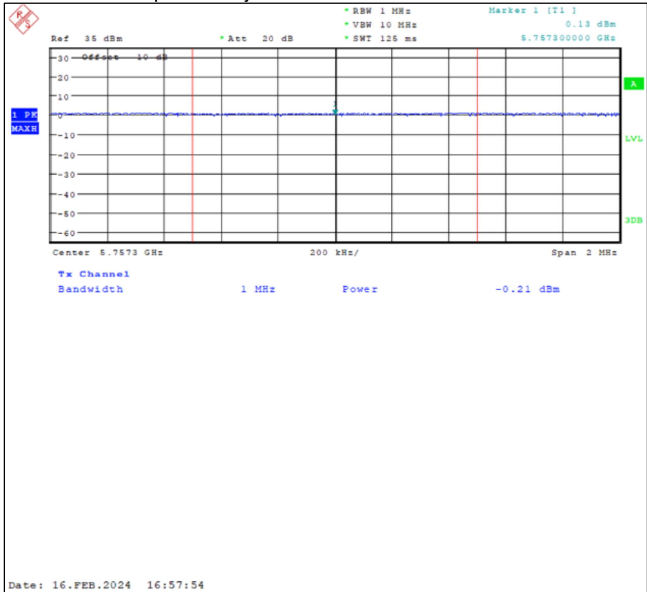
Plot 7-9: Power Spectral Density – 5755 MHz – 802.11a
