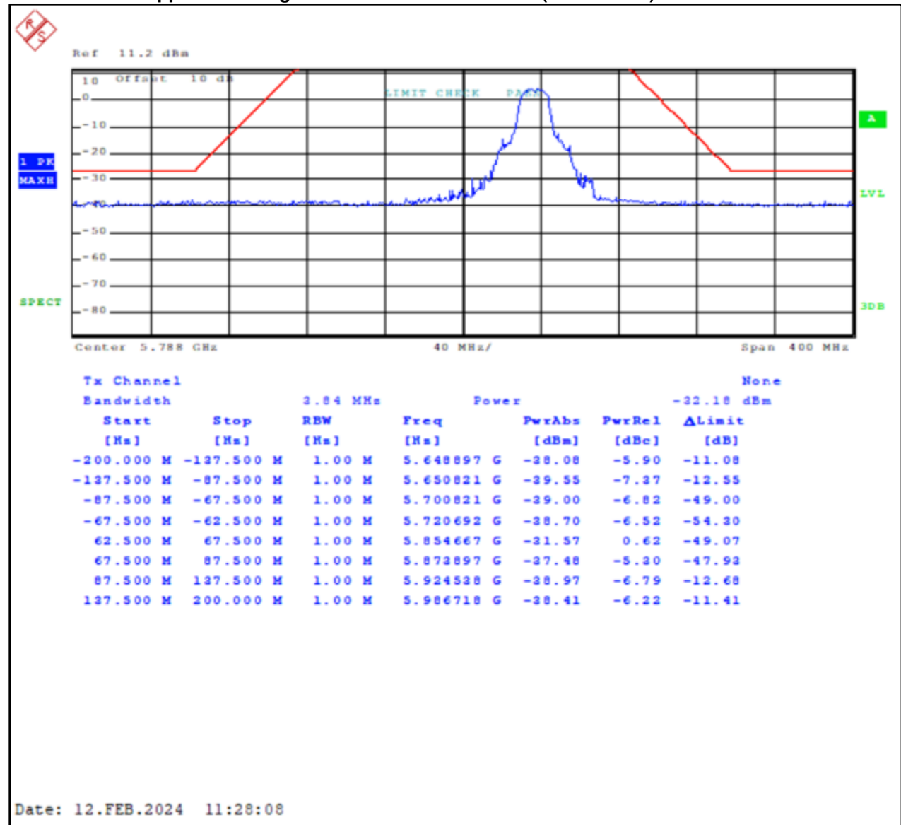
Plot 4-12: Upper Band Edge – Peak – U-NII 3 – 802.11a (20 MHz BW)
