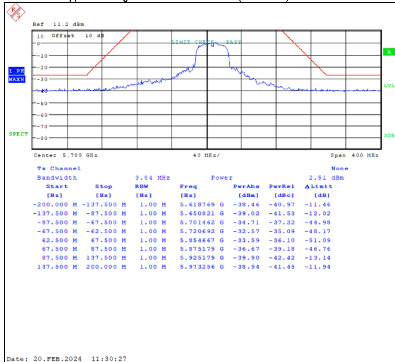
Plot 4-16: Upper Band Edge – Peak – U-NII 3 – 802.11a (40 MHz BW)
