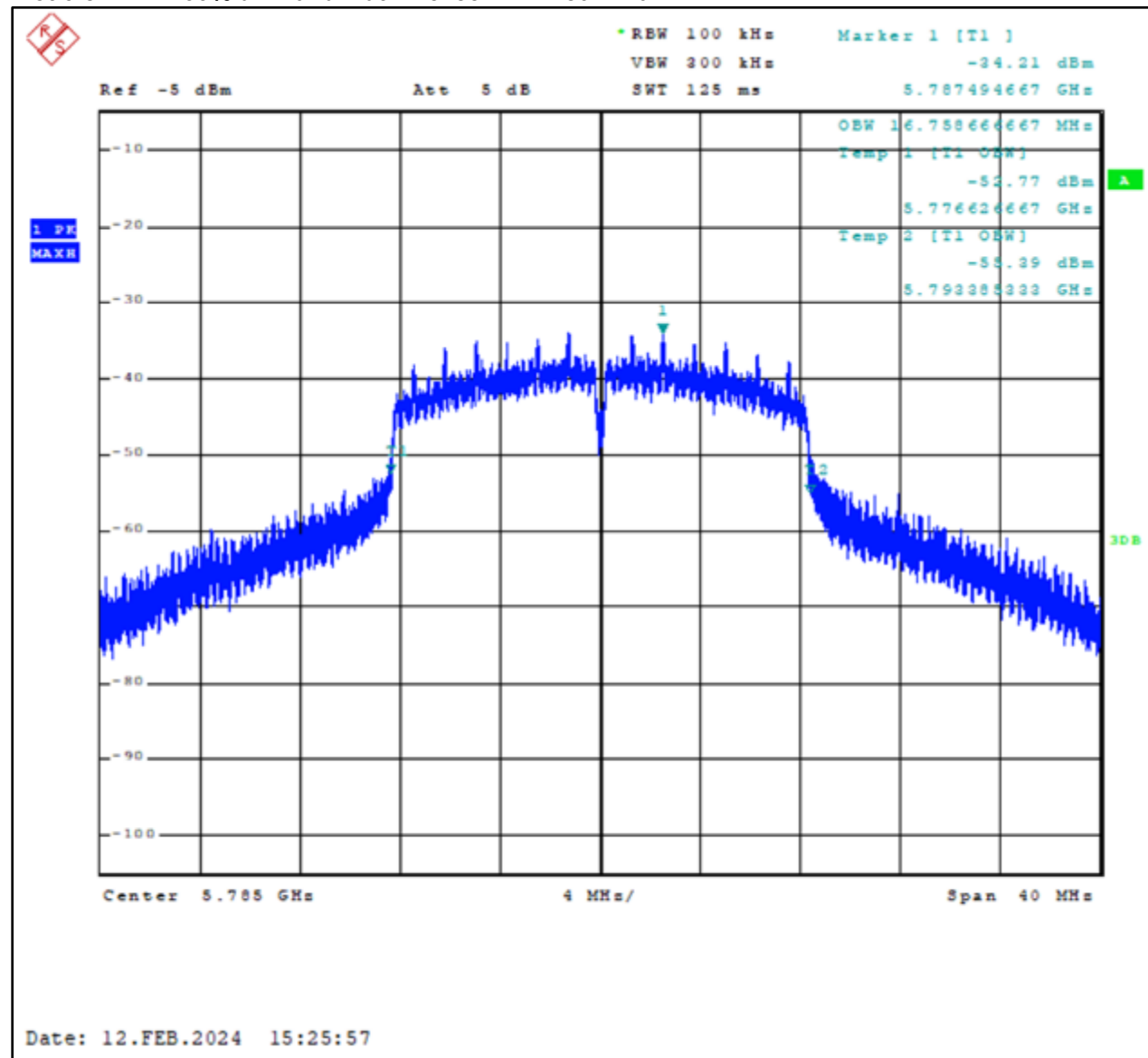
Plot 6-8: 99% dB Bandwidth – 5785 MHz – 802.11a
