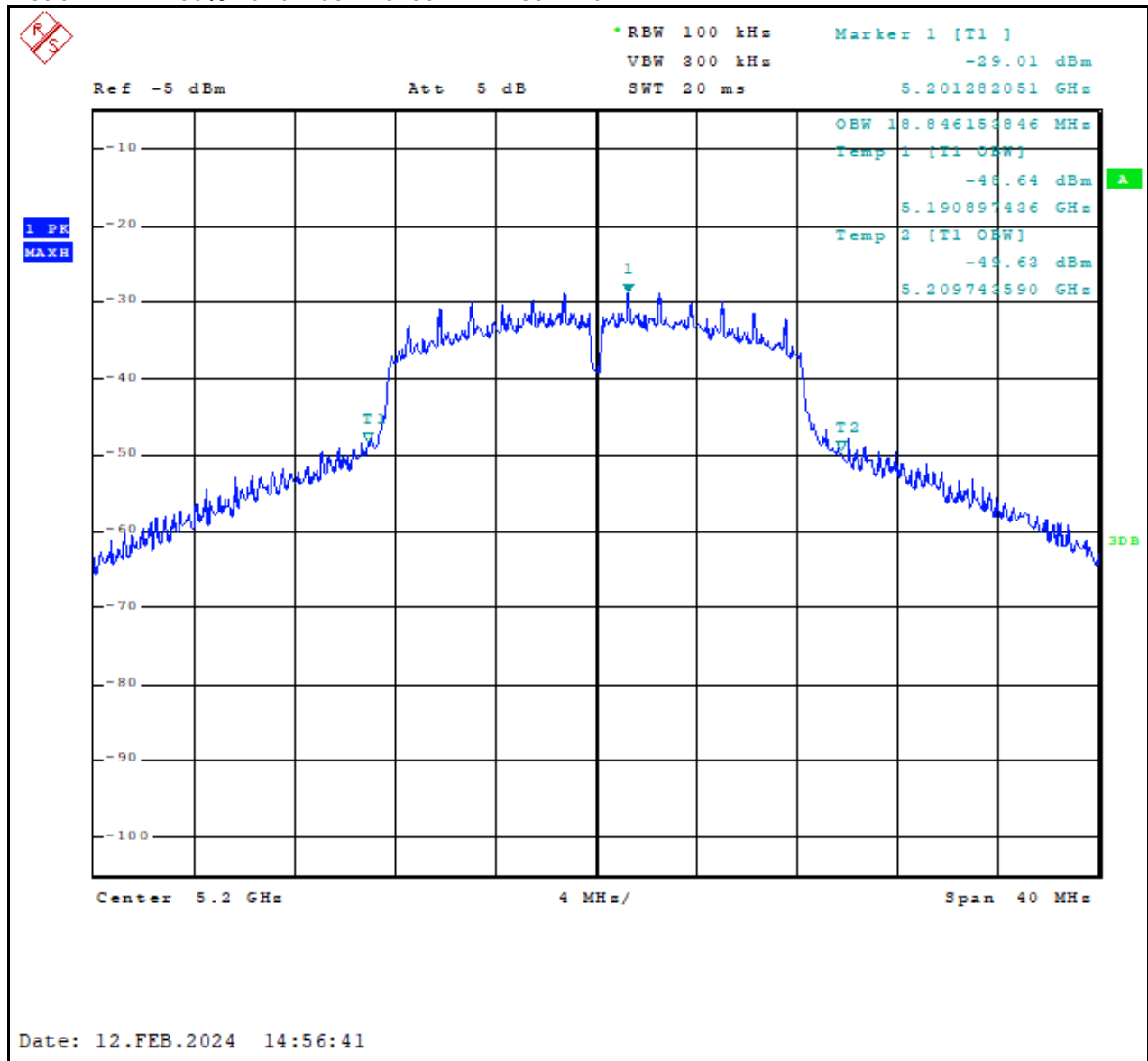
Plot 6-2: 99% Bandwidth – 5200 MHz – 802.11a
