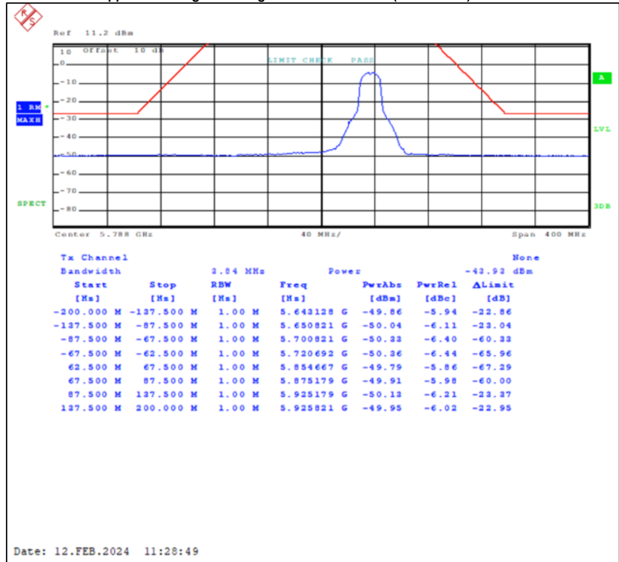
Plot 4-11: Upper Band Edge – Average – U-NII 3 – 802.11a (20 MHz BW)
