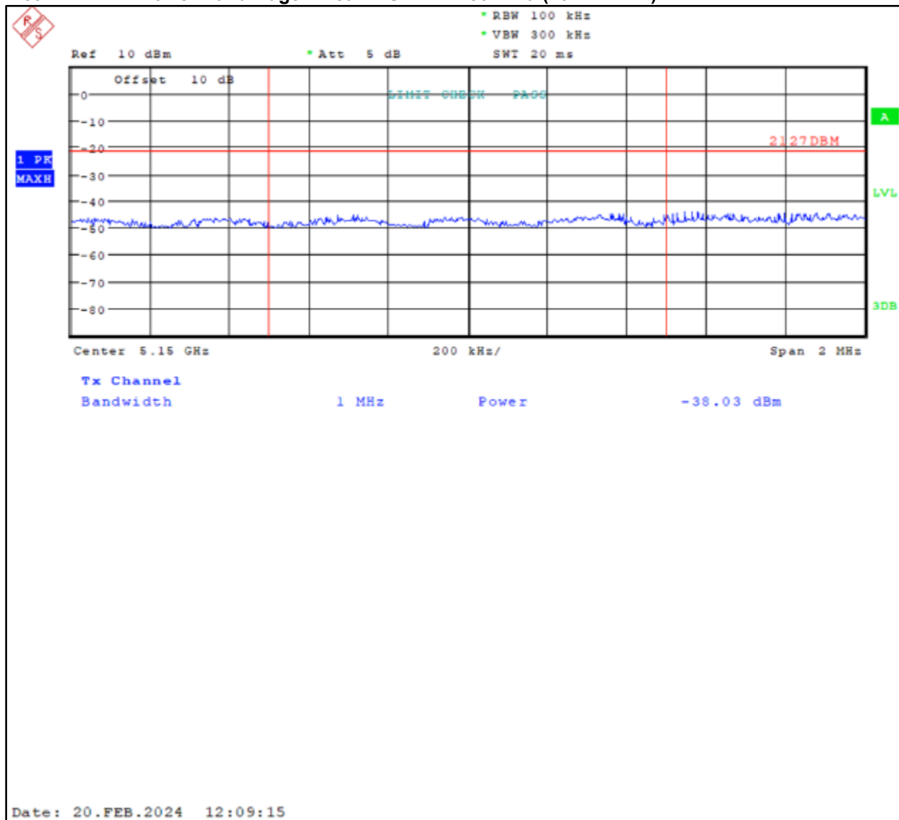
Plot 4-2: Lower Band Edge – Peak – U-NII 1 – 802.11a (20 MHz BW)
