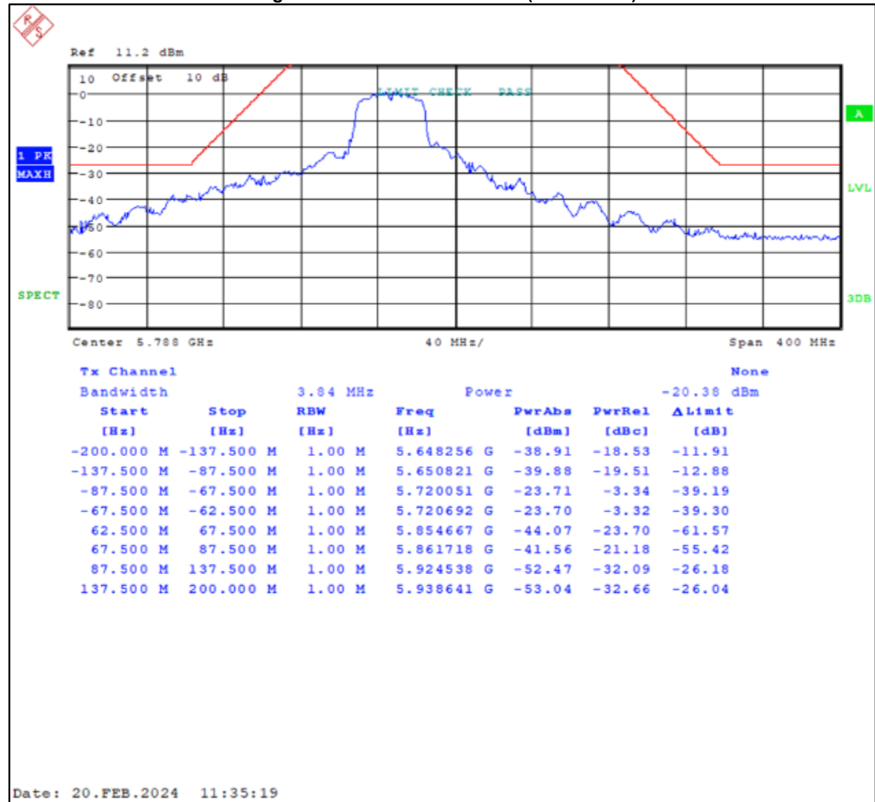
Plot 4-14: Lower Band Edge – Peak – U-NII 3 – 802.11a (40 MHz BW)
