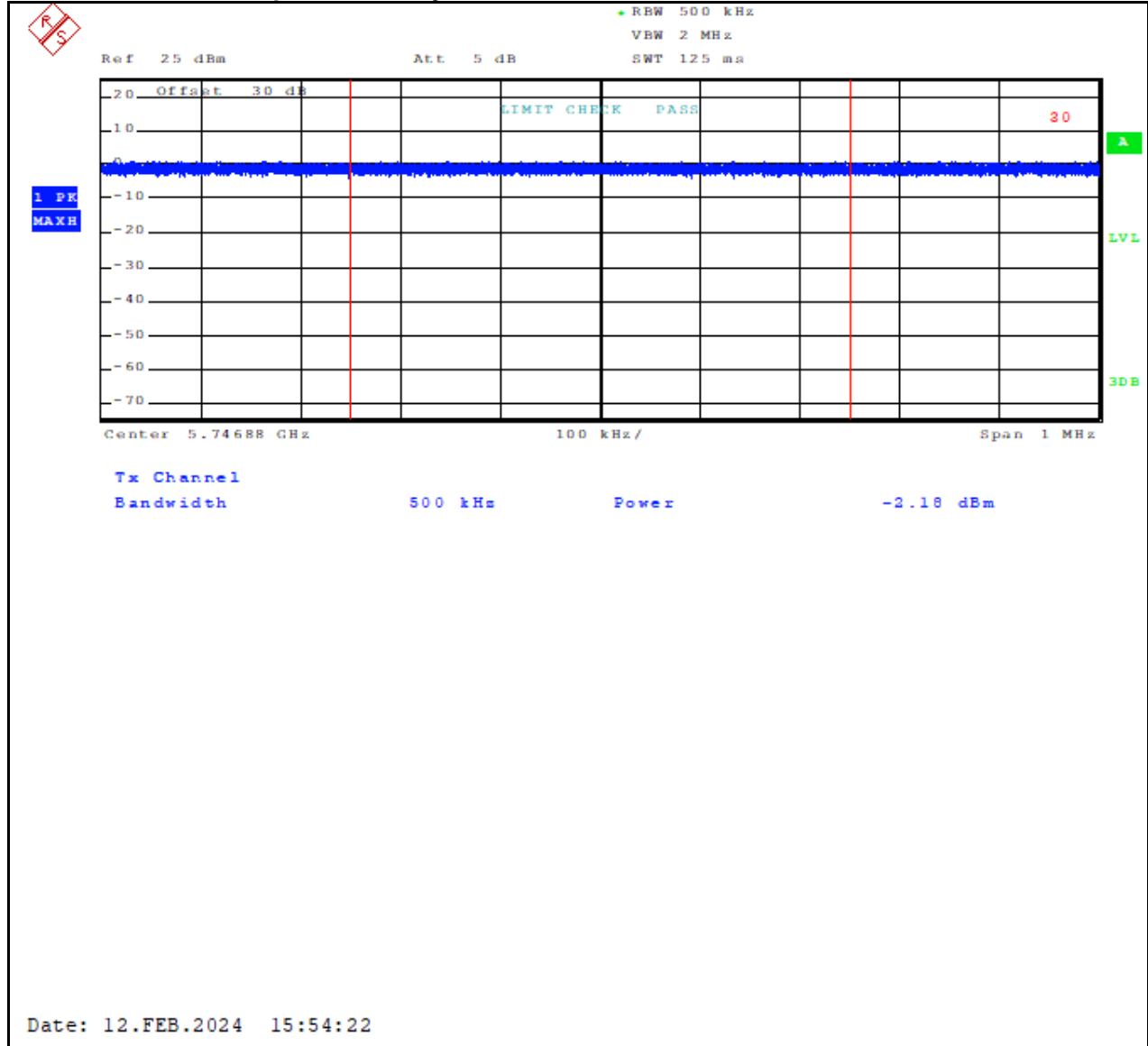
Plot 7-4: Power Spectral Density – 5745 MHz – 802.11a
