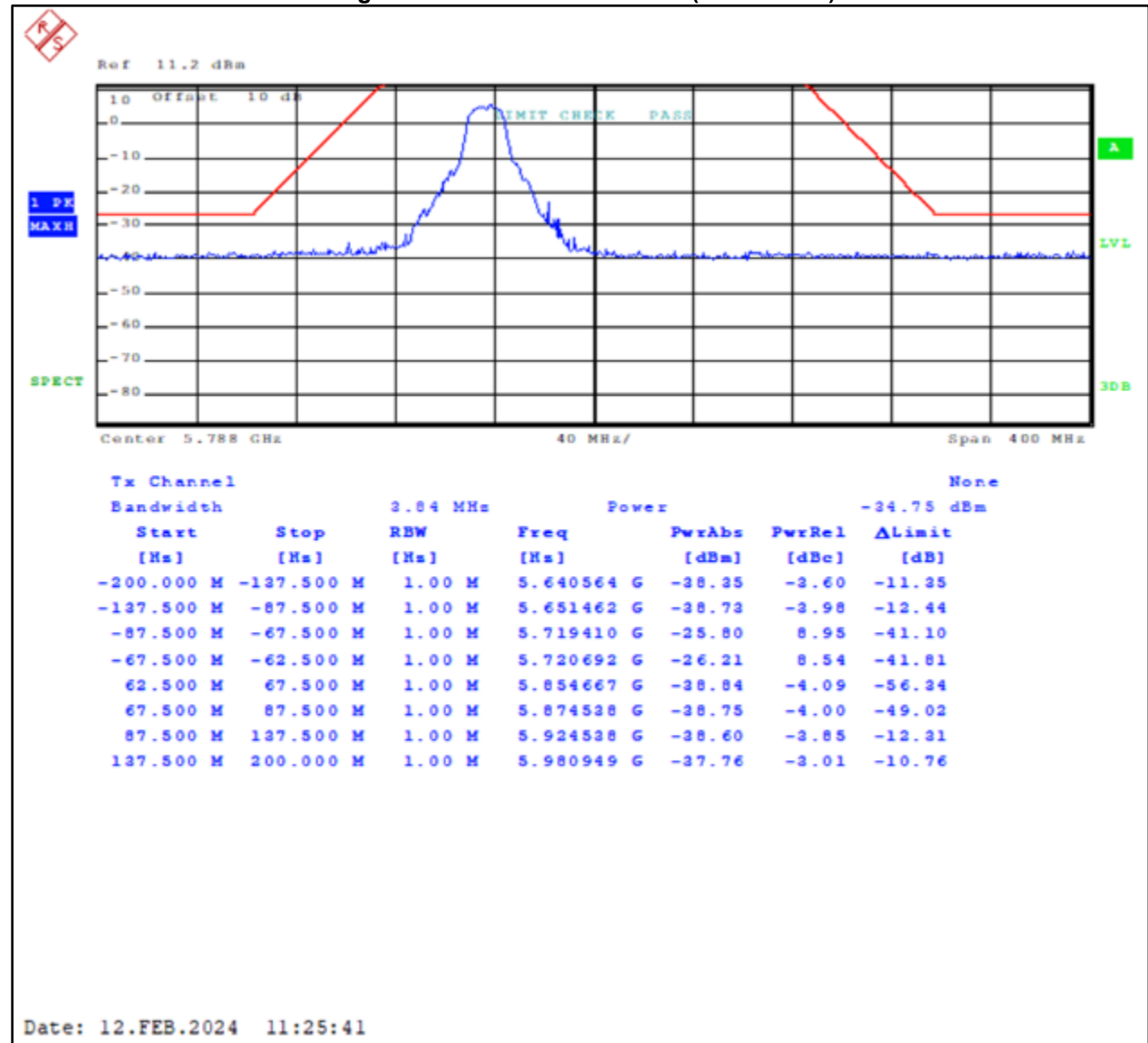
Plot 4-10: Lower Band Edge – Peak – U-NII 3 – 802.11a (20 MHz BW)
