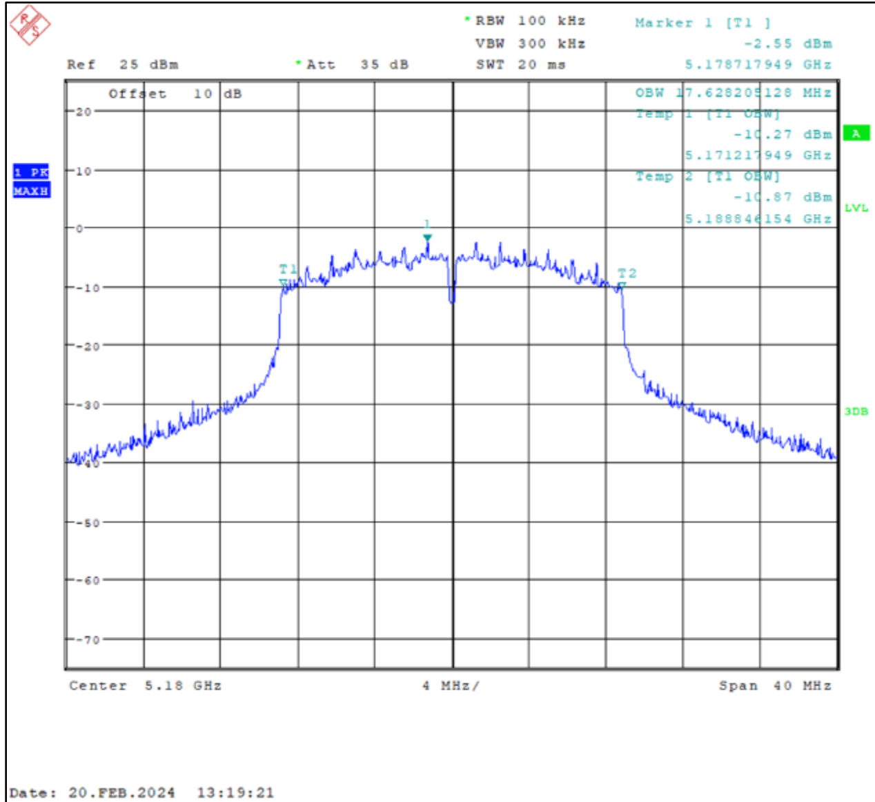
Plot 6-1: 99% Bandwidth – 5180 MHz – 802.11a
