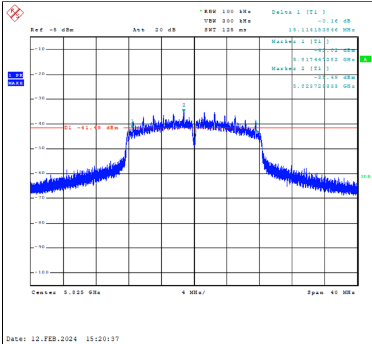
Plot 6-6: 6 dB Bandwidth – 5825 MHz – 802.11a
