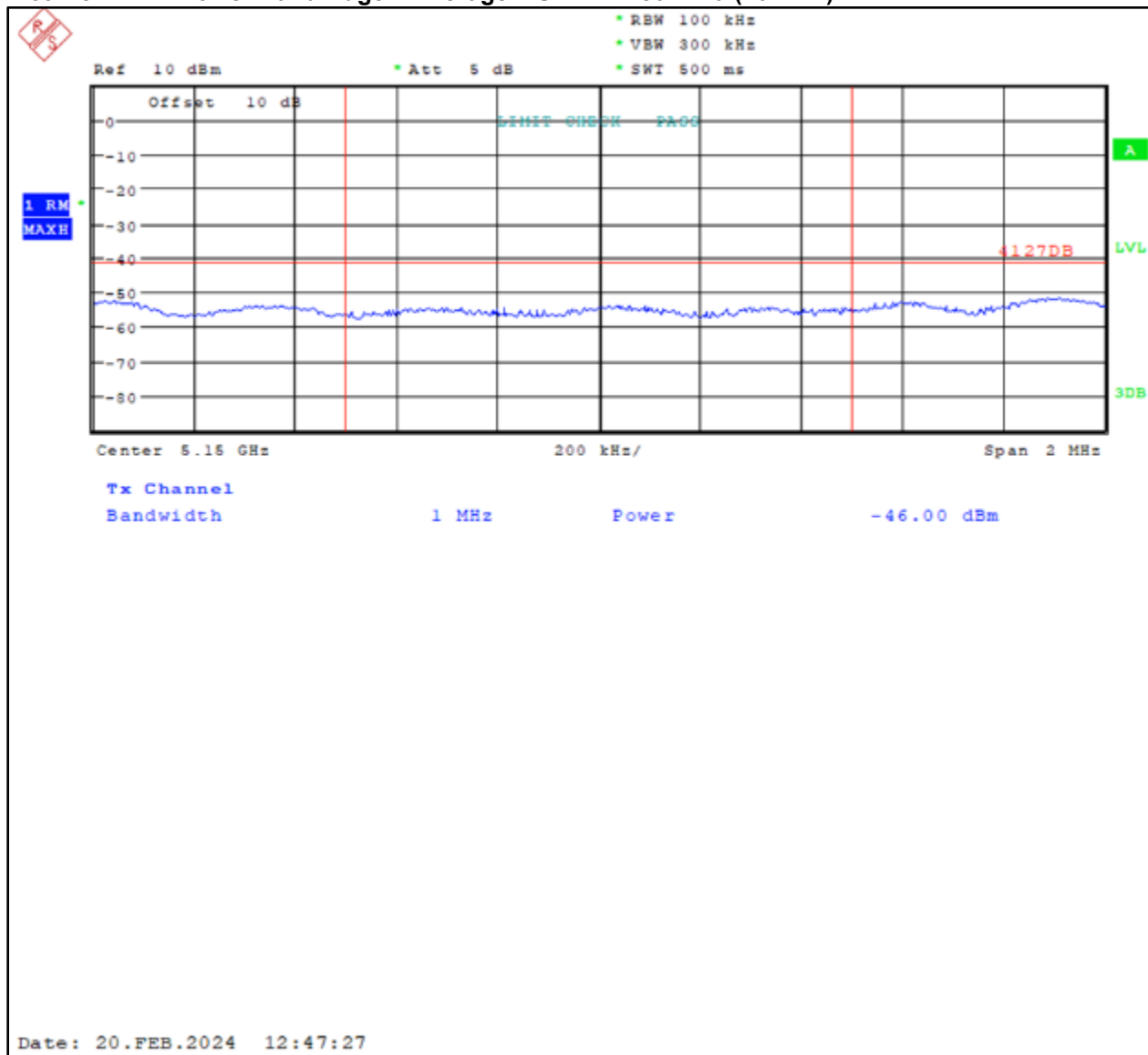
Plot 4-5: Lower Band Edge – Average – U-NII 1 – 802.11a (40 MHz)
