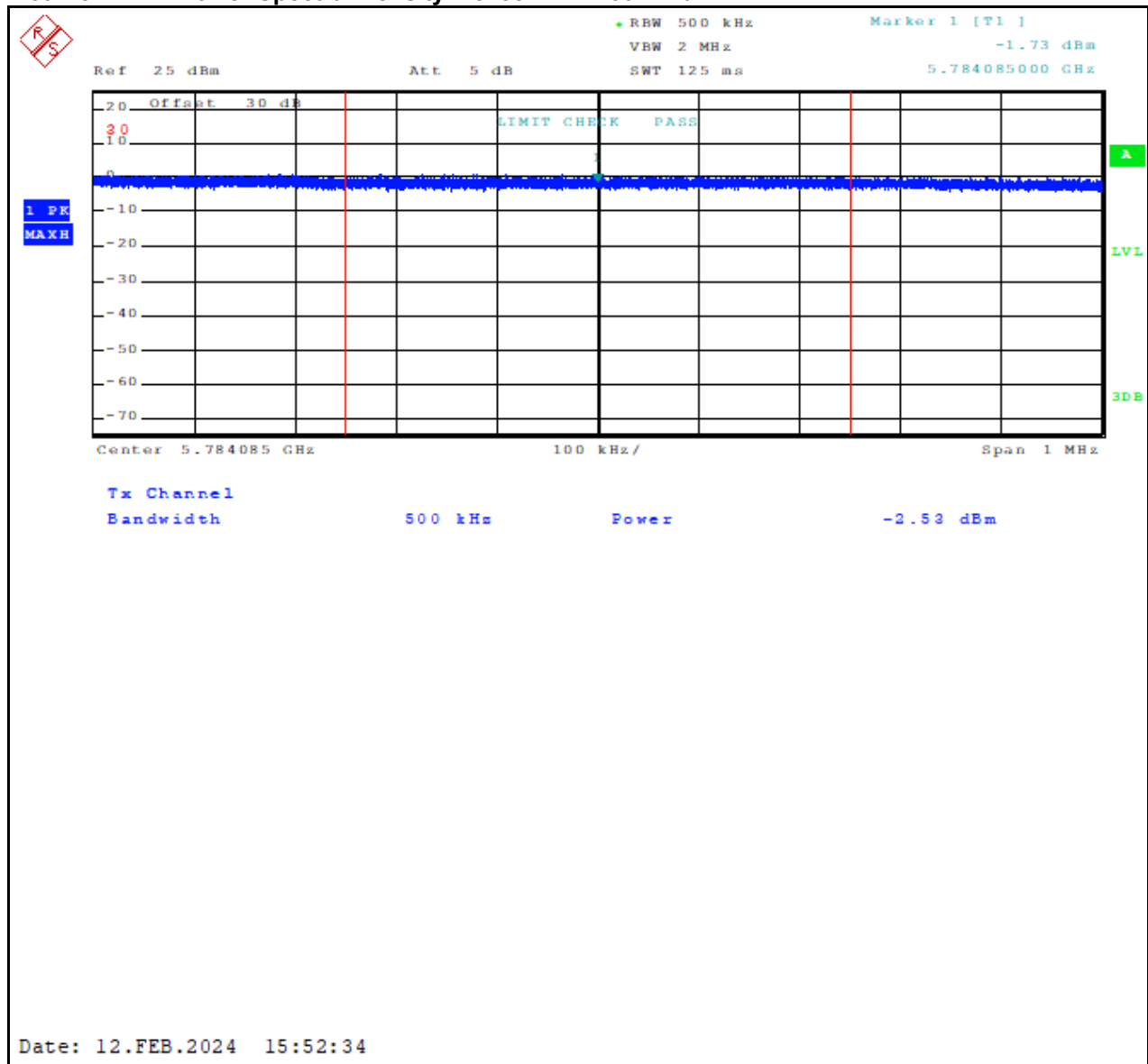
Plot 7-5: Power Spectral Density – 5785 MHz – 802.11a
