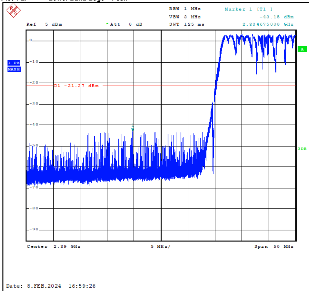
Plot 4-2: Lower Band Edge – Peak
