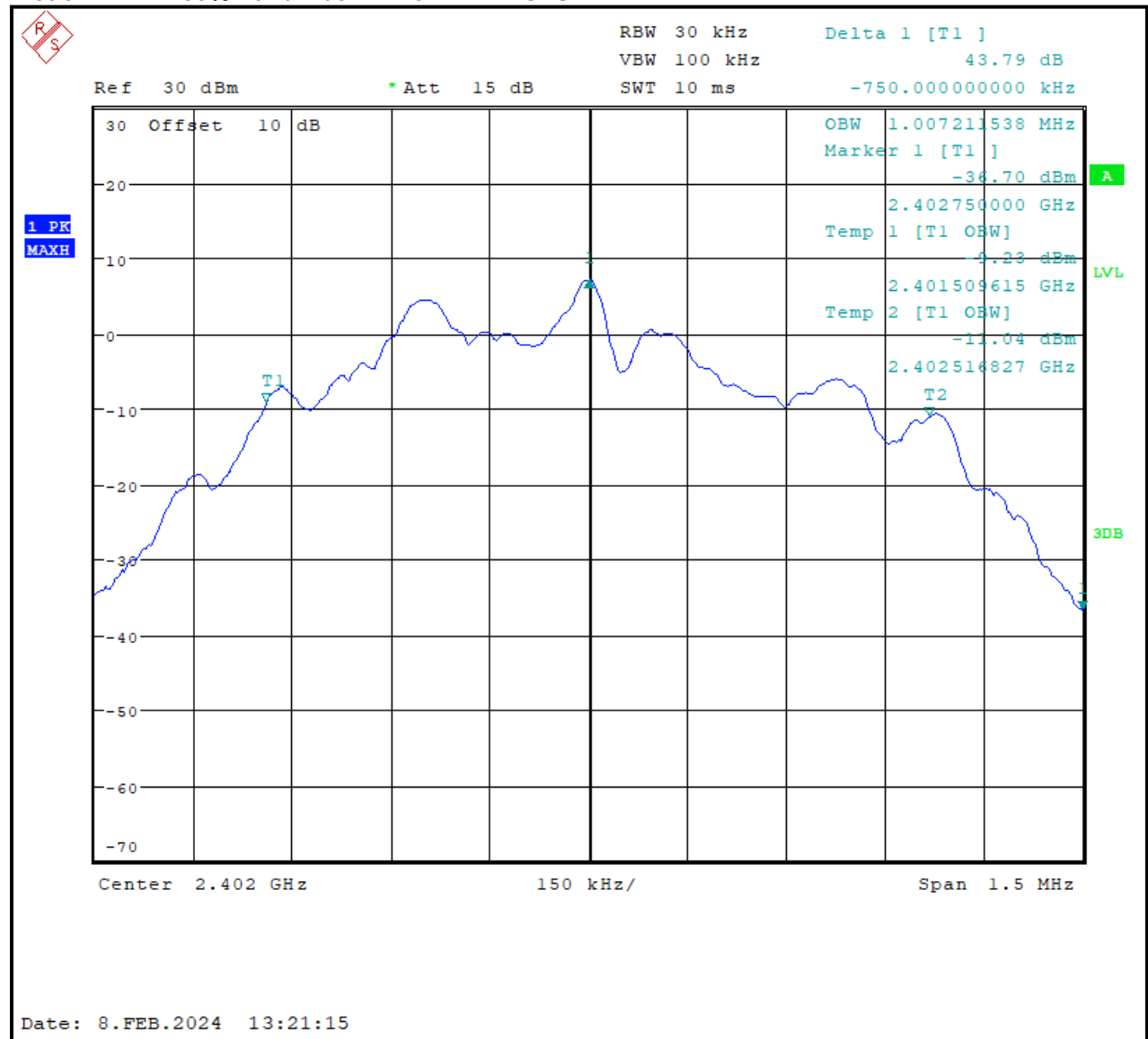
Plot 6-1: 99% Bandwidth – 2402 MHz – GFSK
