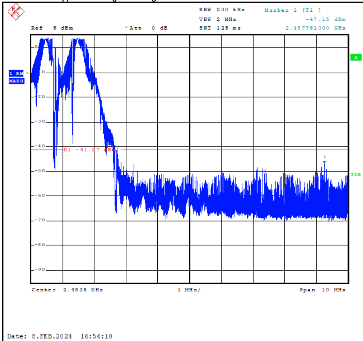
Plot 4-3: Upper Band Edge – Average
