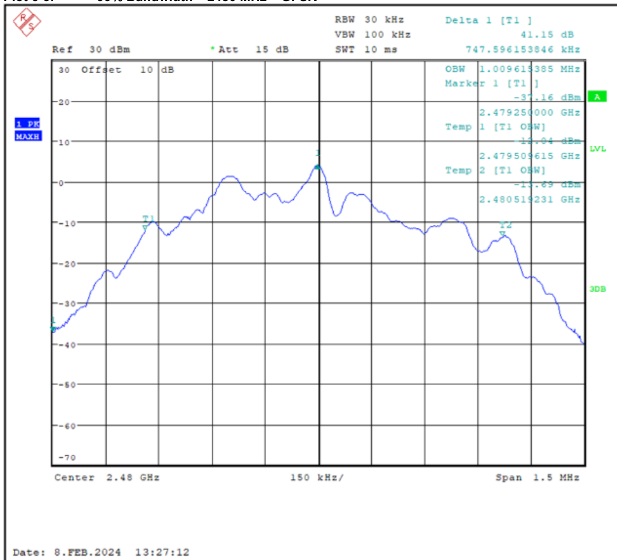
Plot 6-3: 99% Bandwidth – 2480 MHz – GFSK
