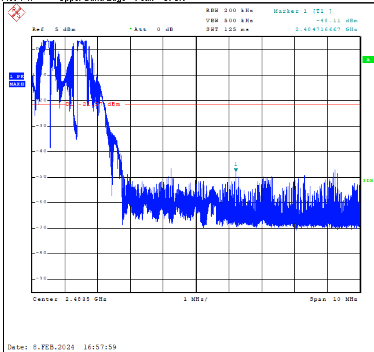
Plot 4-4: Upper Band Edge – Peak – GFSK
