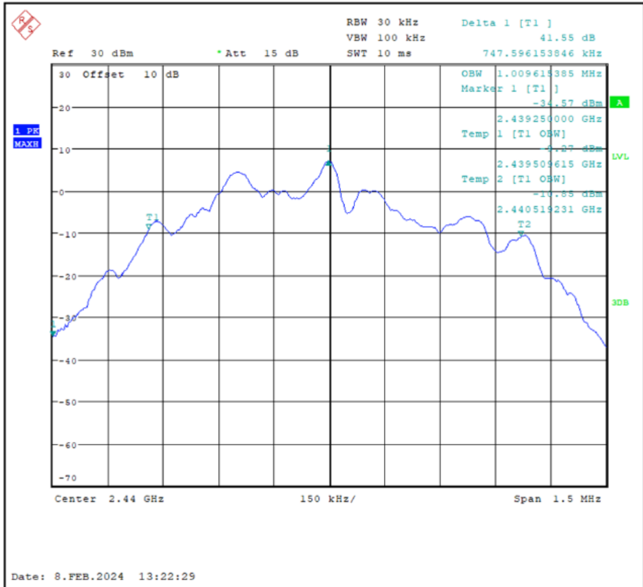
Plot 6-2: 99% Bandwidth – 2440 MHz – GFSK
