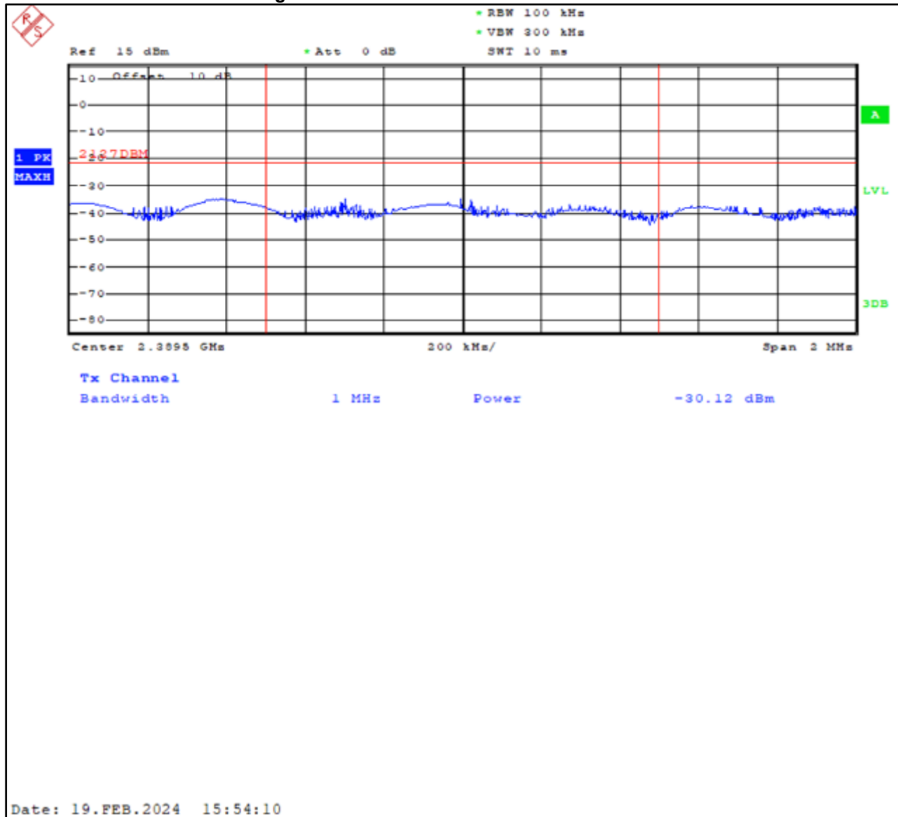
Plot 4-10: Lower Band Edge – Peak – 802.11n
