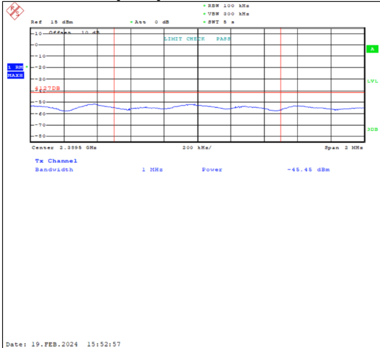
Plot 4-9: Lower Band Edge – Average – 802.11n
