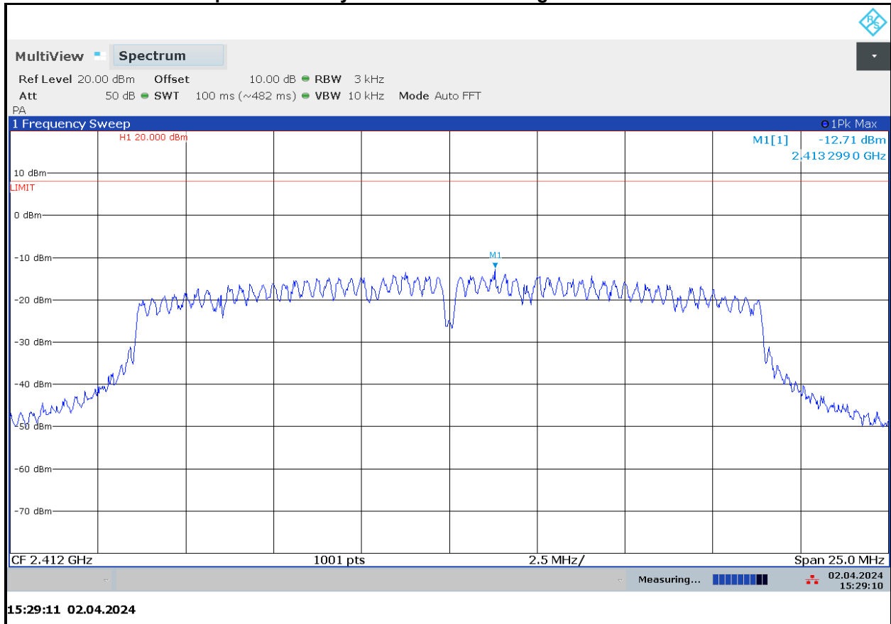
Plot 7-4: Power Spectral Density – 2412 MHz – 802.11g
