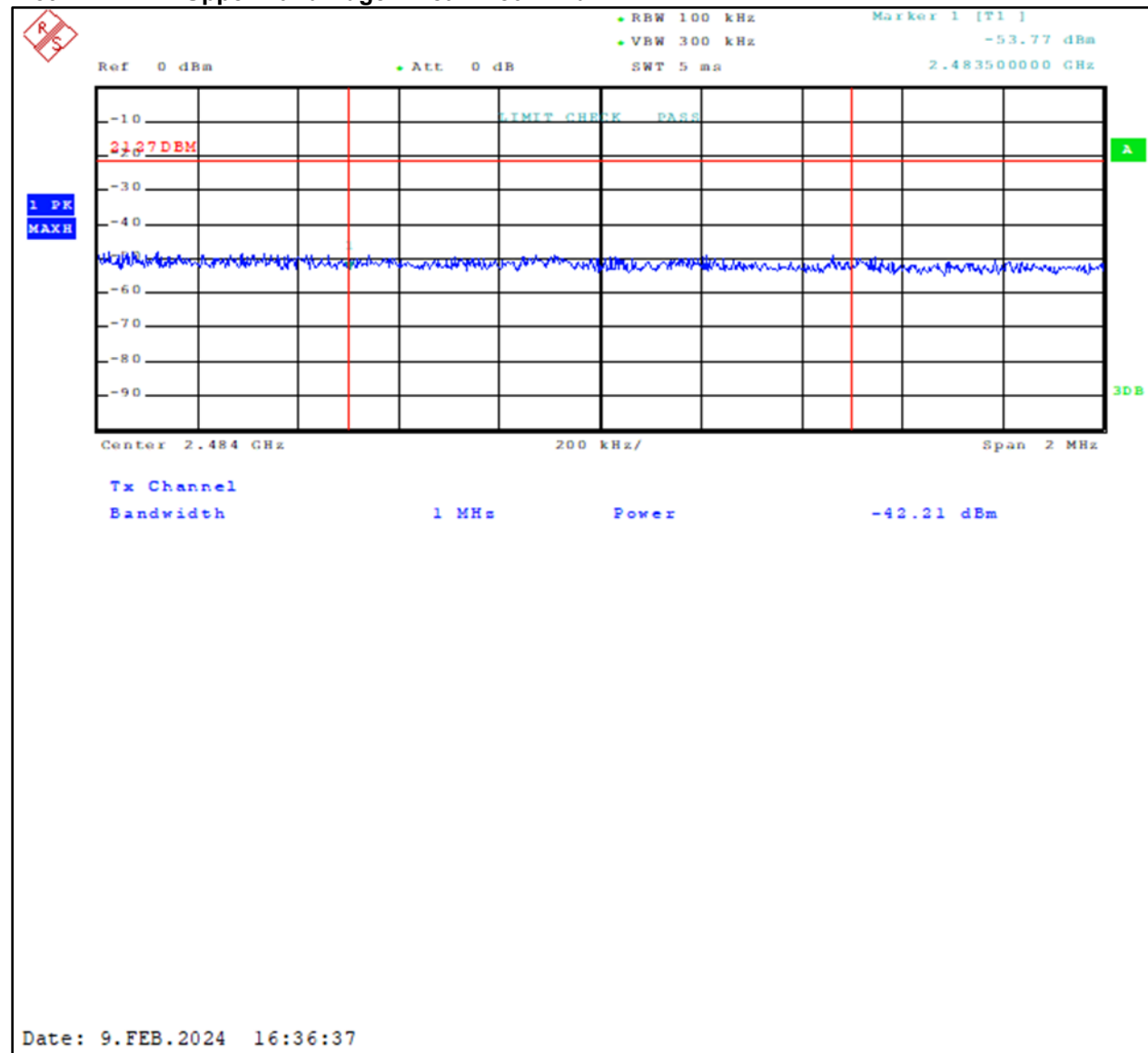
Plot 4-4: Upper Band Edge – Peak – 802.11b
