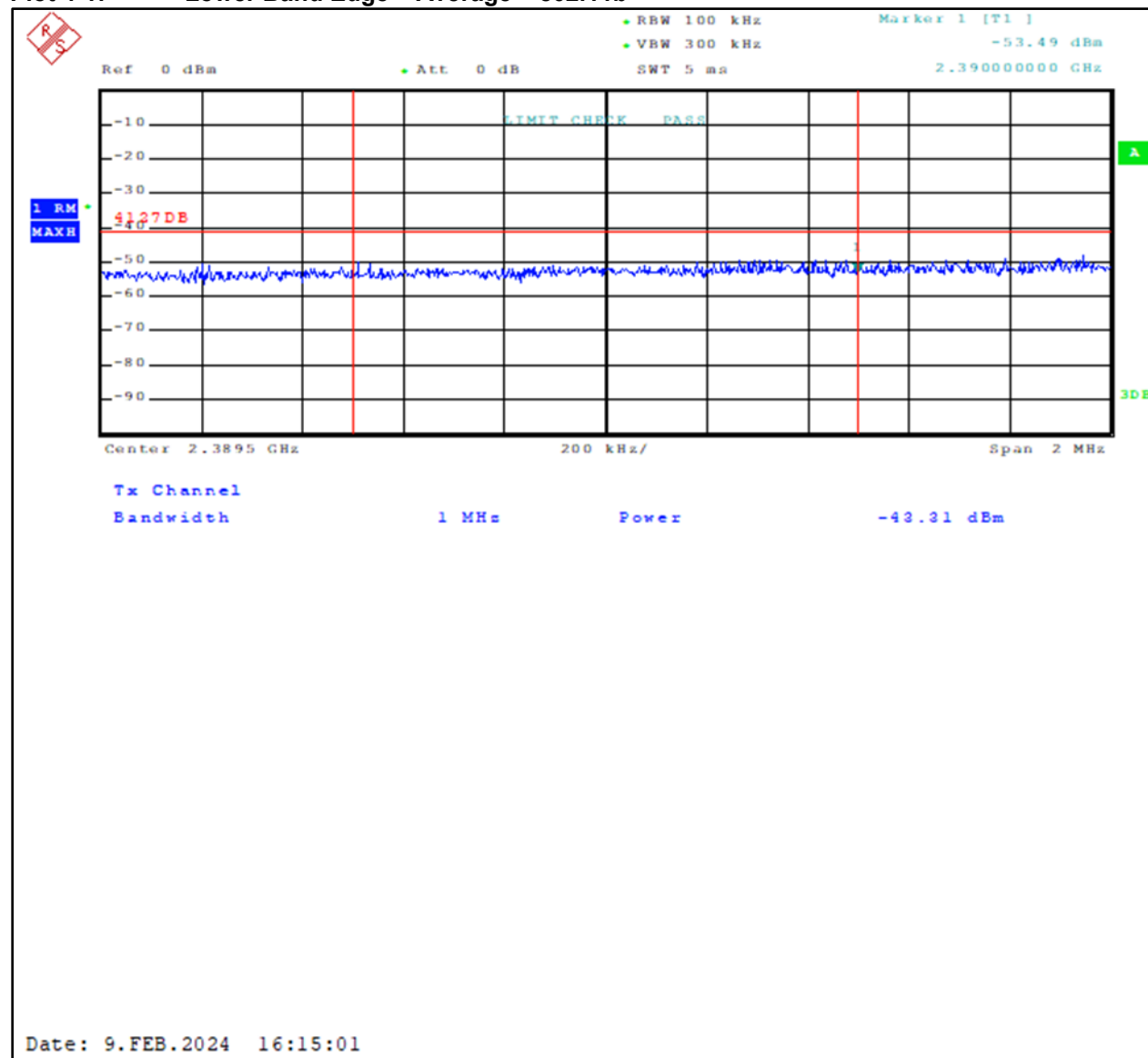
Plot 4-1: Lower Band Edge – Average – 802.11b
