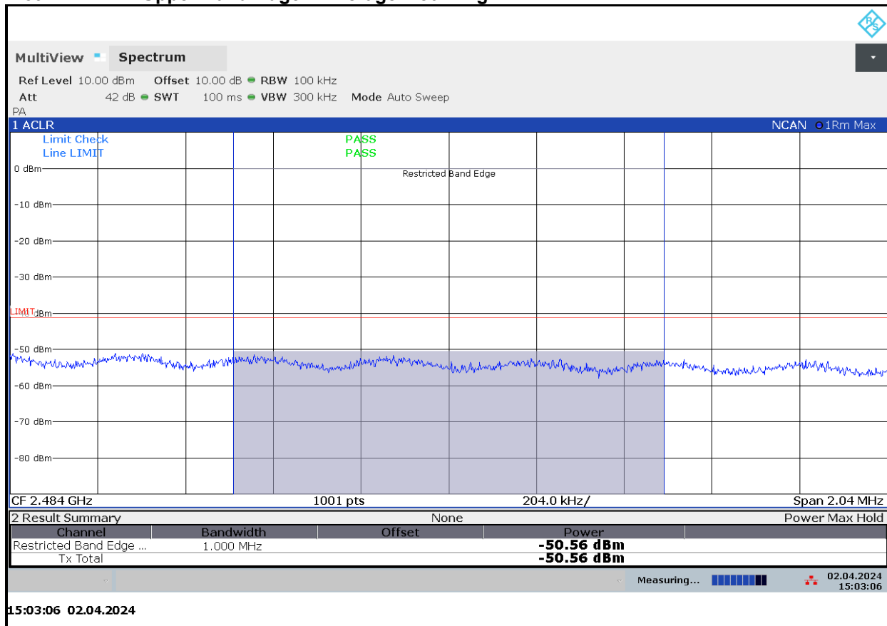
Plot 4-7: Upper Band Edge – Average – 802.11g
