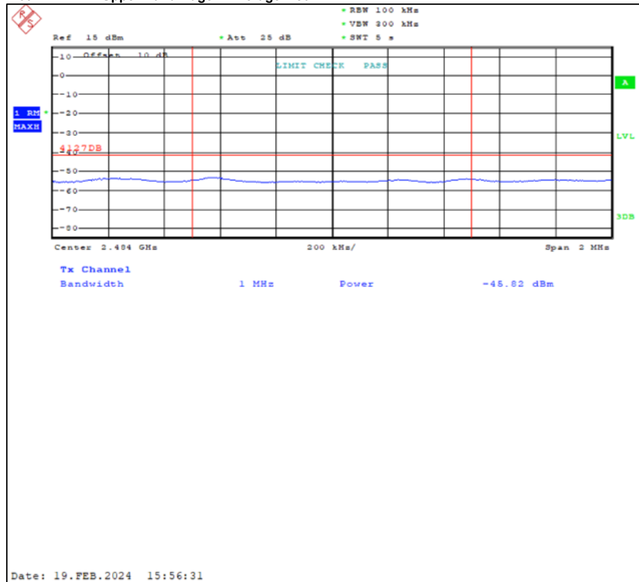
Plot 4-11: Upper Band Edge – Average – 802.11n
