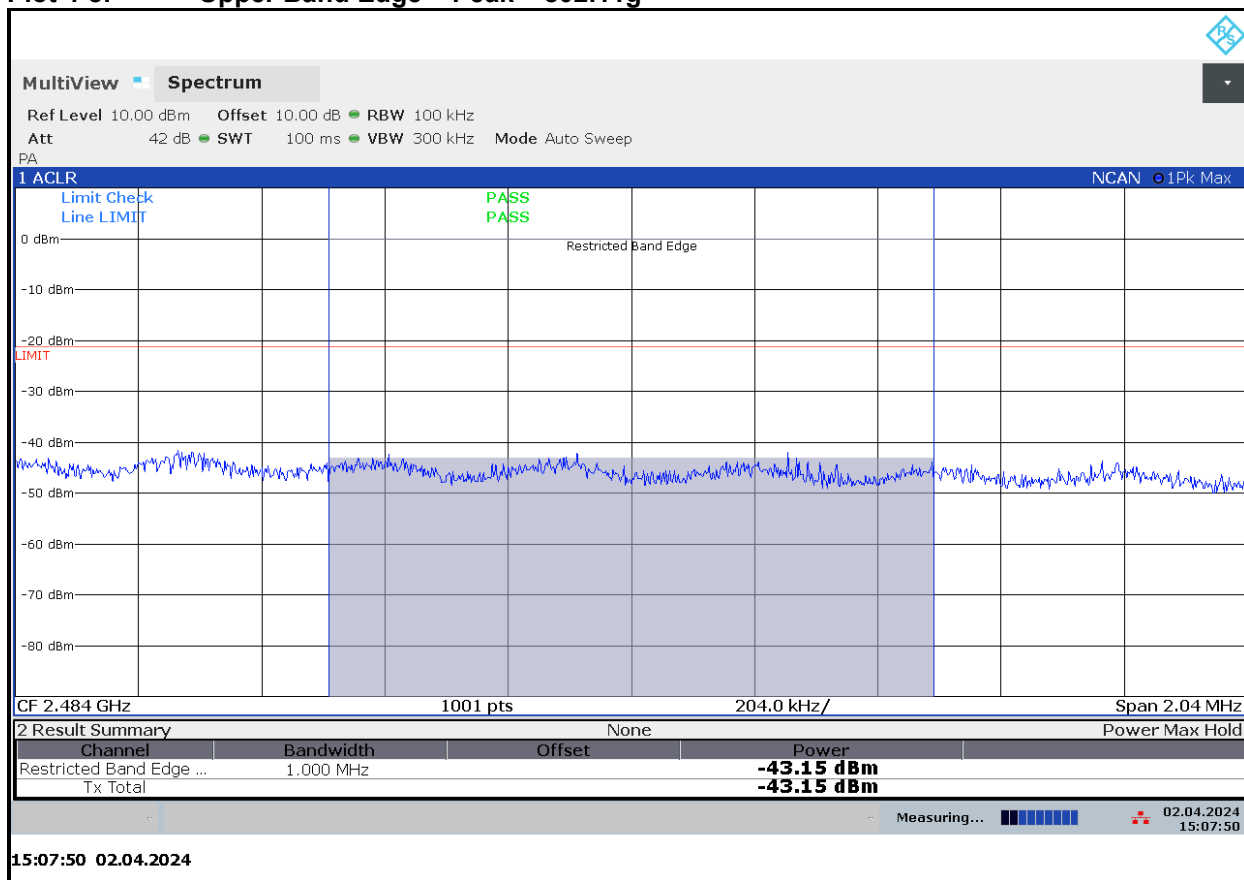
Plot 4-8: Upper Band Edge – Peak – 802.11g
