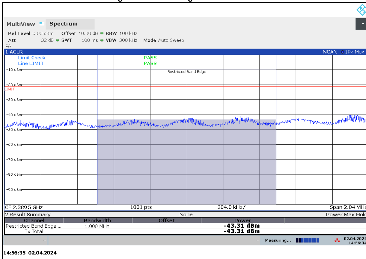
Plot 4-6: Lower Band Edge – Peak – 802.11g
