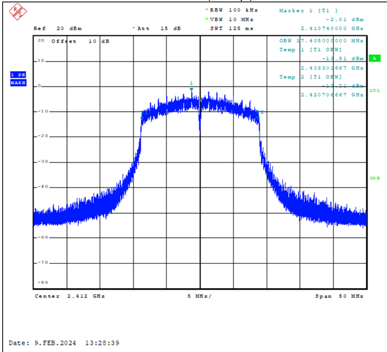
Plot 6-4: 99% Bandwidth – 2412 MHz – 802.11b (11.0 Mbps)
