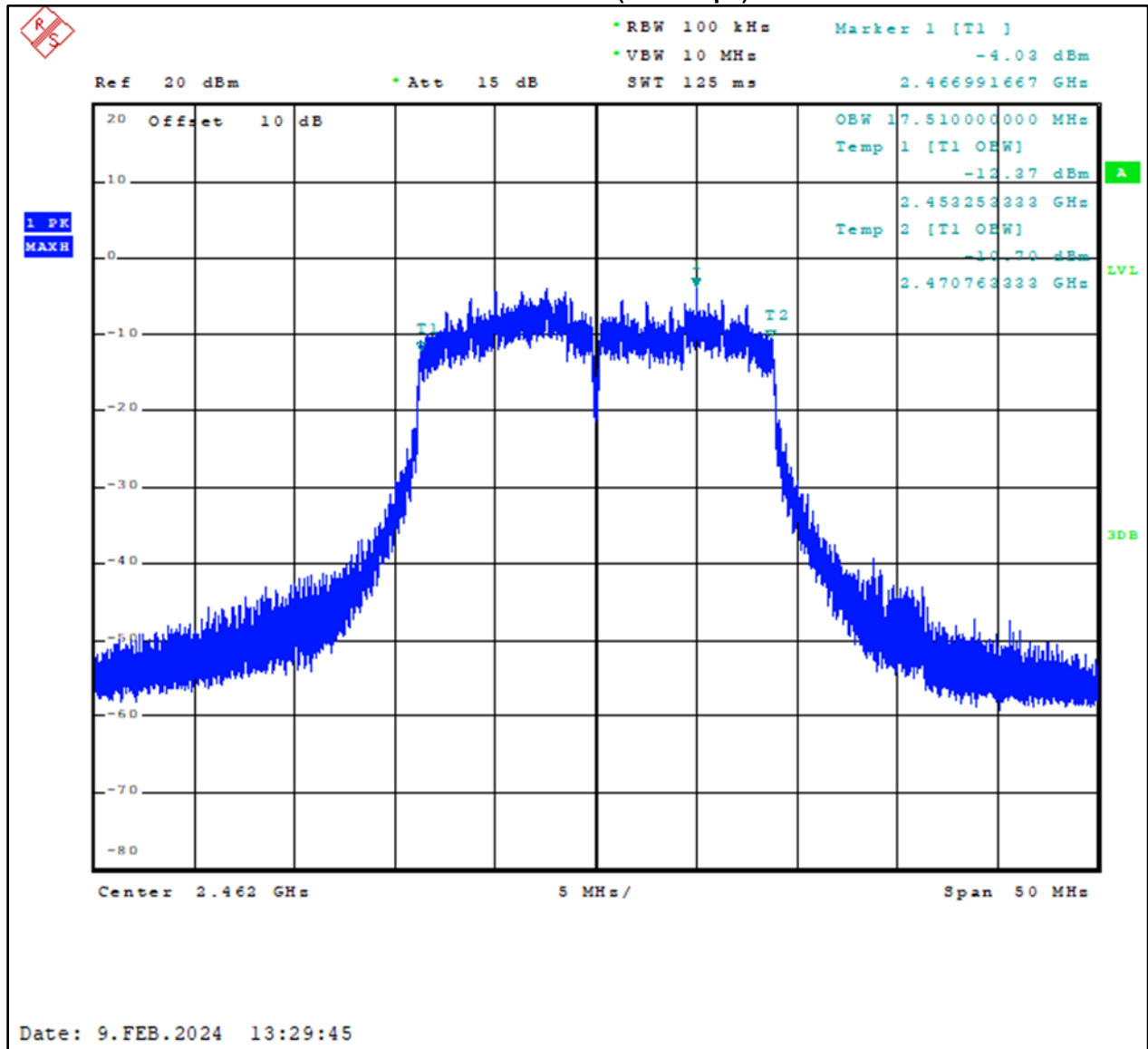
Plot 6-6: 99% Bandwidth – 2462 MHz – 802.11b (11.0 Mbps)
