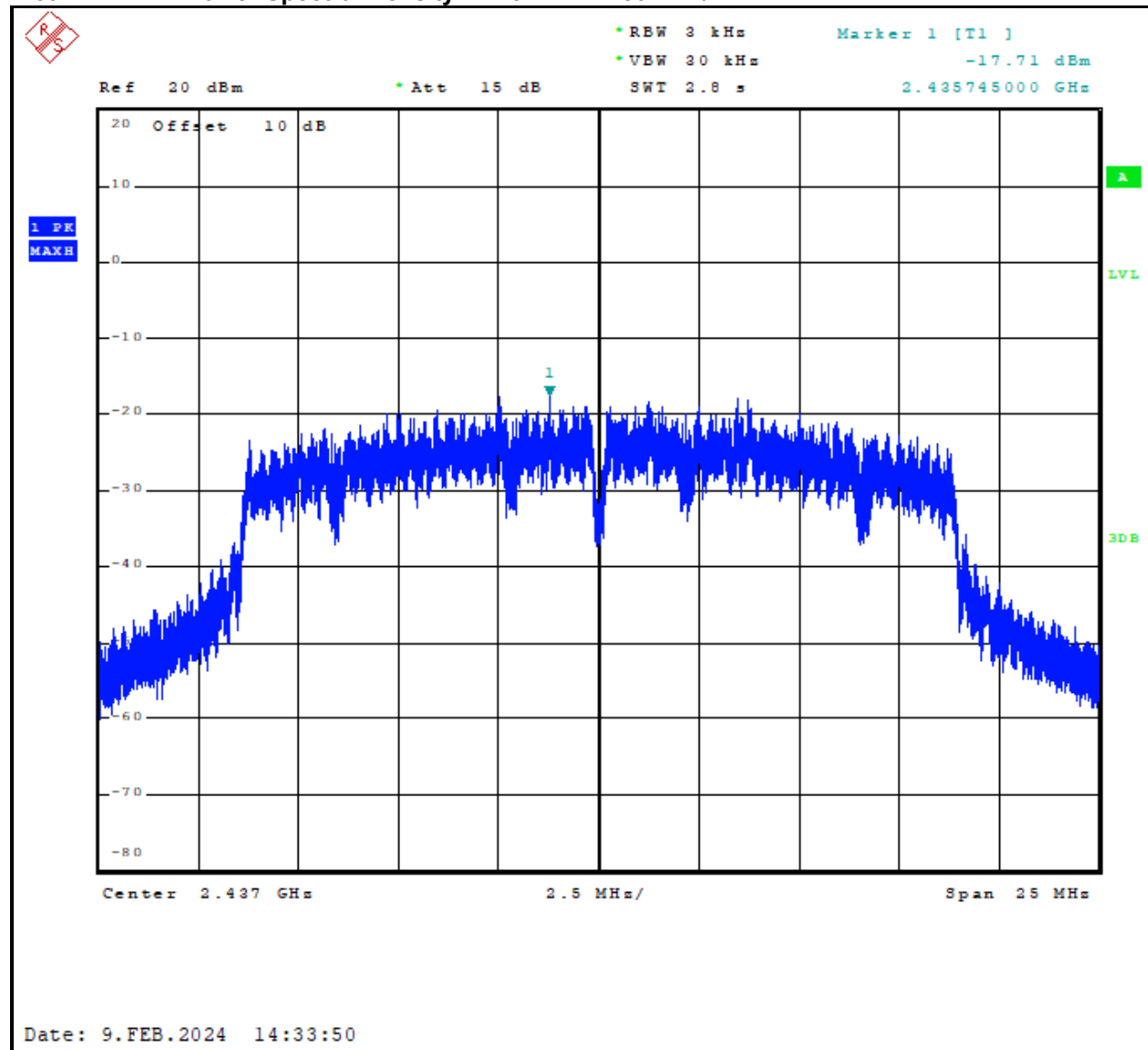
Plot 7-2: Power Spectral Density – 2437 MHz – 802.11b
