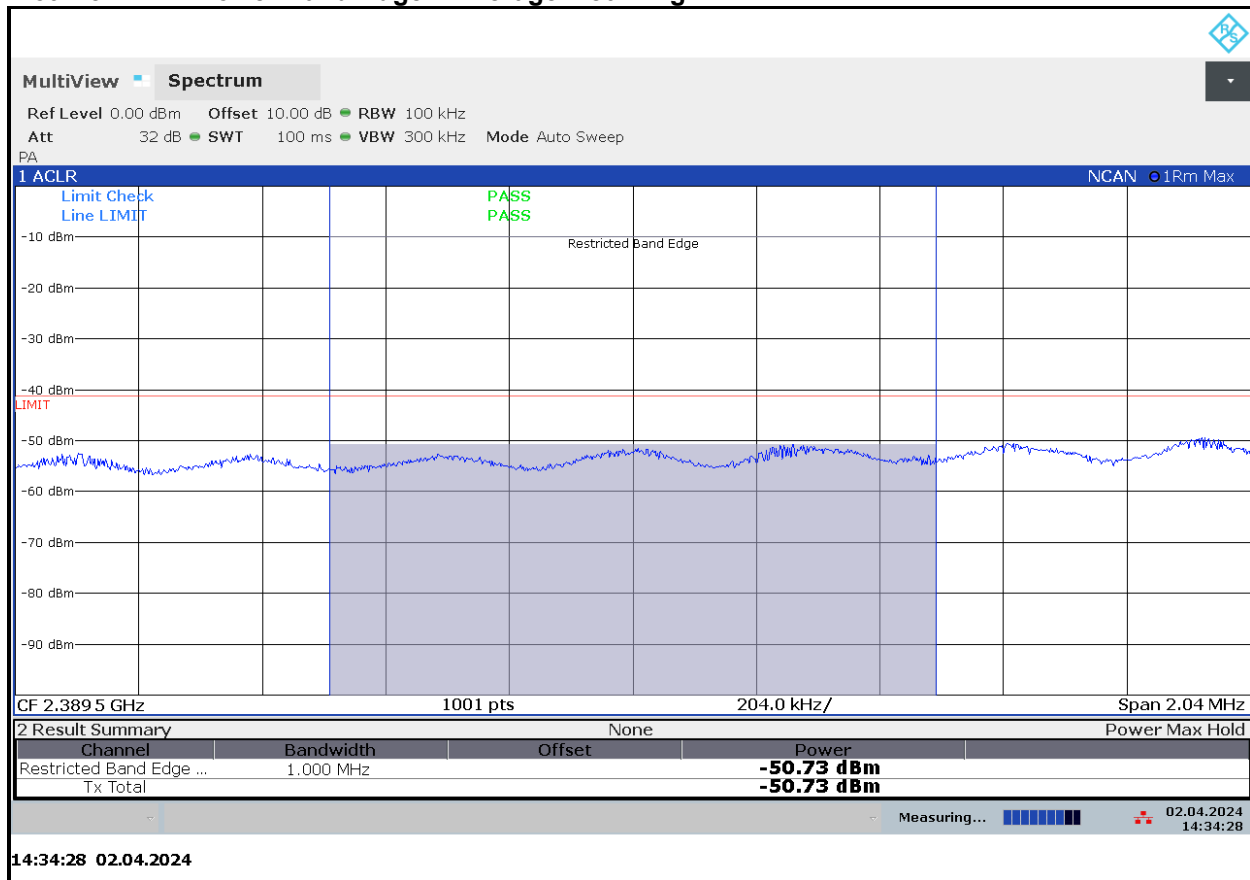
Plot 4-5: Lower Band Edge – Average – 802.11g
