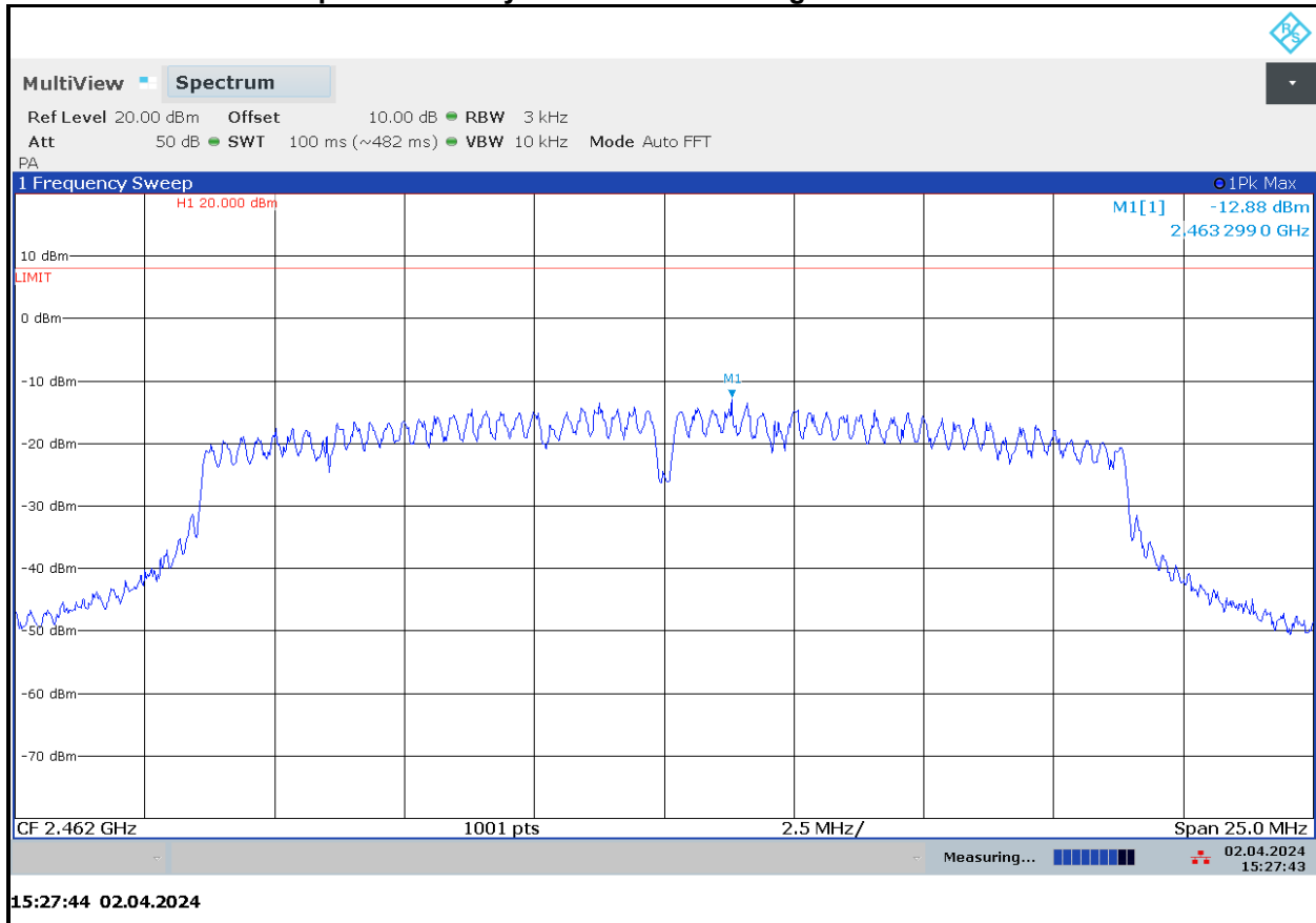
Plot 7-6: Power Spectral Density – 2462 MHz - 802.11g
