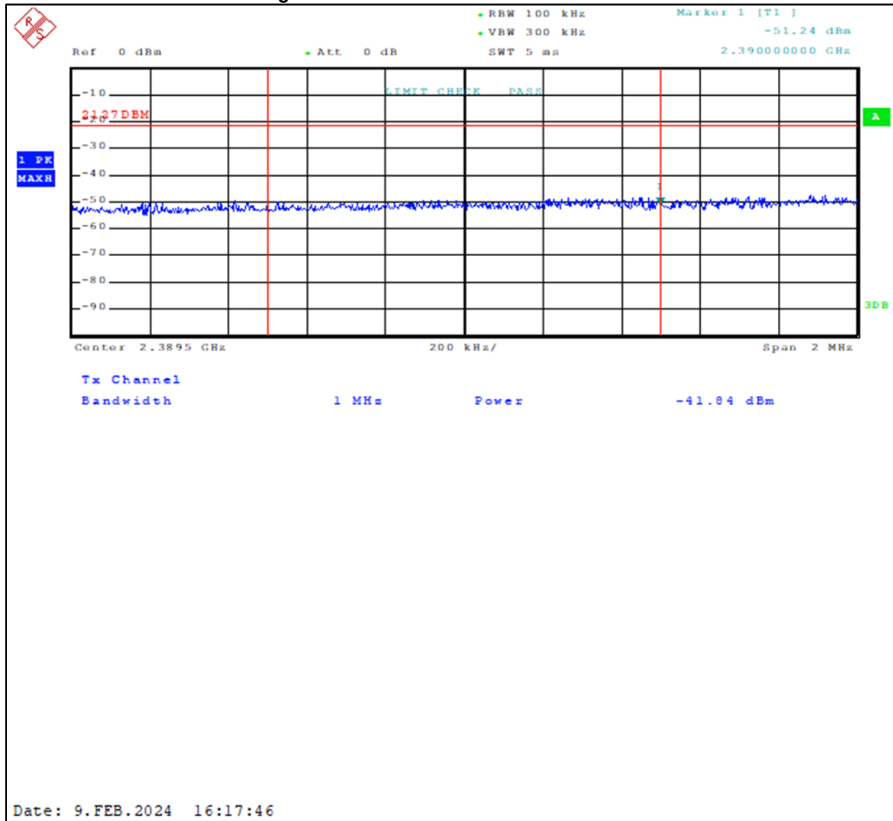
Plot 4-2: Lower Band Edge – Peak – 802.11b
