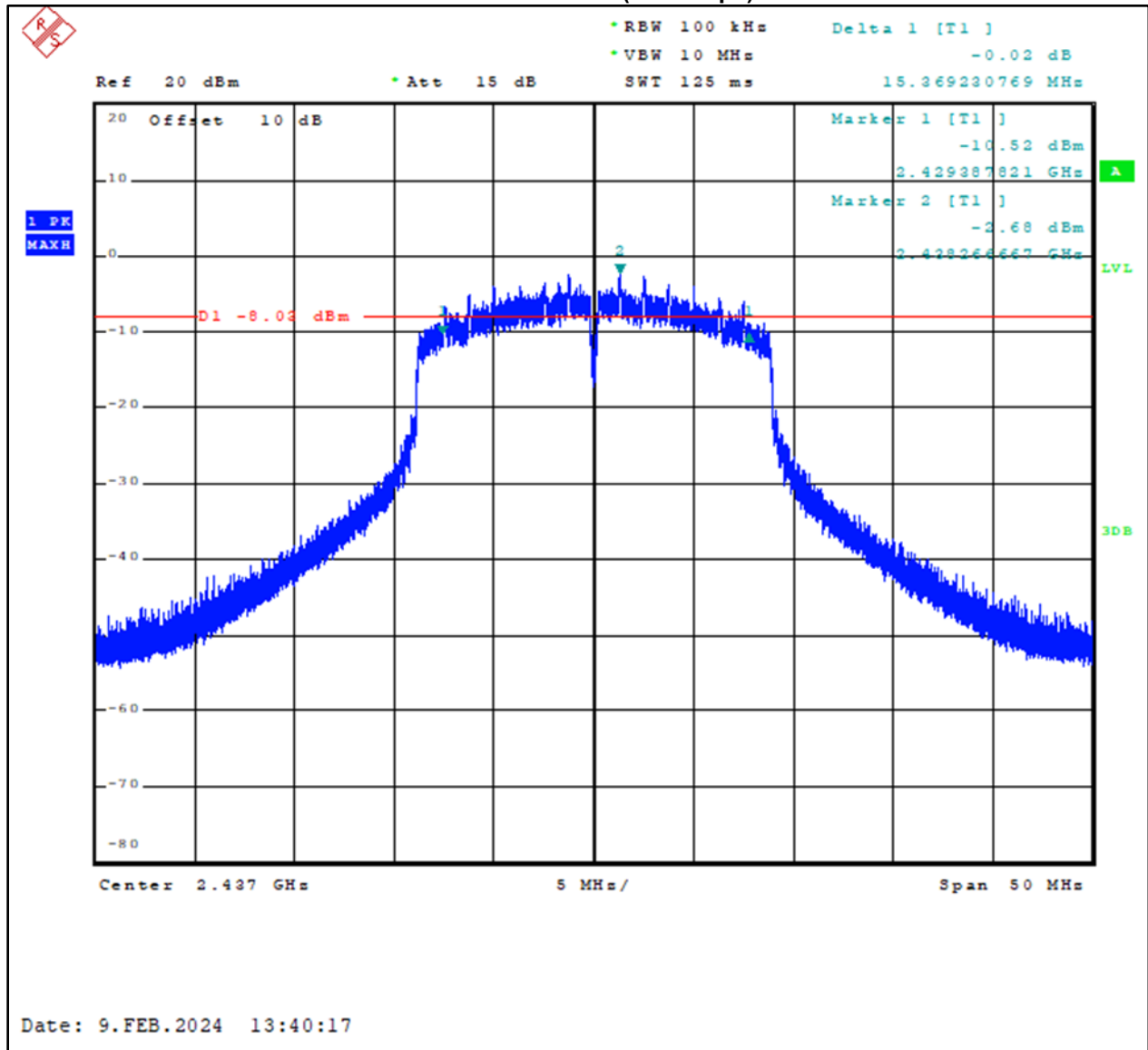
Plot 6-2: 6 dB Bandwidth – 2437 MHz – 802.11b (11.0 Mbps)
