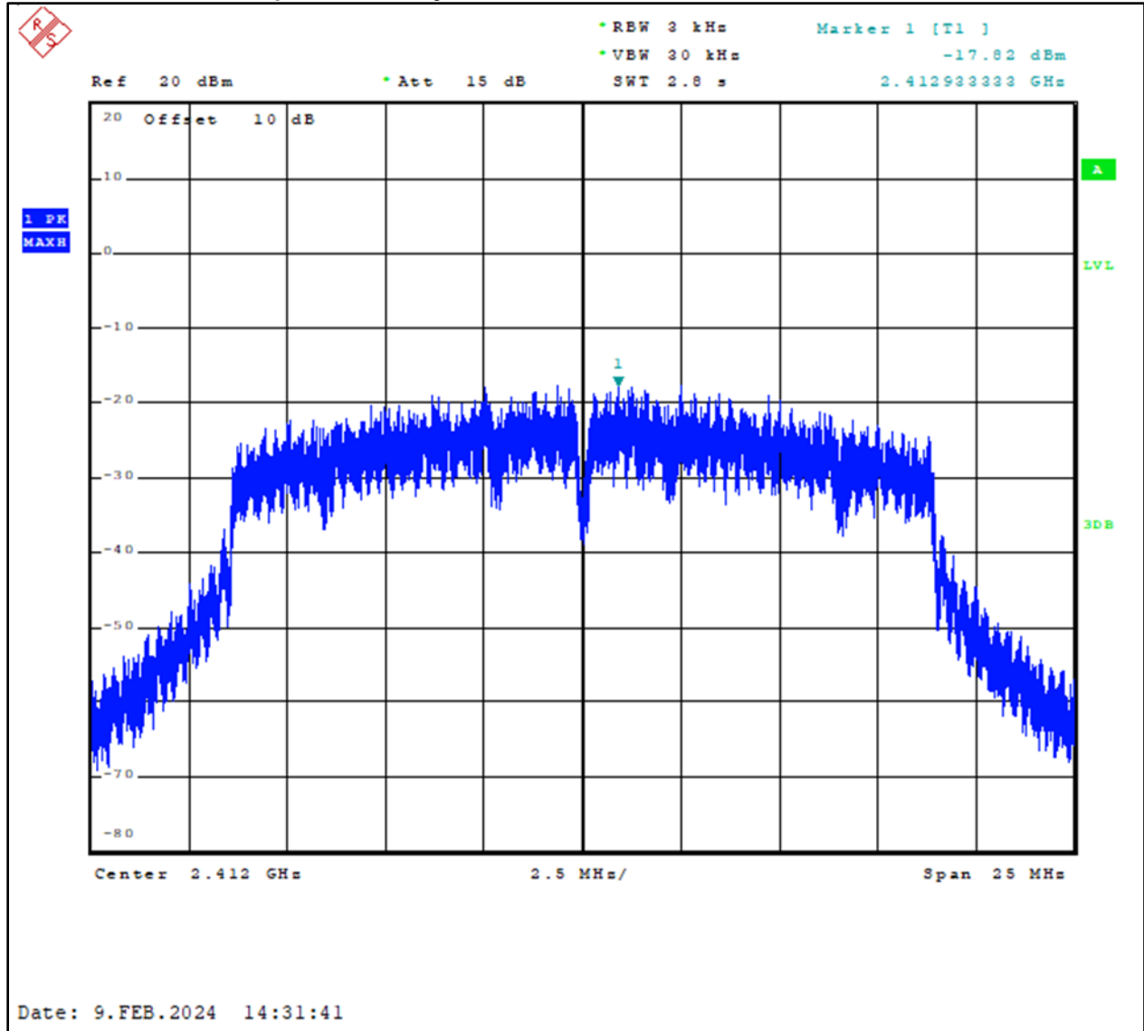
Plot 7-1: Power Spectral Density – 2412 MHz – 802.11b
