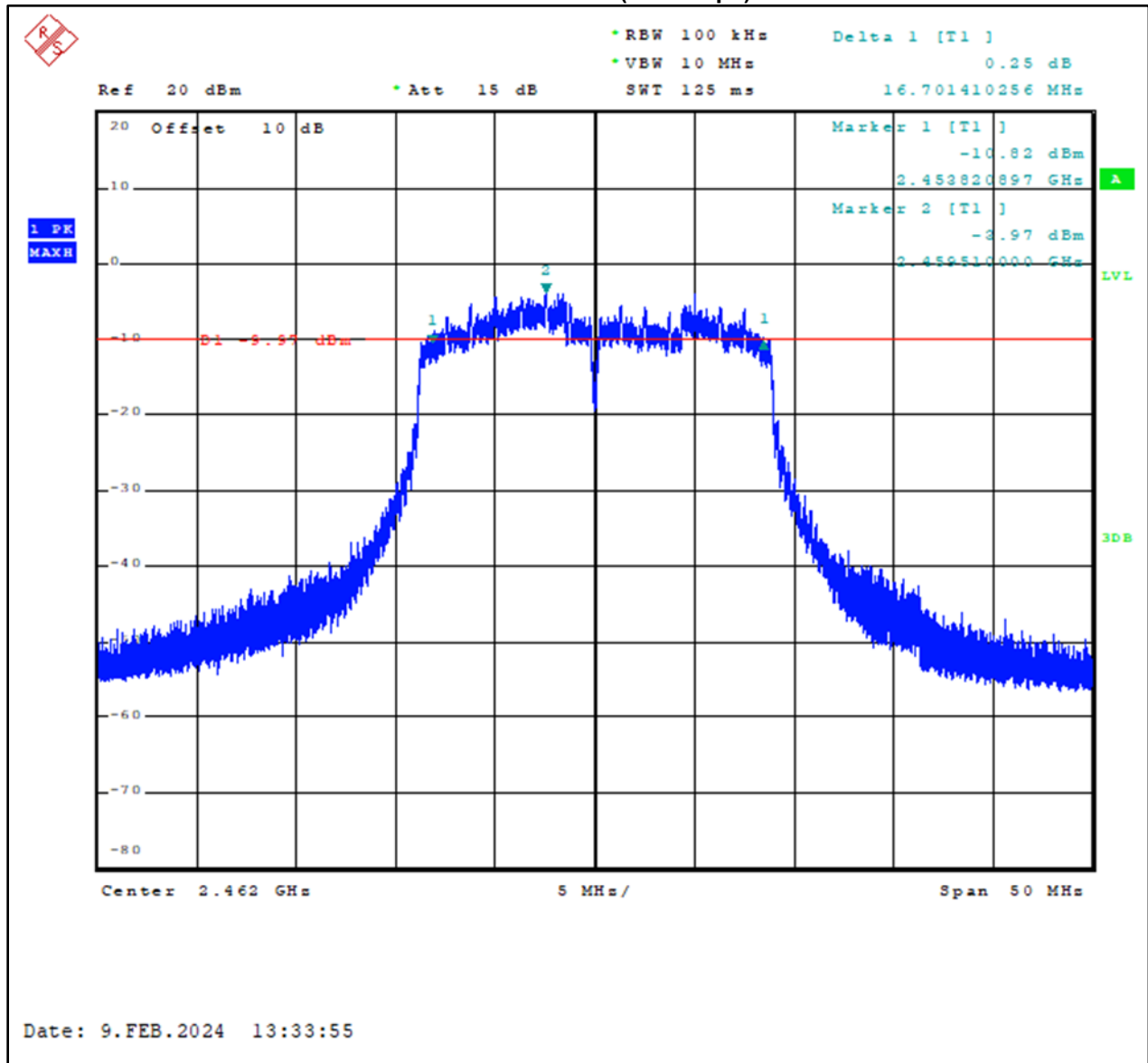
Plot 6-3: 6 dB Bandwidth – 2462 MHz – 802.11b (11.0 Mbps)
