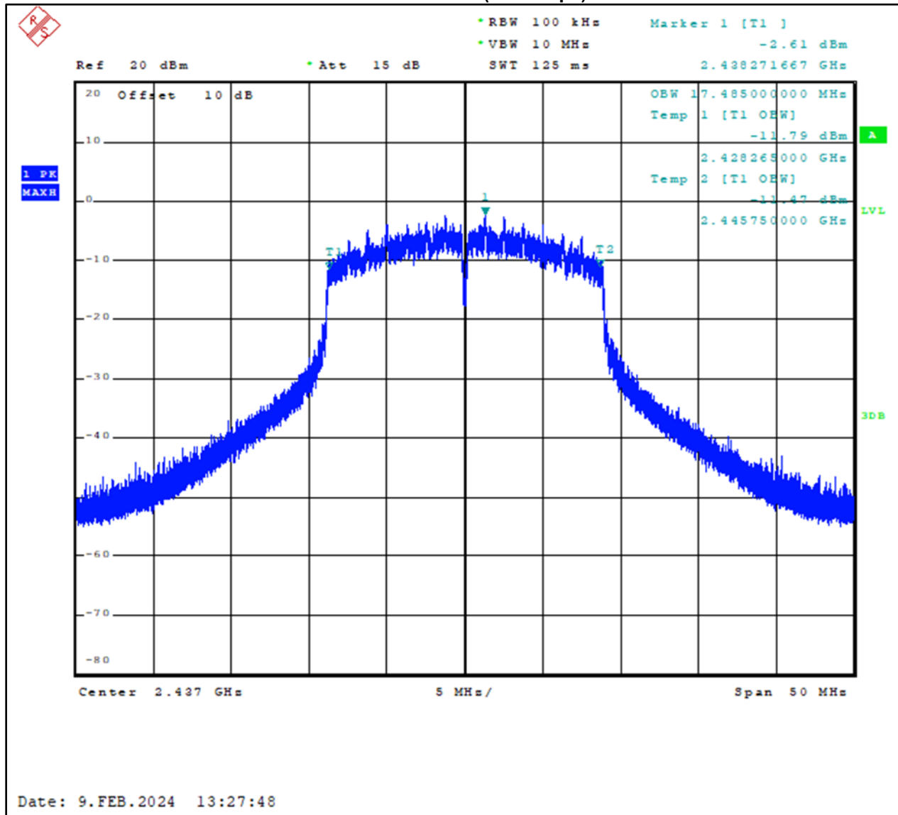
Plot 6-5: 99% Bandwidth – 2437 MHz – 802.11b (11.0 Mbps)
