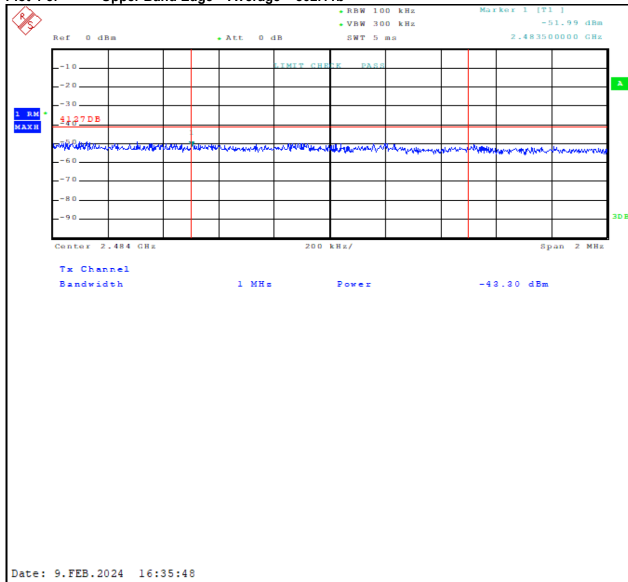
Plot 4-3: Upper Band Edge – Average – 802.11b
