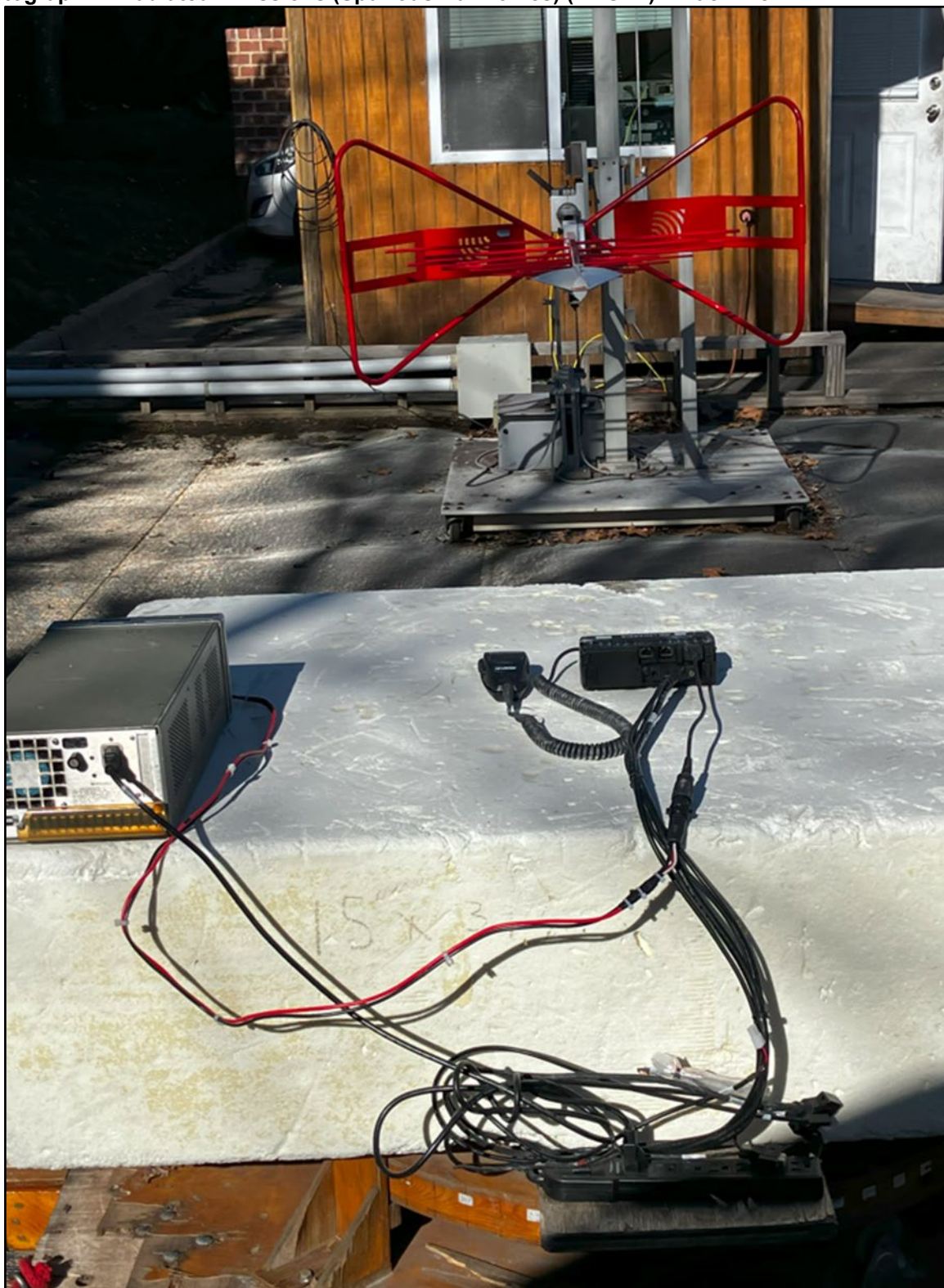
Photograph 2: Radiated Emissions (Spurious/Harmonics) (<1 GHz) – Back View
