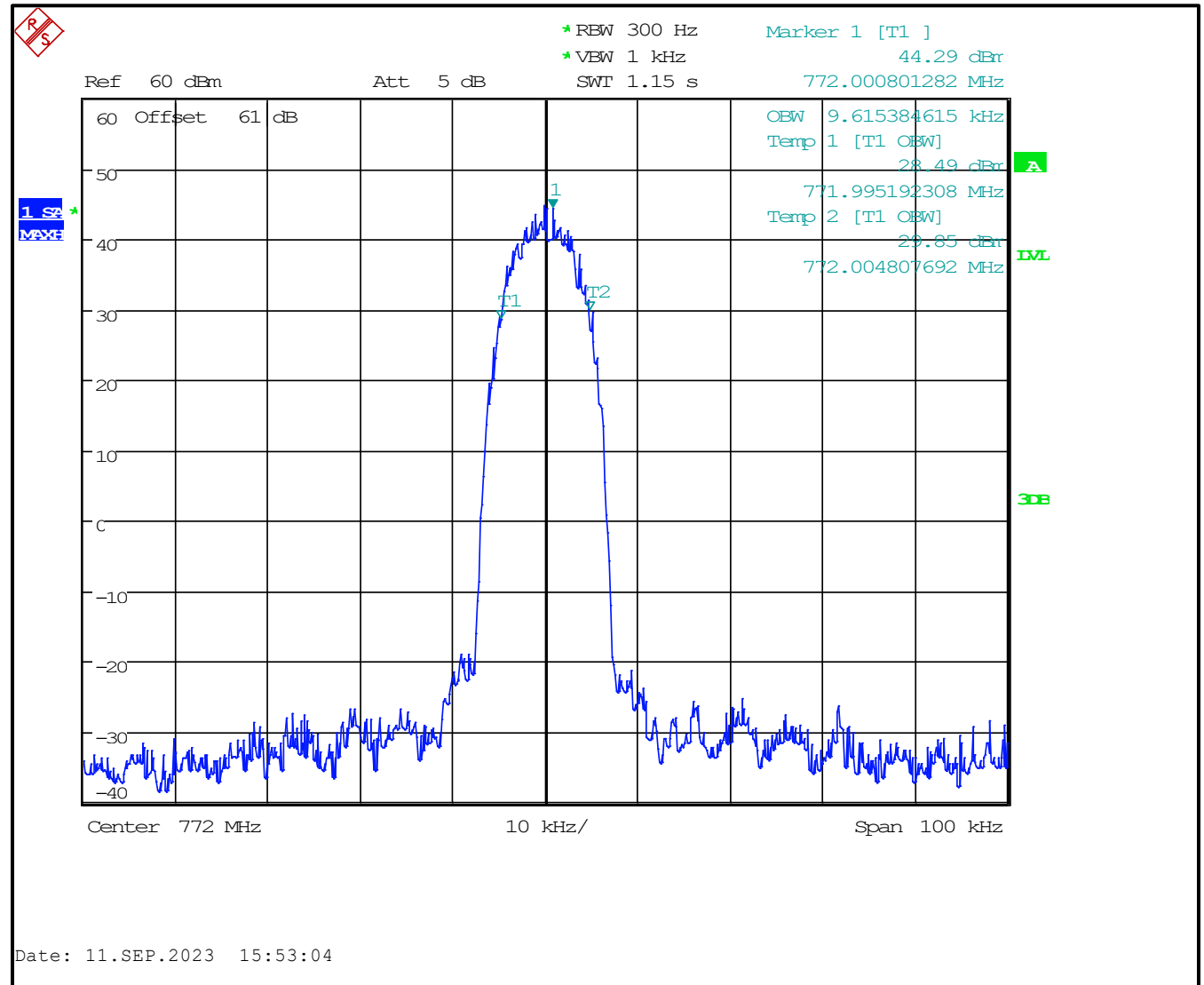
Plot 8-8: 99% BW, 772.000000 MHz, HDQPSK
