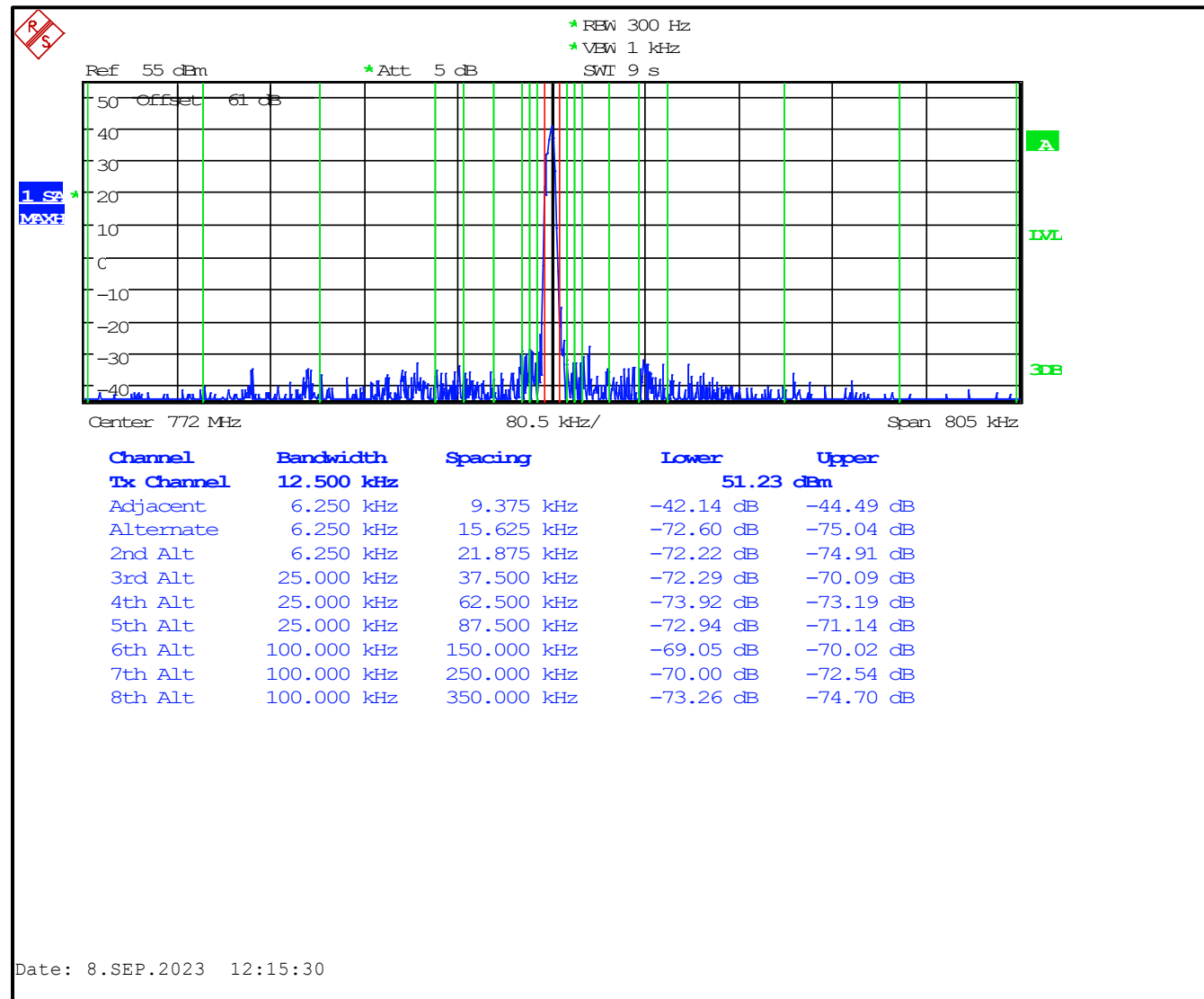
Plot 6-8: Adjacent Channel Power - 772.000000 MHz; HDQPSK Mode (9.375 kHz - 350 kHz)
