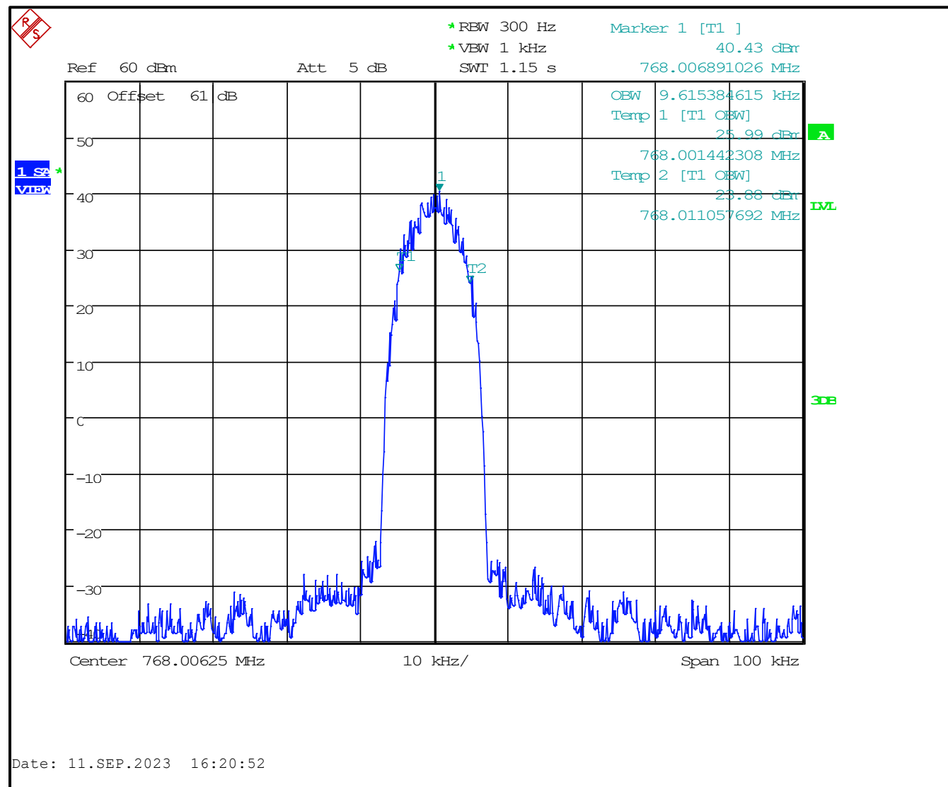
Plot 8-2: 99% BW, 768.00625 MHz, WCQPSK
