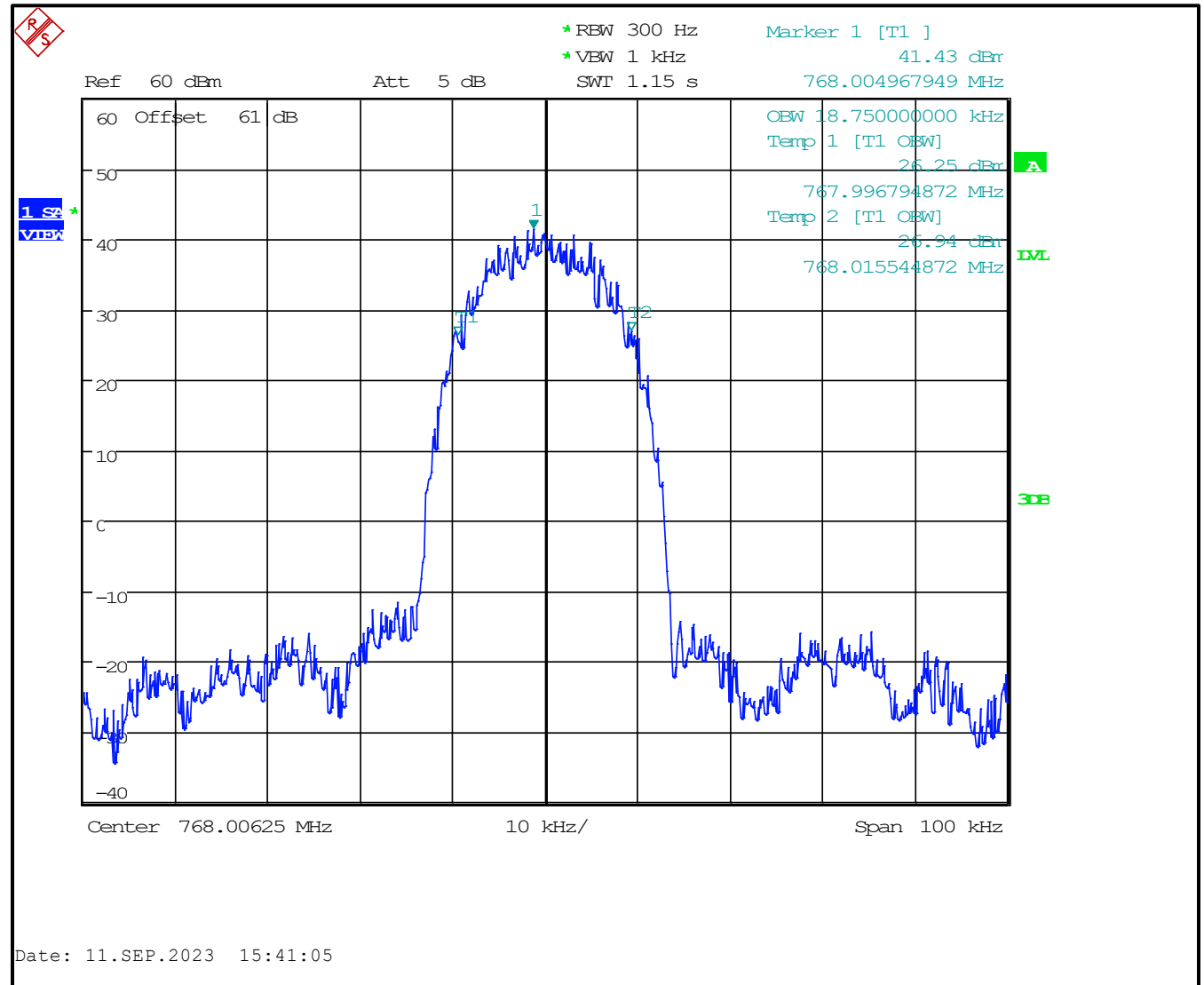
Plot 8-4: 99% BW, 768.00625 MHz, HVD-SMR
