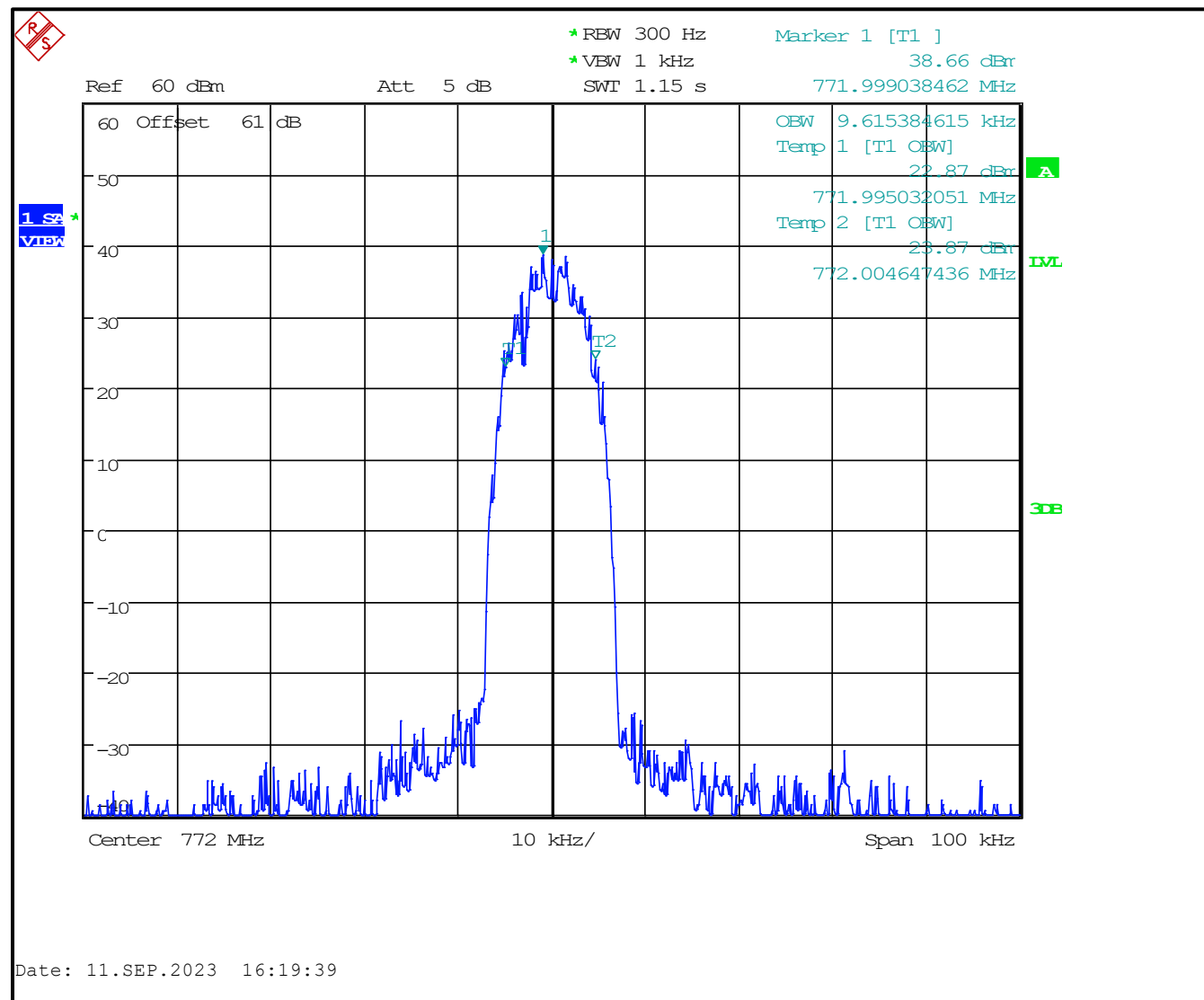
Plot 8-7: 99% BW, 772.000000 MHz, WCQPSK
