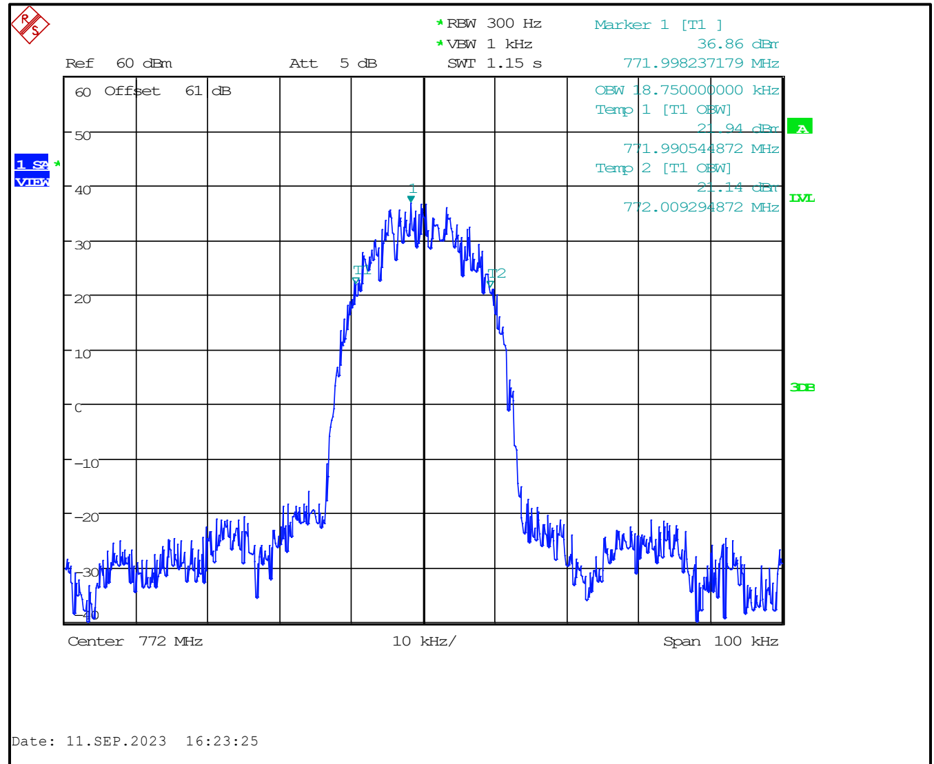
Plot 8-9: 99% BW, 772.000000 MHz, HVD-SMR
