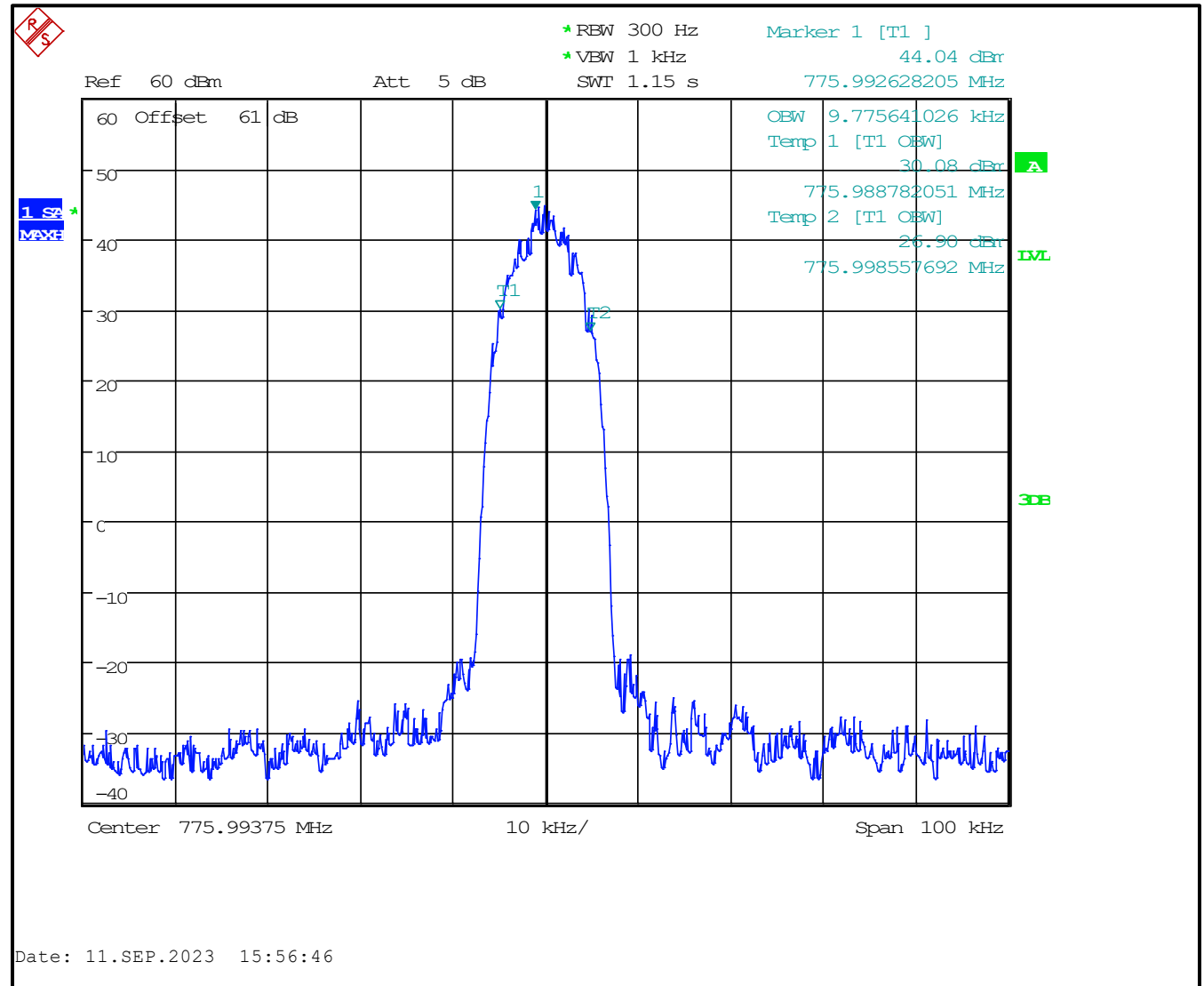
Plot 8-13: 99% BW, 775.993750 MHz, HDQPSK
