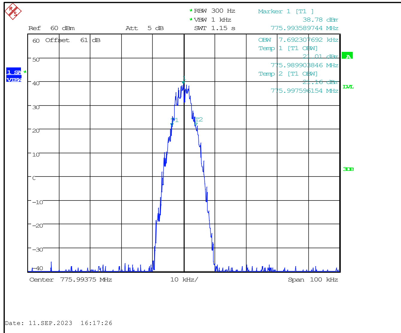
Plot 8-11: 99% BW, 775.993750 MHz, C4FM
