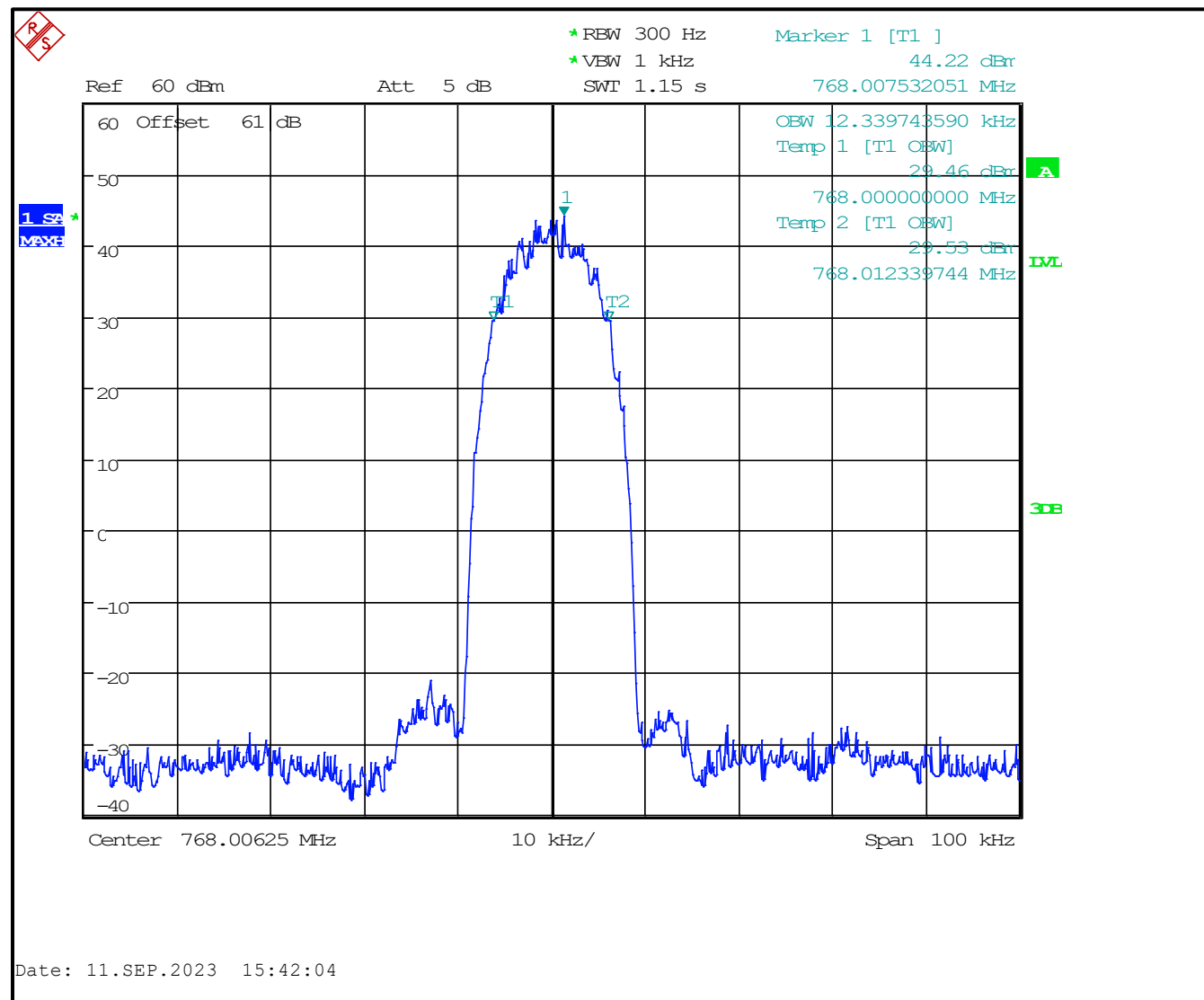
Plot 8-5: 99% BW, 768.00625 MHz, HVD-NPSPAC
